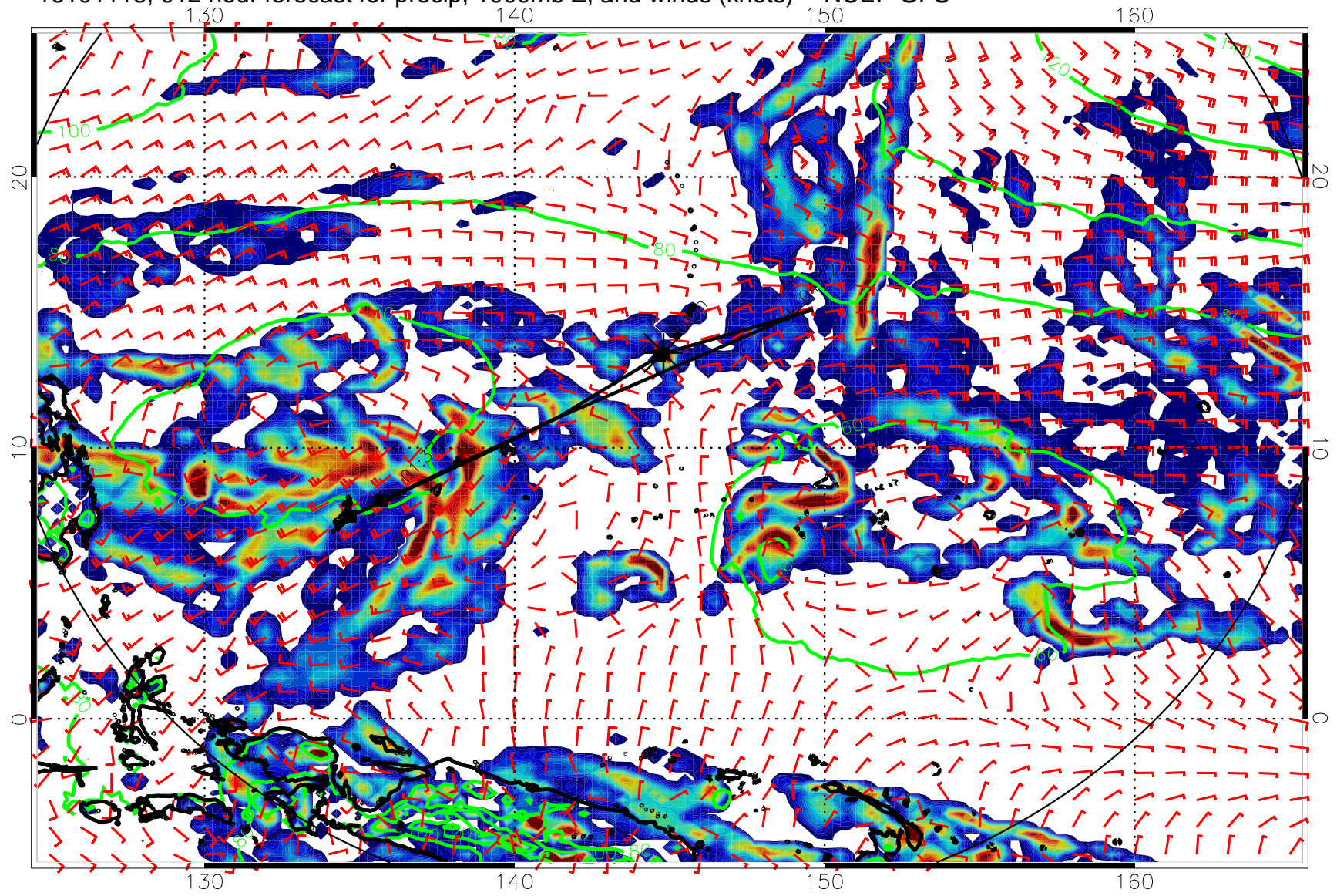
16101118, 012 hour forecast for precip, 1000mb Z, and winds (knots) -- NCEP GFS
