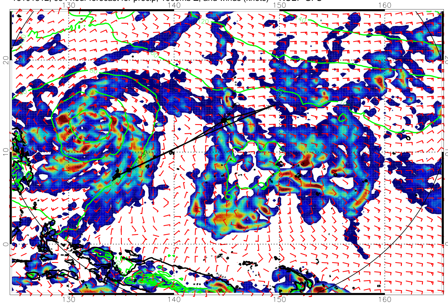
16101312, 054 hour forecast for precip, 1000mb Z, and winds (knots) -- NCEP GFS
