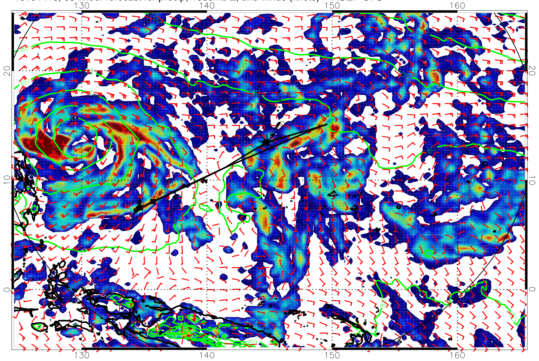
16101418, 084 hour forecast for precip, 1000mb Z, and winds (knots) -- NCEP GFS
