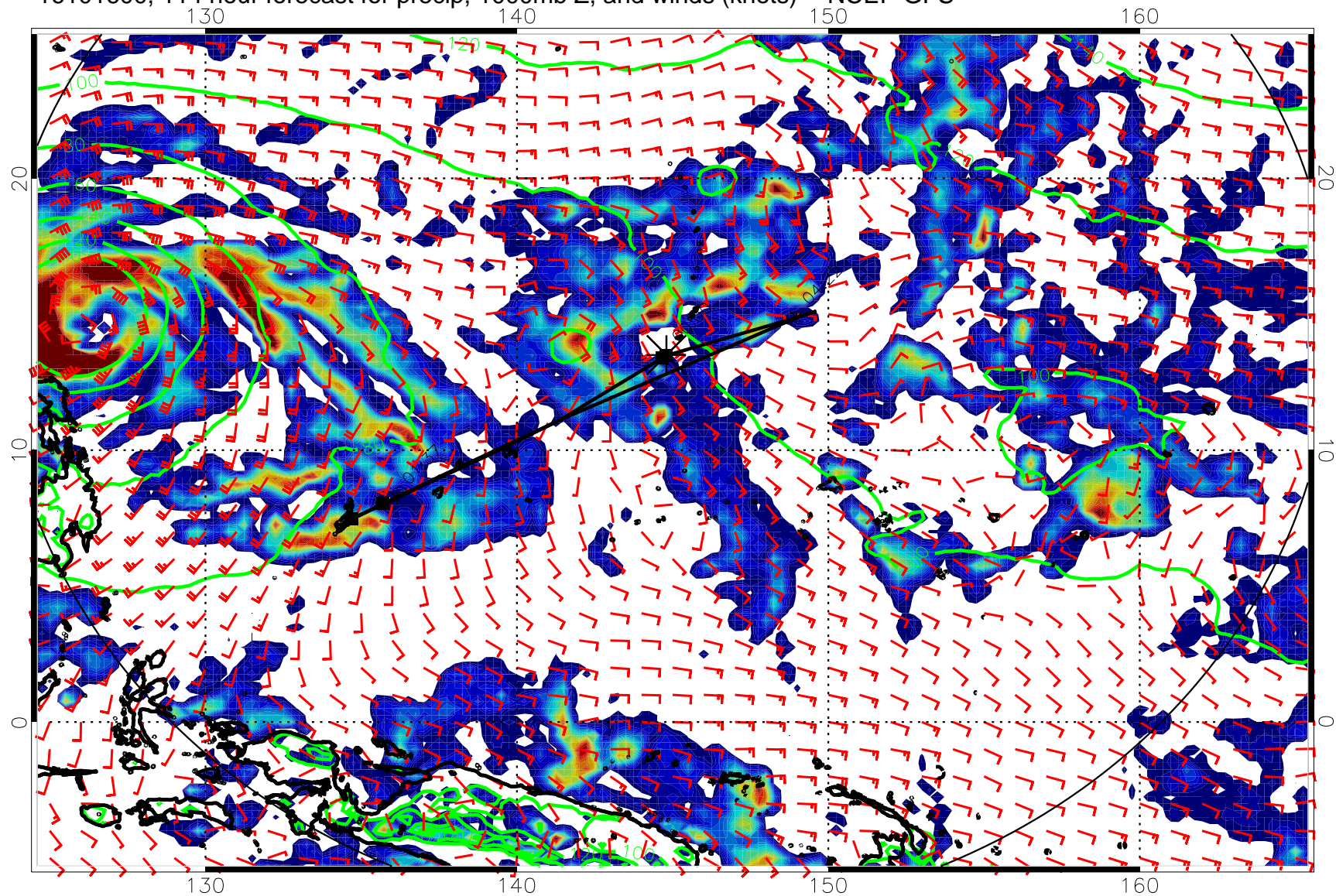
16101600, 114 hour forecast for precip, 1000mb Z, and winds (knots) -- NCEP GFS
