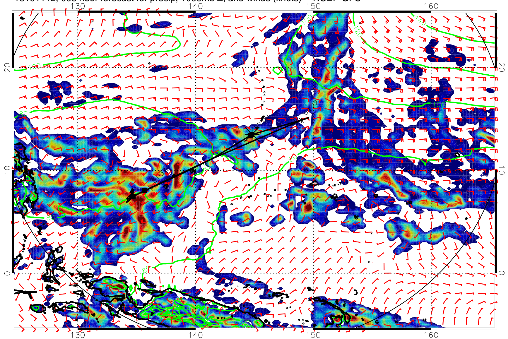
16101112, 006 hour forecast for precip, 1000mb Z, and winds (knots) -- NCEP GFS
