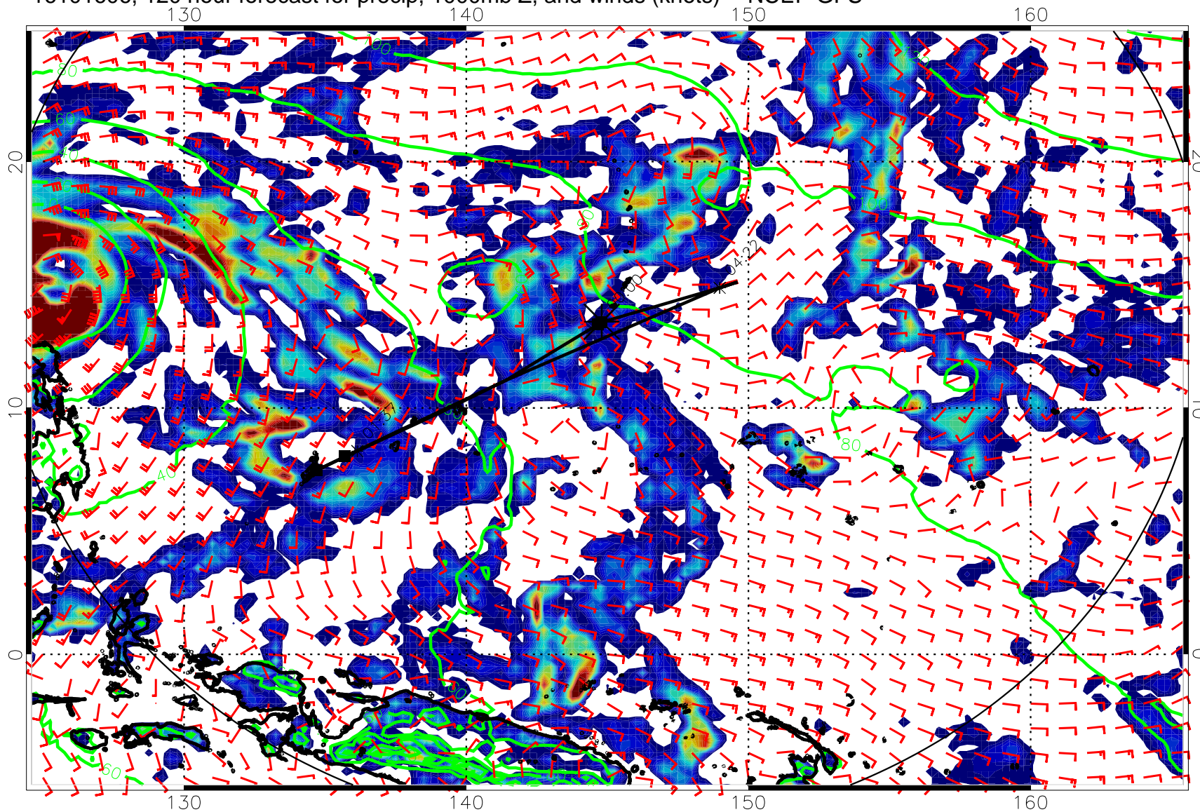
16101606, 120 hour forecast for precip, 1000mb Z, and winds (knots) -- NCEP GFS
