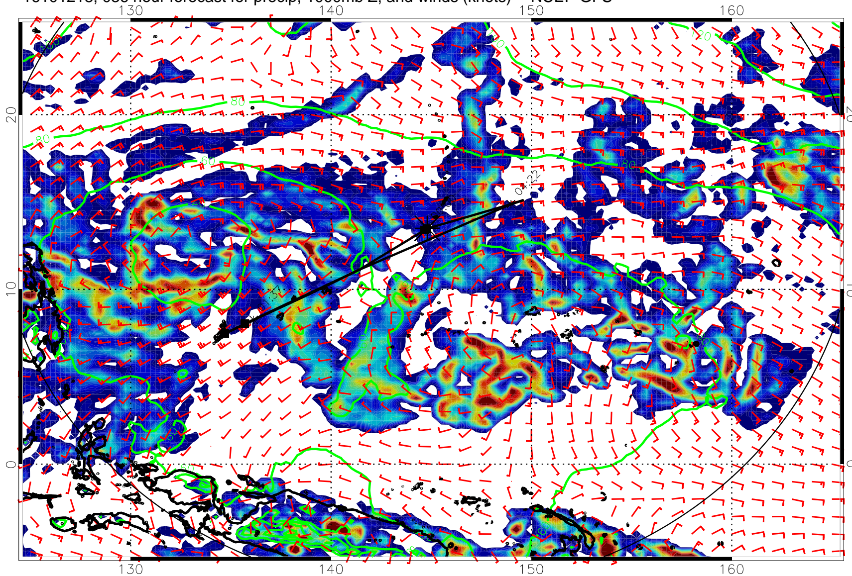
16101218, 036 hour forecast for precip, 1000mb Z, and winds (knots) -- NCEP GFS
