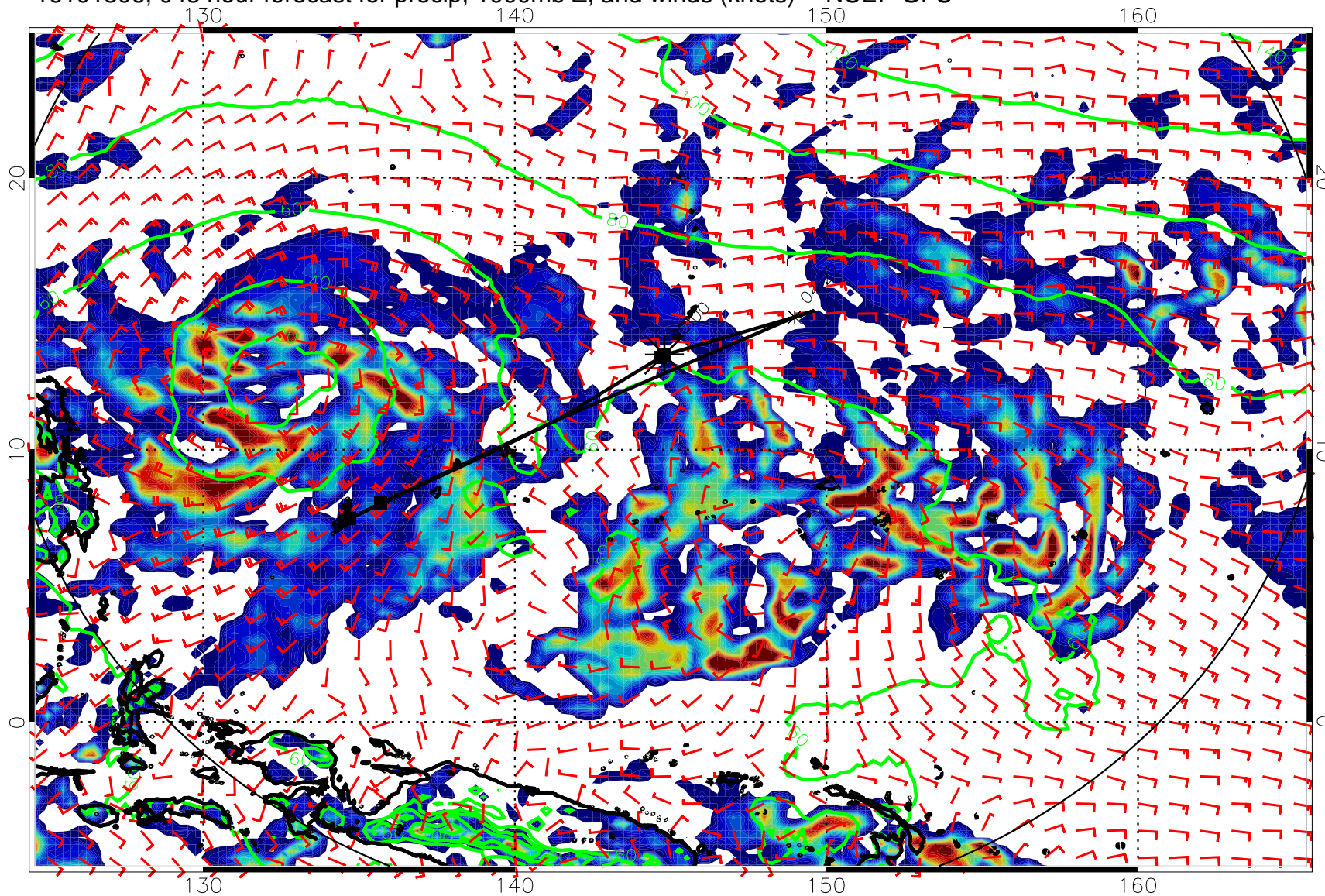
16101306, 048 hour forecast for precip, 1000mb Z, and winds (knots) -- NCEP GFS
