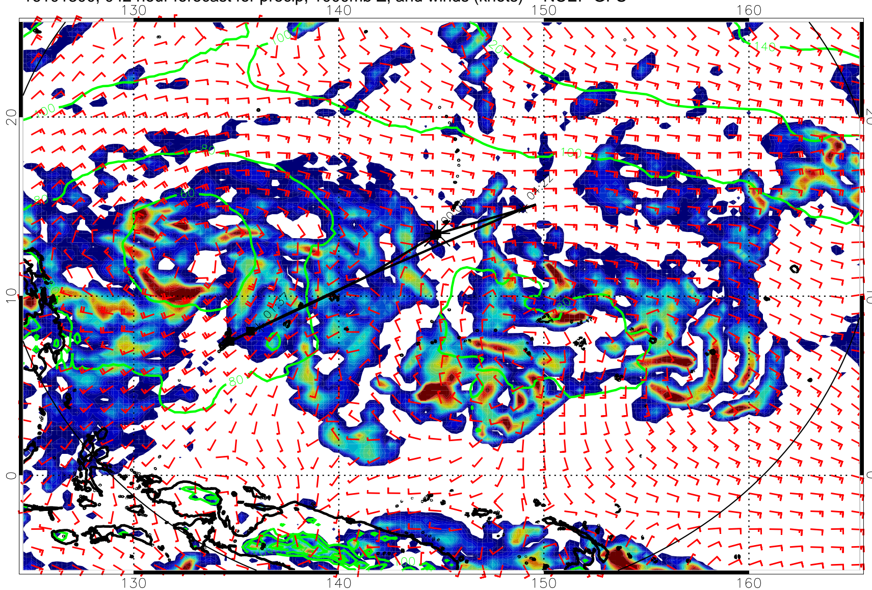
16101300, 042 hour forecast for precip, 1000mb Z, and winds (knots) -- NCEP GFS
