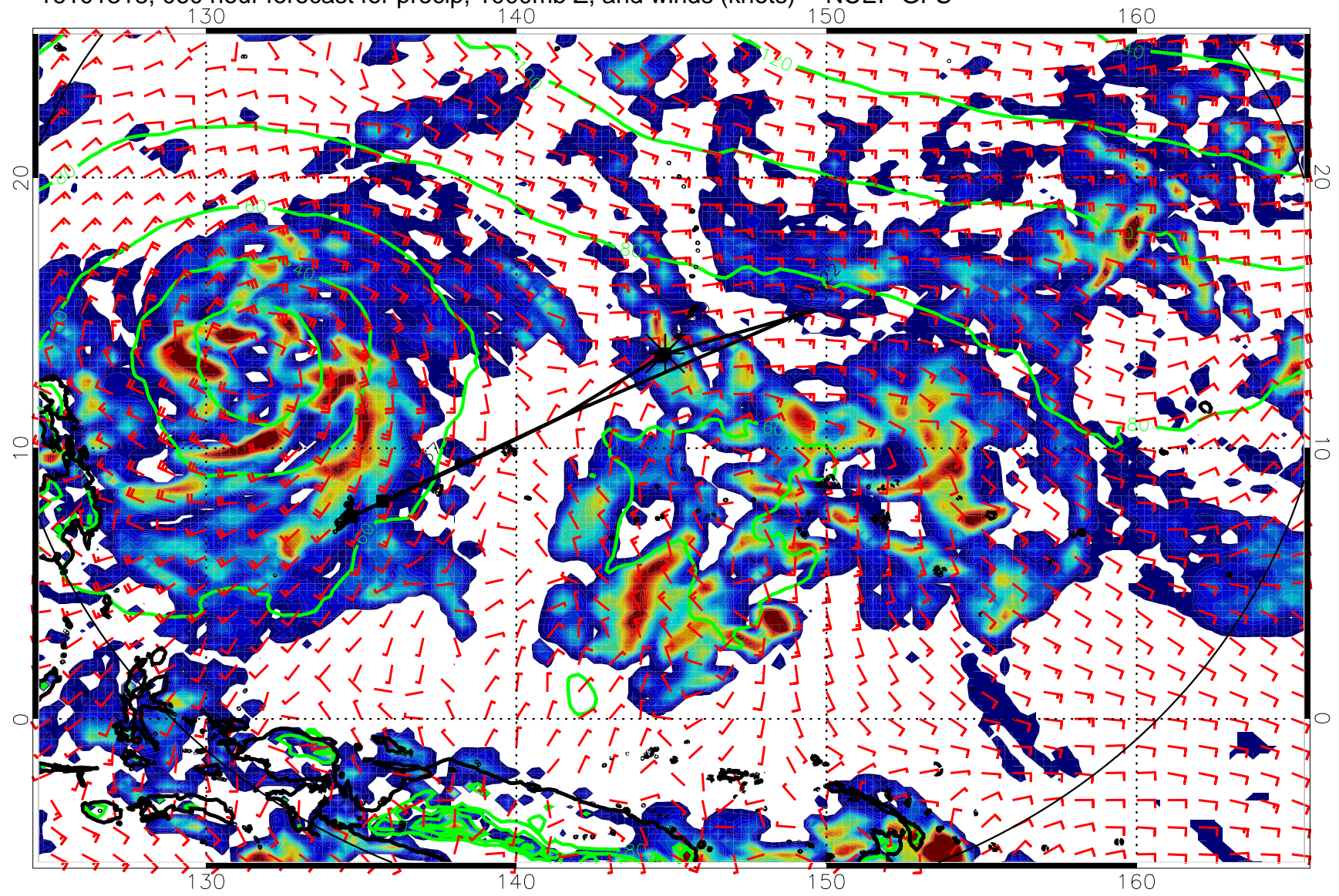
16101318, 060 hour forecast for precip, 1000mb Z, and winds (knots) -- NCEP GFS
