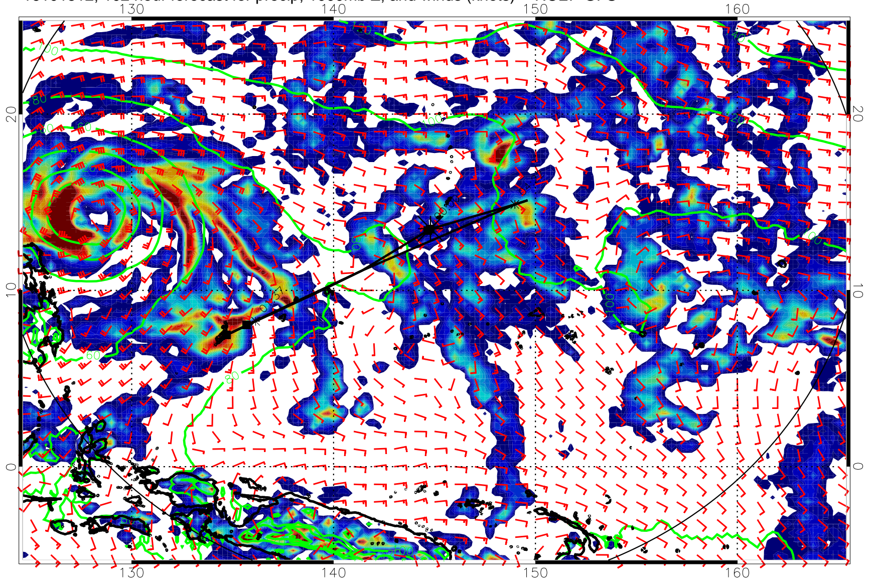
16101512, 102 hour forecast for precip, 1000mb Z, and winds (knots) -- NCEP GFS
