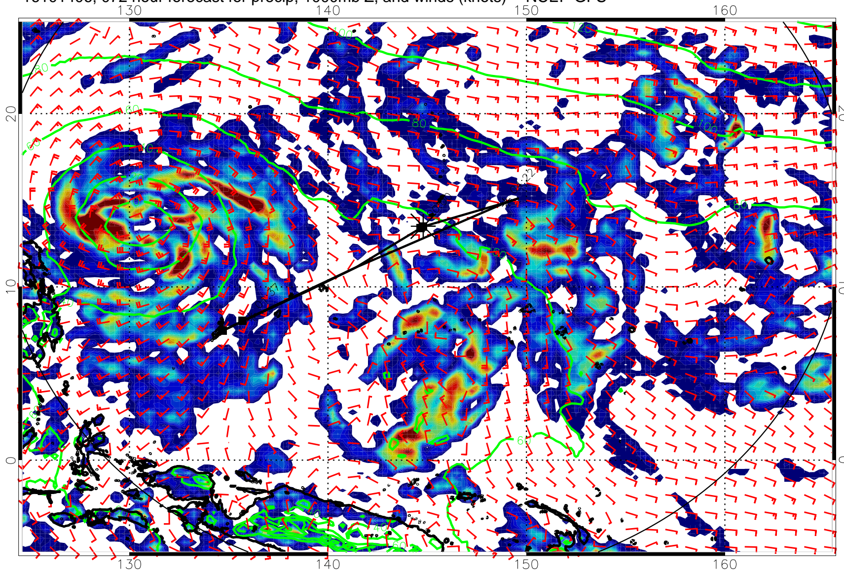
16101406, 072 hour forecast for precip, 1000mb Z, and winds (knots) -- NCEP GFS
