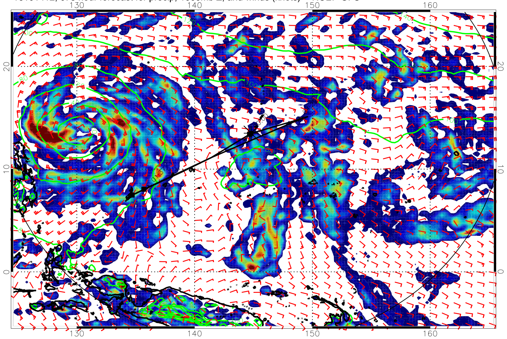
16101412, 078 hour forecast for precip, 1000mb Z, and winds (knots) -- NCEP GFS
