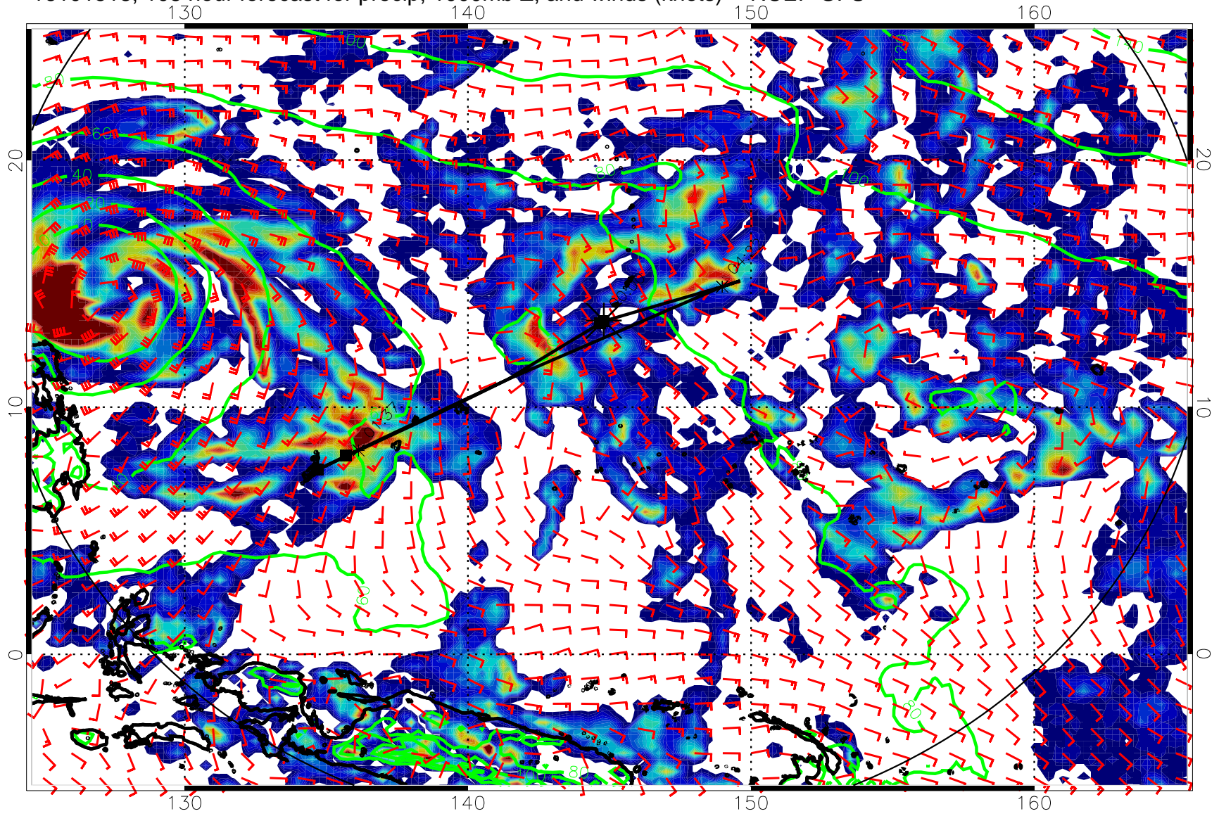
16101518, 108 hour forecast for precip, 1000mb Z, and winds (knots) -- NCEP GFS
