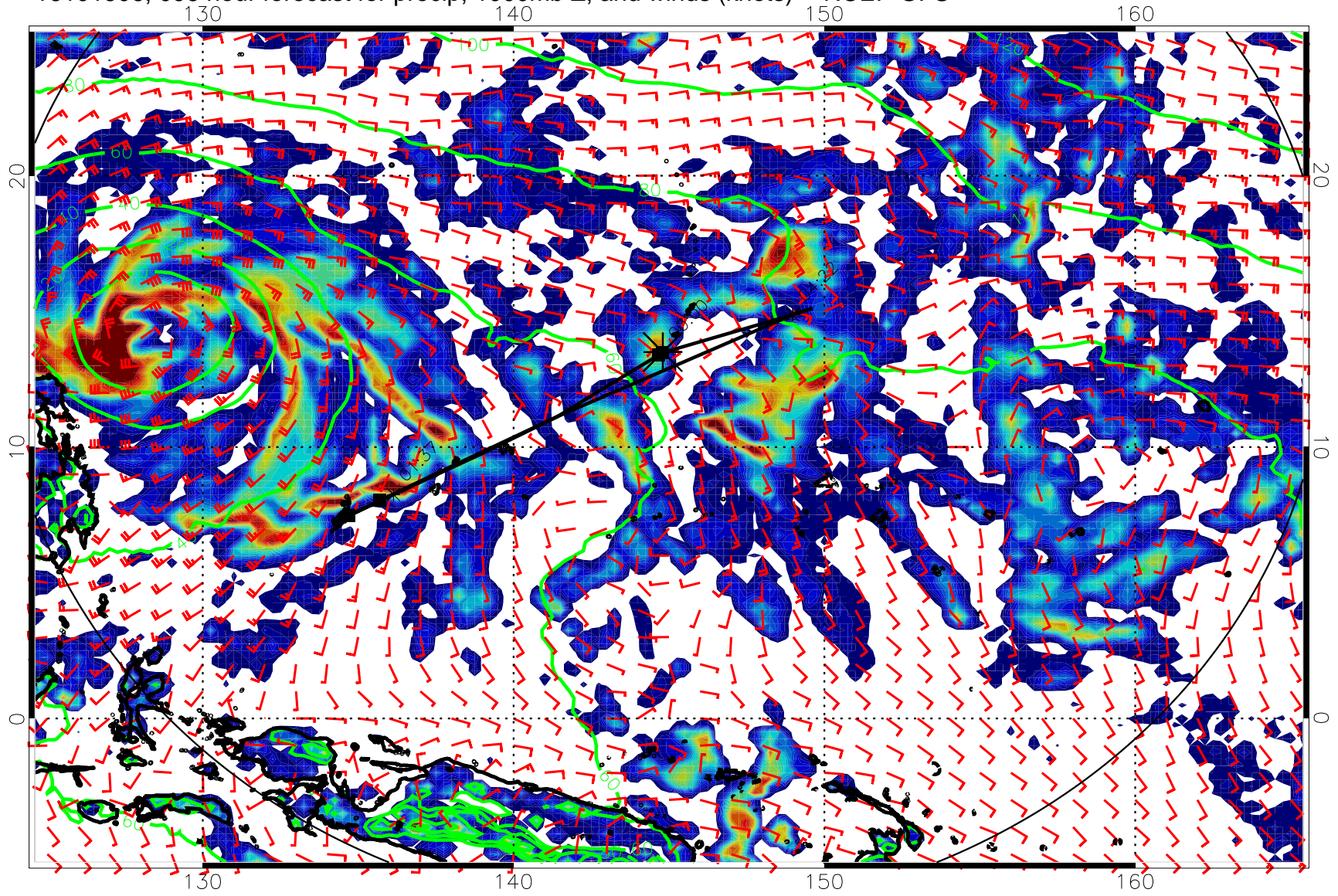
16101506, 096 hour forecast for precip, 1000mb Z, and winds (knots) -- NCEP GFS
