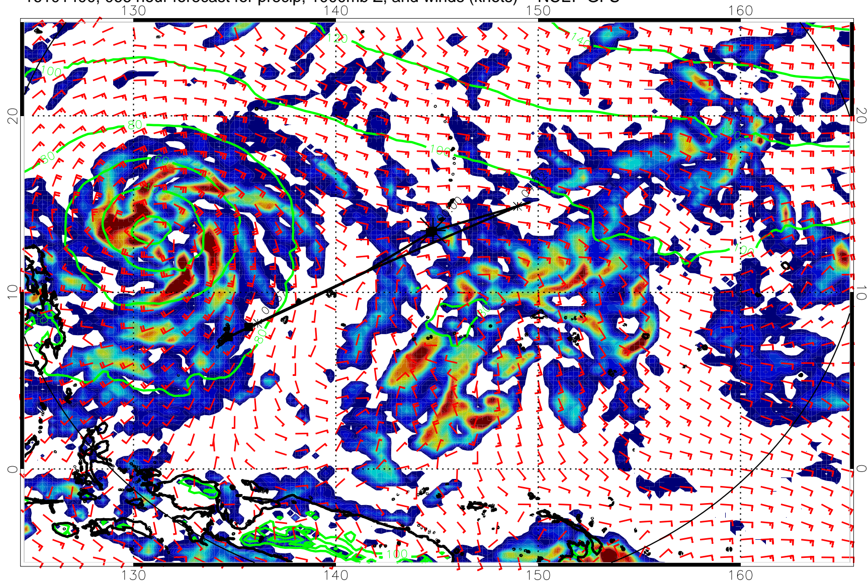
16101400, 066 hour forecast for precip, 1000mb Z, and winds (knots) -- NCEP GFS
