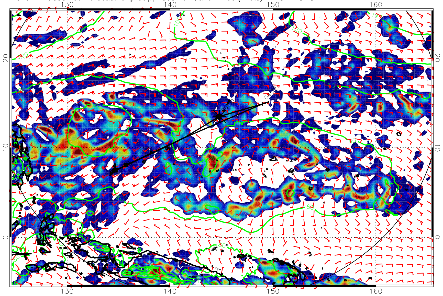
16101212, 030 hour forecast for precip, 1000mb Z, and winds (knots) -- NCEP GFS
