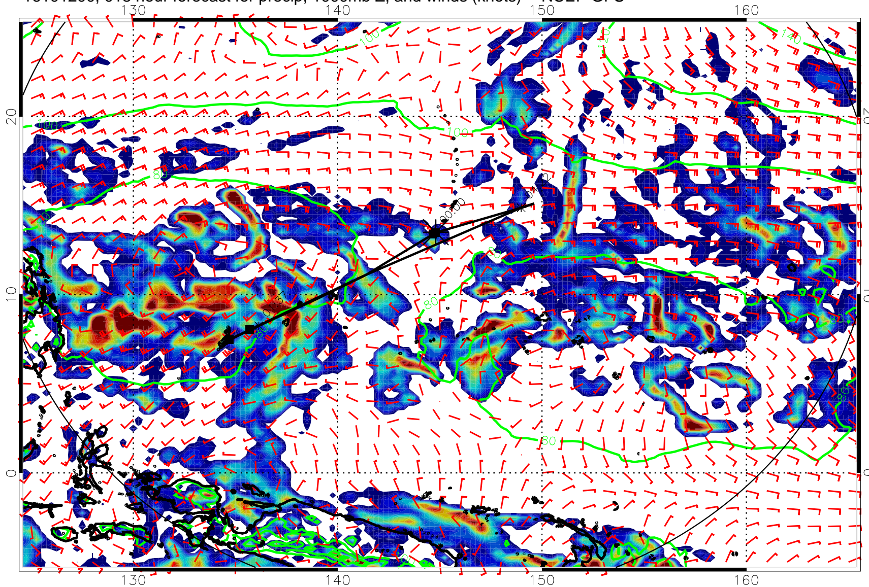
16101200, 018 hour forecast for precip, 1000mb Z, and winds (knots) -- NCEP GFS
