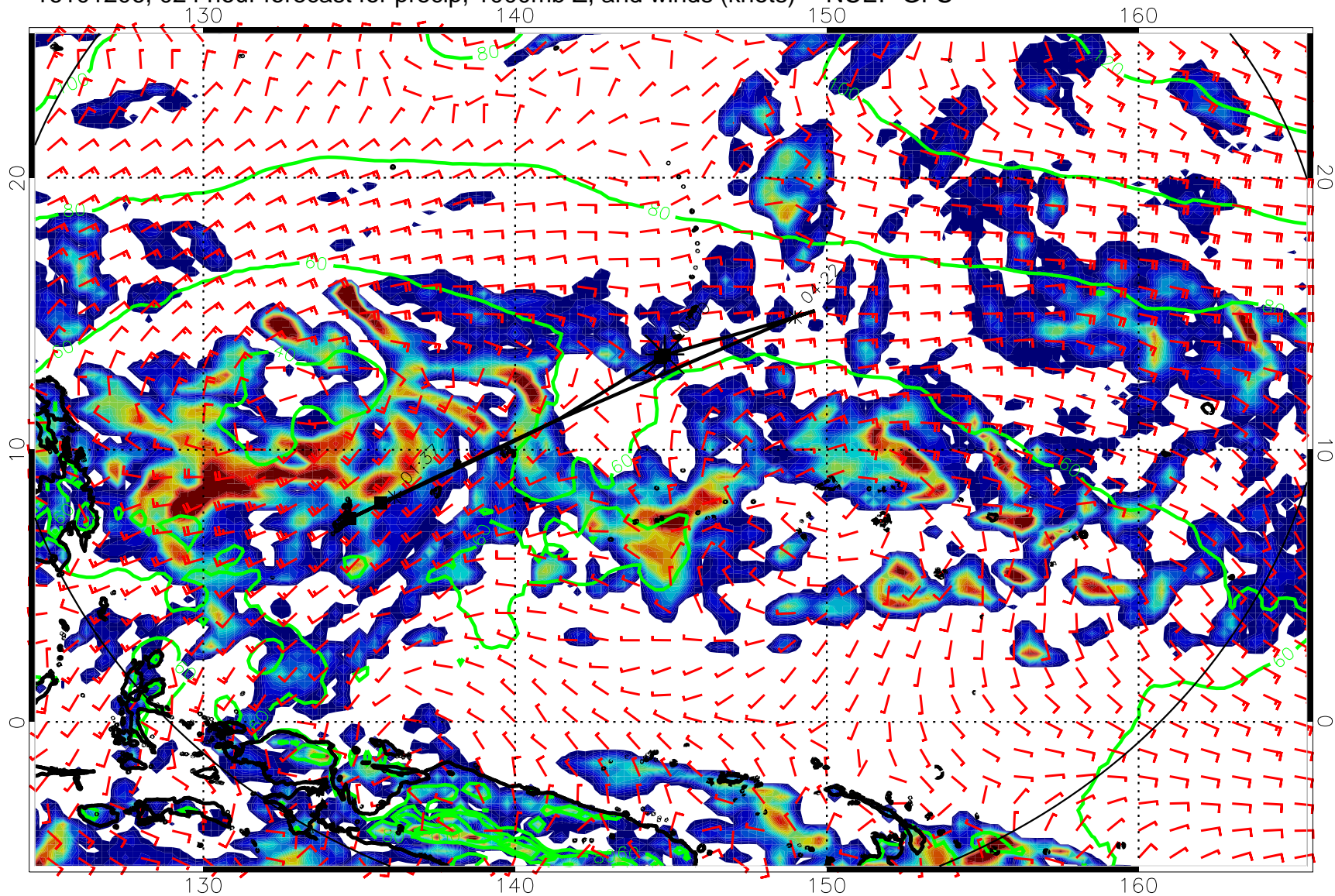
16101206, 024 hour forecast for precip, 1000mb Z, and winds (knots) -- NCEP GFS
