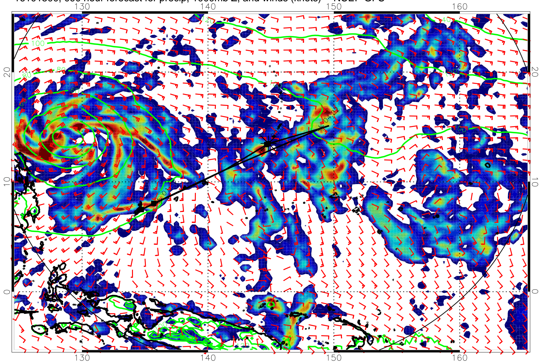
16101500, 090 hour forecast for precip, 1000mb Z, and winds (knots) -- NCEP GFS
