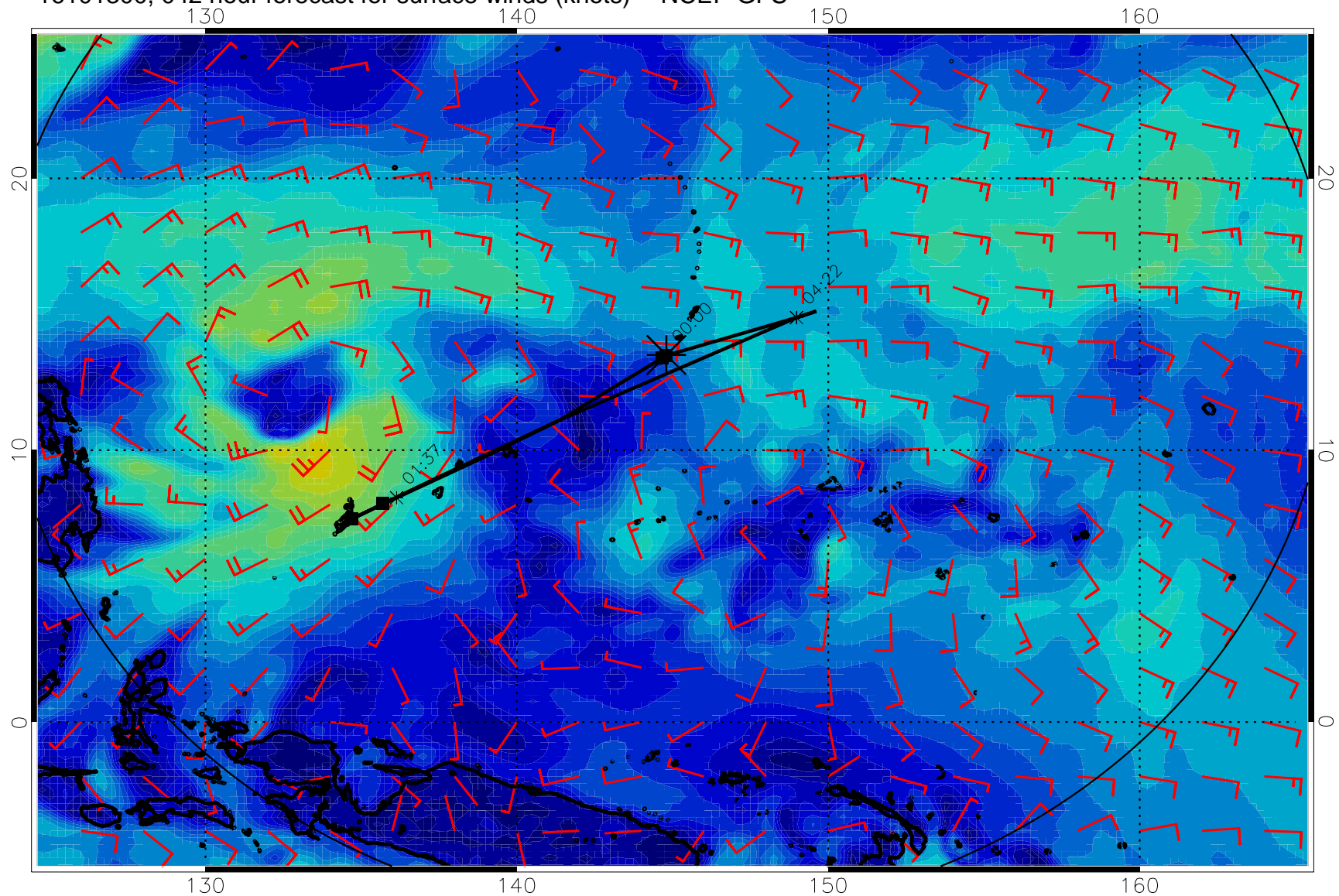
16101300, 042 hour forecast for surface winds (knots) -- NCEP GFS
