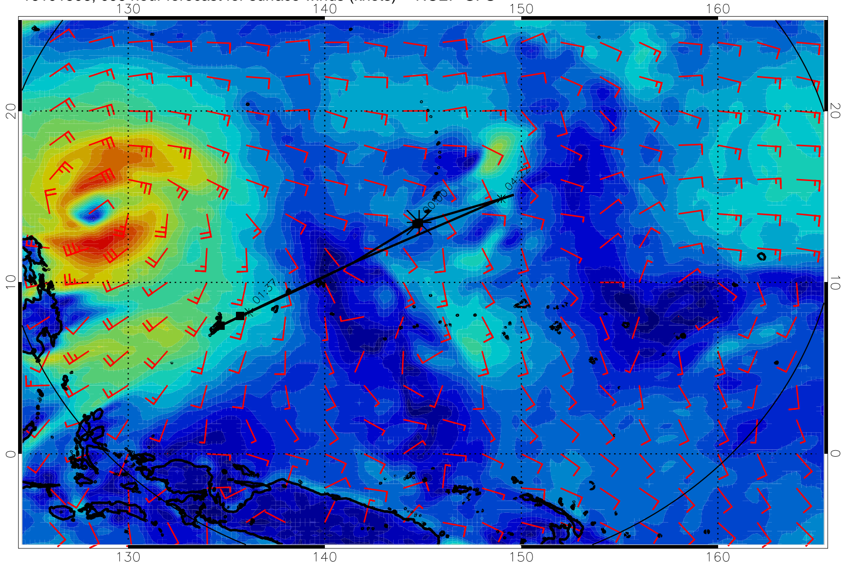
16101506, 096 hour forecast for surface winds (knots) -- NCEP GFS
