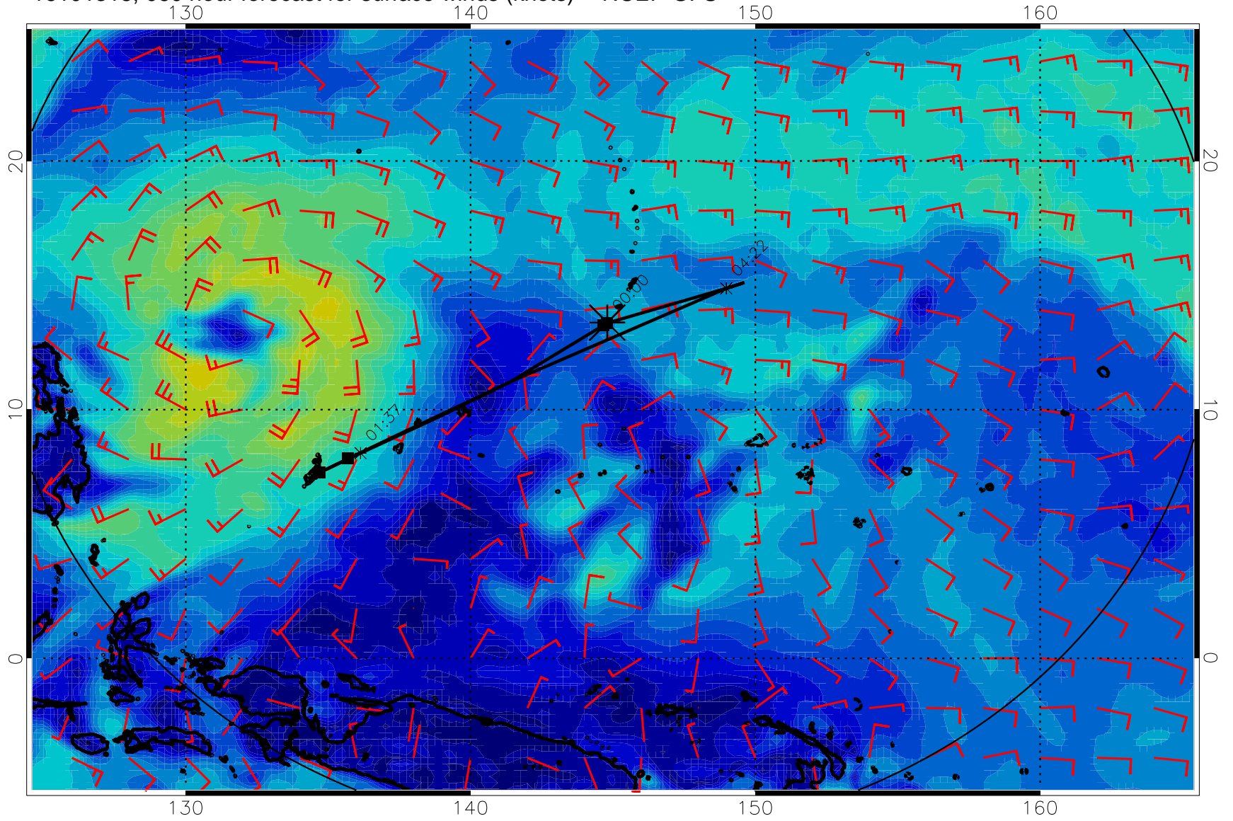
16101318, 060 hour forecast for surface winds (knots) -- NCEP GFS
