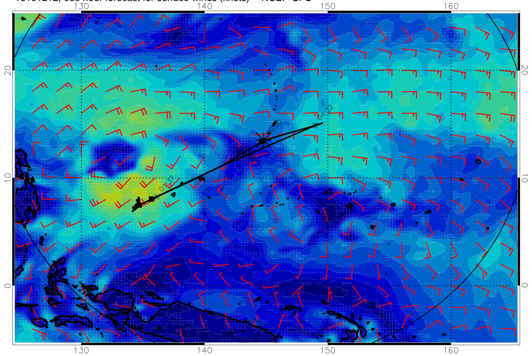
16101212, 030 hour forecast for surface winds (knots) -- NCEP GFS
