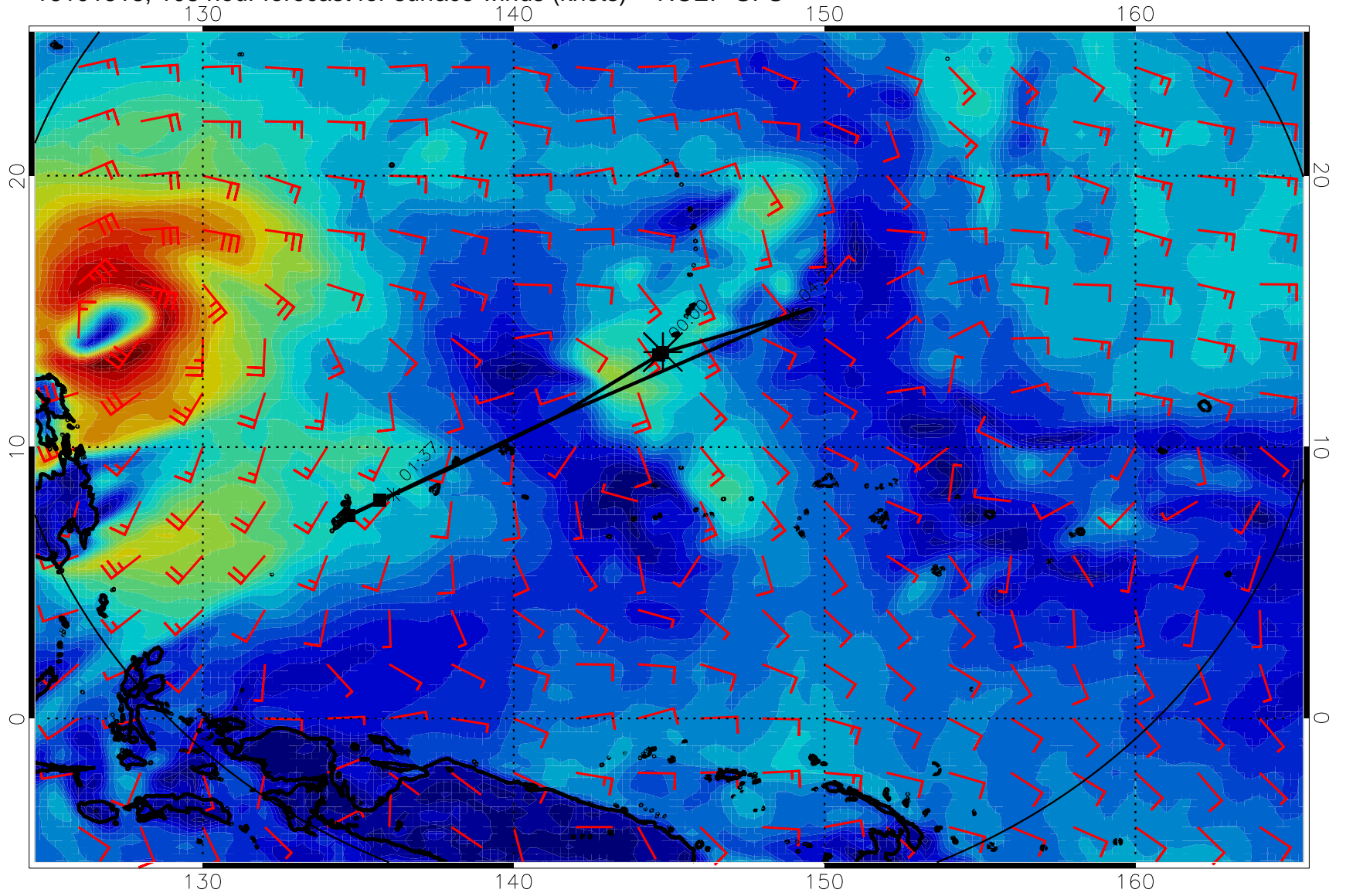
16101518, 108 hour forecast for surface winds (knots) -- NCEP GFS
