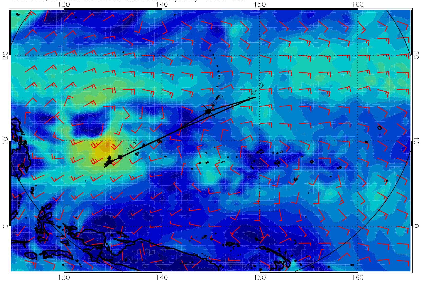
16101218, 036 hour forecast for surface winds (knots) -- NCEP GFS
