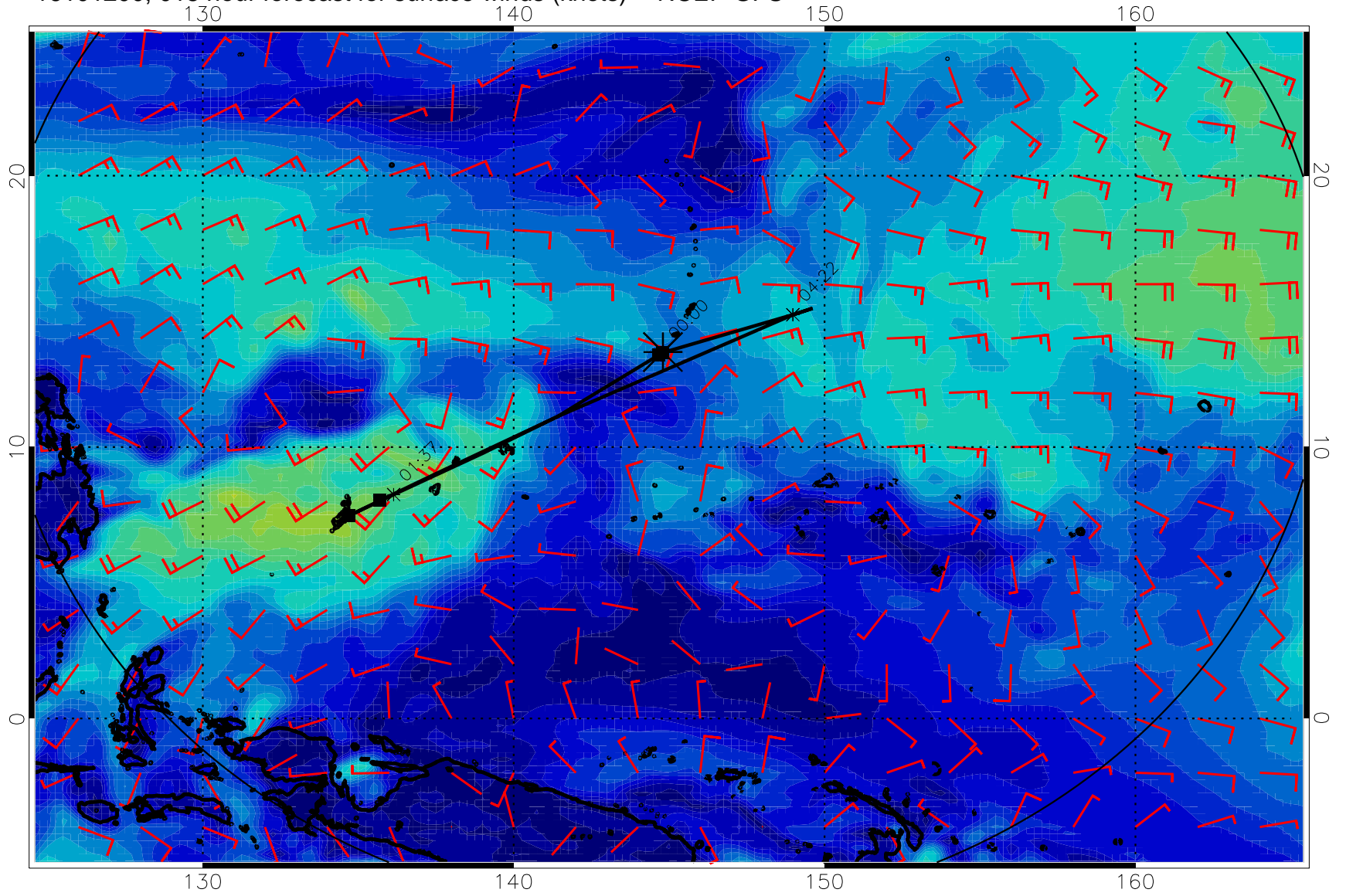
16101200, 018 hour forecast for surface winds (knots) -- NCEP GFS
