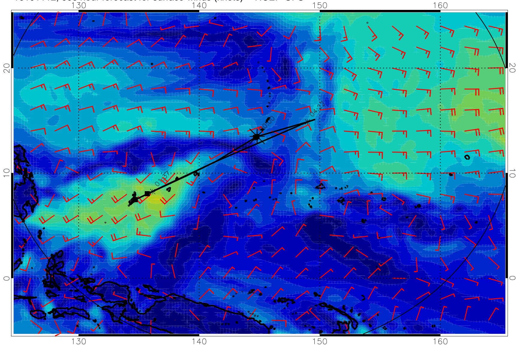
16101112, 006 hour forecast for surface winds (knots) -- NCEP GFS
