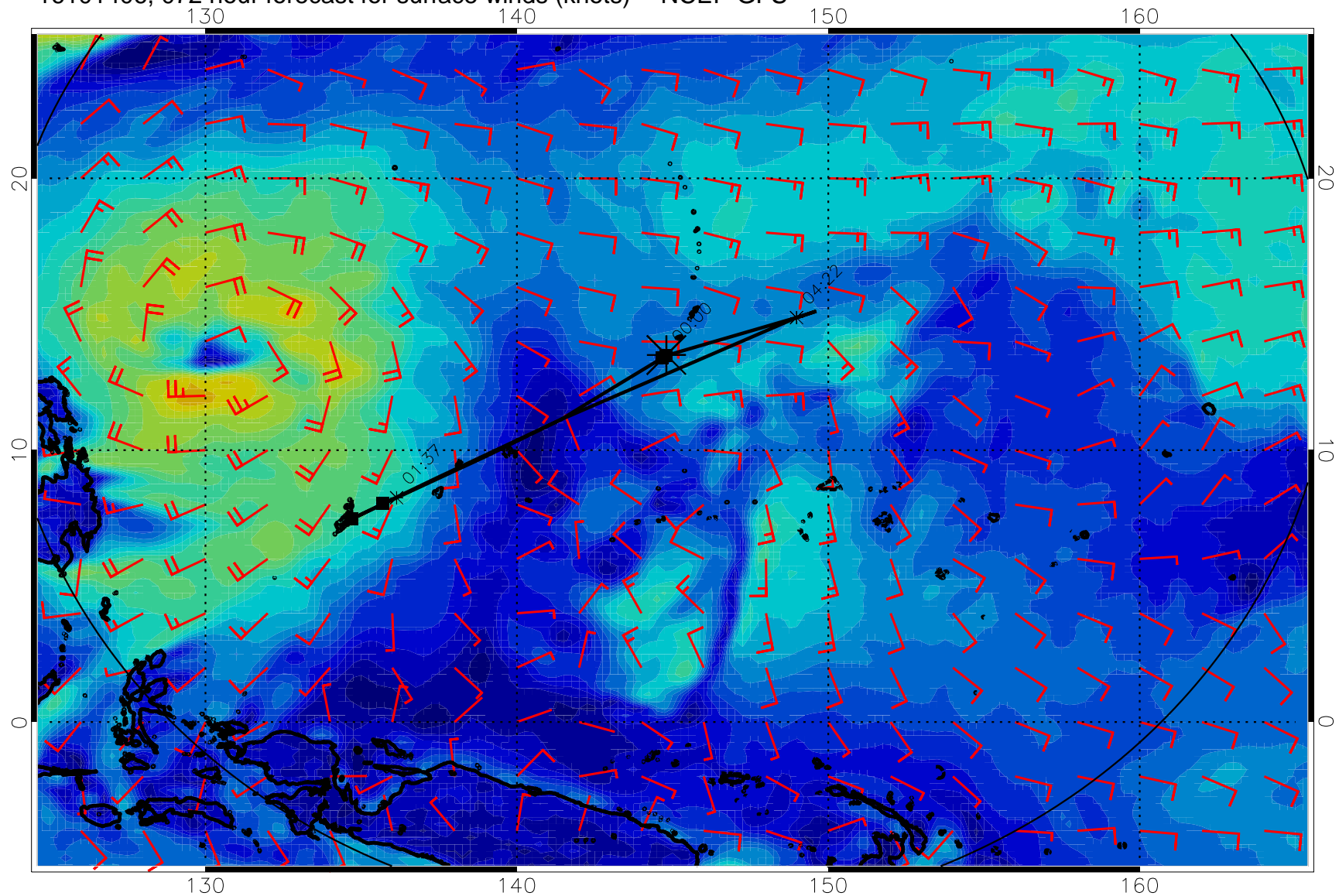
16101406, 072 hour forecast for surface winds (knots) -- NCEP GFS
