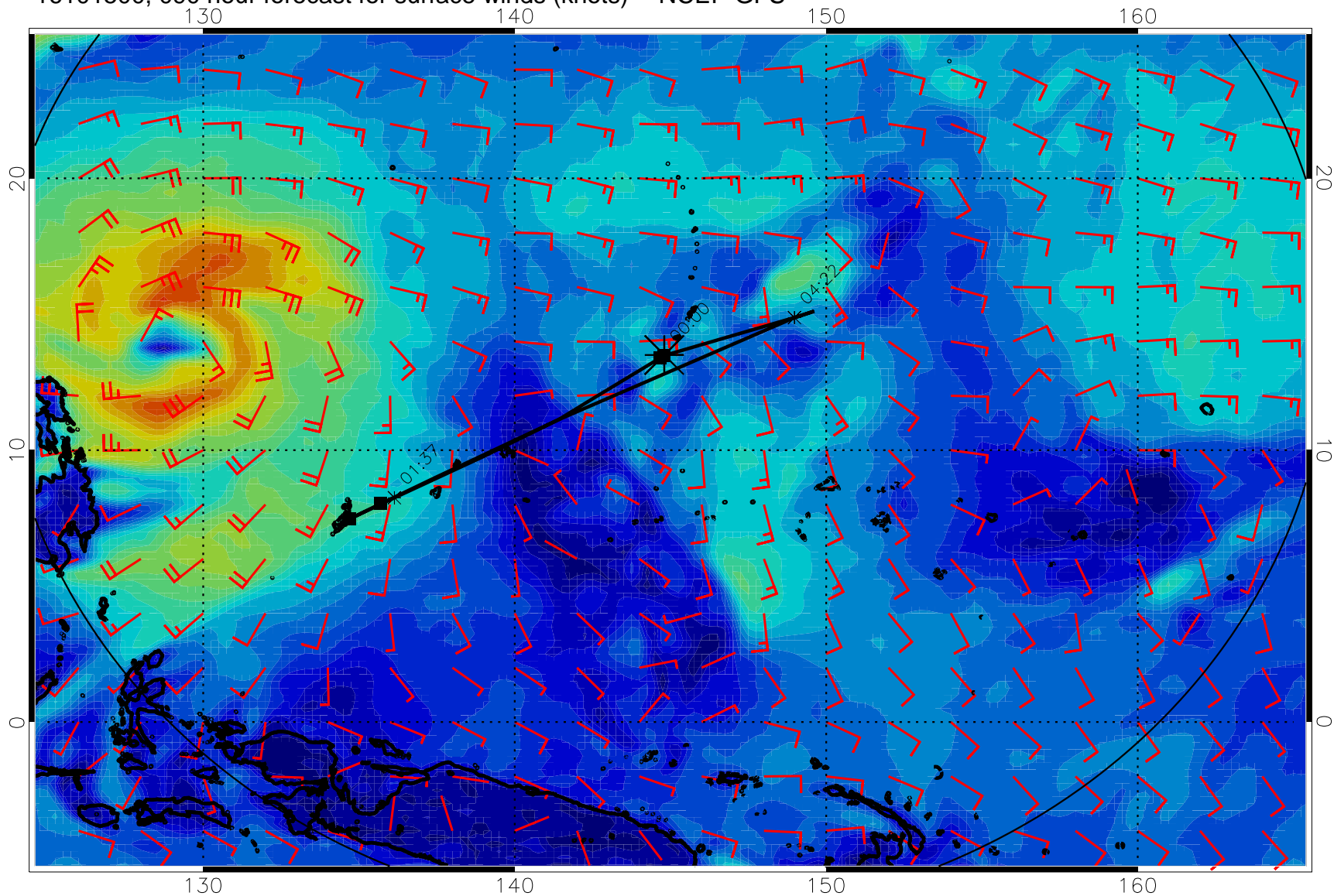
16101500, 090 hour forecast for surface winds (knots) -- NCEP GFS
