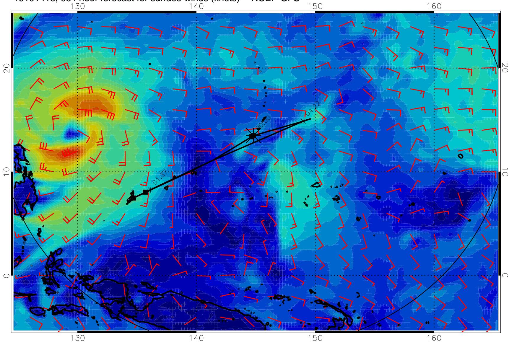
16101418, 084 hour forecast for surface winds (knots) -- NCEP GFS
