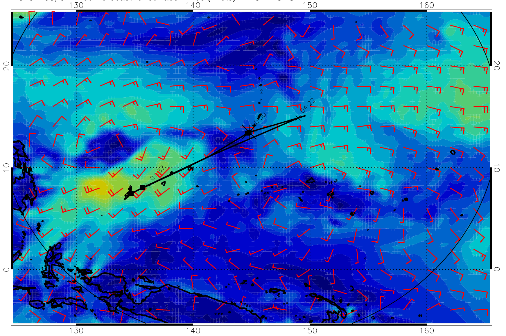
16101206, 024 hour forecast for surface winds (knots) -- NCEP GFS
