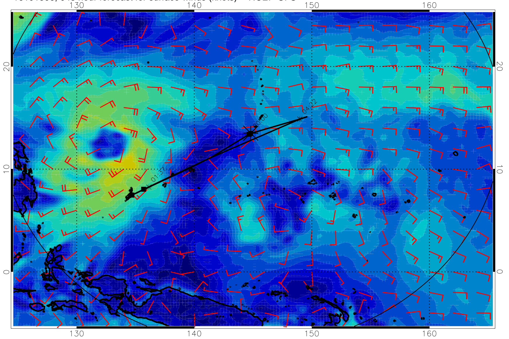
16101306, 048 hour forecast for surface winds (knots) -- NCEP GFS
