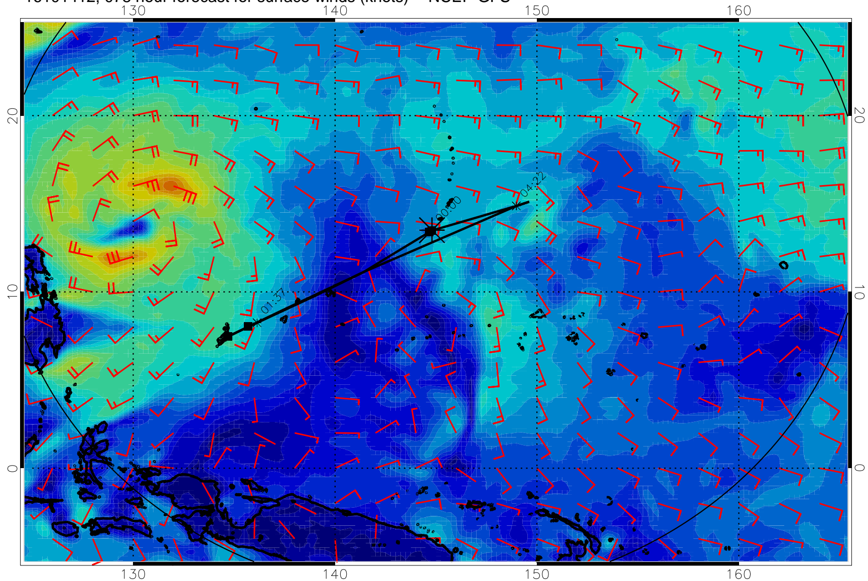
16101412, 078 hour forecast for surface winds (knots) -- NCEP GFS
