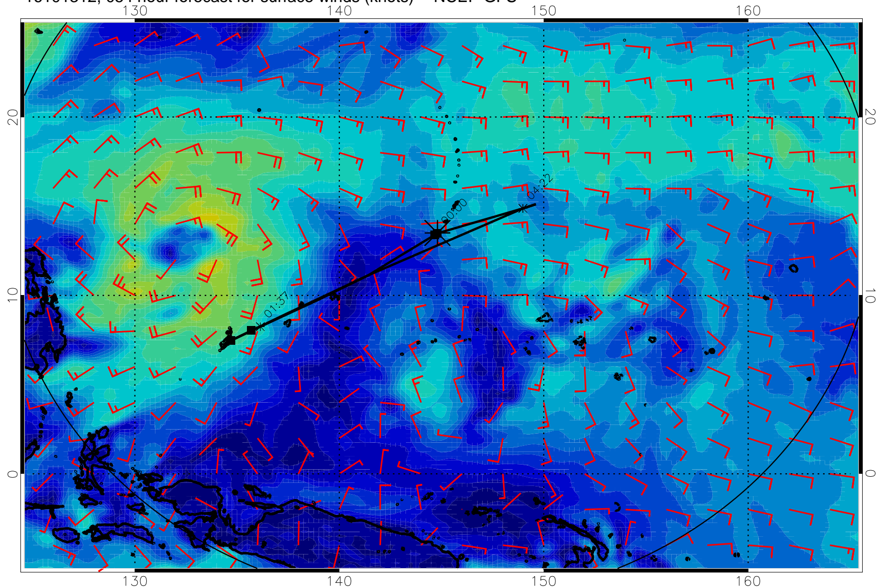
16101312, 054 hour forecast for surface winds (knots) -- NCEP GFS
