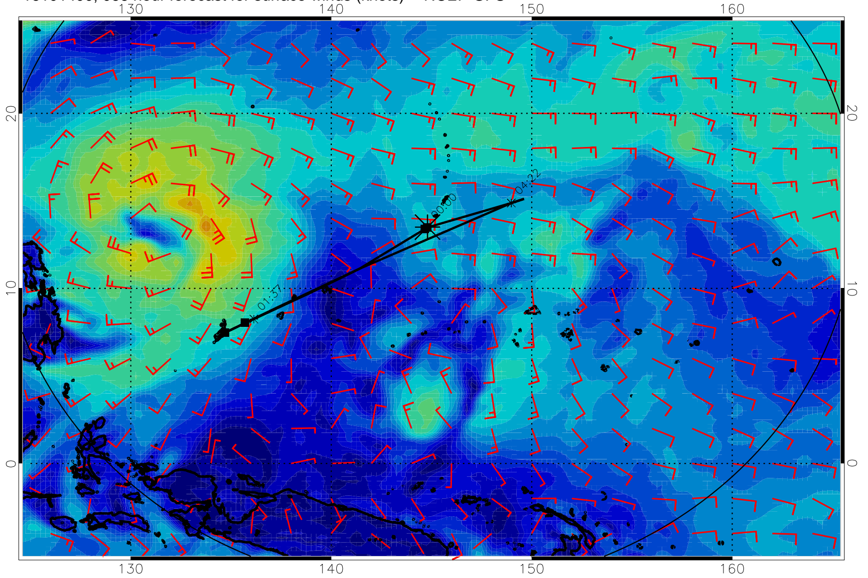
16101400, 066 hour forecast for surface winds (knots) -- NCEP GFS
