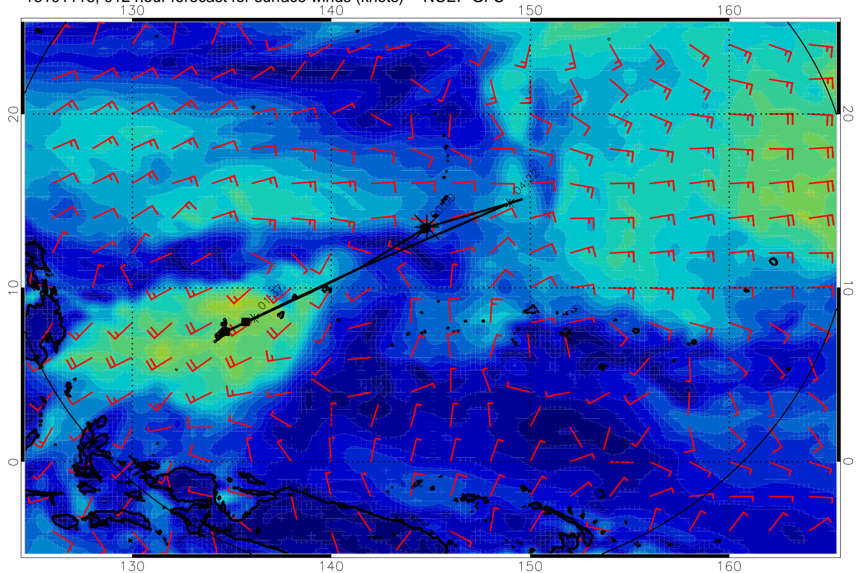
16101118, 012 hour forecast for surface winds (knots) -- NCEP GFS
