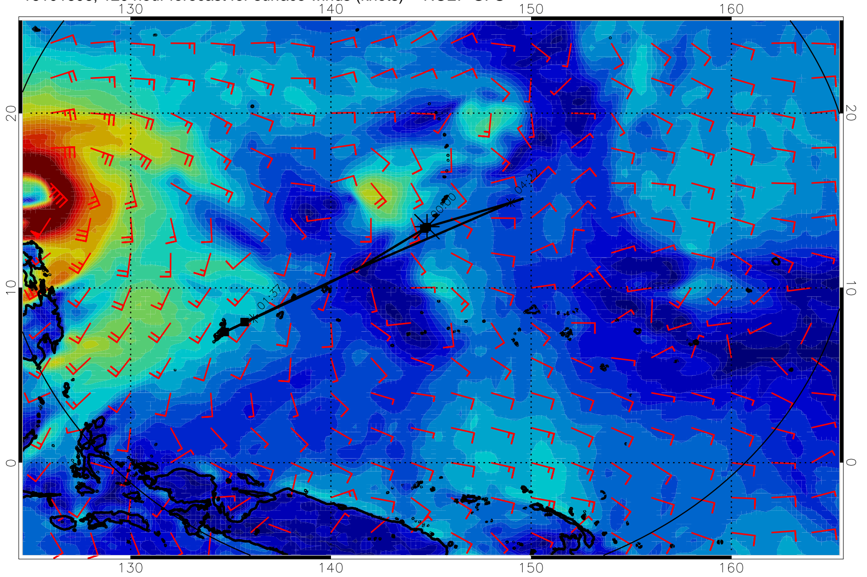
16101606, 120 hour forecast for surface winds (knots) -- NCEP GFS
