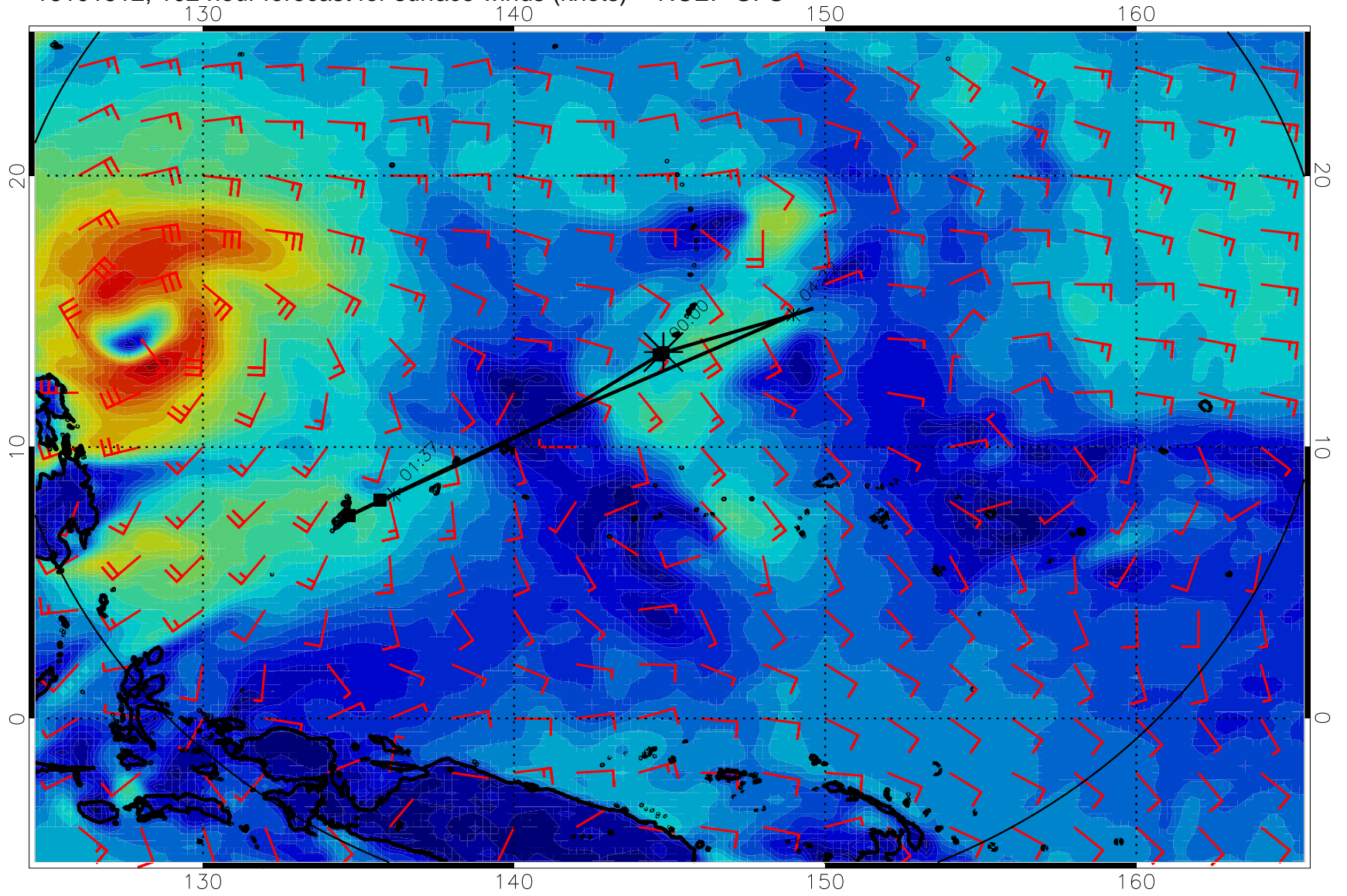
16101512, 102 hour forecast for surface winds (knots) -- NCEP GFS
