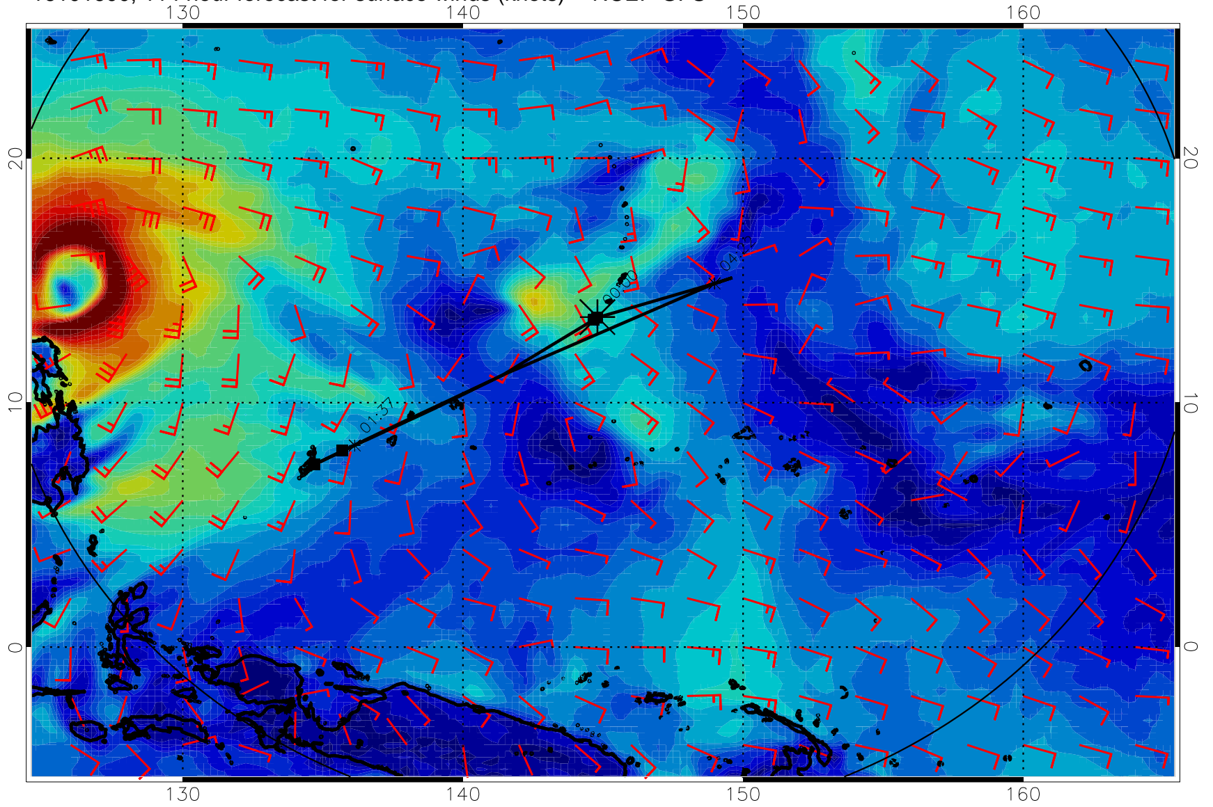
16101600, 114 hour forecast for surface winds (knots) -- NCEP GFS
