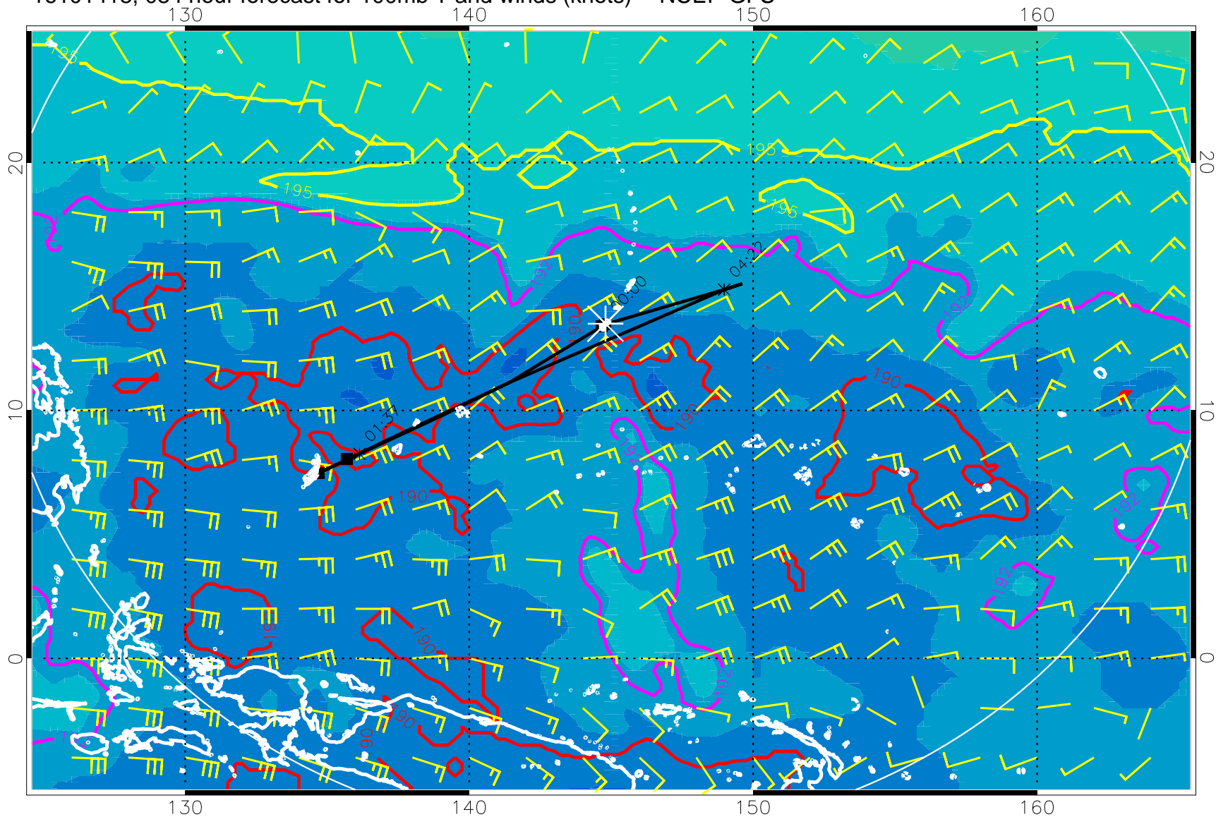
16101418, 084 hour forecast for 100mb T and winds (knots) -- NCEP GFS
