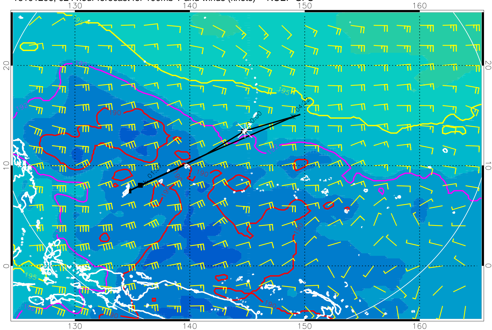
16101206, 024 hour forecast for 100mb T and winds (knots) -- NCEP GFS
