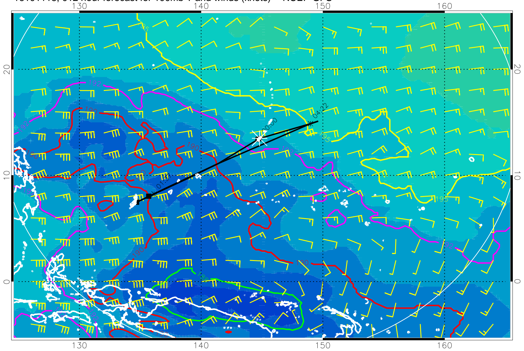
16101118, 012 hour forecast for 100mb T and winds (knots) -- NCEP GFS
