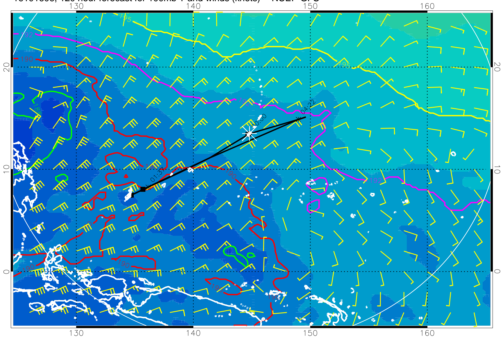
16101606, 120 hour forecast for 100mb T and winds (knots) -- NCEP GFS
