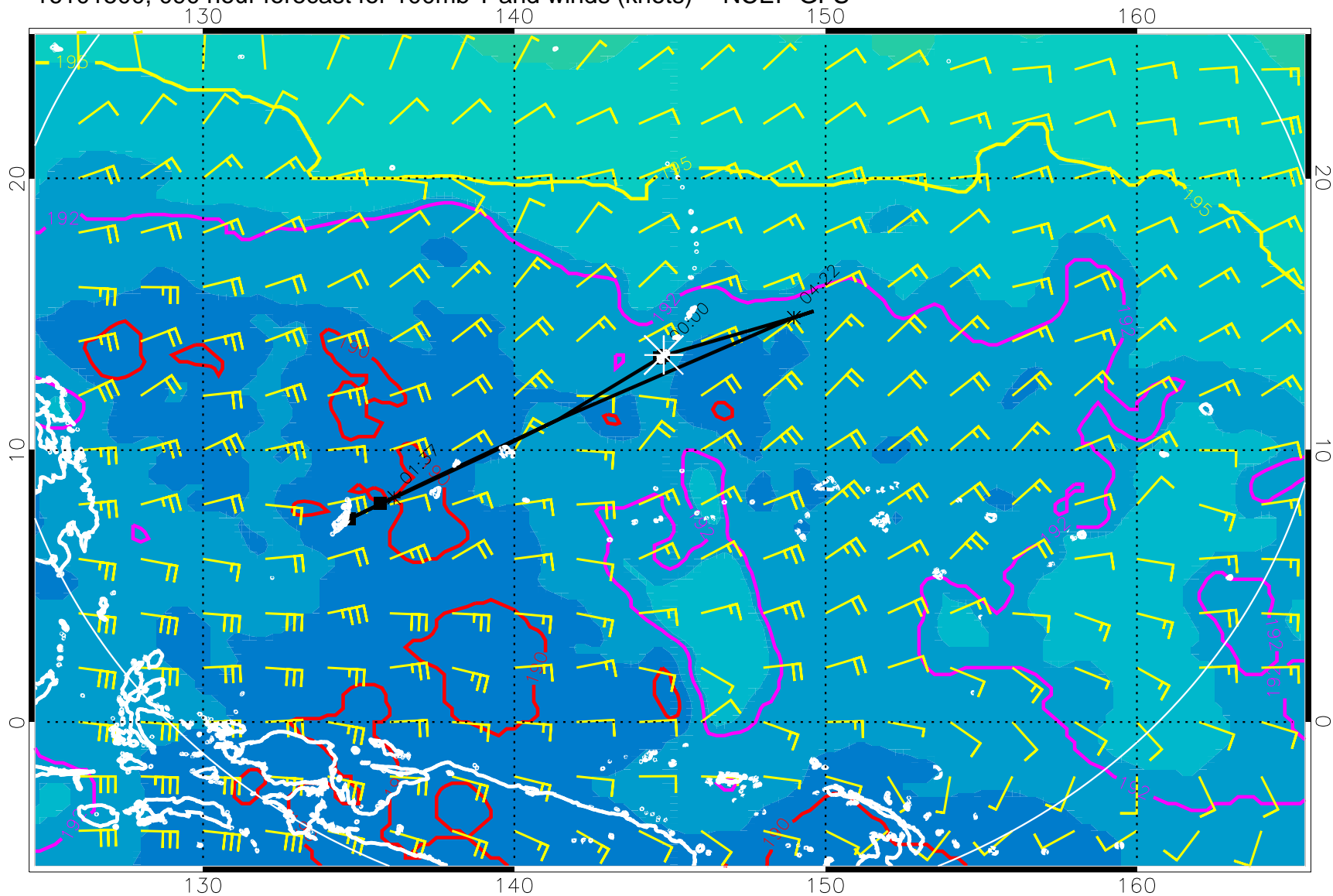
16101500, 090 hour forecast for 100mb T and winds (knots) -- NCEP GFS
