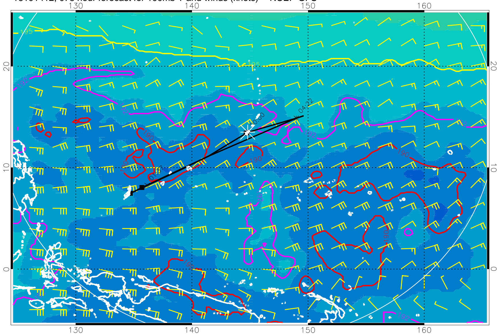
16101412, 078 hour forecast for 100mb T and winds (knots) -- NCEP GFS
