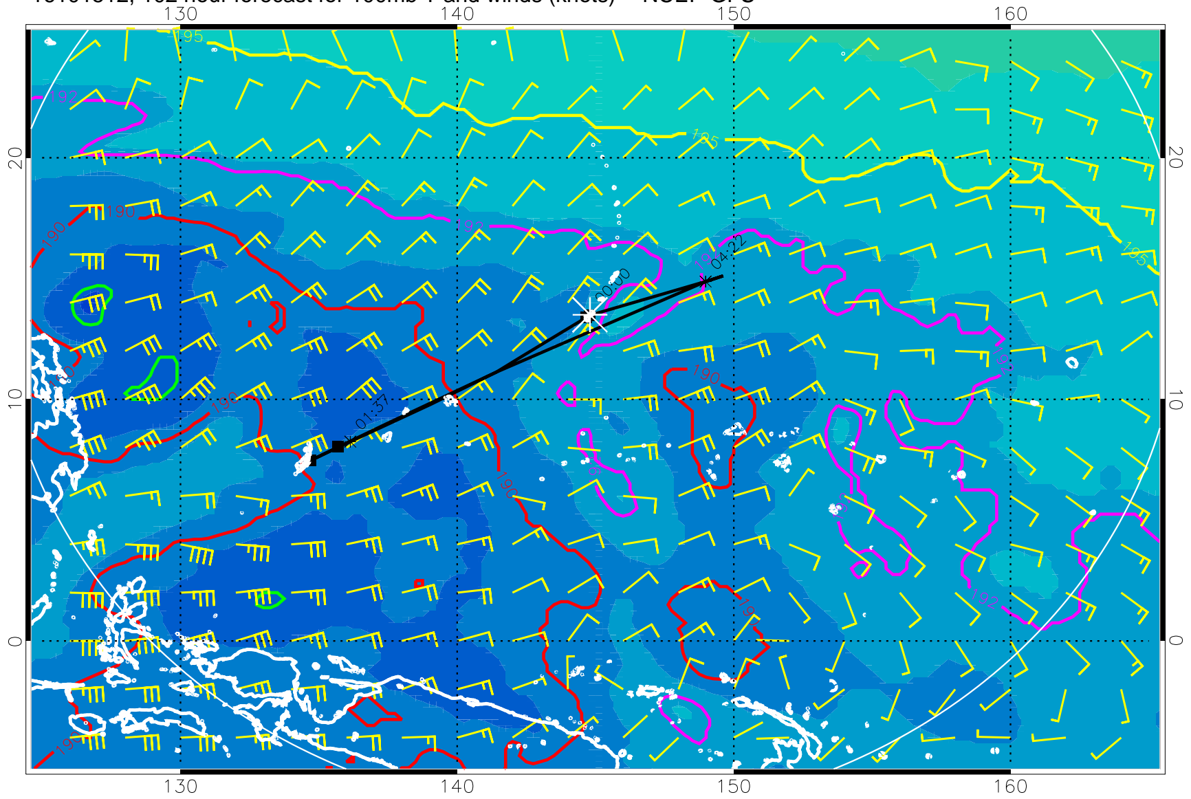
16101512, 102 hour forecast for 100mb T and winds (knots) -- NCEP GFS
