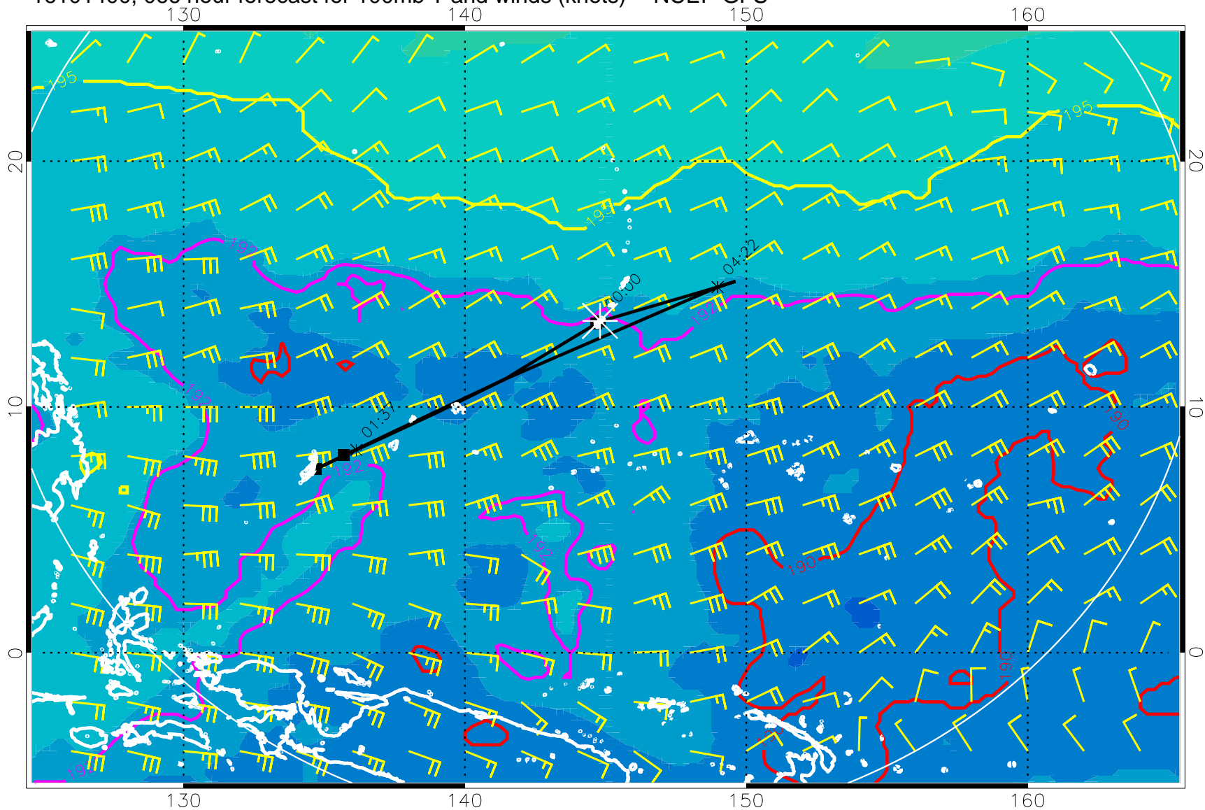
16101400, 066 hour forecast for 100mb T and winds (knots) -- NCEP GFS
