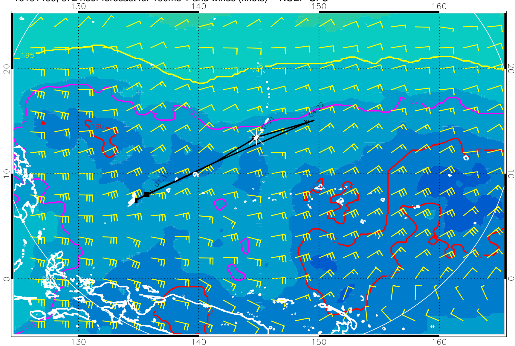
16101406, 072 hour forecast for 100mb T and winds (knots) -- NCEP GFS
