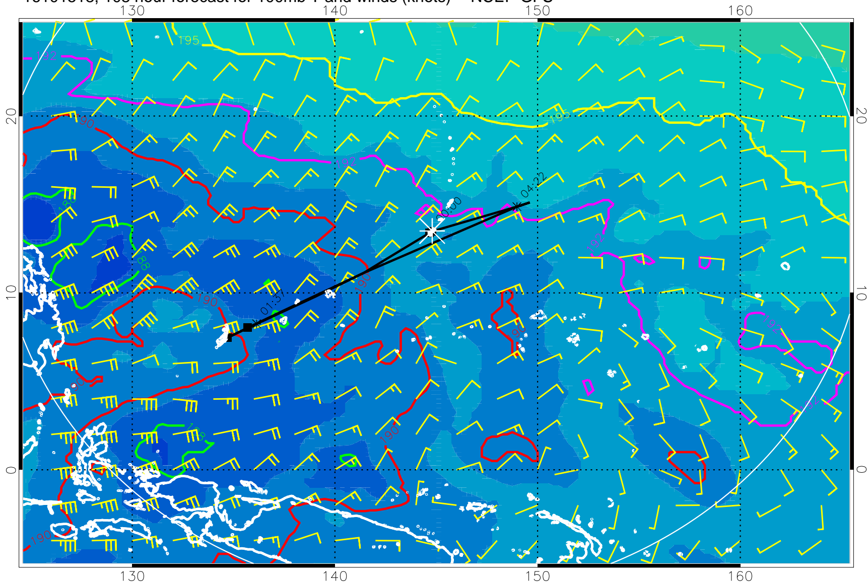
16101518, 108 hour forecast for 100mb T and winds (knots) -- NCEP GFS
