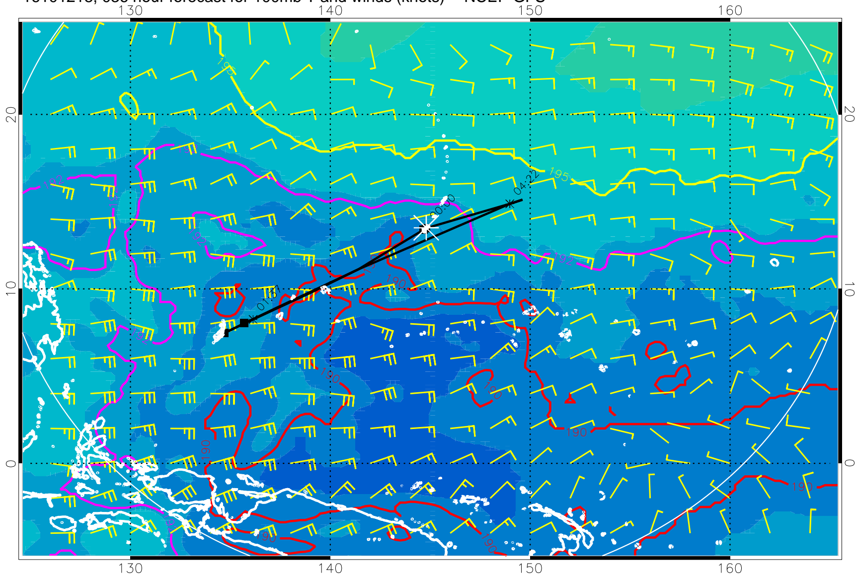
16101218, 036 hour forecast for 100mb T and winds (knots) -- NCEP GFS
