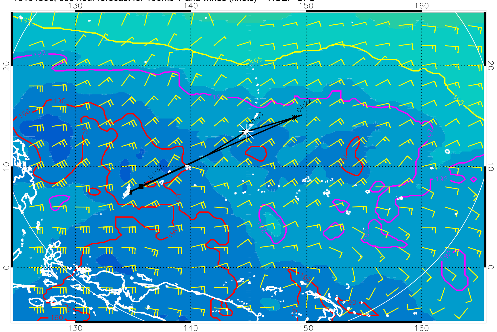
16101506, 096 hour forecast for 100mb T and winds (knots) -- NCEP GFS
