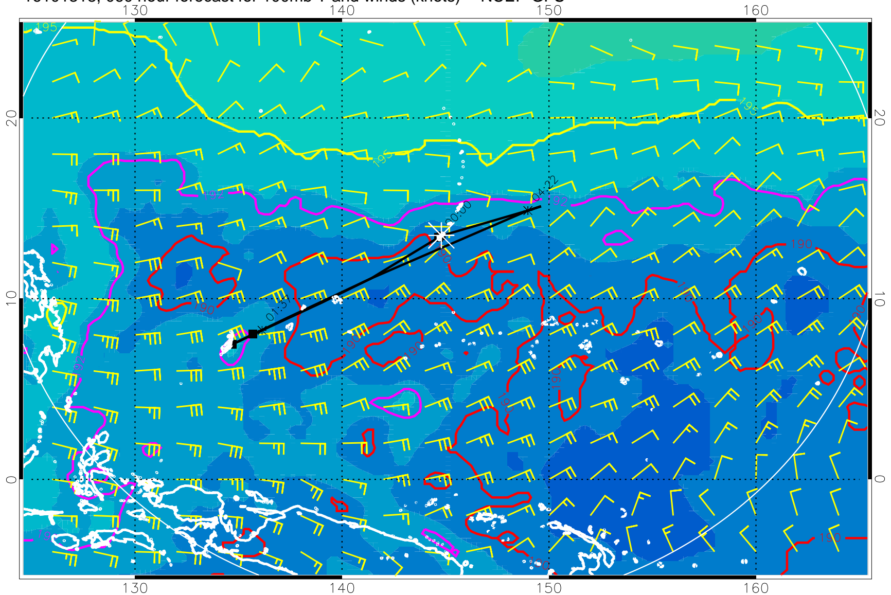
16101318, 060 hour forecast for 100mb T and winds (knots) -- NCEP GFS
