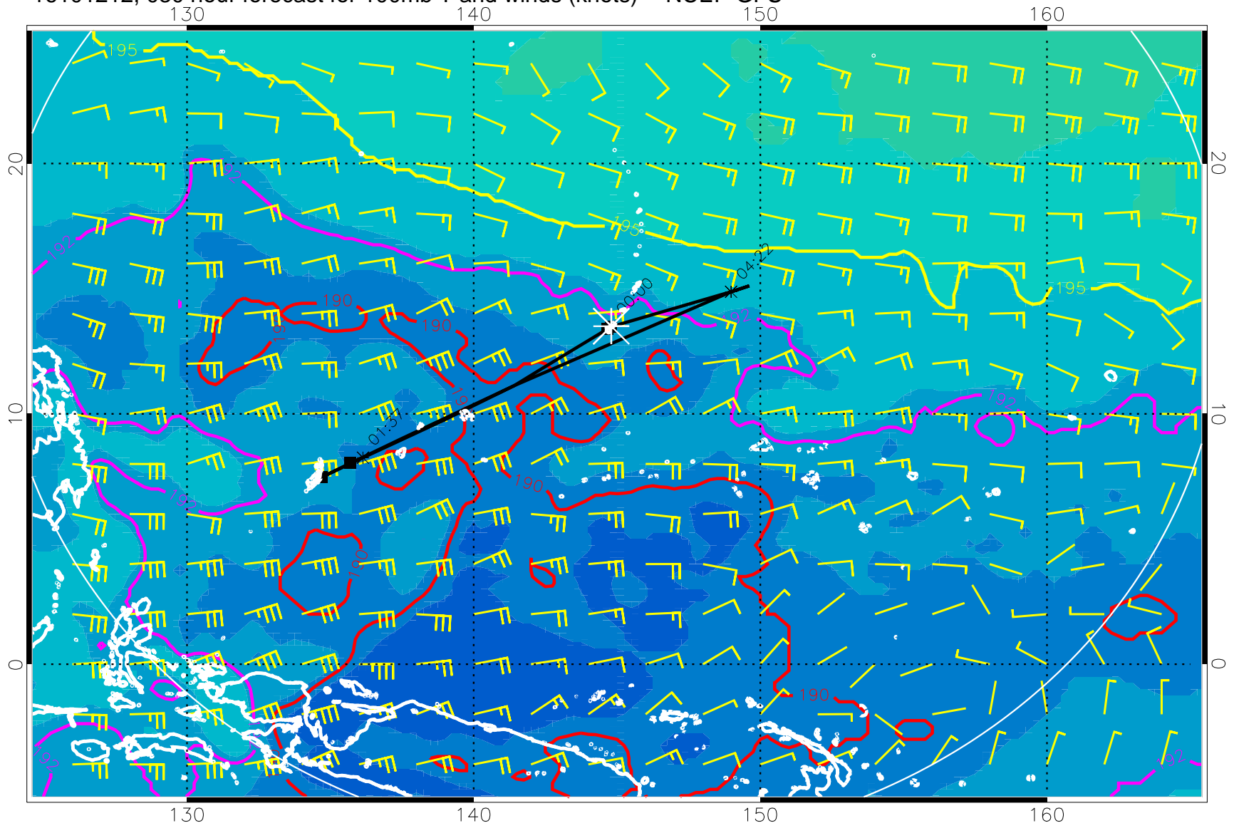
16101212, 030 hour forecast for 100mb T and winds (knots) -- NCEP GFS
