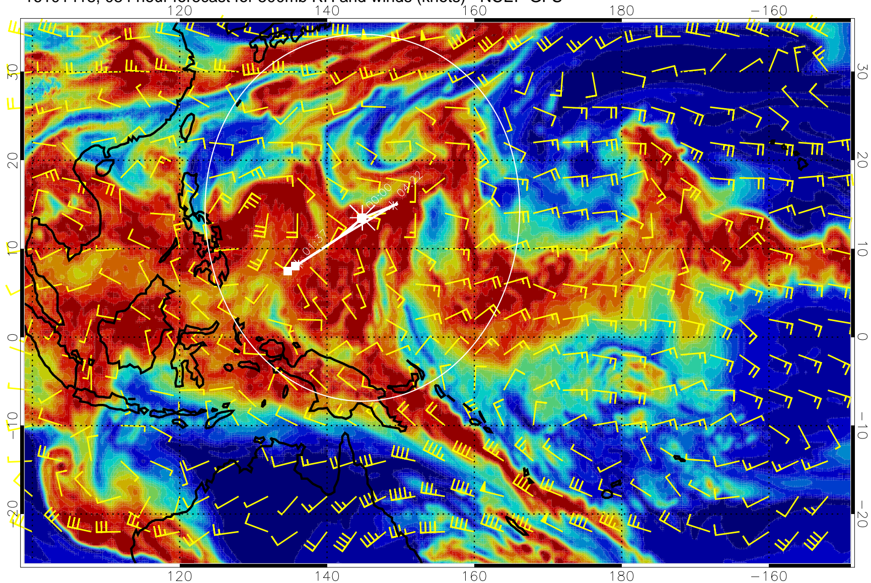
16101418, 084 hour forecast for 500mb RH and winds (knots) - NCEP GFS
