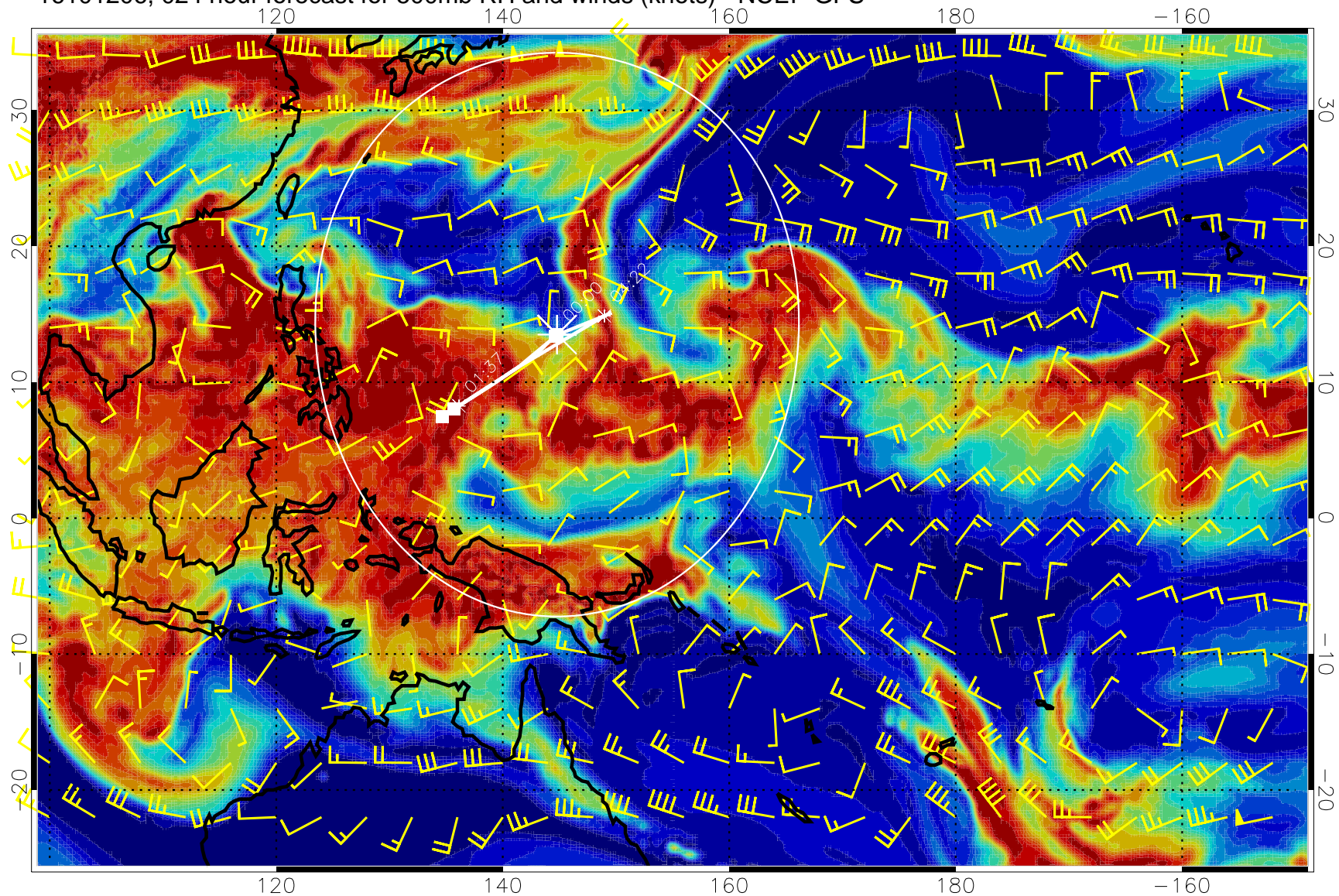
16101206, 024 hour forecast for 500mb RH and winds (knots) - NCEP GFS
