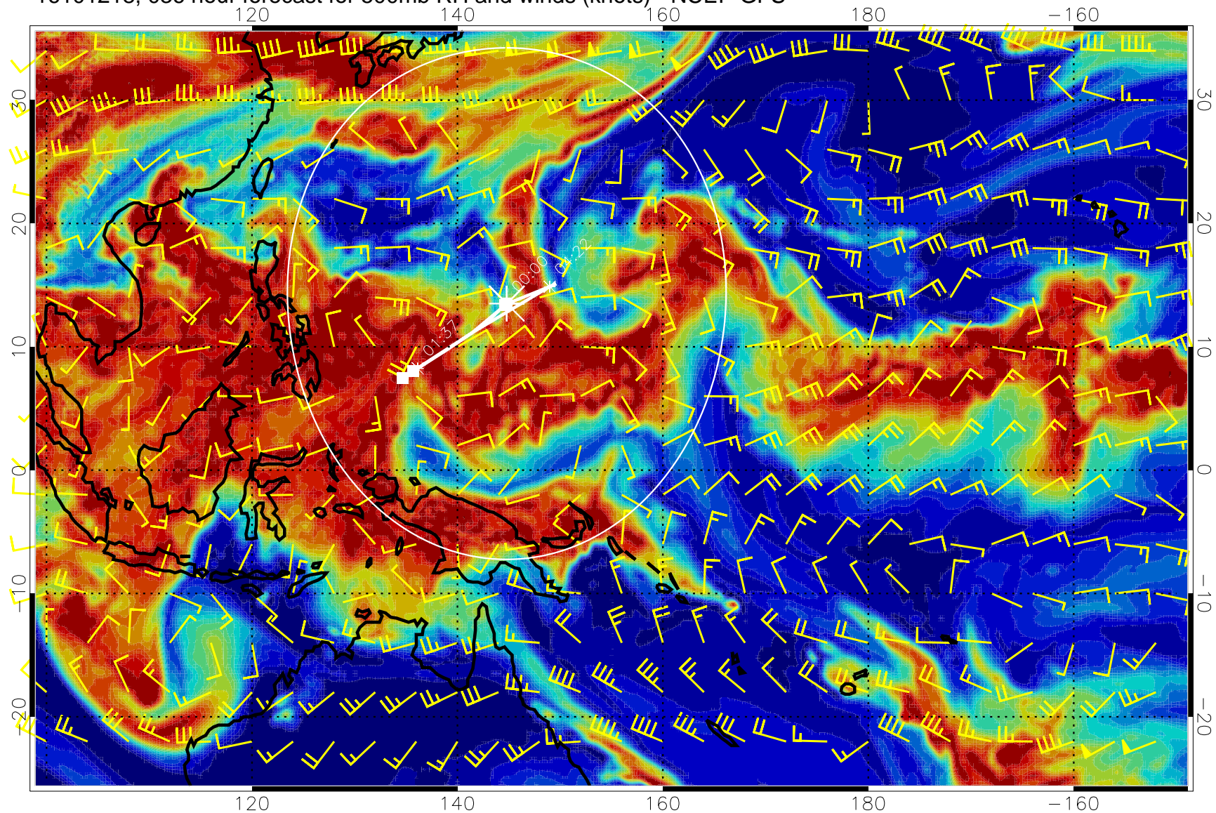
16101218, 036 hour forecast for 500mb RH and winds (knots) - NCEP GFS
