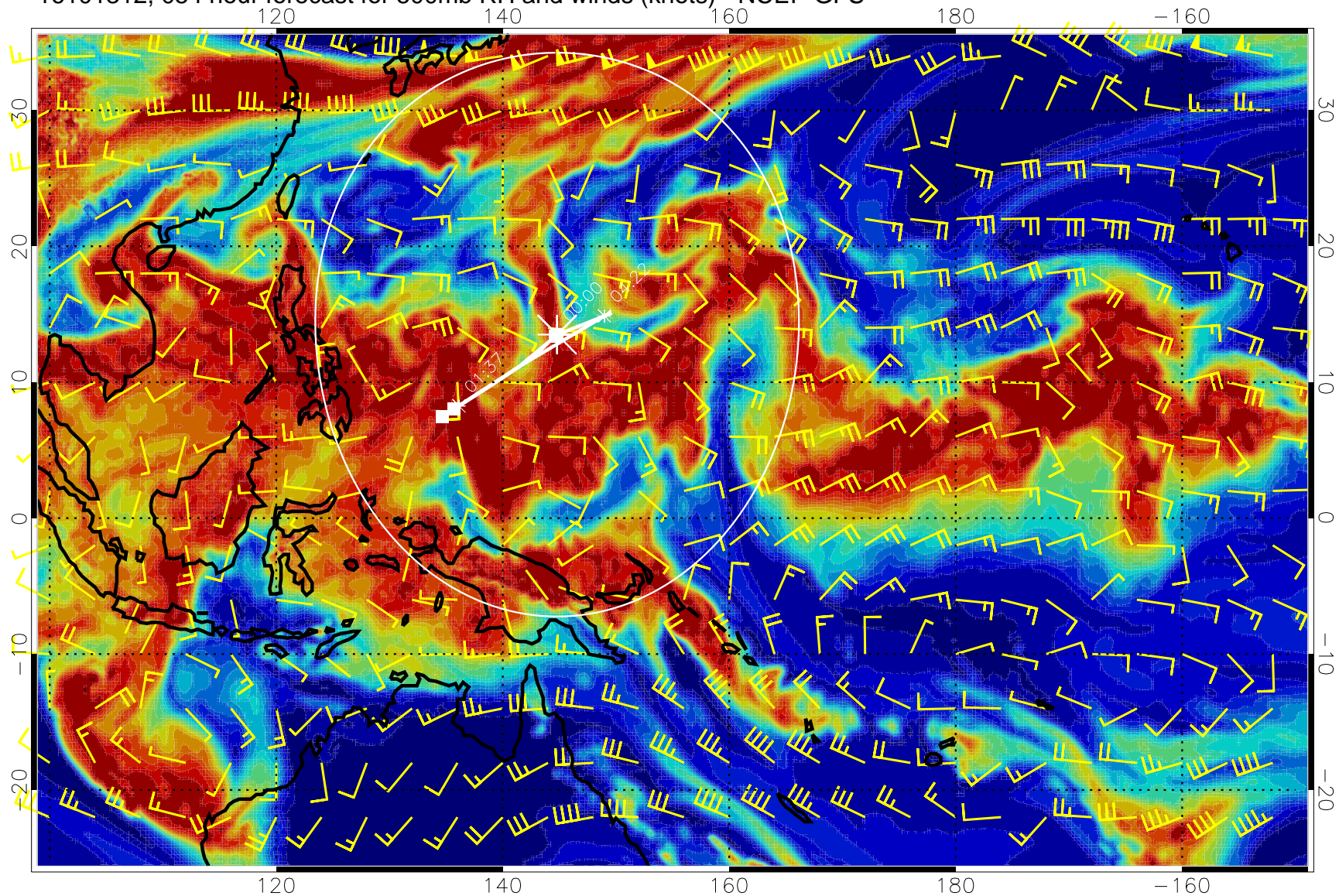
16101312, 054 hour forecast for 500mb RH and winds (knots) - NCEP GFS
