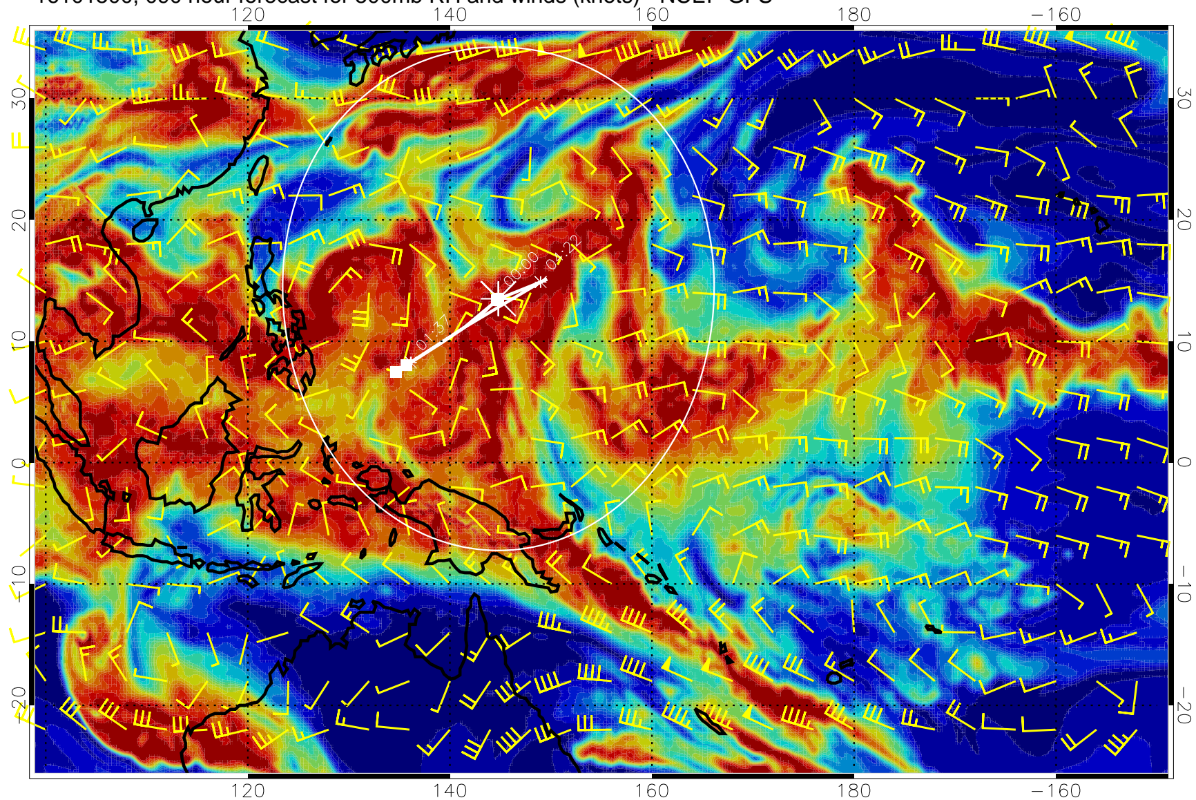
16101500, 090 hour forecast for 500mb RH and winds (knots) - NCEP GFS
