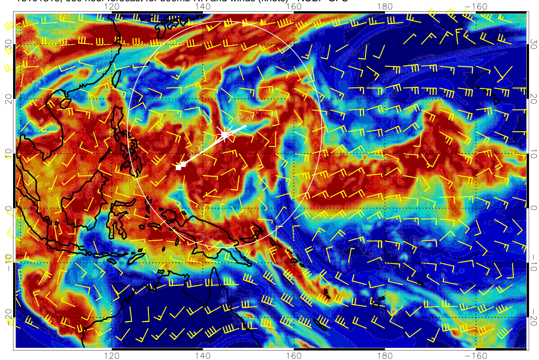
16101318, 060 hour forecast for 500mb RH and winds (knots) - NCEP GFS
