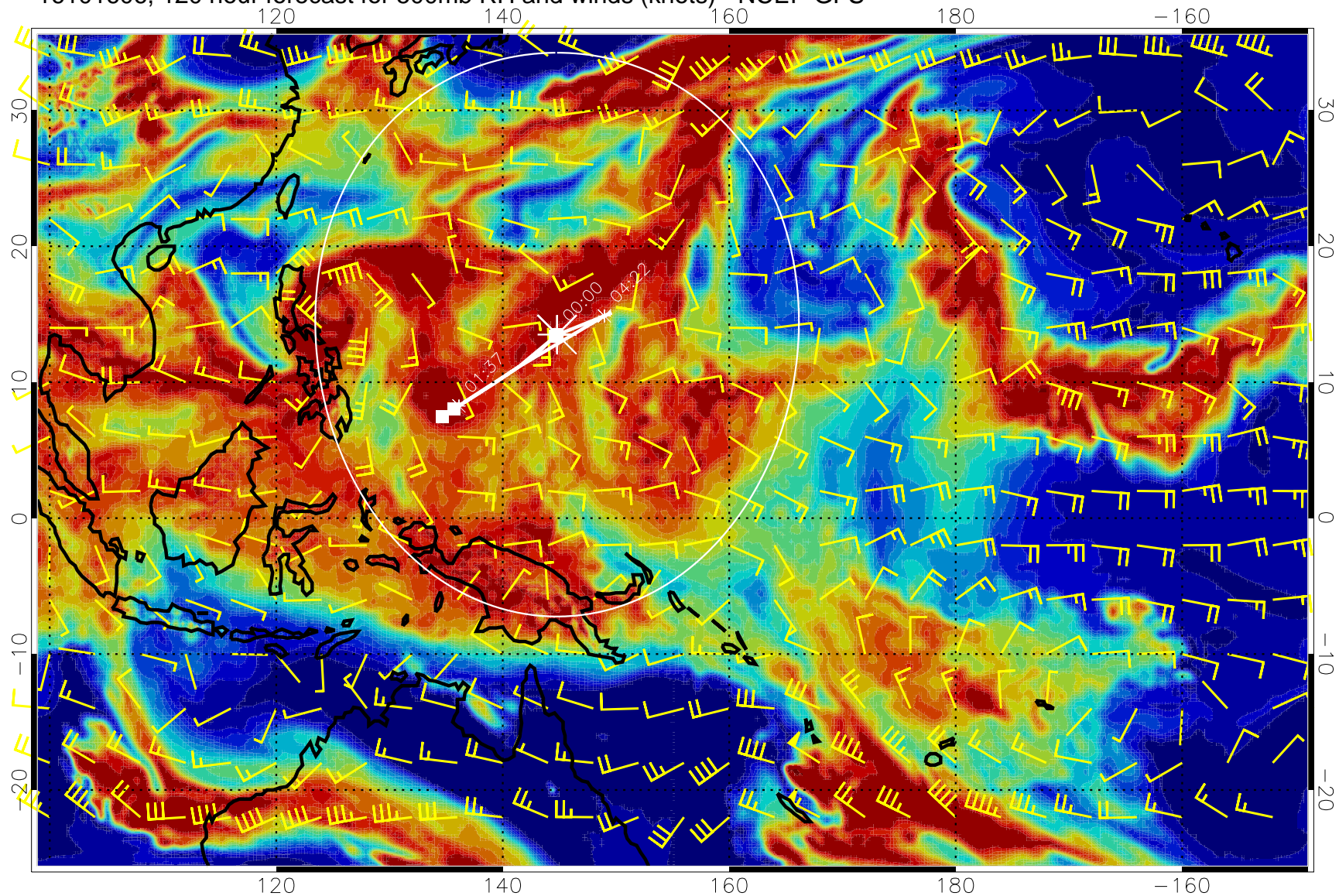
16101606, 120 hour forecast for 500mb RH and winds (knots) - NCEP GFS
