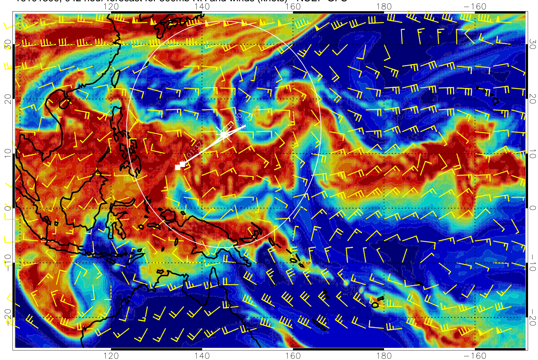
16101300, 042 hour forecast for 500mb RH and winds (knots) - NCEP GFS
