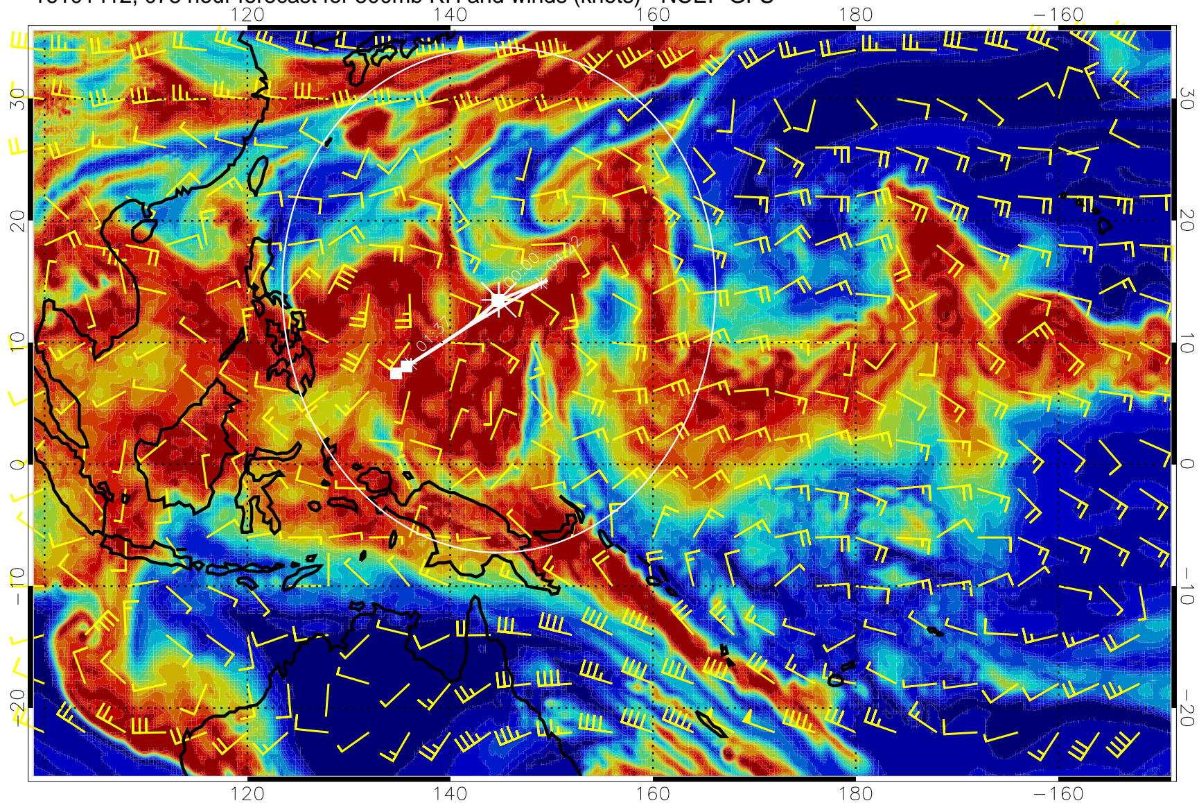
16101412, 078 hour forecast for 500mb RH and winds (knots) - NCEP GFS
