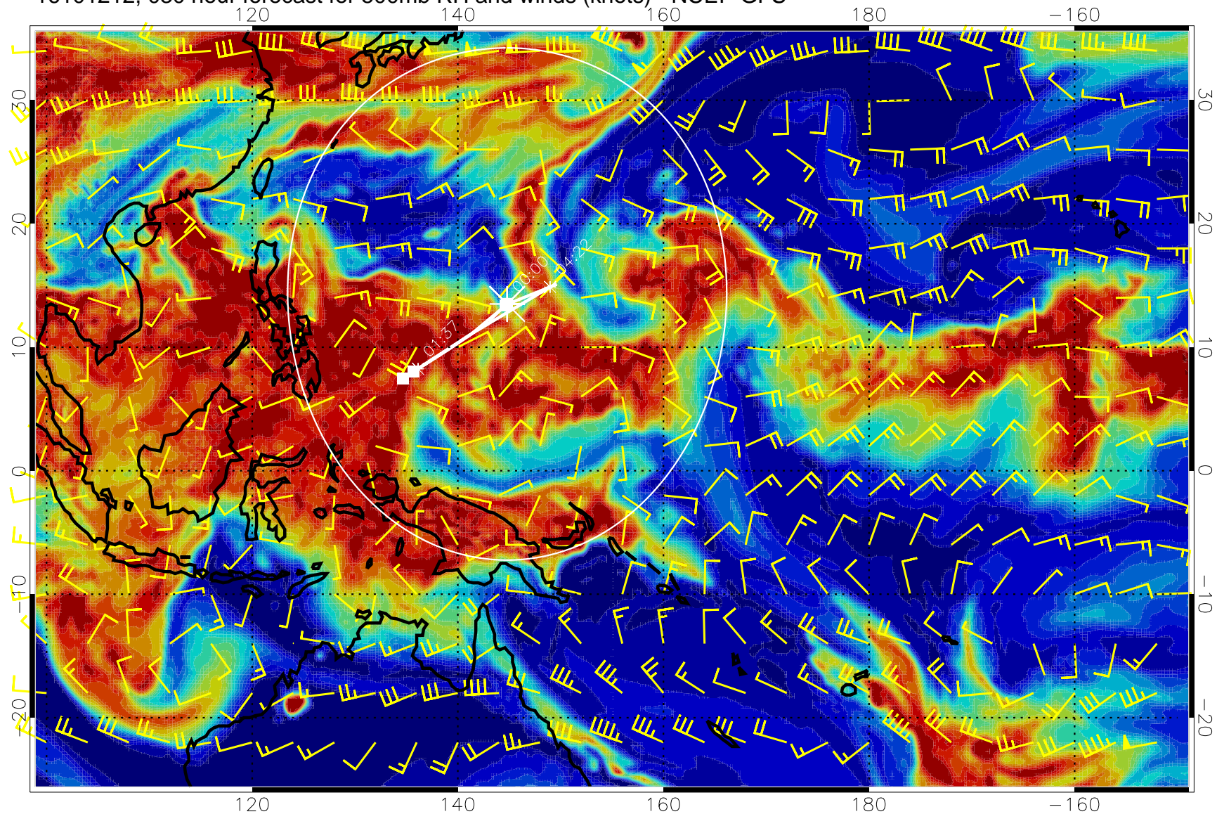
16101212, 030 hour forecast for 500mb RH and winds (knots) - NCEP GFS
