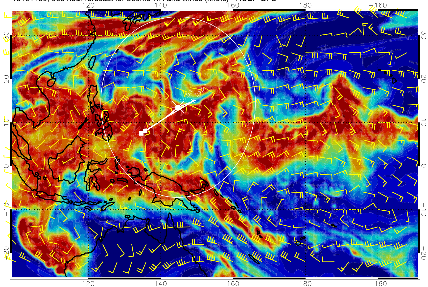
16101400, 066 hour forecast for 500mb RH and winds (knots) - NCEP GFS
