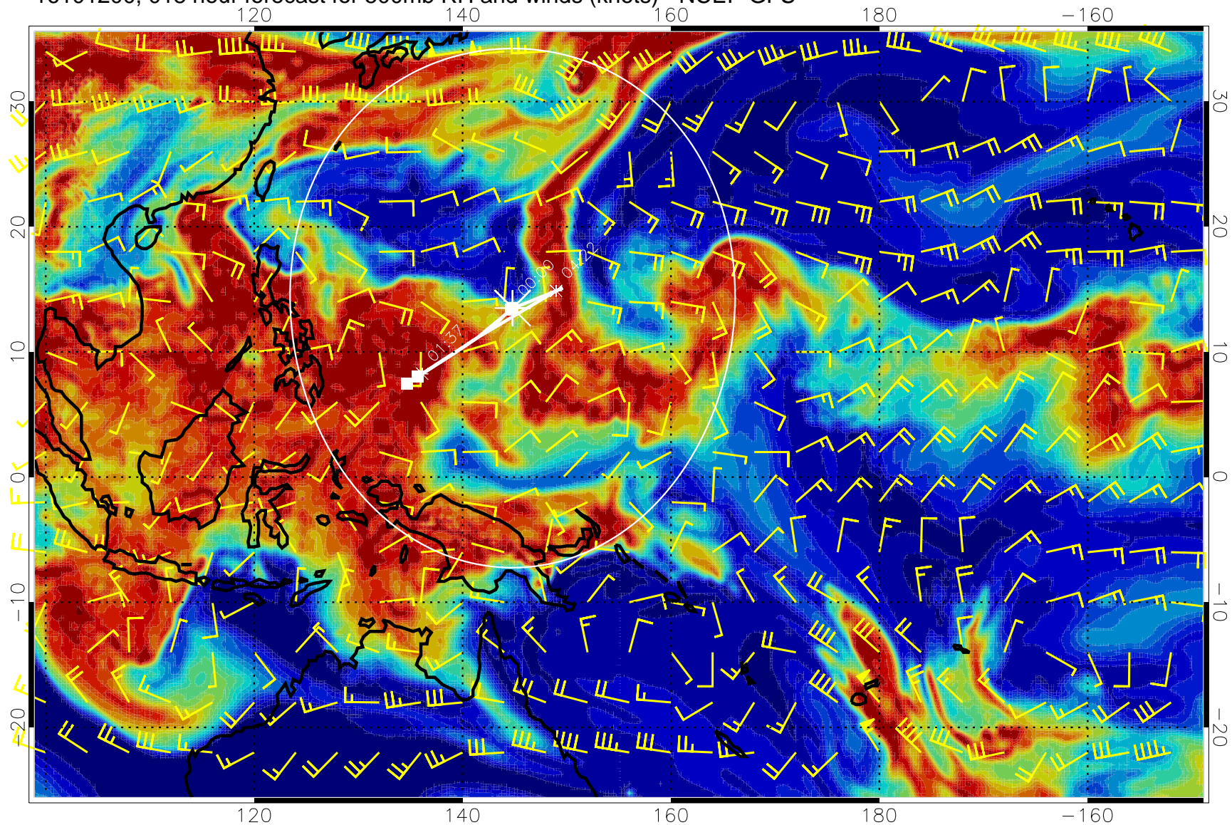
16101200, 018 hour forecast for 500mb RH and winds (knots) - NCEP GFS
