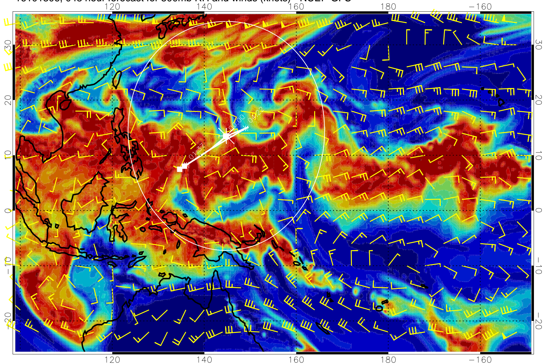
16101306, 048 hour forecast for 500mb RH and winds (knots) - NCEP GFS
