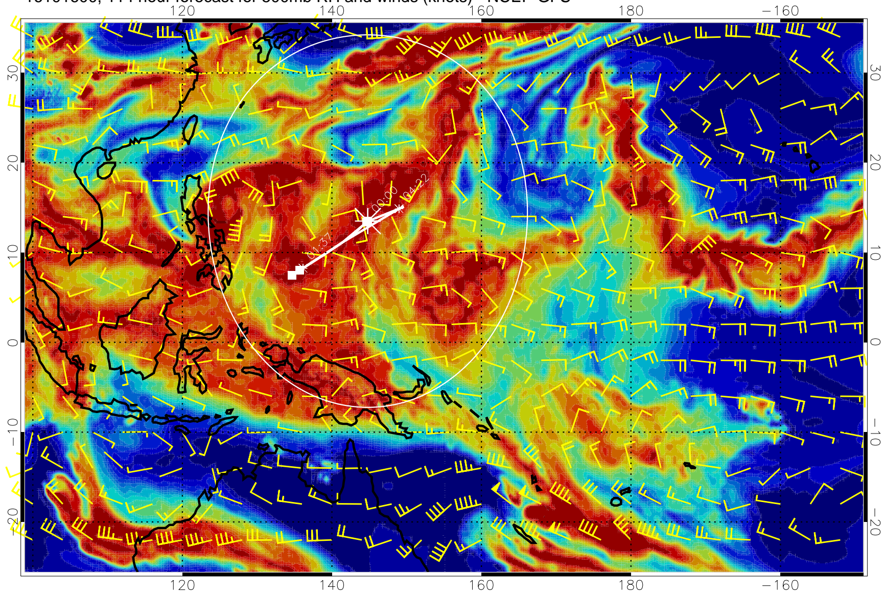
16101600, 114 hour forecast for 500mb RH and winds (knots) - NCEP GFS
