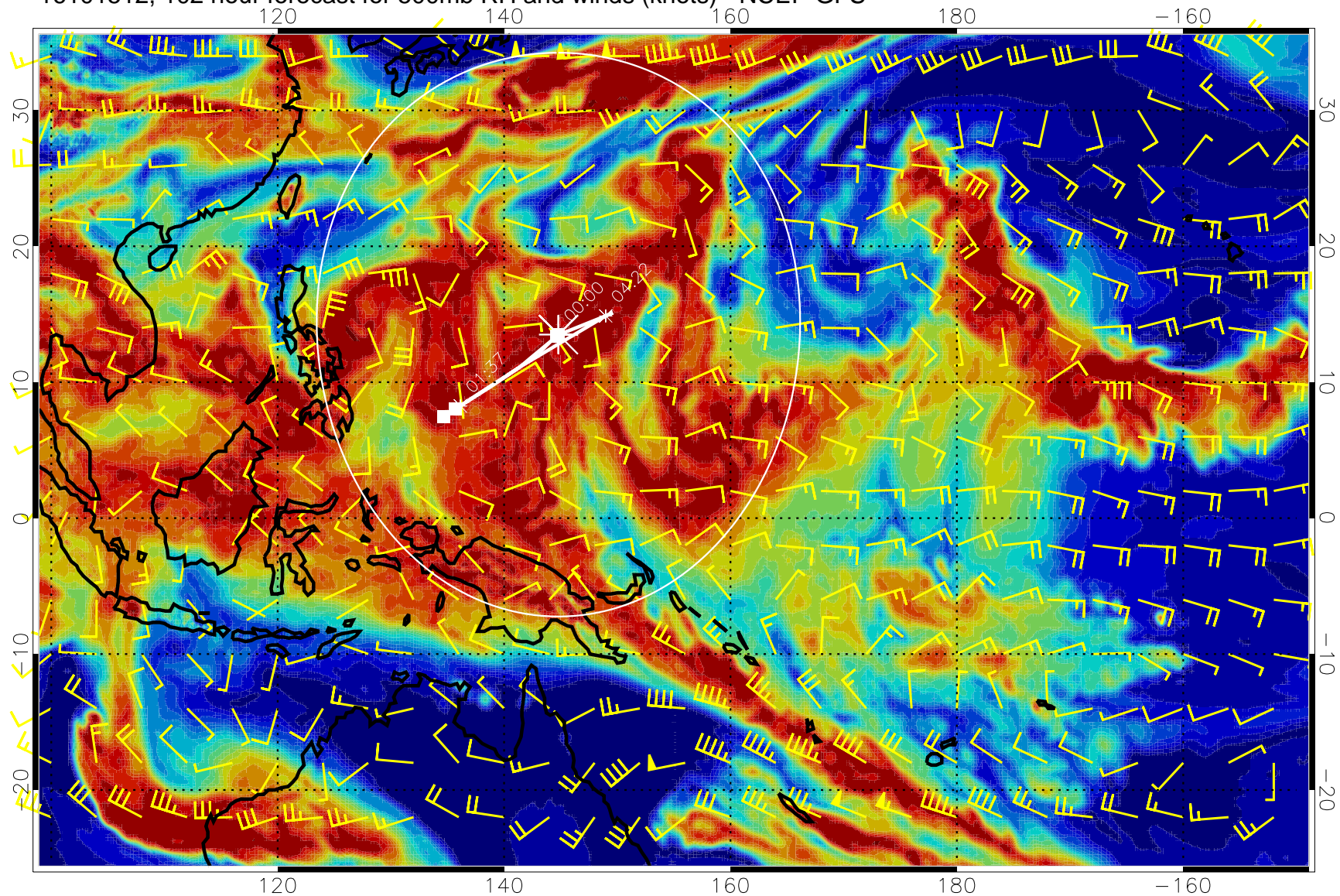
16101512, 102 hour forecast for 500mb RH and winds (knots) - NCEP GFS
