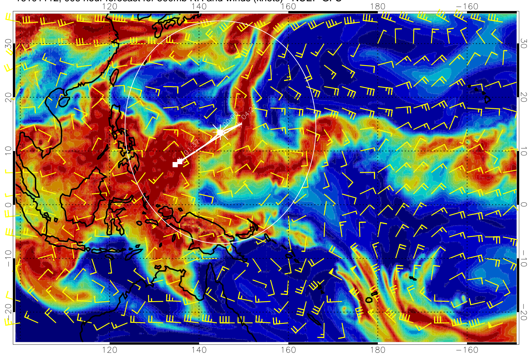
16101112, 006 hour forecast for 500mb RH and winds (knots) - NCEP GFS
