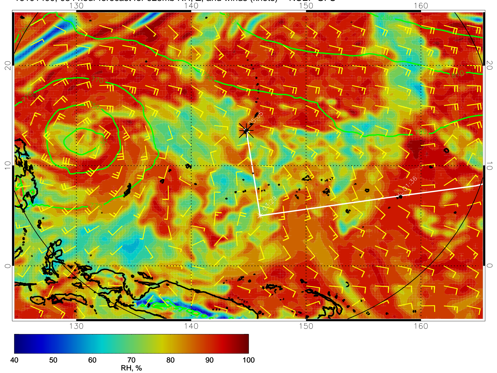
16101400, 084 hour forecast for 925mb RH, Z, and winds (knots) -- NCEP GFS
