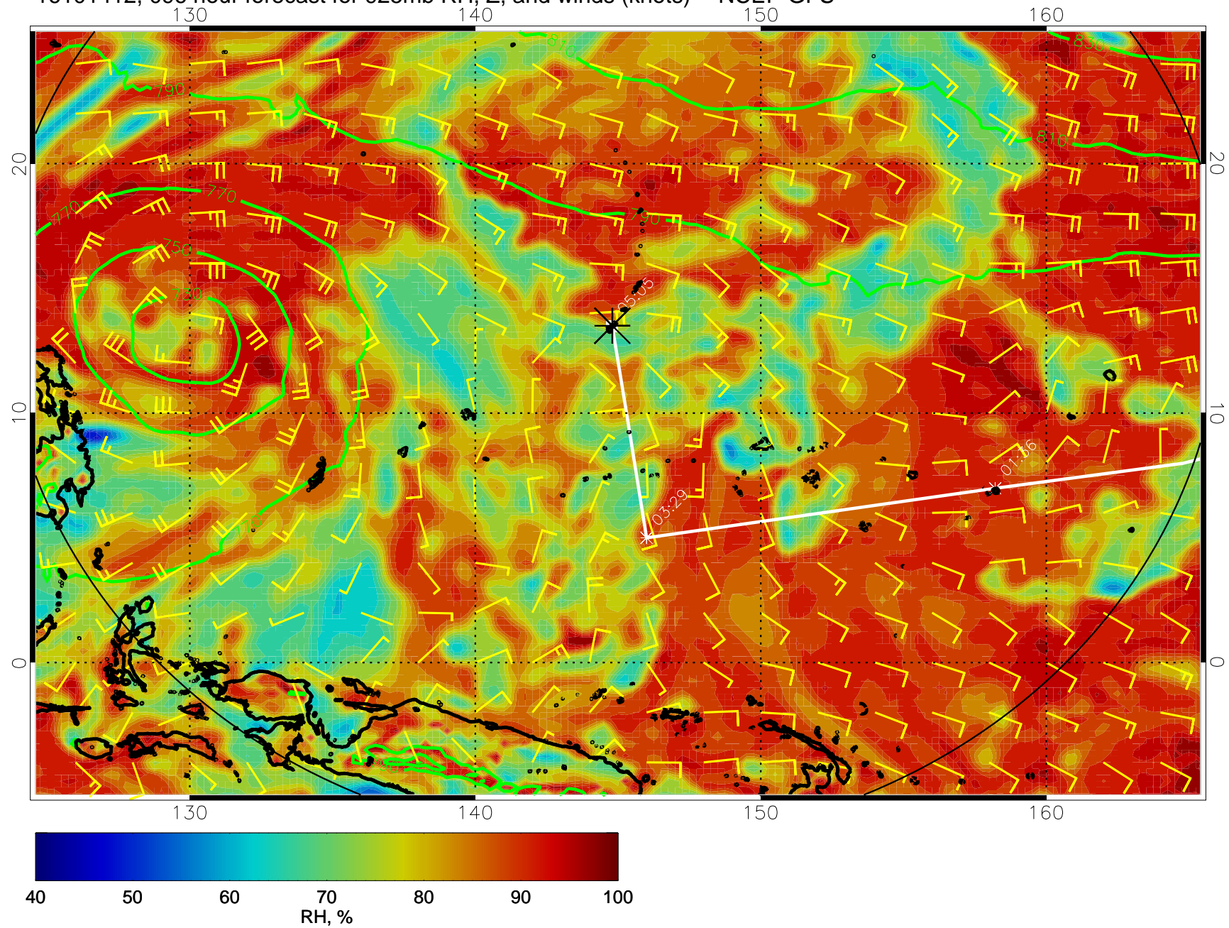
16101412, 096 hour forecast for 925mb RH, Z, and winds (knots) -- NCEP GFS
