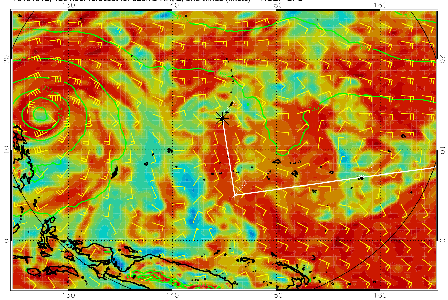
16101512, 120 hour forecast for 925mb RH, Z, and winds (knots) -- NCEP GFS
