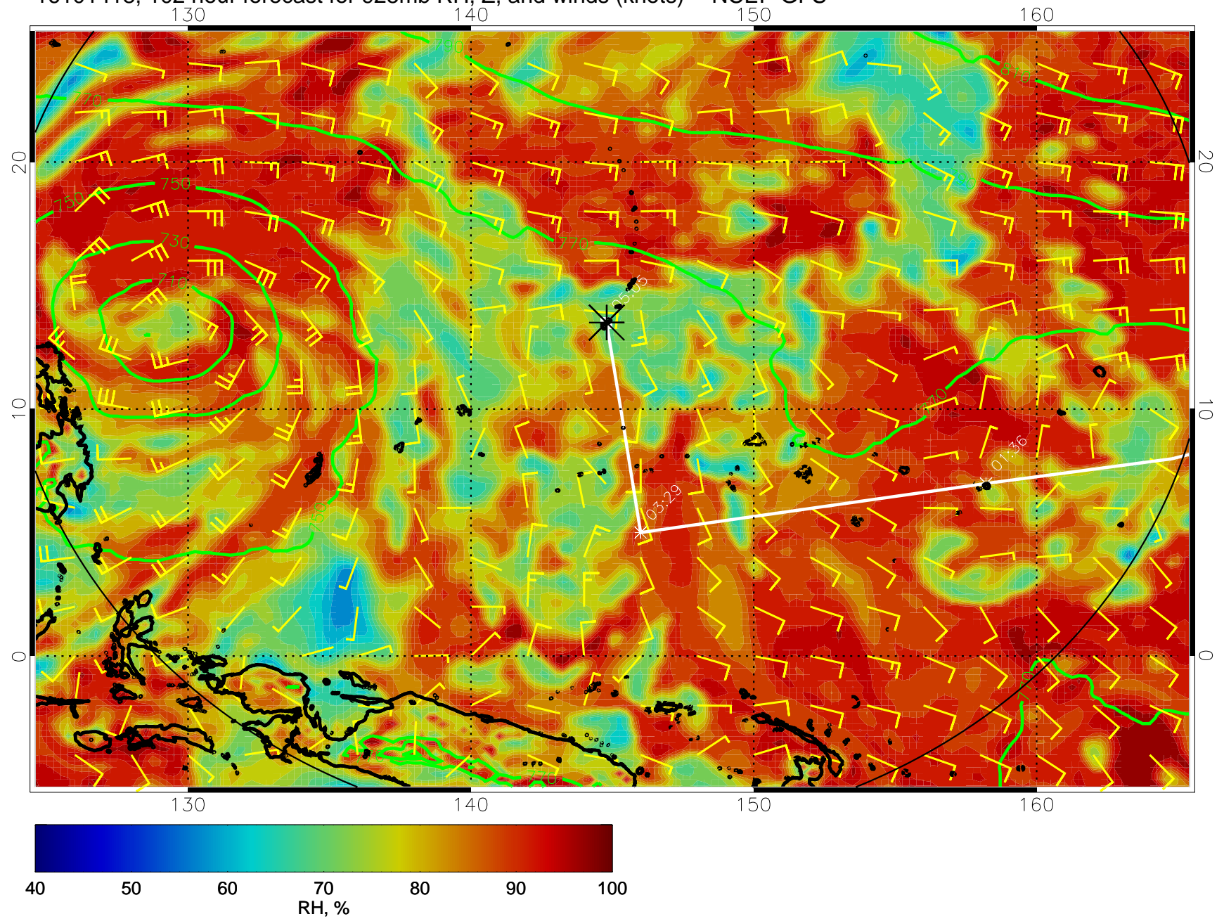
16101418, 102 hour forecast for 925mb RH, Z, and winds (knots) -- NCEP GFS
