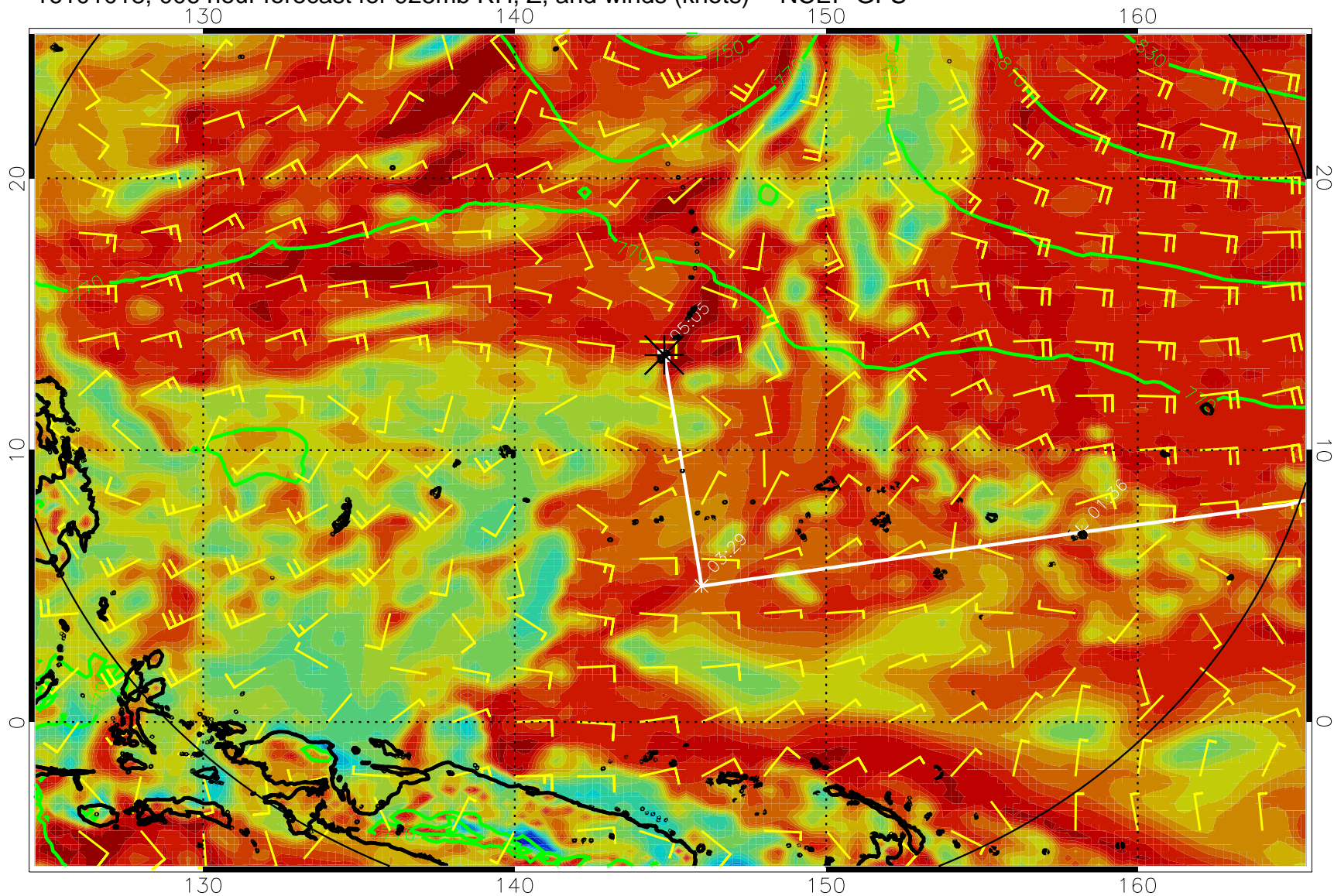
16101018, 006 hour forecast for 925mb RH, Z, and winds (knots) -- NCEP GFS
