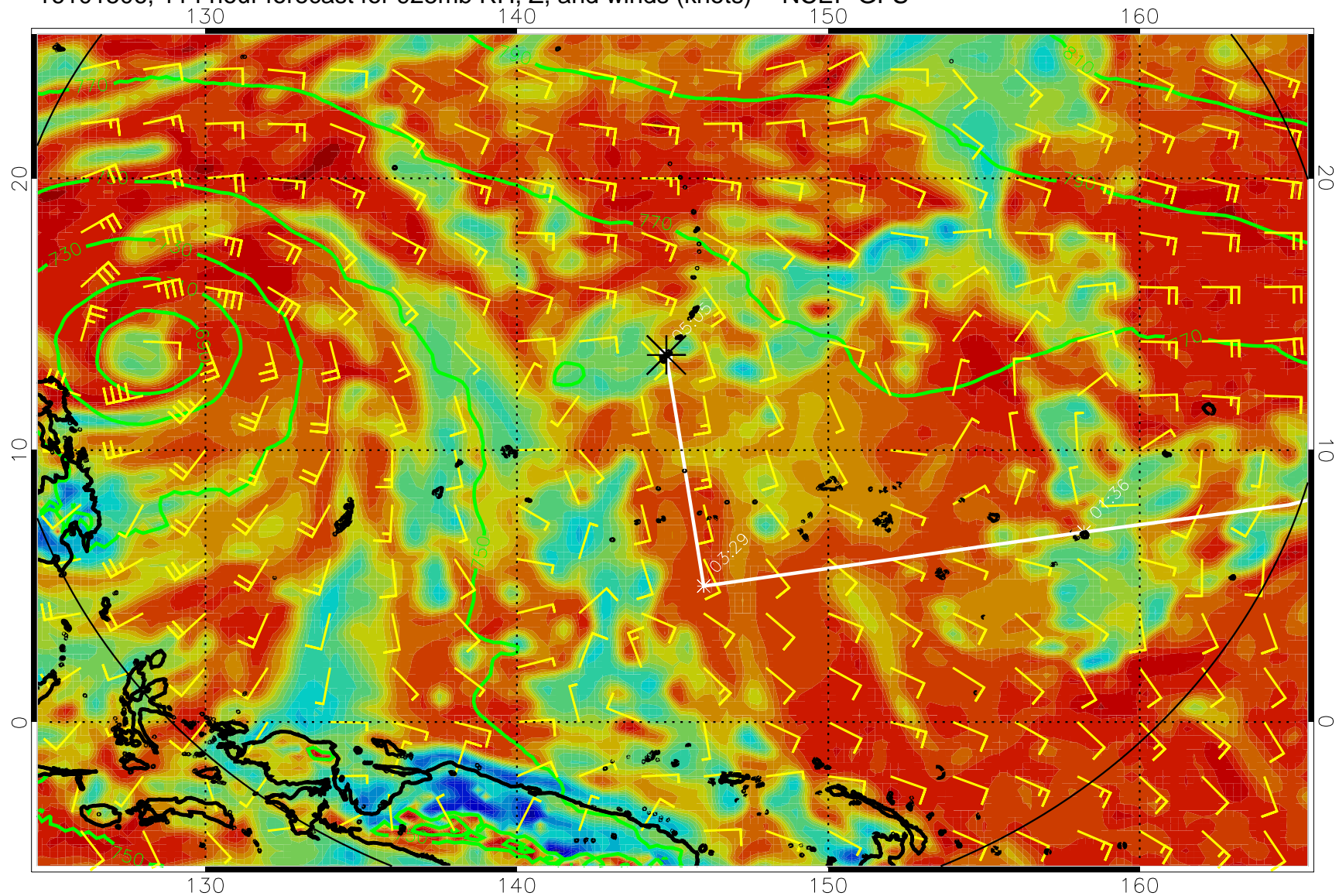
16101506, 114 hour forecast for 925mb RH, Z, and winds (knots) -- NCEP GFS
