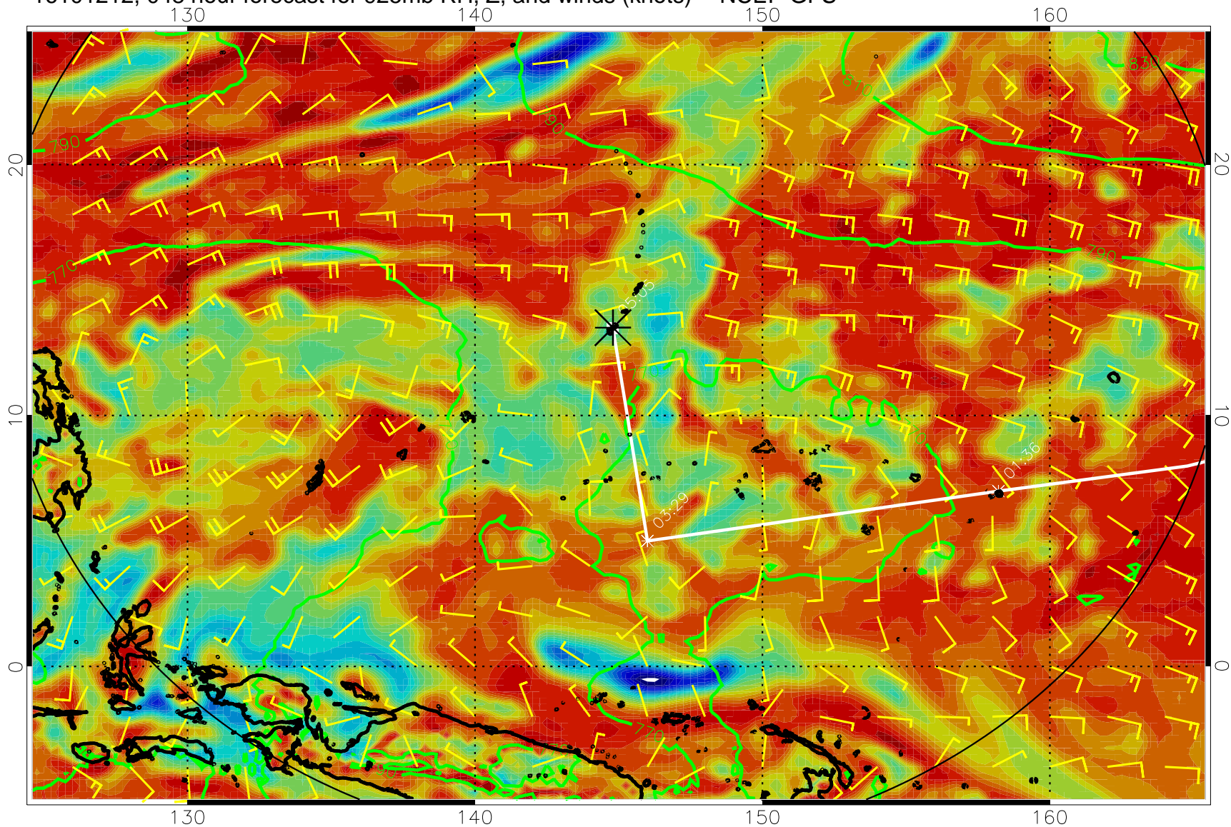
16101212, 048 hour forecast for 925mb RH, Z, and winds (knots) -- NCEP GFS
