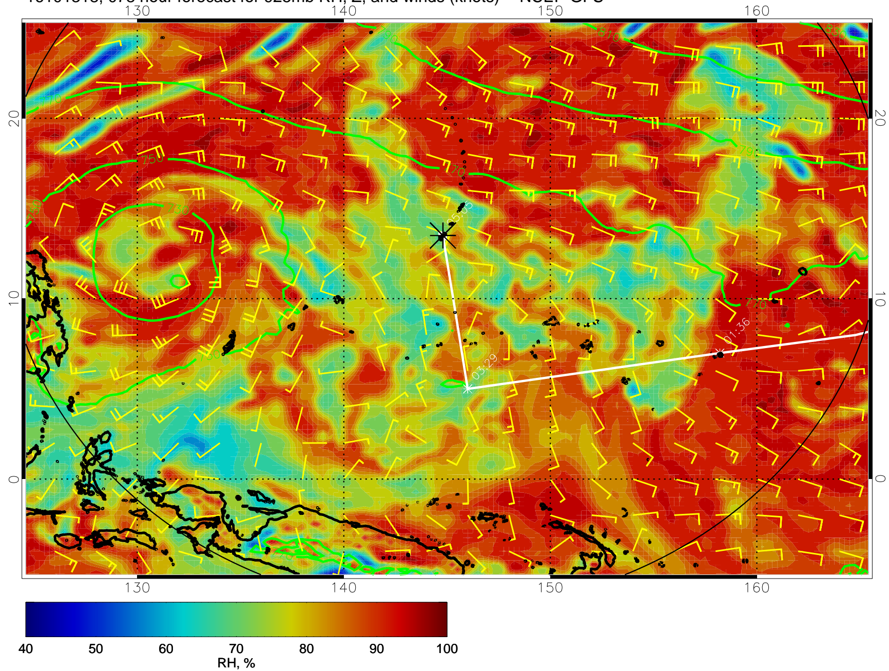
16101318, 078 hour forecast for 925mb RH, Z, and winds (knots) -- NCEP GFS
