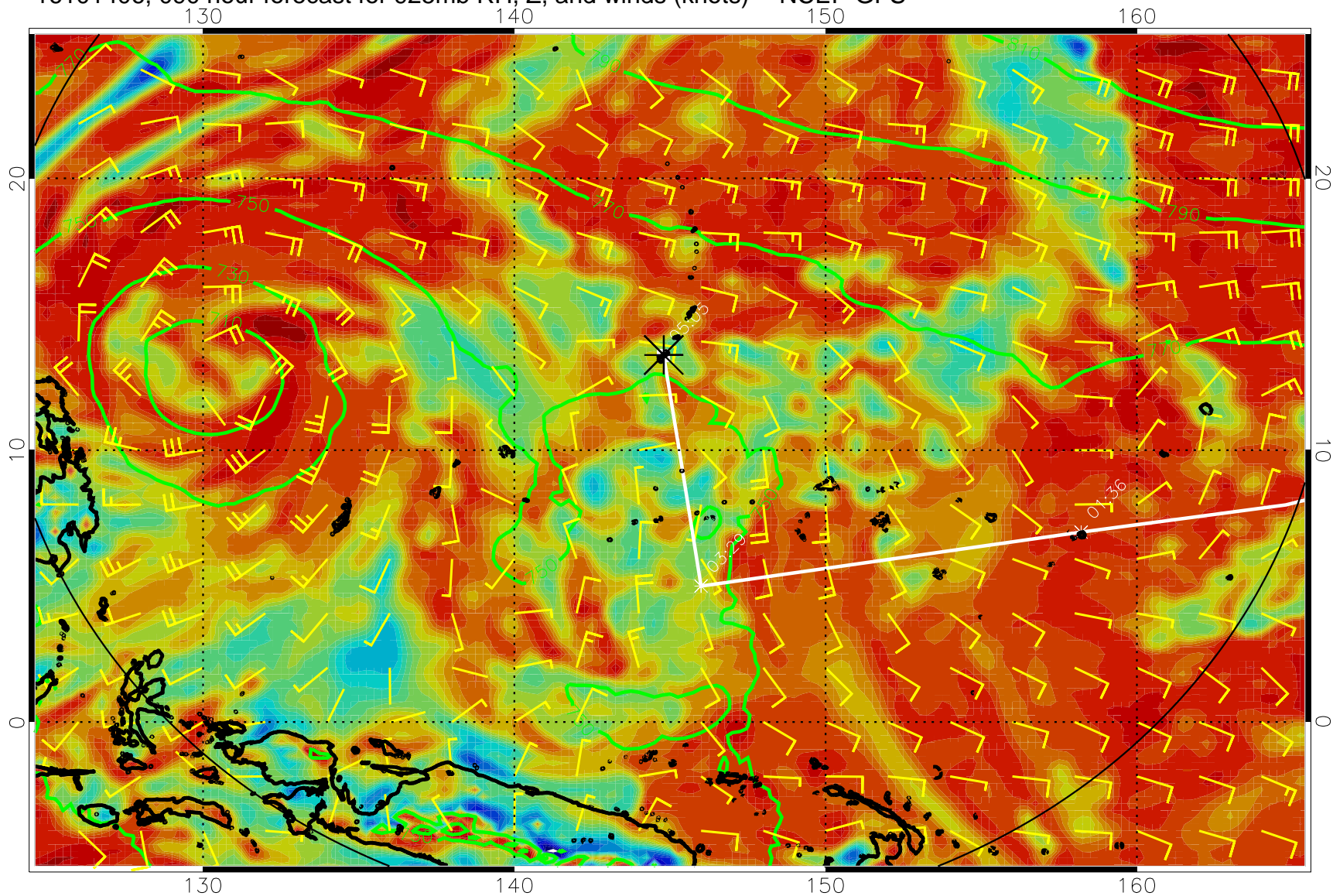
16101406, 090 hour forecast for 925mb RH, Z, and winds (knots) -- NCEP GFS
