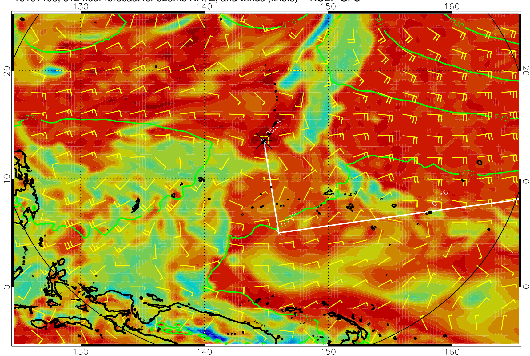
16101100, 012 hour forecast for 925mb RH, Z, and winds (knots) -- NCEP GFS
