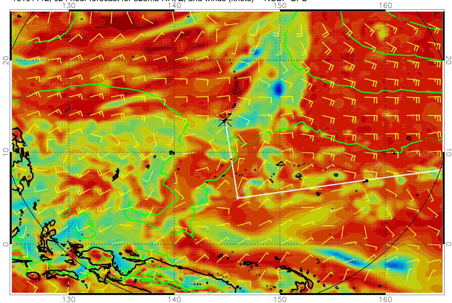
16101112, 024 hour forecast for 925mb RH, Z, and winds (knots) -- NCEP GFS
