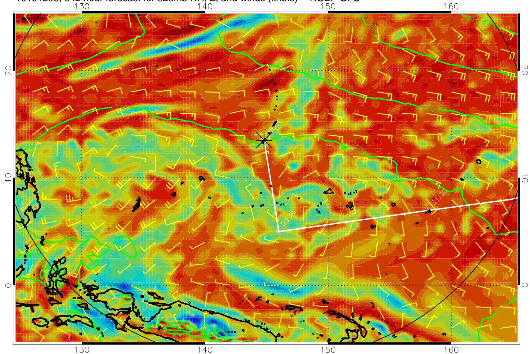
16101206, 042 hour forecast for 925mb RH, Z, and winds (knots) -- NCEP GFS
