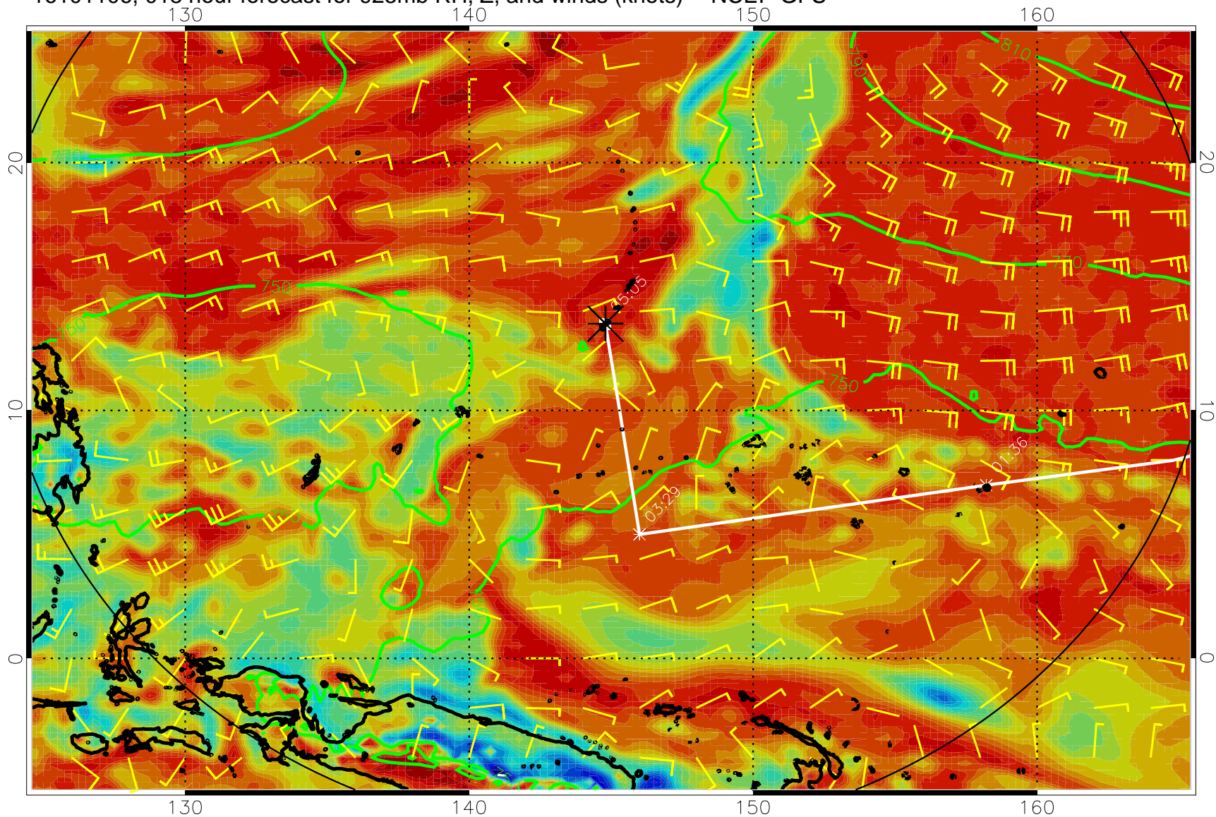
16101106, 018 hour forecast for 925mb RH, Z, and winds (knots) -- NCEP GFS
