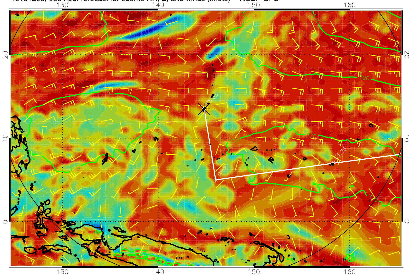
16101200, 036 hour forecast for 925mb RH, Z, and winds (knots) -- NCEP GFS
