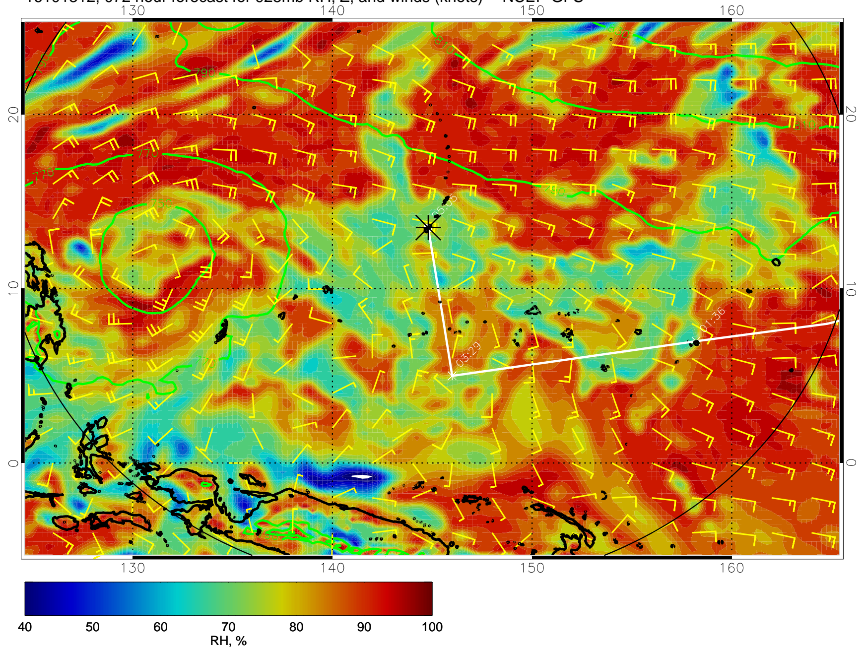
16101312, 072 hour forecast for 925mb RH, Z, and winds (knots) -- NCEP GFS
