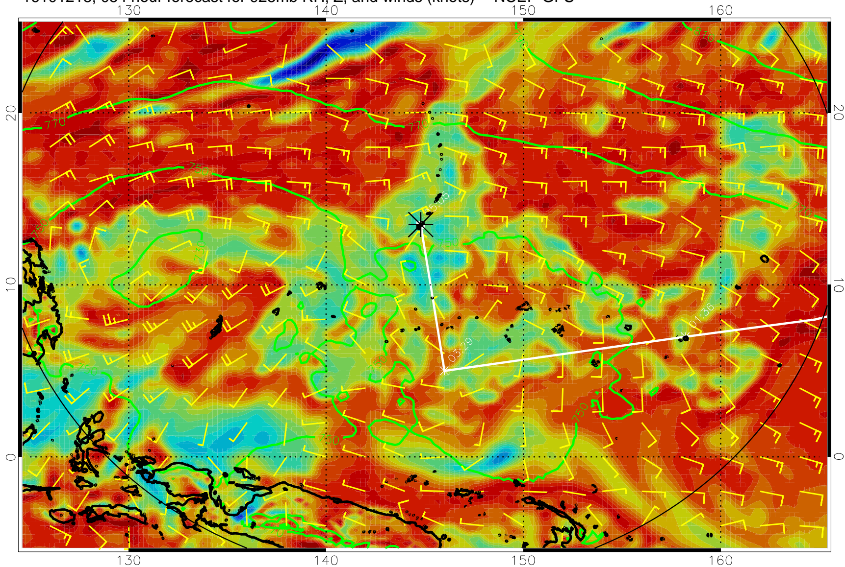
16101218, 054 hour forecast for 925mb RH, Z, and winds (knots) -- NCEP GFS
