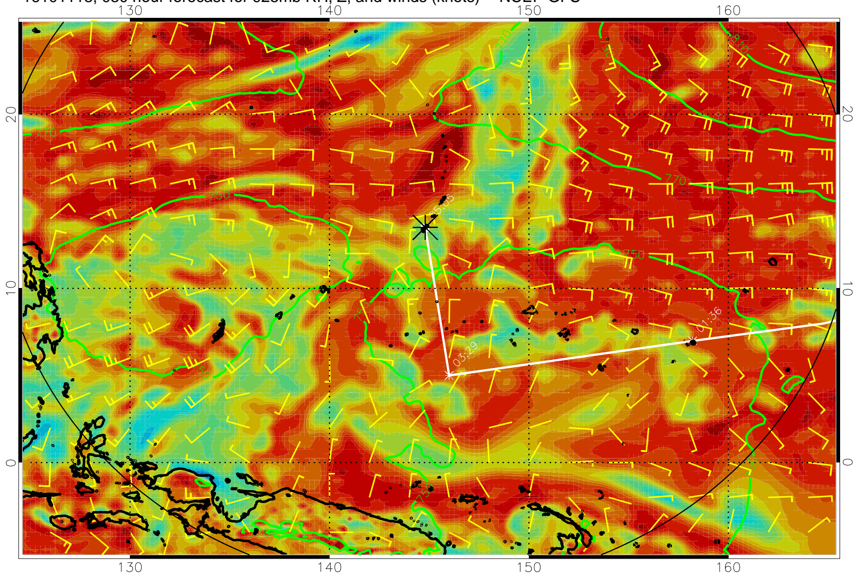
16101118, 030 hour forecast for 925mb RH, Z, and winds (knots) -- NCEP GFS
