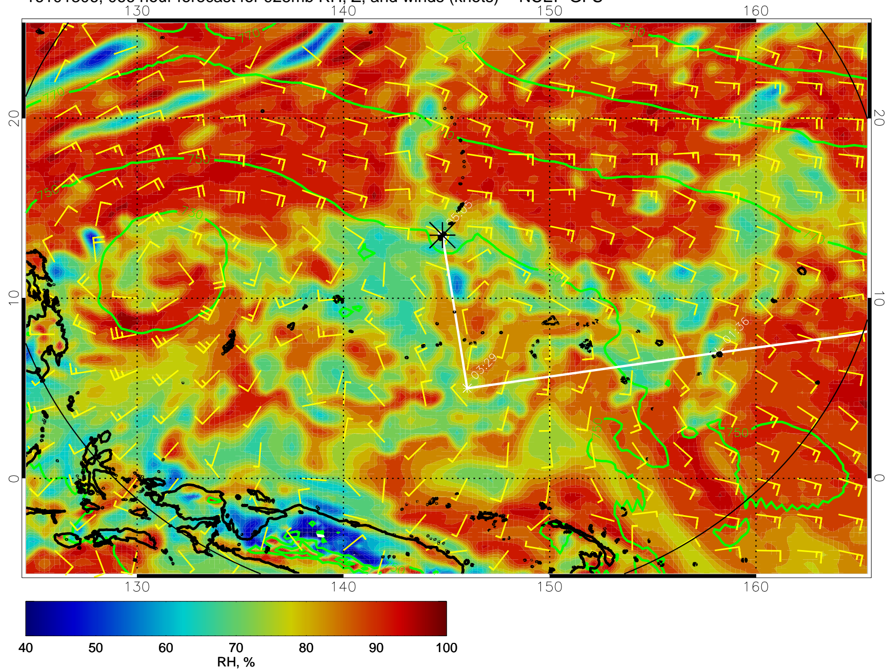
16101306, 066 hour forecast for 925mb RH, Z, and winds (knots) -- NCEP GFS
