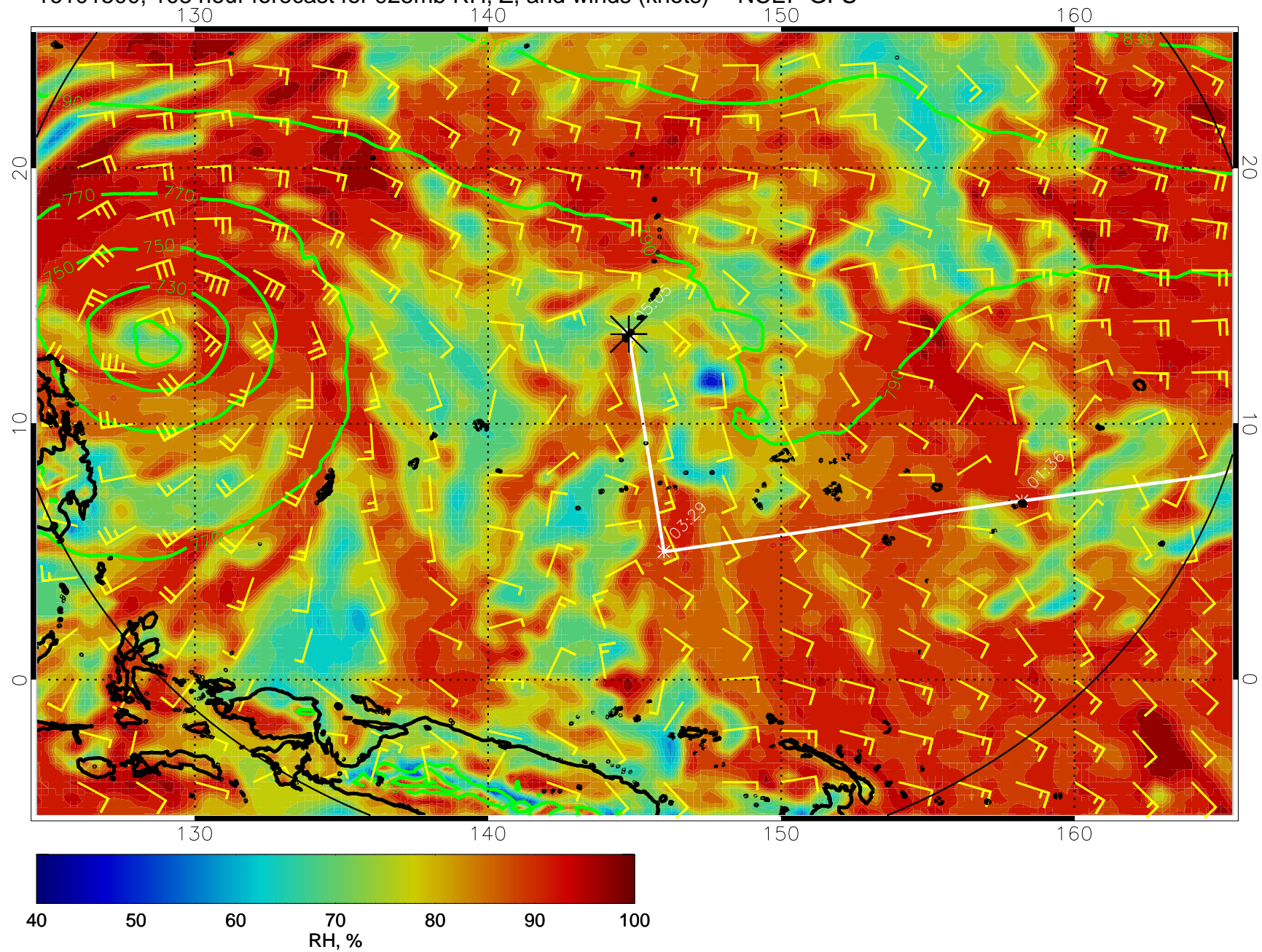
16101500, 108 hour forecast for 925mb RH, Z, and winds (knots) -- NCEP GFS
