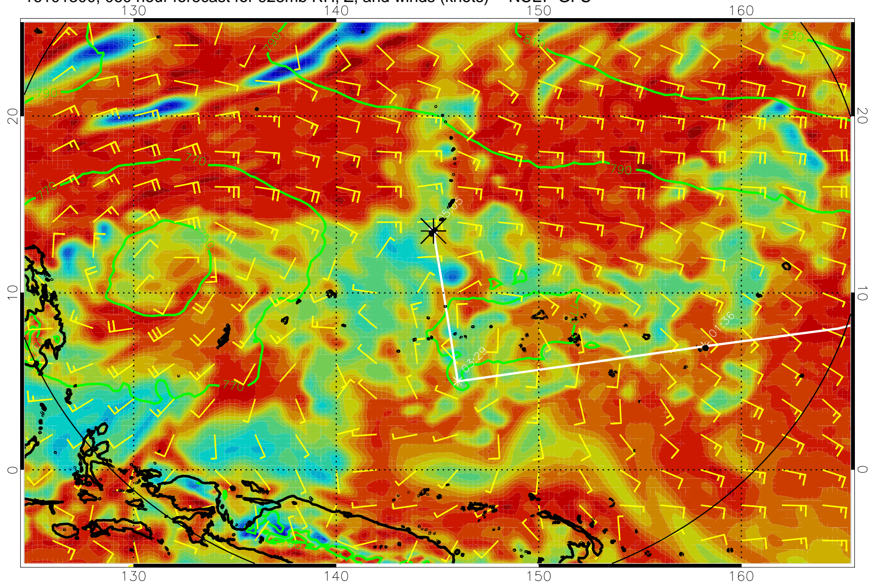
16101300, 060 hour forecast for 925mb RH, Z, and winds (knots) -- NCEP GFS
