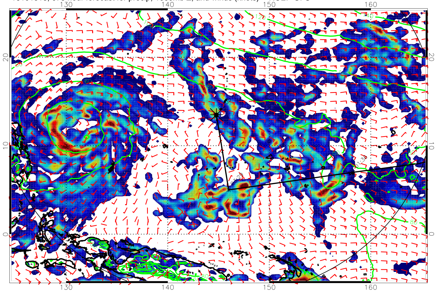
16101318, 078 hour forecast for precip, 1000mb Z, and winds (knots) -- NCEP GFS
