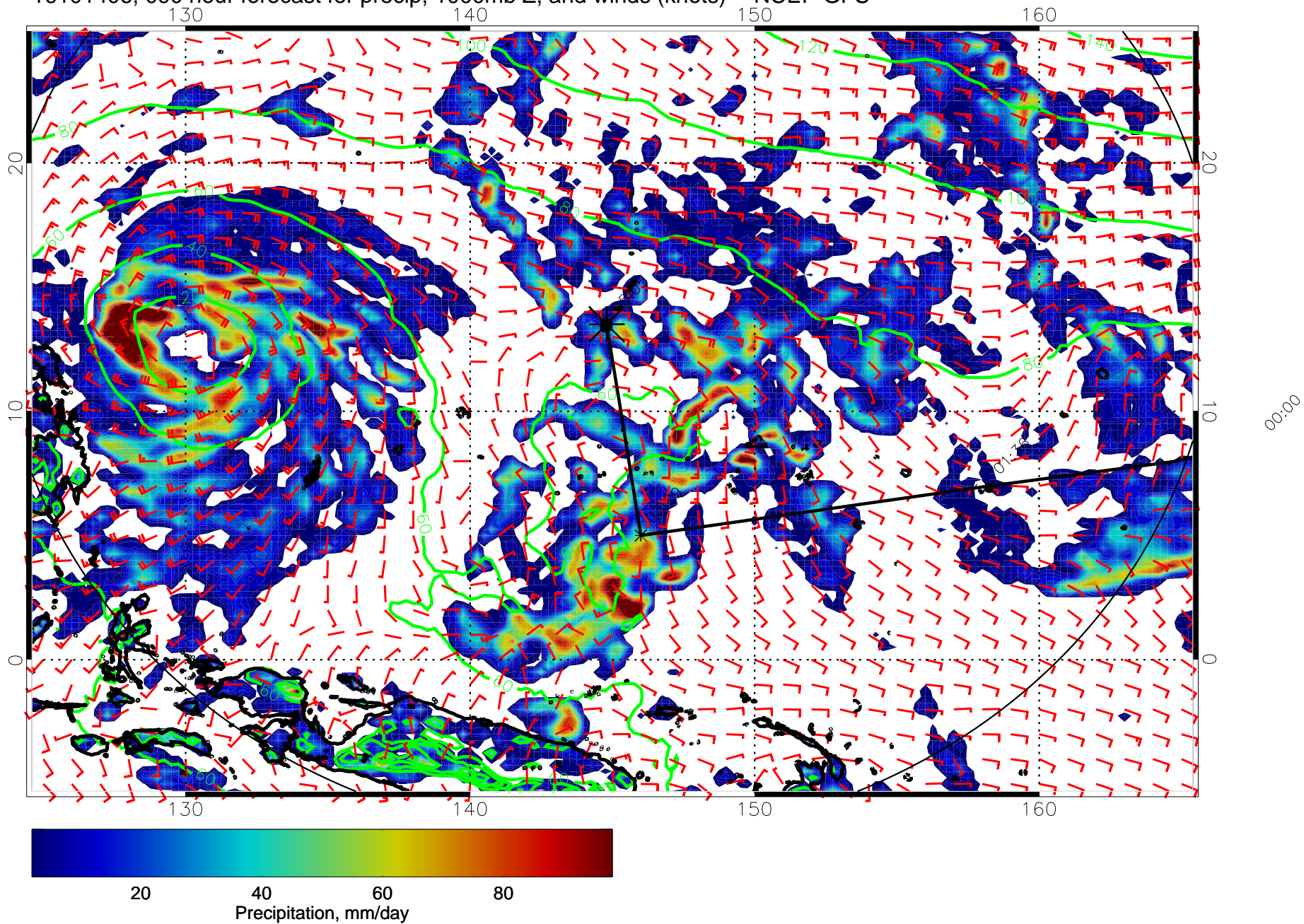
16101406, 090 hour forecast for precip, 1000mb Z, and winds (knots) -- NCEP GFS
