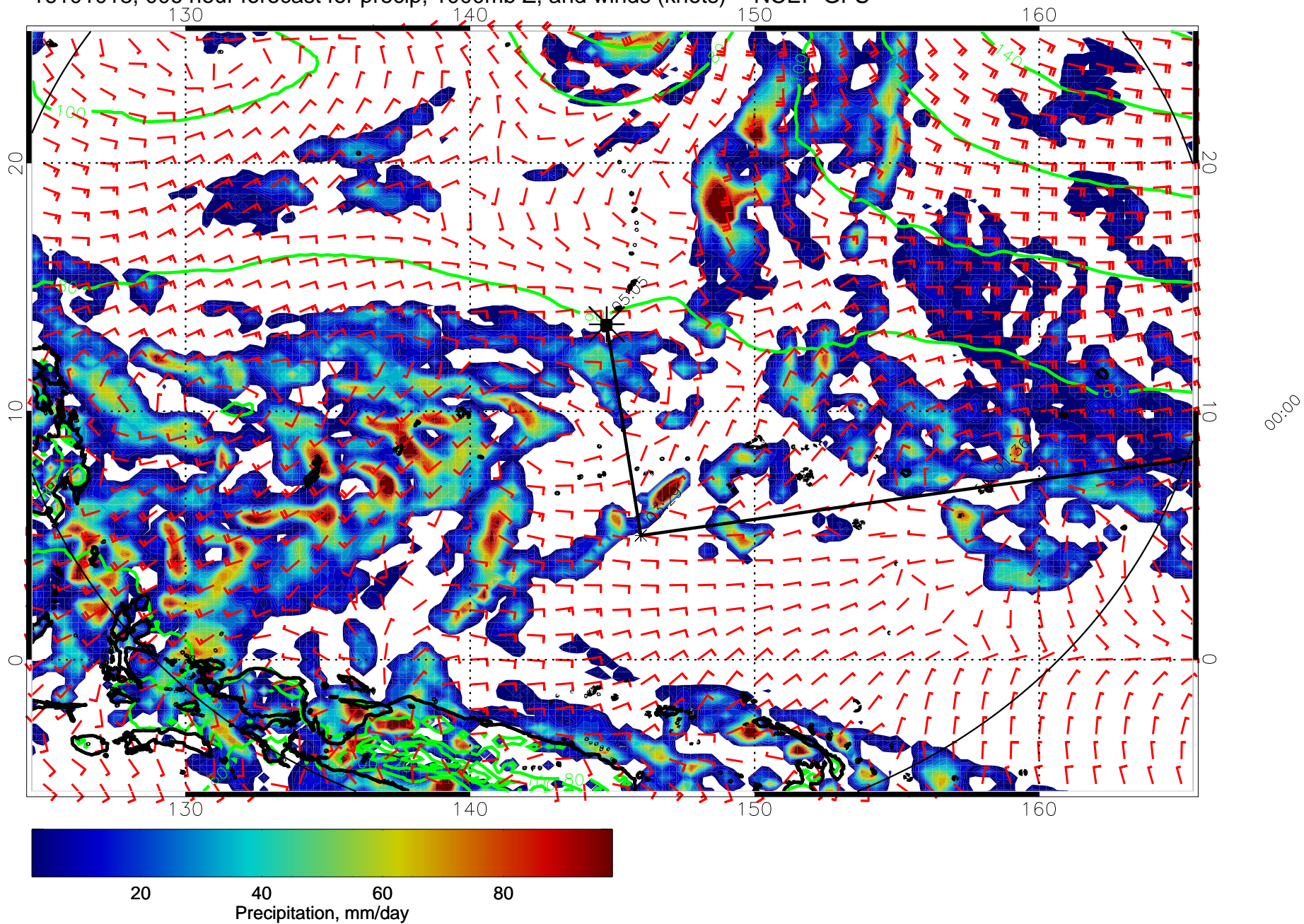
16101018, 006 hour forecast for precip, 1000mb Z, and winds (knots) -- NCEP GFS
