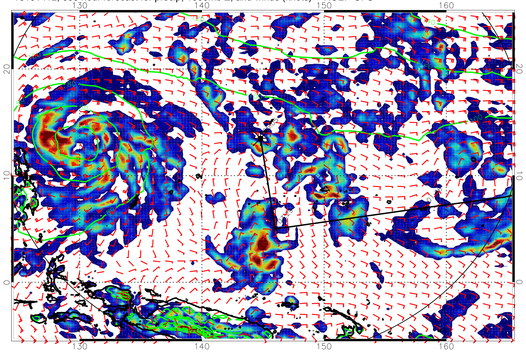
16101412, 096 hour forecast for precip, 1000mb Z, and winds (knots) -- NCEP GFS
