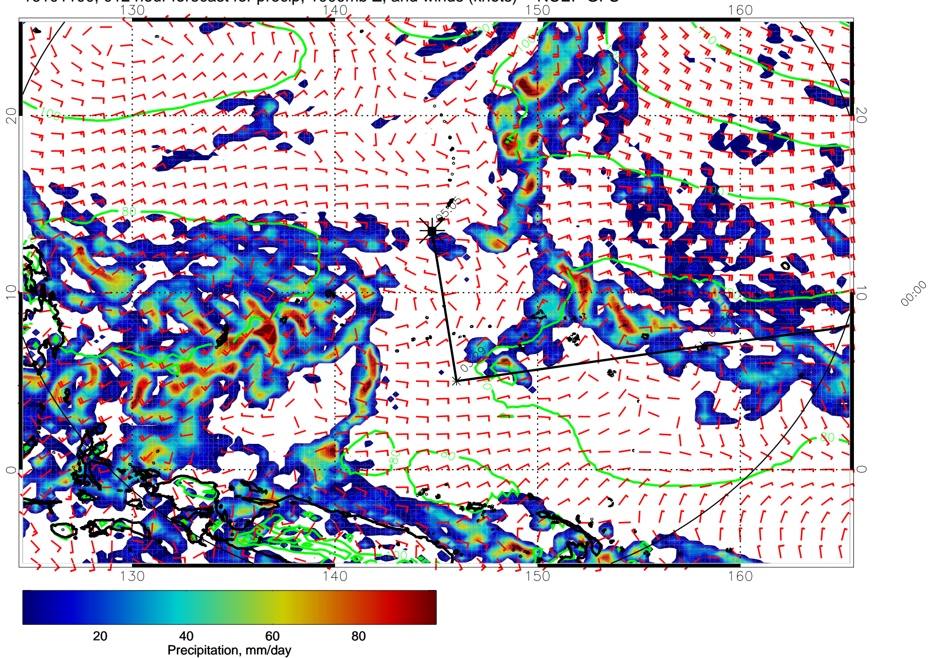
16101100, 012 hour forecast for precip, 1000mb Z, and winds (knots) -- NCEP GFS
