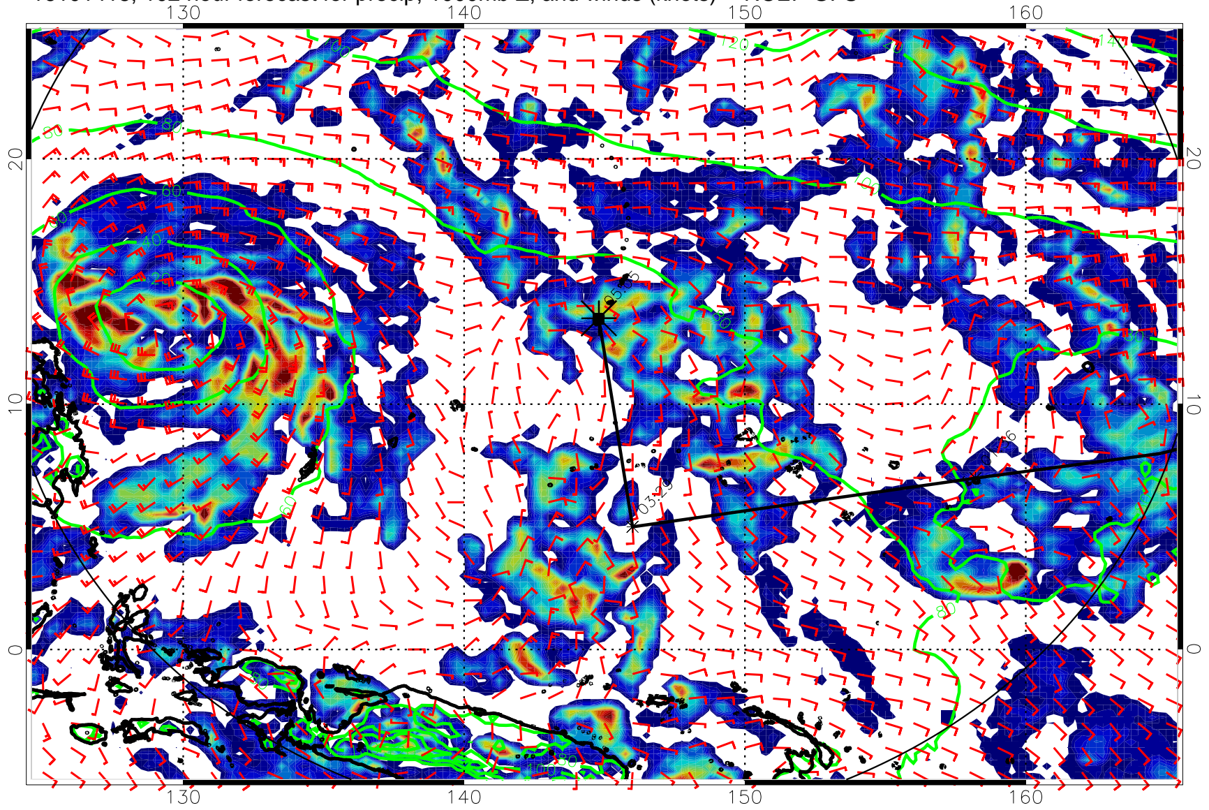
16101418, 102 hour forecast for precip, 1000mb Z, and winds (knots) -- NCEP GFS
