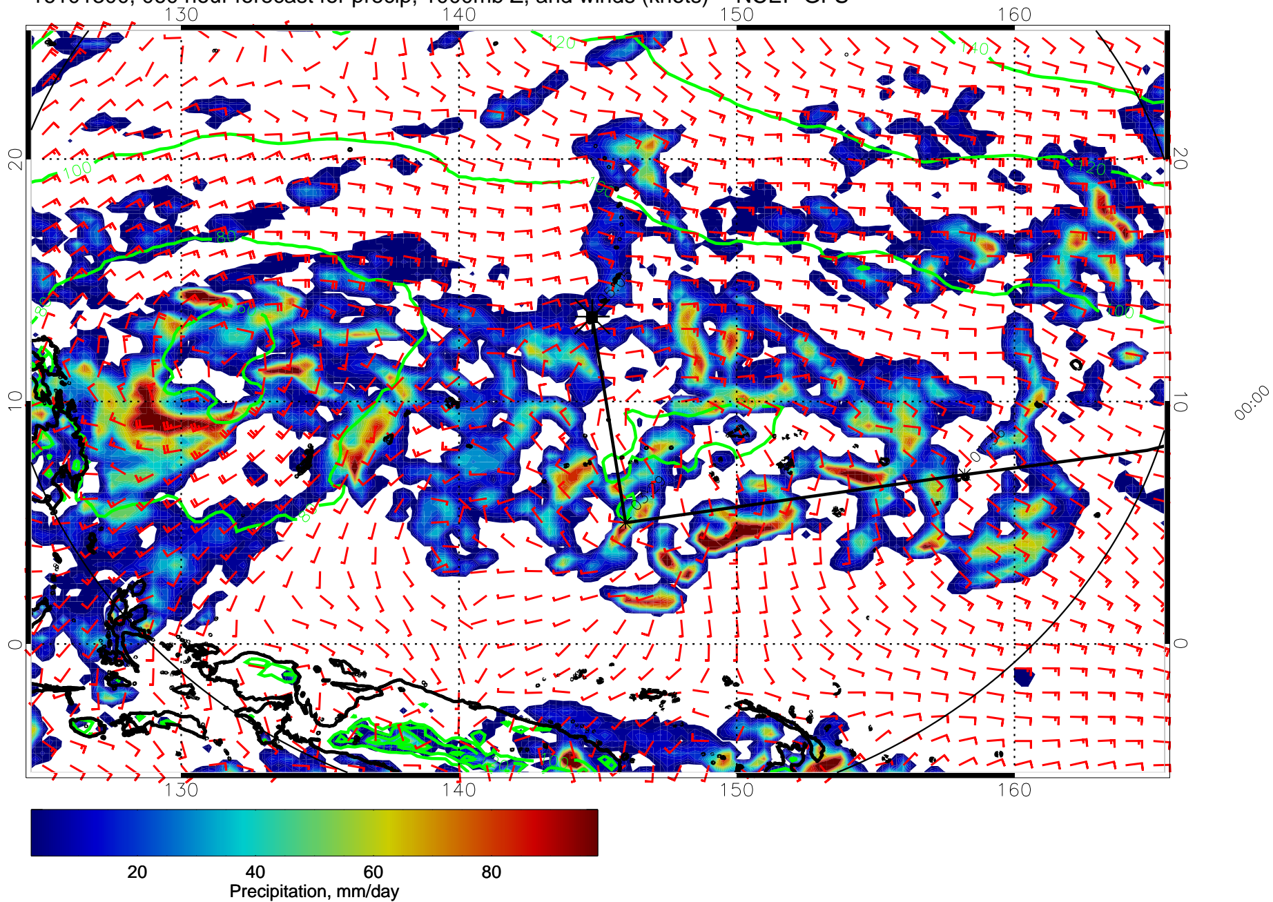
16101300, 060 hour forecast for precip, 1000mb Z, and winds (knots) -- NCEP GFS
