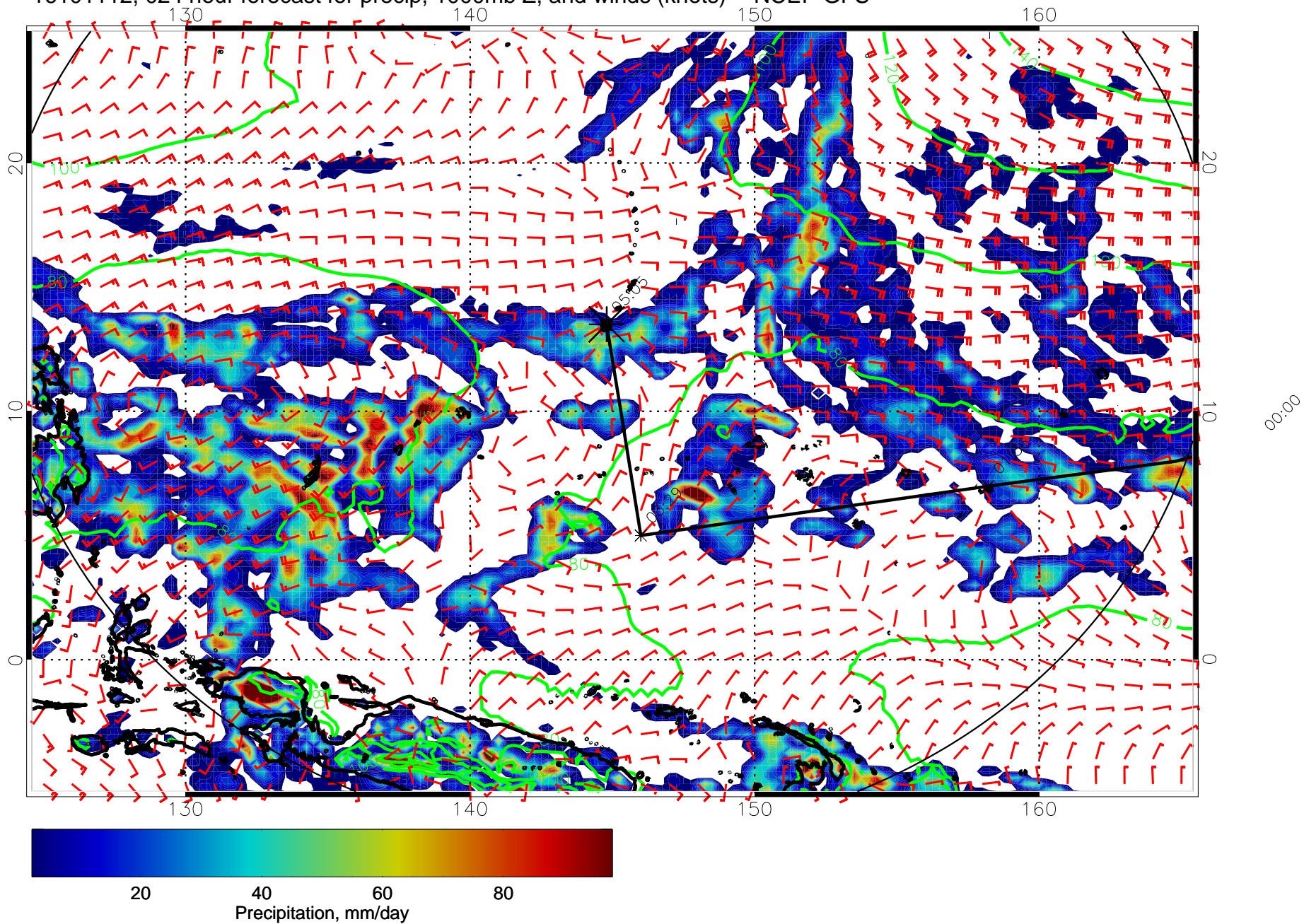
16101112, 024 hour forecast for precip, 1000mb Z, and winds (knots) -- NCEP GFS
