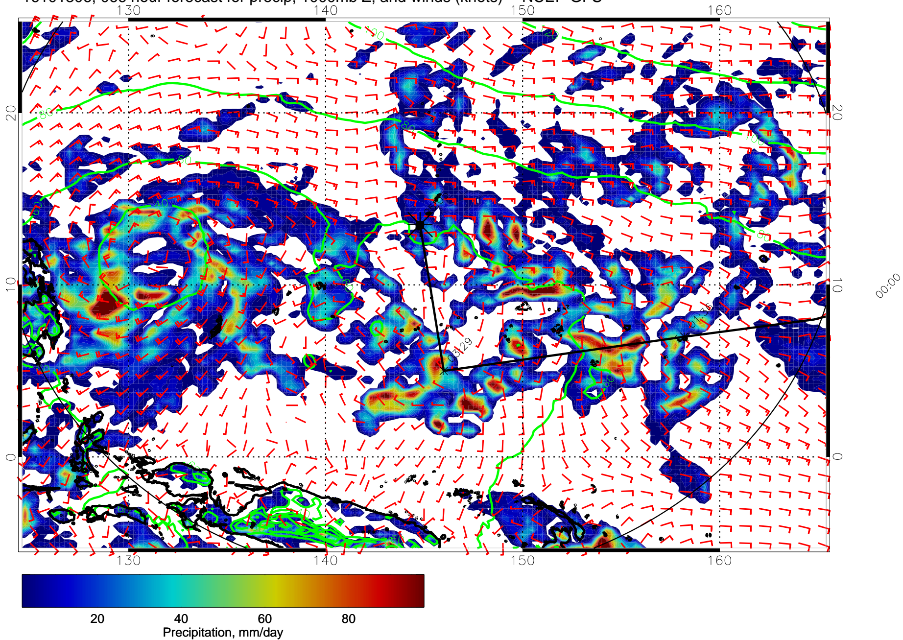
16101306, 066 hour forecast for precip, 1000mb Z, and winds (knots) -- NCEP GFS
