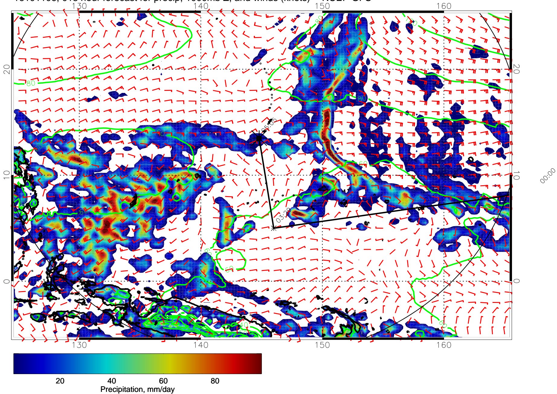
16101106, 018 hour forecast for precip, 1000mb Z, and winds (knots) -- NCEP GFS
