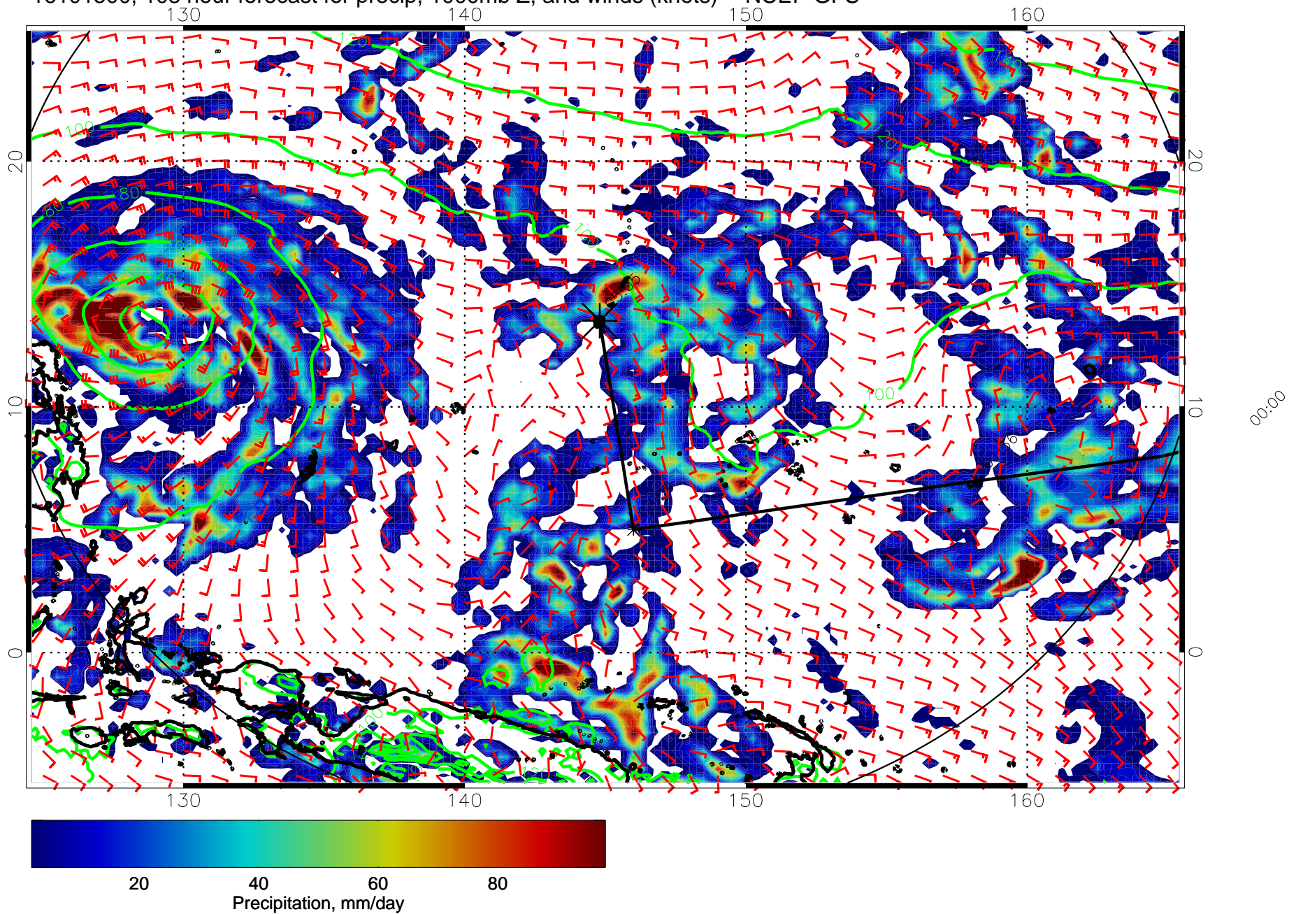
16101500, 108 hour forecast for precip, 1000mb Z, and winds (knots) -- NCEP GFS
