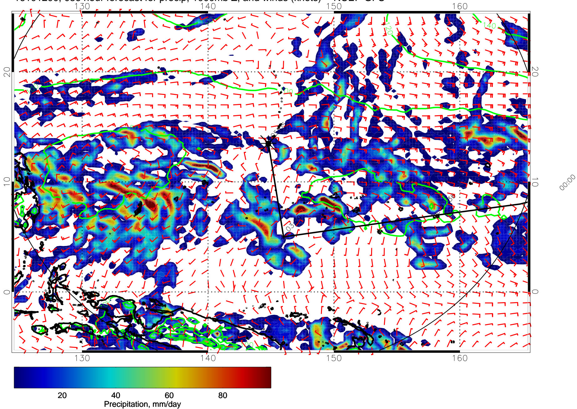
16101200, 036 hour forecast for precip, 1000mb Z, and winds (knots) -- NCEP GFS
