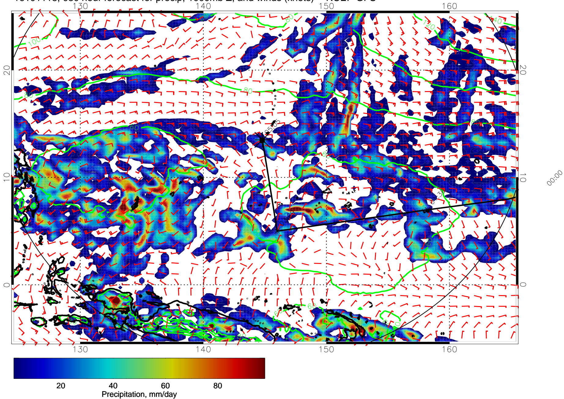
16101118, 030 hour forecast for precip, 1000mb Z, and winds (knots) -- NCEP GFS
