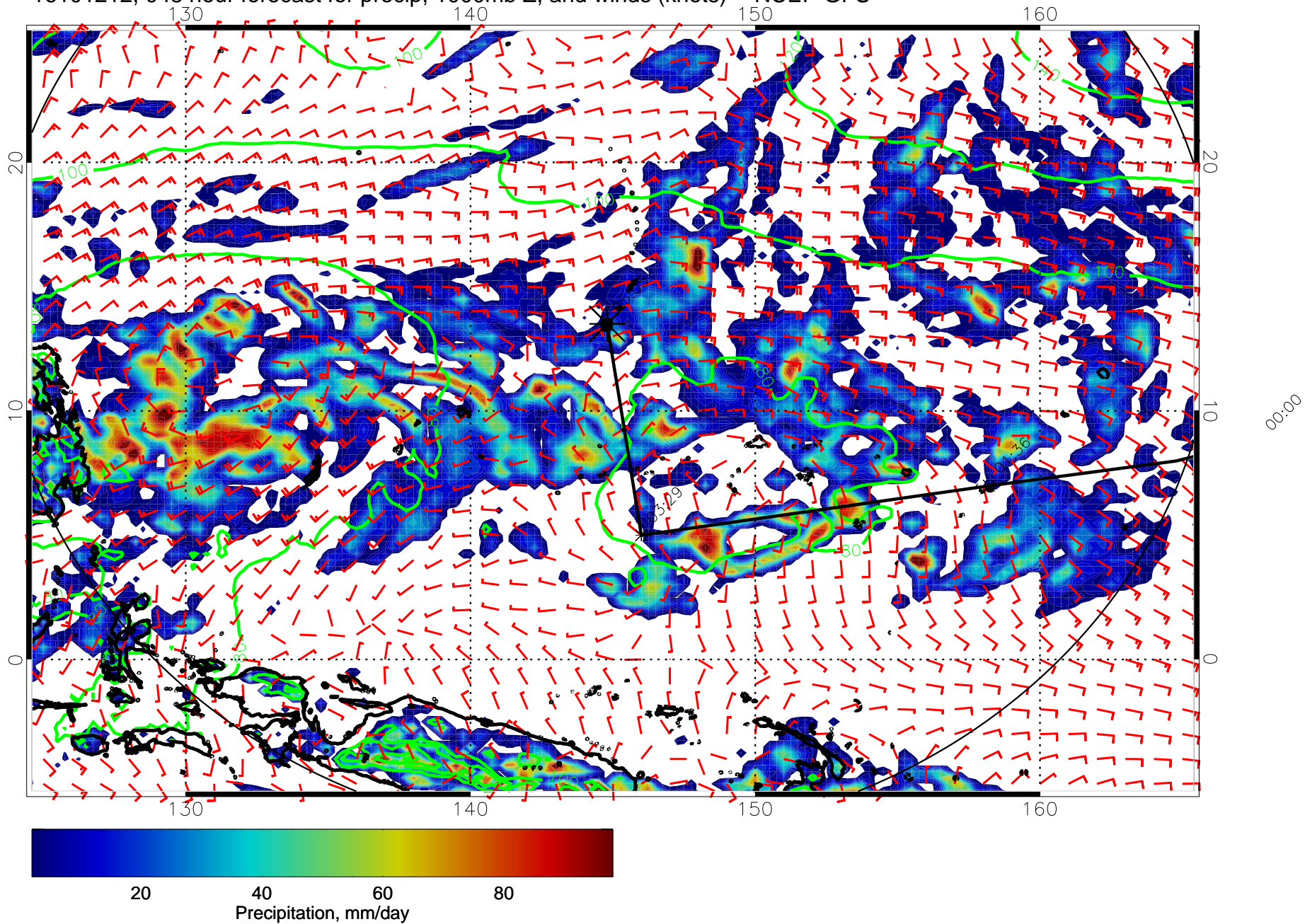
16101212, 048 hour forecast for precip, 1000mb Z, and winds (knots) -- NCEP GFS
