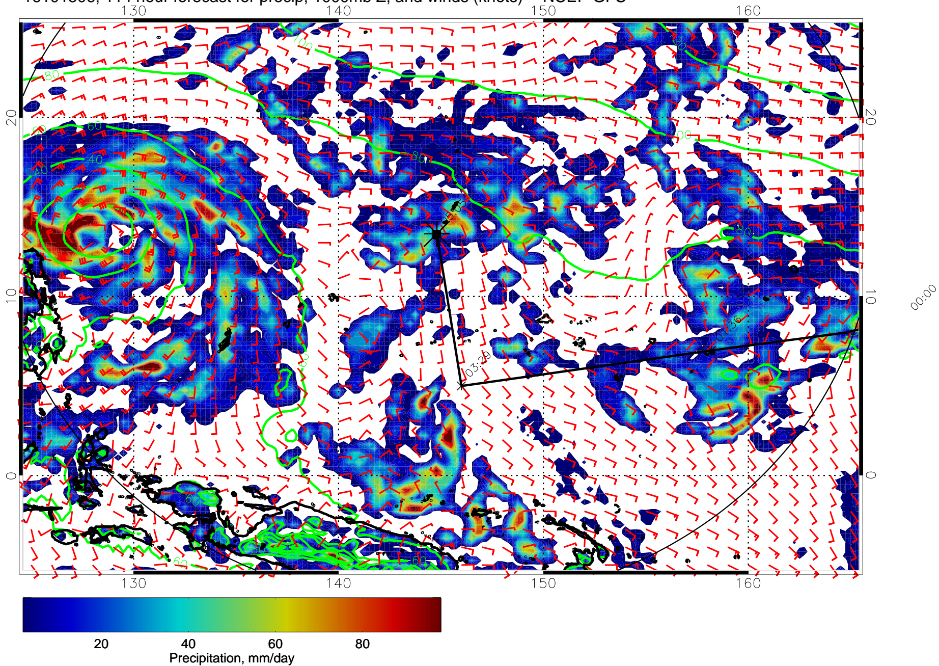
16101506, 114 hour forecast for precip, 1000mb Z, and winds (knots) -- NCEP GFS
