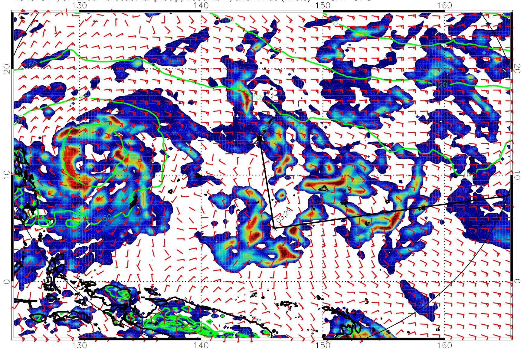
16101312, 072 hour forecast for precip, 1000mb Z, and winds (knots) -- NCEP GFS
