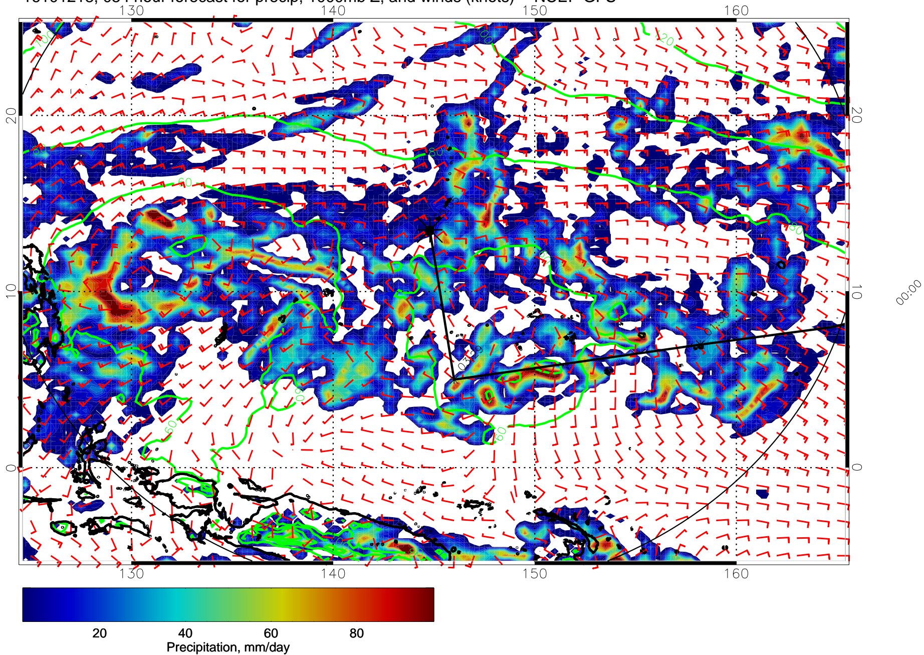
16101218, 054 hour forecast for precip, 1000mb Z, and winds (knots) -- NCEP GFS
