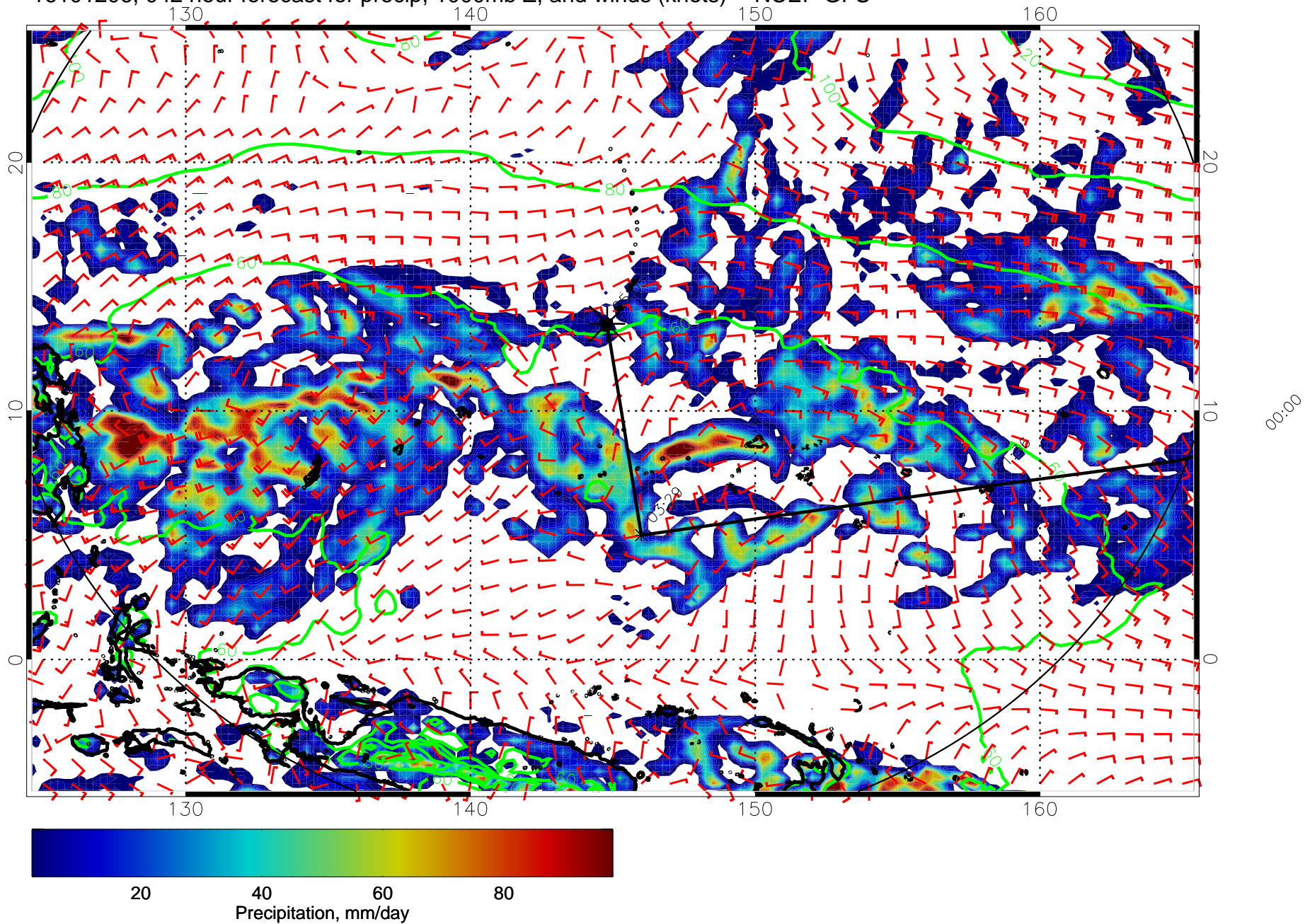
16101206, 042 hour forecast for precip, 1000mb Z, and winds (knots) -- NCEP GFS
