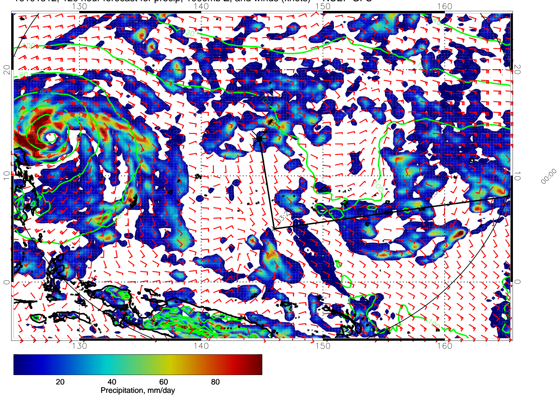
16101512, 120 hour forecast for precip, 1000mb Z, and winds (knots) -- NCEP GFS
