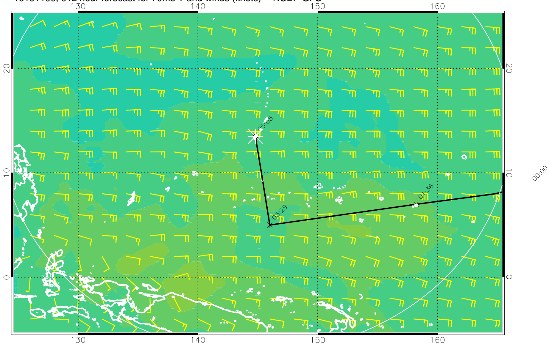
16101100, 012 hour forecast for 70mb T and winds (knots) -- NCEP GFS
