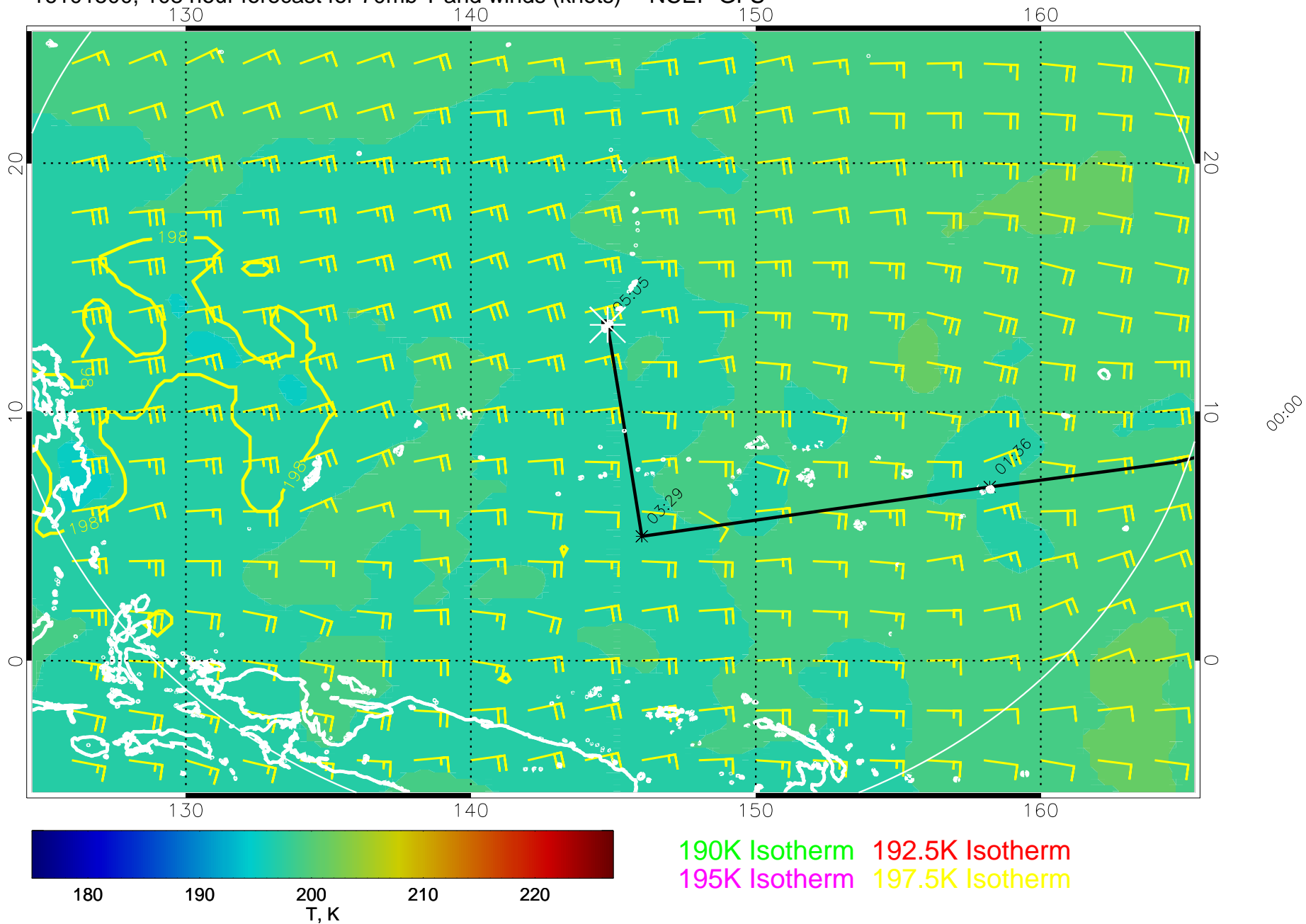
16101500, 108 hour forecast for 70mb T and winds (knots) -- NCEP GFS
