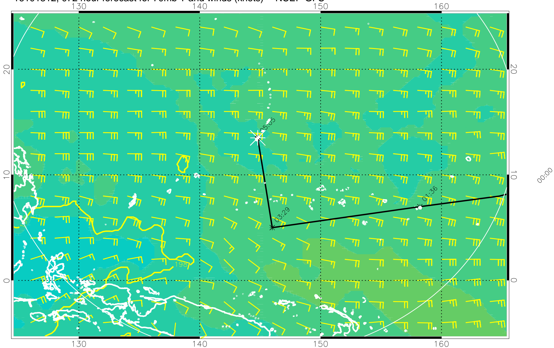
16101312, 072 hour forecast for 70mb T and winds (knots) -- NCEP GFS
