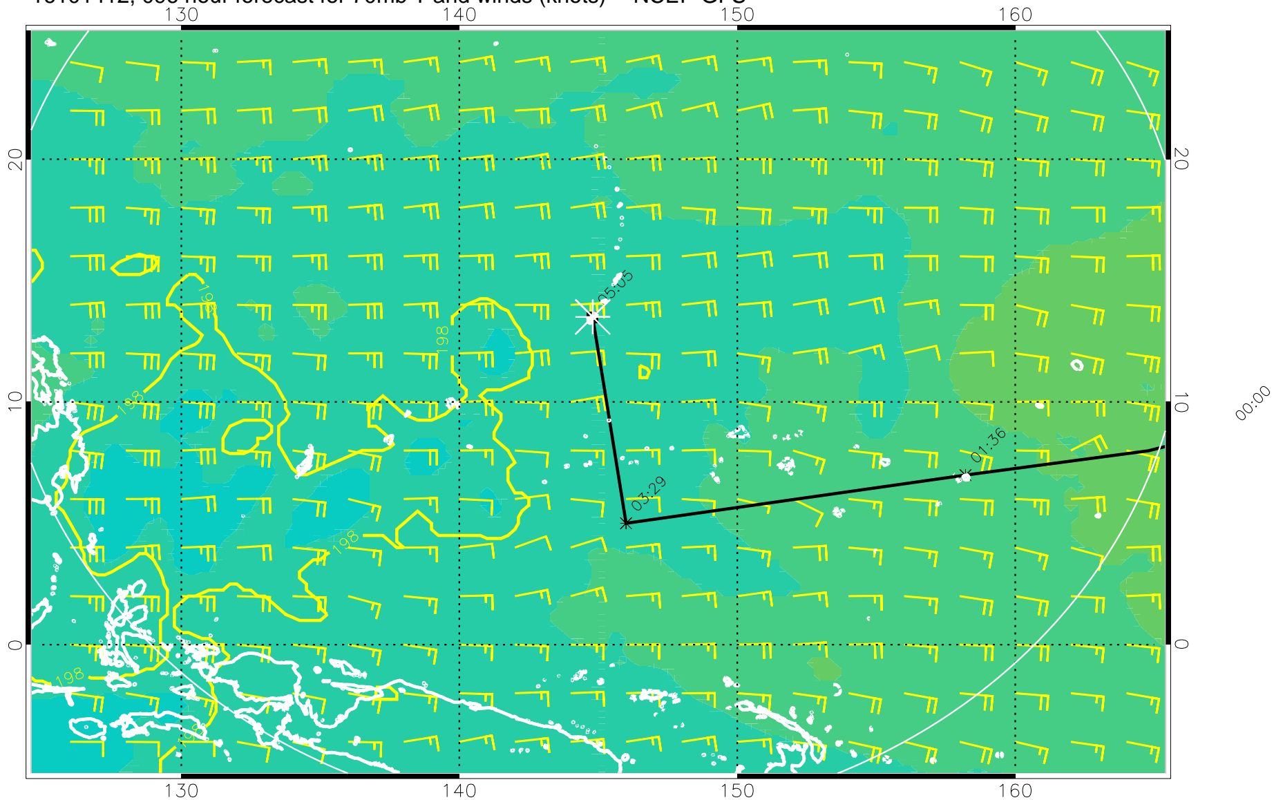
16101412, 096 hour forecast for 70mb T and winds (knots) -- NCEP GFS
