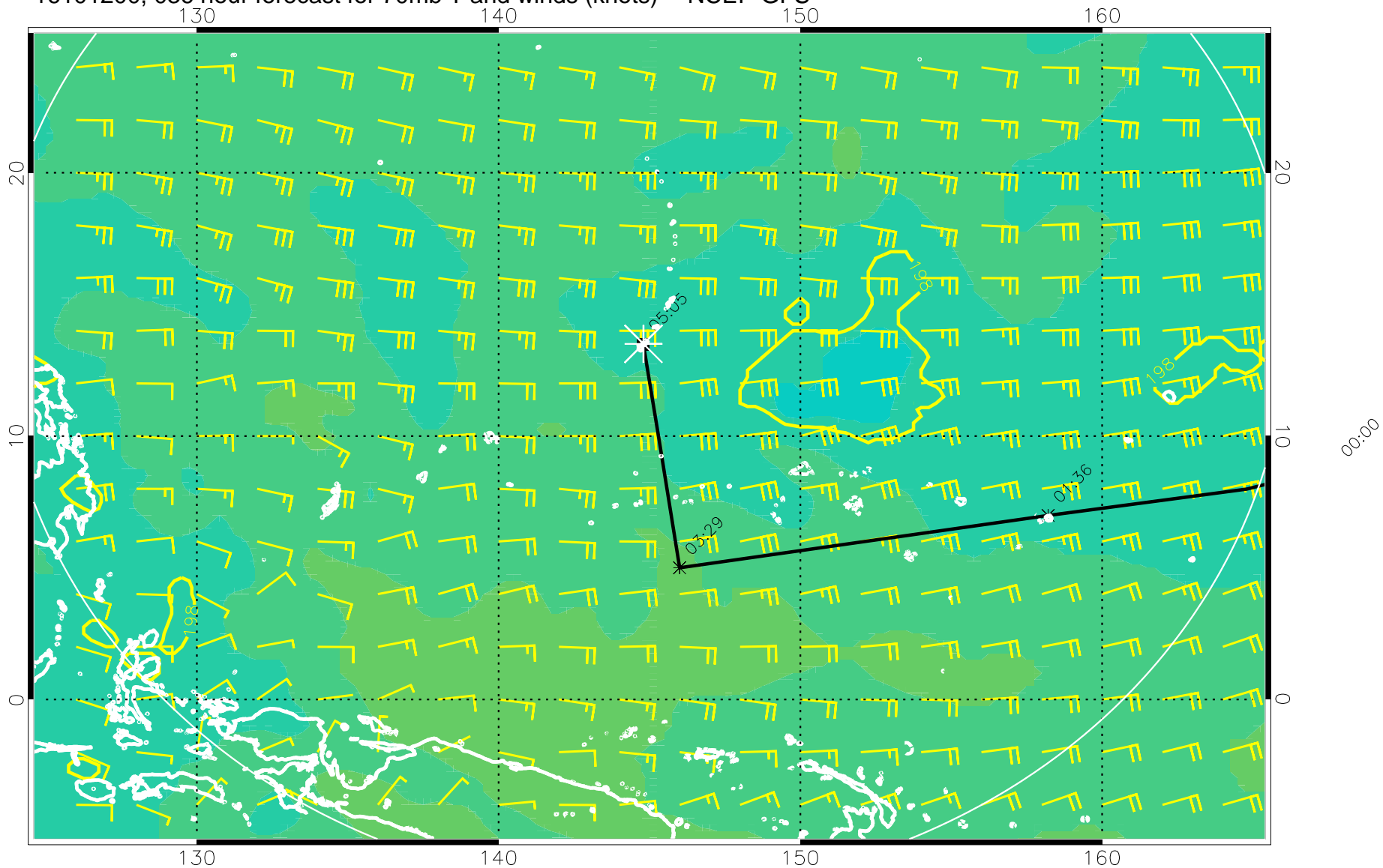
16101200, 036 hour forecast for 70mb T and winds (knots) -- NCEP GFS
