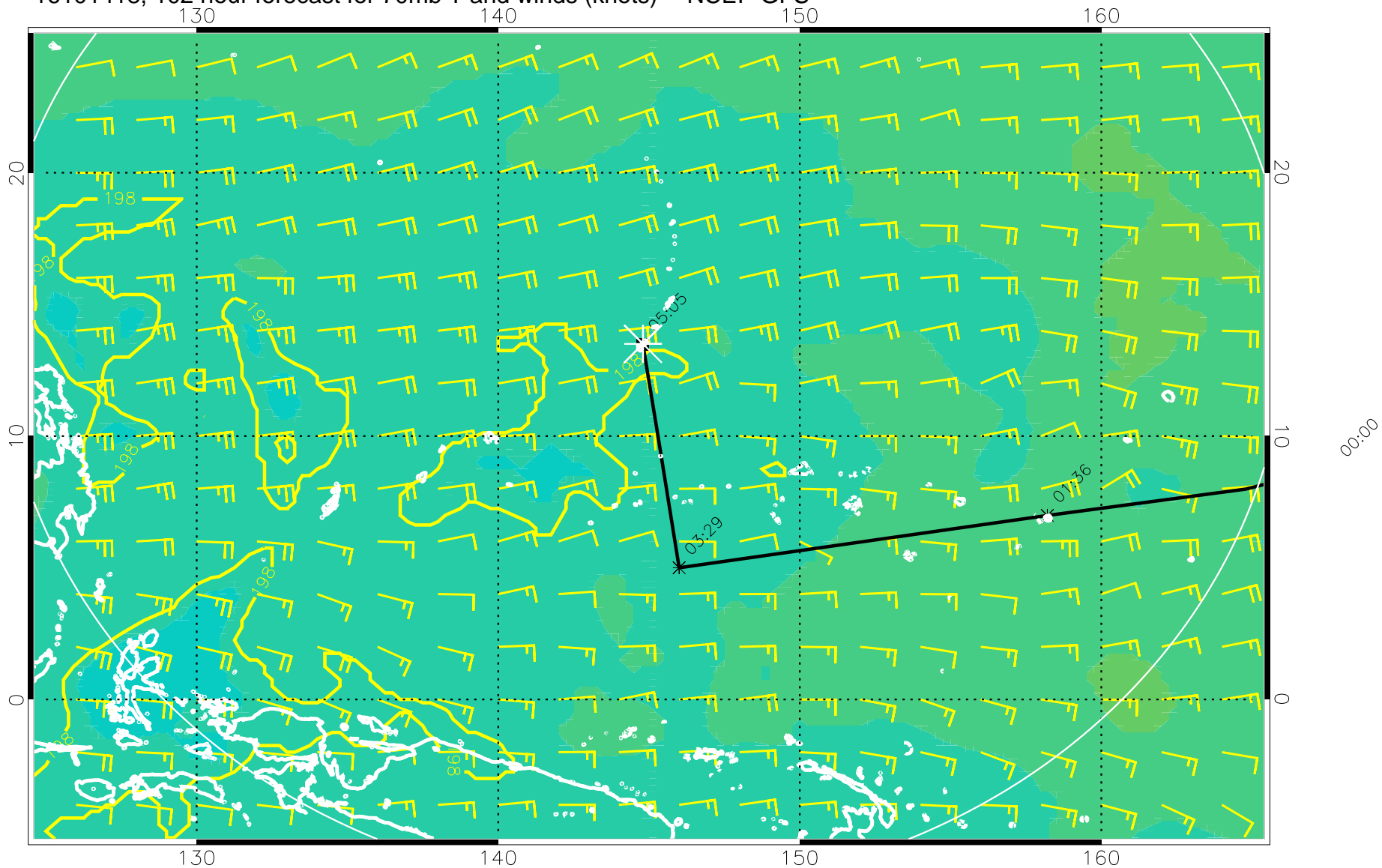
16101418, 102 hour forecast for 70mb T and winds (knots) -- NCEP GFS
