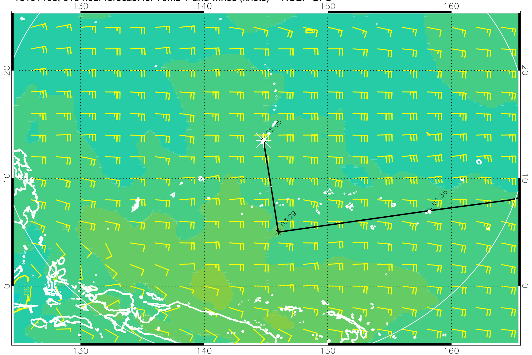
16101106, 018 hour forecast for 70mb T and winds (knots) -- NCEP GFS
