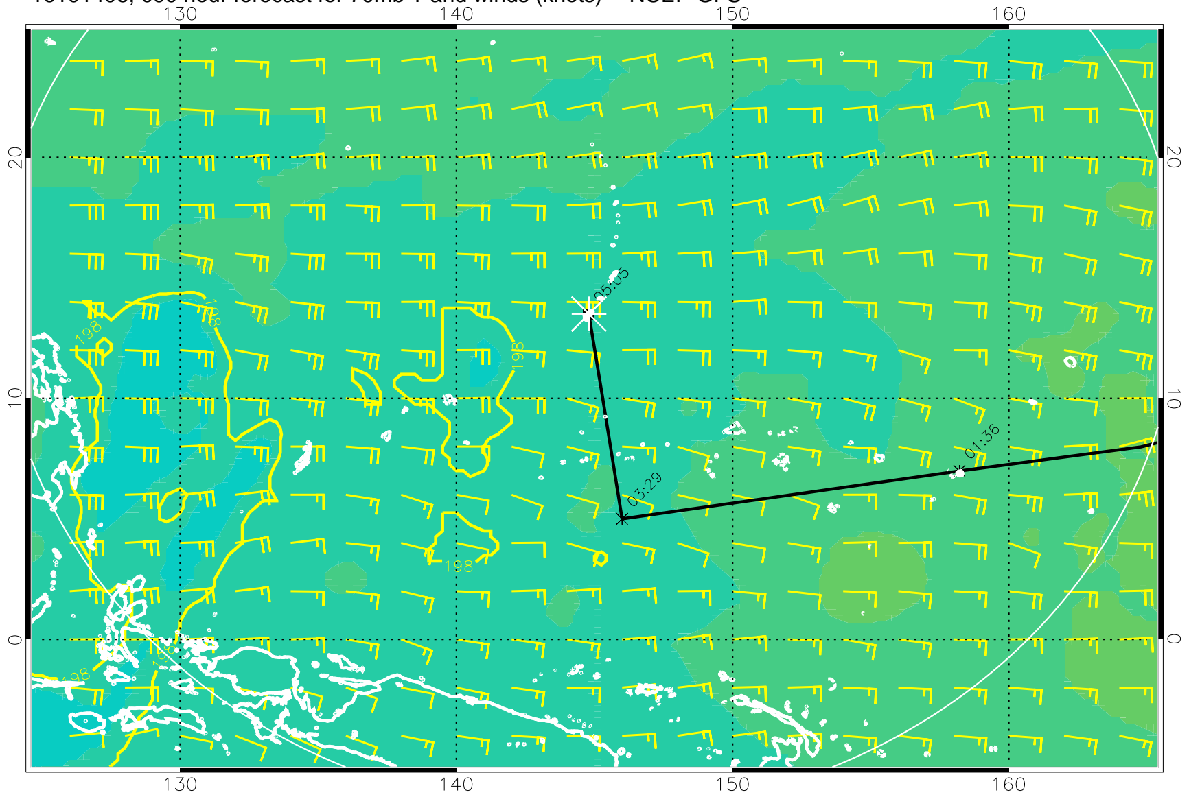
16101406, 090 hour forecast for 70mb T and winds (knots) -- NCEP GFS
