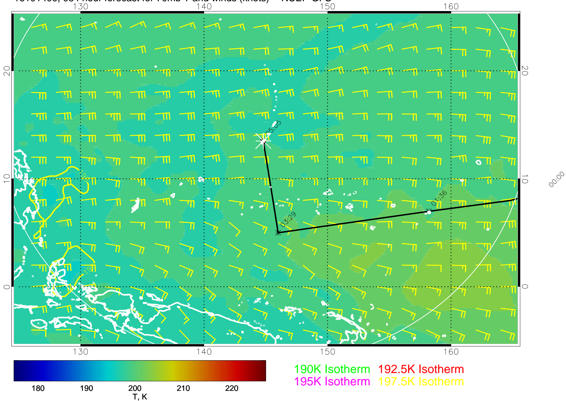
16101400, 084 hour forecast for 70mb T and winds (knots) -- NCEP GFS
