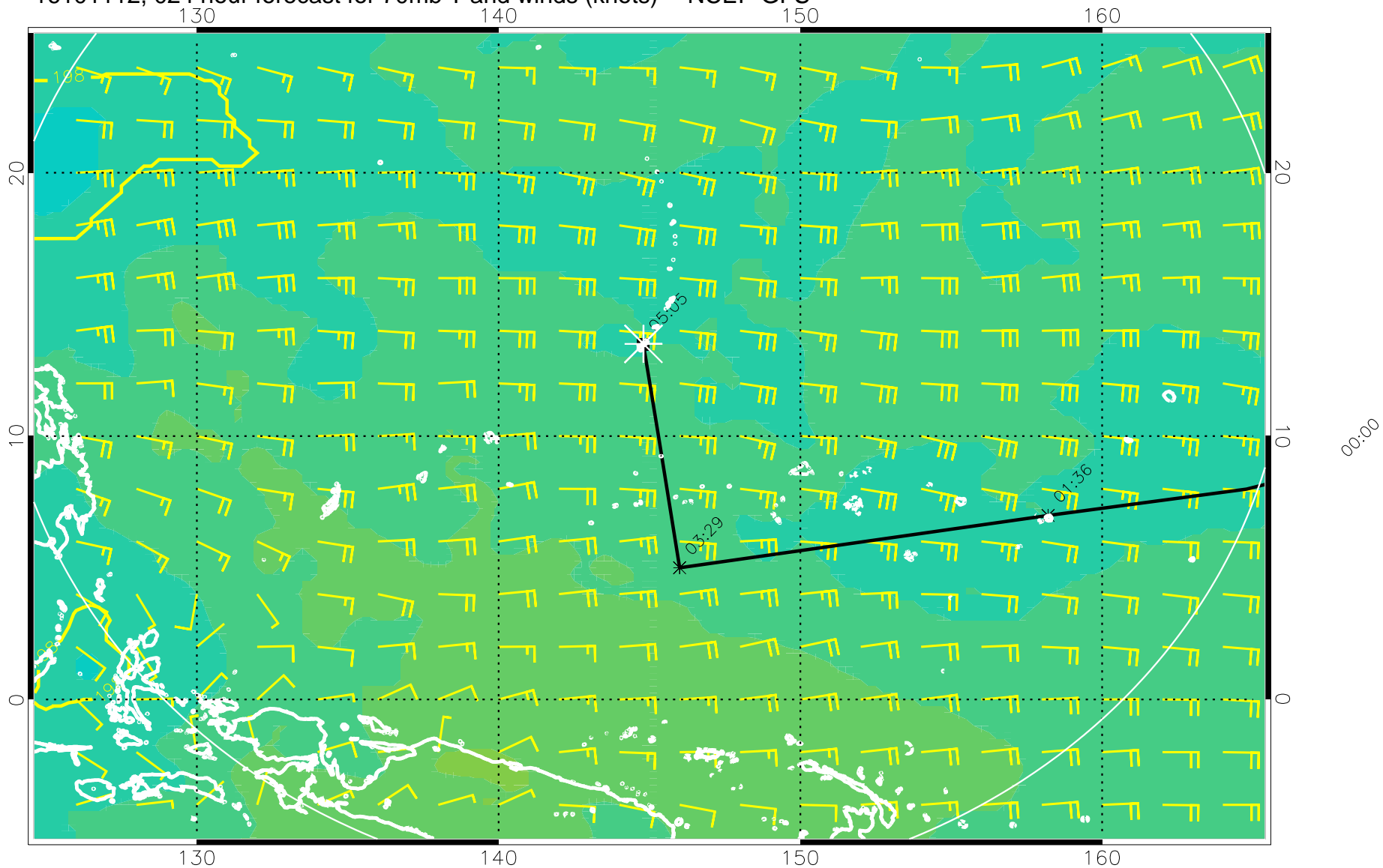
16101112, 024 hour forecast for 70mb T and winds (knots) -- NCEP GFS
