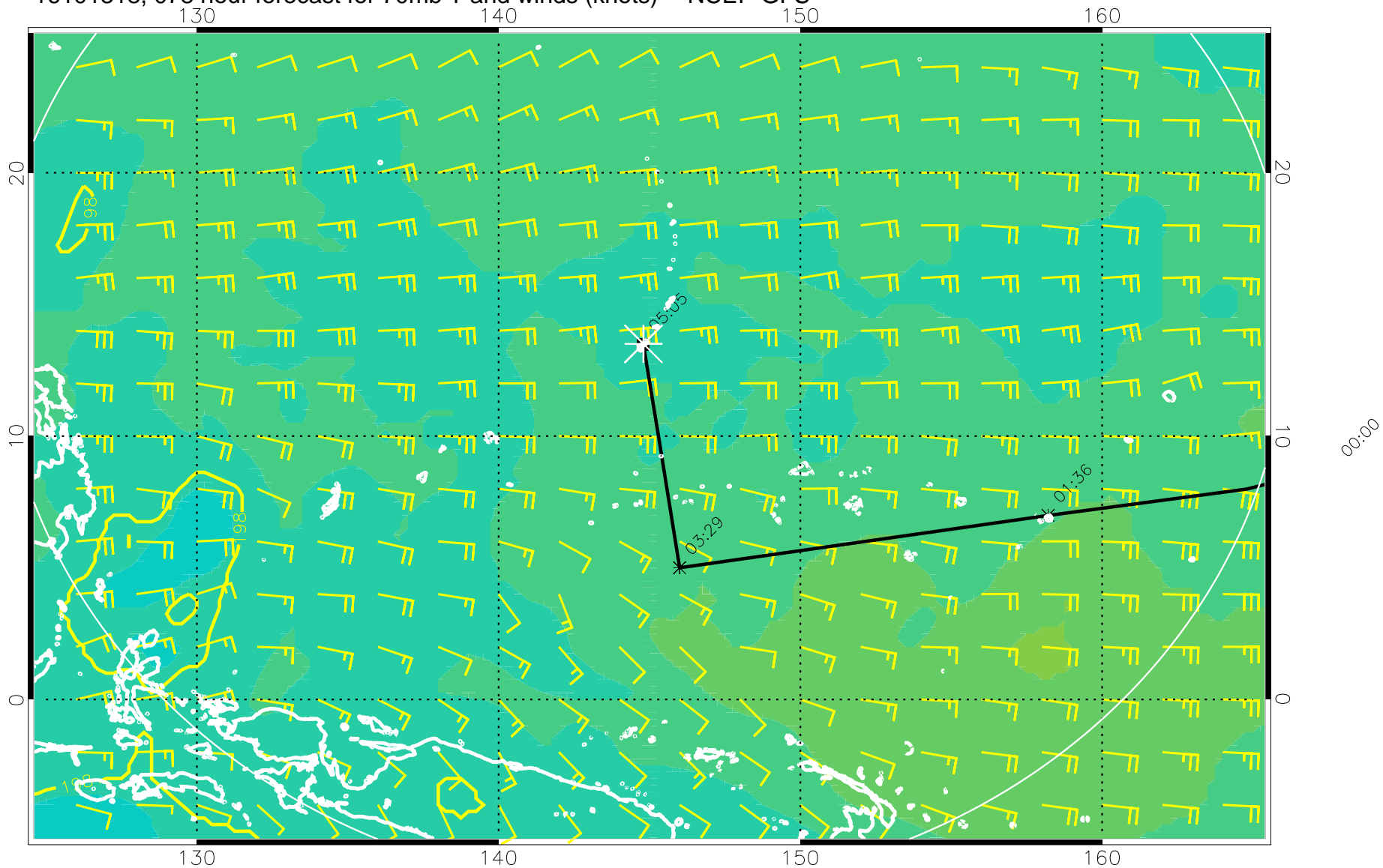
16101318, 078 hour forecast for 70mb T and winds (knots) -- NCEP GFS
