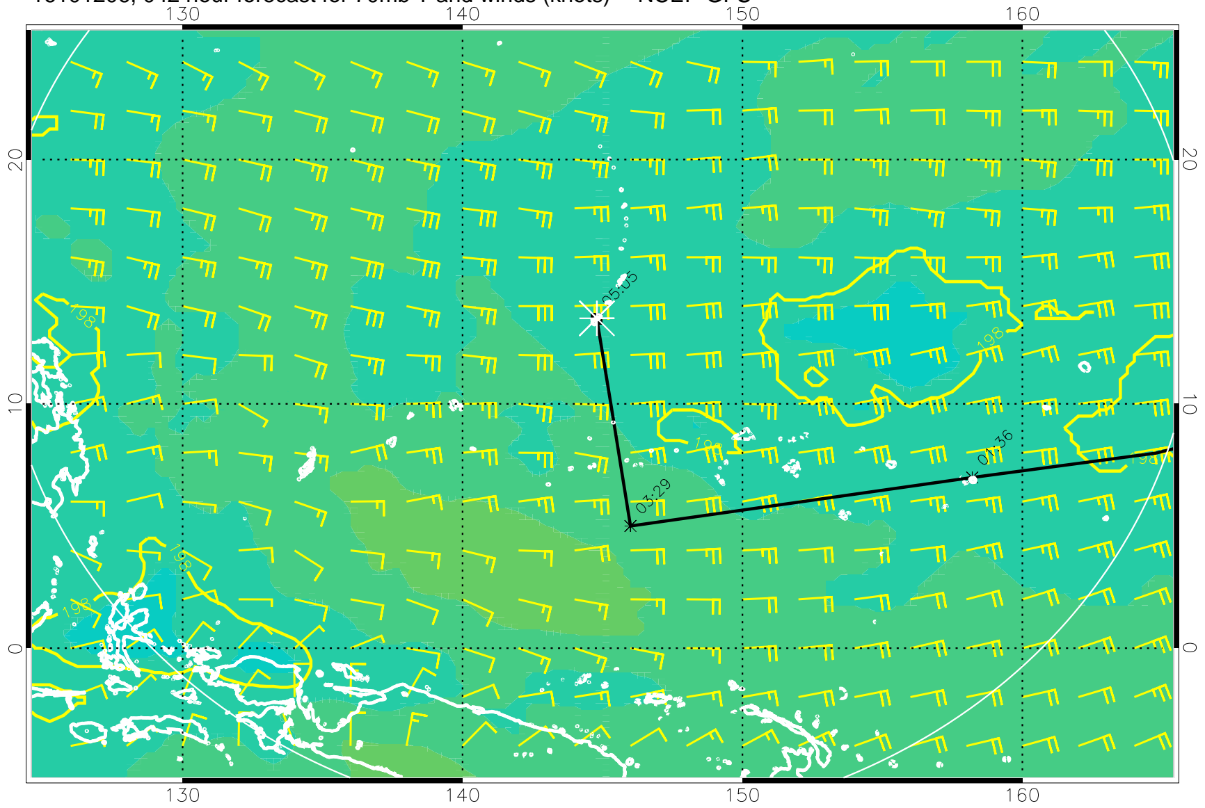
16101206, 042 hour forecast for 70mb T and winds (knots) -- NCEP GFS
