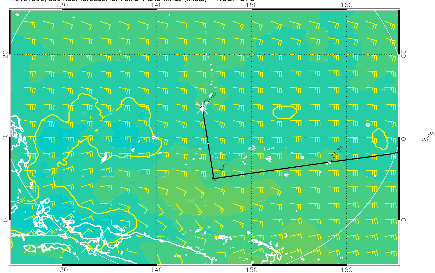
16101306, 066 hour forecast for 70mb T and winds (knots) -- NCEP GFS
