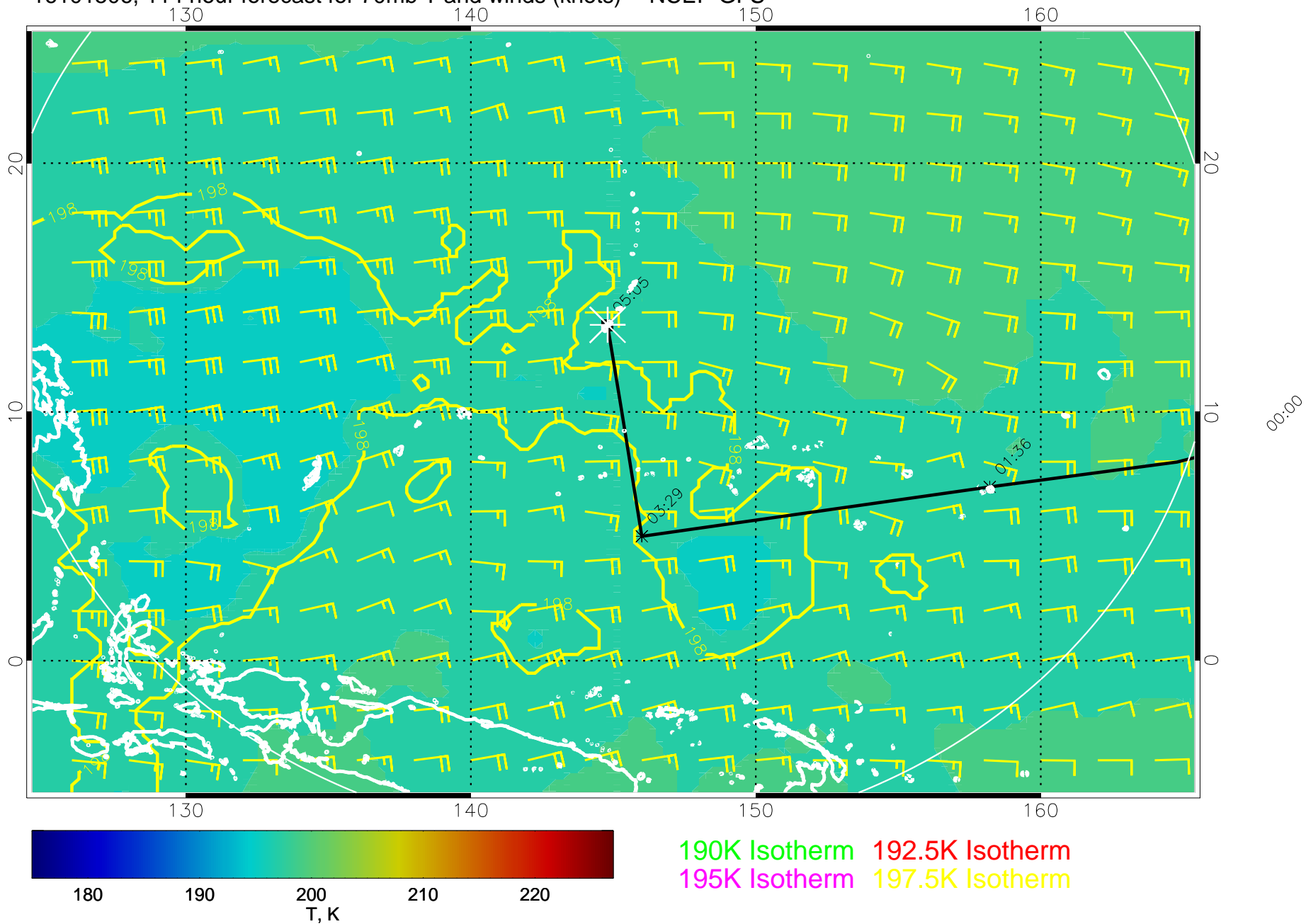
16101506, 114 hour forecast for 70mb T and winds (knots) -- NCEP GFS
