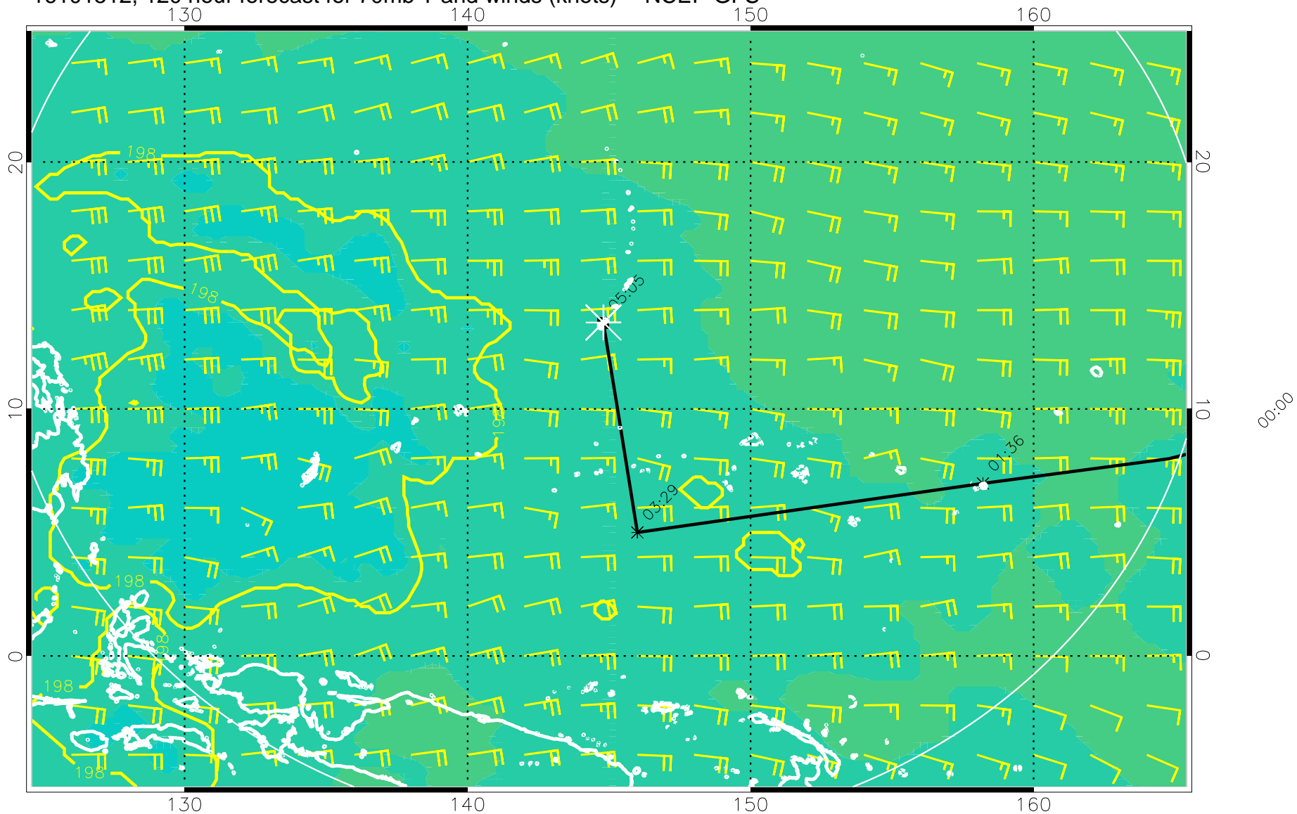
16101512, 120 hour forecast for 70mb T and winds (knots) -- NCEP GFS
