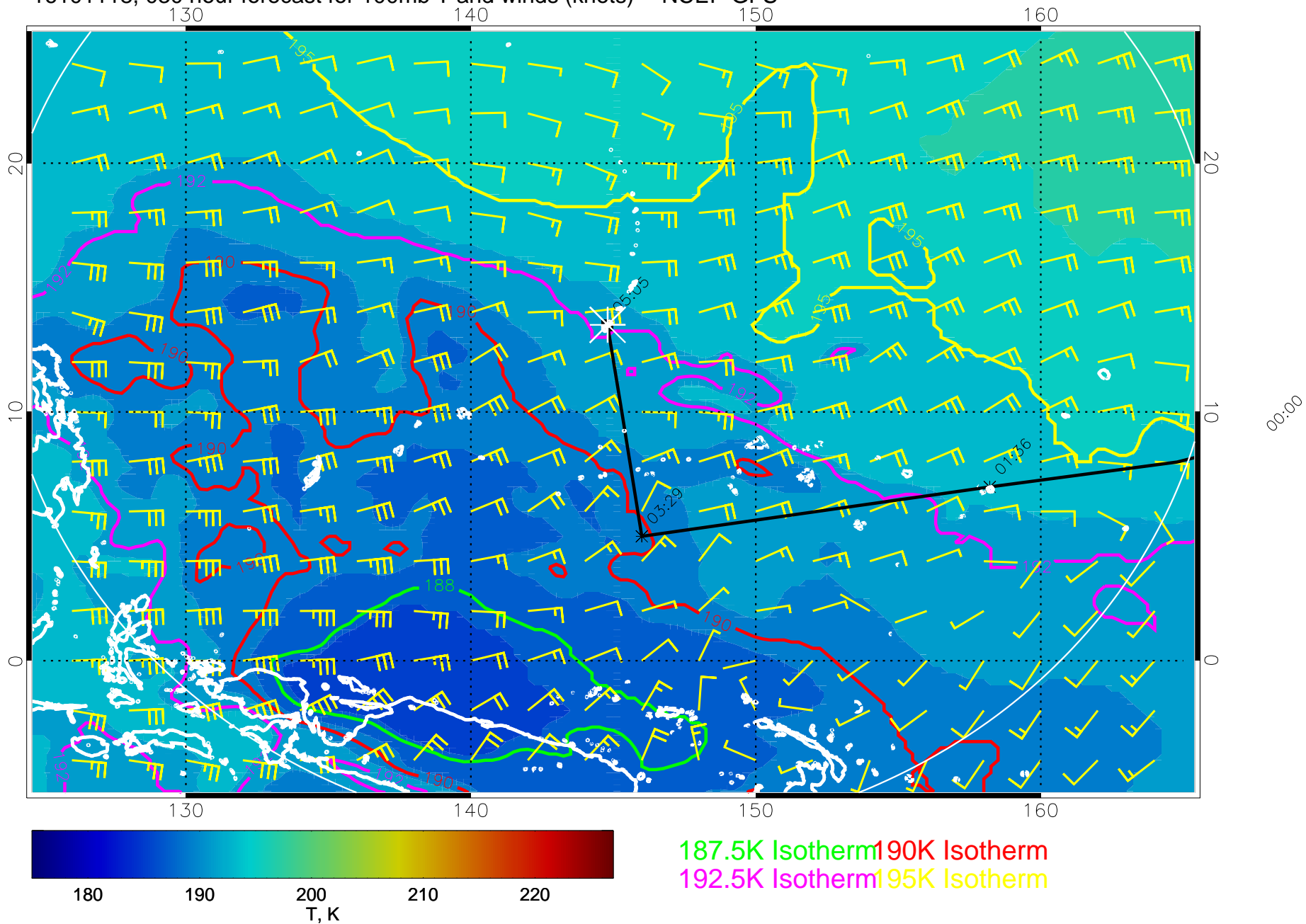
16101118, 030 hour forecast for 100mb T and winds (knots) -- NCEP GFS
