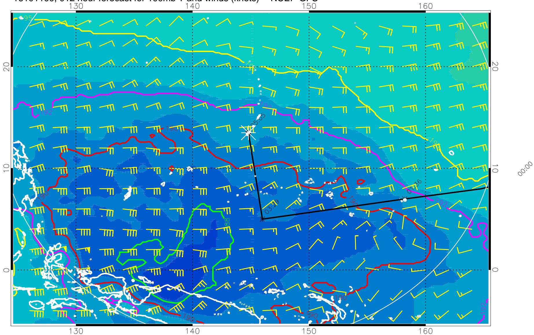
16101100, 012 hour forecast for 100mb T and winds (knots) -- NCEP GFS
