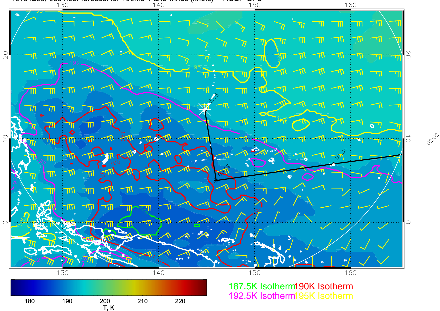
16101200, 036 hour forecast for 100mb T and winds (knots) -- NCEP GFS
