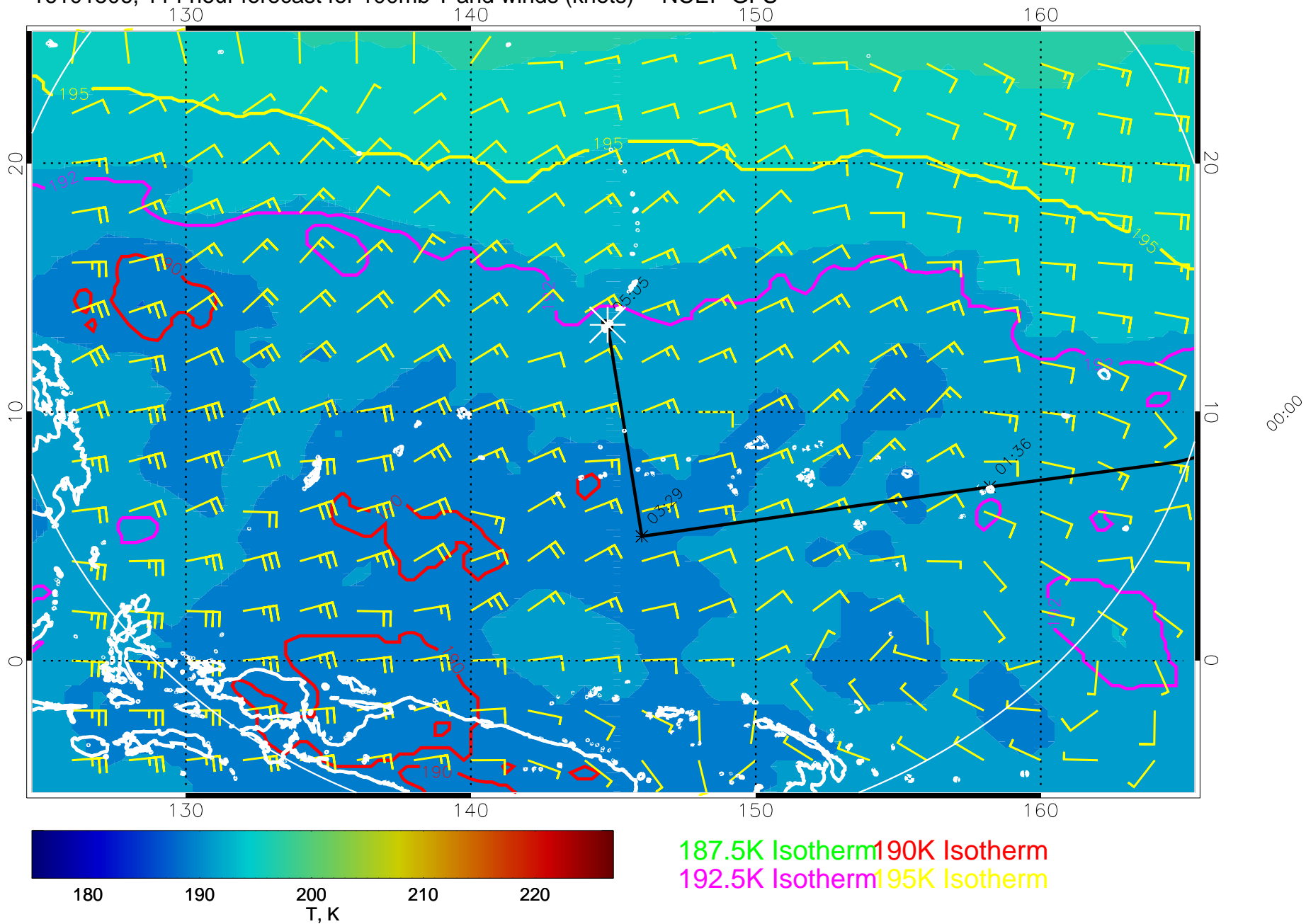
16101506, 114 hour forecast for 100mb T and winds (knots) -- NCEP GFS
