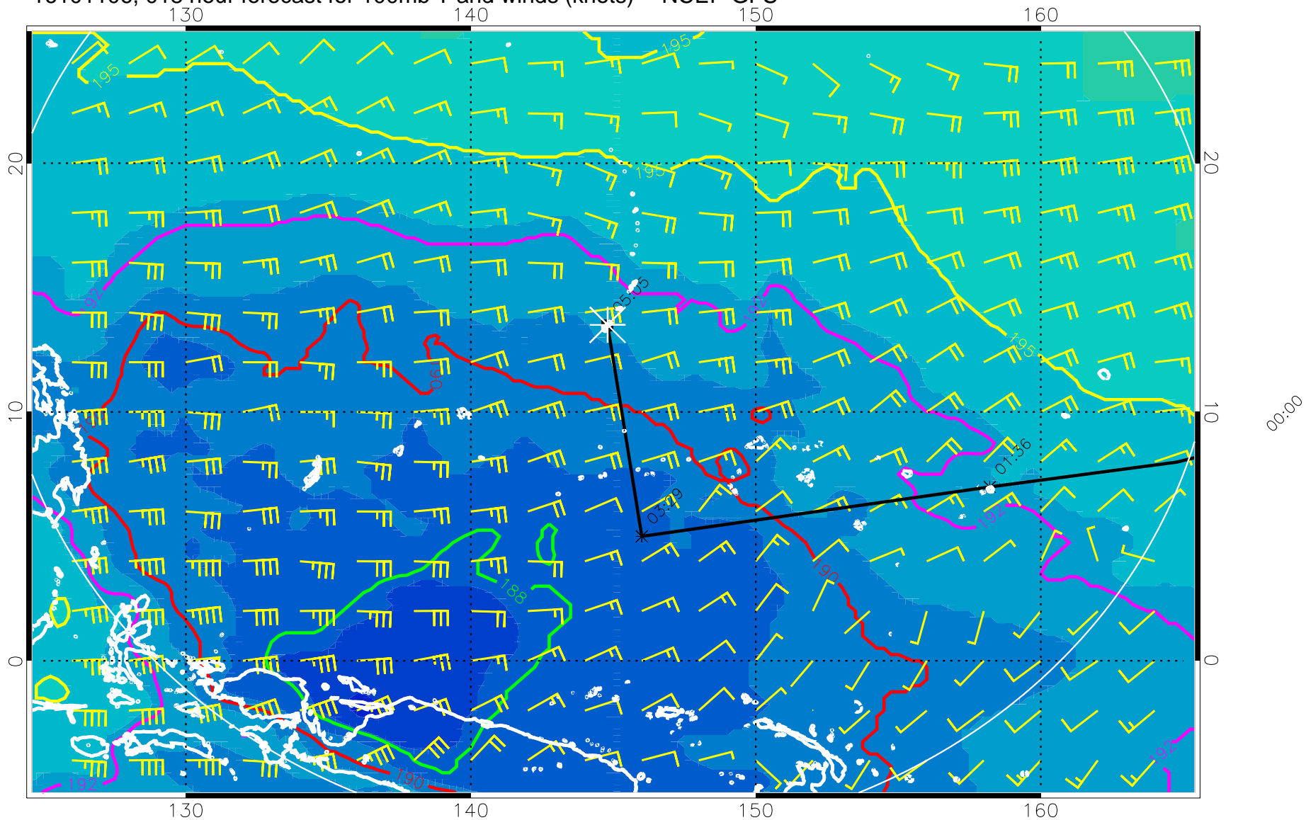
16101106, 018 hour forecast for 100mb T and winds (knots) -- NCEP GFS
