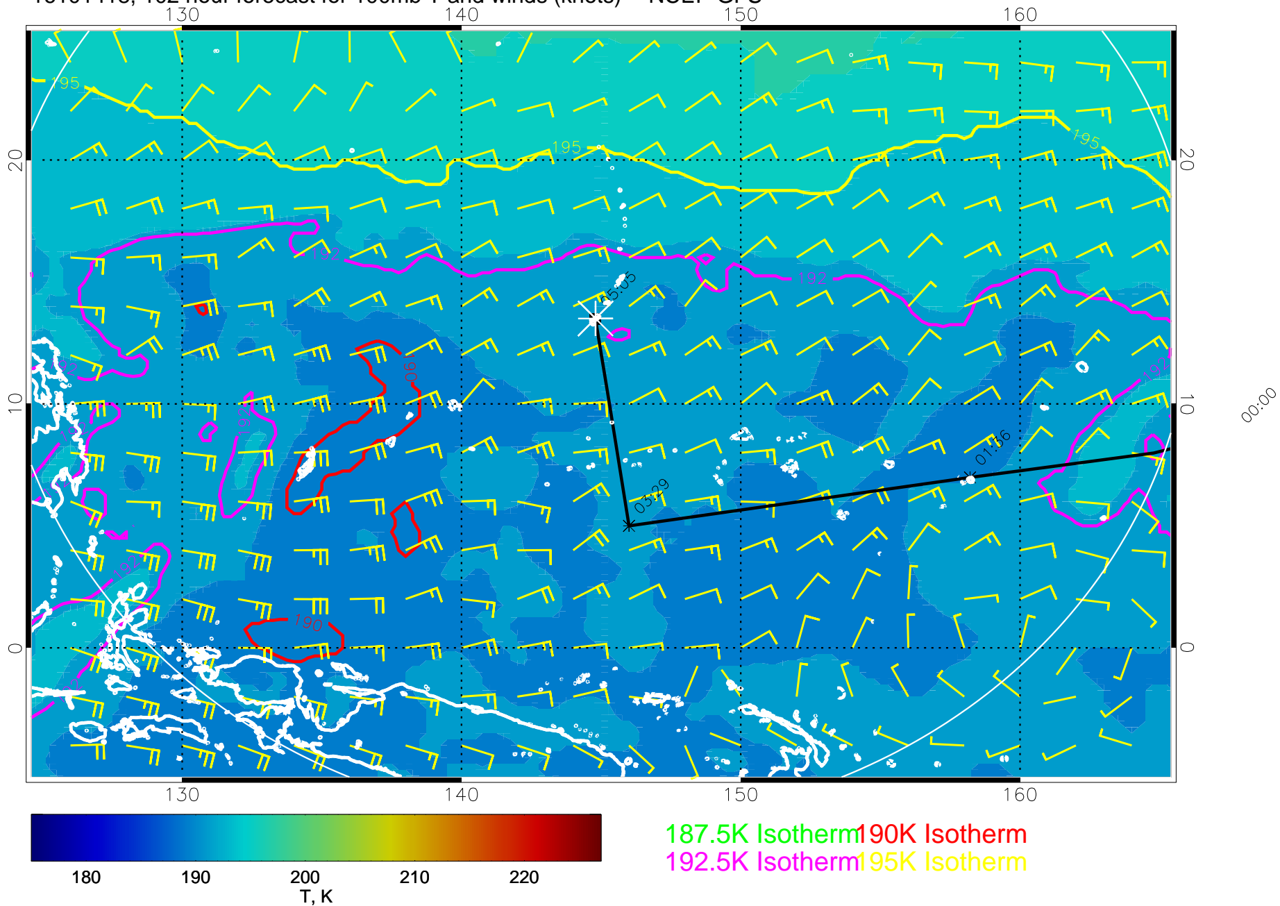
16101418, 102 hour forecast for 100mb T and winds (knots) -- NCEP GFS
