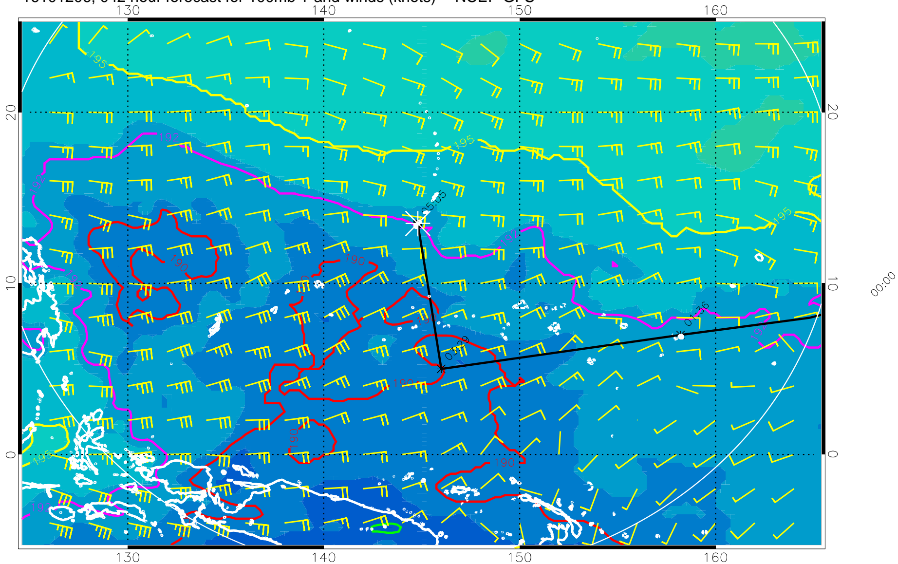
16101206, 042 hour forecast for 100mb T and winds (knots) -- NCEP GFS
