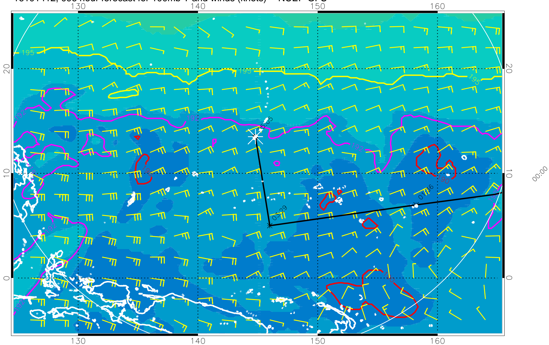
16101412, 096 hour forecast for 100mb T and winds (knots) -- NCEP GFS
