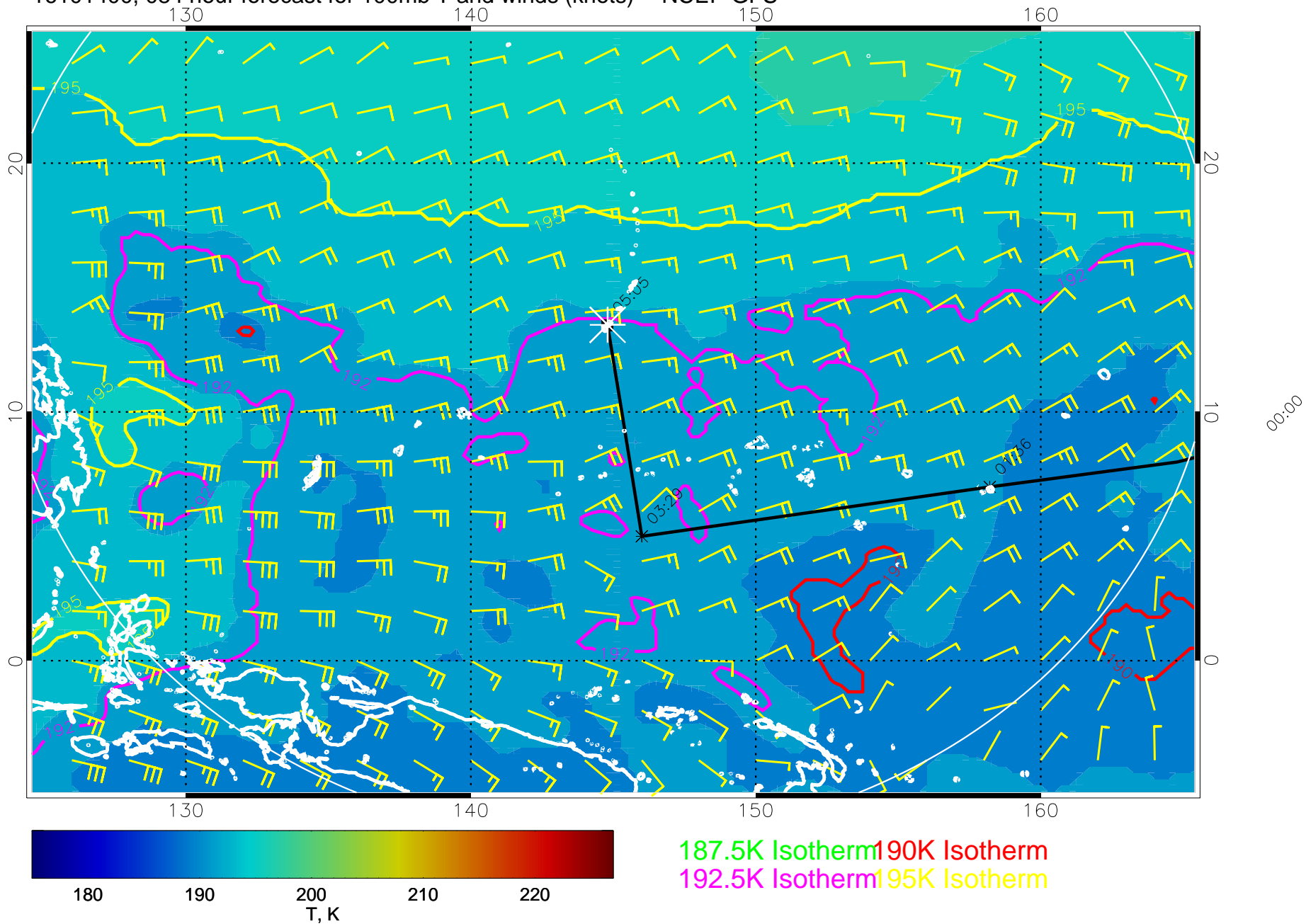
16101400, 084 hour forecast for 100mb T and winds (knots) -- NCEP GFS
