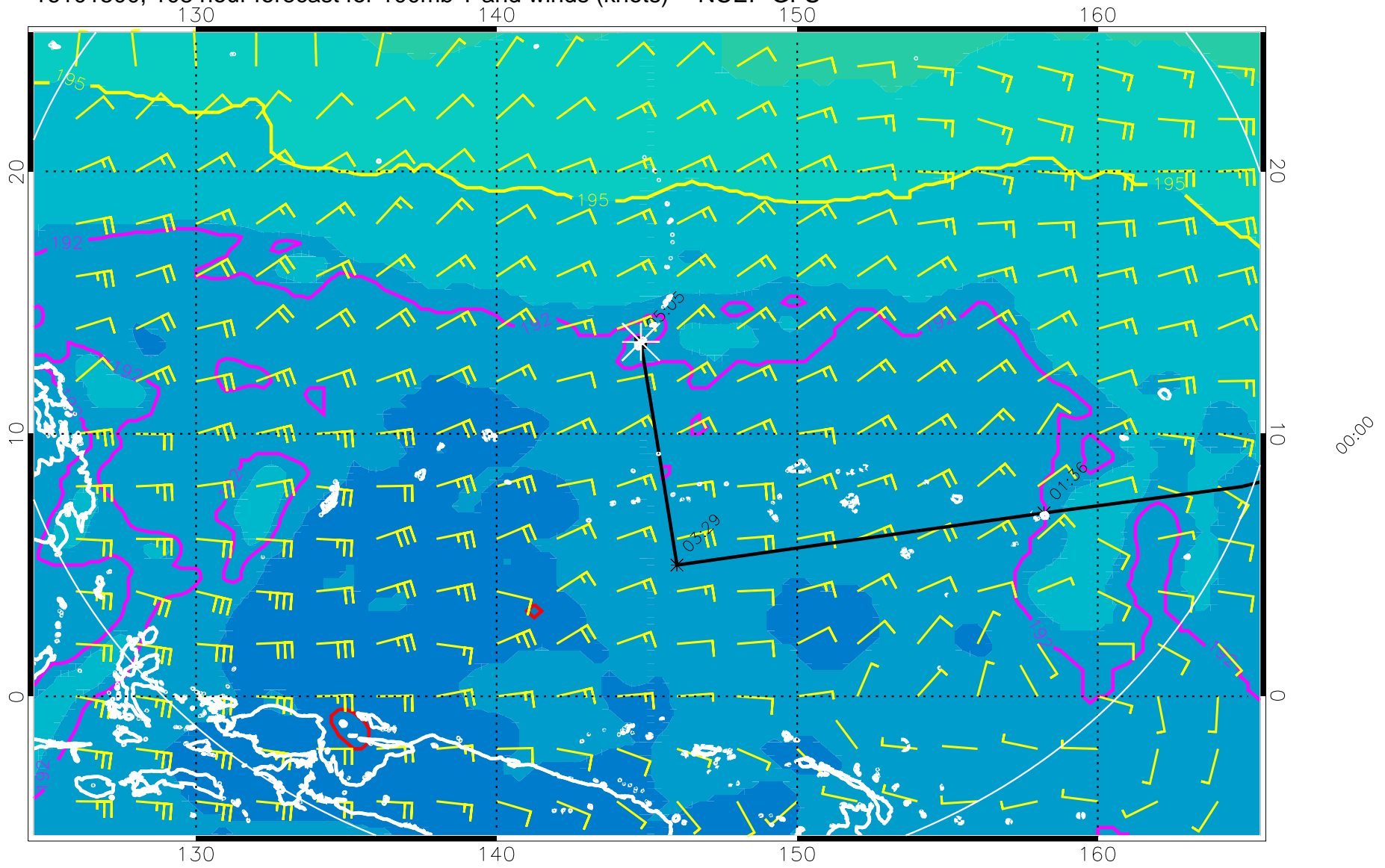
16101500, 108 hour forecast for 100mb T and winds (knots) -- NCEP GFS
