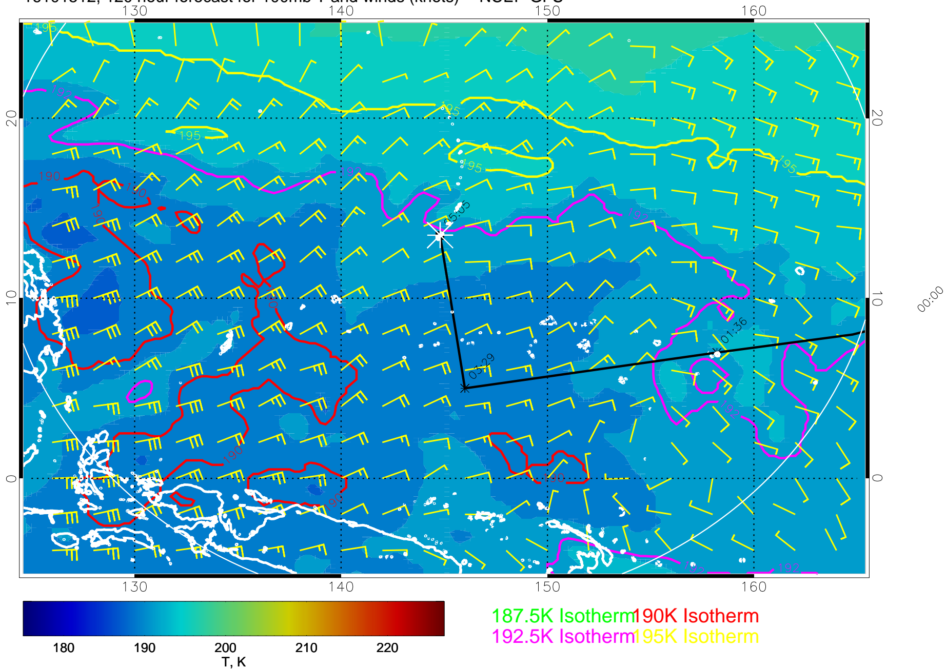
16101512, 120 hour forecast for 100mb T and winds (knots) -- NCEP GFS
