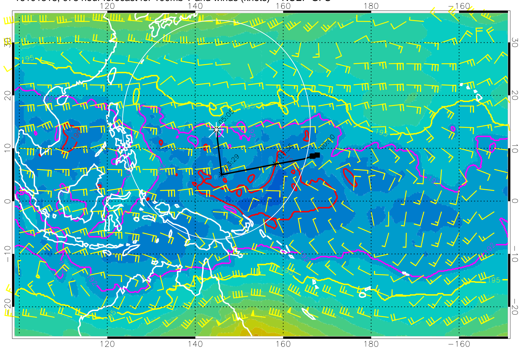
16101318, 078 hour forecast for 100mb T and winds (knots) -- NCEP GFS
