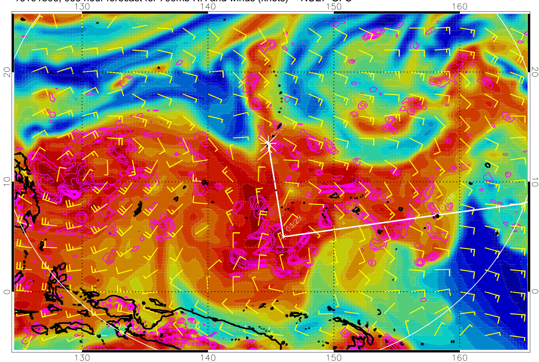
16101306, 066 hour forecast for 700mb RH and winds (knots) -- NCEP GFS
