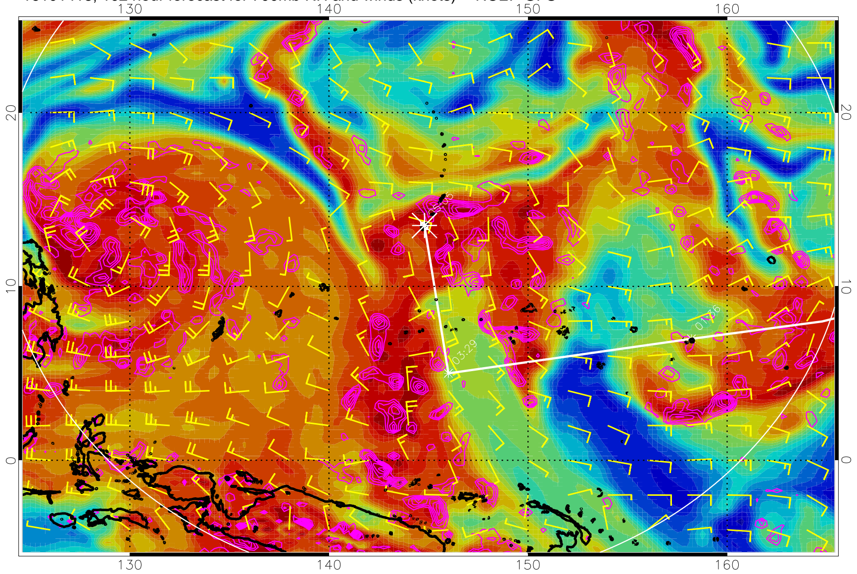
16101418, 102 hour forecast for 700mb RH and winds (knots) -- NCEP GFS
