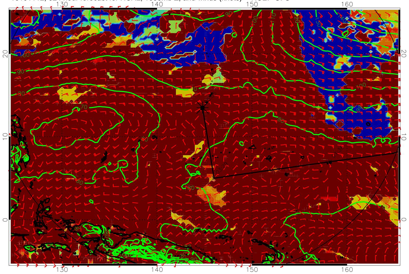
16101112, 024 hour forecast for HCAL, 1000mb Z, and winds (knots) -- NCEP GFS
