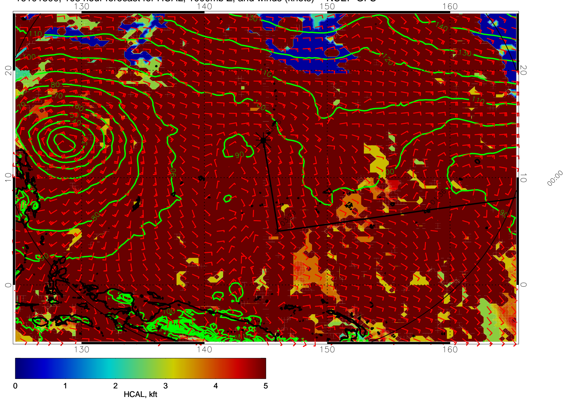
16101500, 108 hour forecast for HCAL, 1000mb Z, and winds (knots) -- NCEP GFS
