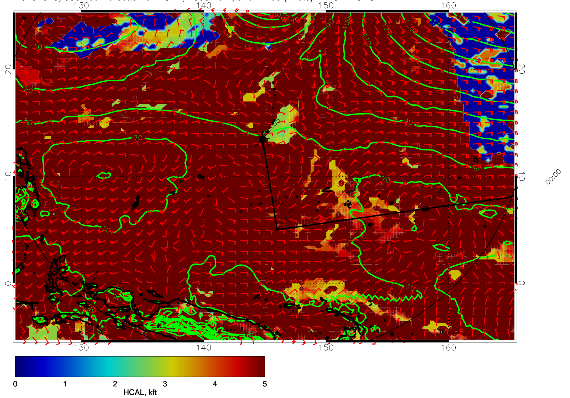
16101018, 006 hour forecast for HCAL, 1000mb Z, and winds (knots) -- NCEP GFS
