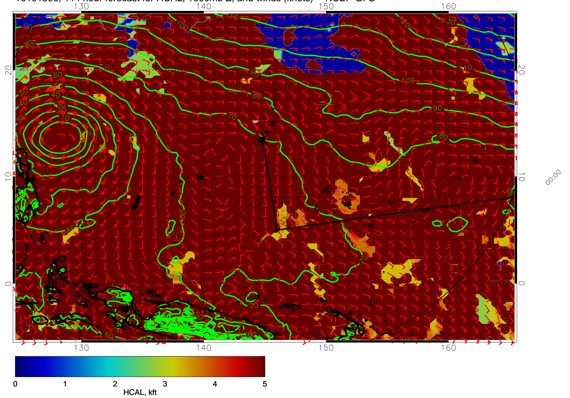
16101506, 114 hour forecast for HCAL, 1000mb Z, and winds (knots) -- NCEP GFS
