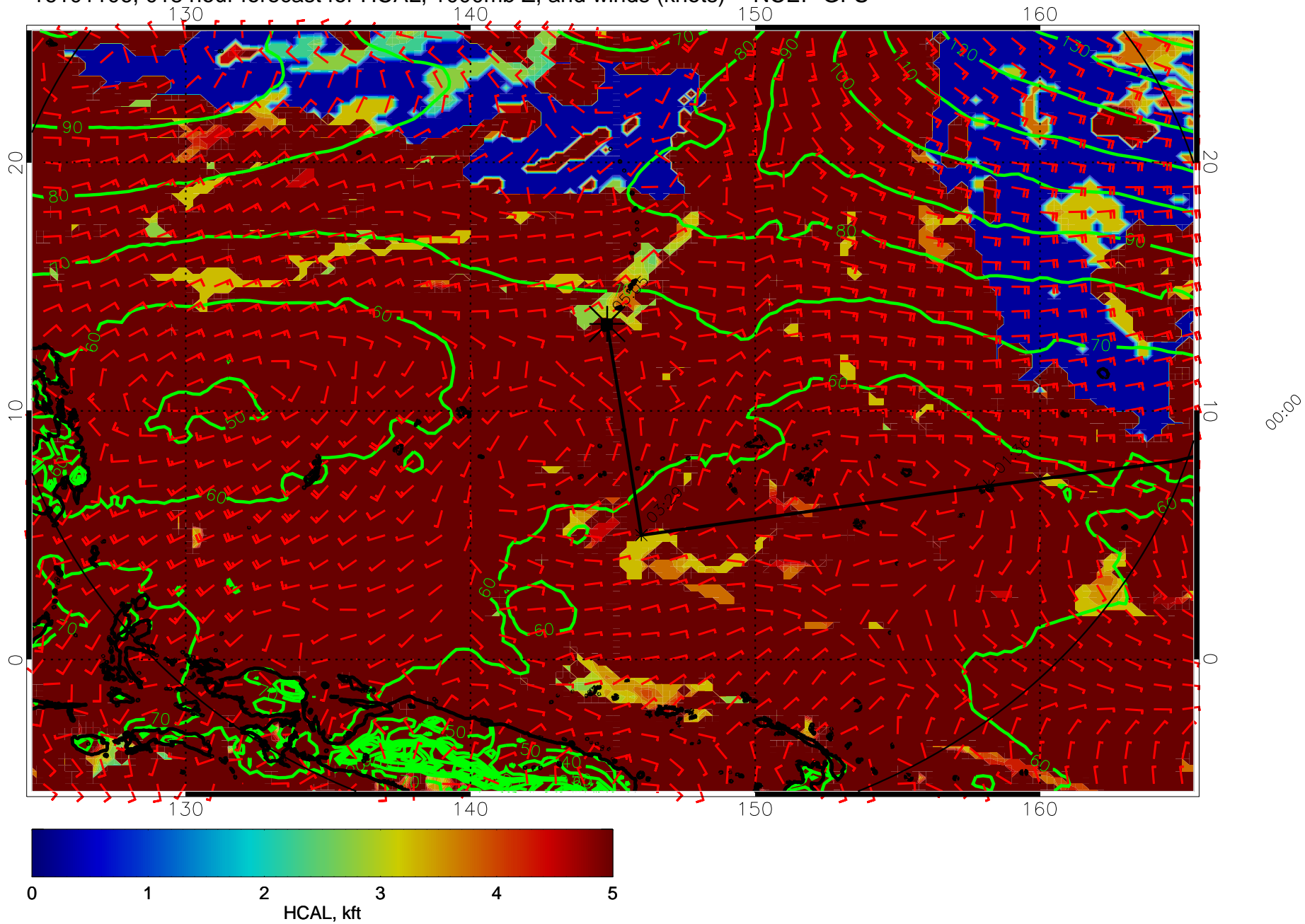
16101106, 018 hour forecast for HCAL, 1000mb Z, and winds (knots) -- NCEP GFS
