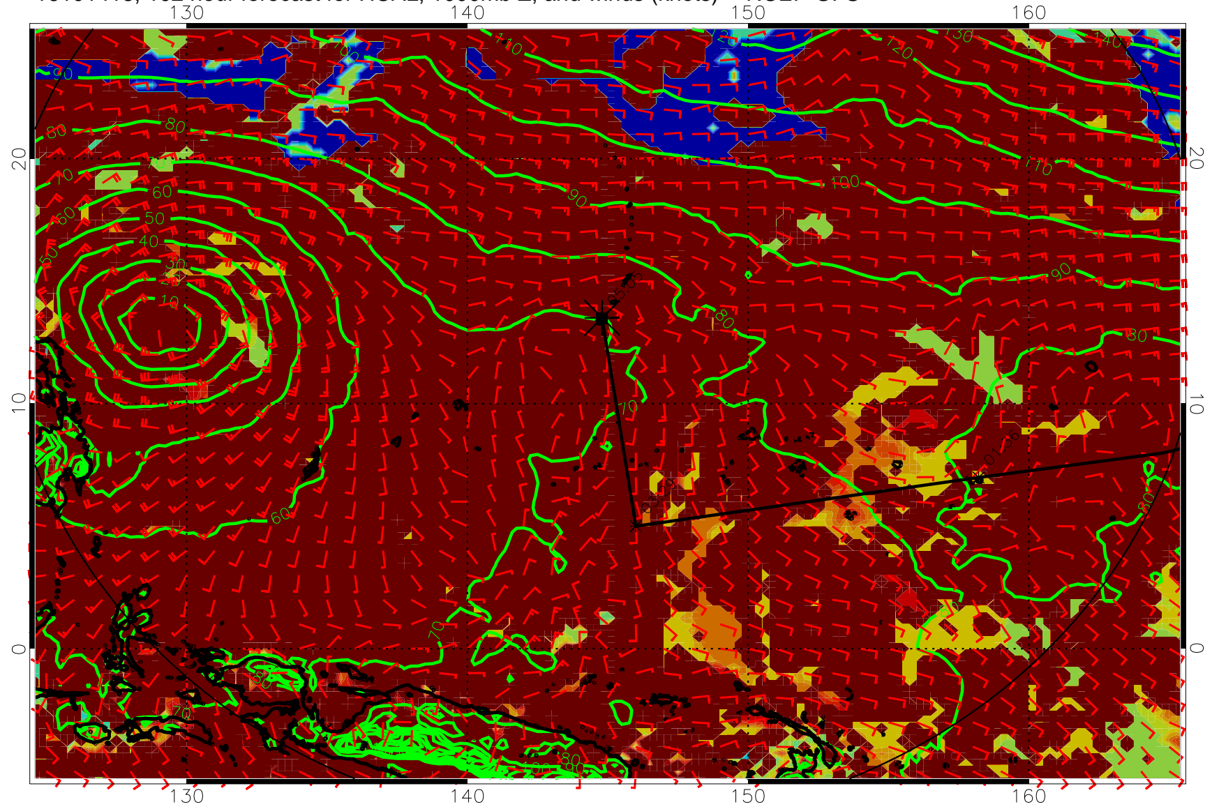
16101418, 102 hour forecast for HCAL, 1000mb Z, and winds (knots) -- NCEP GFS
