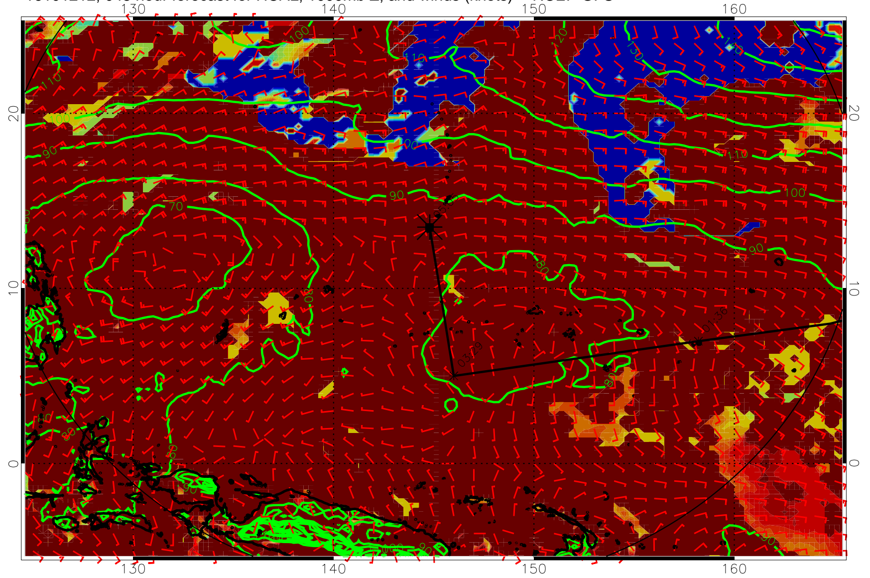
16101212, 048 hour forecast for HCAL, 1000mb Z, and winds (knots) -- NCEP GFS
