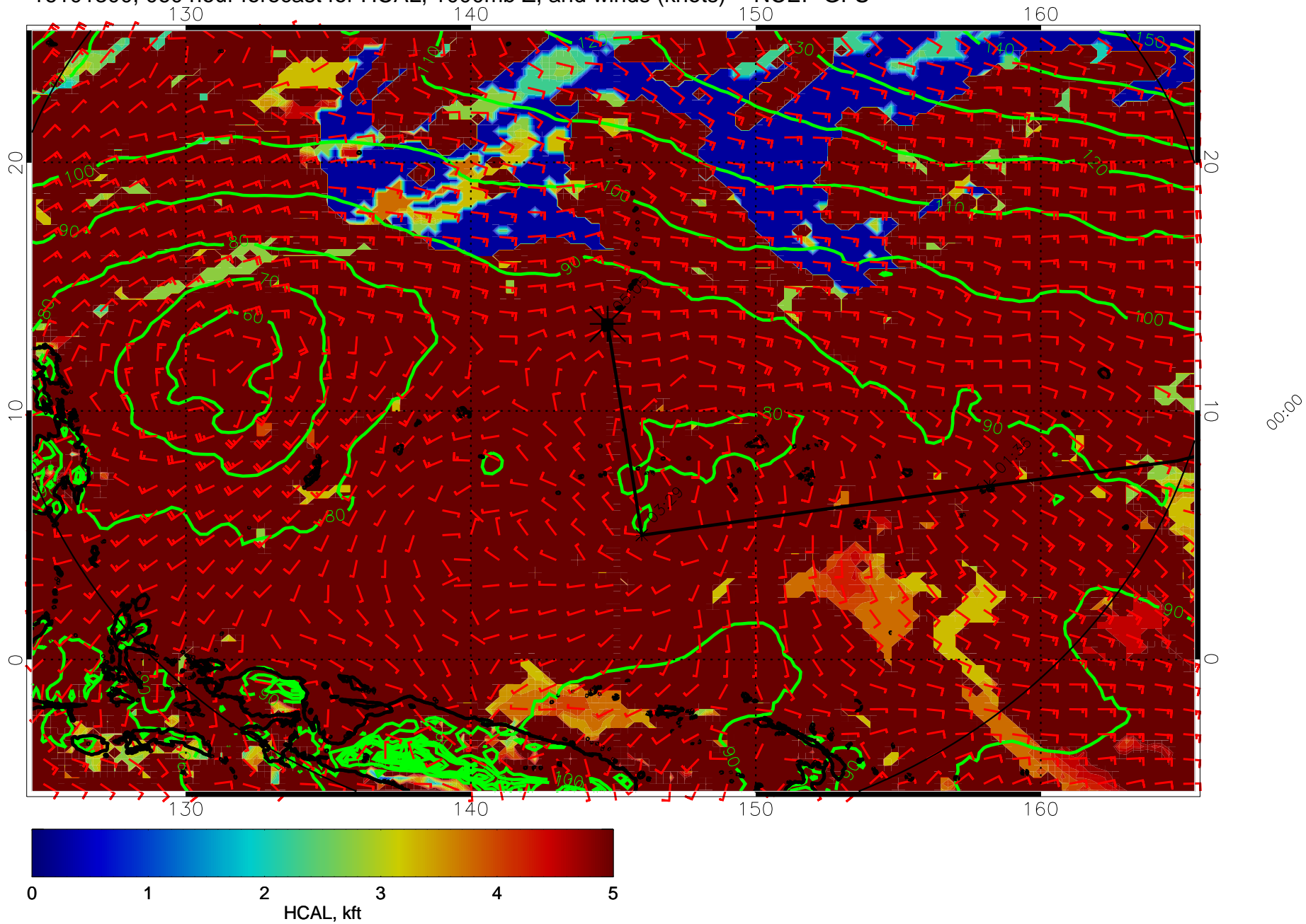
16101300, 060 hour forecast for HCAL, 1000mb Z, and winds (knots) -- NCEP GFS
