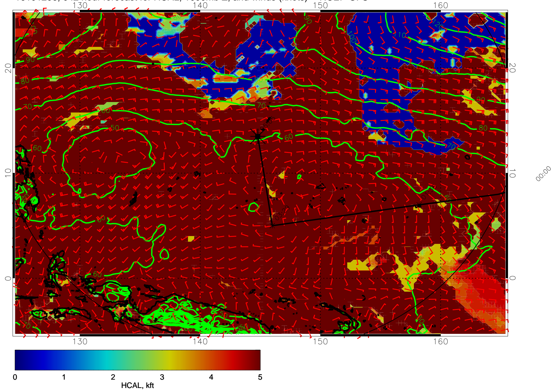
16101206, 042 hour forecast for HCAL, 1000mb Z, and winds (knots) -- NCEP GFS
