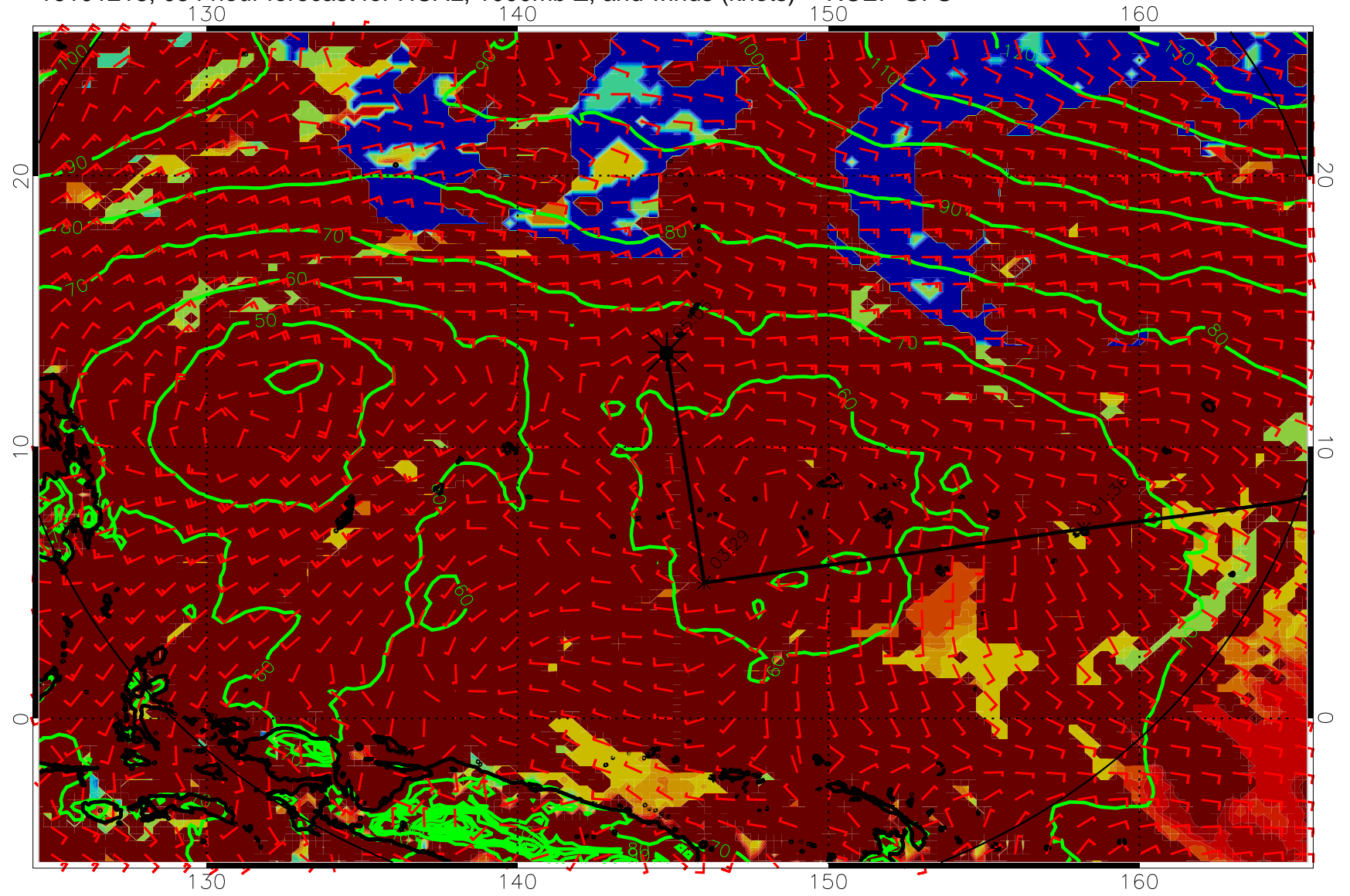
16101218, 054 hour forecast for HCAL, 1000mb Z, and winds (knots) -- NCEP GFS
