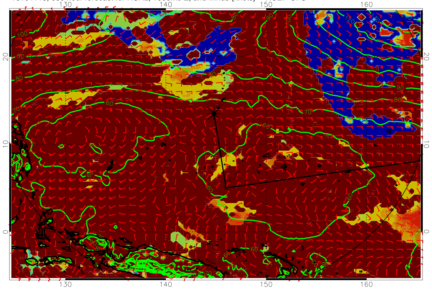
16101118, 030 hour forecast for HCAL, 1000mb Z, and winds (knots) -- NCEP GFS
