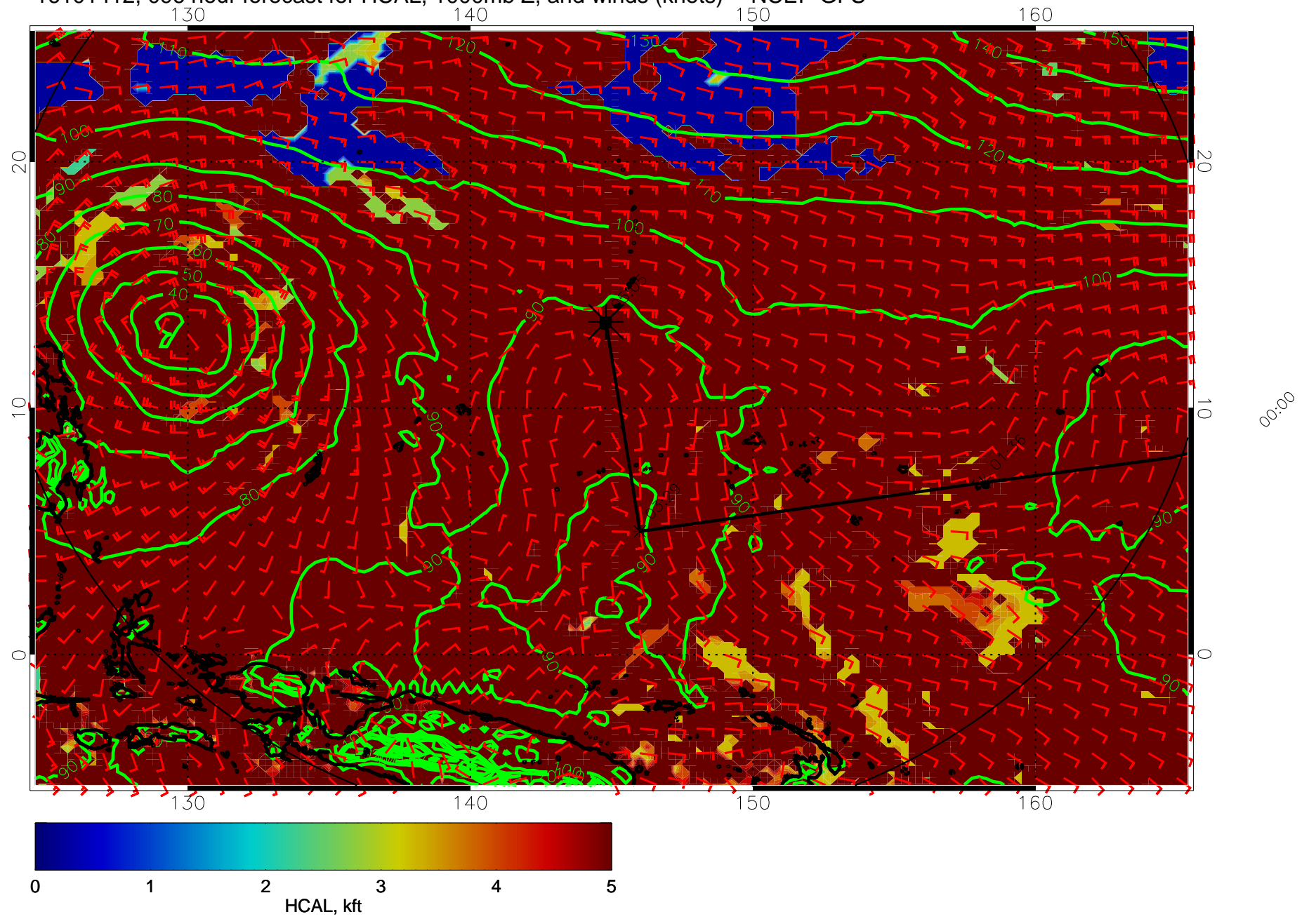
16101412, 096 hour forecast for HCAL, 1000mb Z, and winds (knots) -- NCEP GFS
