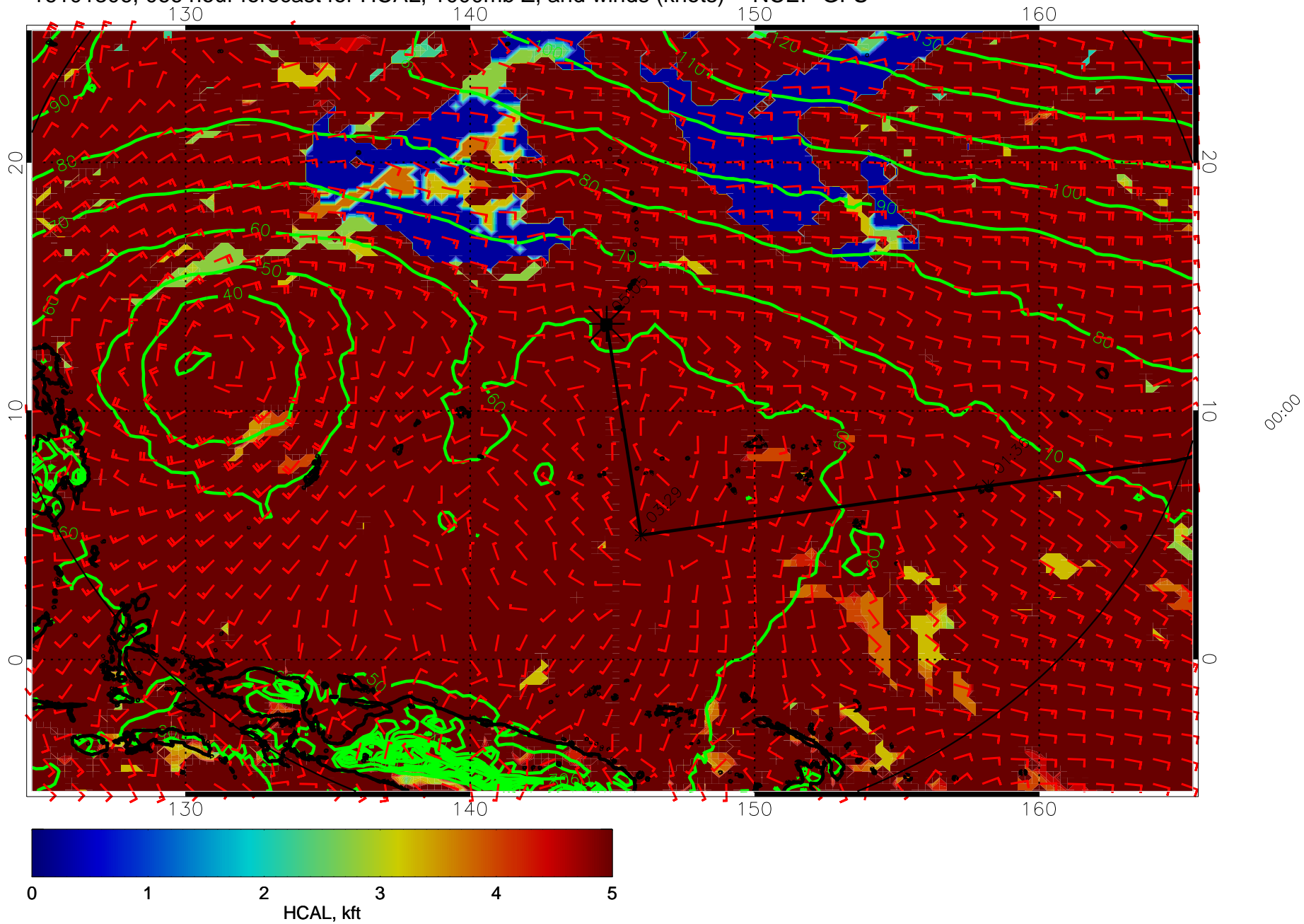
16101306, 066 hour forecast for HCAL, 1000mb Z, and winds (knots) -- NCEP GFS
