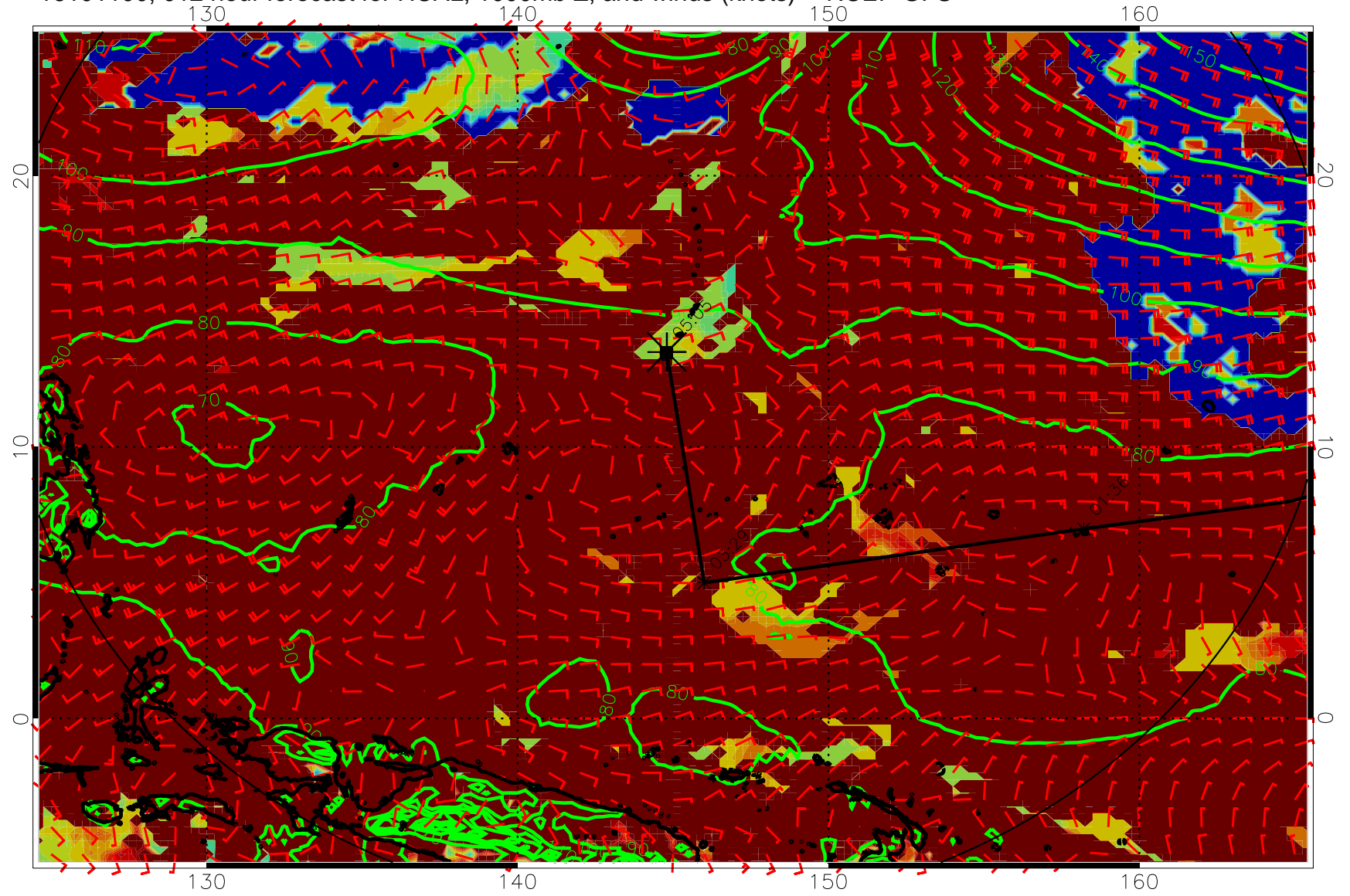
16101100, 012 hour forecast for HCAL, 1000mb Z, and winds (knots) -- NCEP GFS
