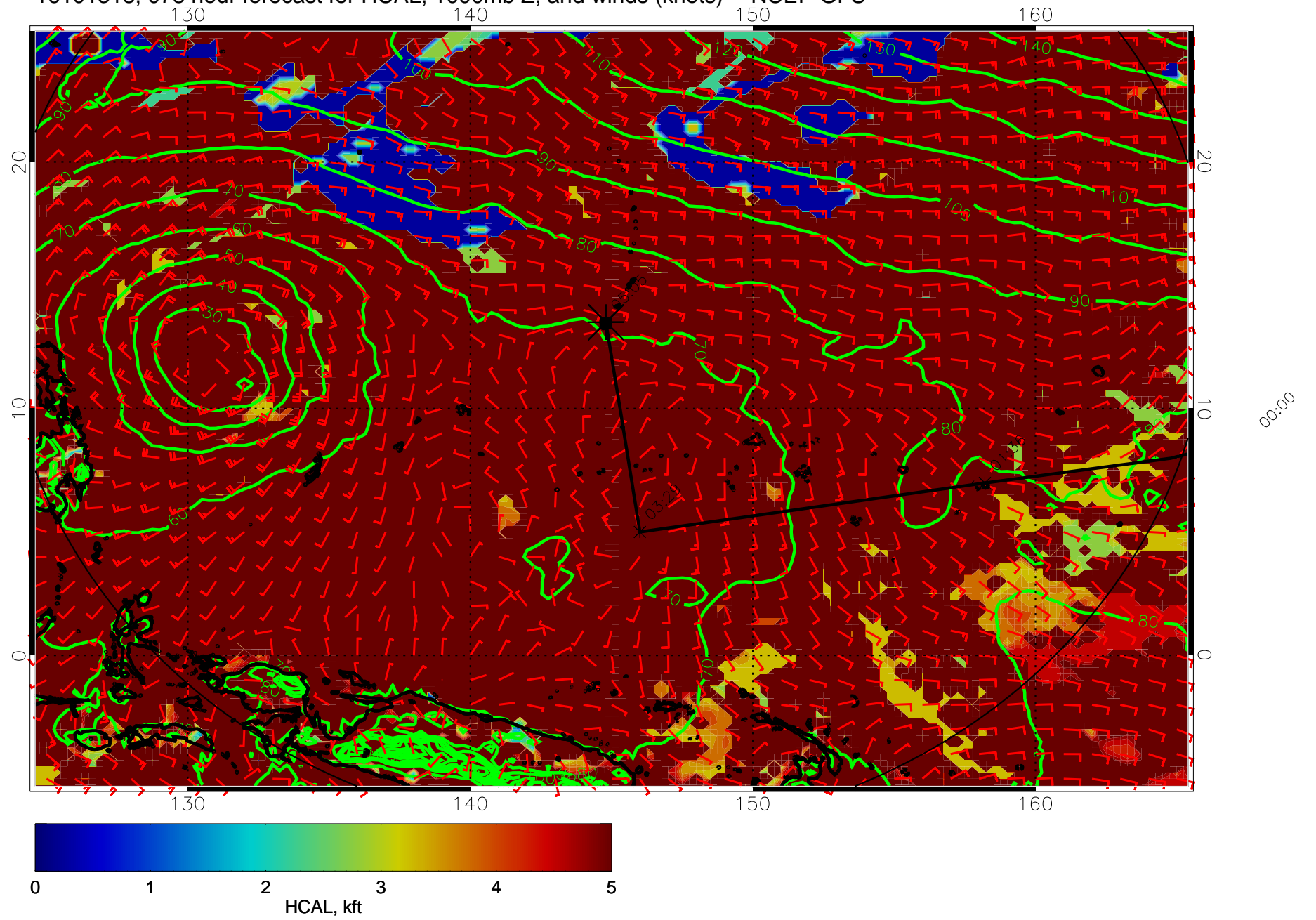
16101318, 078 hour forecast for HCAL, 1000mb Z, and winds (knots) -- NCEP GFS
