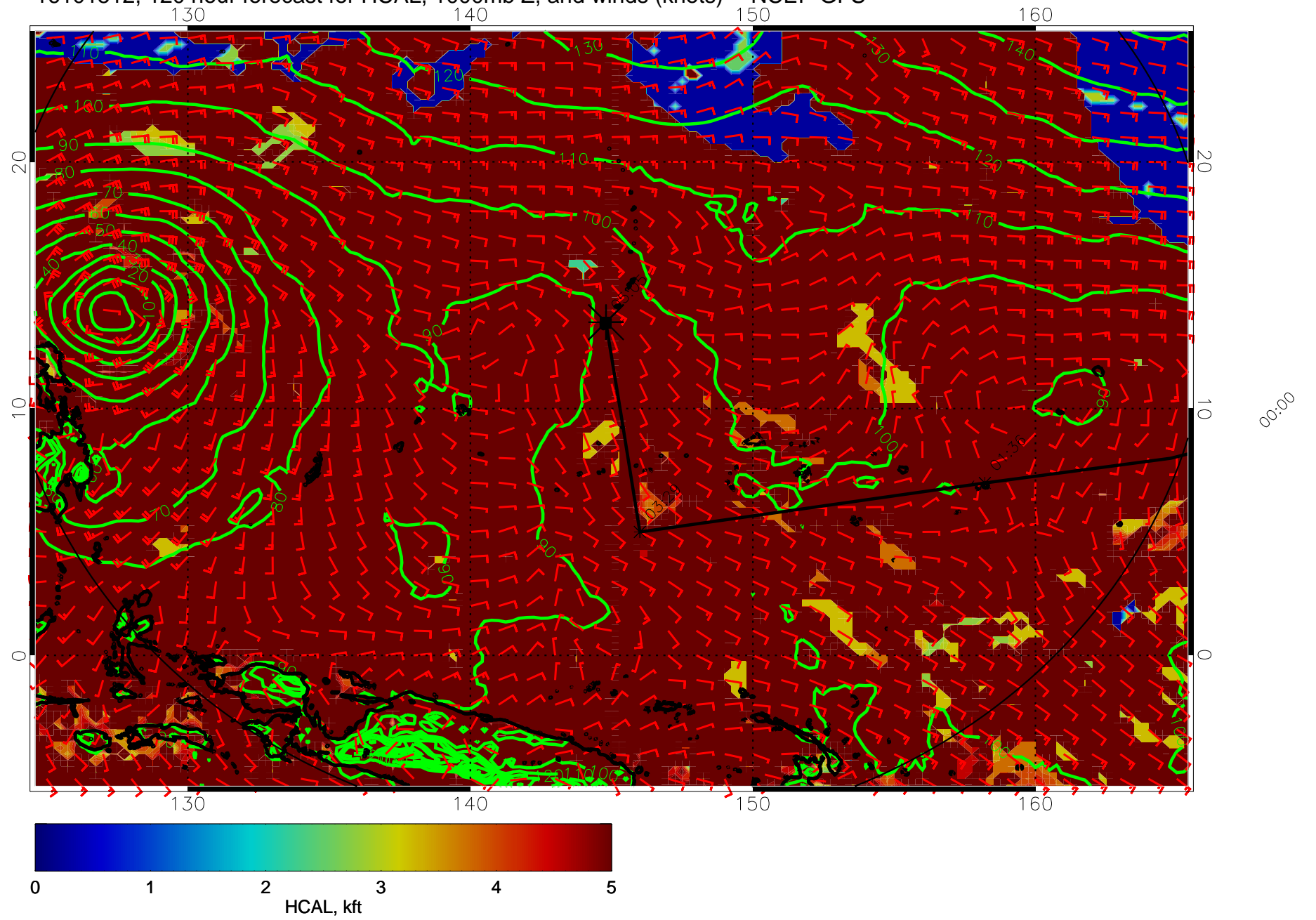
16101512, 120 hour forecast for HCAL, 1000mb Z, and winds (knots) -- NCEP GFS
