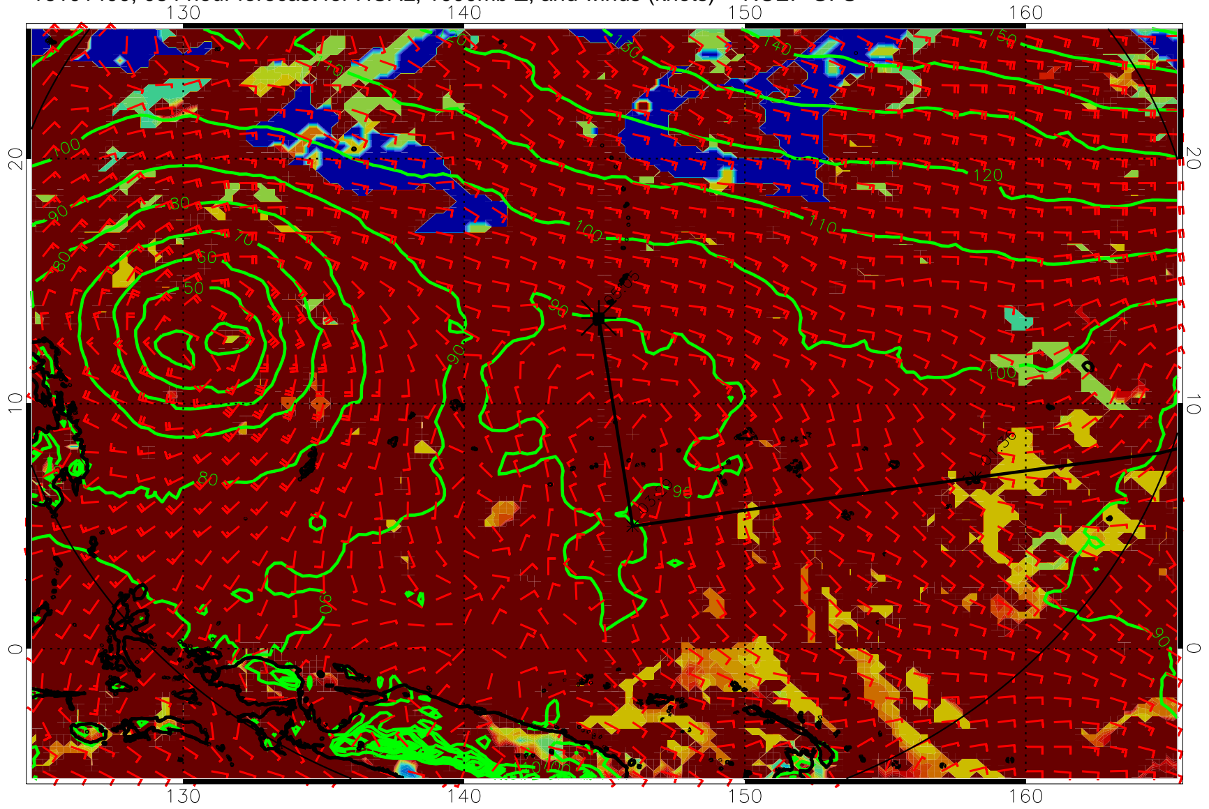
16101400, 084 hour forecast for HCAL, 1000mb Z, and winds (knots) -- NCEP GFS
