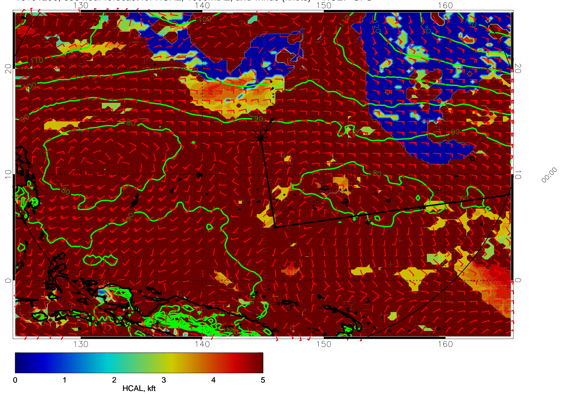
16101200, 036 hour forecast for HCAL, 1000mb Z, and winds (knots) -- NCEP GFS
