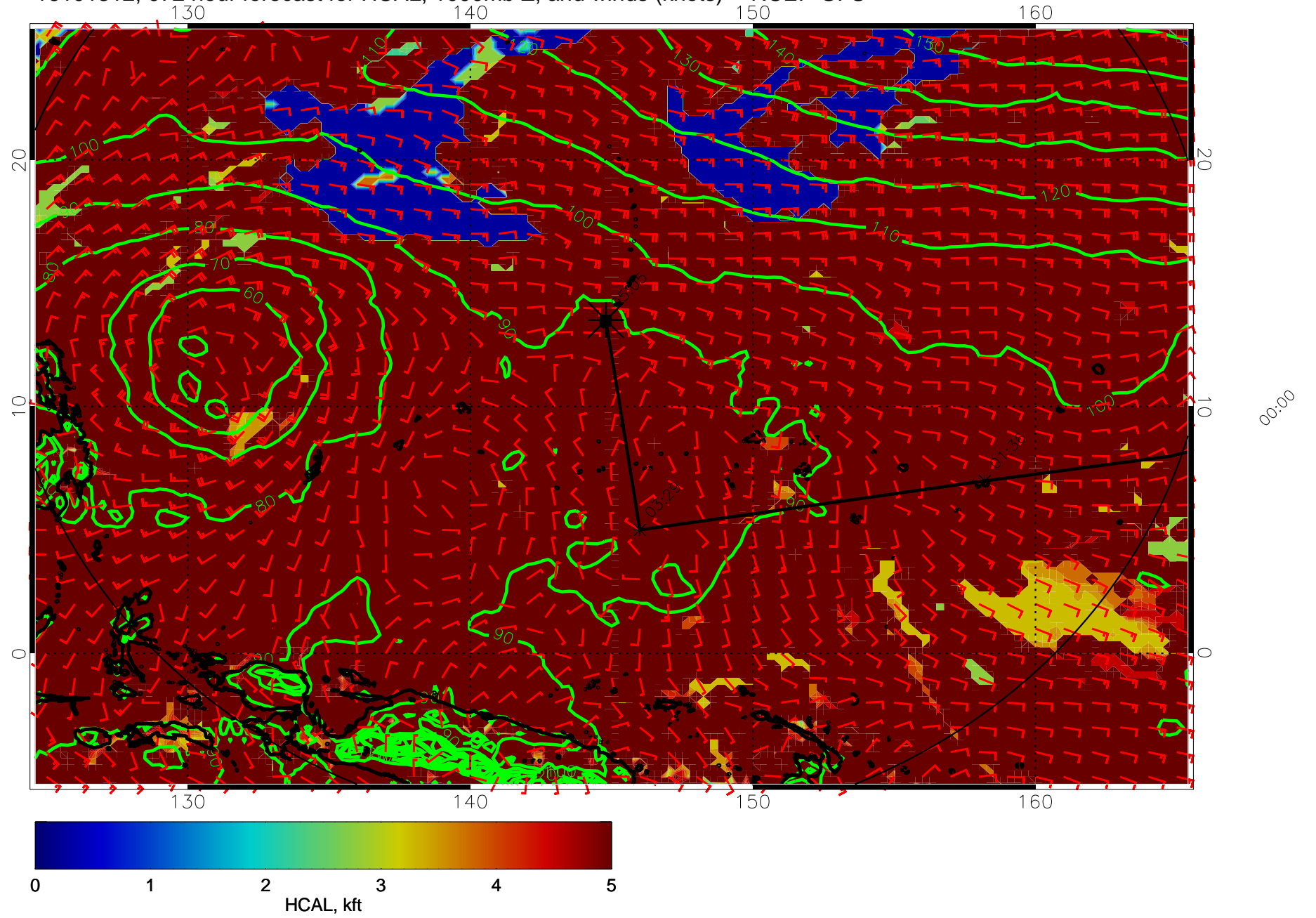
16101312, 072 hour forecast for HCAL, 1000mb Z, and winds (knots) -- NCEP GFS
