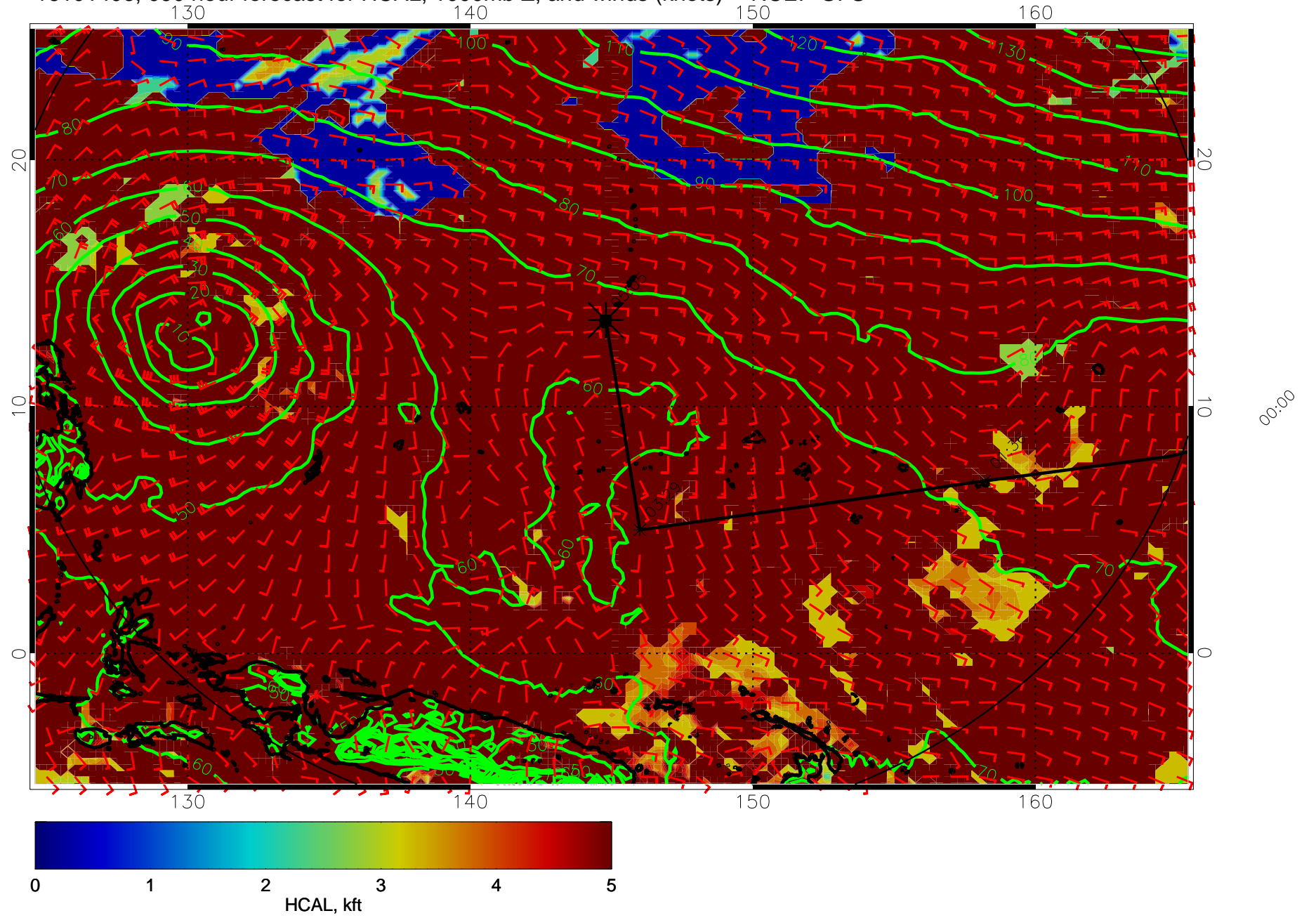
16101406, 090 hour forecast for HCAL, 1000mb Z, and winds (knots) -- NCEP GFS
