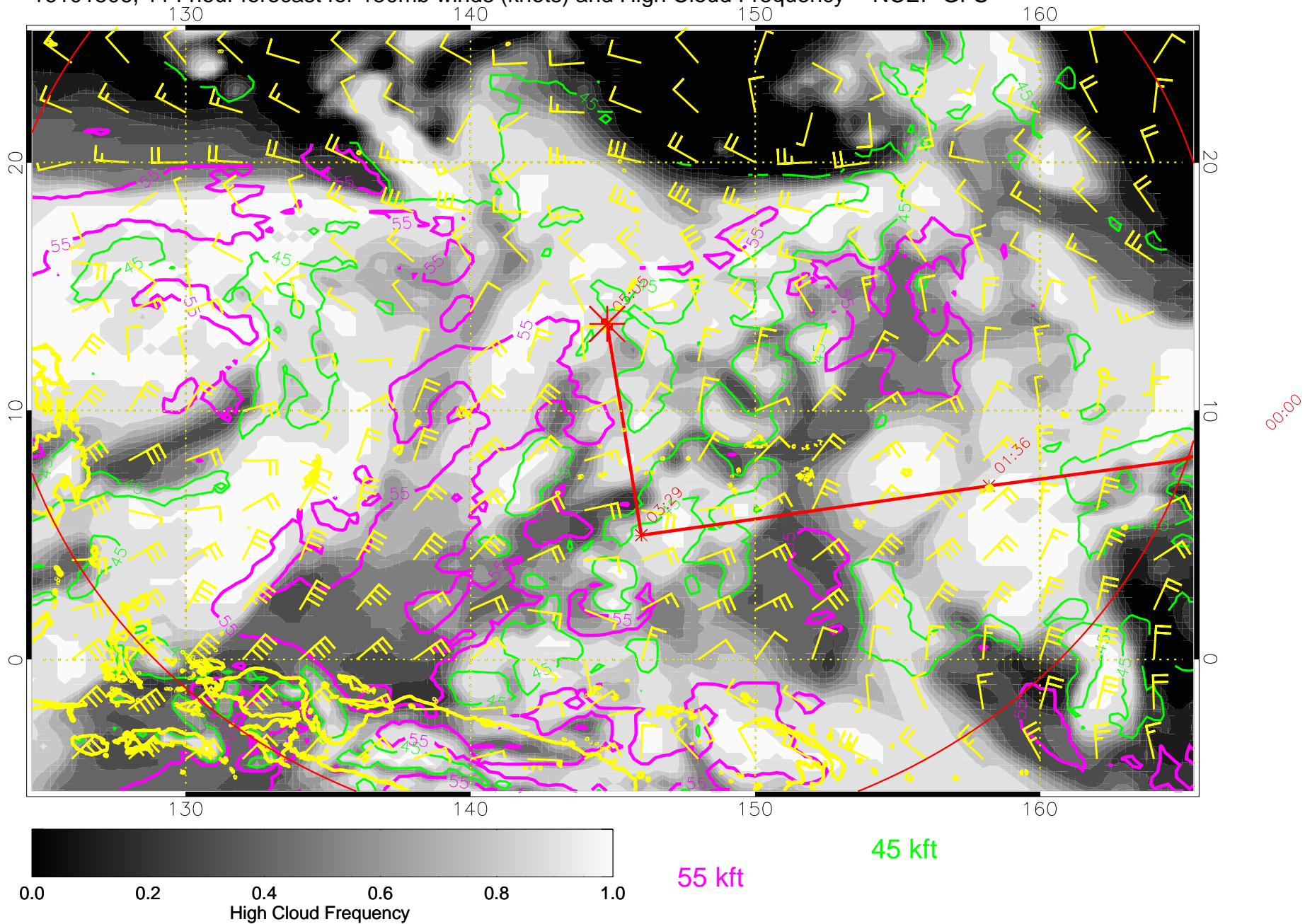
16101506, 114 hour forecast for 150mb winds (knots) and High Cloud Frequency -- NCEP GFS
