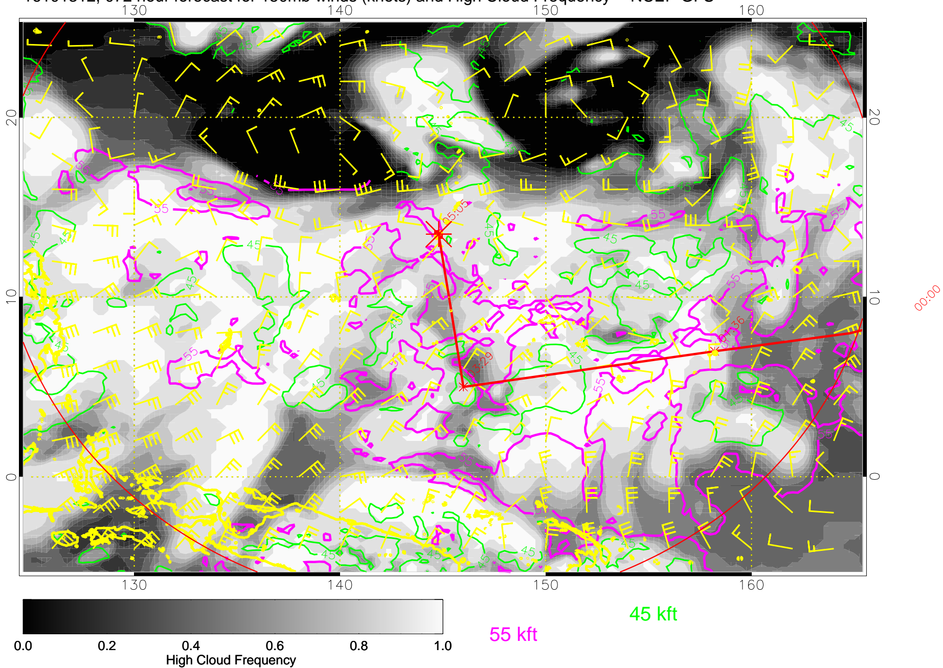
16101312, 072 hour forecast for 150mb winds (knots) and High Cloud Frequency -- NCEP GFS
