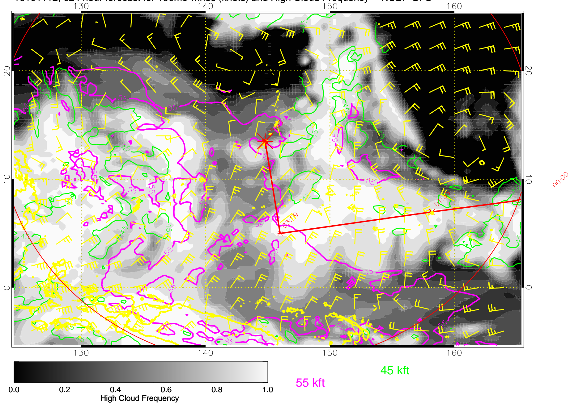
16101112, 024 hour forecast for 150mb winds (knots) and High Cloud Frequency -- NCEP GFS
