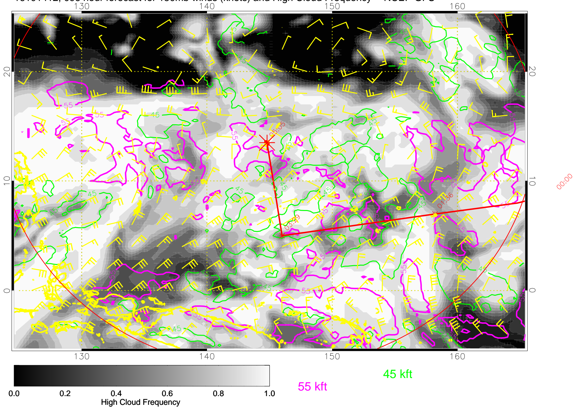
16101412, 096 hour forecast for 150mb winds (knots) and High Cloud Frequency -- NCEP GFS
