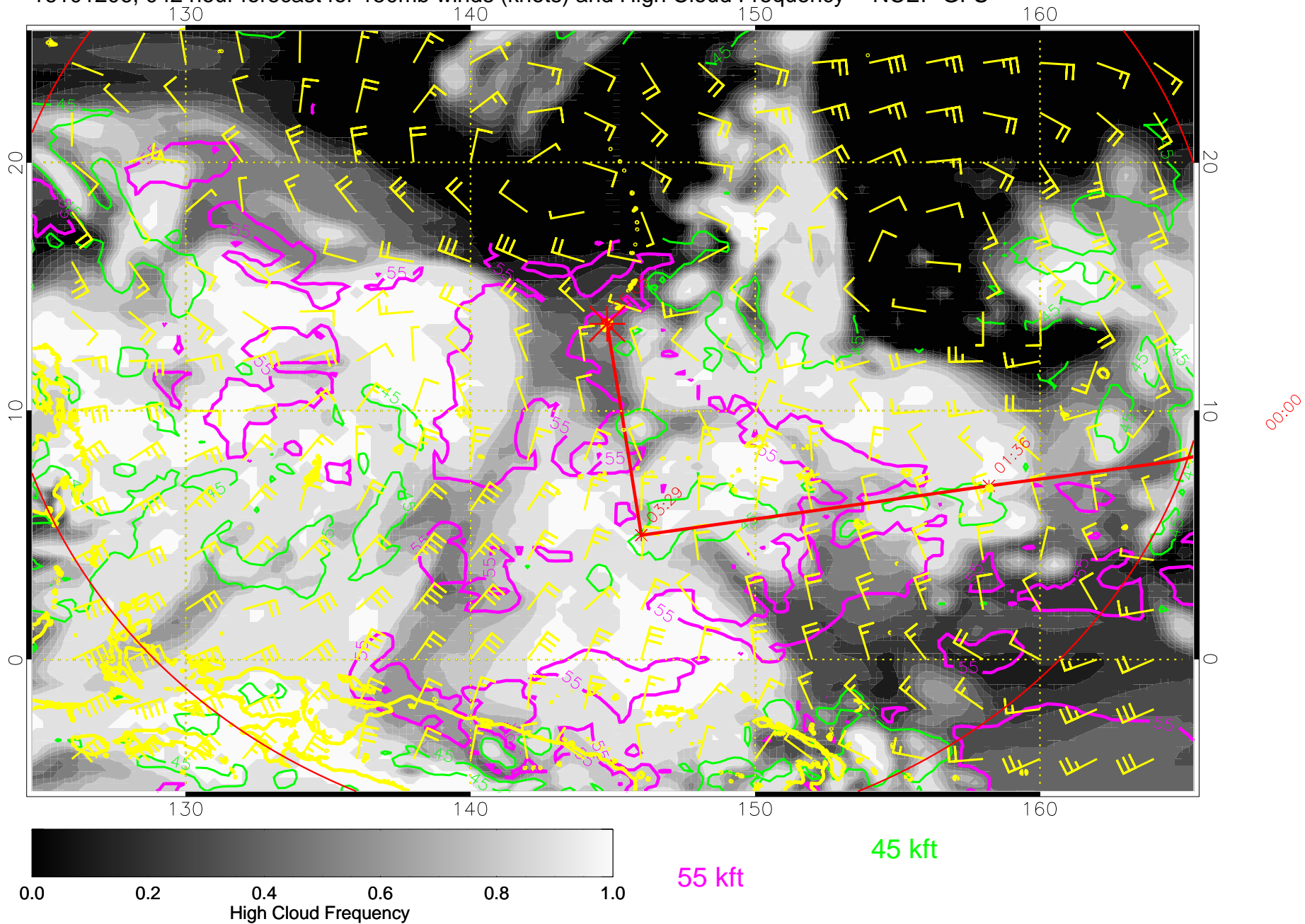
16101206, 042 hour forecast for 150mb winds (knots) and High Cloud Frequency -- NCEP GFS
