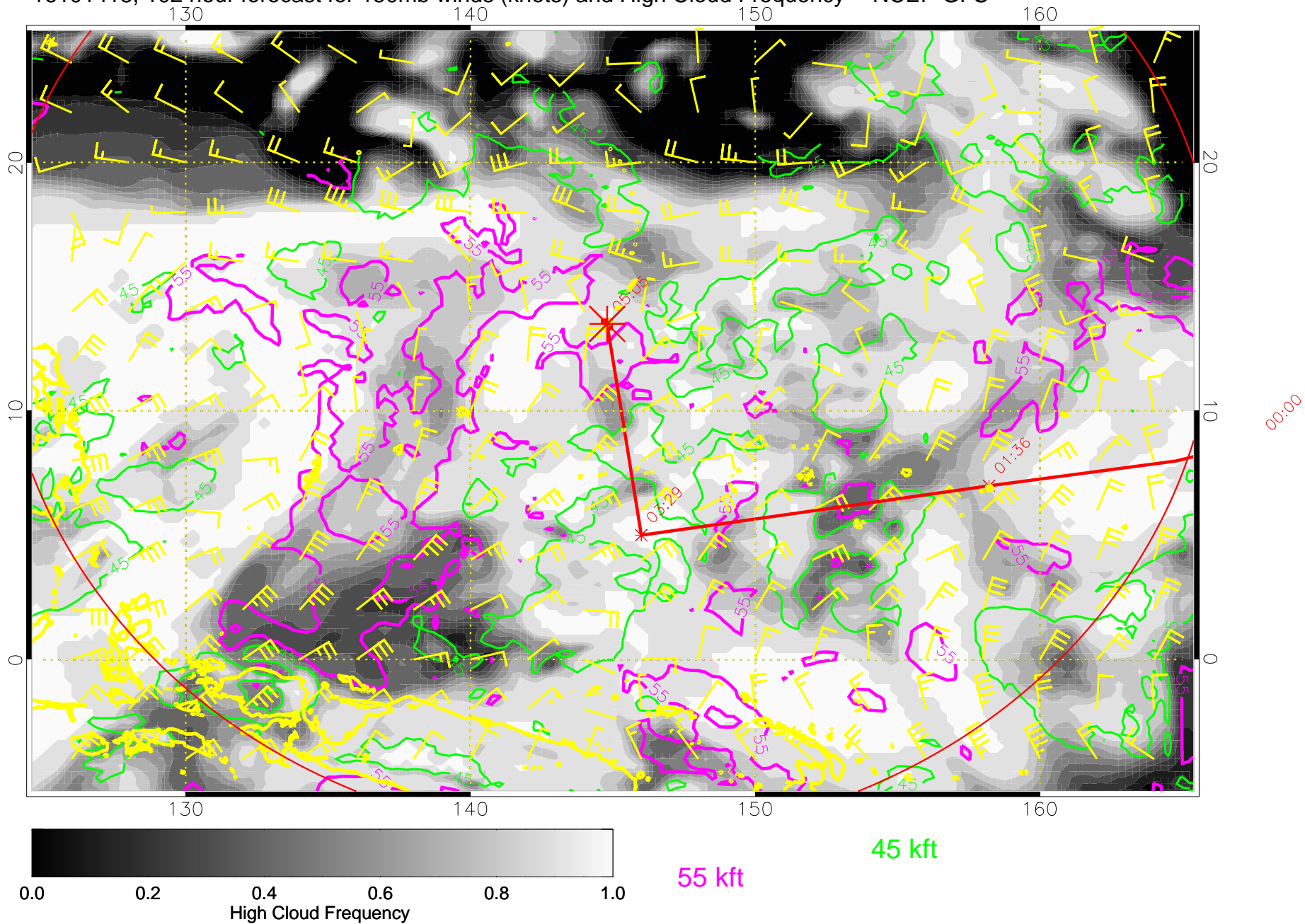
16101418, 102 hour forecast for 150mb winds (knots) and High Cloud Frequency -- NCEP GFS
