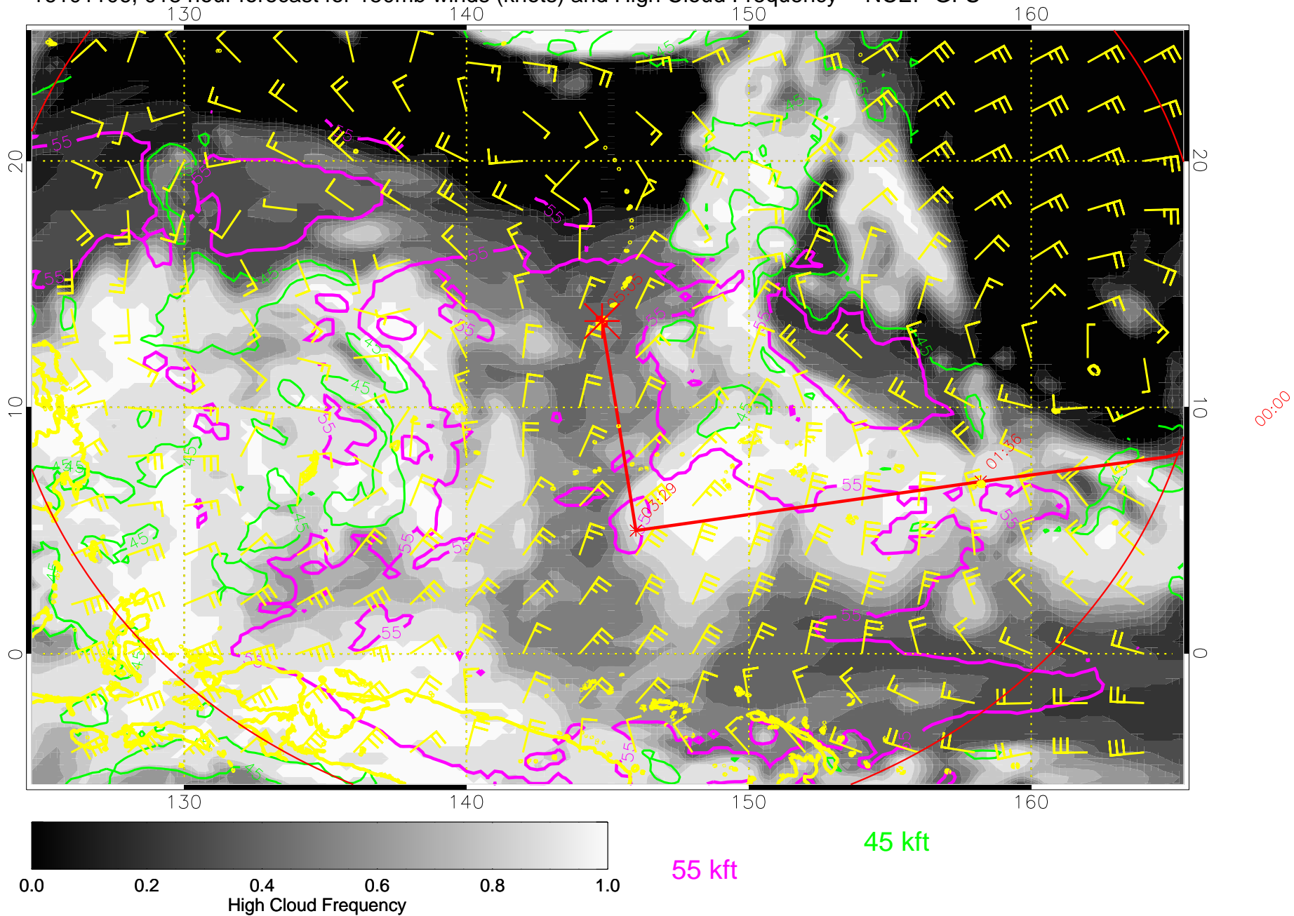
16101106, 018 hour forecast for 150mb winds (knots) and High Cloud Frequency -- NCEP GFS
