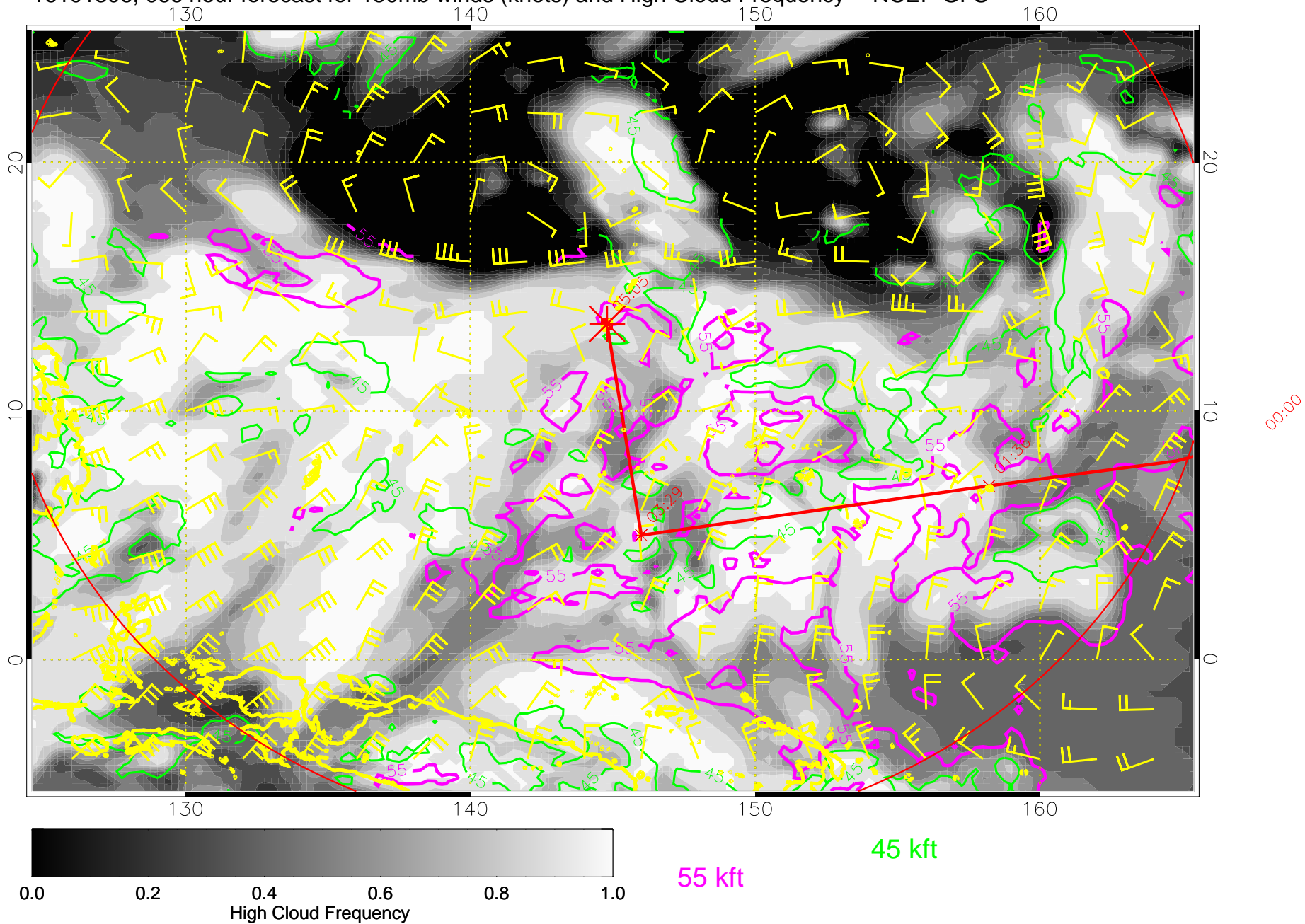
16101306, 066 hour forecast for 150mb winds (knots) and High Cloud Frequency -- NCEP GFS
