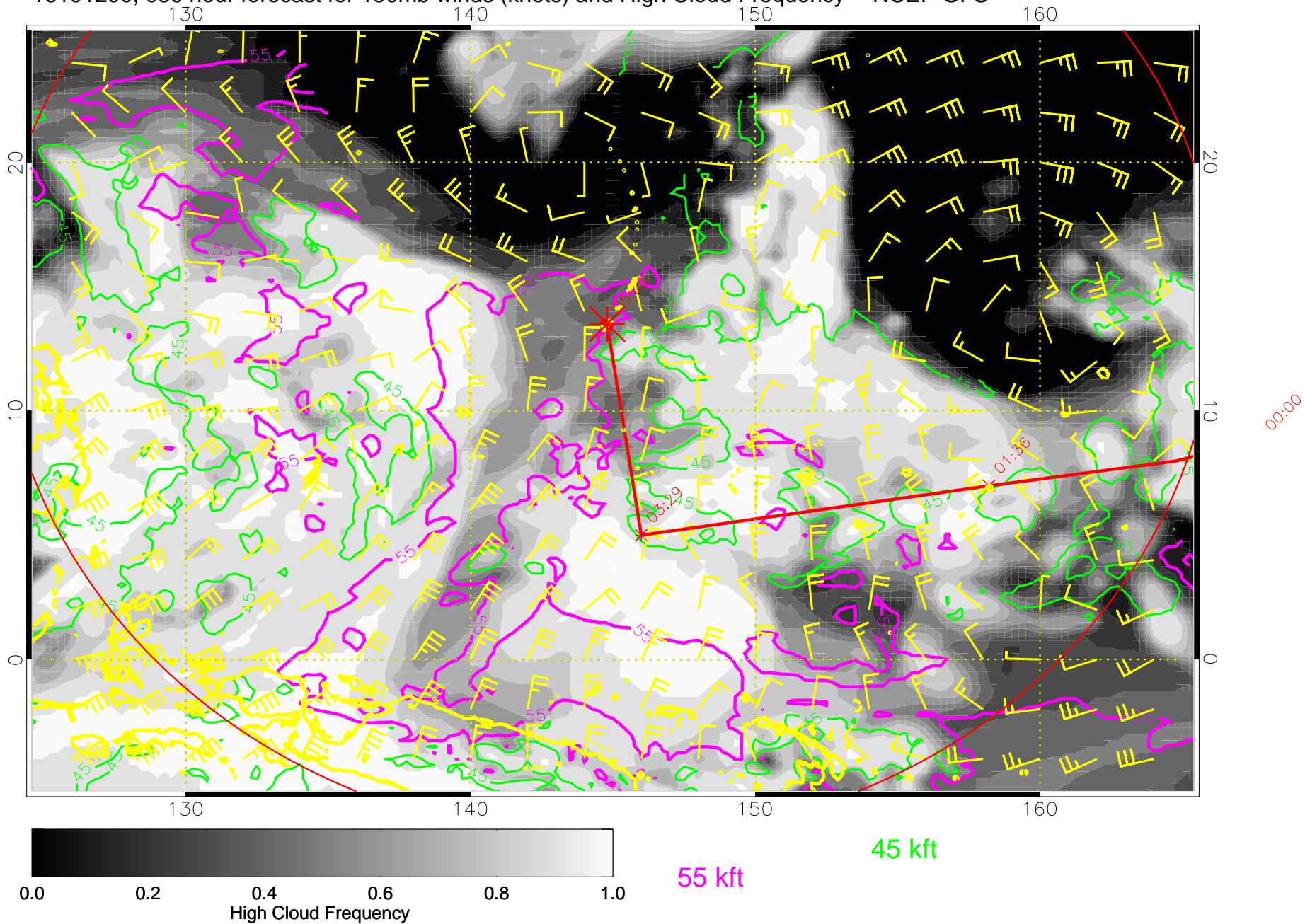
16101200, 036 hour forecast for 150mb winds (knots) and High Cloud Frequency -- NCEP GFS
