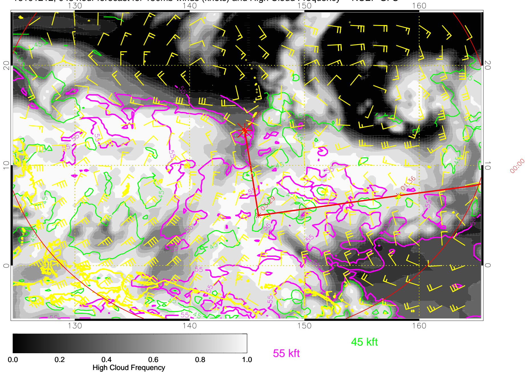
16101212, 048 hour forecast for 150mb winds (knots) and High Cloud Frequency -- NCEP GFS
