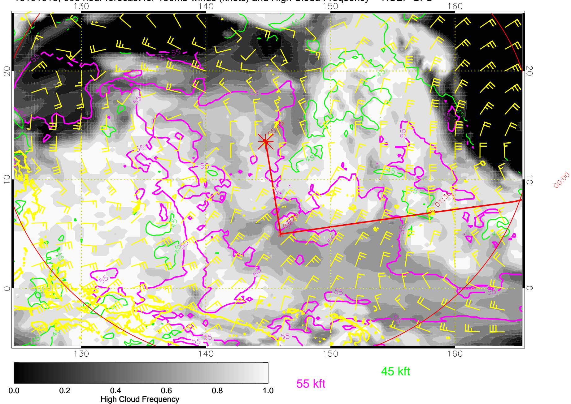
16101018, 006 hour forecast for 150mb winds (knots) and High Cloud Frequency -- NCEP GFS
