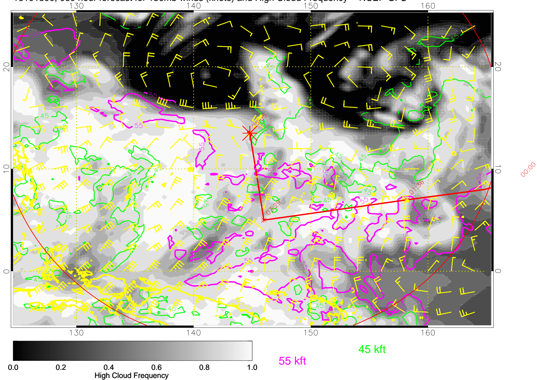
16101300, 060 hour forecast for 150mb winds (knots) and High Cloud Frequency -- NCEP GFS
