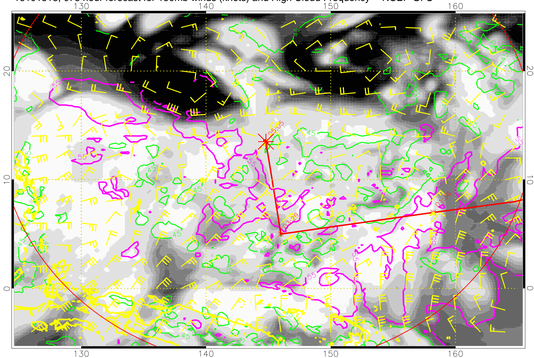
16101318, 078 hour forecast for 150mb winds (knots) and High Cloud Frequency -- NCEP GFS
