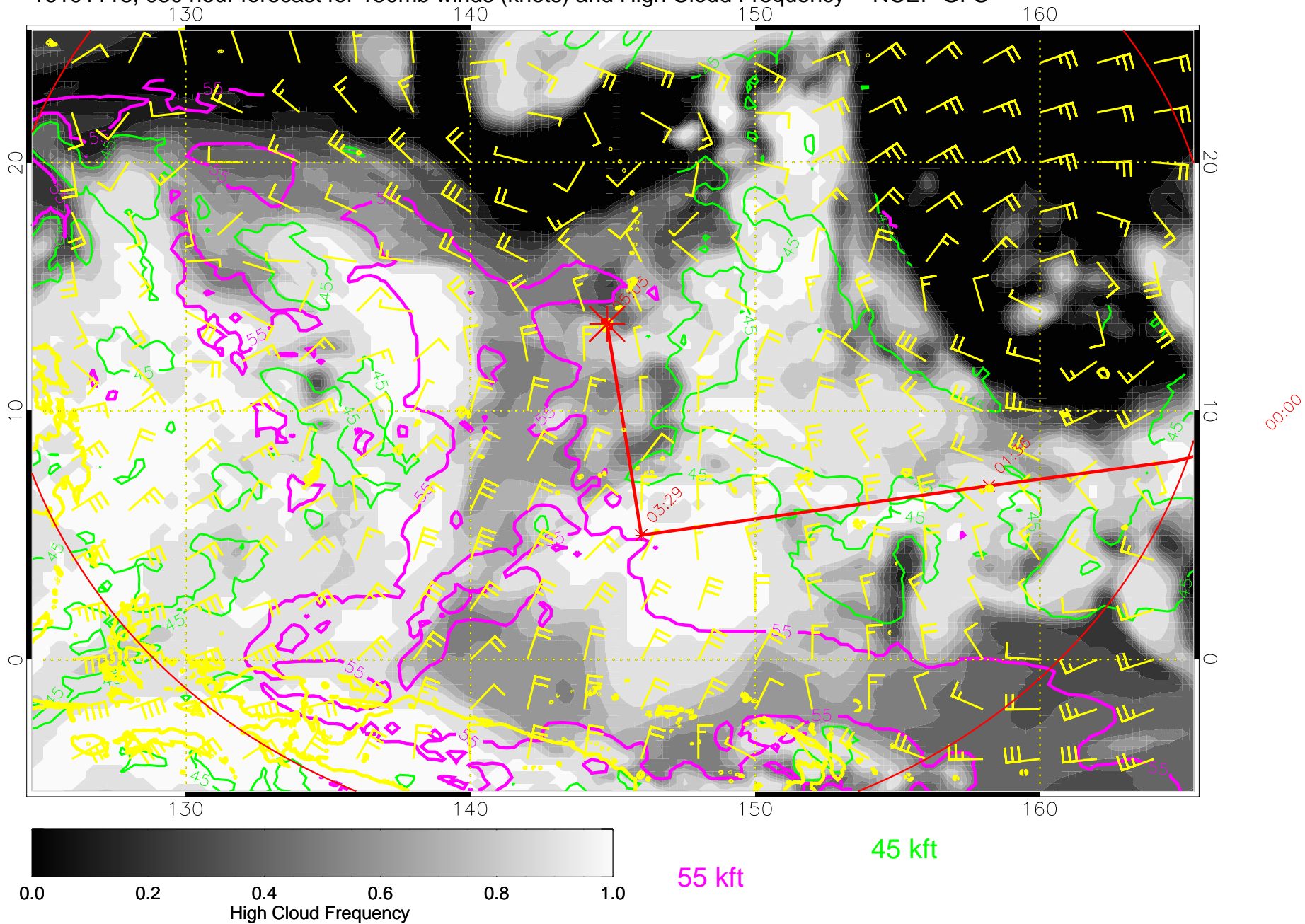
16101118, 030 hour forecast for 150mb winds (knots) and High Cloud Frequency -- NCEP GFS
