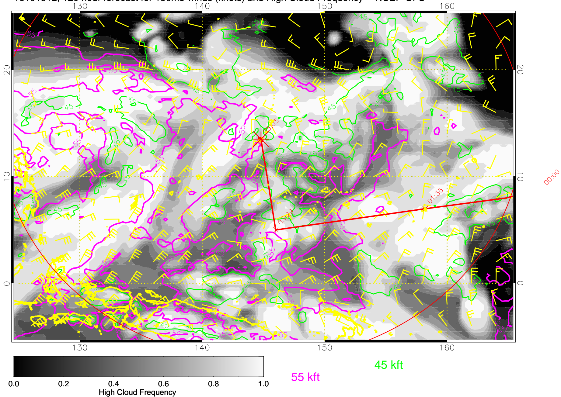
16101512, 120 hour forecast for 150mb winds (knots) and High Cloud Frequency -- NCEP GFS
