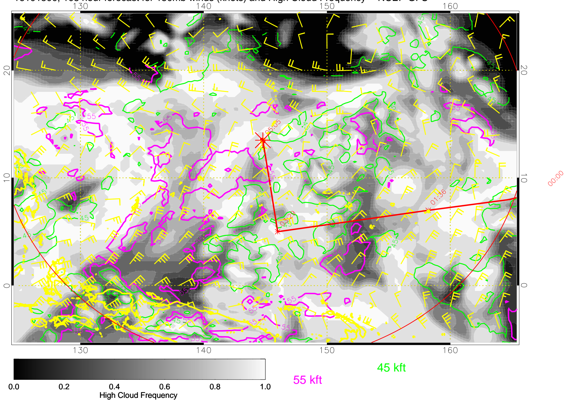
16101500, 108 hour forecast for 150mb winds (knots) and High Cloud Frequency -- NCEP GFS
