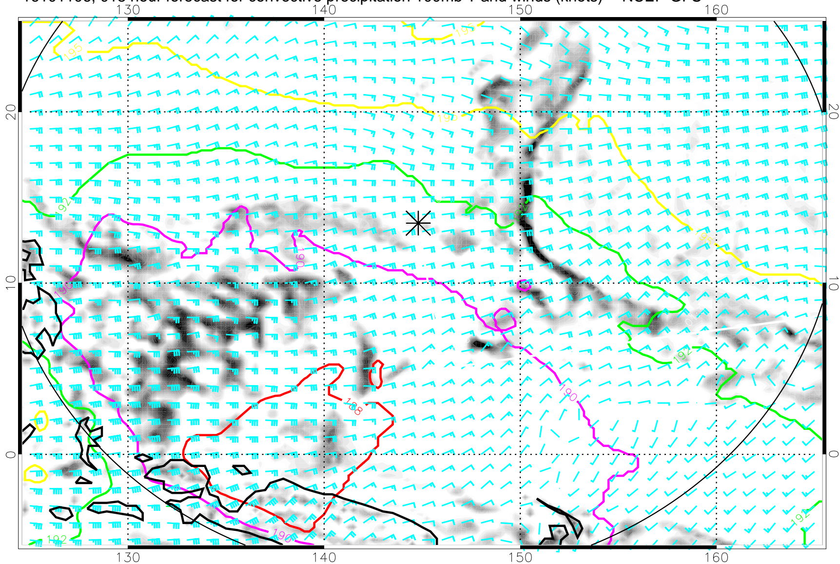
16101106, 018 hour forecast for convective precipitation 100mb T and winds (knots) -- NCEP GFS
