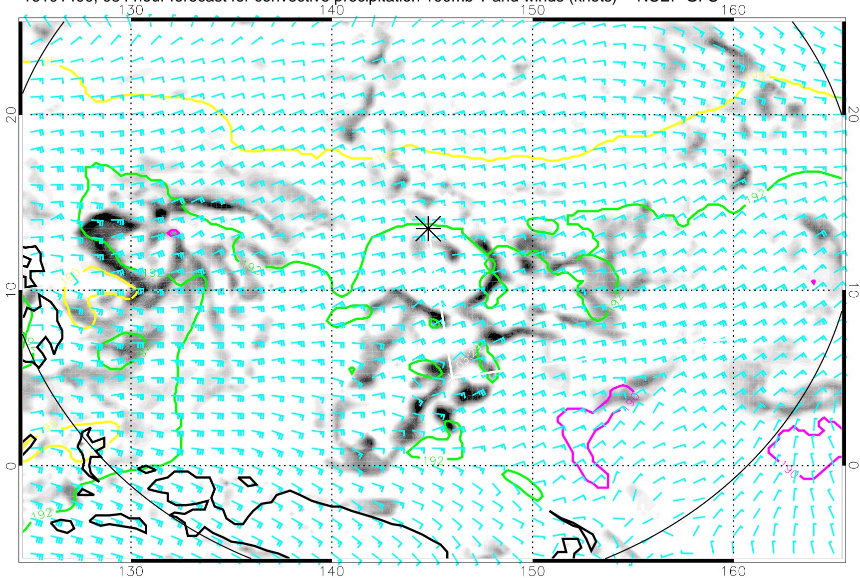
16101400, 084 hour forecast for convective precipitation 100mb T and winds (knots) -- NCEP GFS
