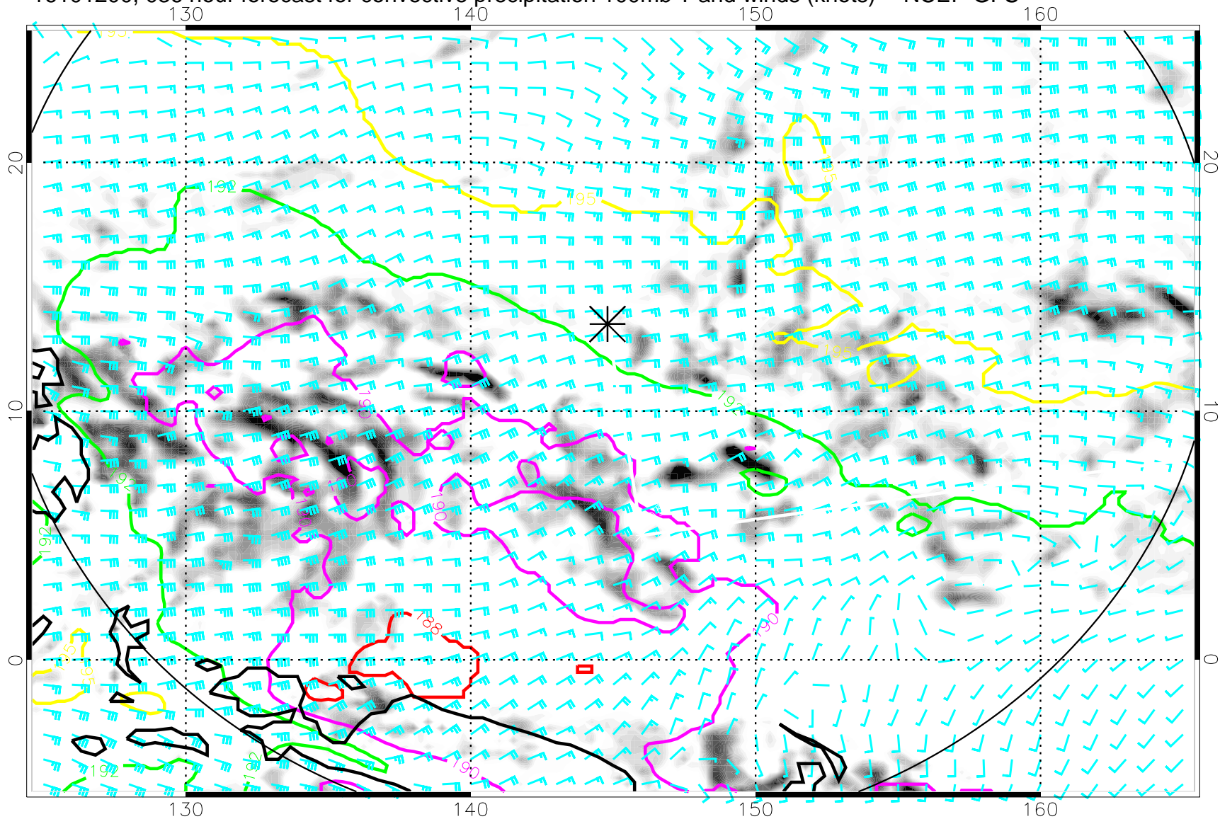
16101200, 036 hour forecast for convective precipitation 100mb T and winds (knots) -- NCEP GFS
