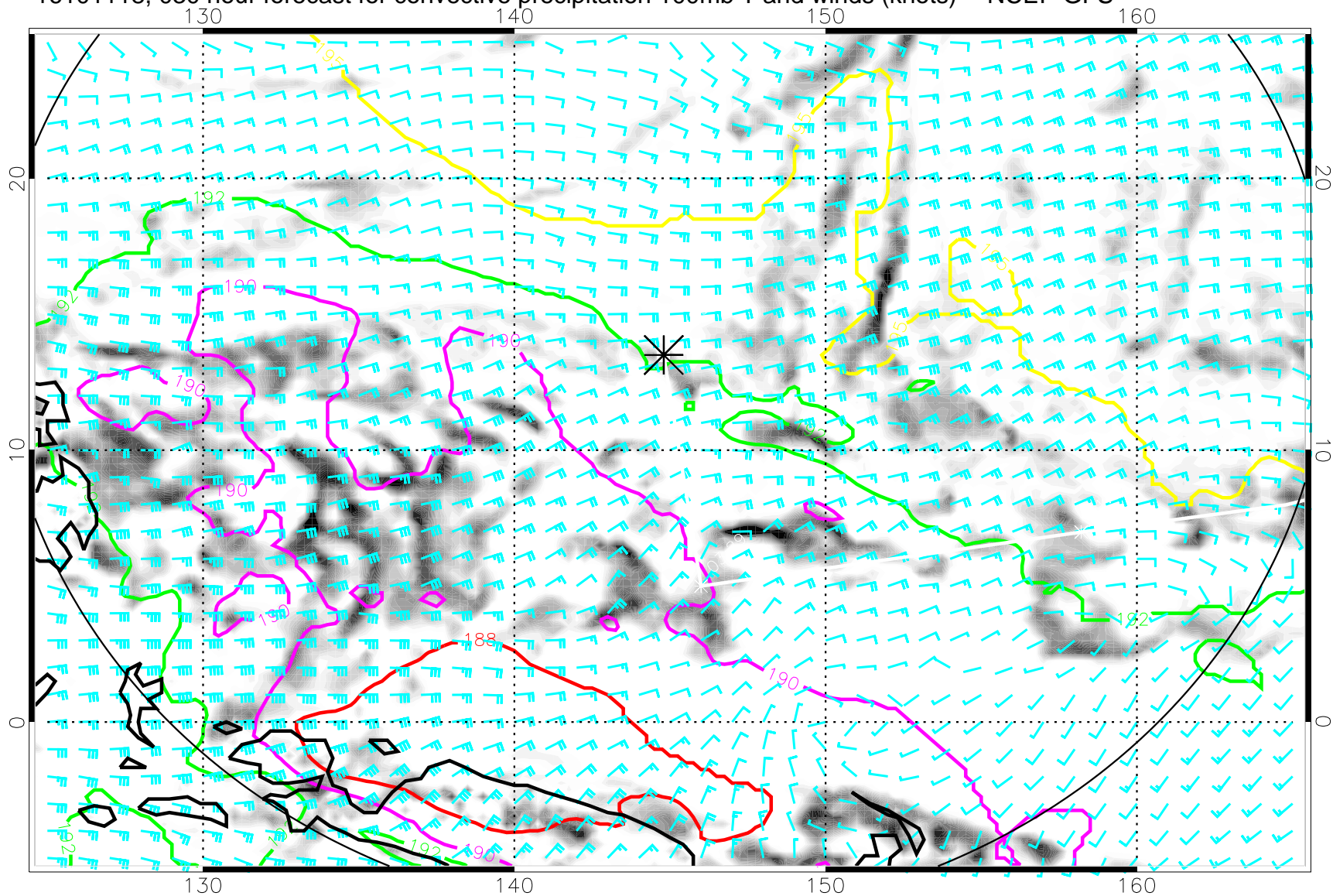
16101118, 030 hour forecast for convective precipitation 100mb T and winds (knots) -- NCEP GFS
