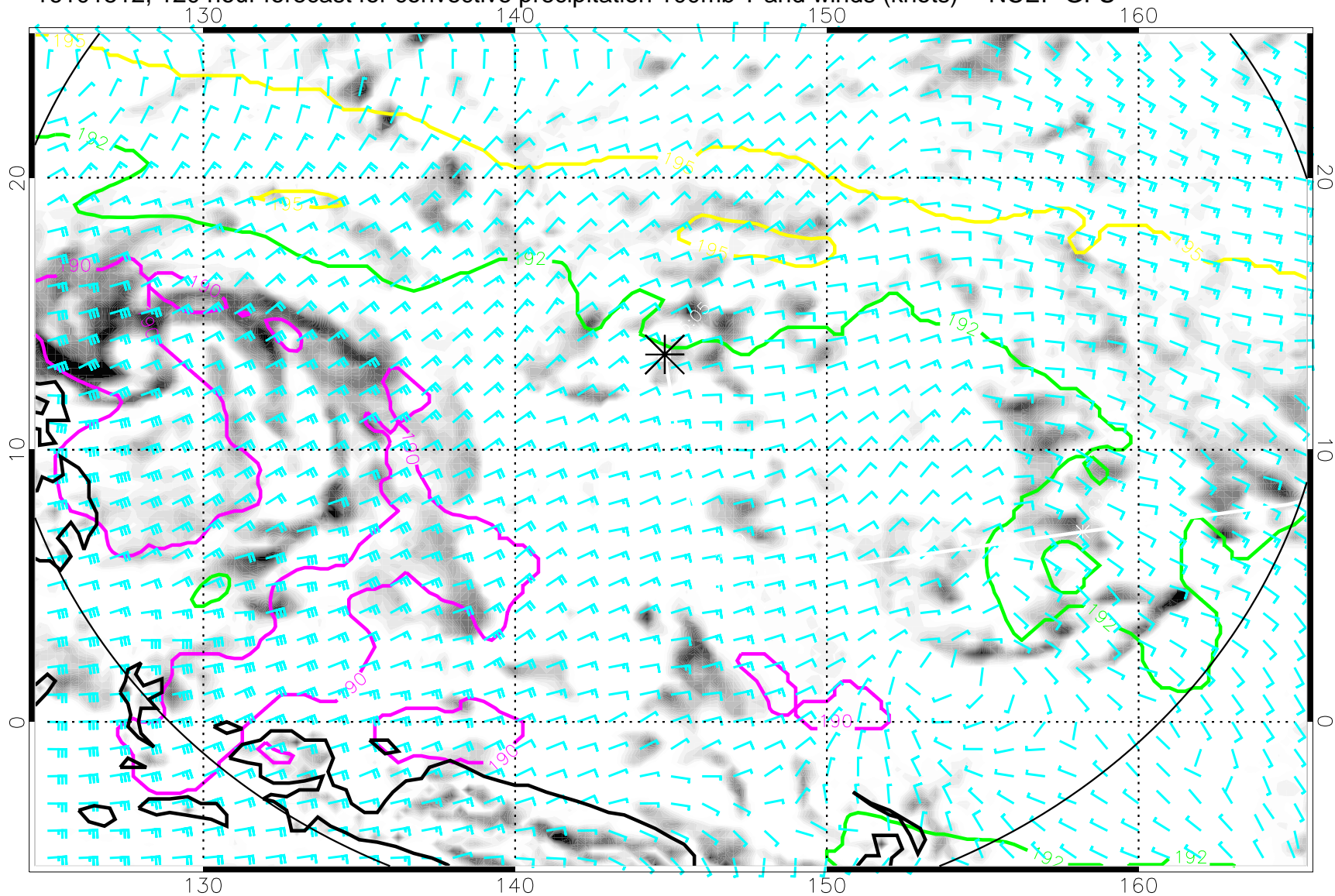
16101512, 120 hour forecast for convective precipitation 100mb T and winds (knots) -- NCEP GFS
