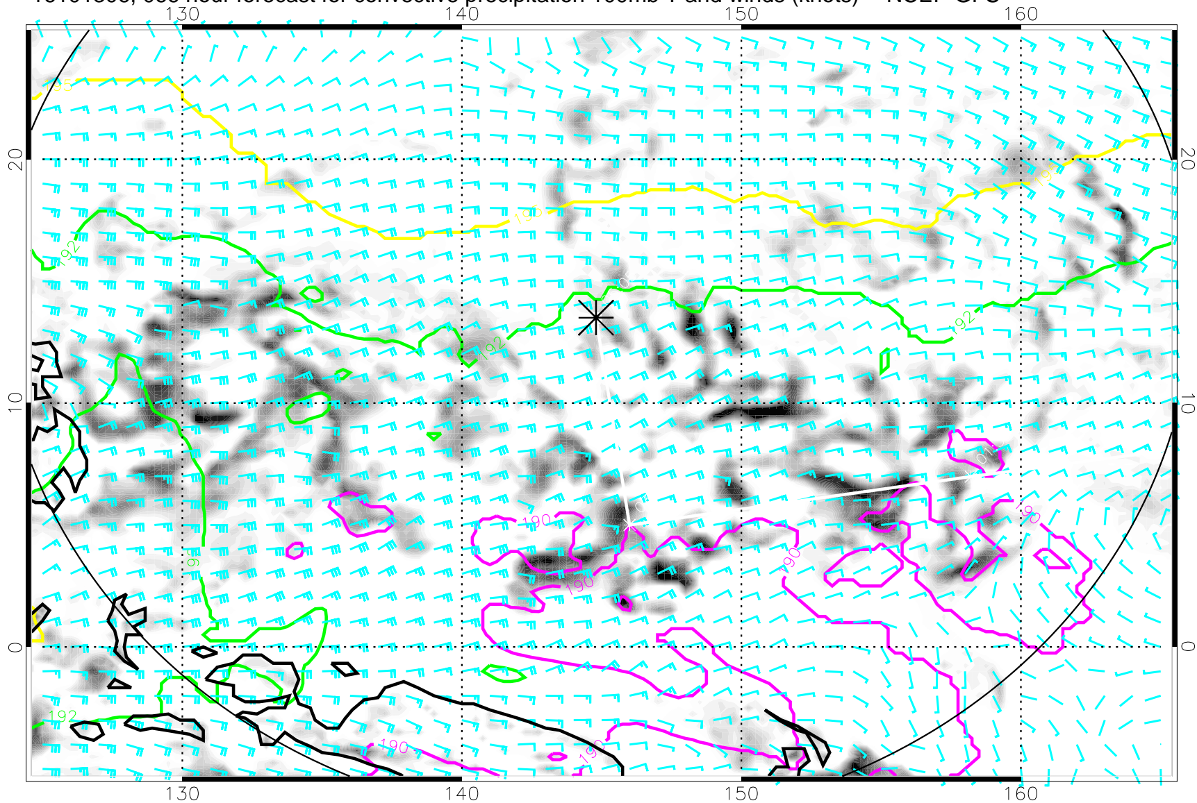
16101306, 066 hour forecast for convective precipitation 100mb T and winds (knots) -- NCEP GFS
