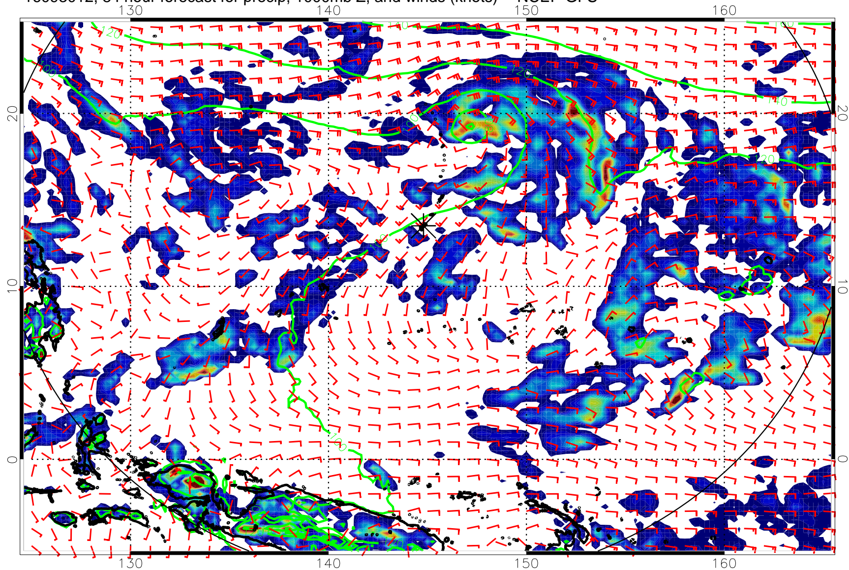
16093012, 84 hour forecast for precip, 1000mb Z, and winds (knots) -- NCEP GFS
