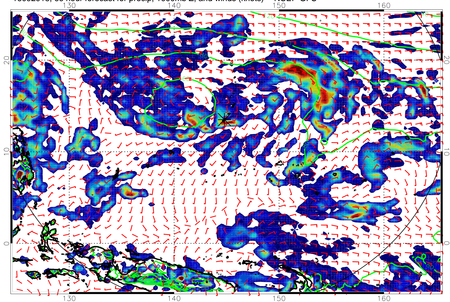
16092918, 66 hour forecast for precip, 1000mb Z, and winds (knots) -- NCEP GFS
