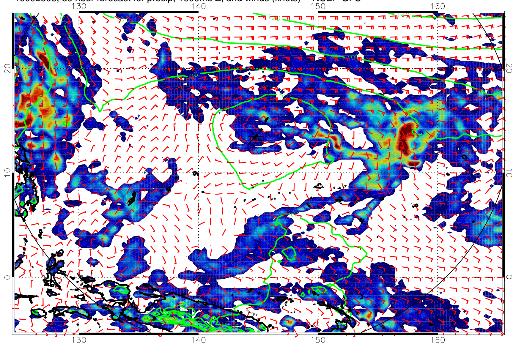
16092806, 30 hour forecast for precip, 1000mb Z, and winds (knots) -- NCEP GFS
