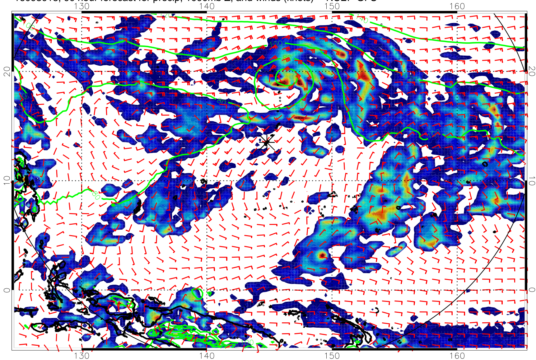
16093018, 90 hour forecast for precip, 1000mb Z, and winds (knots) -- NCEP GFS
