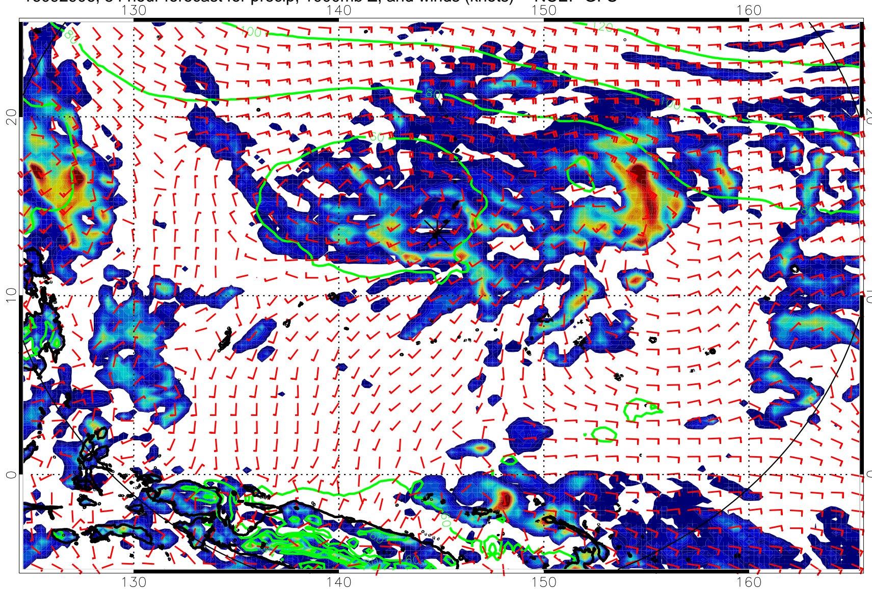
16092906, 54 hour forecast for precip, 1000mb Z, and winds (knots) -- NCEP GFS
