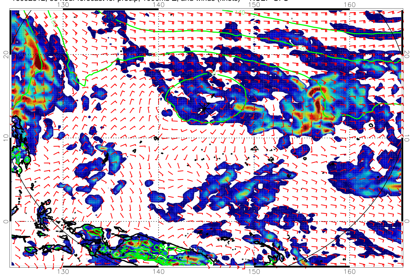
16092812, 36 hour forecast for precip, 1000mb Z, and winds (knots) -- NCEP GFS
