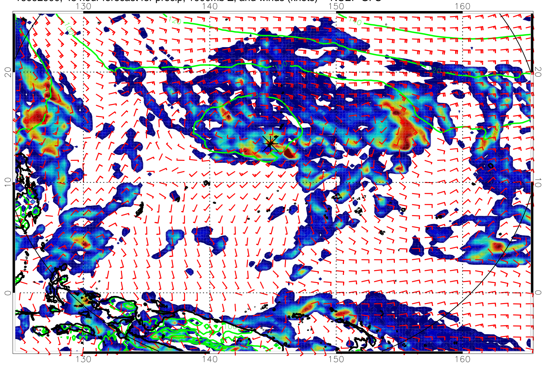
16092900, 48 hour forecast for precip, 1000mb Z, and winds (knots) -- NCEP GFS
