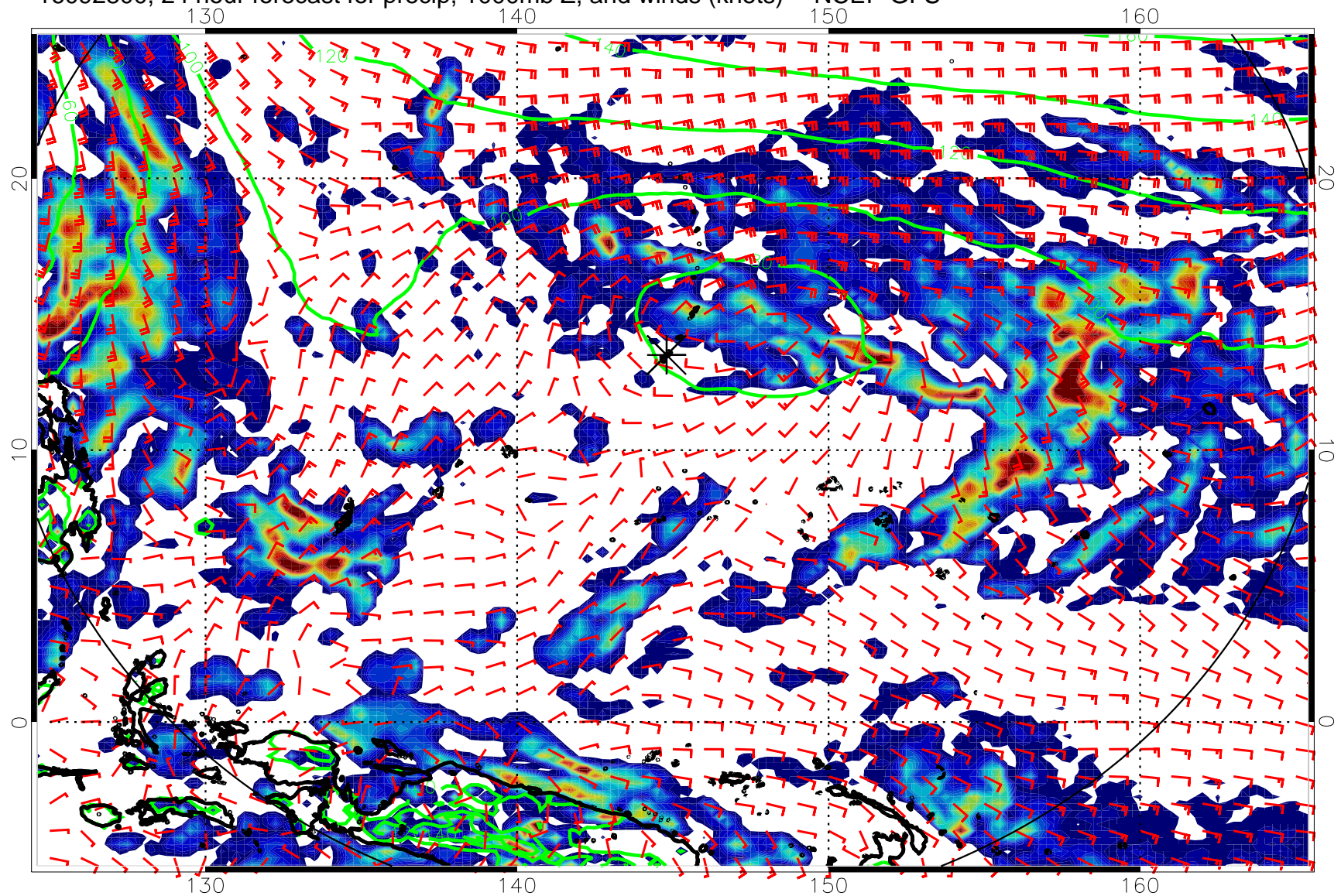
16092800, 24 hour forecast for precip, 1000mb Z, and winds (knots) -- NCEP GFS
