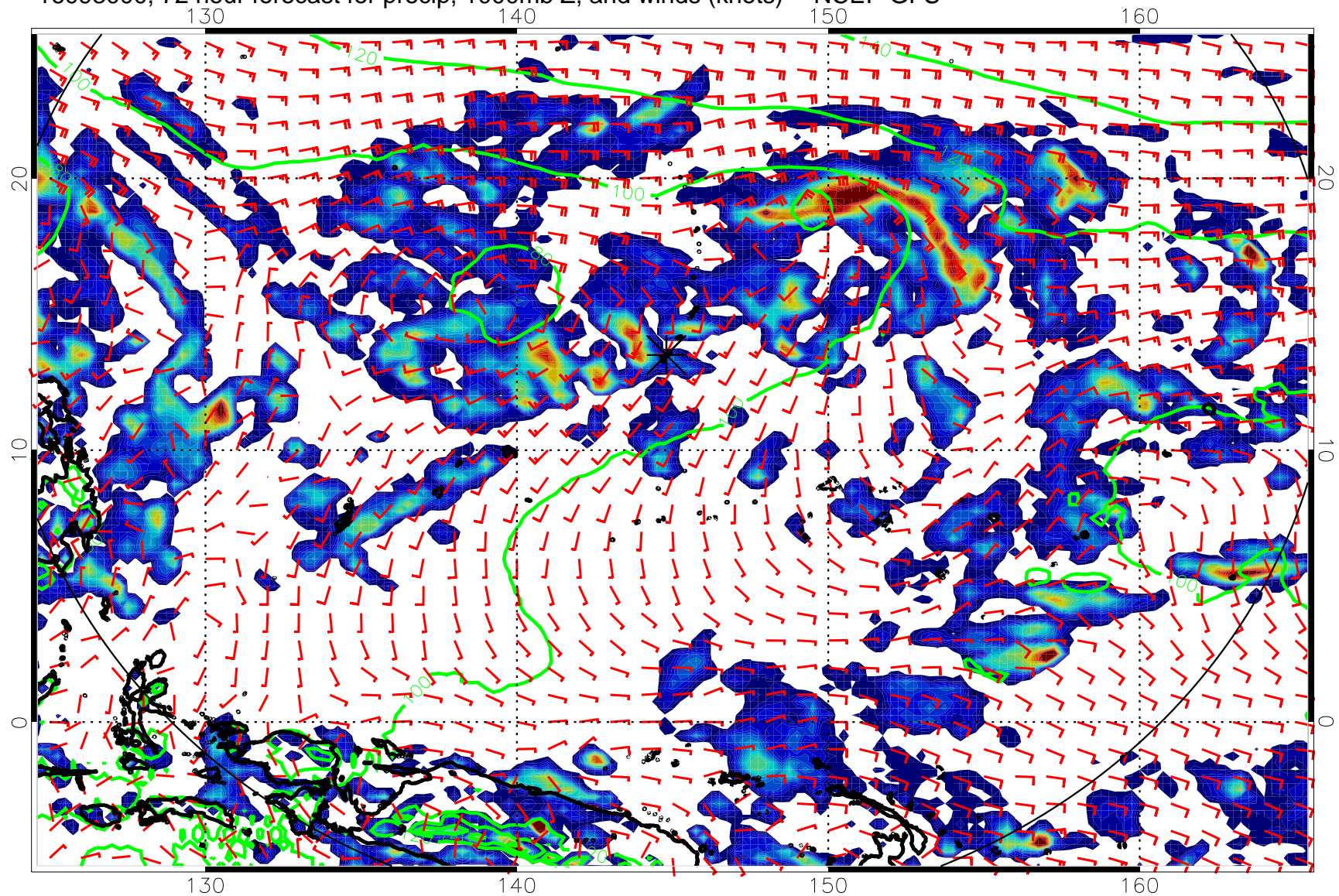
16093000, 72 hour forecast for precip, 1000mb Z, and winds (knots) -- NCEP GFS
