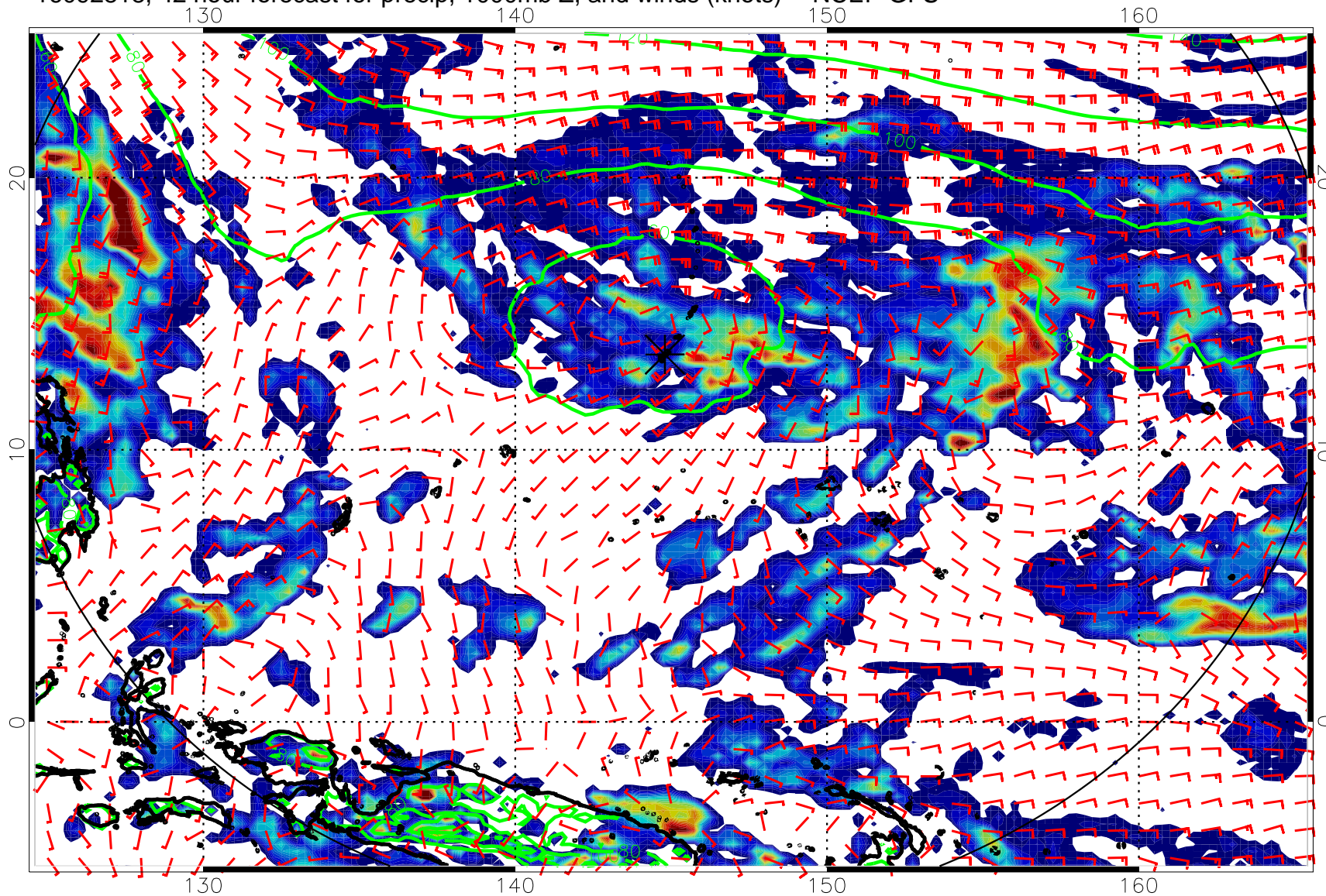
16092818, 42 hour forecast for precip, 1000mb Z, and winds (knots) -- NCEP GFS
