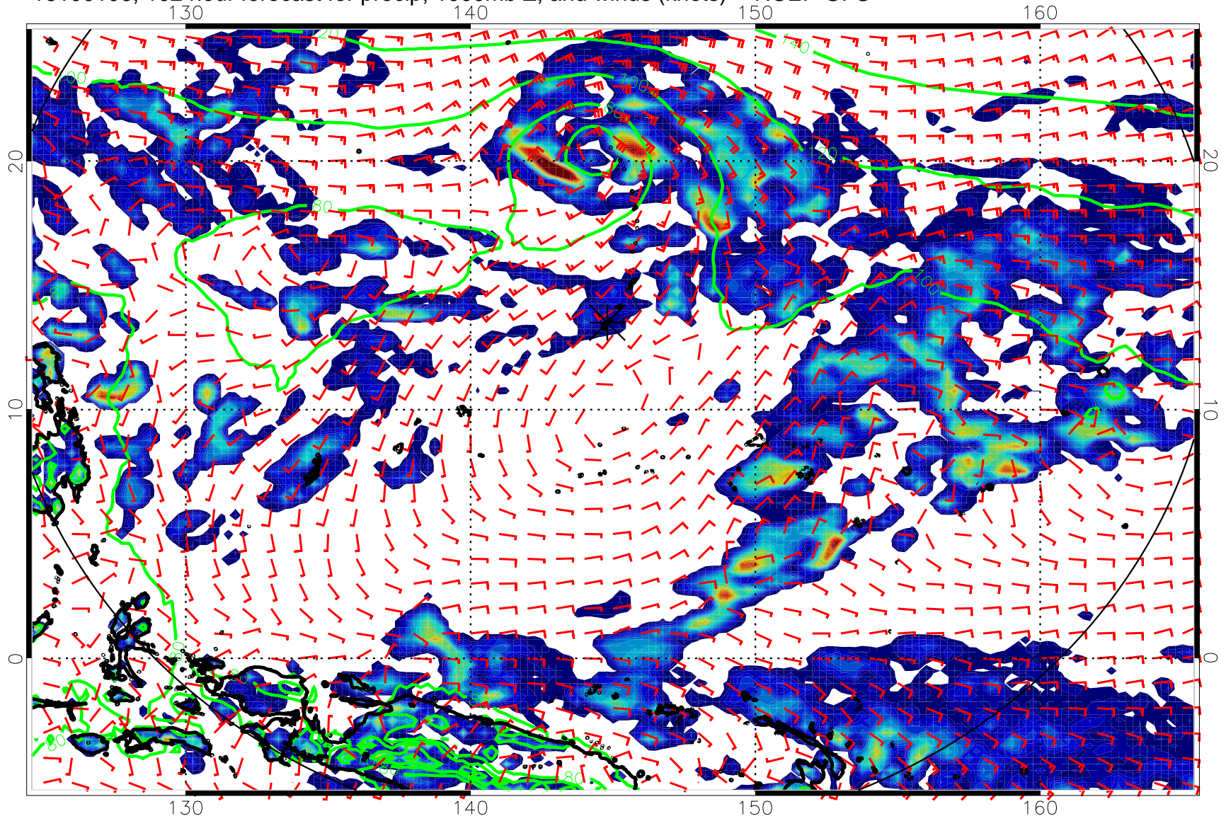
16100106, 102 hour forecast for precip, 1000mb Z, and winds (knots) -- NCEP GFS
