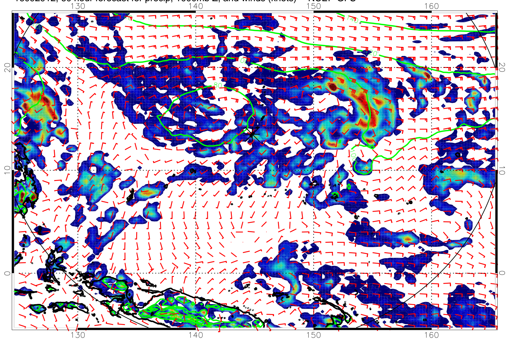
16092912, 60 hour forecast for precip, 1000mb Z, and winds (knots) -- NCEP GFS
