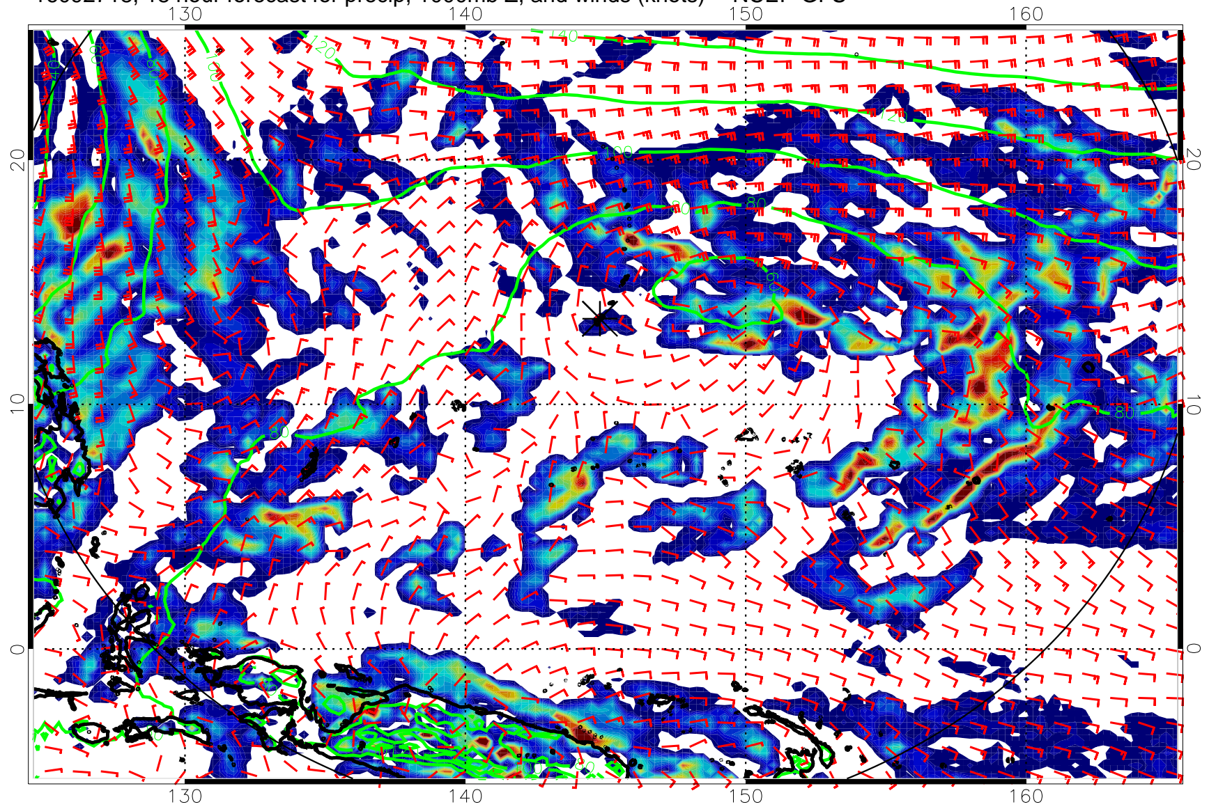
16092718, 18 hour forecast for precip, 1000mb Z, and winds (knots) -- NCEP GFS
