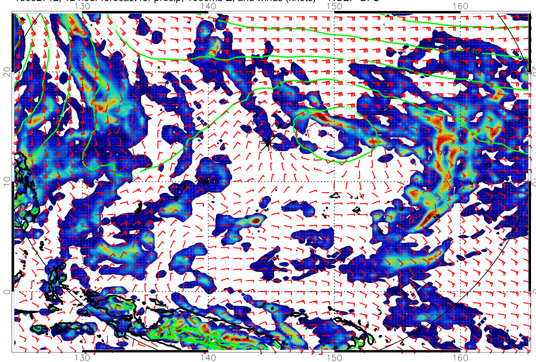
16092712, 12 hour forecast for precip, 1000mb Z, and winds (knots) -- NCEP GFS
