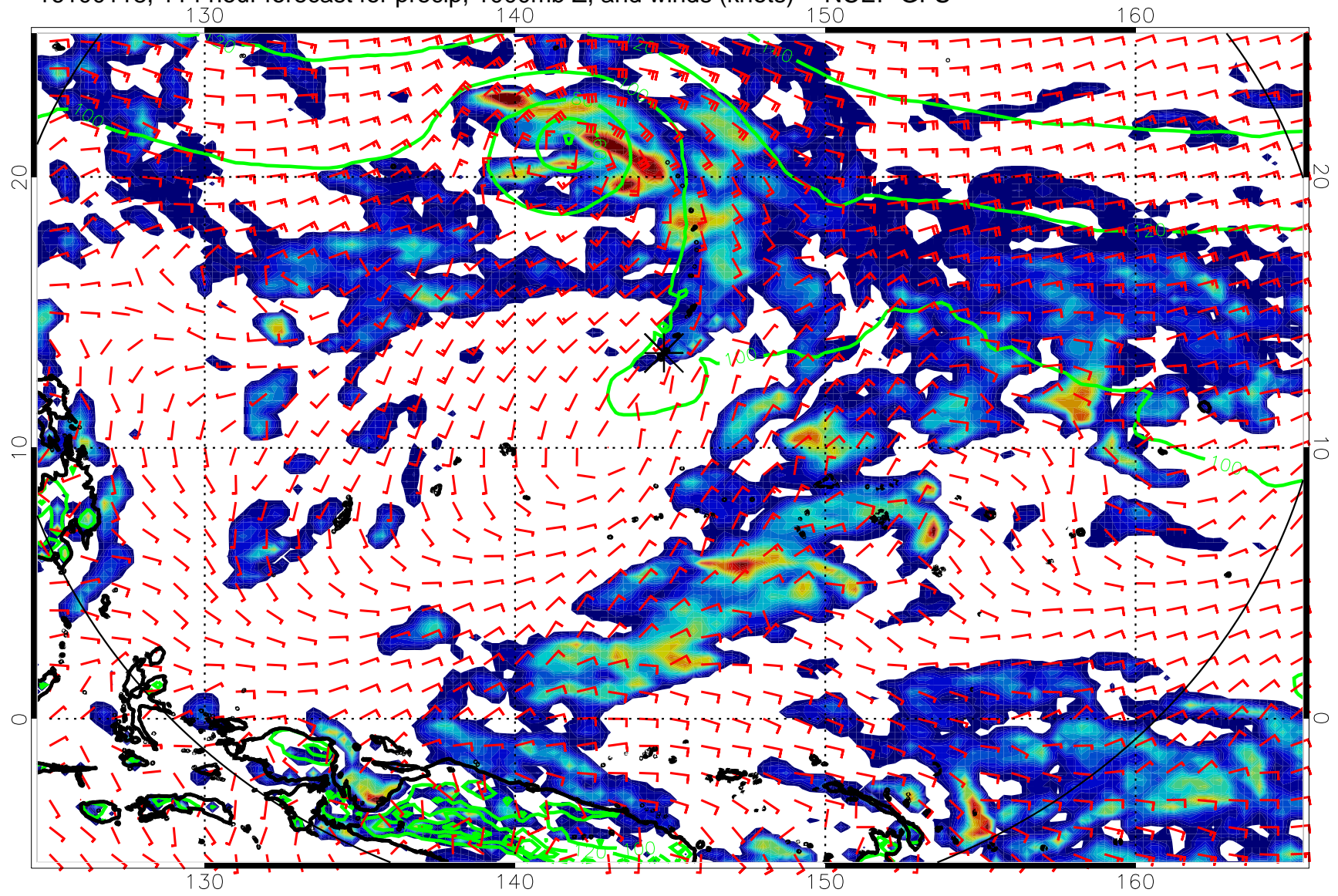
16100118, 114 hour forecast for precip, 1000mb Z, and winds (knots) -- NCEP GFS
