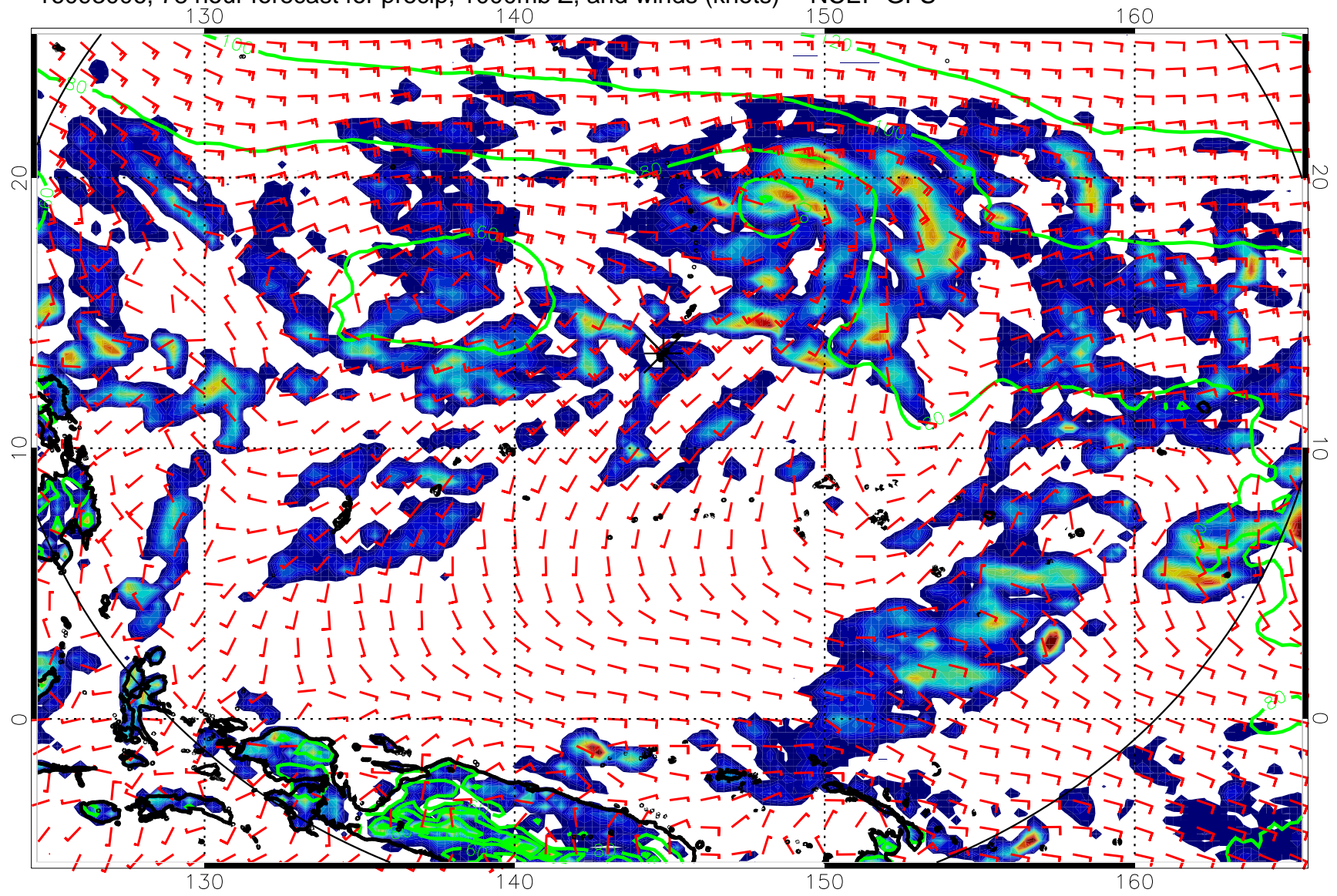
16093006, 78 hour forecast for precip, 1000mb Z, and winds (knots) -- NCEP GFS
