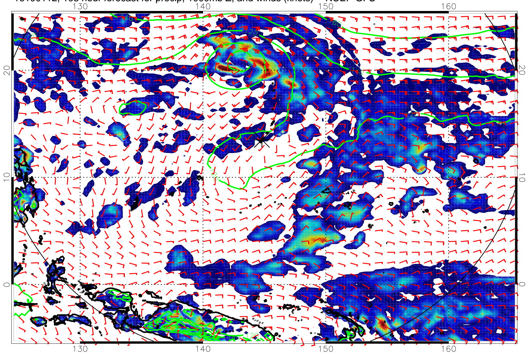
16100112, 108 hour forecast for precip, 1000mb Z, and winds (knots) -- NCEP GFS
