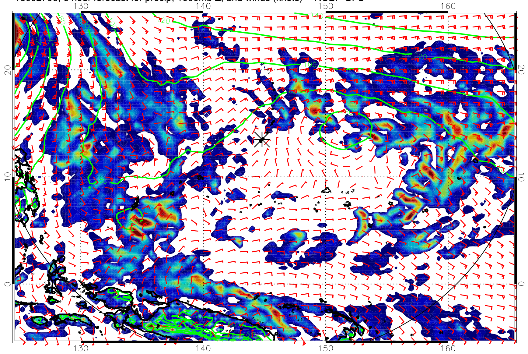
16092706, 6 hour forecast for precip, 1000mb Z, and winds (knots) -- NCEP GFS
