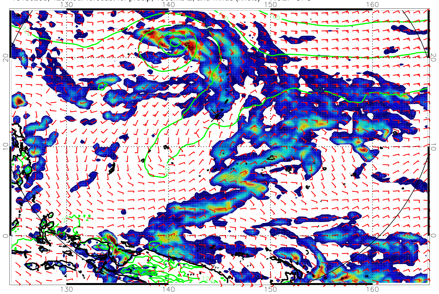
16100200, 120 hour forecast for precip, 1000mb Z, and winds (knots) -- NCEP GFS
