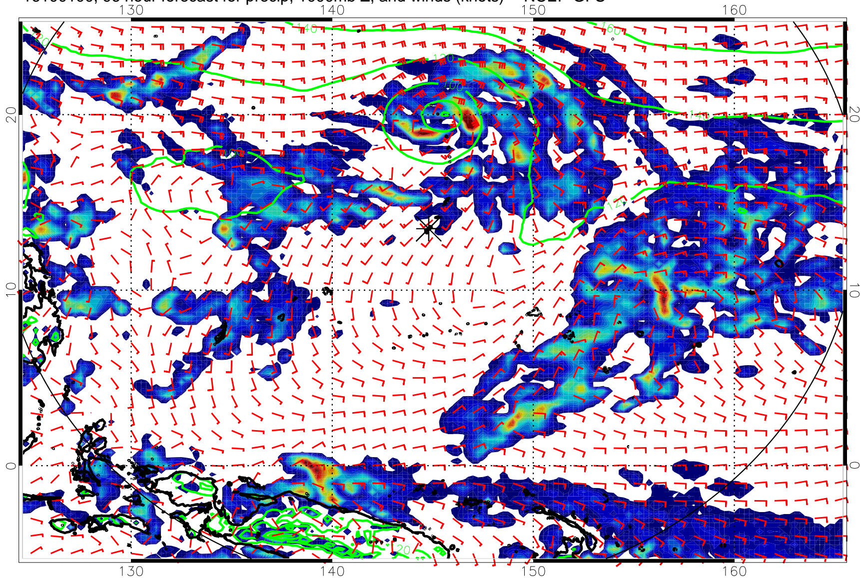
16100100, 96 hour forecast for precip, 1000mb Z, and winds (knots) -- NCEP GFS
