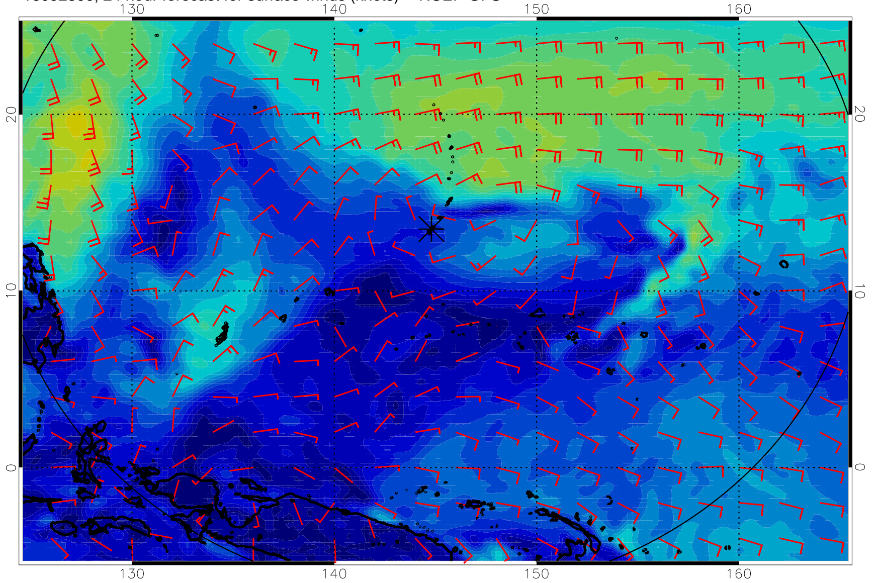
16092800, 24 hour forecast for surface winds (knots) -- NCEP GFS
