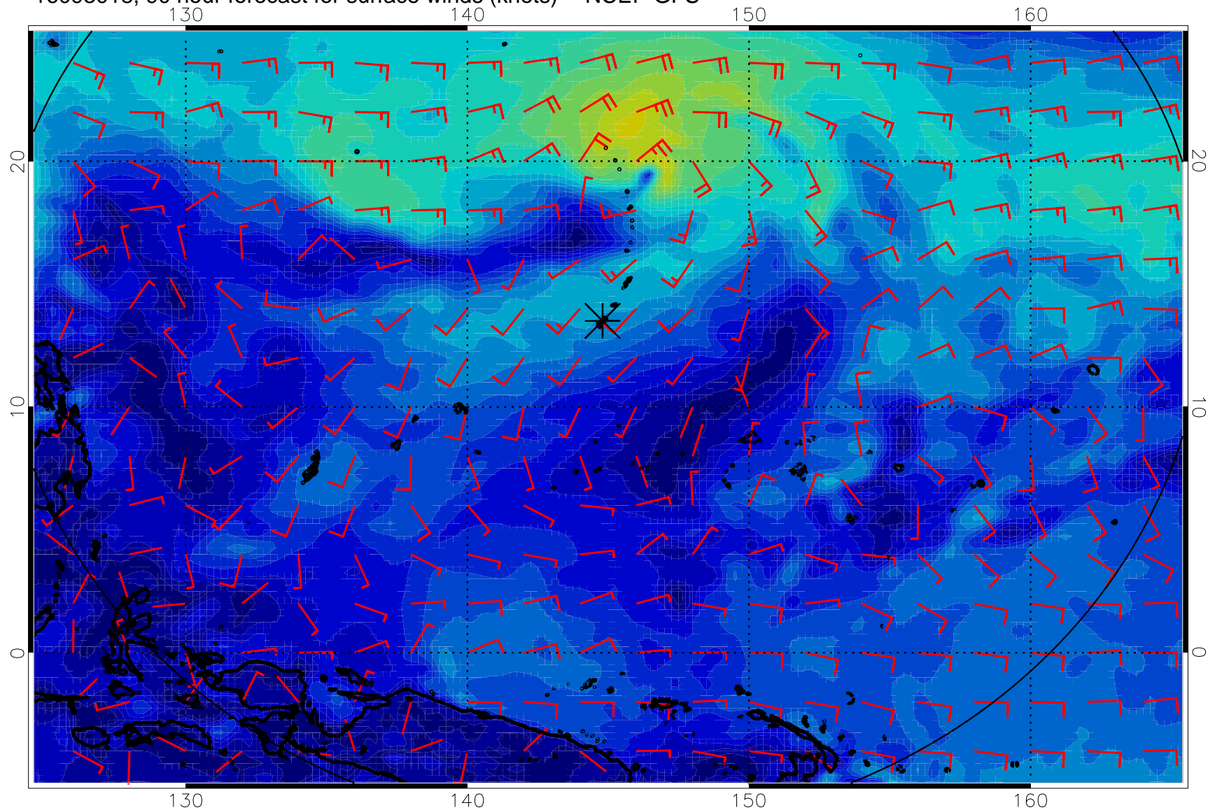
16093018, 90 hour forecast for surface winds (knots) -- NCEP GFS
