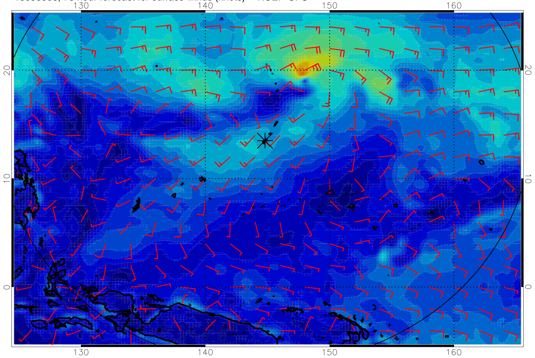
16093006, 78 hour forecast for surface winds (knots) -- NCEP GFS
