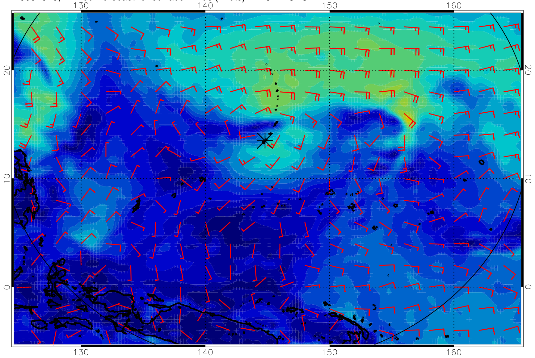
16092818, 42 hour forecast for surface winds (knots) -- NCEP GFS
