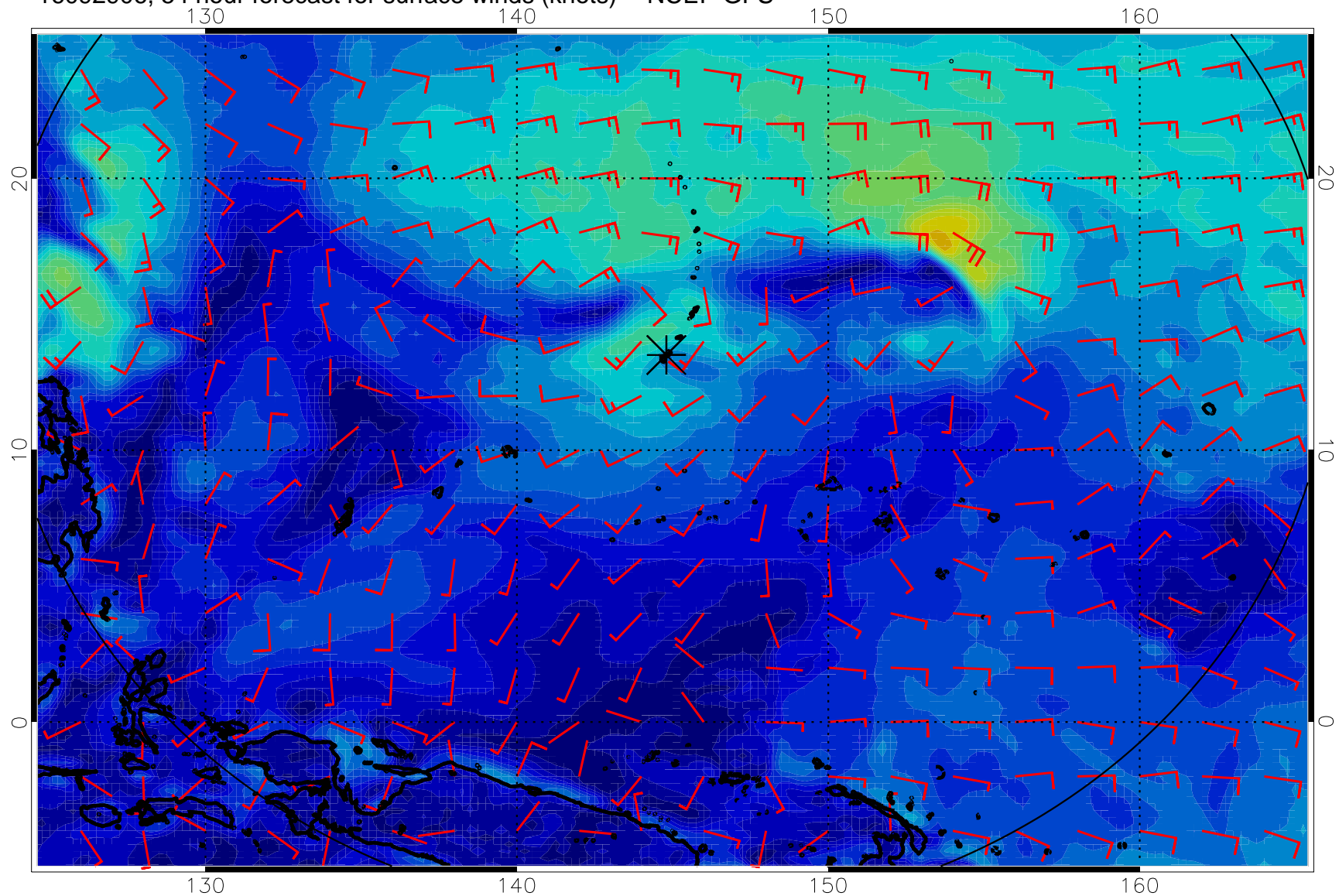
16092906, 54 hour forecast for surface winds (knots) -- NCEP GFS
