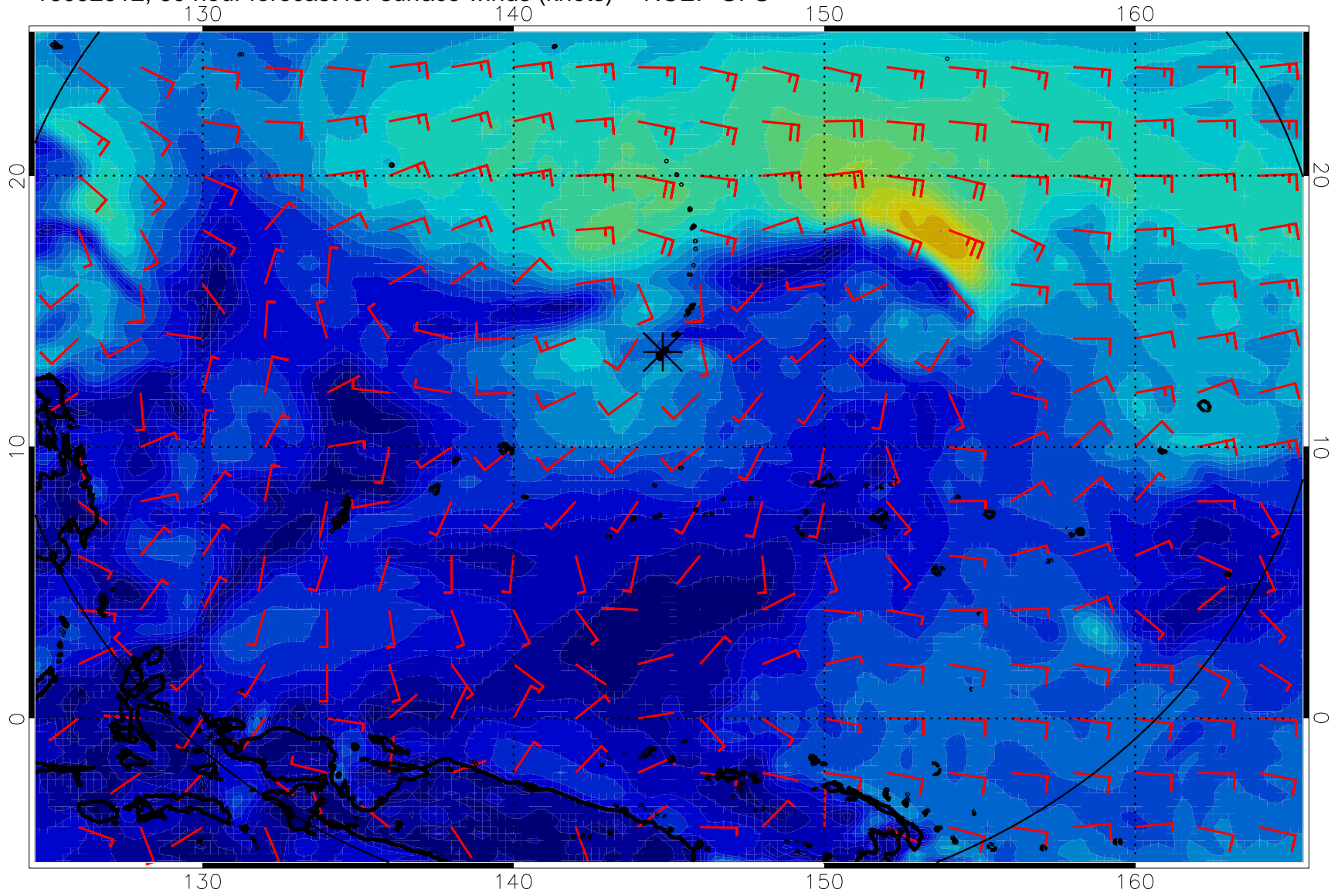
16092912, 60 hour forecast for surface winds (knots) -- NCEP GFS
