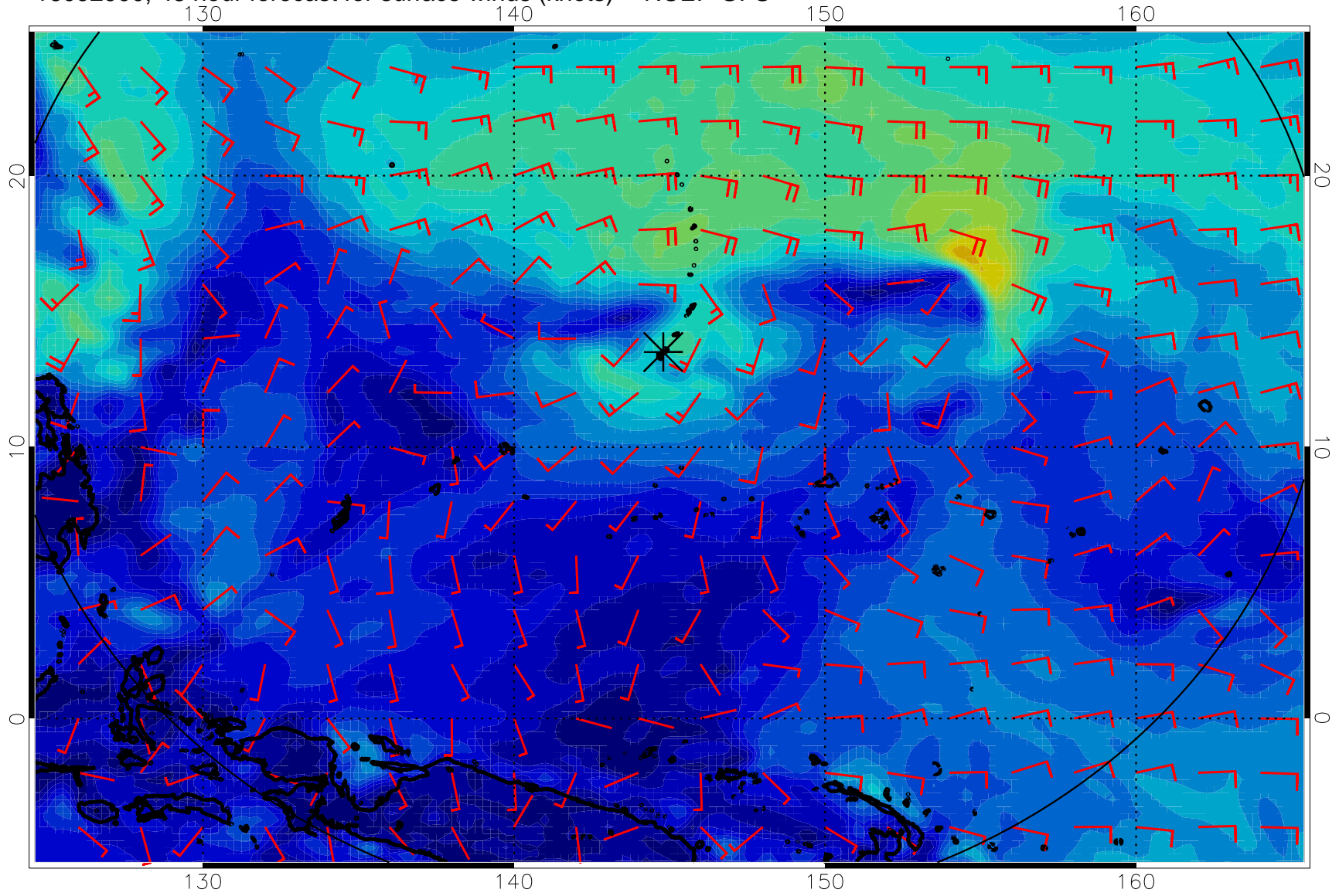
16092900, 48 hour forecast for surface winds (knots) -- NCEP GFS
