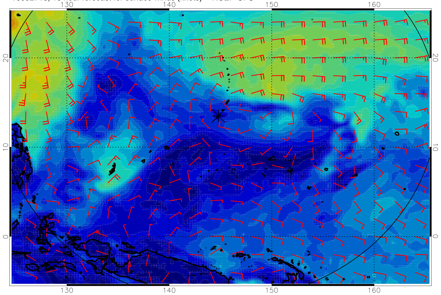
16092718, 18 hour forecast for surface winds (knots) -- NCEP GFS
