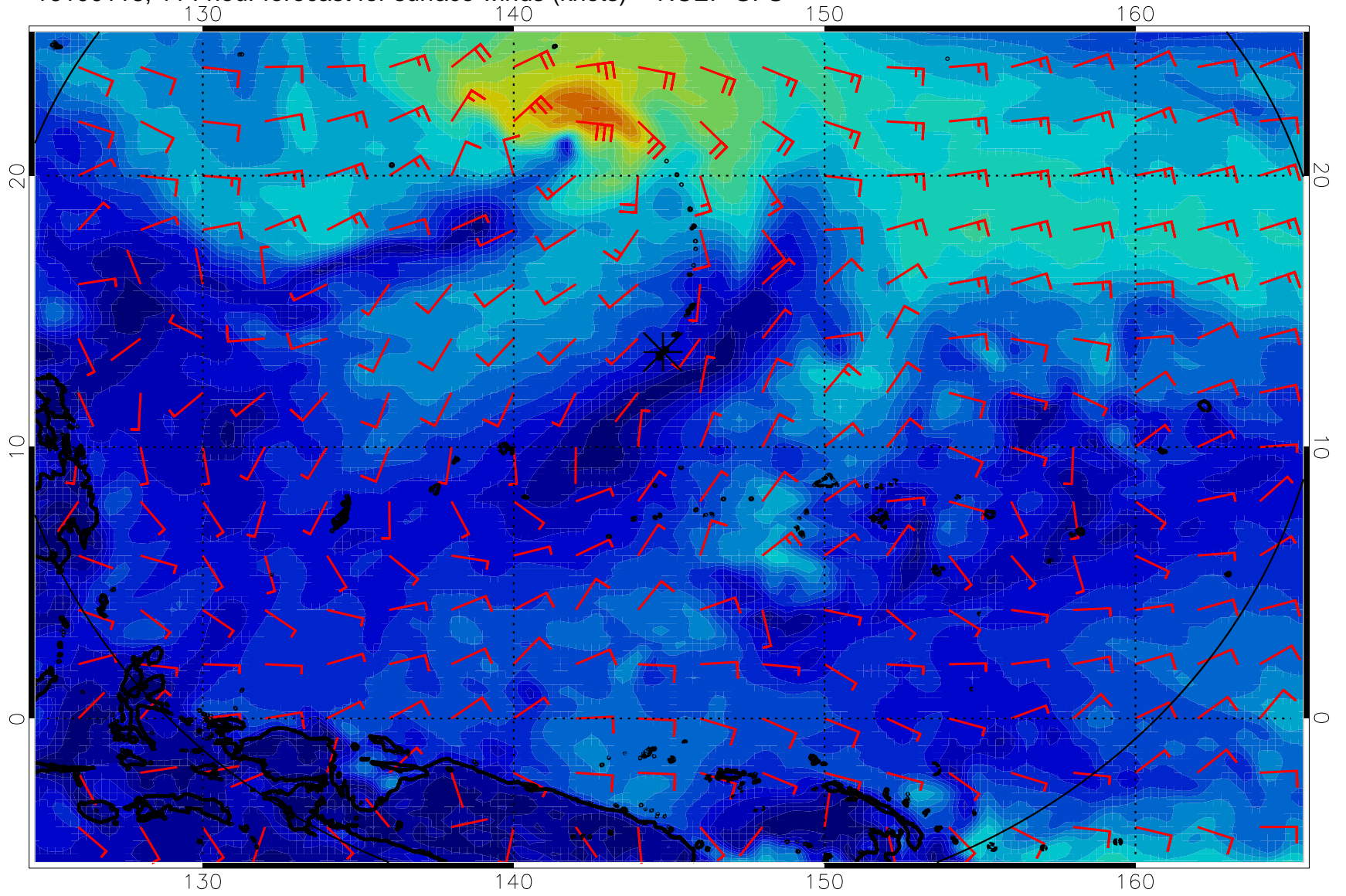
16100118, 114 hour forecast for surface winds (knots) -- NCEP GFS
