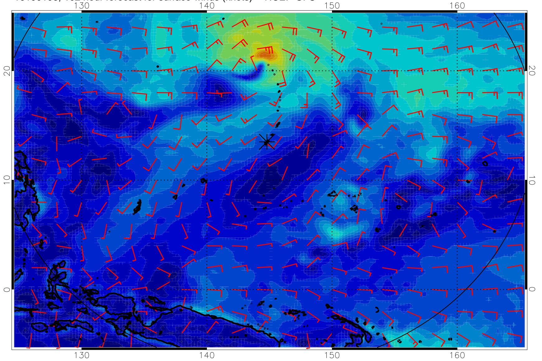
16100106, 102 hour forecast for surface winds (knots) -- NCEP GFS
