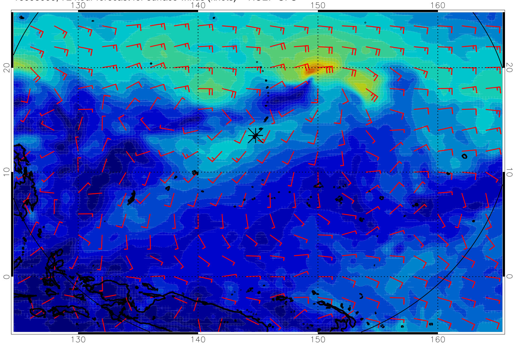
16093000, 72 hour forecast for surface winds (knots) -- NCEP GFS
