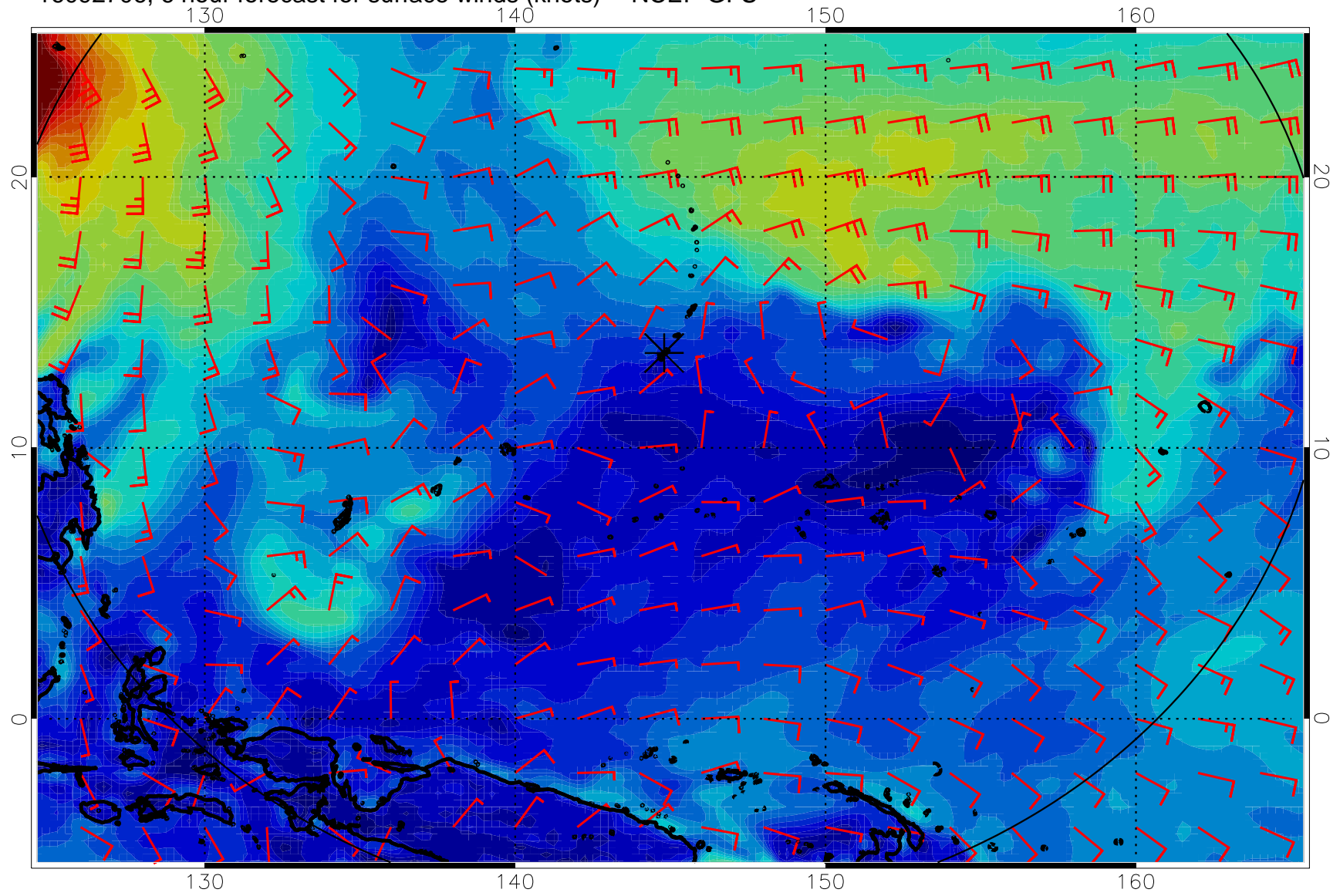
16092706, 6 hour forecast for surface winds (knots) -- NCEP GFS
