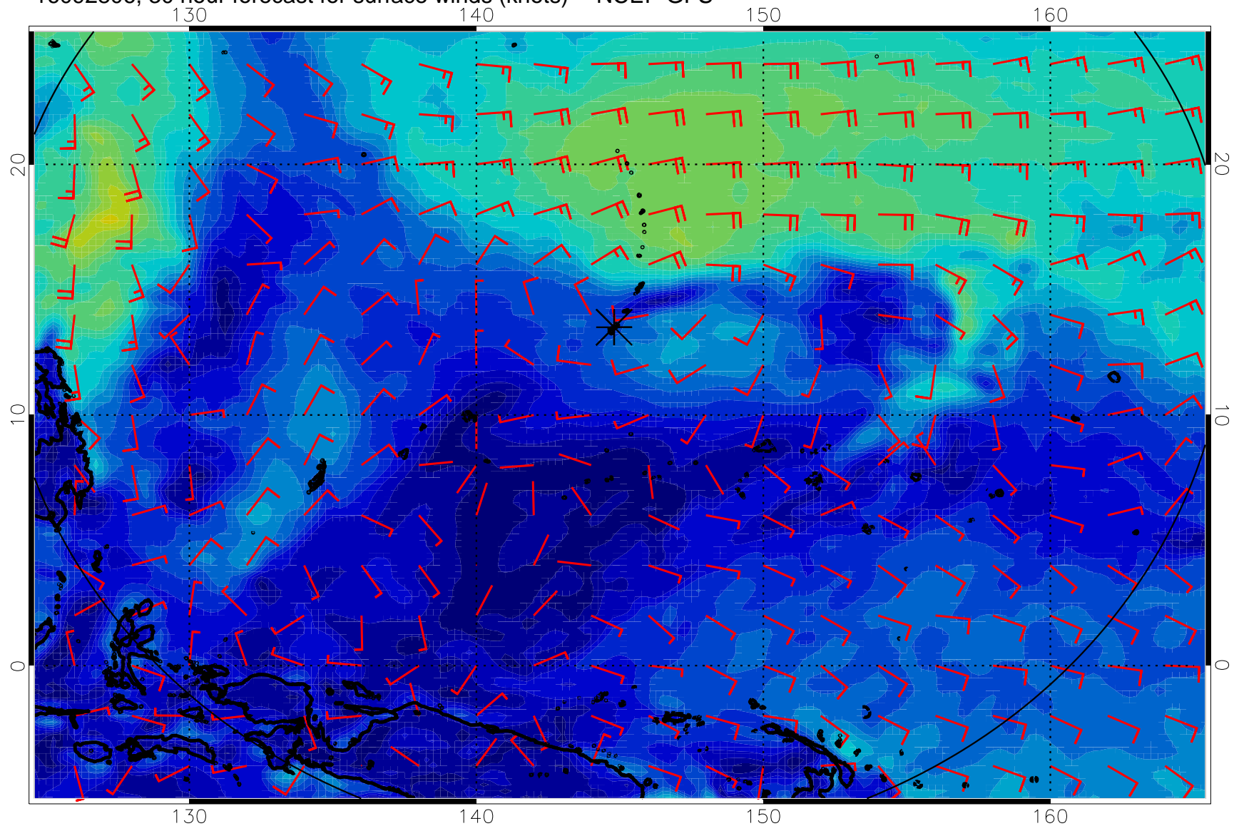
16092806, 30 hour forecast for surface winds (knots) -- NCEP GFS
