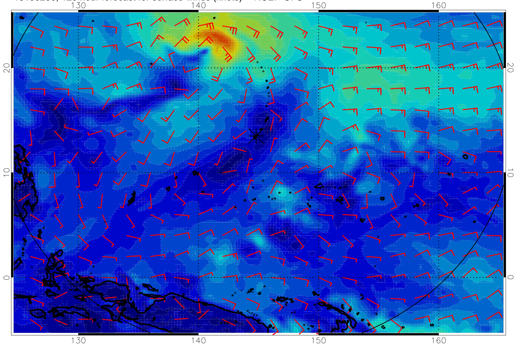
16100200, 120 hour forecast for surface winds (knots) -- NCEP GFS
