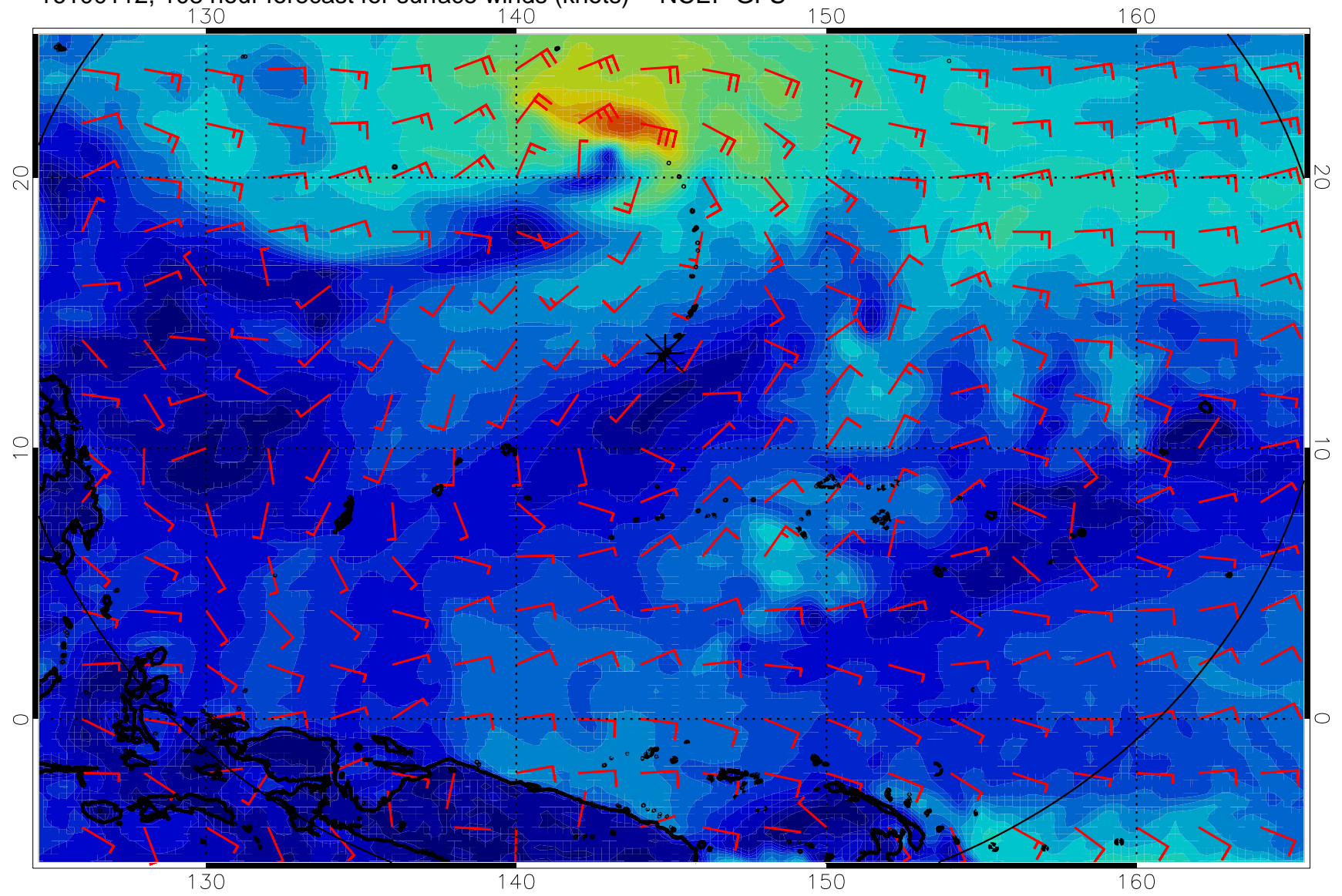
16100112, 108 hour forecast for surface winds (knots) -- NCEP GFS
