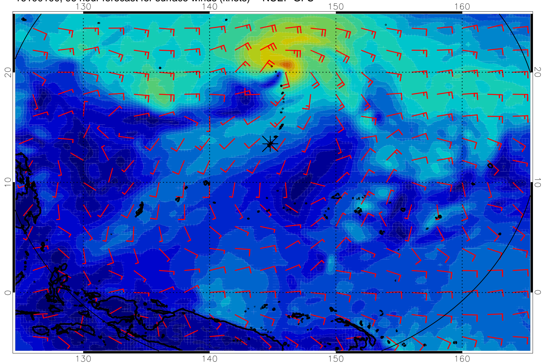
16100100, 96 hour forecast for surface winds (knots) -- NCEP GFS
