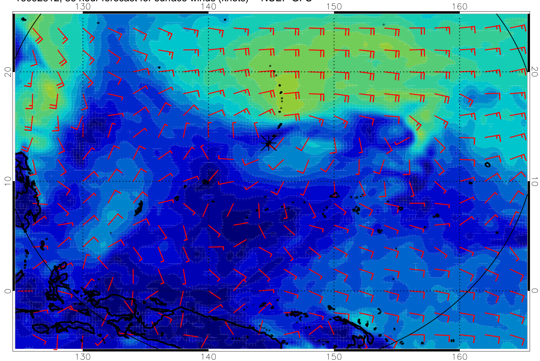
16092812, 36 hour forecast for surface winds (knots) -- NCEP GFS
