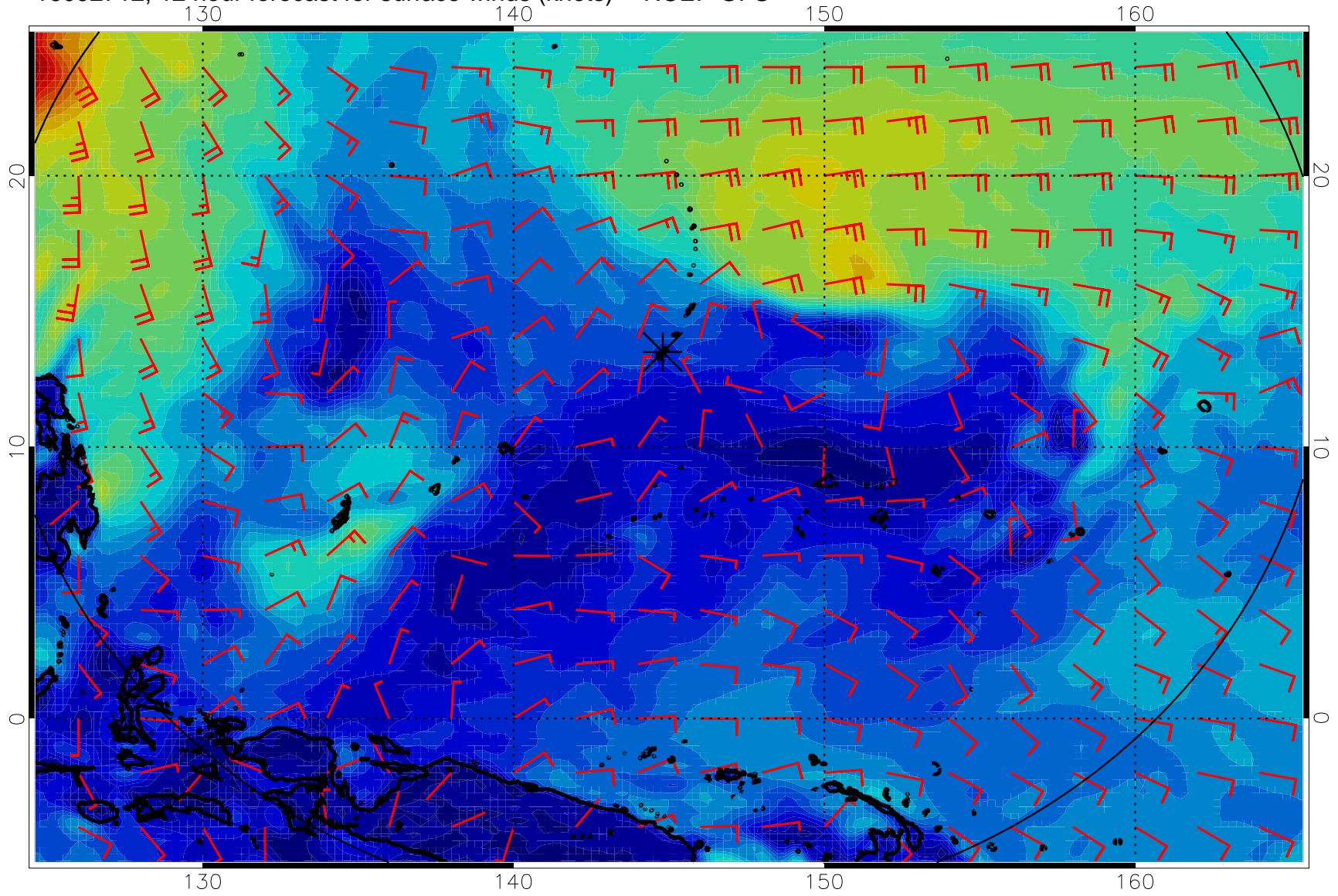
16092712, 12 hour forecast for surface winds (knots) -- NCEP GFS
