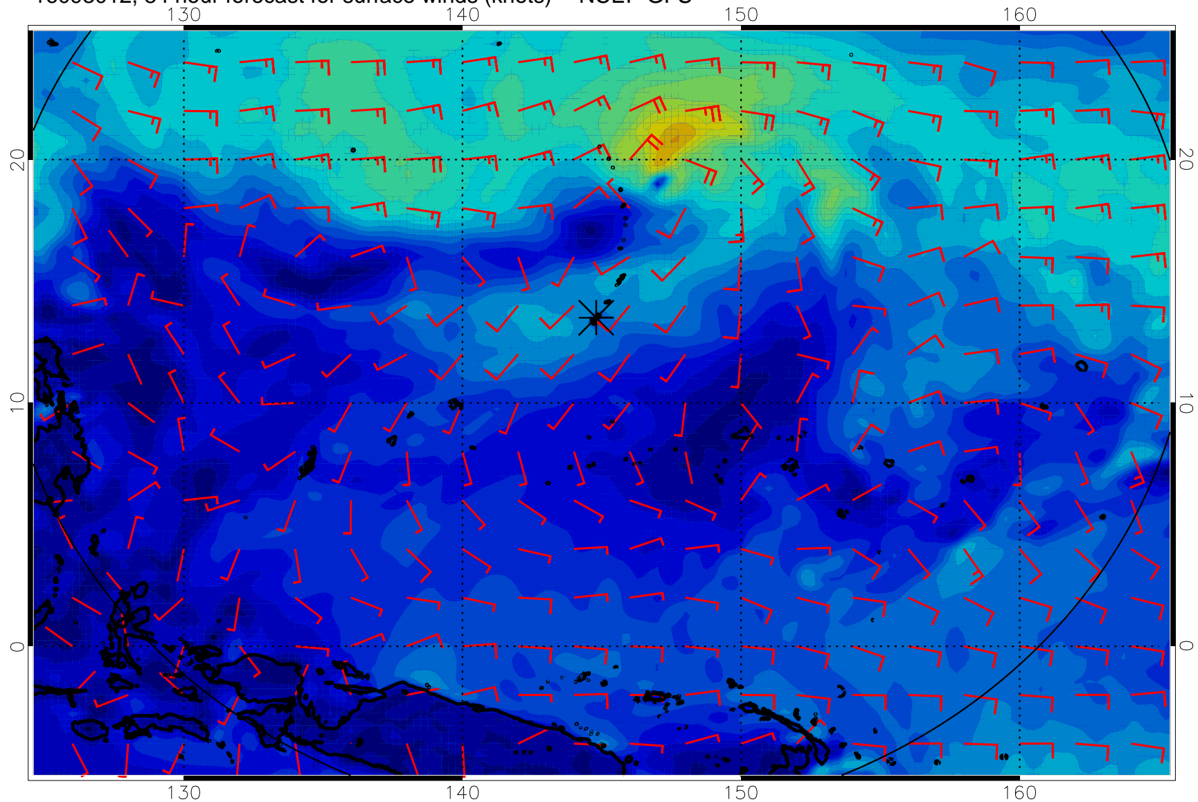
16093012, 84 hour forecast for surface winds (knots) -- NCEP GFS
