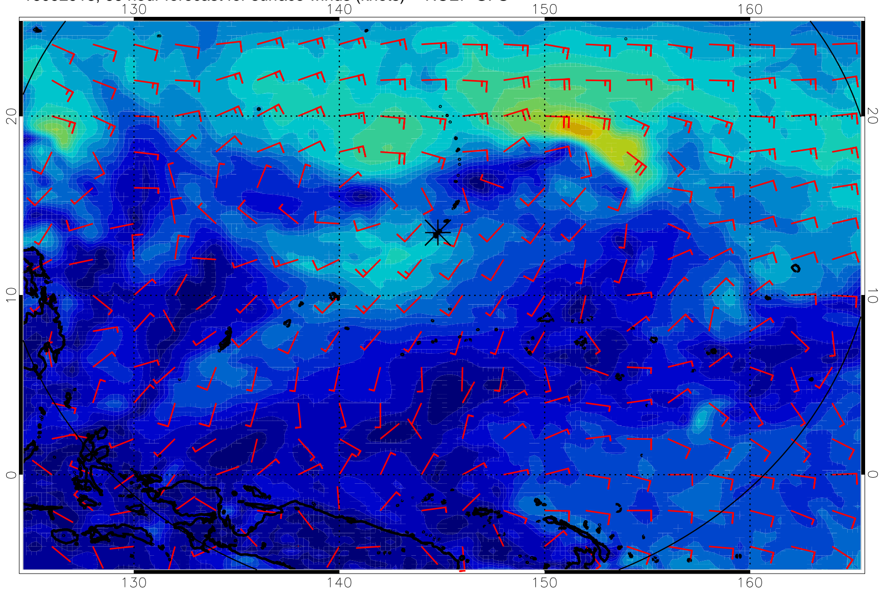
16092918, 66 hour forecast for surface winds (knots) -- NCEP GFS
