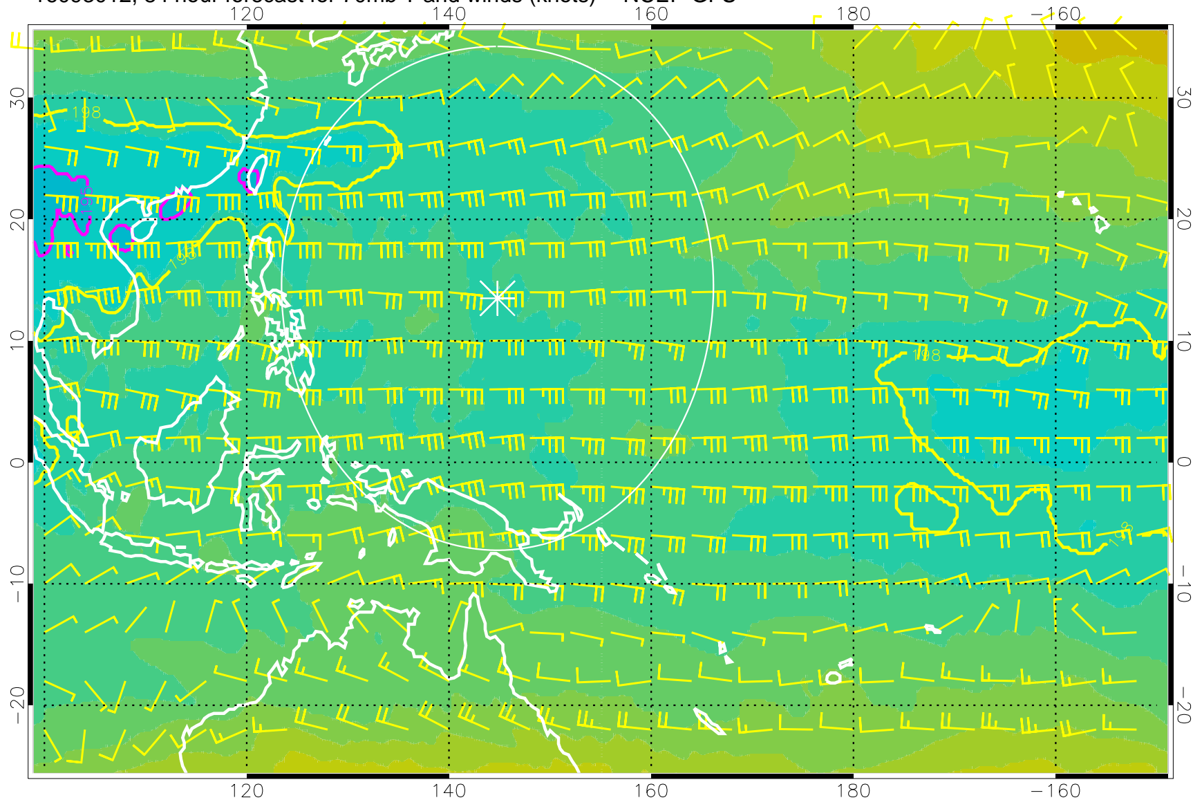
16093012, 84 hour forecast for 70mb T and winds (knots) -- NCEP GFS
