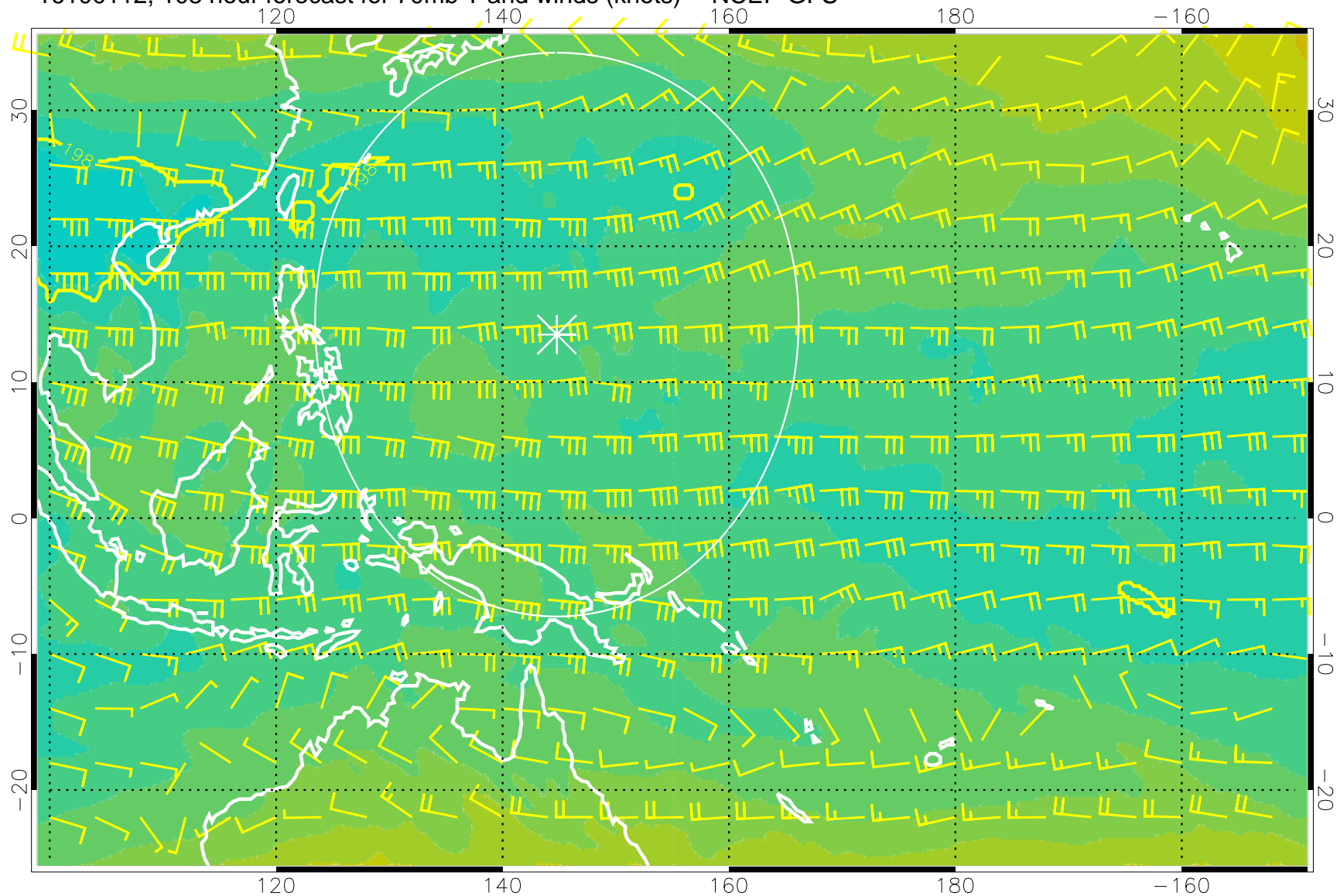
16100112, 108 hour forecast for 70mb T and winds (knots) -- NCEP GFS
