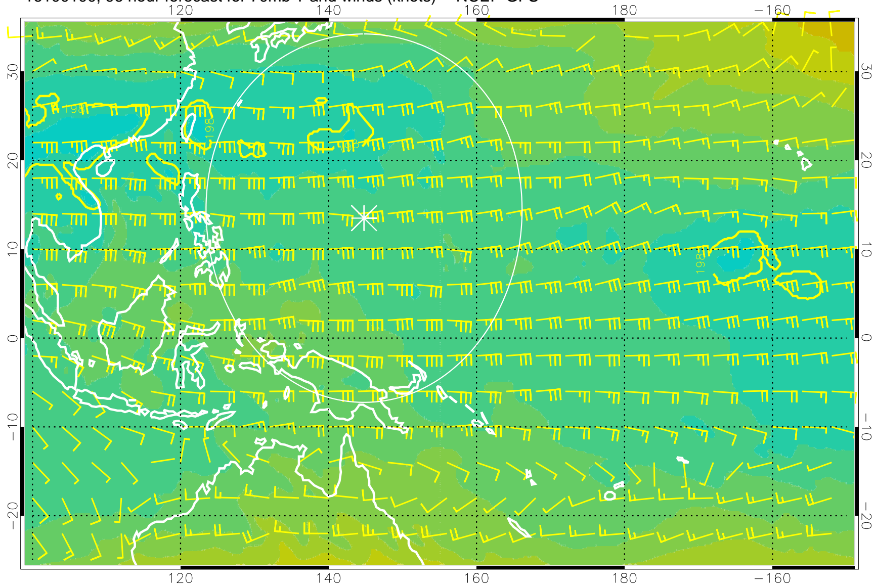
16100100, 96 hour forecast for 70mb T and winds (knots) -- NCEP GFS
