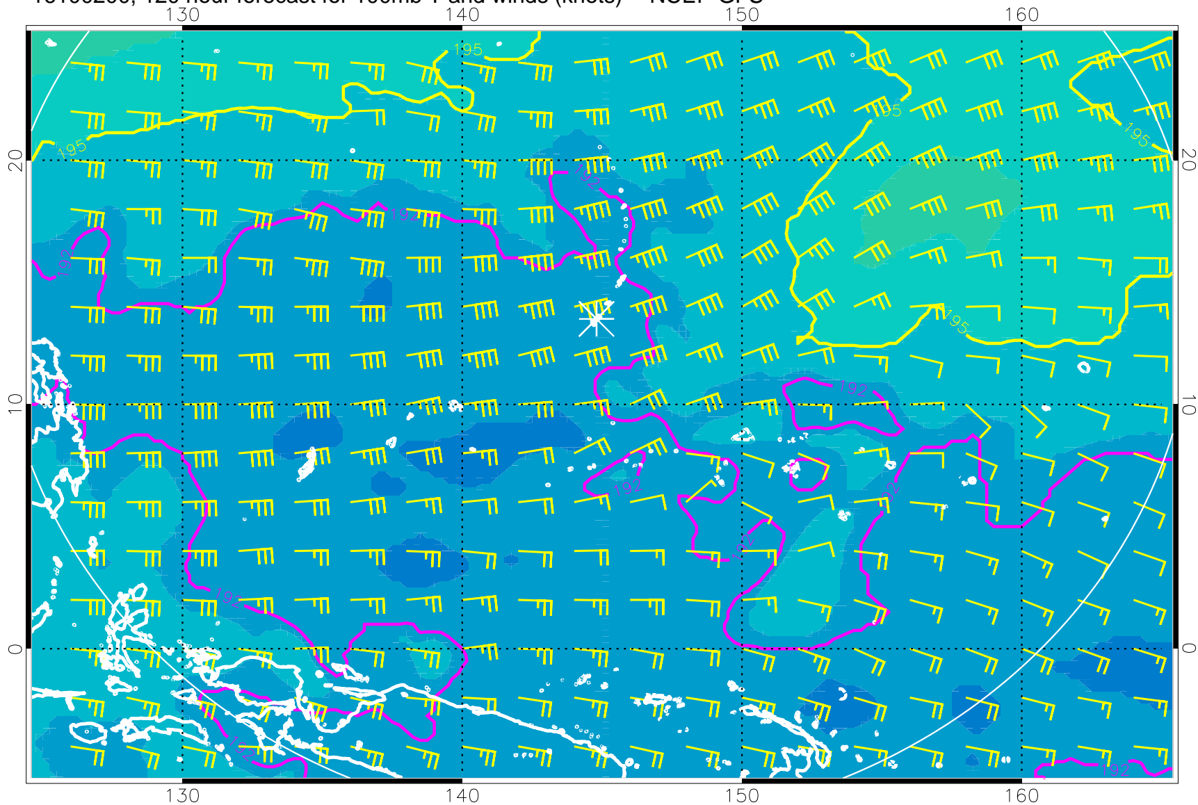
16100200, 120 hour forecast for 100mb T and winds (knots) -- NCEP GFS
