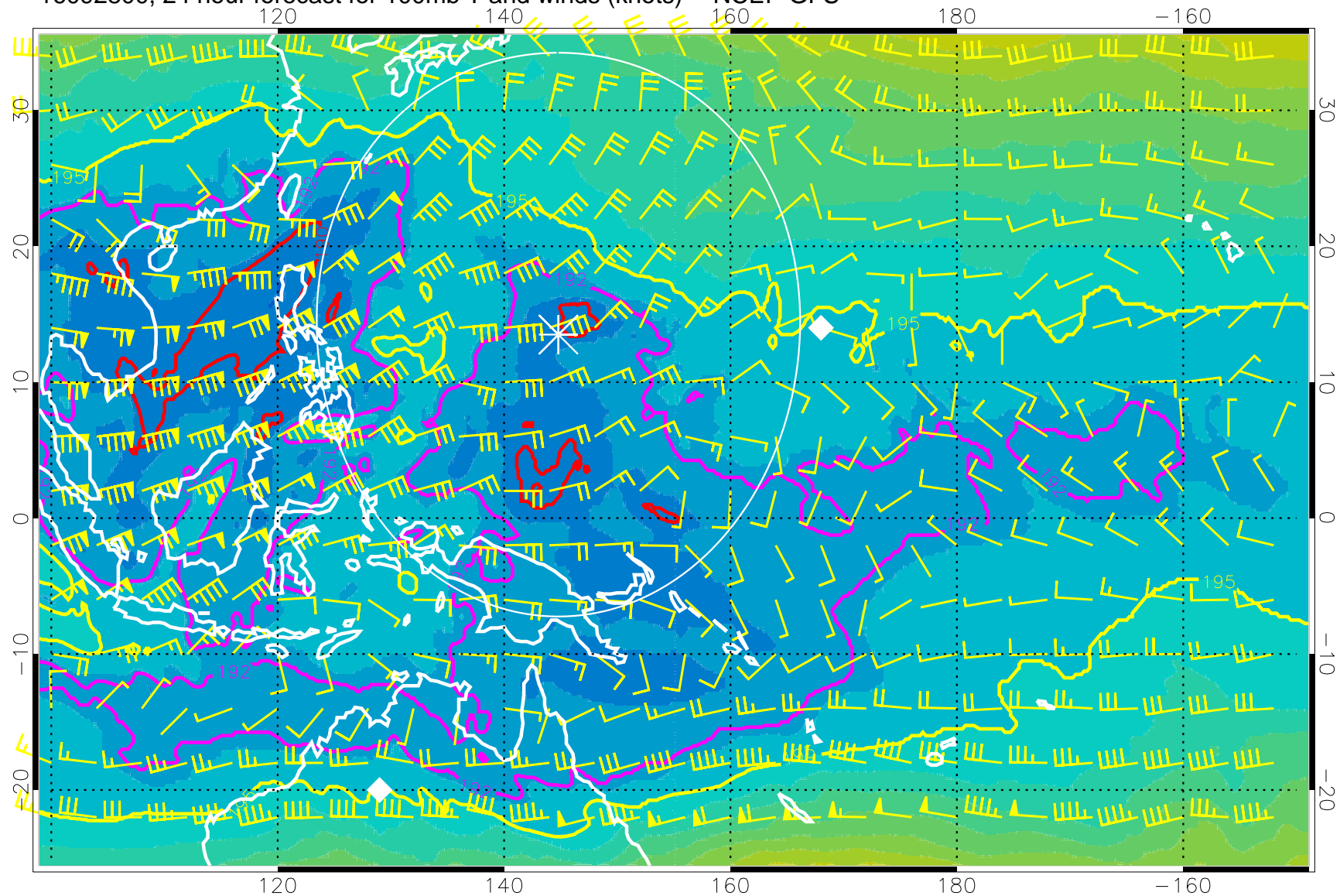
16092800, 24 hour forecast for 100mb T and winds (knots) -- NCEP GFS
