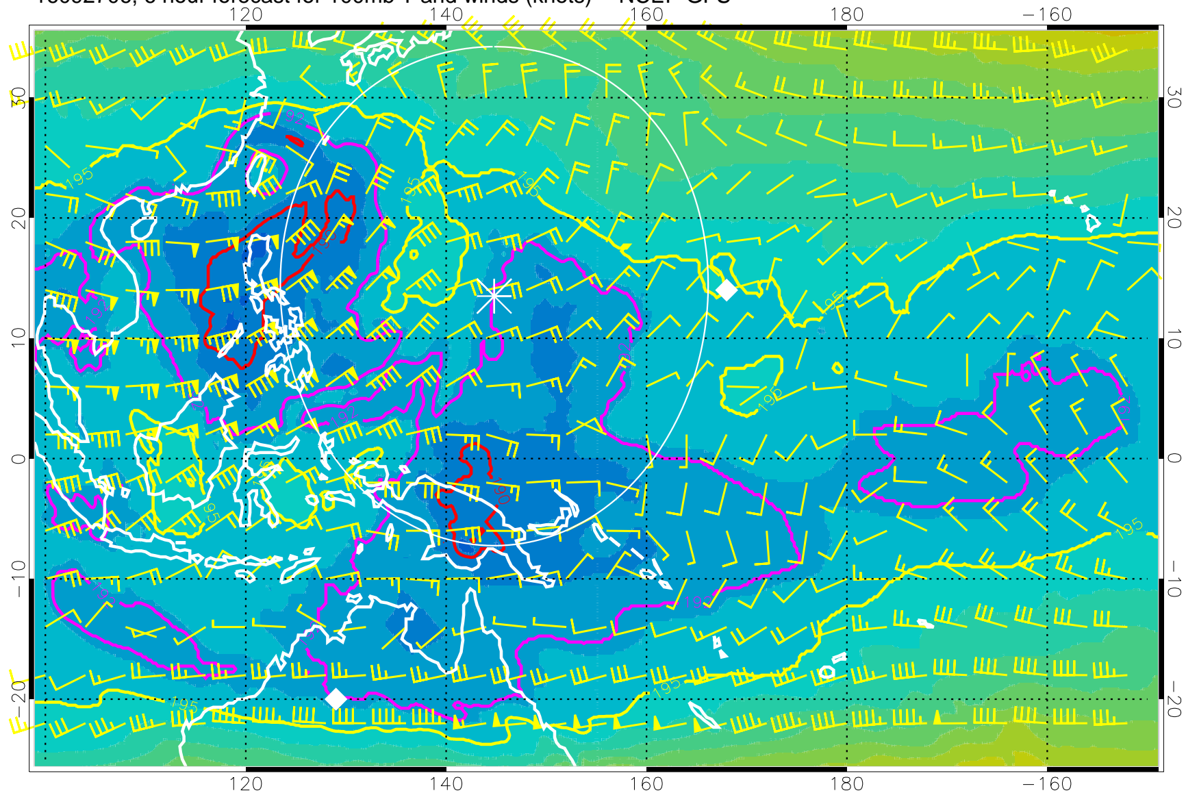
16092706, 6 hour forecast for 100mb T and winds (knots) -- NCEP GFS
