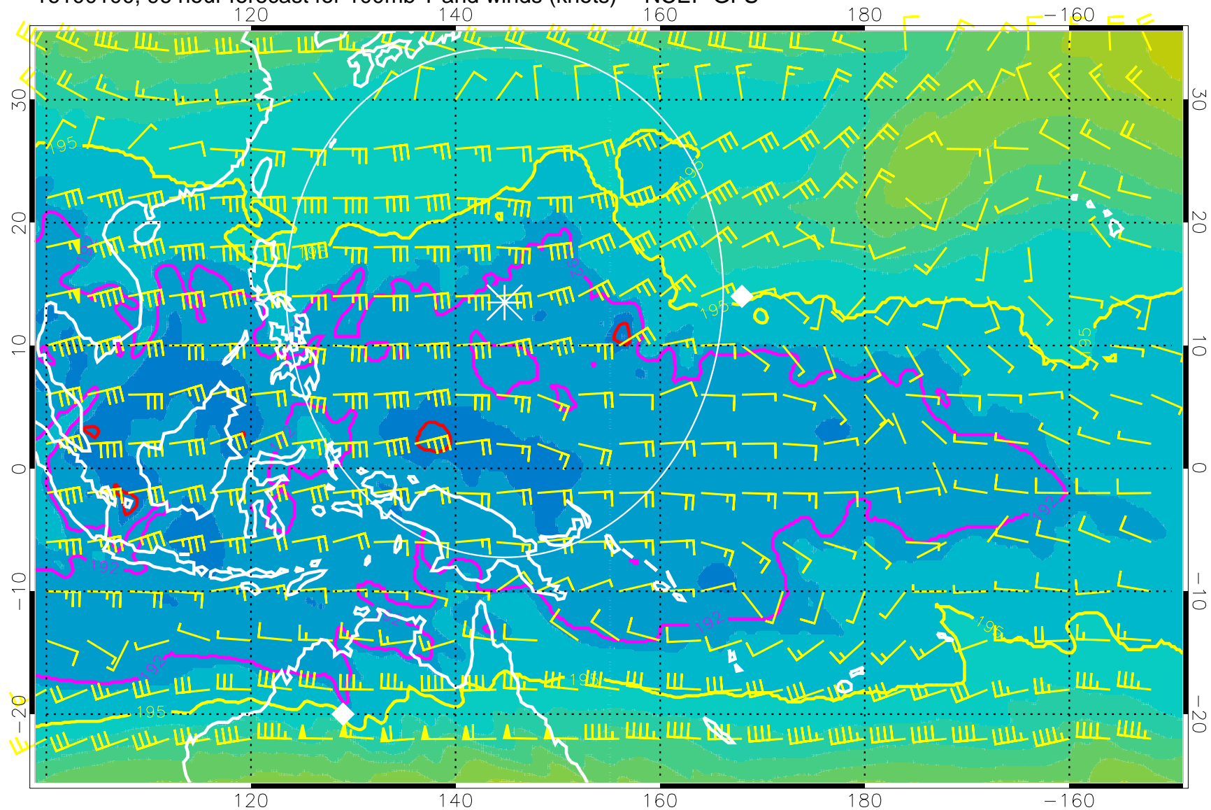
16100100, 96 hour forecast for 100mb T and winds (knots) -- NCEP GFS
