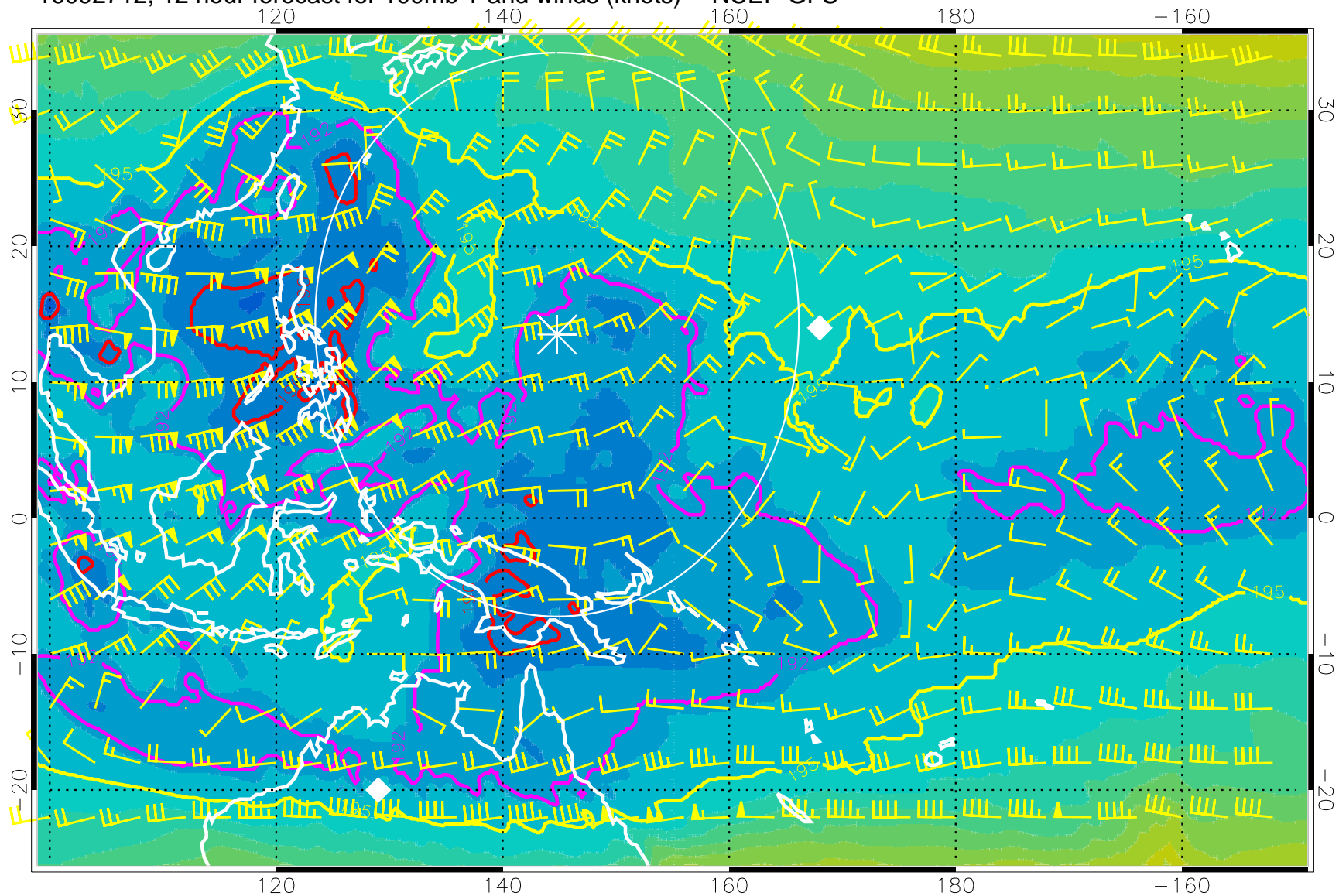
16092712, 12 hour forecast for 100mb T and winds (knots) -- NCEP GFS
