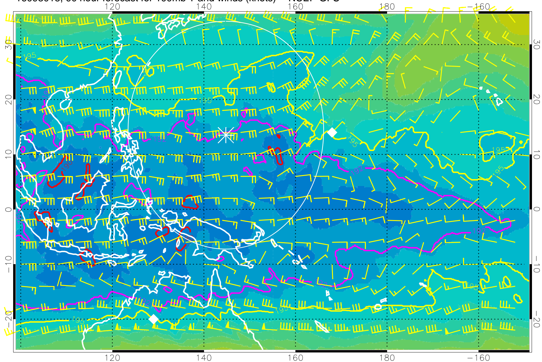
16093018, 90 hour forecast for 100mb T and winds (knots) -- NCEP GFS
