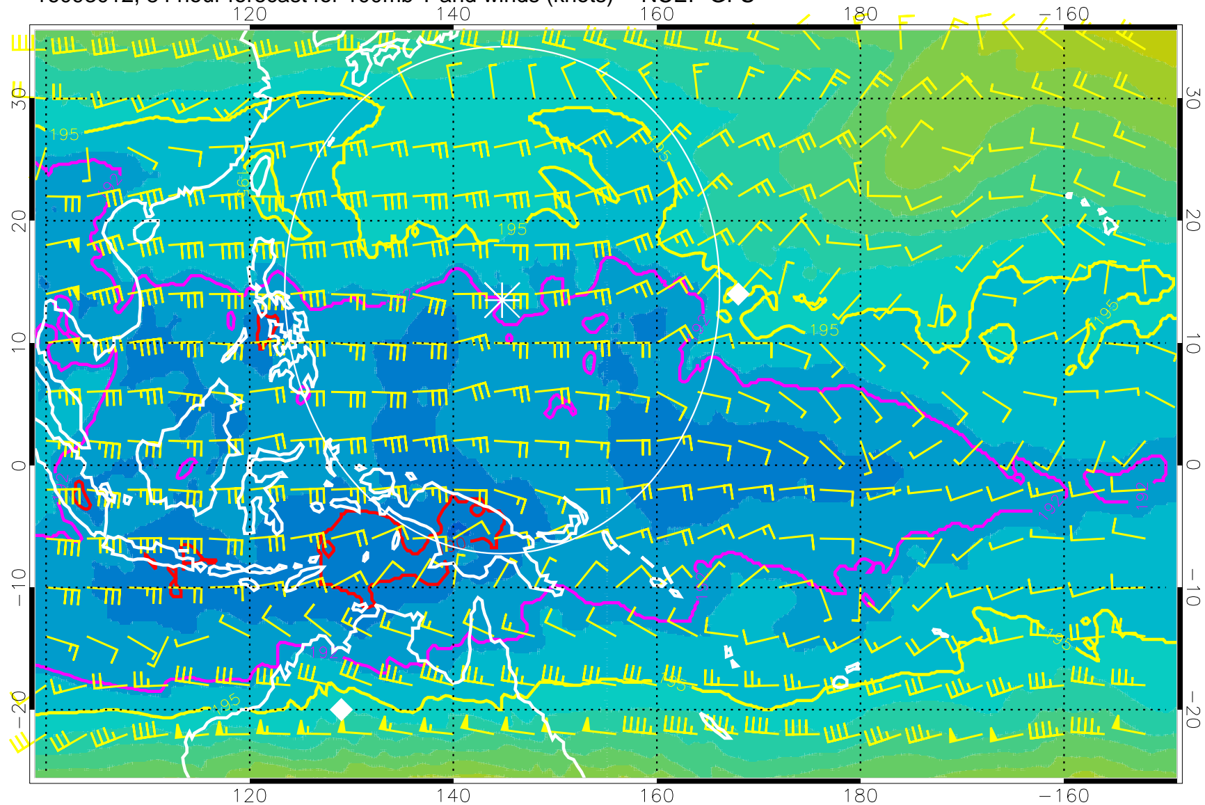
16093012, 84 hour forecast for 100mb T and winds (knots) -- NCEP GFS
