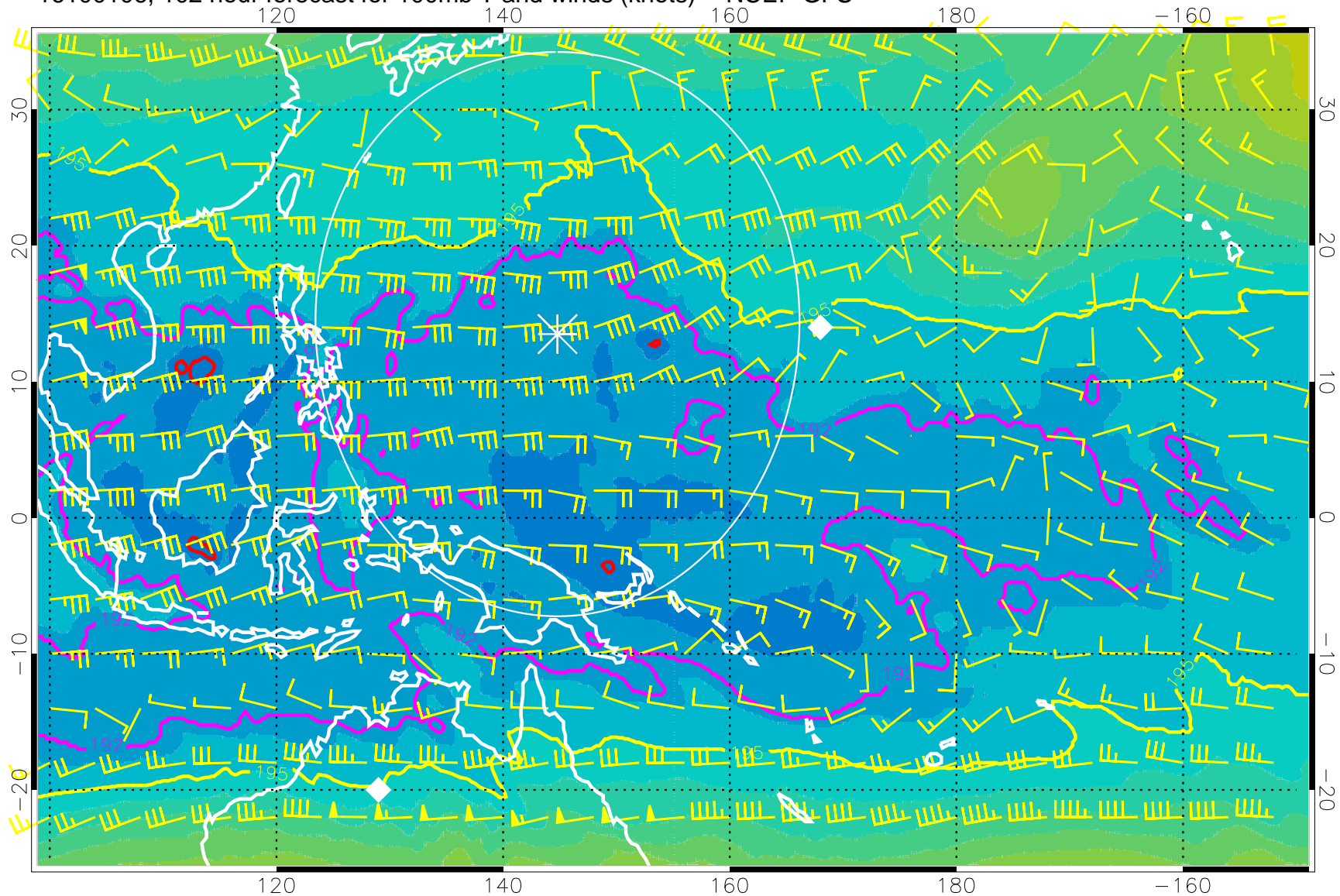
16100106, 102 hour forecast for 100mb T and winds (knots) -- NCEP GFS
