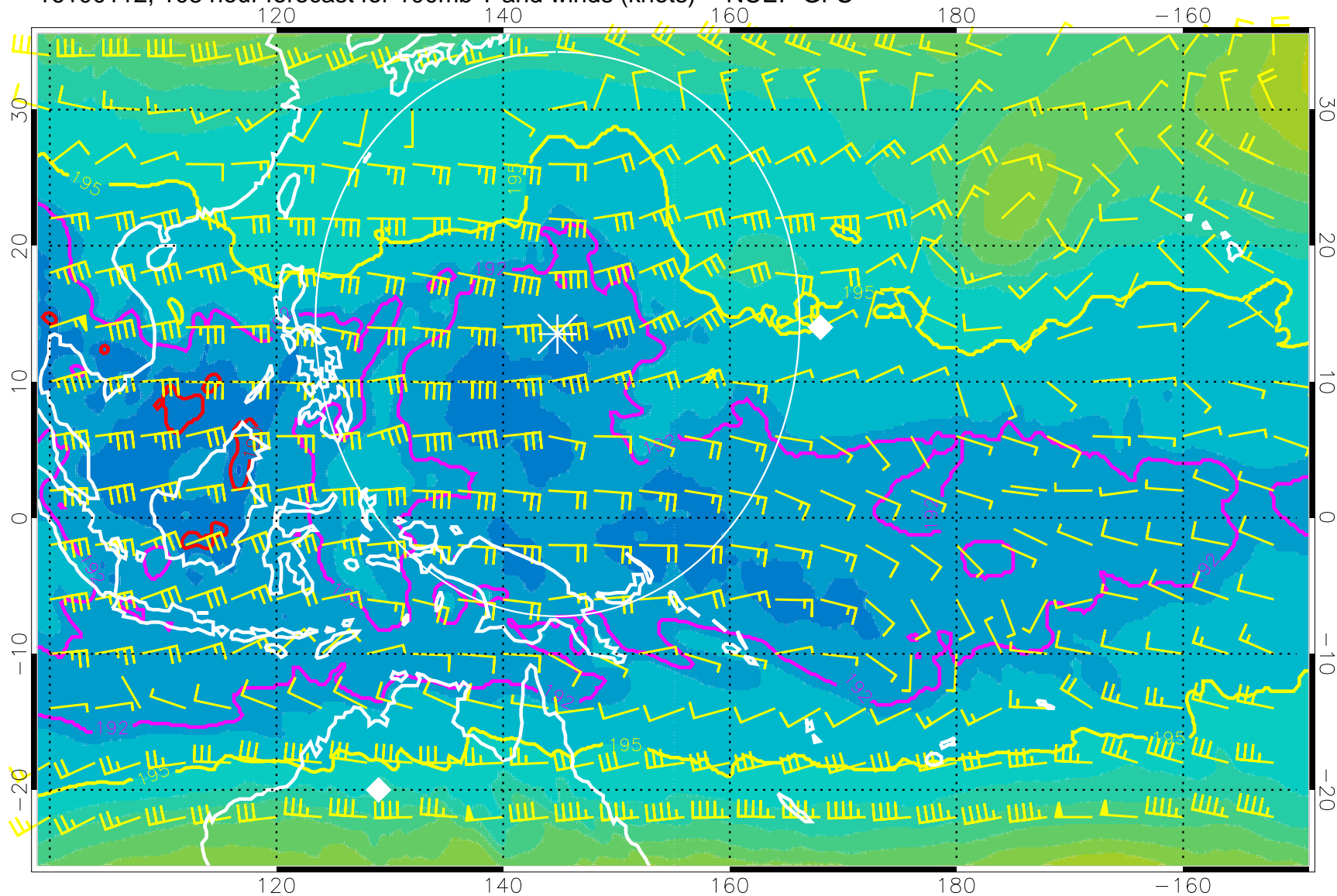
16100112, 108 hour forecast for 100mb T and winds (knots) -- NCEP GFS
