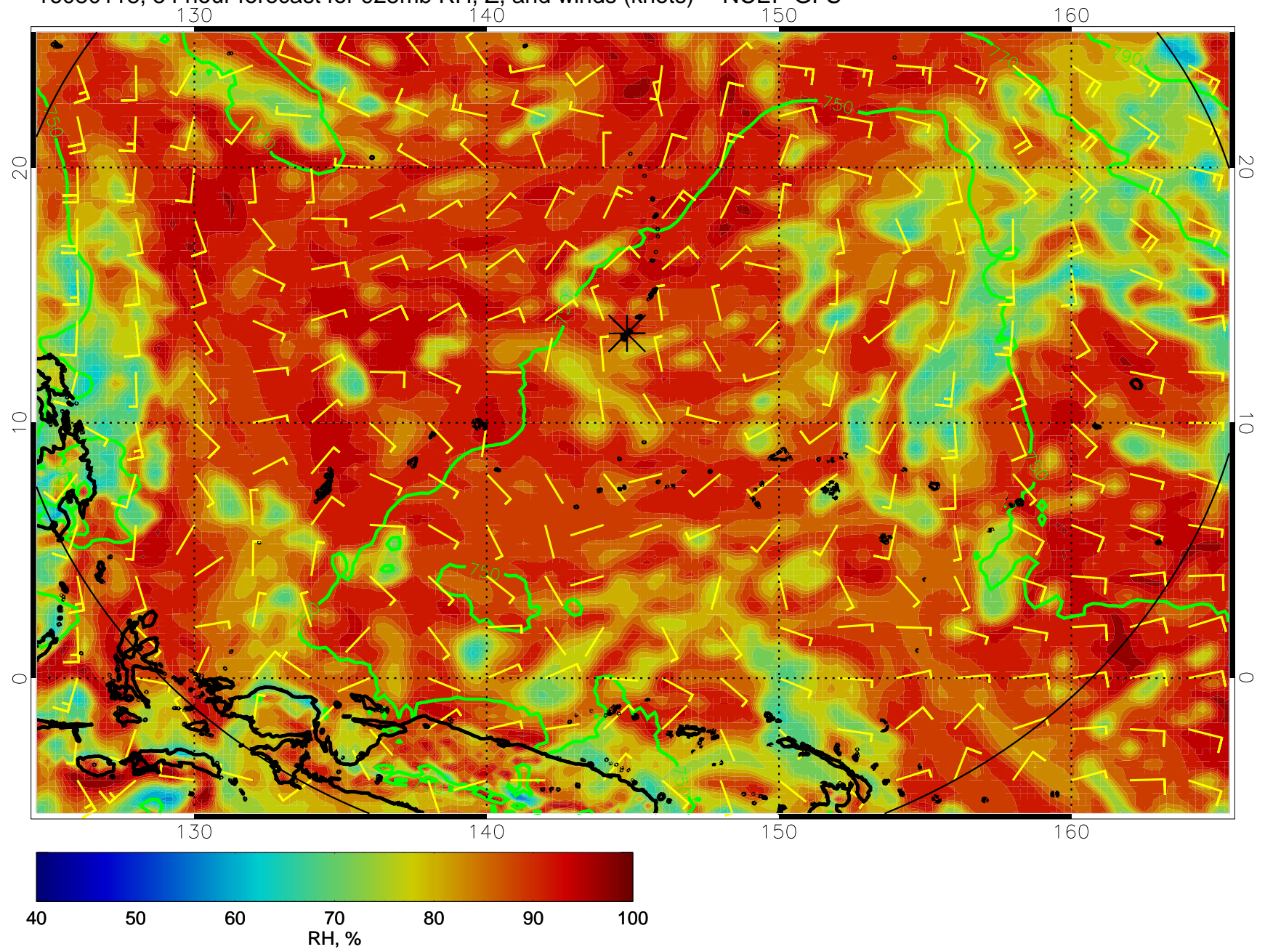
16080118, 54 hour forecast for 925mb RH, Z, and winds (knots) -- NCEP GFS
