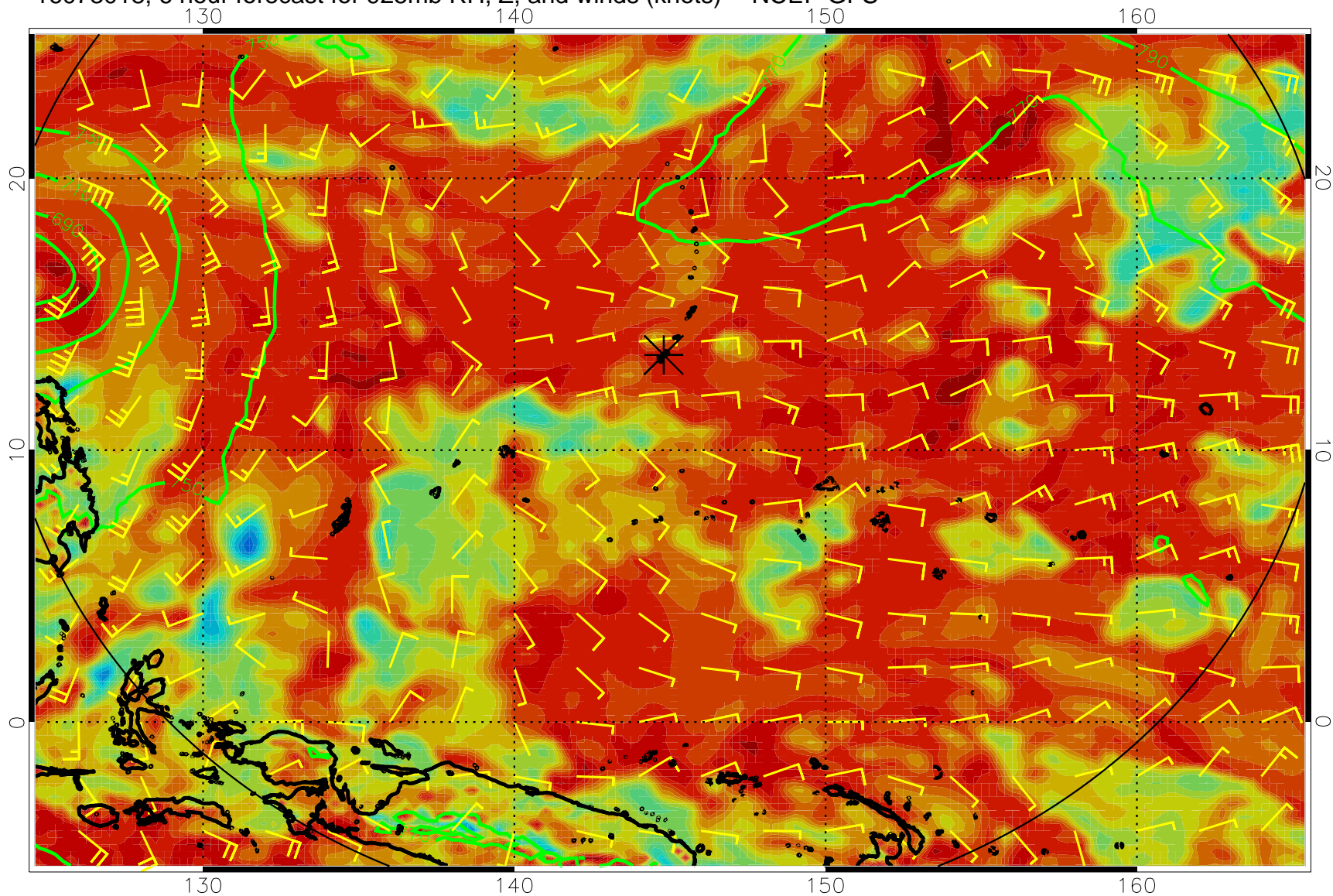
16073018, 6 hour forecast for 925mb RH, Z, and winds (knots) -- NCEP GFS
