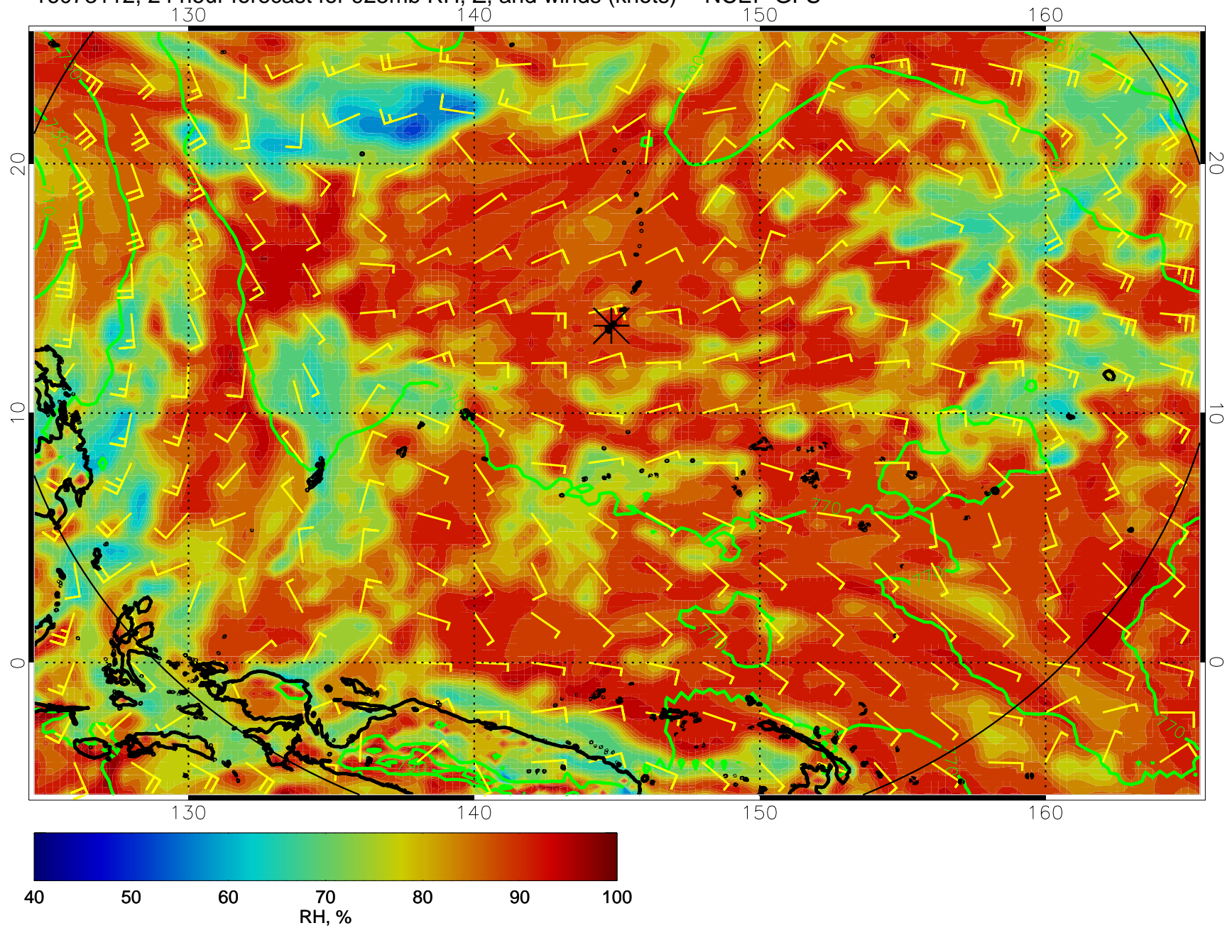
16073112, 24 hour forecast for 925mb RH, Z, and winds (knots) -- NCEP GFS
