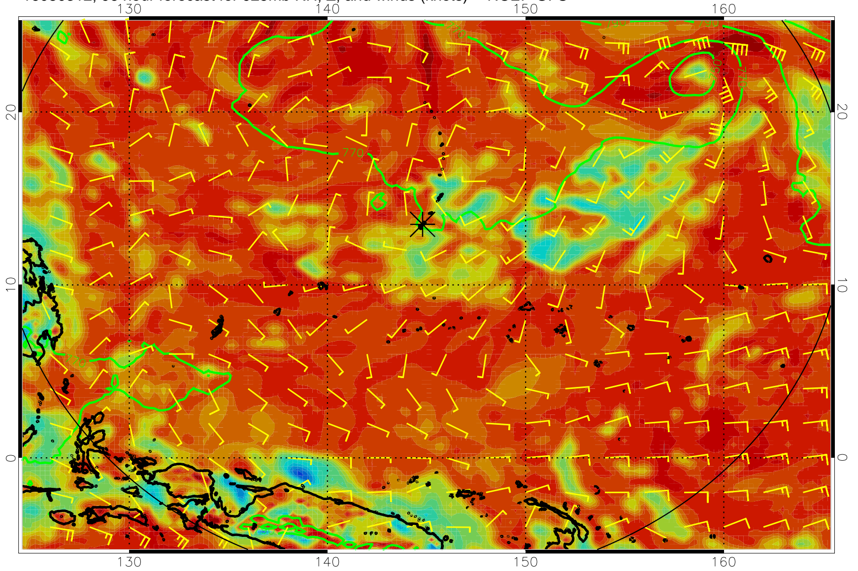
16080312, 96 hour forecast for 925mb RH, Z, and winds (knots) -- NCEP GFS
