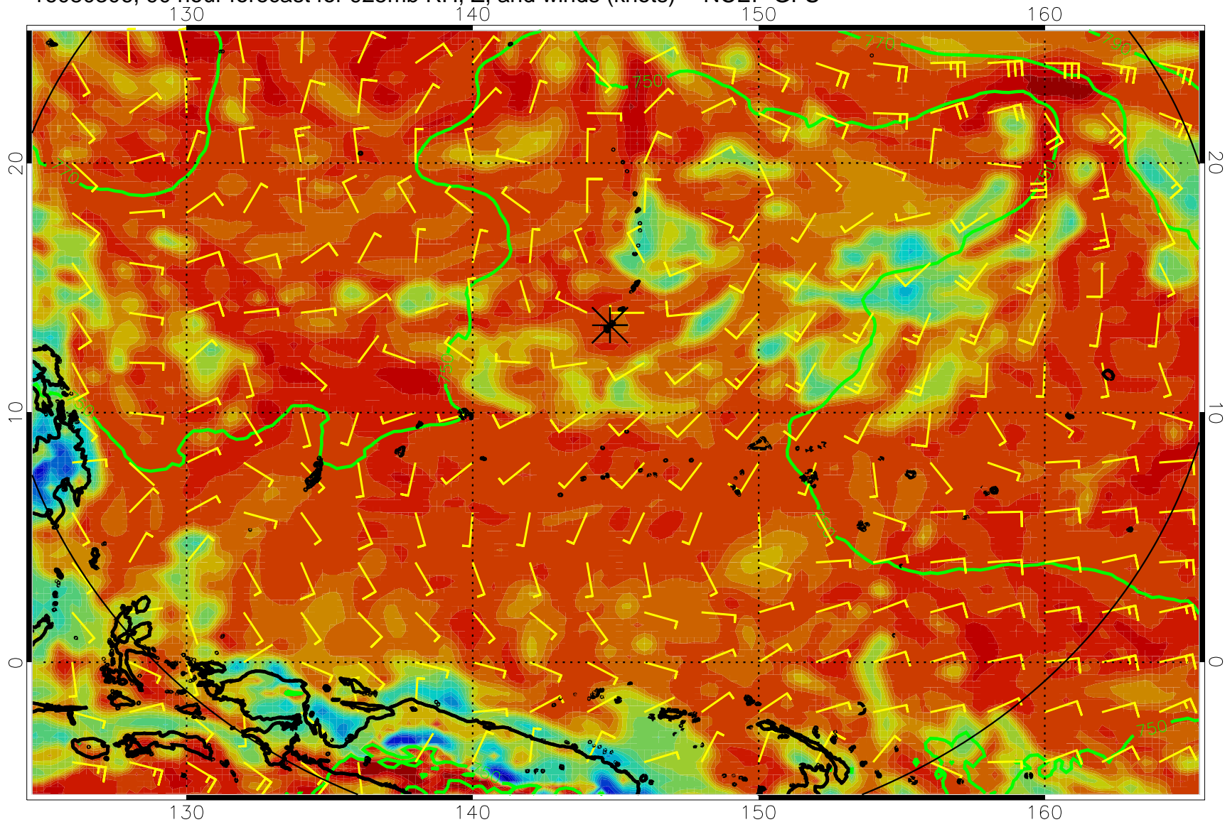
16080306, 90 hour forecast for 925mb RH, Z, and winds (knots) -- NCEP GFS
