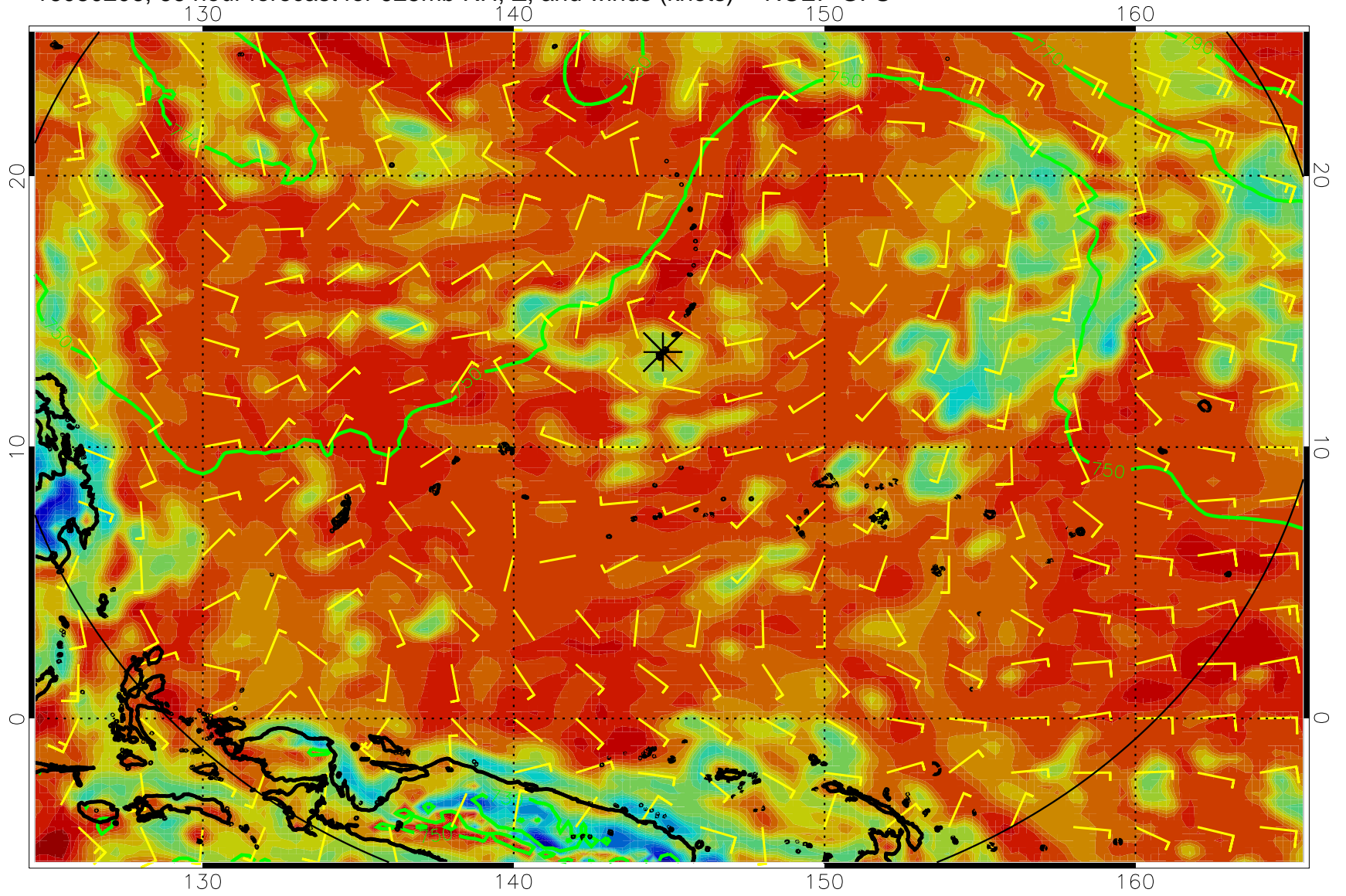
16080206, 66 hour forecast for 925mb RH, Z, and winds (knots) -- NCEP GFS
