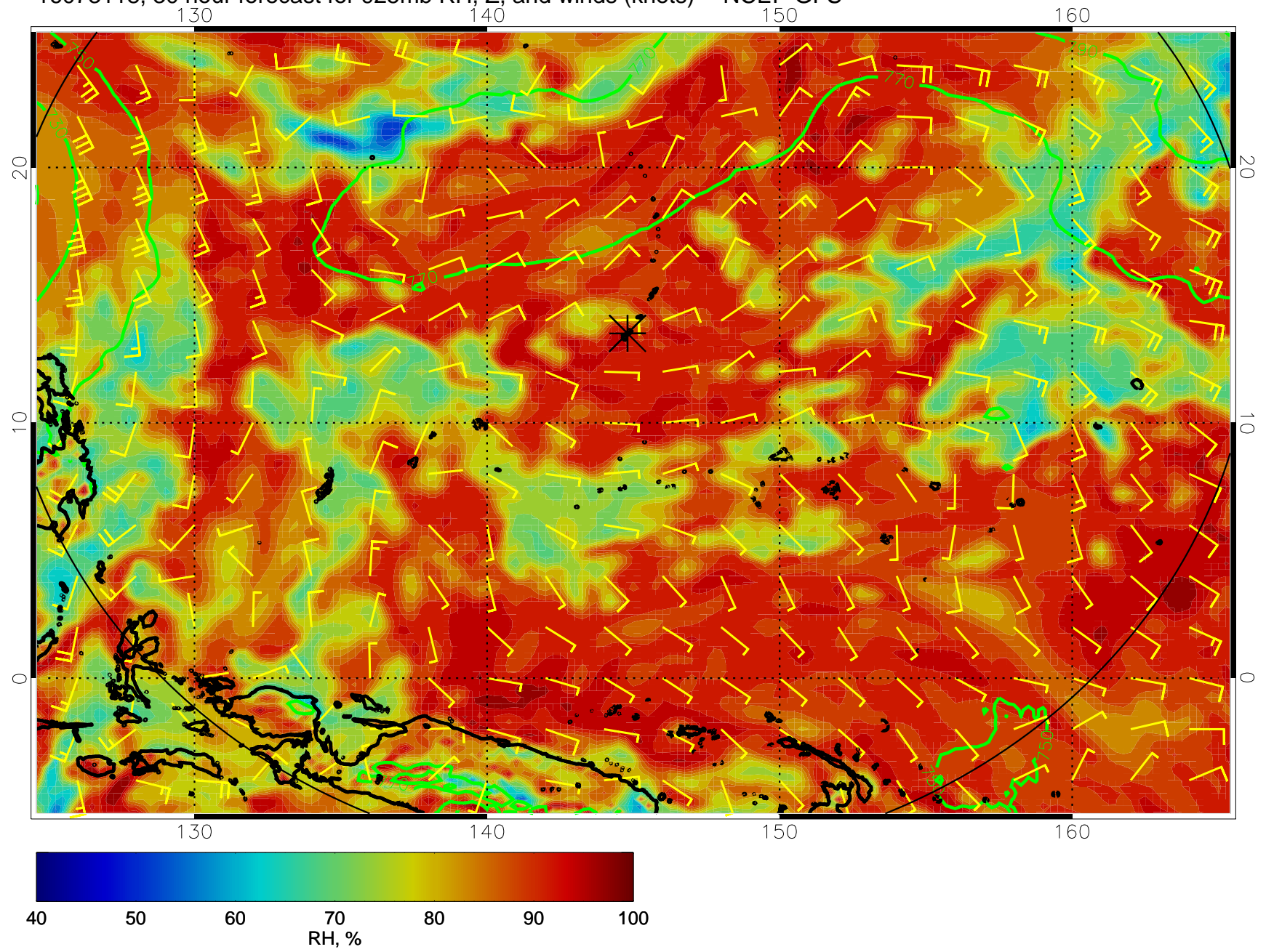
16073118, 30 hour forecast for 925mb RH, Z, and winds (knots) -- NCEP GFS
