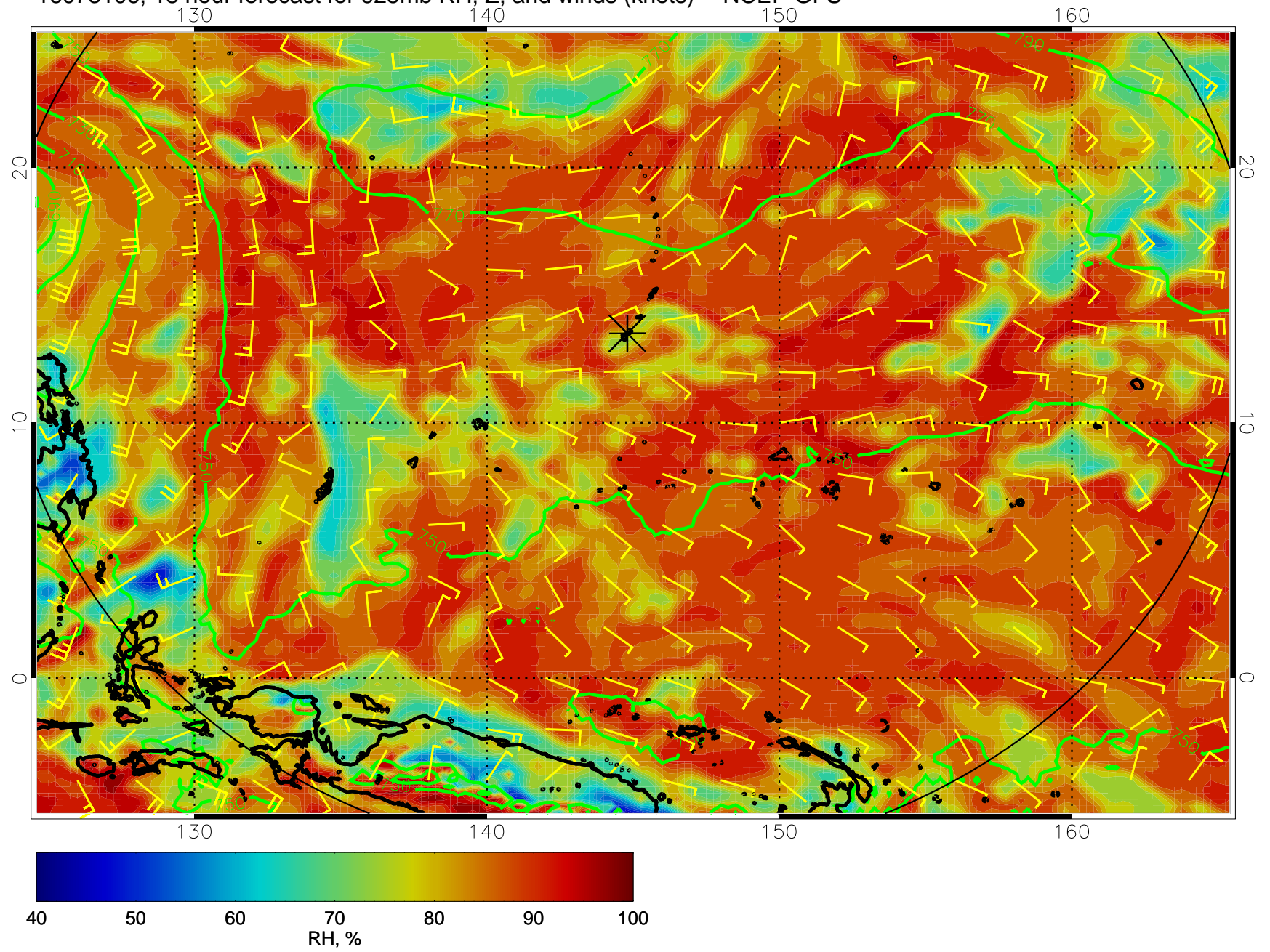
16073106, 18 hour forecast for 925mb RH, Z, and winds (knots) -- NCEP GFS
