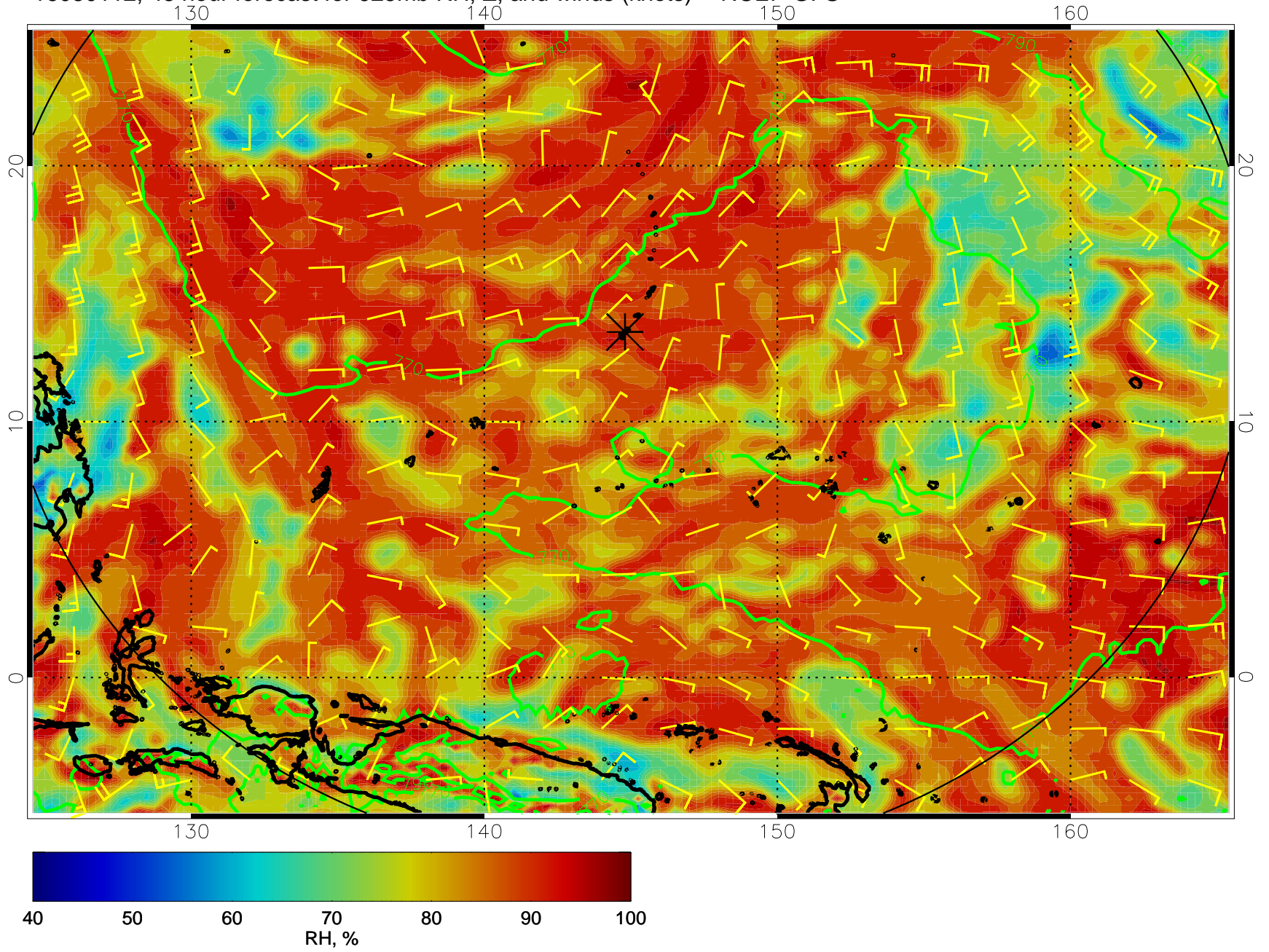
16080112, 48 hour forecast for 925mb RH, Z, and winds (knots) -- NCEP GFS
