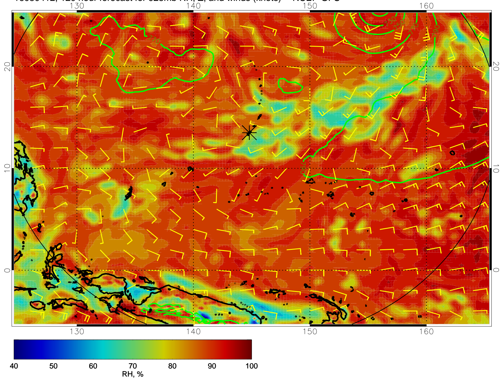
16080412, 120 hour forecast for 925mb RH, Z, and winds (knots) -- NCEP GFS
