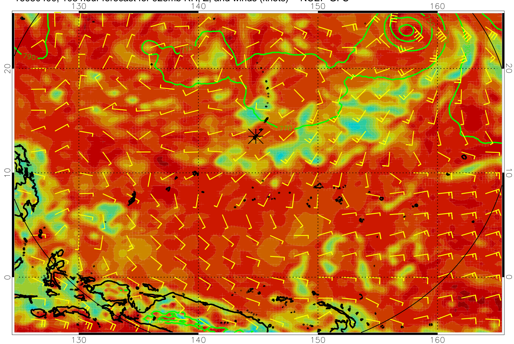
16080400, 108 hour forecast for 925mb RH, Z, and winds (knots) -- NCEP GFS
