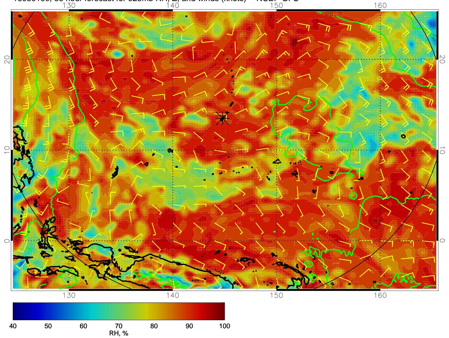
16080100, 36 hour forecast for 925mb RH, Z, and winds (knots) -- NCEP GFS
