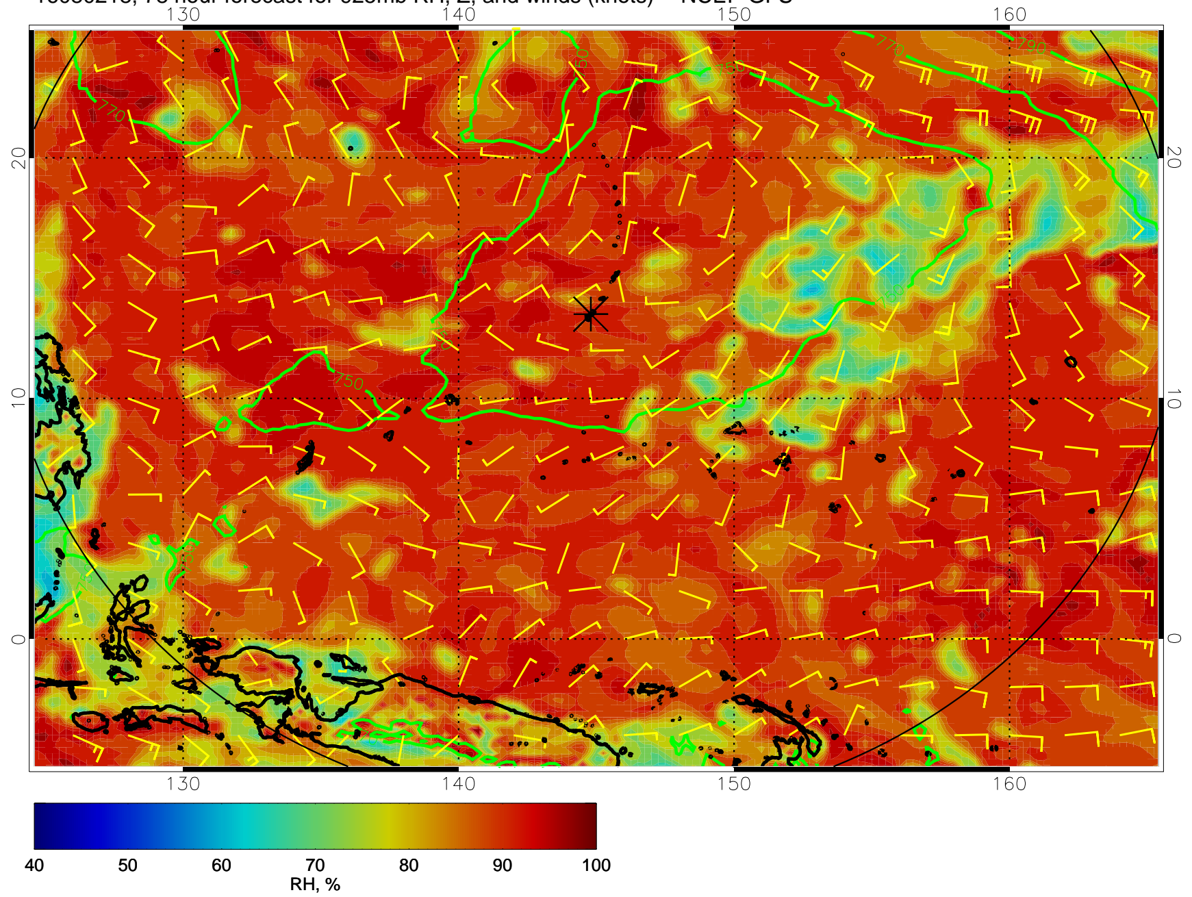
16080218, 78 hour forecast for 925mb RH, Z, and winds (knots) -- NCEP GFS
