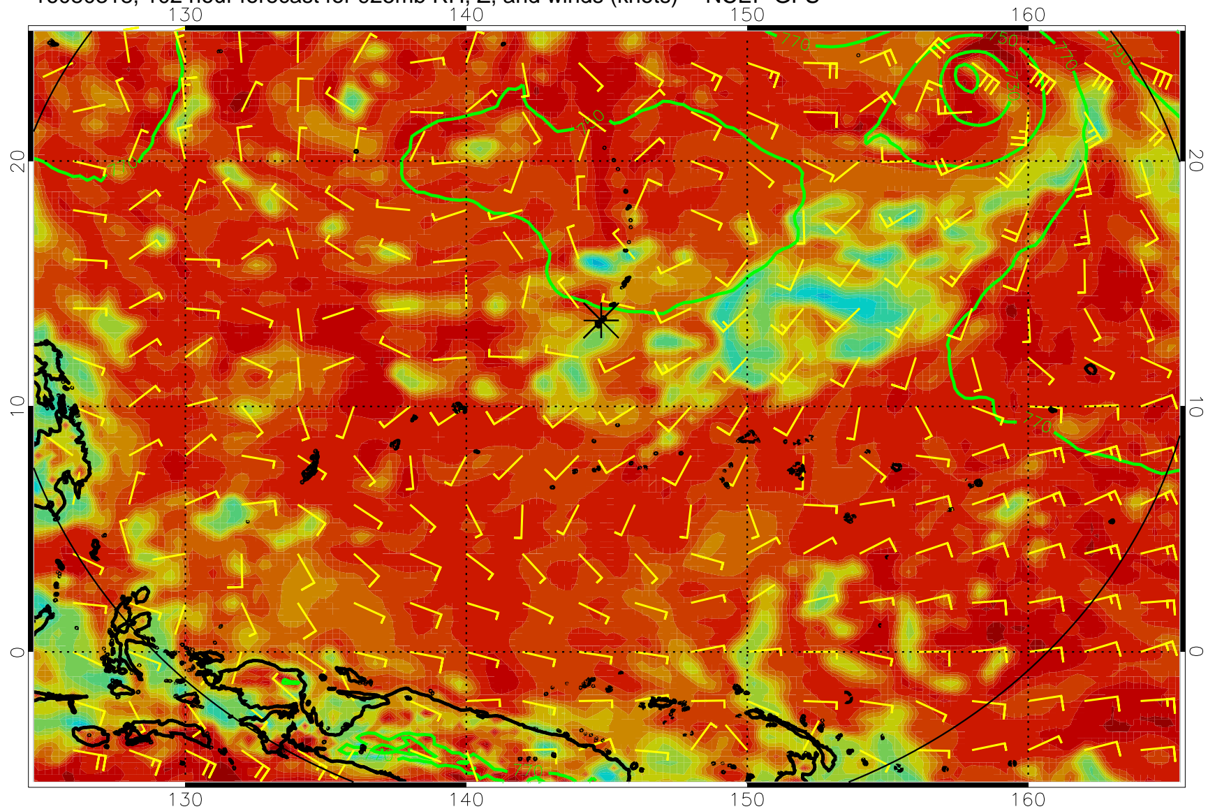
16080318, 102 hour forecast for 925mb RH, Z, and winds (knots) -- NCEP GFS
