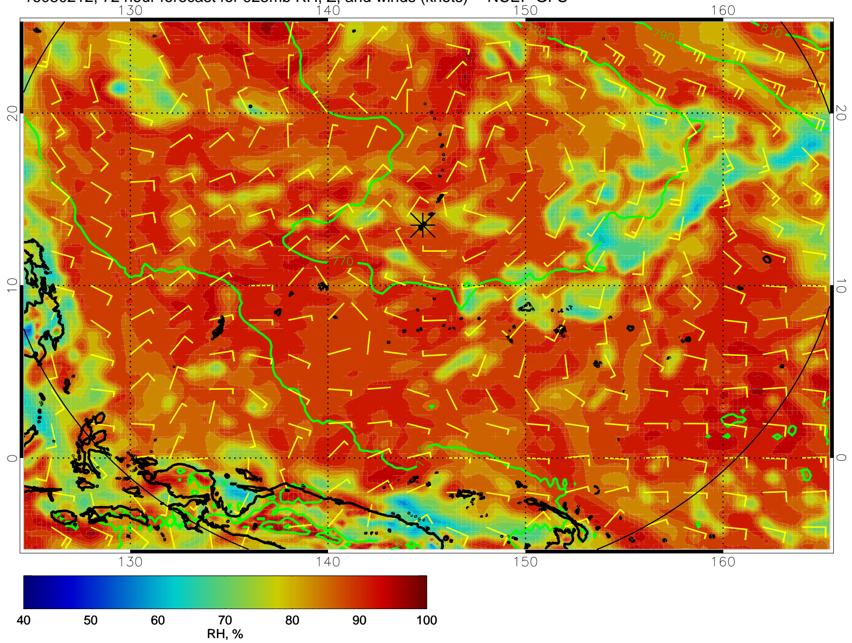
16080212, 72 hour forecast for 925mb RH, Z, and winds (knots) -- NCEP GFS
