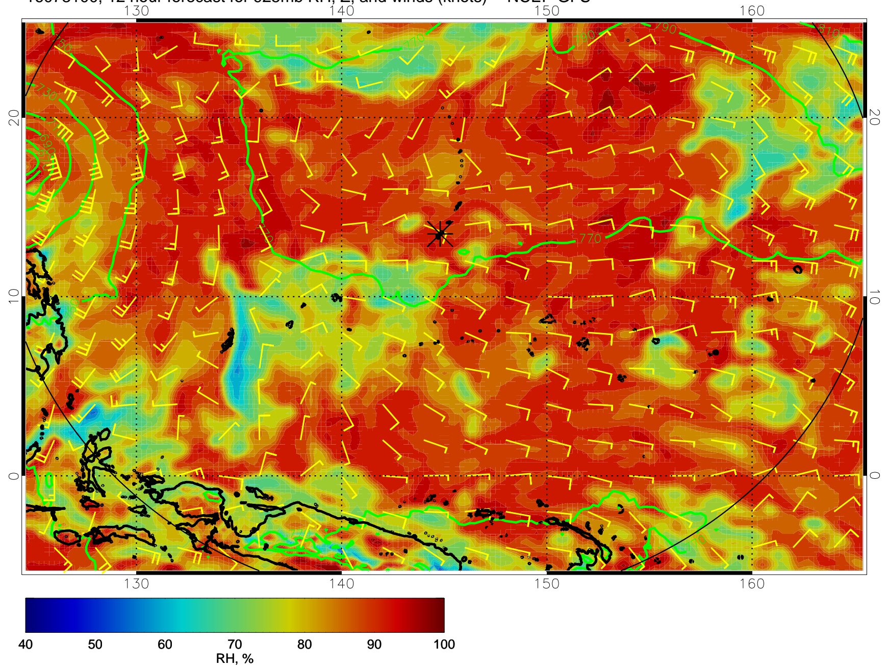
16073100, 12 hour forecast for 925mb RH, Z, and winds (knots) -- NCEP GFS
