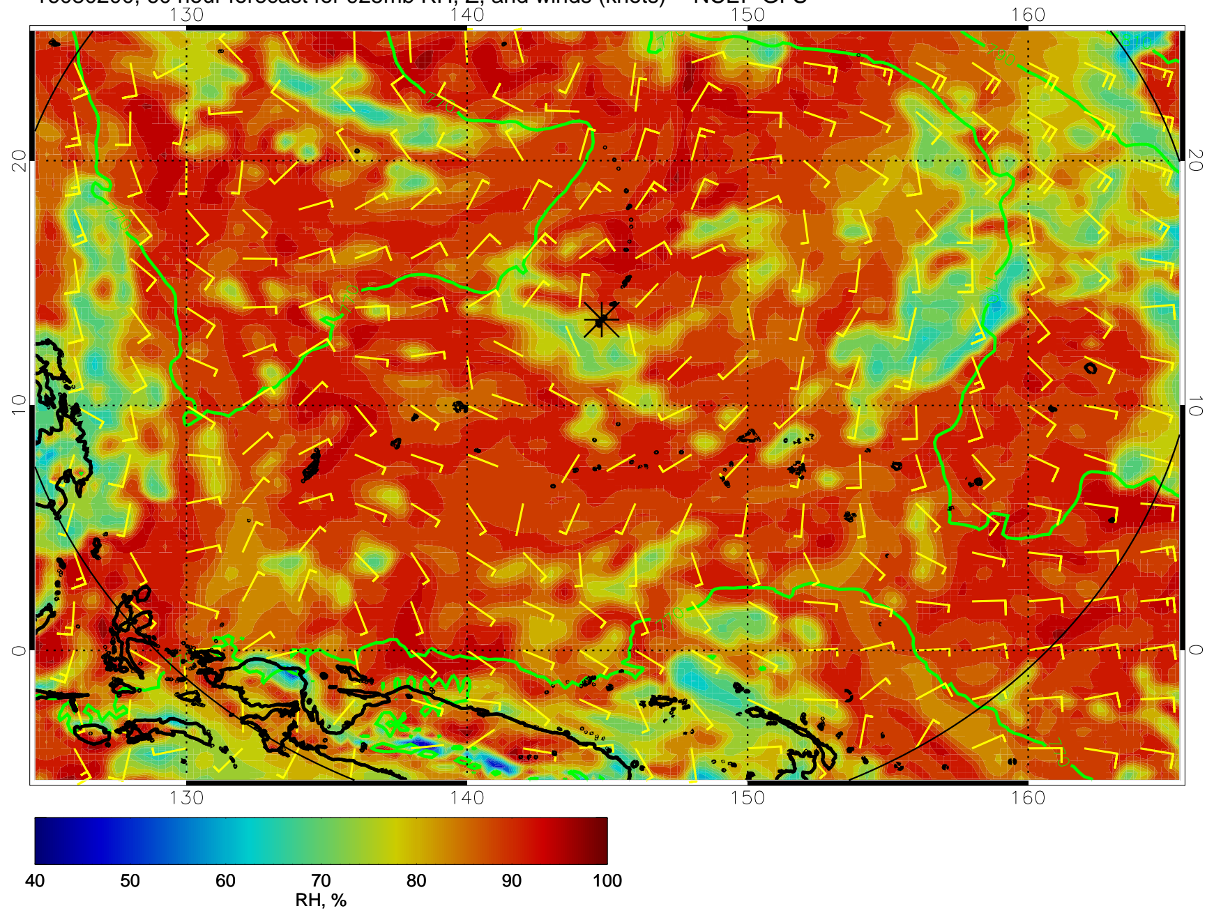
16080200, 60 hour forecast for 925mb RH, Z, and winds (knots) -- NCEP GFS
