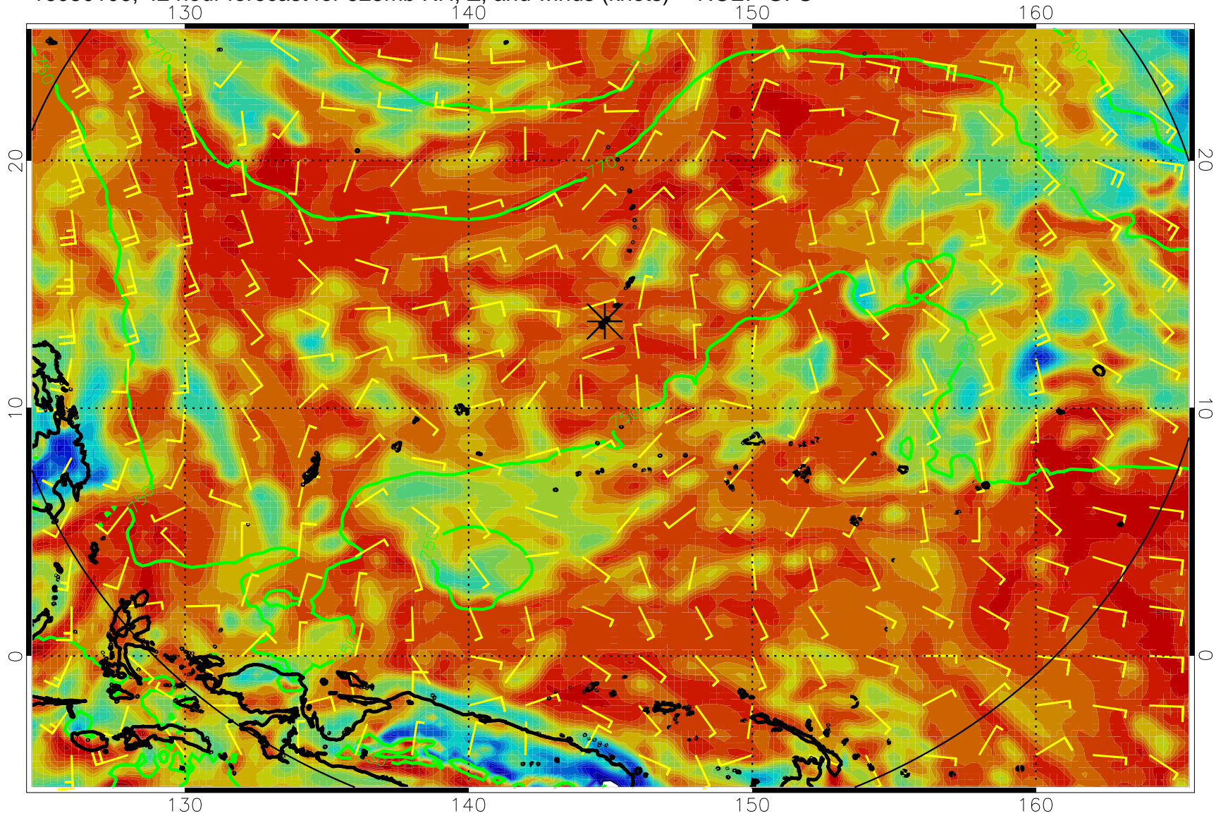
16080106, 42 hour forecast for 925mb RH, Z, and winds (knots) -- NCEP GFS
