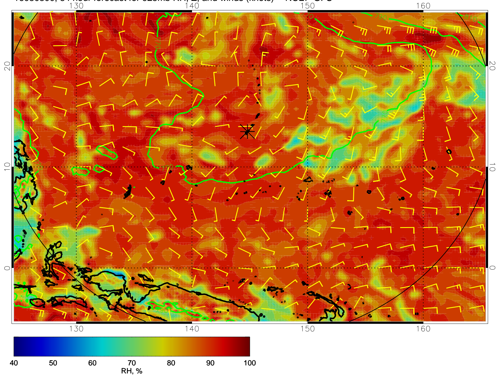
16080300, 84 hour forecast for 925mb RH, Z, and winds (knots) -- NCEP GFS
