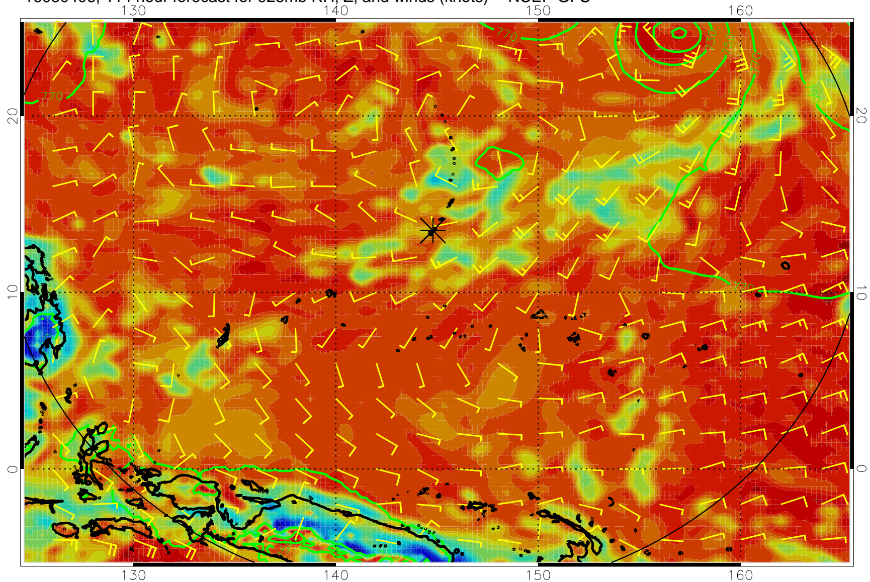
16080406, 114 hour forecast for 925mb RH, Z, and winds (knots) -- NCEP GFS
