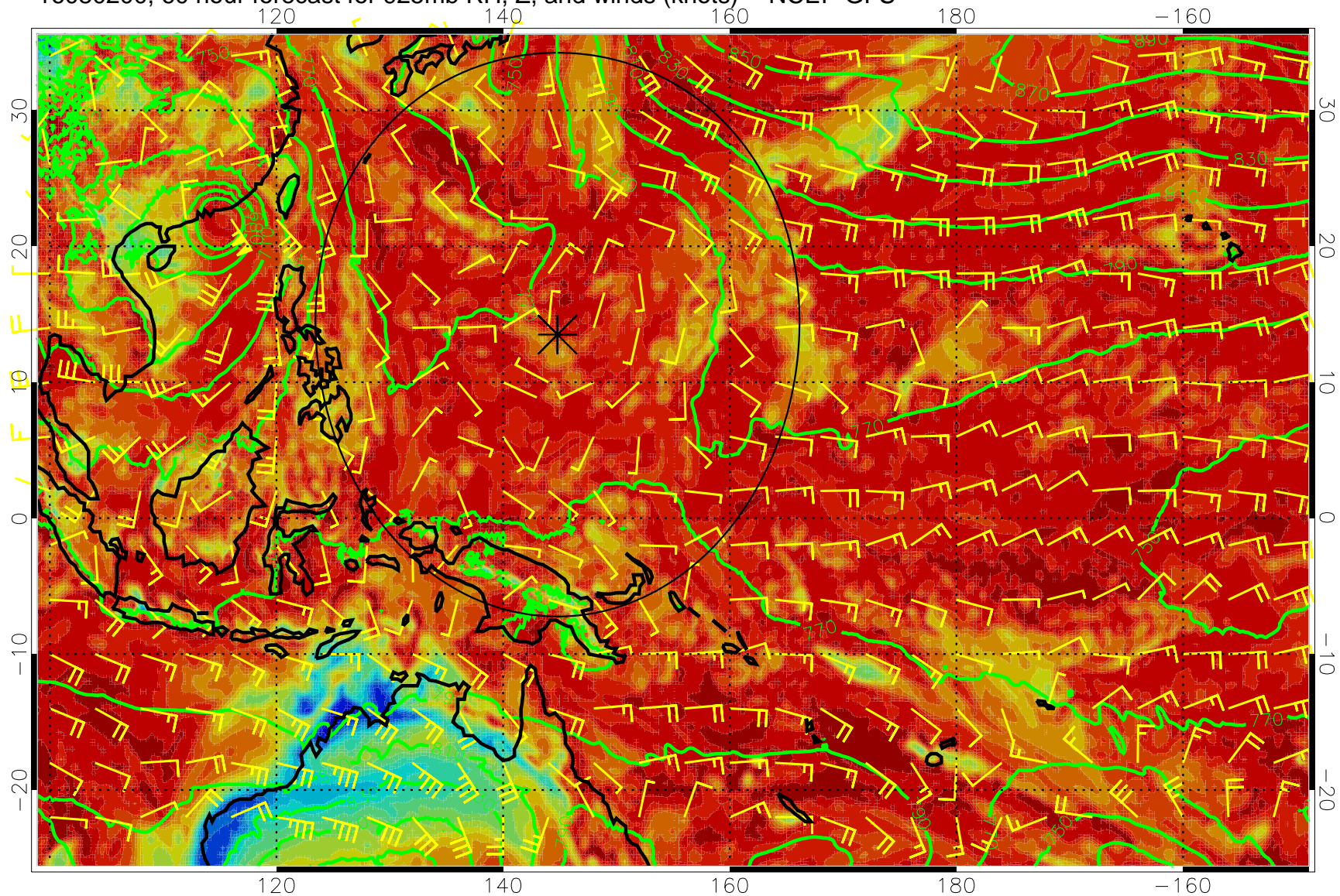
16080200, 60 hour forecast for 925mb RH, Z, and winds (knots) -- NCEP GFS
