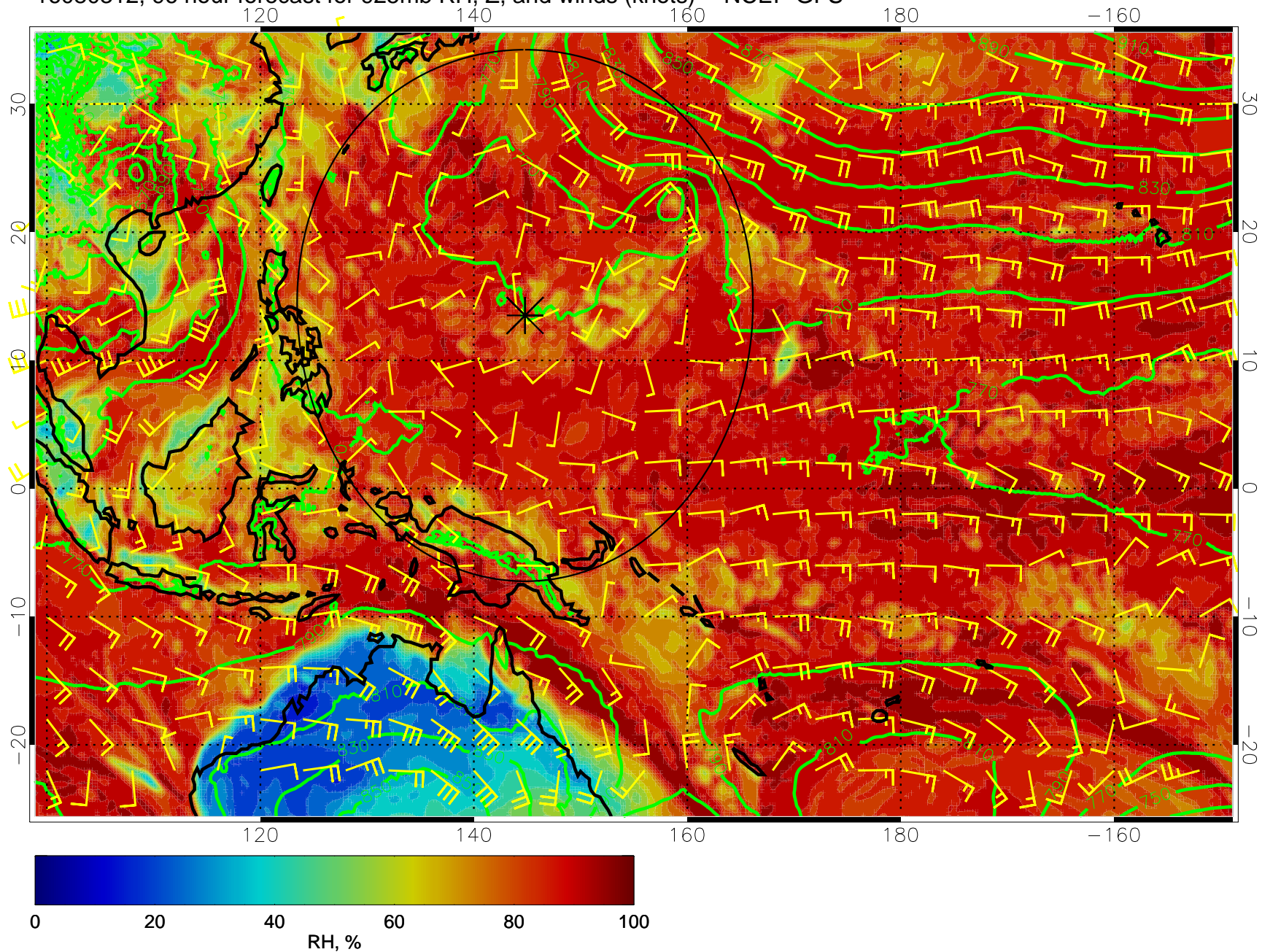
16080312, 96 hour forecast for 925mb RH, Z, and winds (knots) -- NCEP GFS
