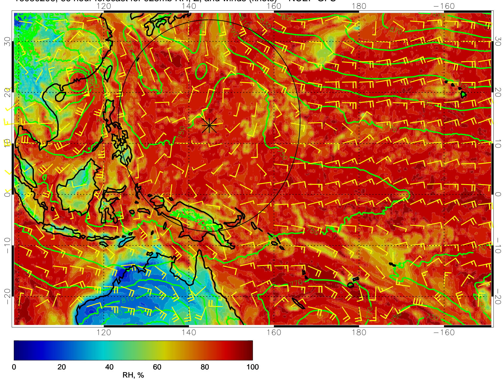
16080206, 66 hour forecast for 925mb RH, Z, and winds (knots) -- NCEP GFS
