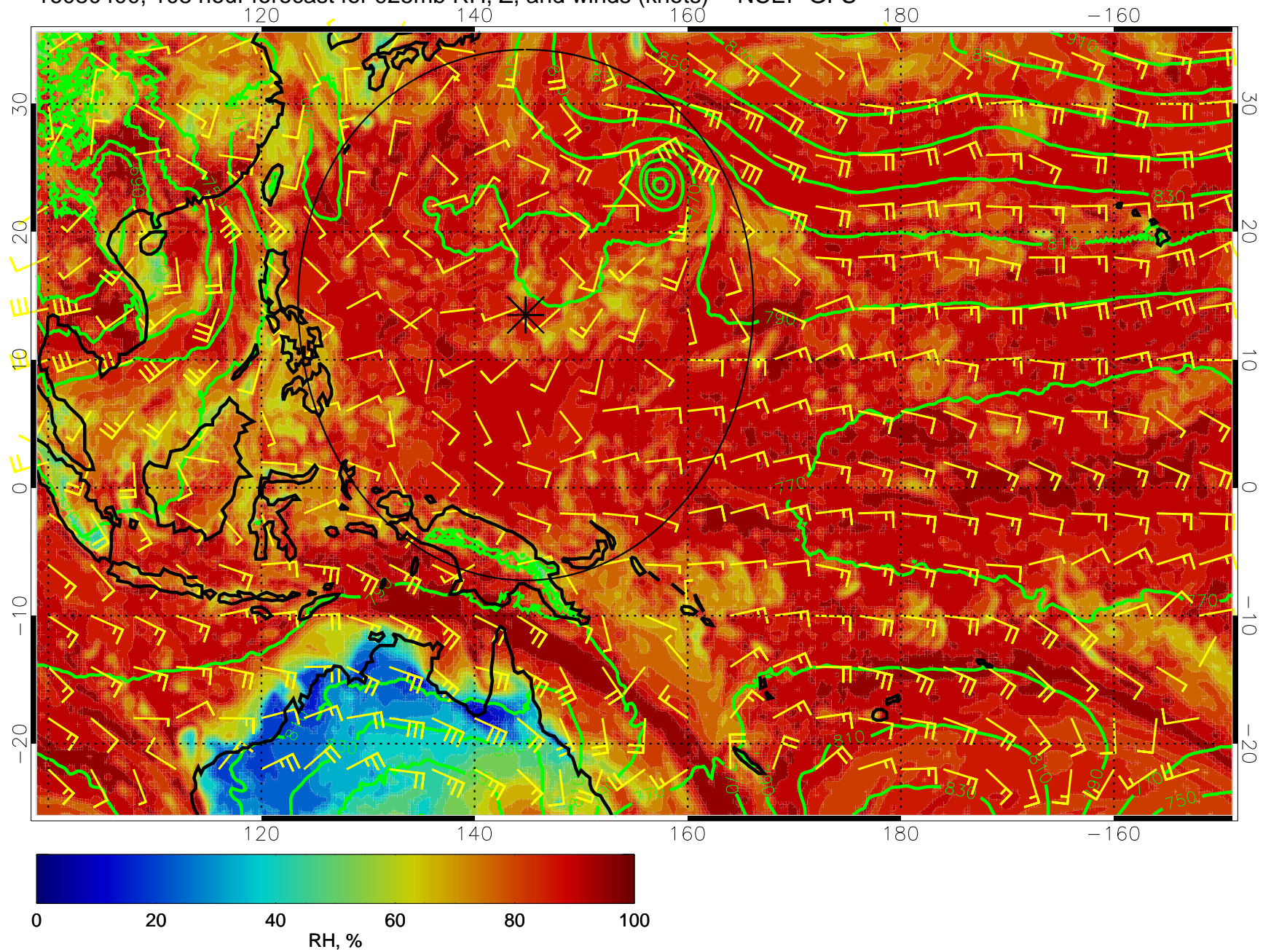
16080400, 108 hour forecast for 925mb RH, Z, and winds (knots) -- NCEP GFS
