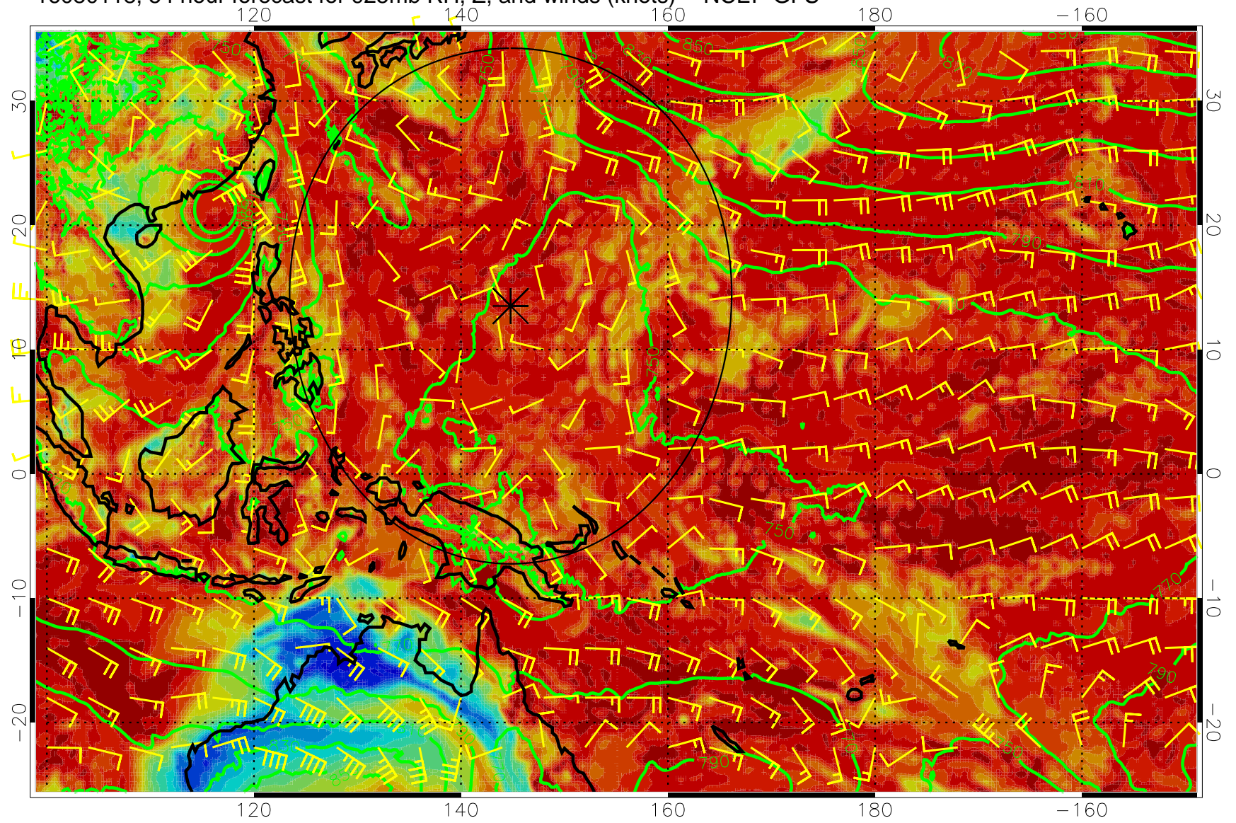
16080118, 54 hour forecast for 925mb RH, Z, and winds (knots) -- NCEP GFS
