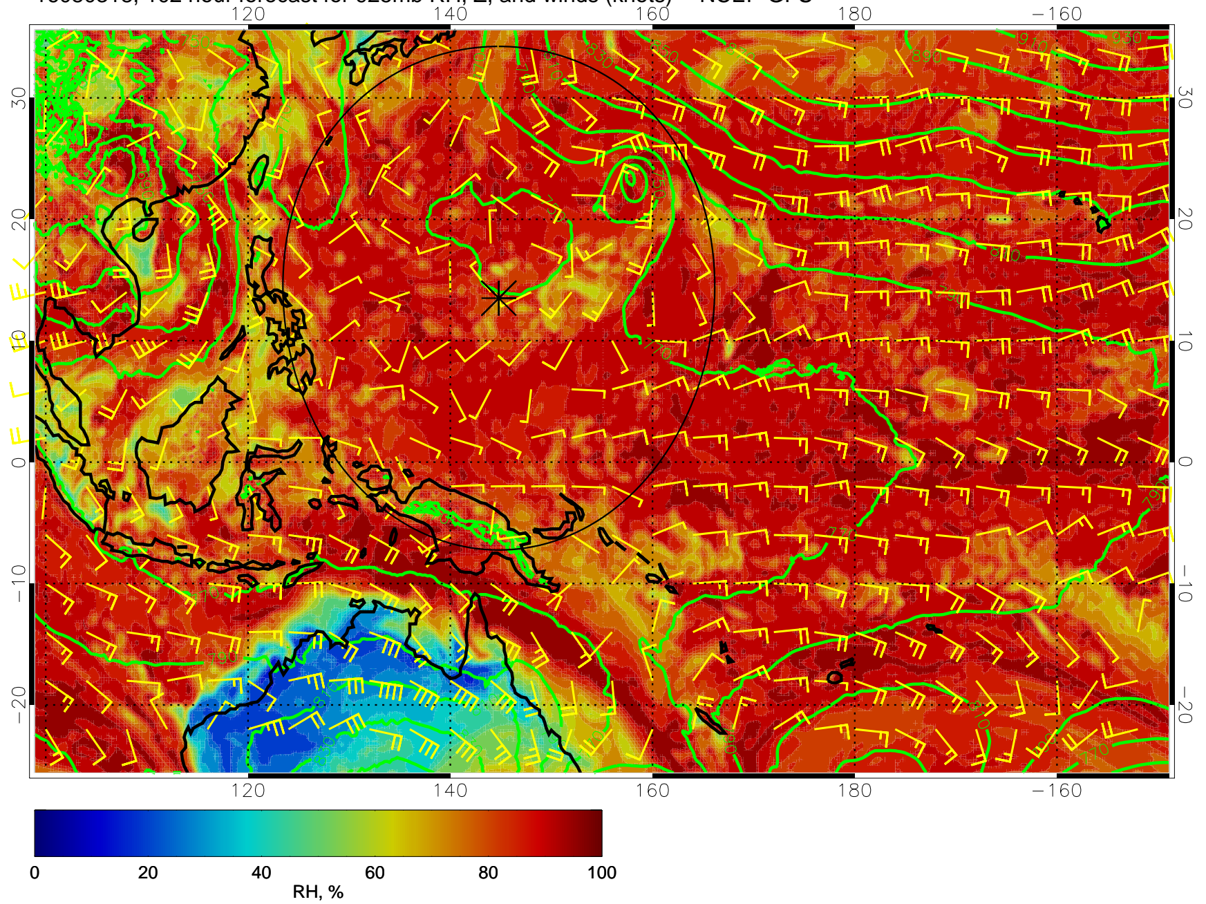
16080318, 102 hour forecast for 925mb RH, Z, and winds (knots) -- NCEP GFS
