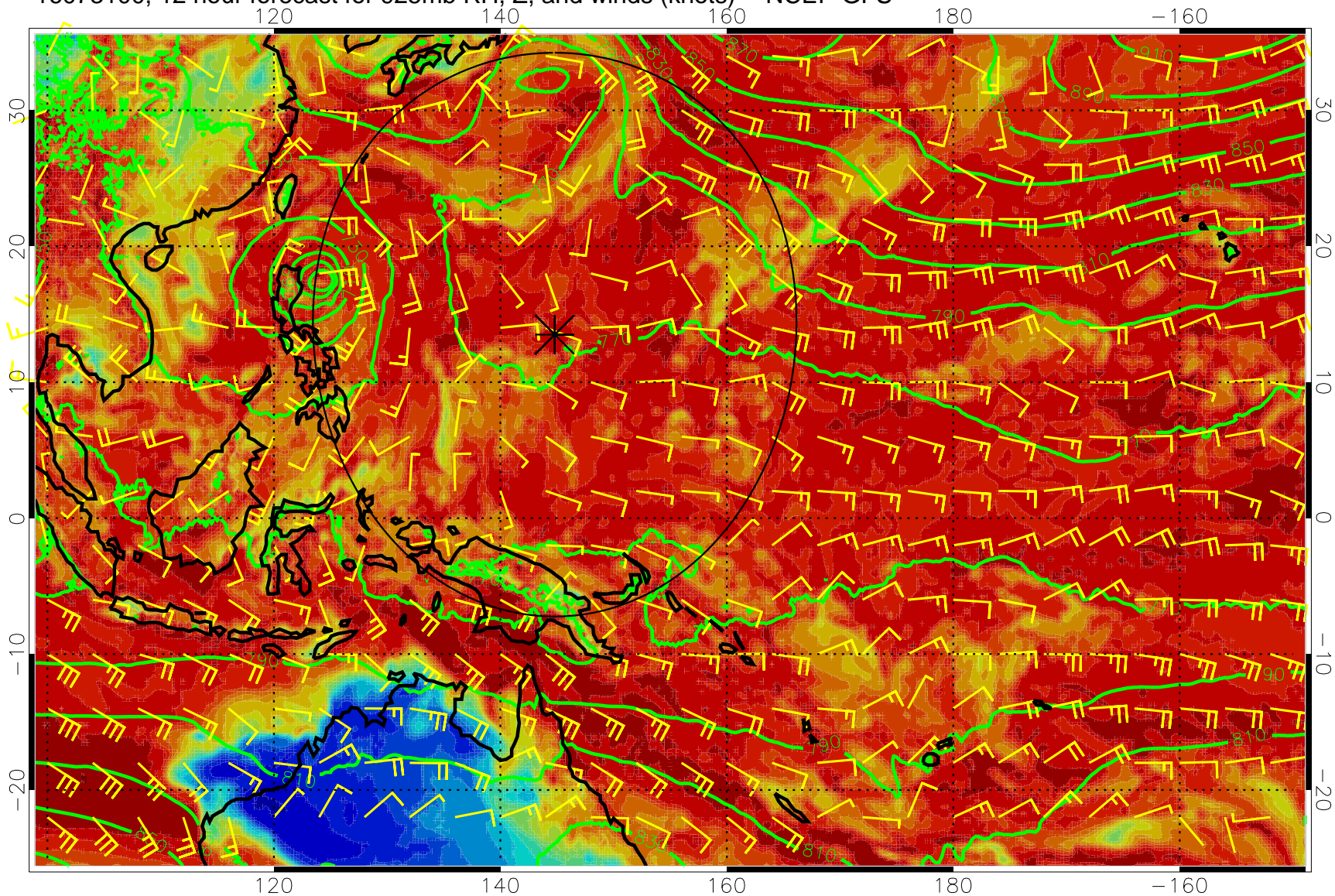
16073100, 12 hour forecast for 925mb RH, Z, and winds (knots) -- NCEP GFS
