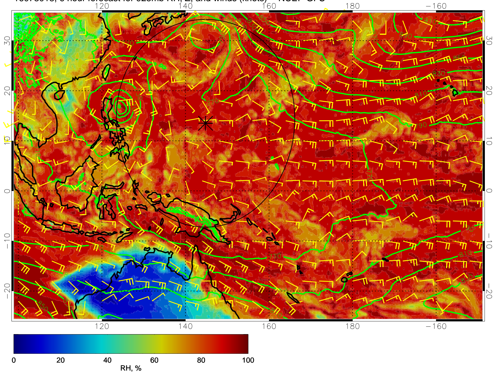
16073018, 6 hour forecast for 925mb RH, Z, and winds (knots) -- NCEP GFS
