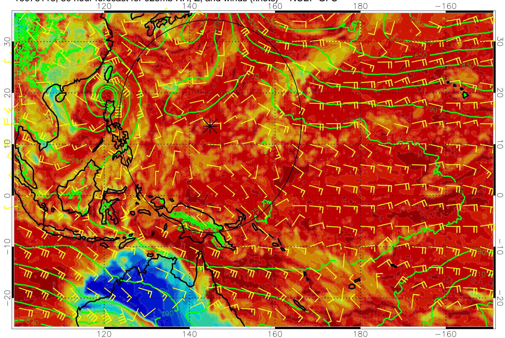
16073118, 30 hour forecast for 925mb RH, Z, and winds (knots) -- NCEP GFS
