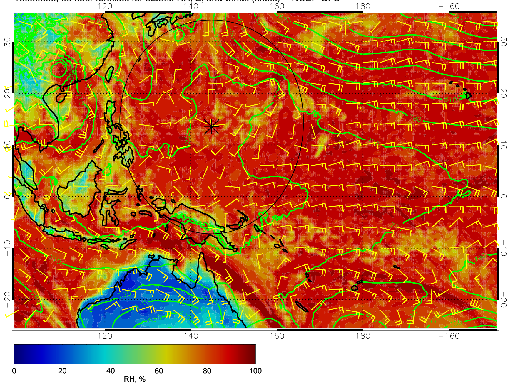
16080306, 90 hour forecast for 925mb RH, Z, and winds (knots) -- NCEP GFS
