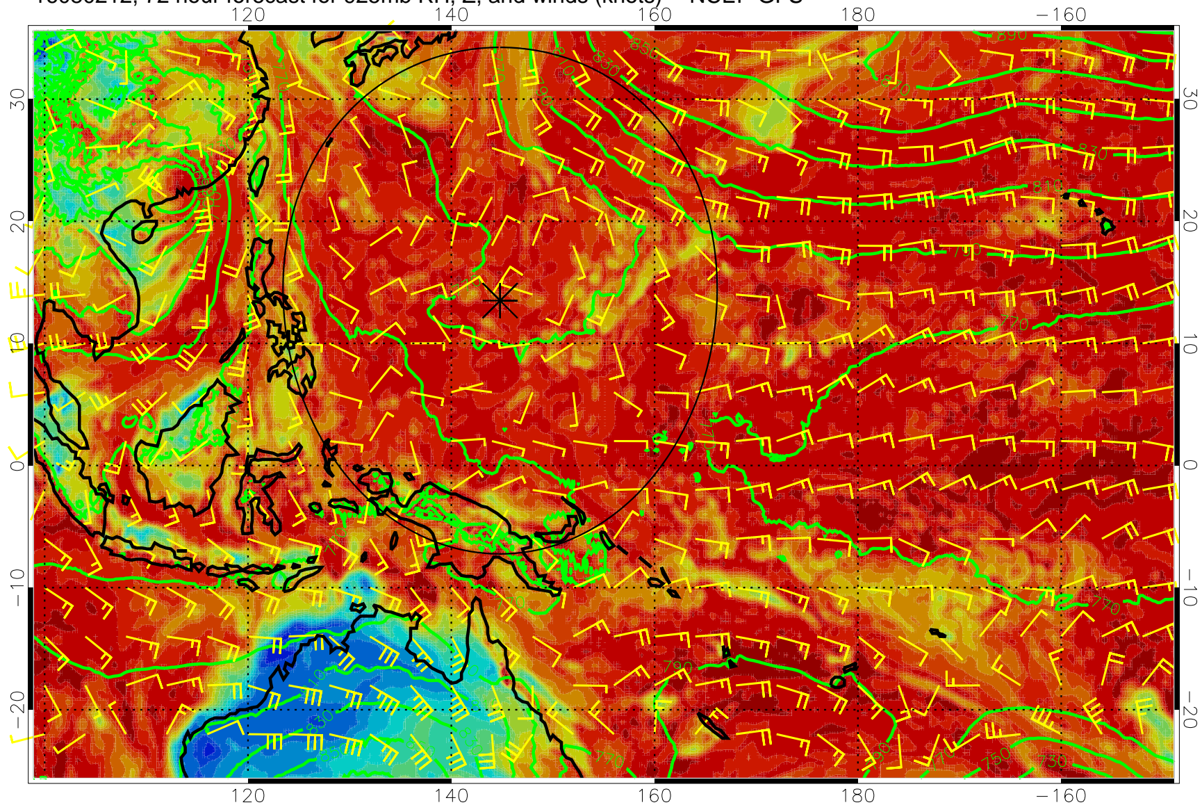
16080212, 72 hour forecast for 925mb RH, Z, and winds (knots) -- NCEP GFS
