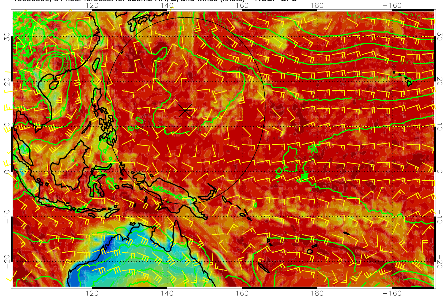
16080300, 84 hour forecast for 925mb RH, Z, and winds (knots) -- NCEP GFS
