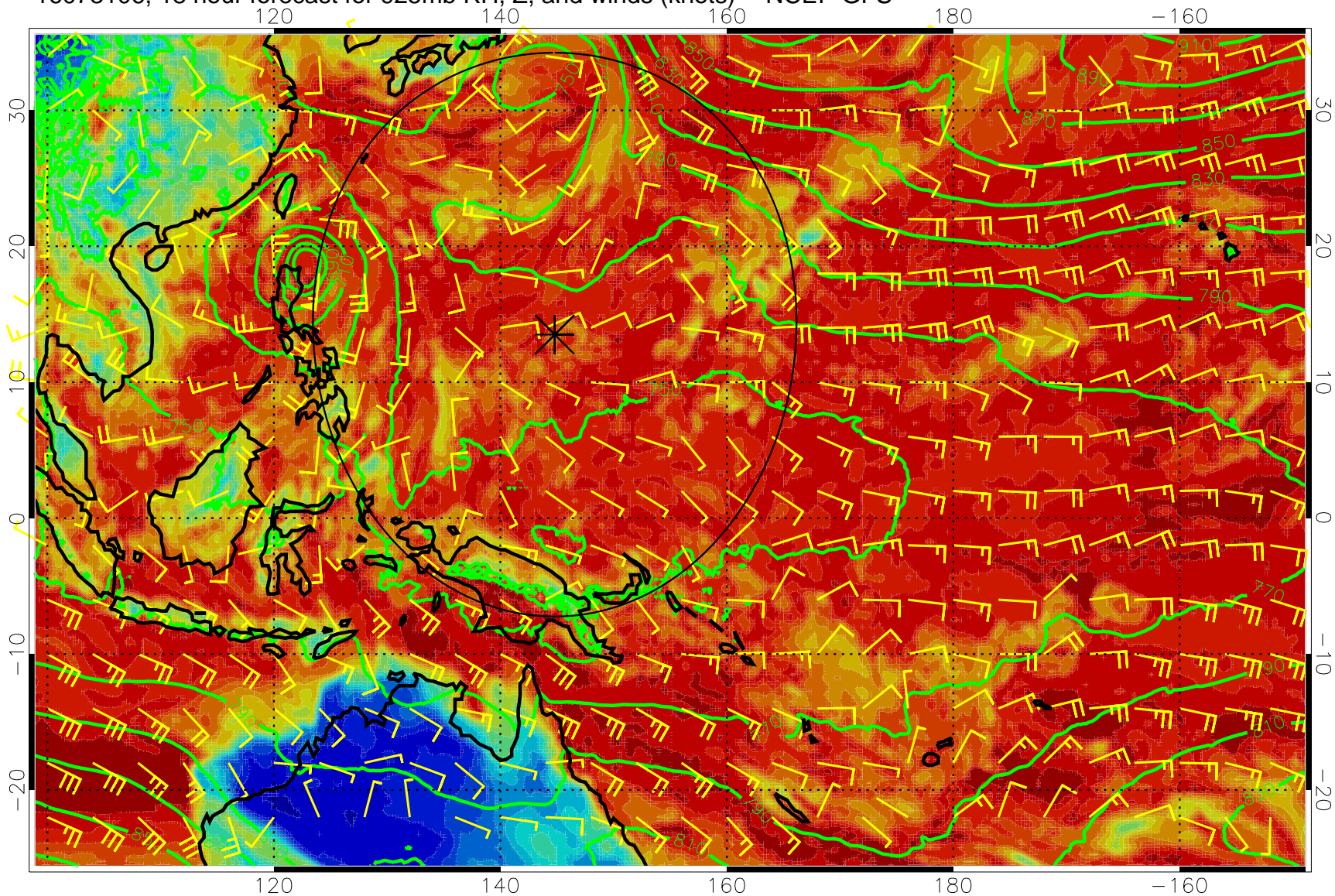
16073106, 18 hour forecast for 925mb RH, Z, and winds (knots) -- NCEP GFS
