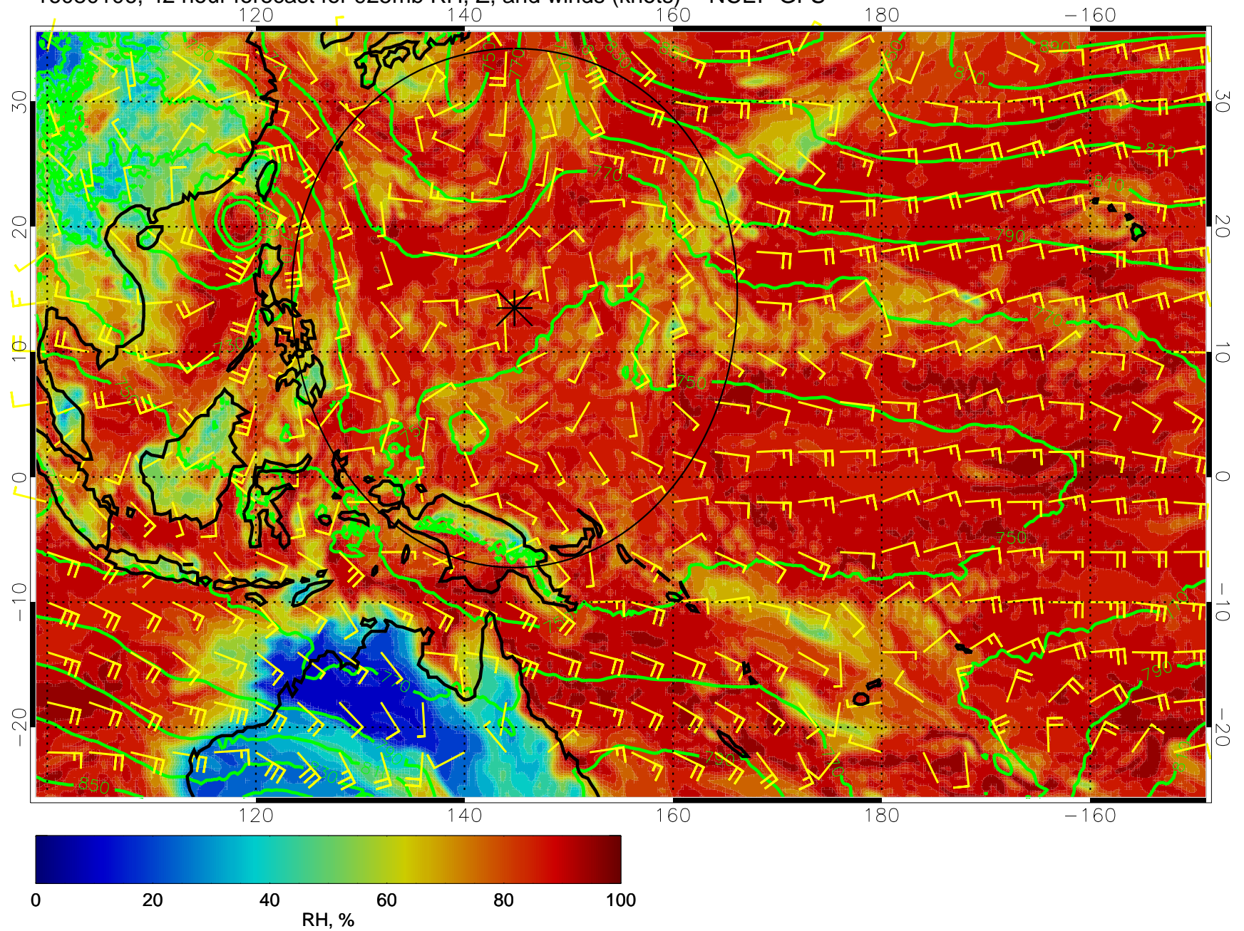
16080106, 42 hour forecast for 925mb RH, Z, and winds (knots) -- NCEP GFS
