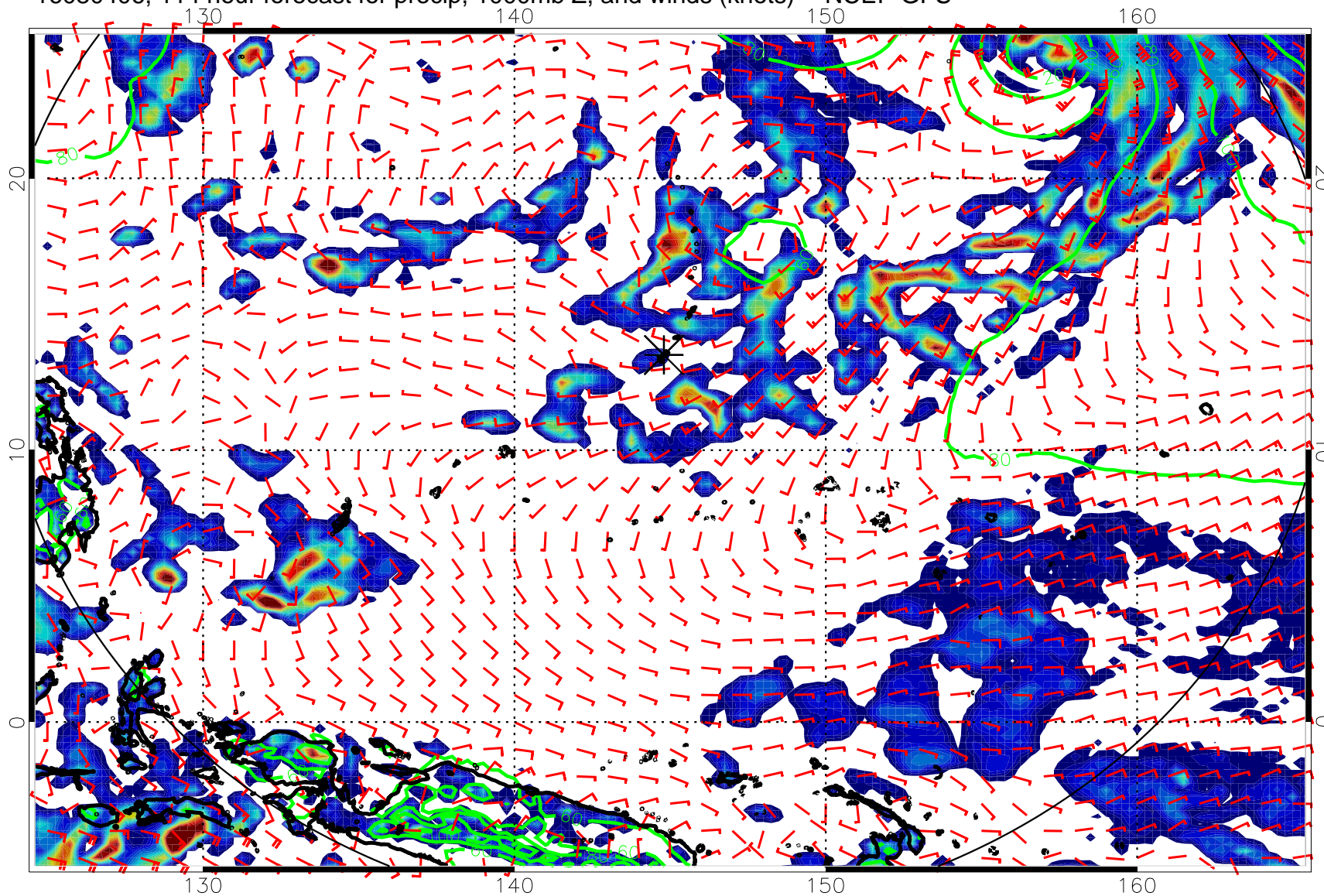
16080406, 114 hour forecast for precip, 1000mb Z, and winds (knots) -- NCEP GFS
