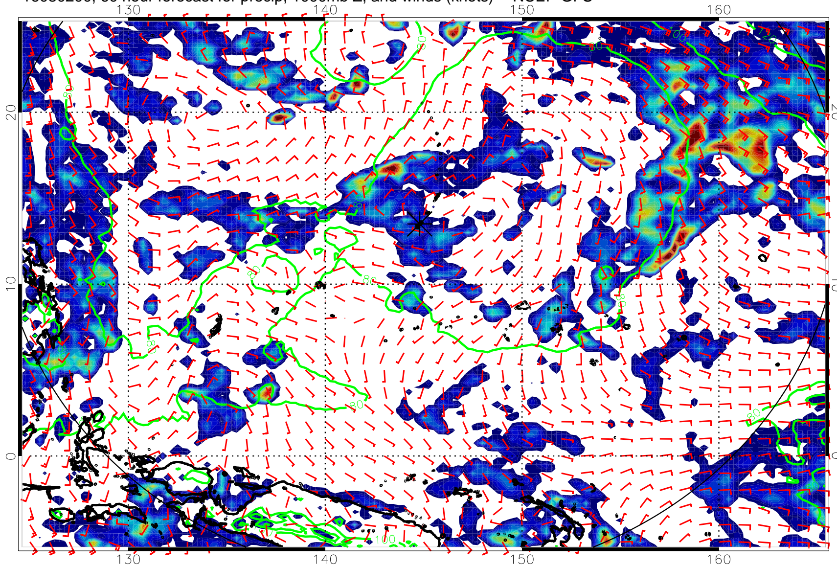
16080200, 60 hour forecast for precip, 1000mb Z, and winds (knots) -- NCEP GFS
