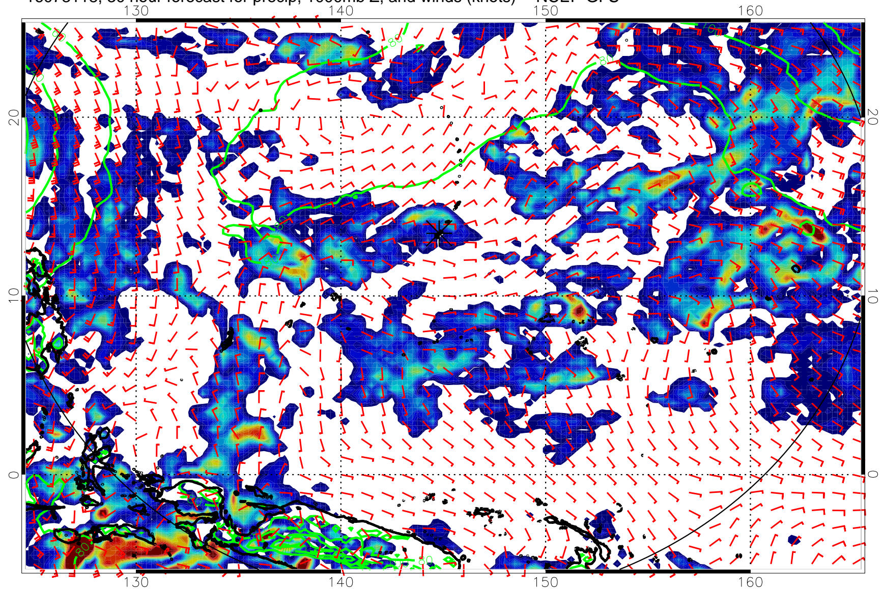
16073118, 30 hour forecast for precip, 1000mb Z, and winds (knots) -- NCEP GFS
