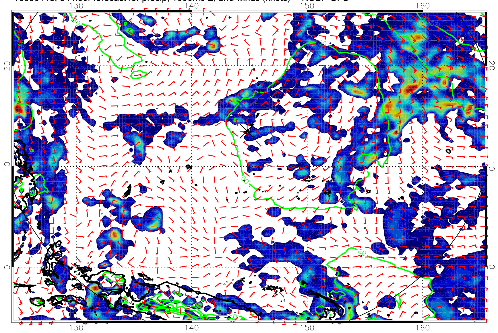
16080118, 54 hour forecast for precip, 1000mb Z, and winds (knots) -- NCEP GFS
