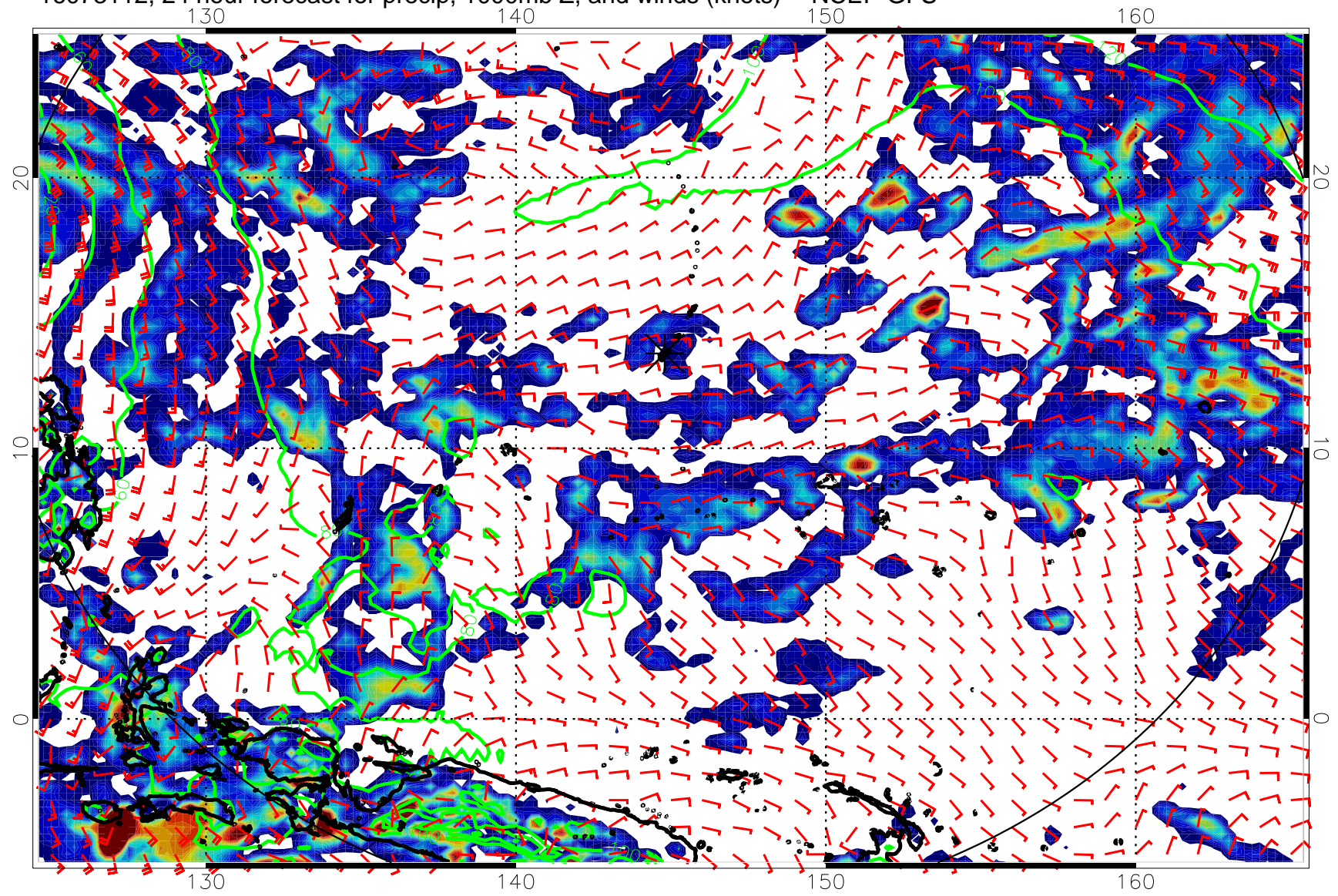
16073112, 24 hour forecast for precip, 1000mb Z, and winds (knots) -- NCEP GFS
