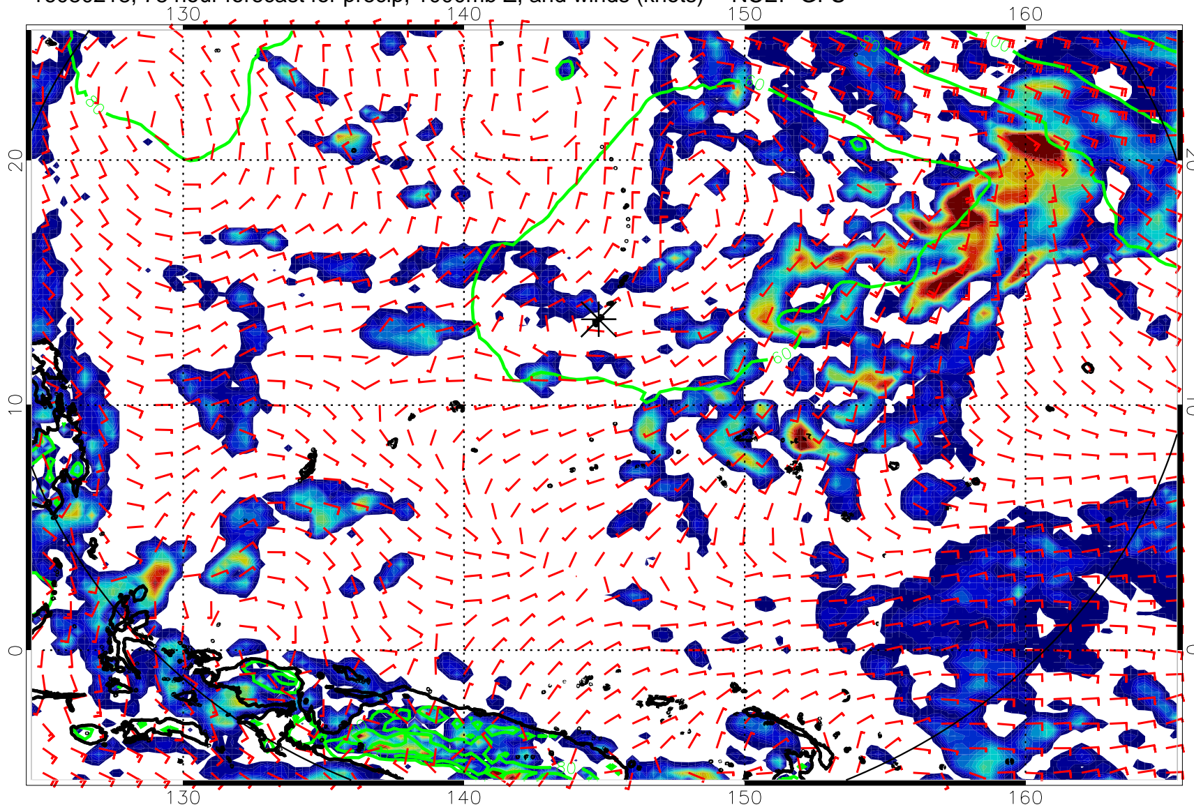
16080218, 78 hour forecast for precip, 1000mb Z, and winds (knots) -- NCEP GFS
