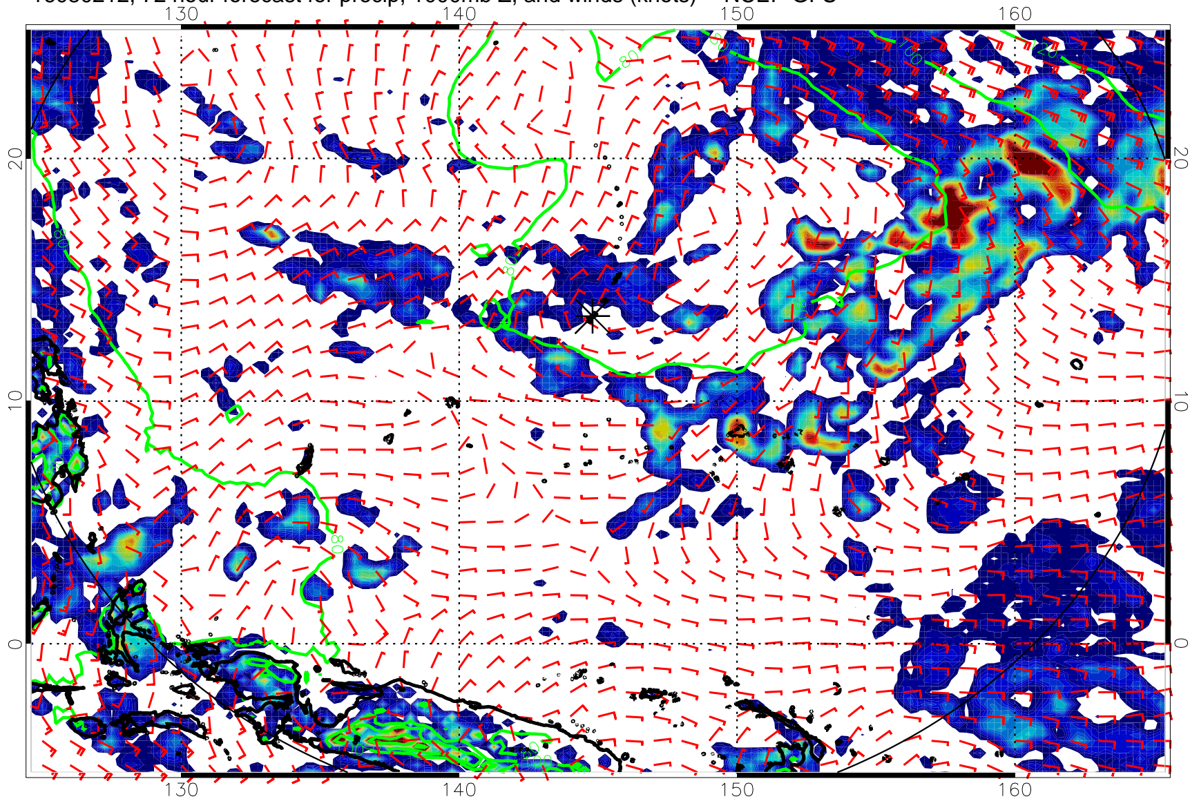
16080212, 72 hour forecast for precip, 1000mb Z, and winds (knots) -- NCEP GFS
