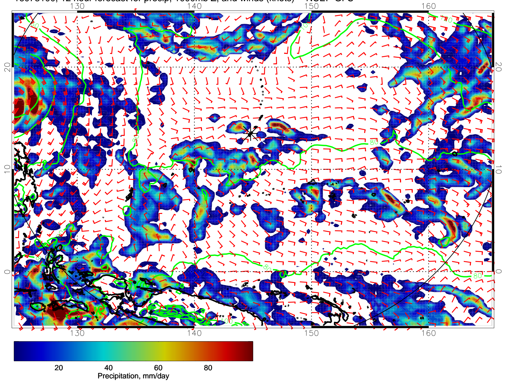
16073100, 12 hour forecast for precip, 1000mb Z, and winds (knots) -- NCEP GFS
