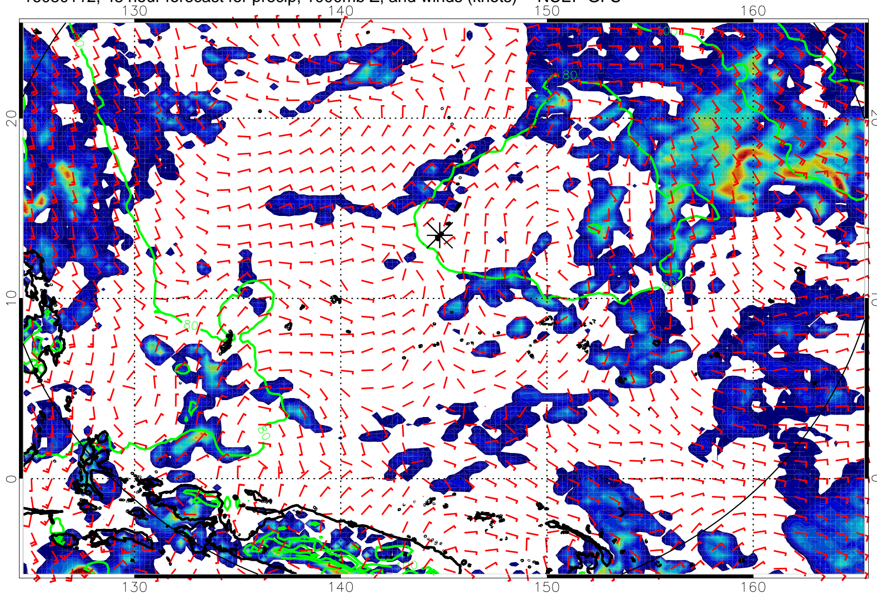
16080112, 48 hour forecast for precip, 1000mb Z, and winds (knots) -- NCEP GFS
