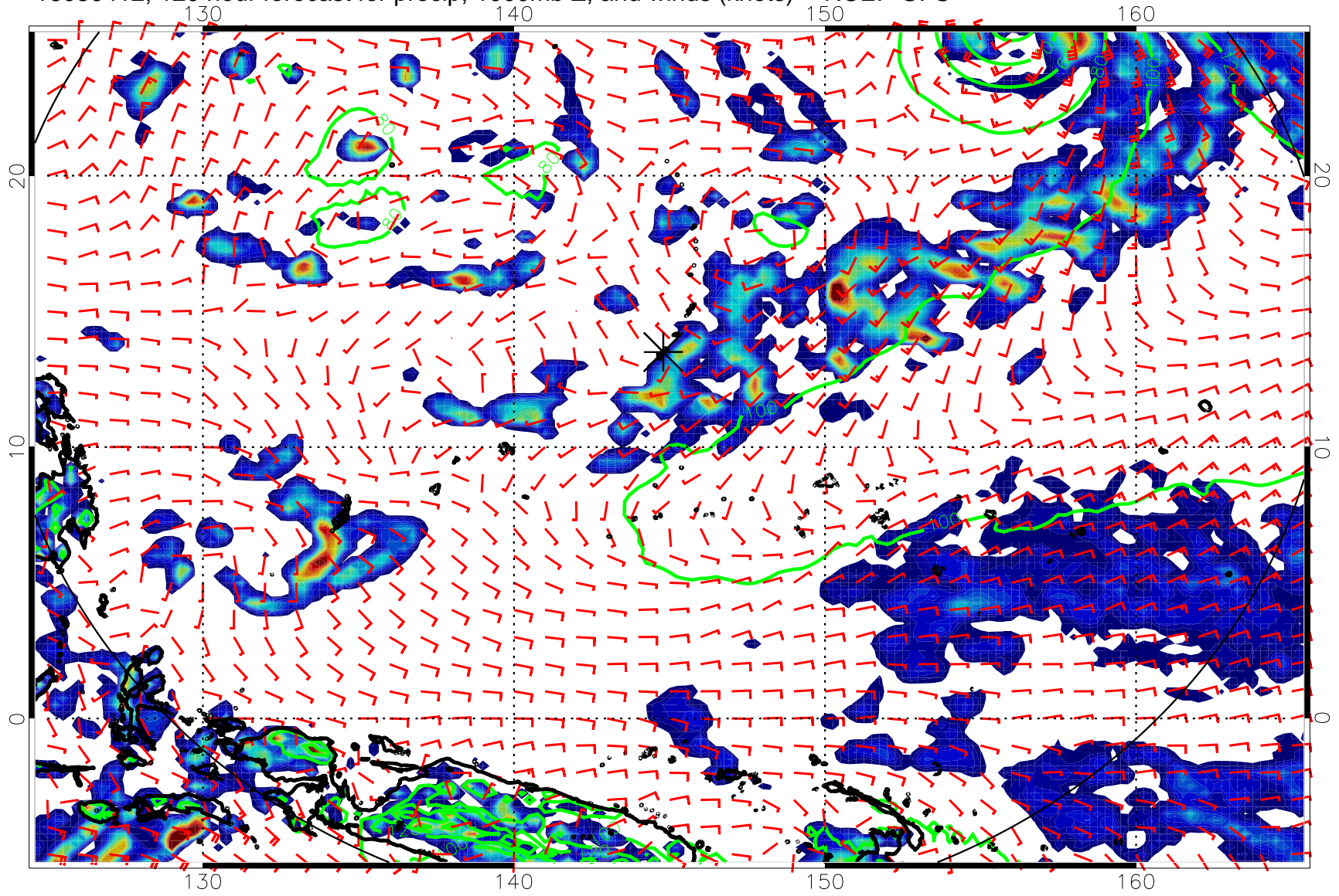
16080412, 120 hour forecast for precip, 1000mb Z, and winds (knots) -- NCEP GFS
