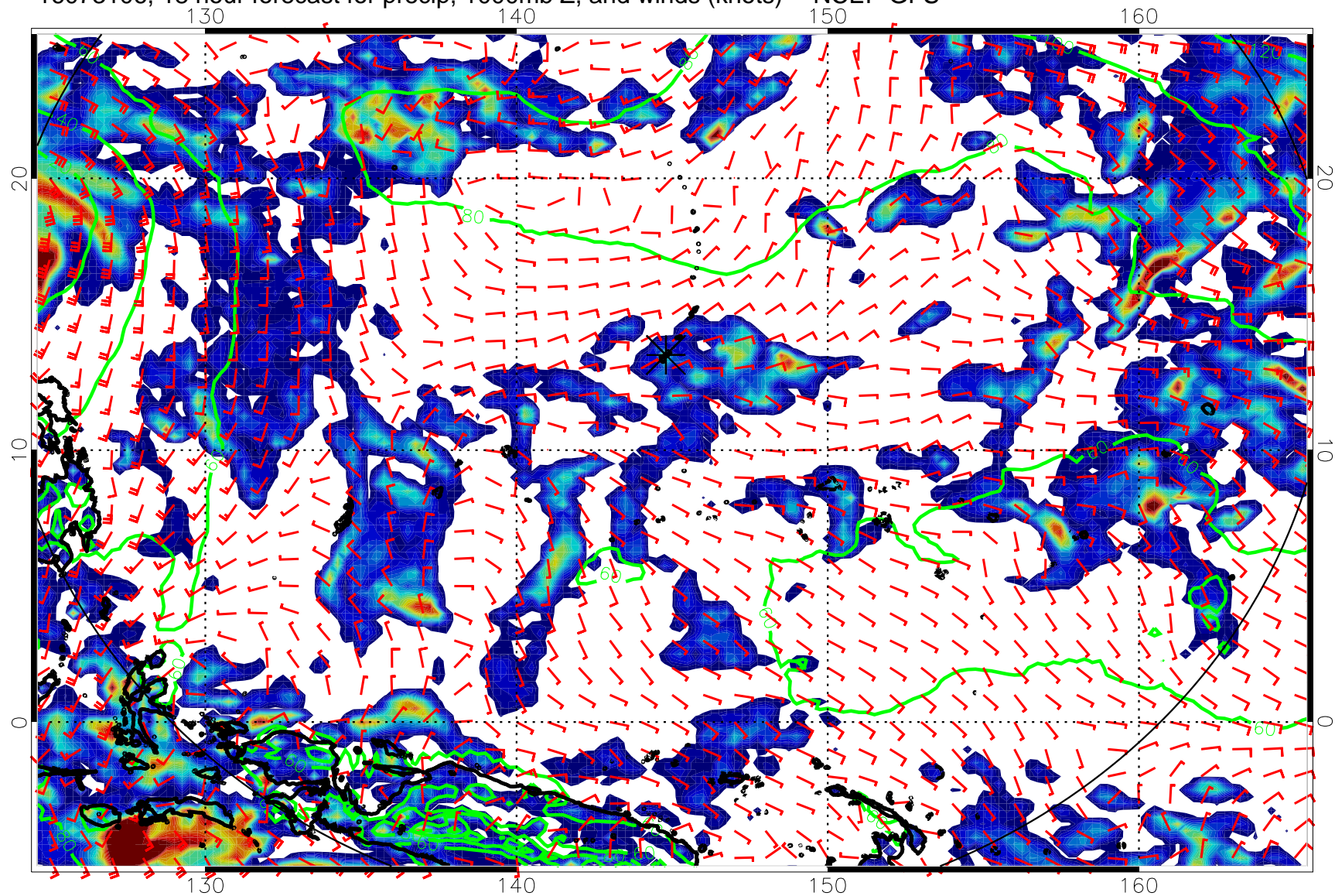
16073106, 18 hour forecast for precip, 1000mb Z, and winds (knots) -- NCEP GFS
