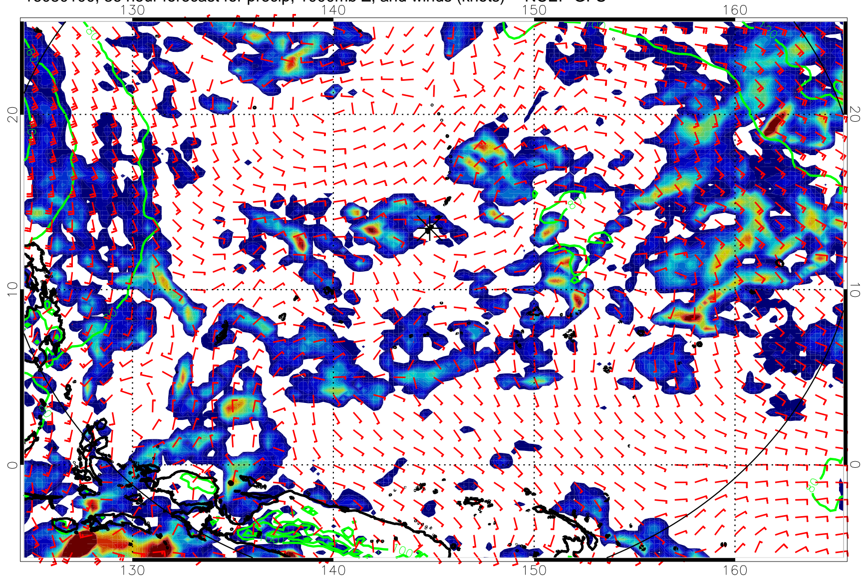
16080100, 36 hour forecast for precip, 1000mb Z, and winds (knots) -- NCEP GFS
