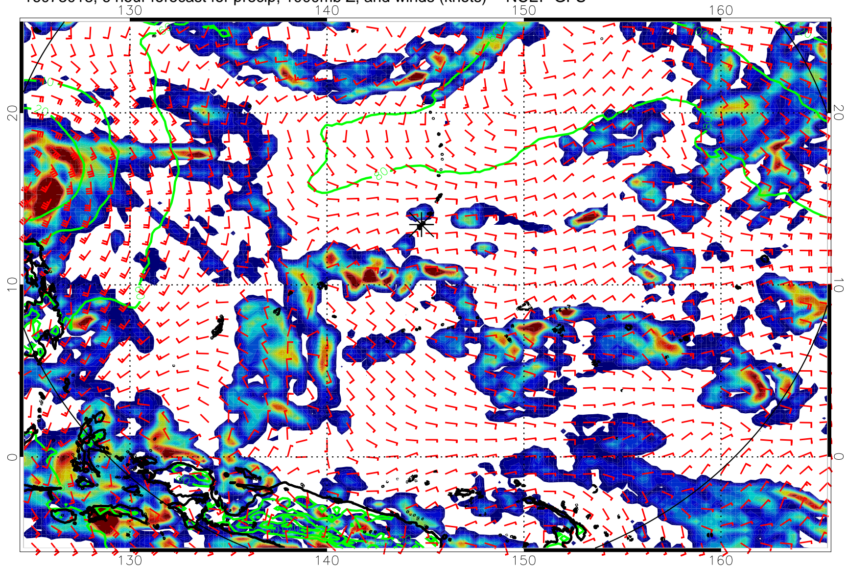
16073018, 6 hour forecast for precip, 1000mb Z, and winds (knots) -- NCEP GFS
