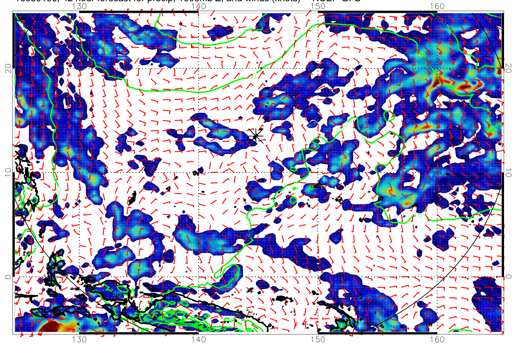
16080106, 42 hour forecast for precip, 1000mb Z, and winds (knots) -- NCEP GFS
