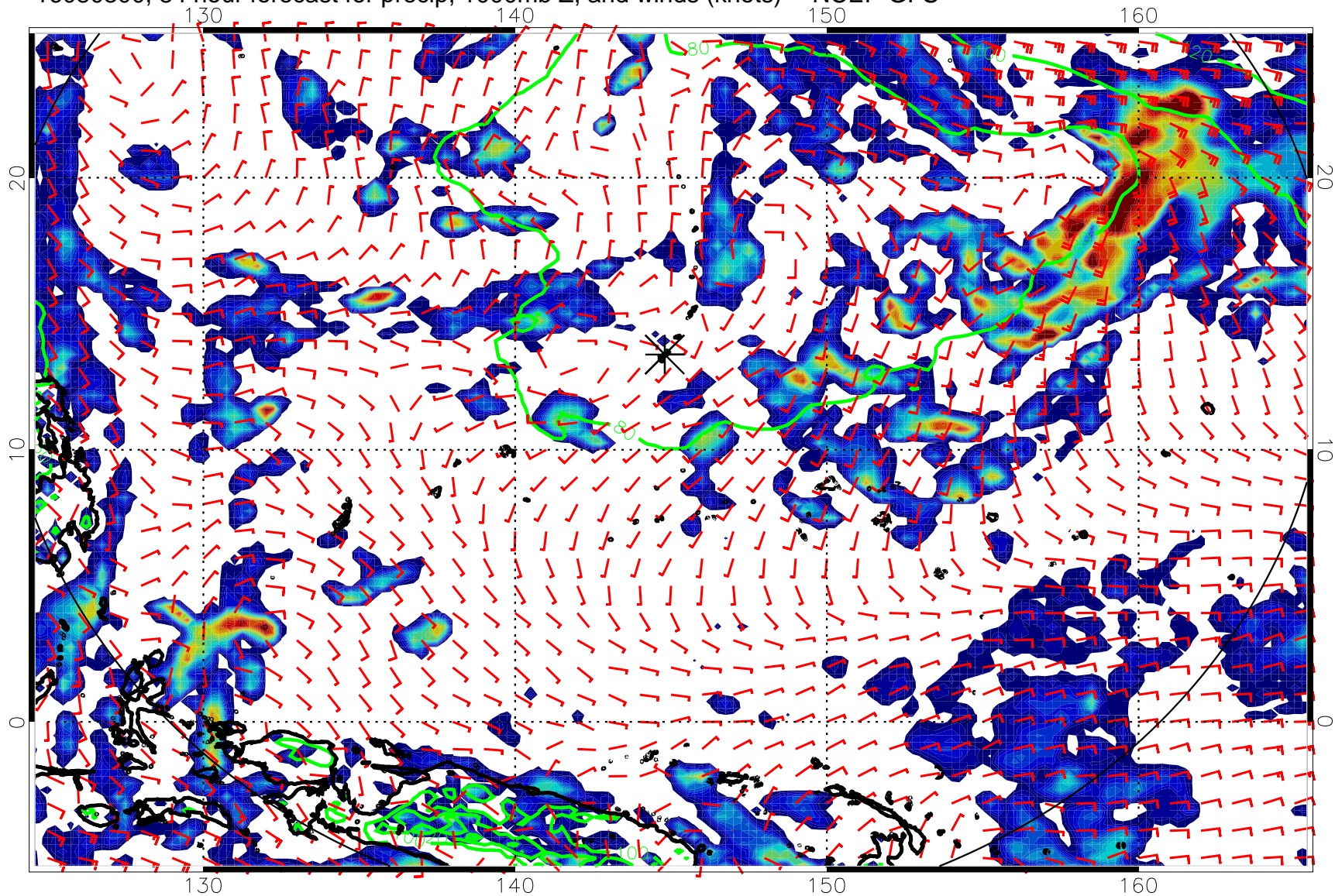
16080300, 84 hour forecast for precip, 1000mb Z, and winds (knots) -- NCEP GFS
