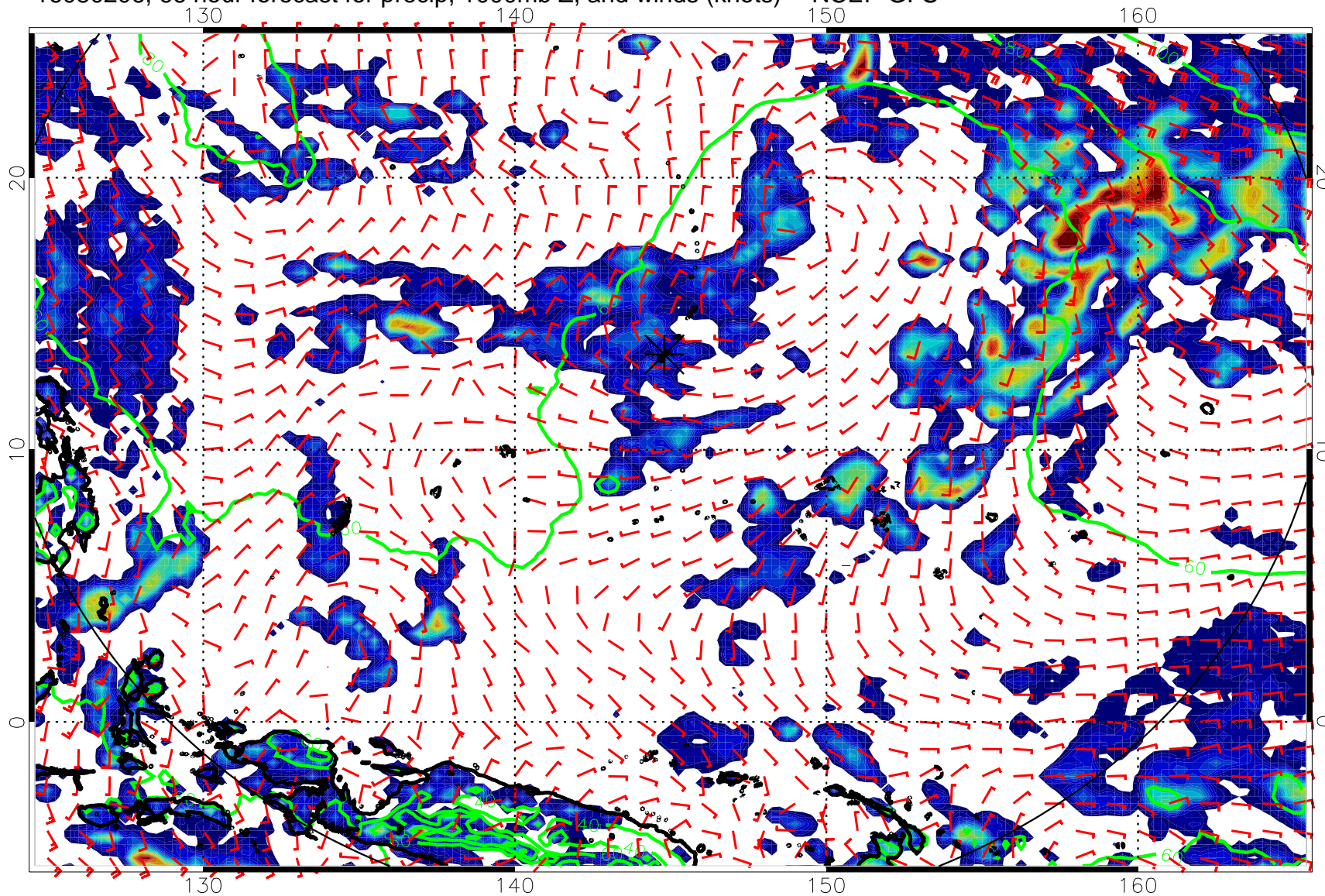
16080206, 66 hour forecast for precip, 1000mb Z, and winds (knots) -- NCEP GFS
