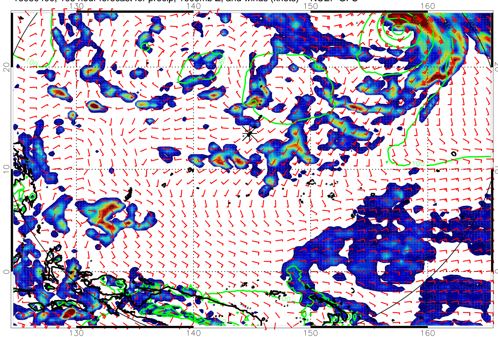
16080400, 108 hour forecast for precip, 1000mb Z, and winds (knots) -- NCEP GFS
