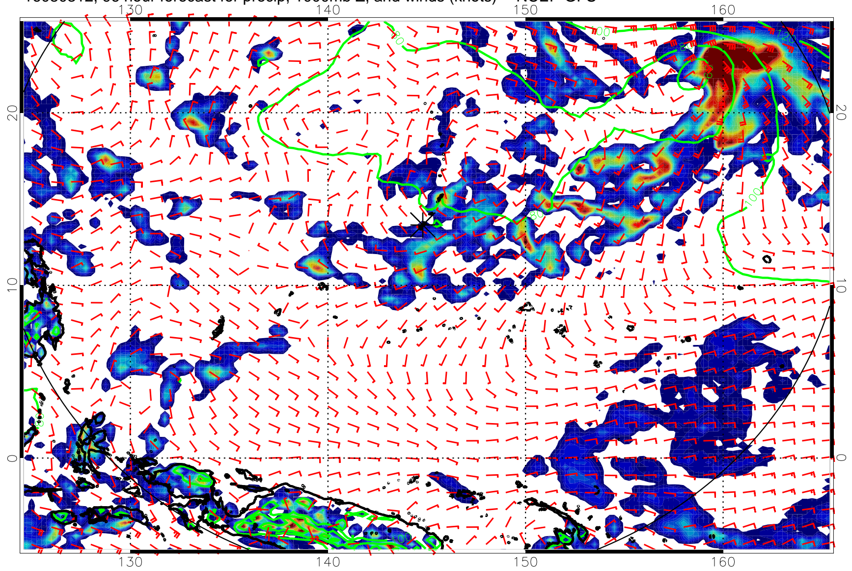
16080312, 96 hour forecast for precip, 1000mb Z, and winds (knots) -- NCEP GFS
