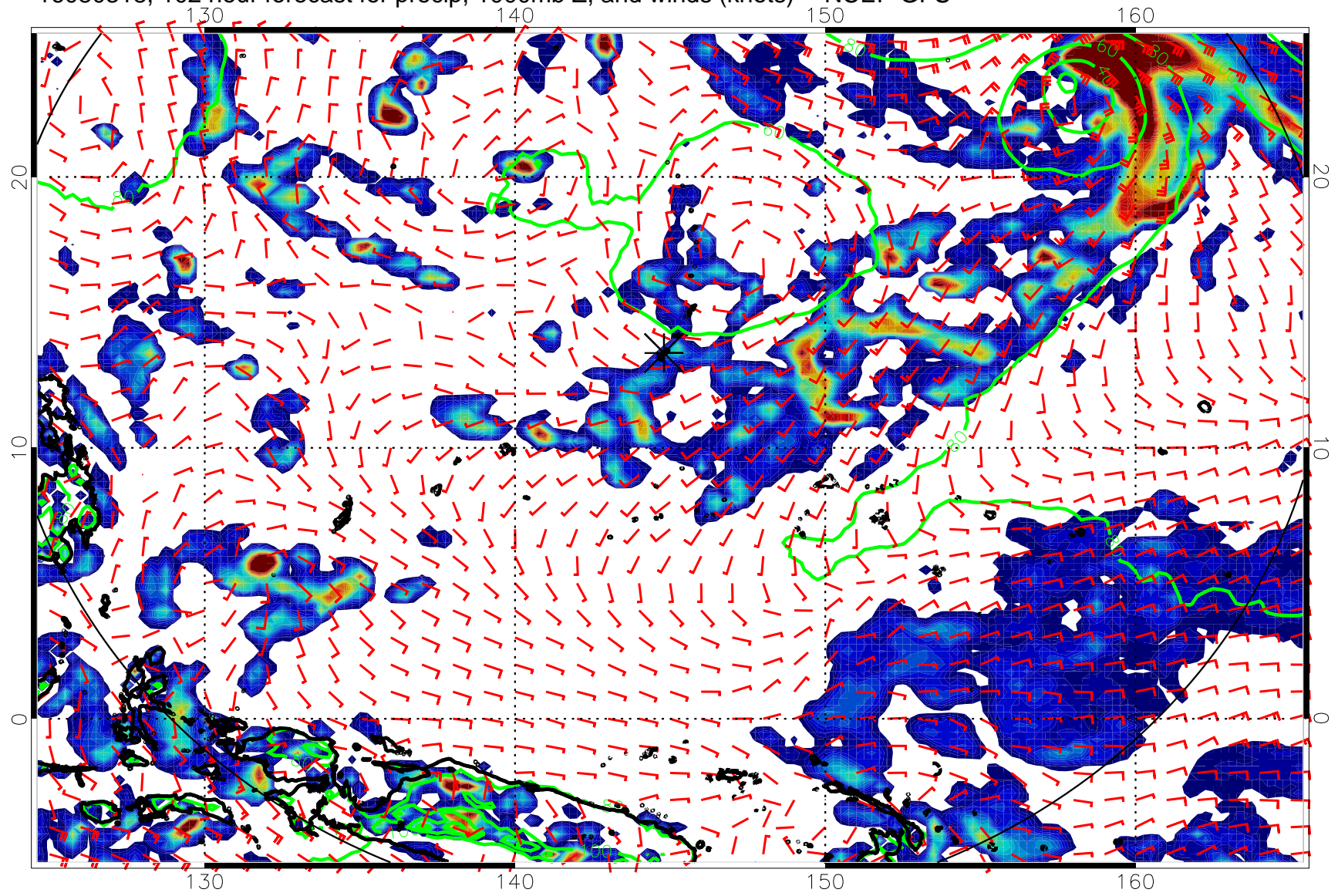
16080318, 102 hour forecast for precip, 1000mb Z, and winds (knots) -- NCEP GFS
