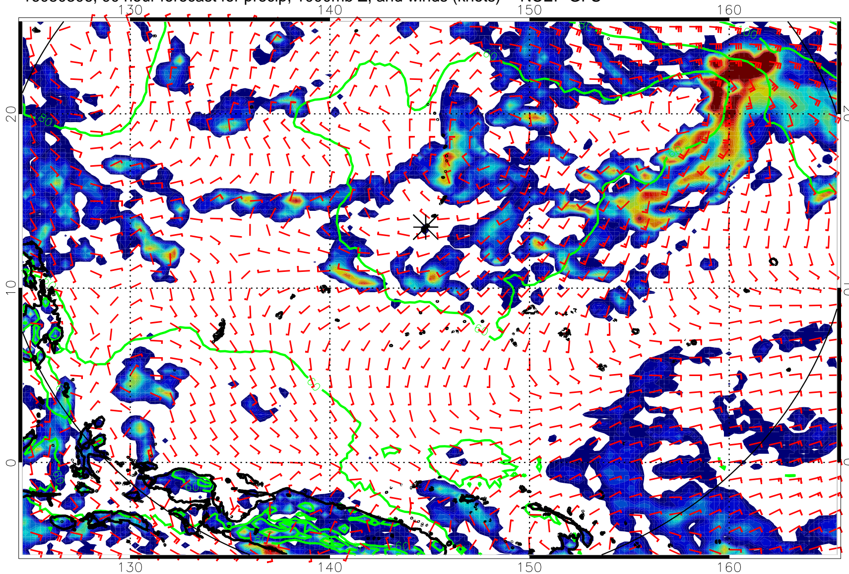
16080306, 90 hour forecast for precip, 1000mb Z, and winds (knots) -- NCEP GFS
