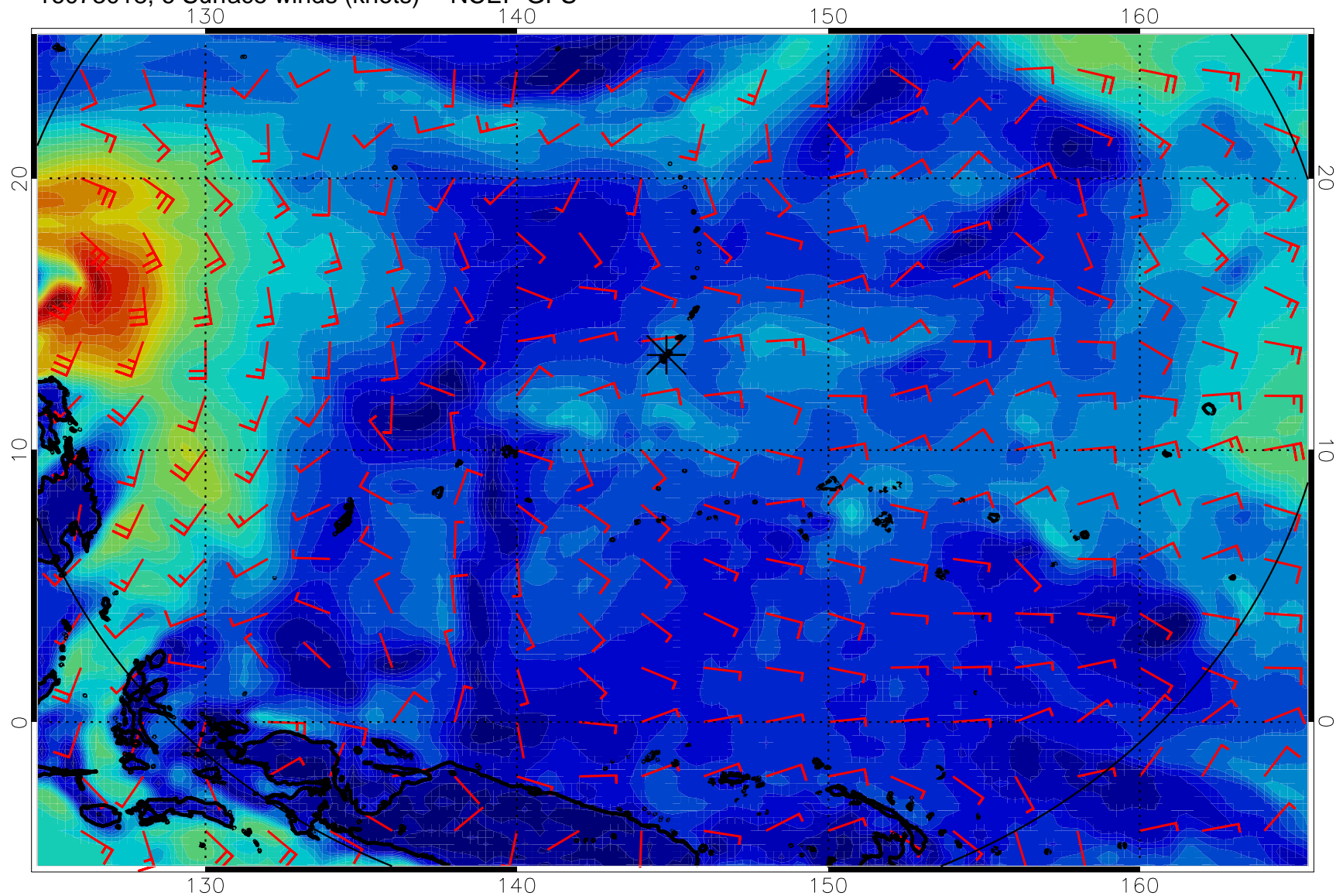
16073018, 6 Surface winds (knots) -- NCEP GFS
