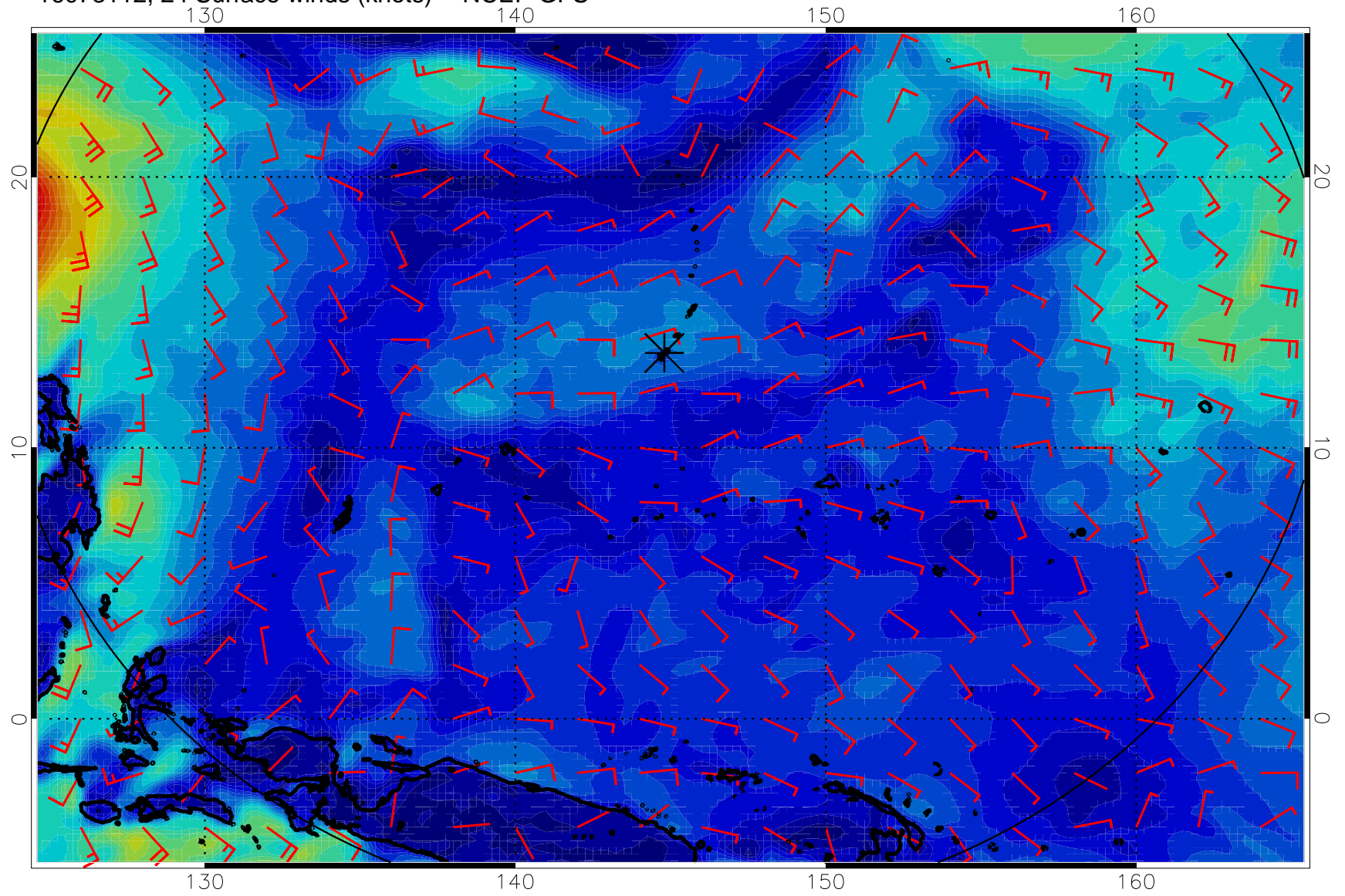
16073112, 24 Surface winds (knots) -- NCEP GFS
