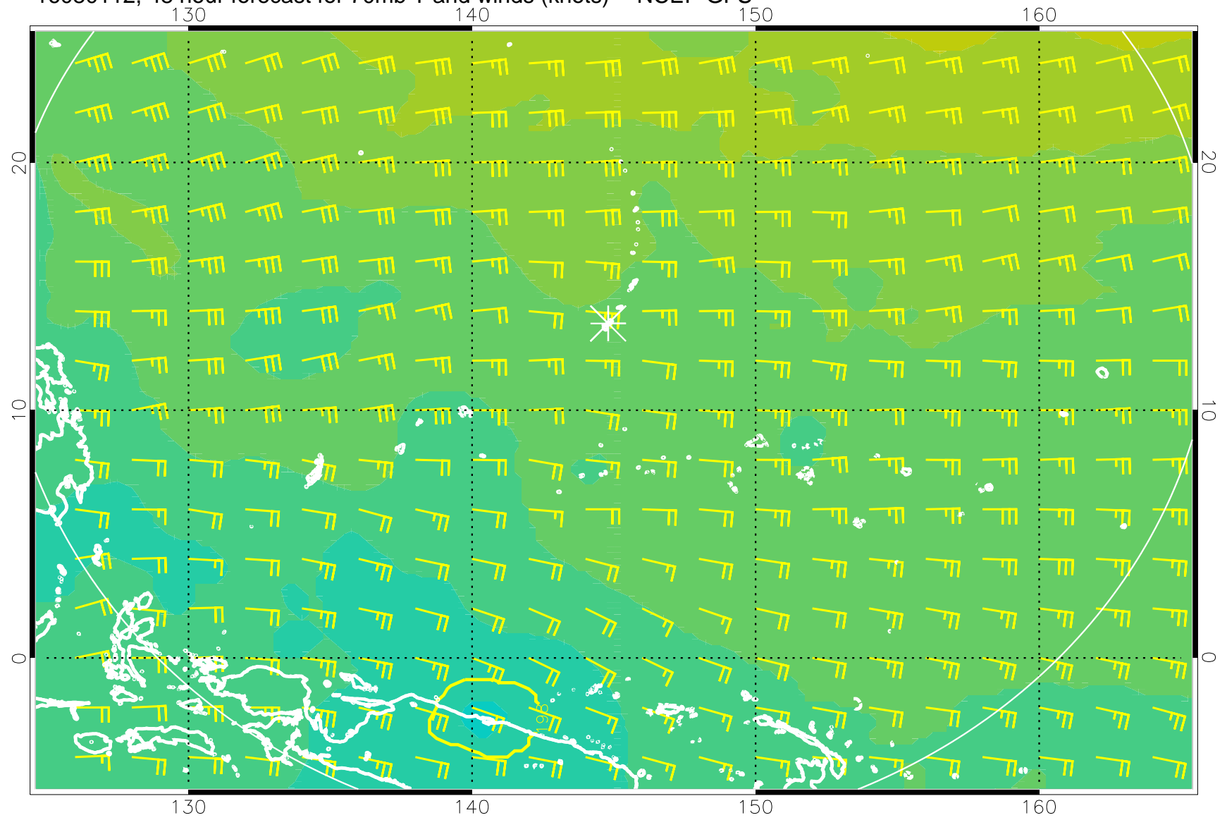
16080112, 48 hour forecast for 70mb T and winds (knots) -- NCEP GFS
