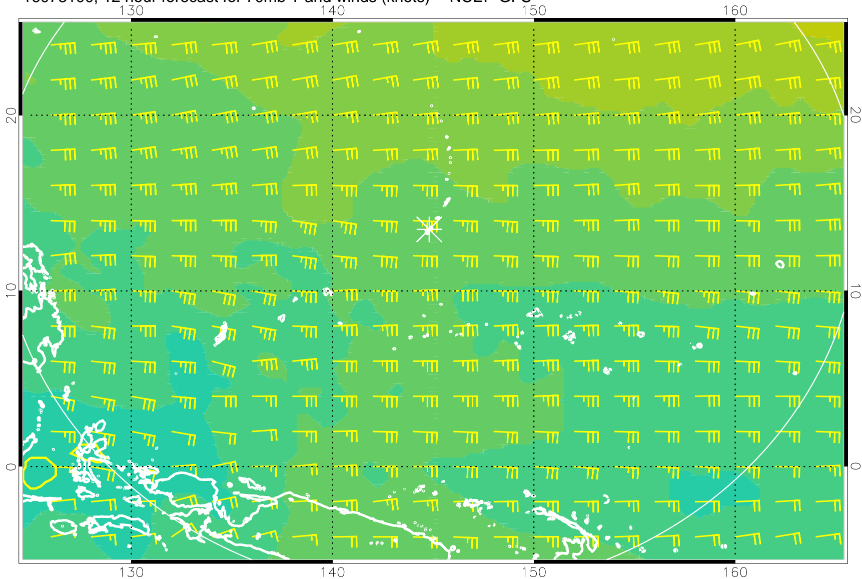
16073100, 12 hour forecast for 70mb T and winds (knots) -- NCEP GFS
