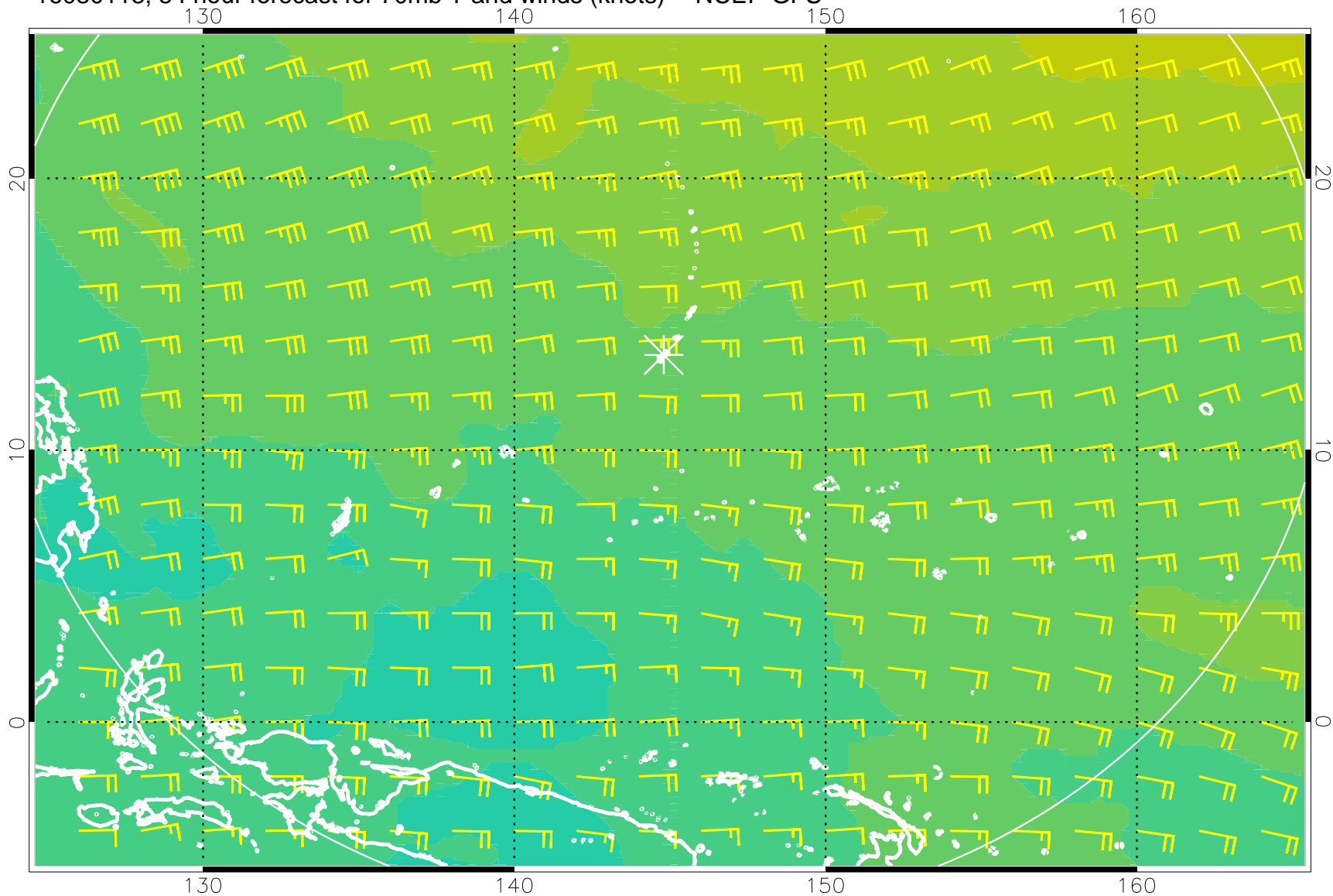
16080118, 54 hour forecast for 70mb T and winds (knots) -- NCEP GFS
