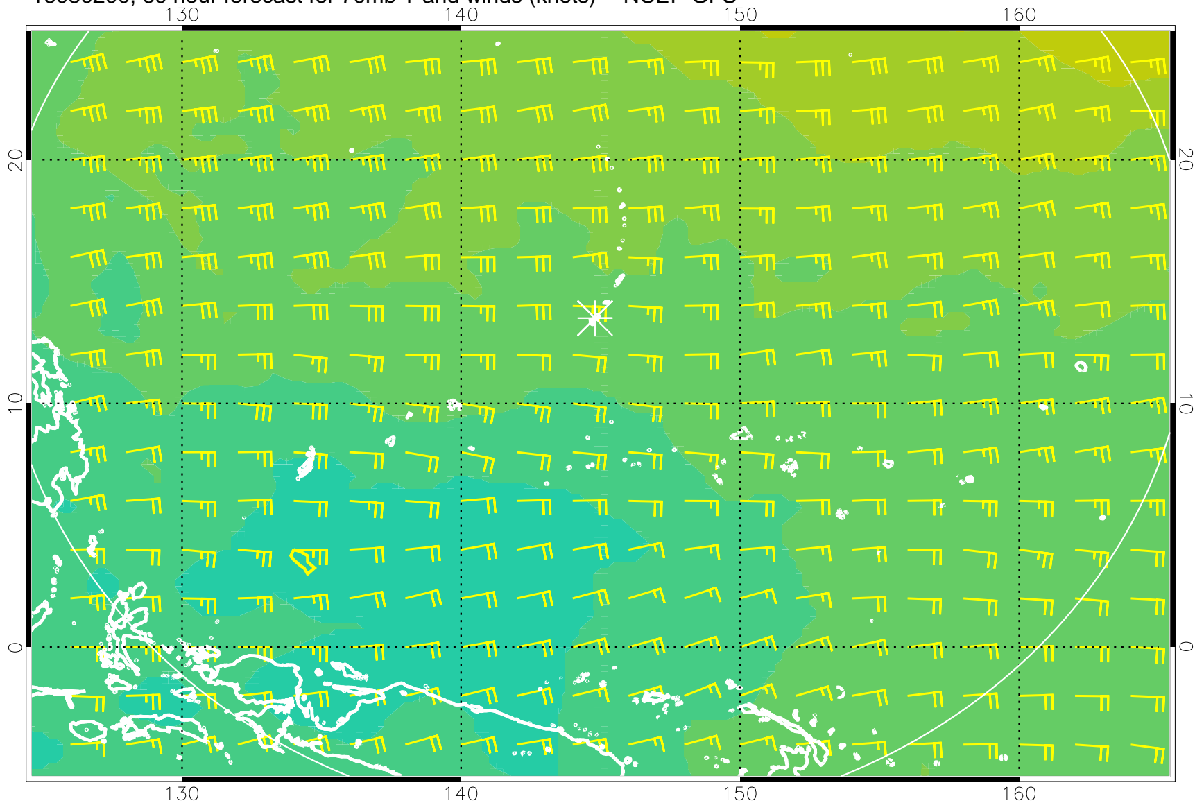
16080200, 60 hour forecast for 70mb T and winds (knots) -- NCEP GFS
