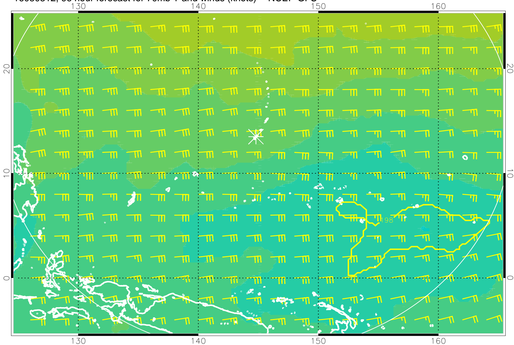
16080312, 96 hour forecast for 70mb T and winds (knots) -- NCEP GFS
