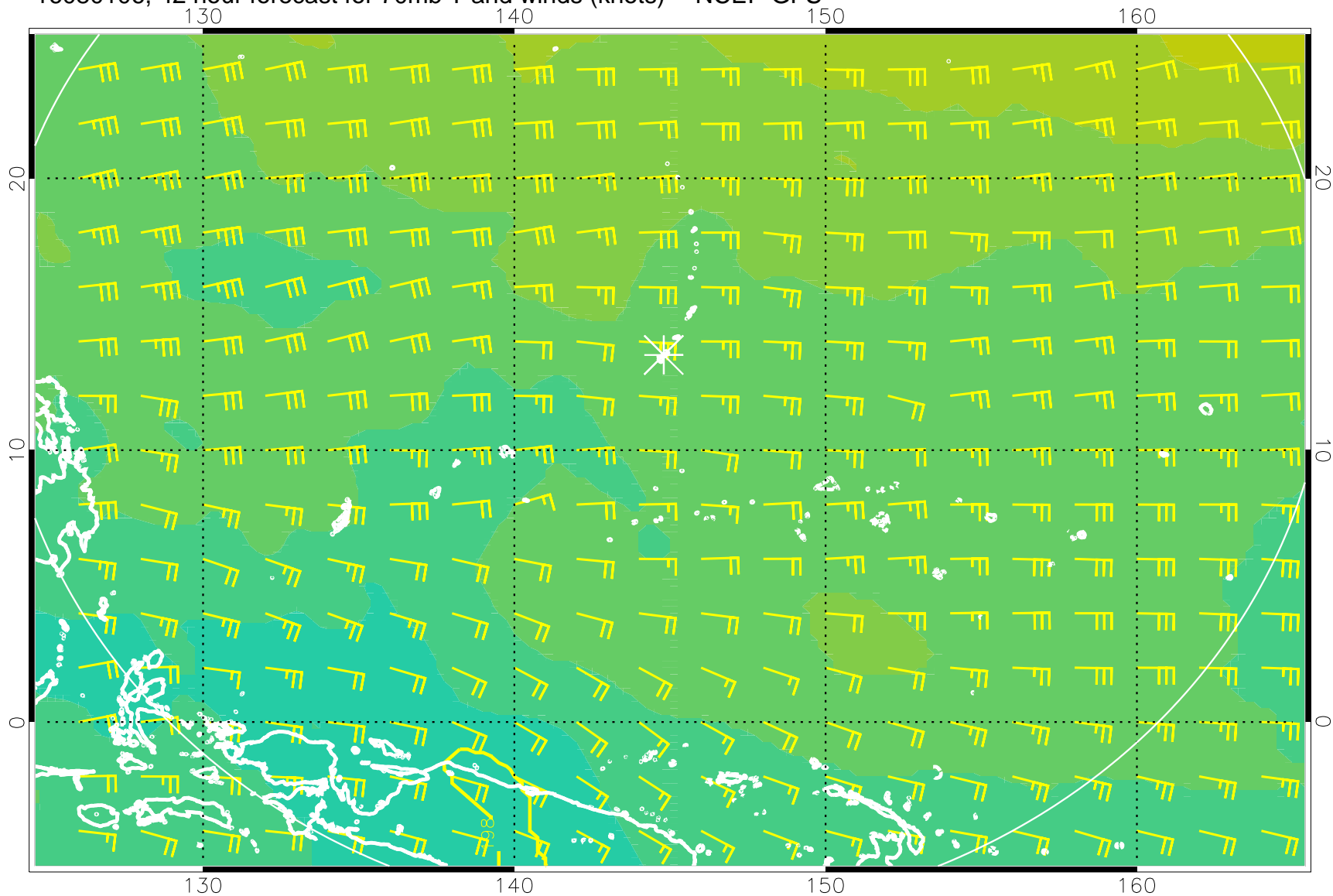
16080106, 42 hour forecast for 70mb T and winds (knots) -- NCEP GFS
