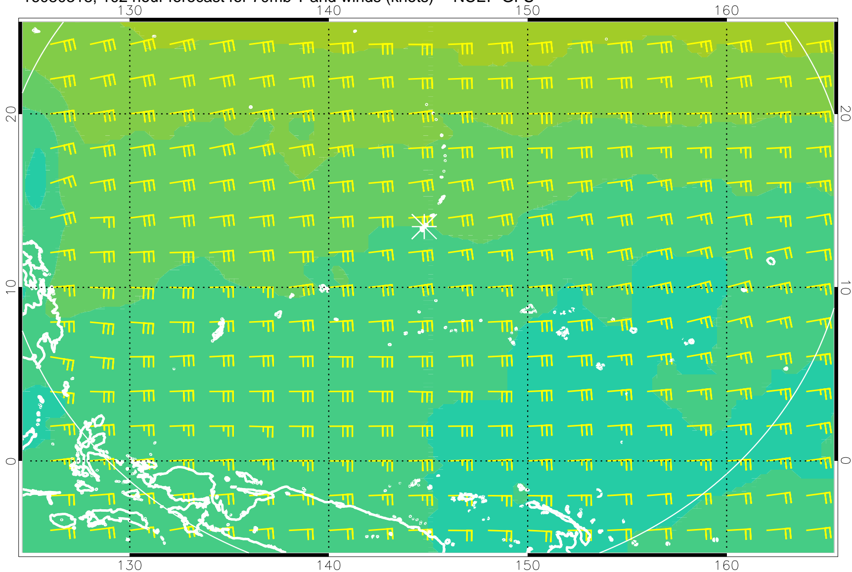
16080318, 102 hour forecast for 70mb T and winds (knots) -- NCEP GFS
