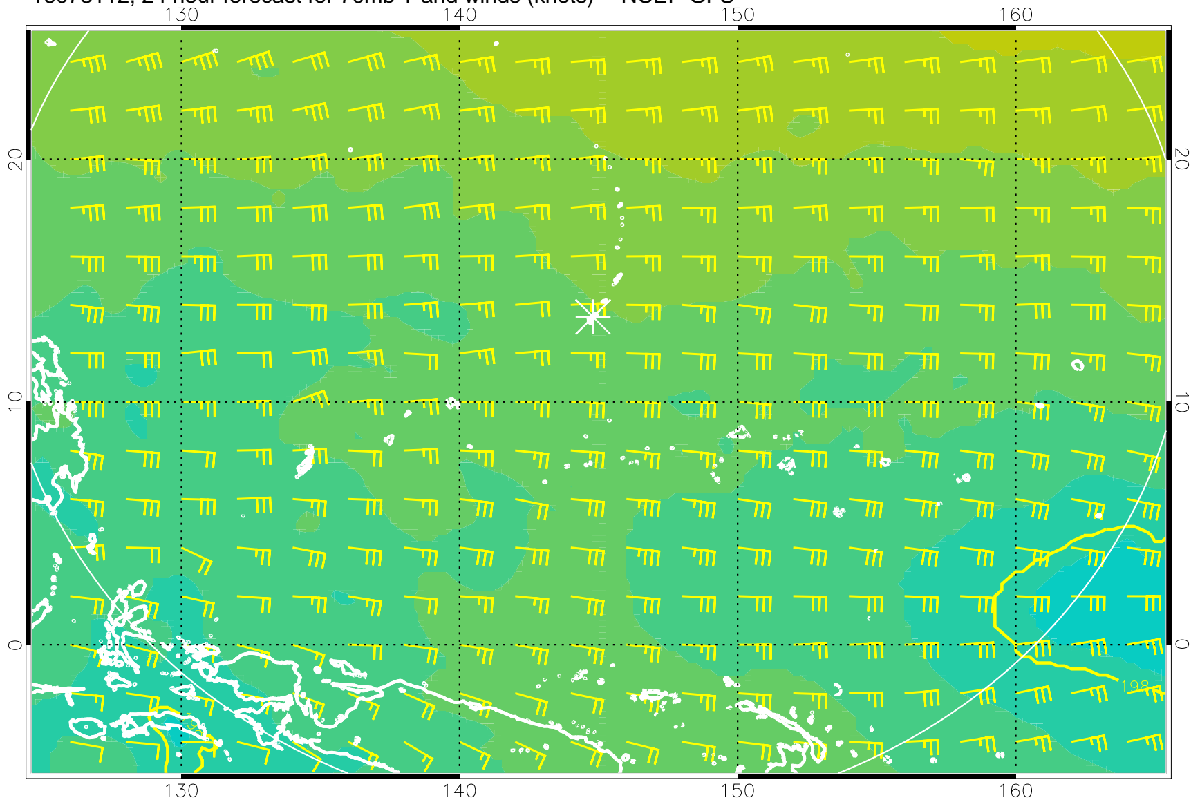
16073112, 24 hour forecast for 70mb T and winds (knots) -- NCEP GFS
