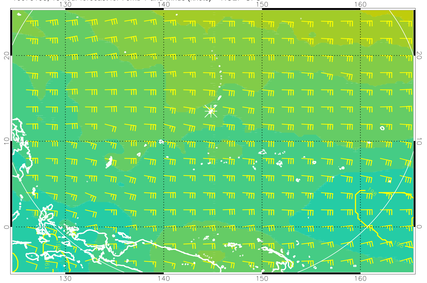
16073106, 18 hour forecast for 70mb T and winds (knots) -- NCEP GFS
