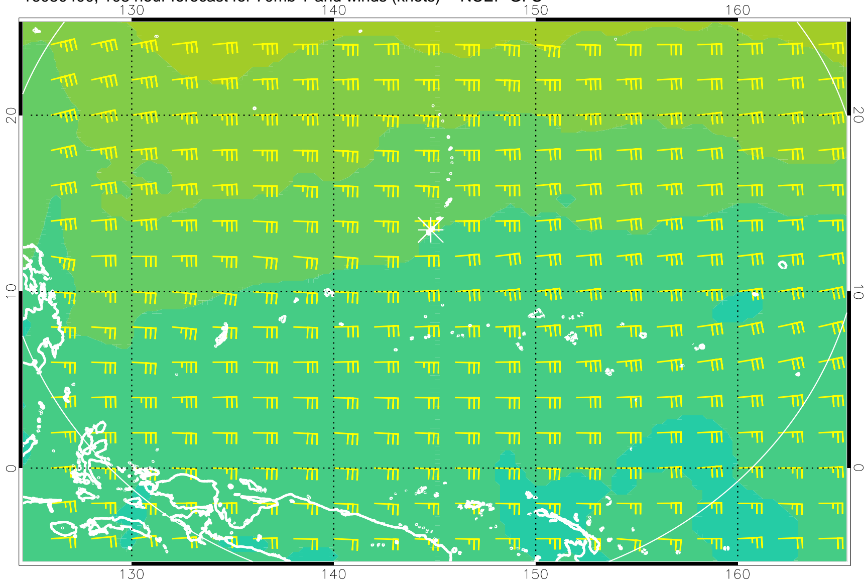
16080400, 108 hour forecast for 70mb T and winds (knots) -- NCEP GFS
