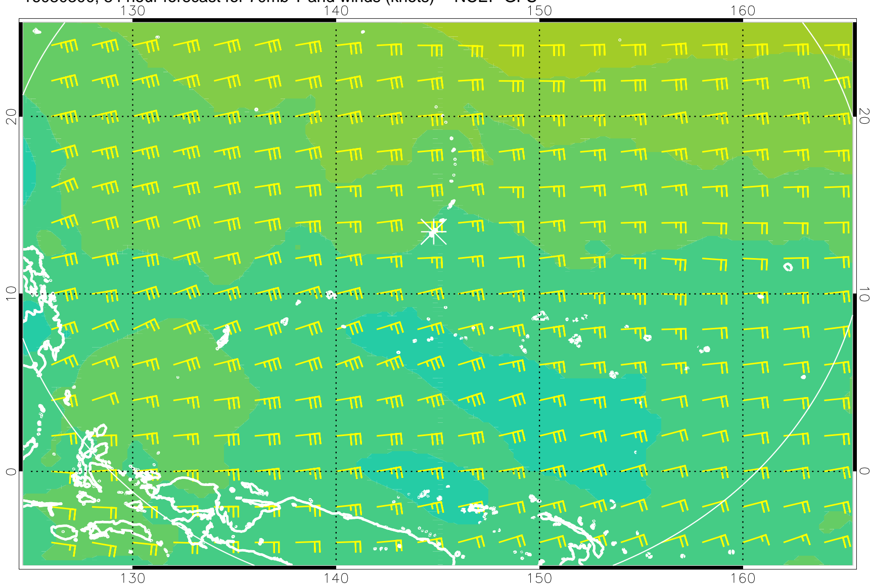
16080300, 84 hour forecast for 70mb T and winds (knots) -- NCEP GFS
