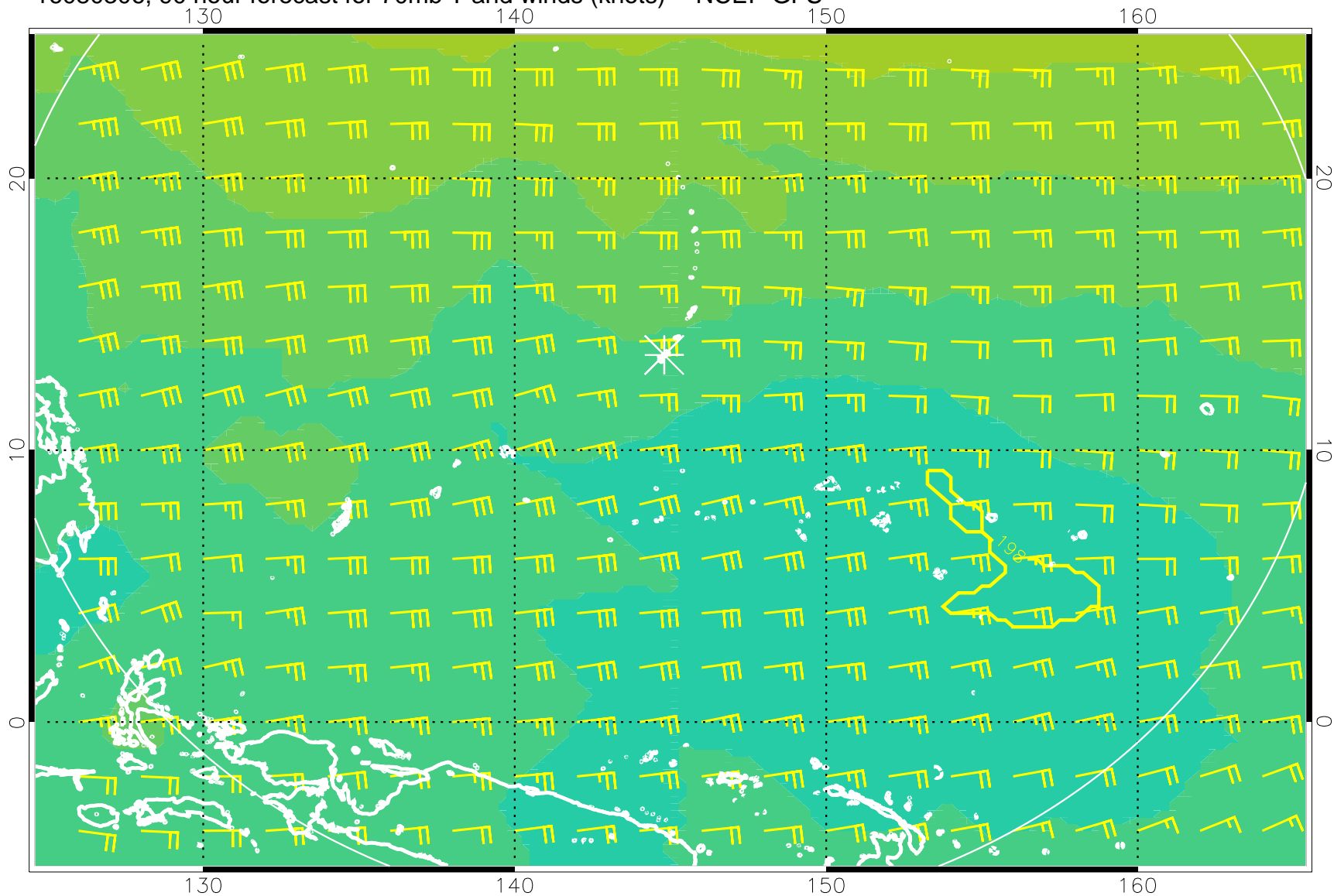
16080306, 90 hour forecast for 70mb T and winds (knots) -- NCEP GFS
