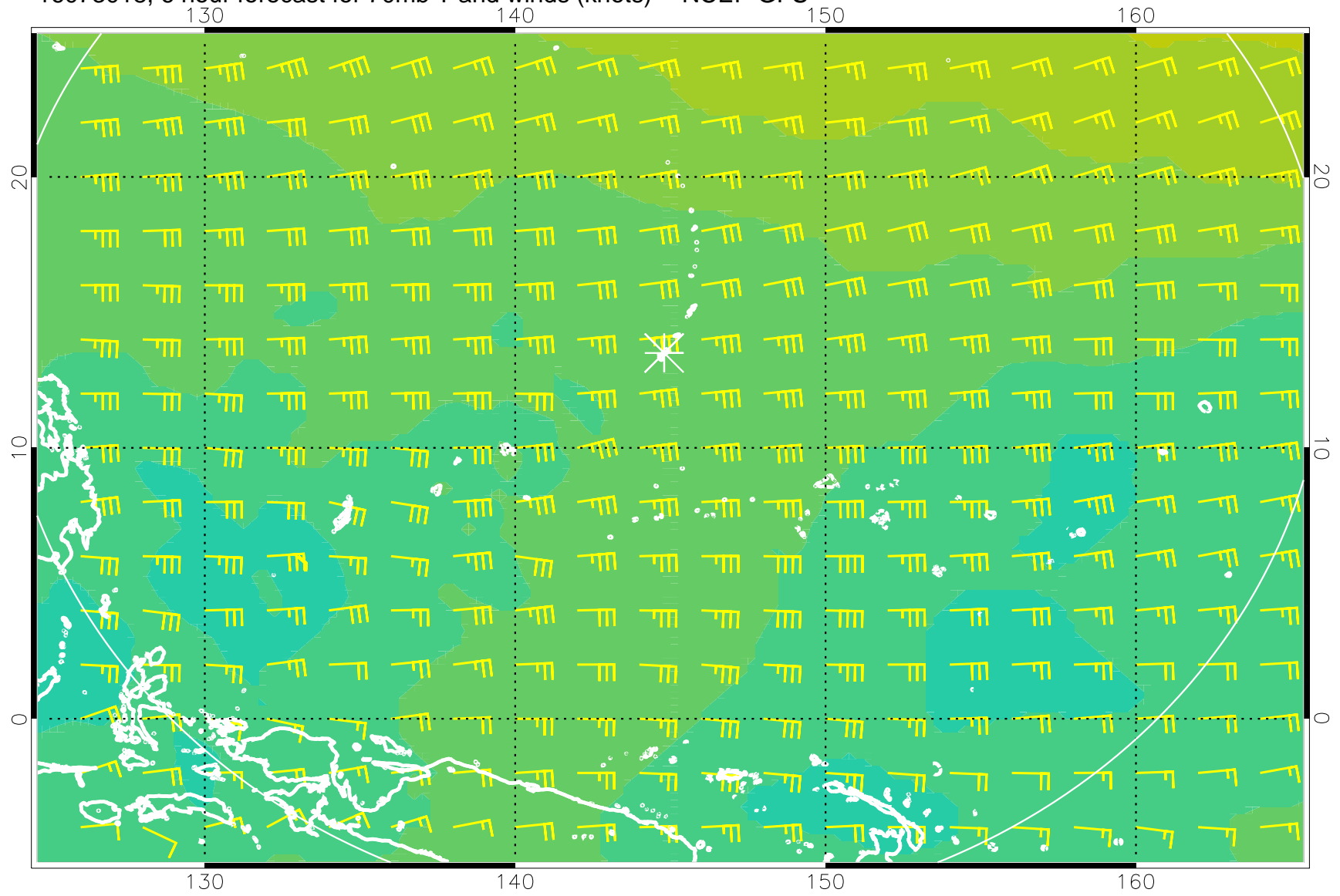
16073018, 6 hour forecast for 70mb T and winds (knots) -- NCEP GFS
