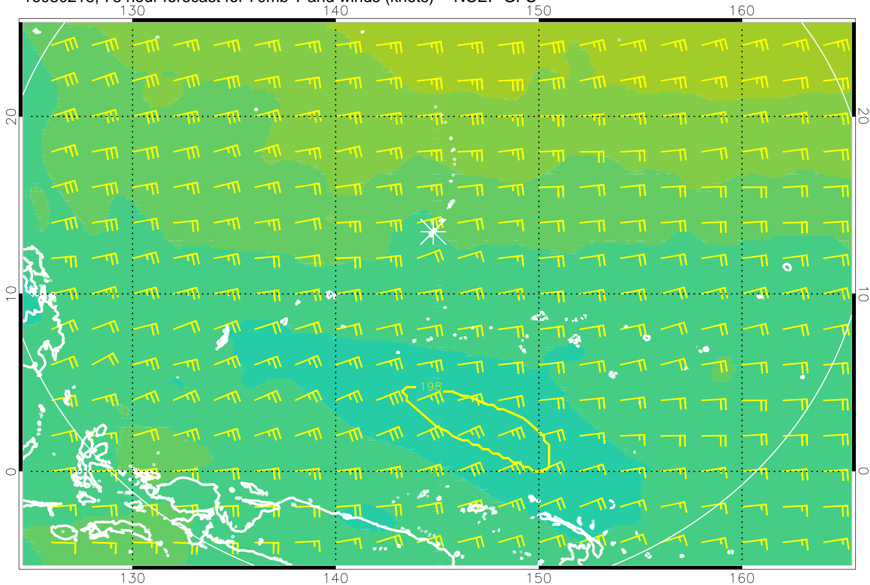
16080218, 78 hour forecast for 70mb T and winds (knots) -- NCEP GFS
