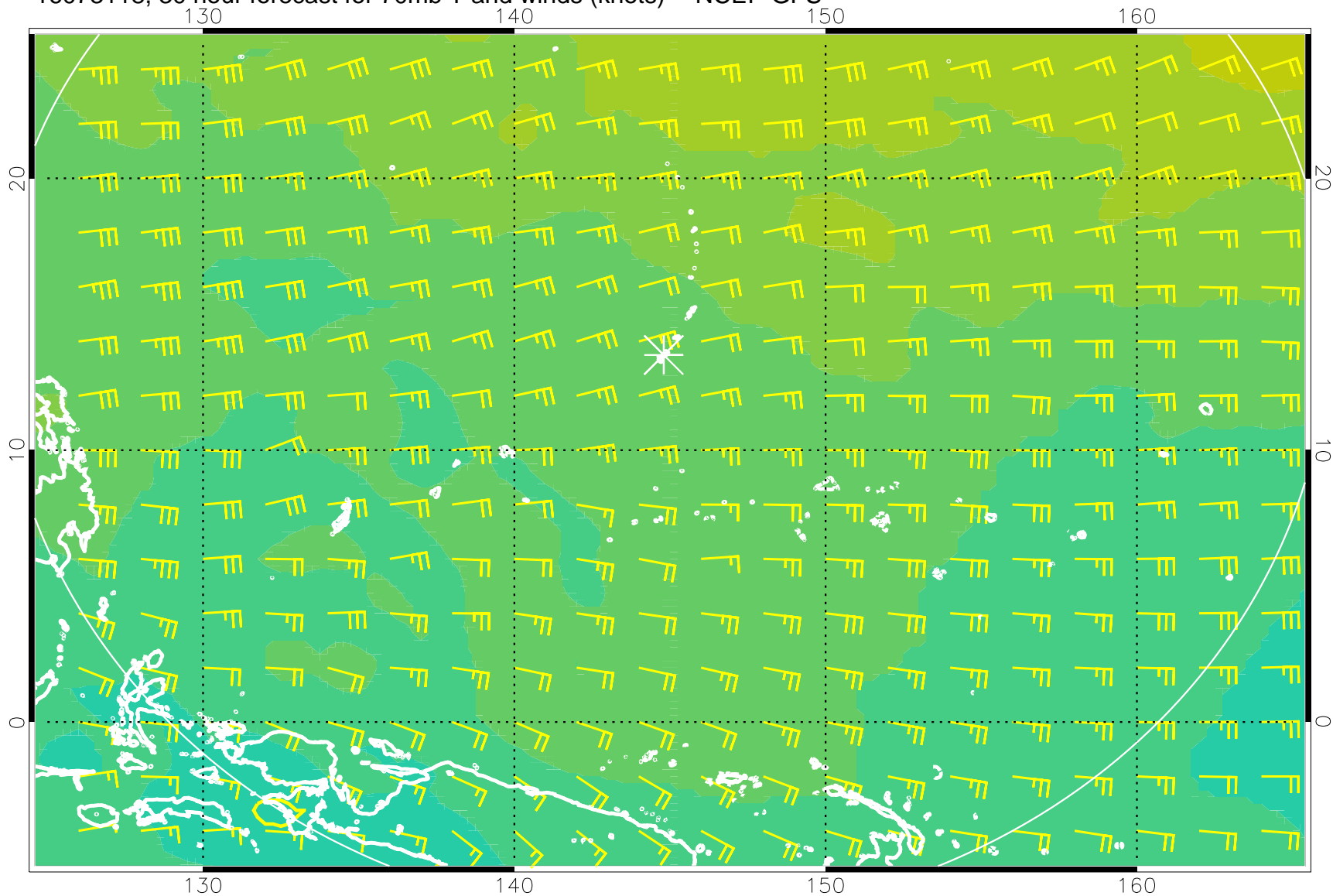
16073118, 30 hour forecast for 70mb T and winds (knots) -- NCEP GFS
