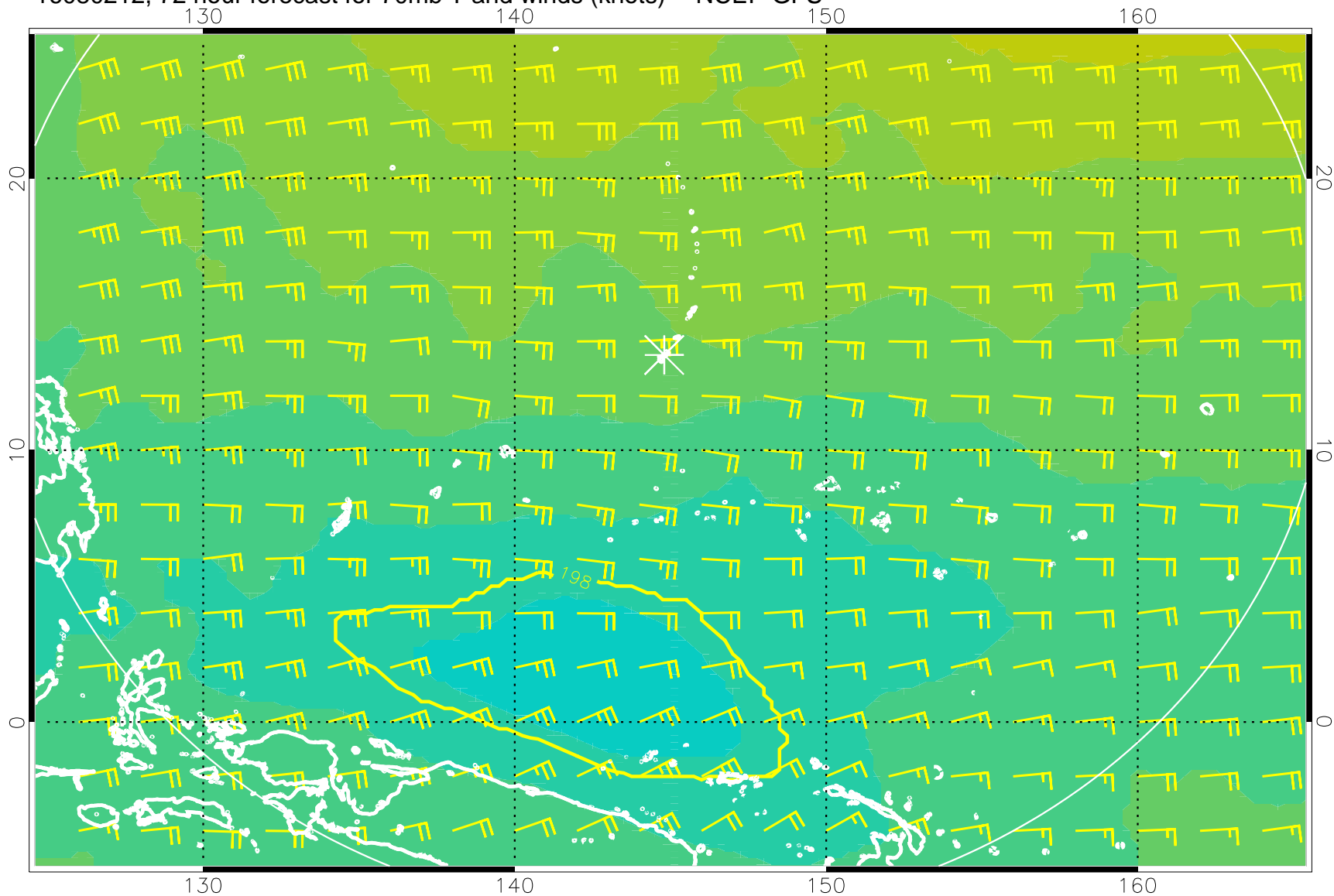
16080212, 72 hour forecast for 70mb T and winds (knots) -- NCEP GFS
