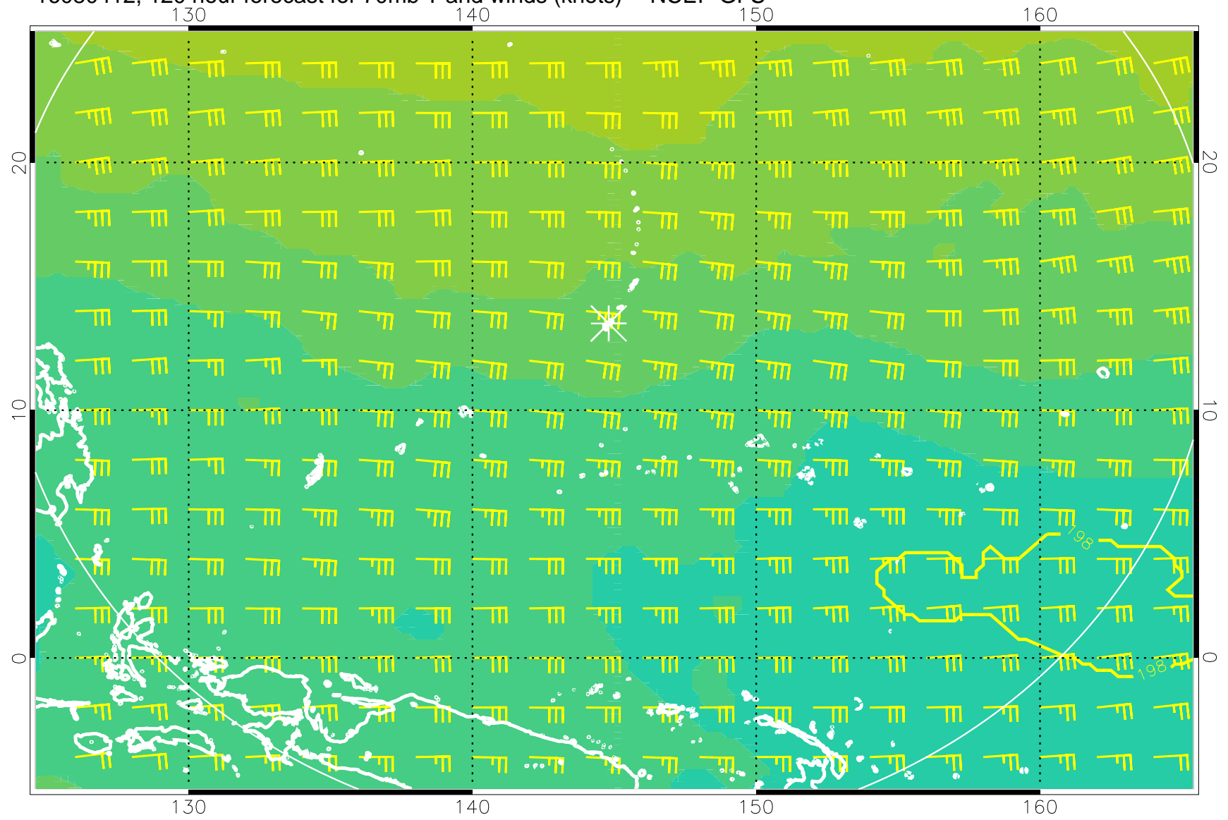
16080412, 120 hour forecast for 70mb T and winds (knots) -- NCEP GFS
