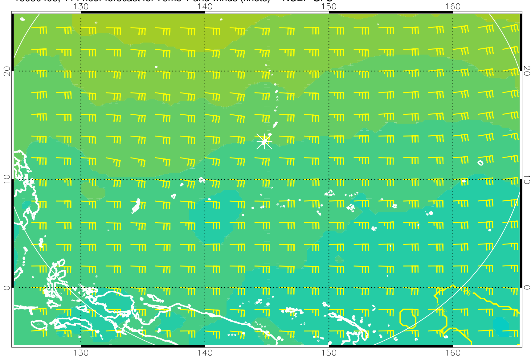
16080406, 114 hour forecast for 70mb T and winds (knots) -- NCEP GFS
