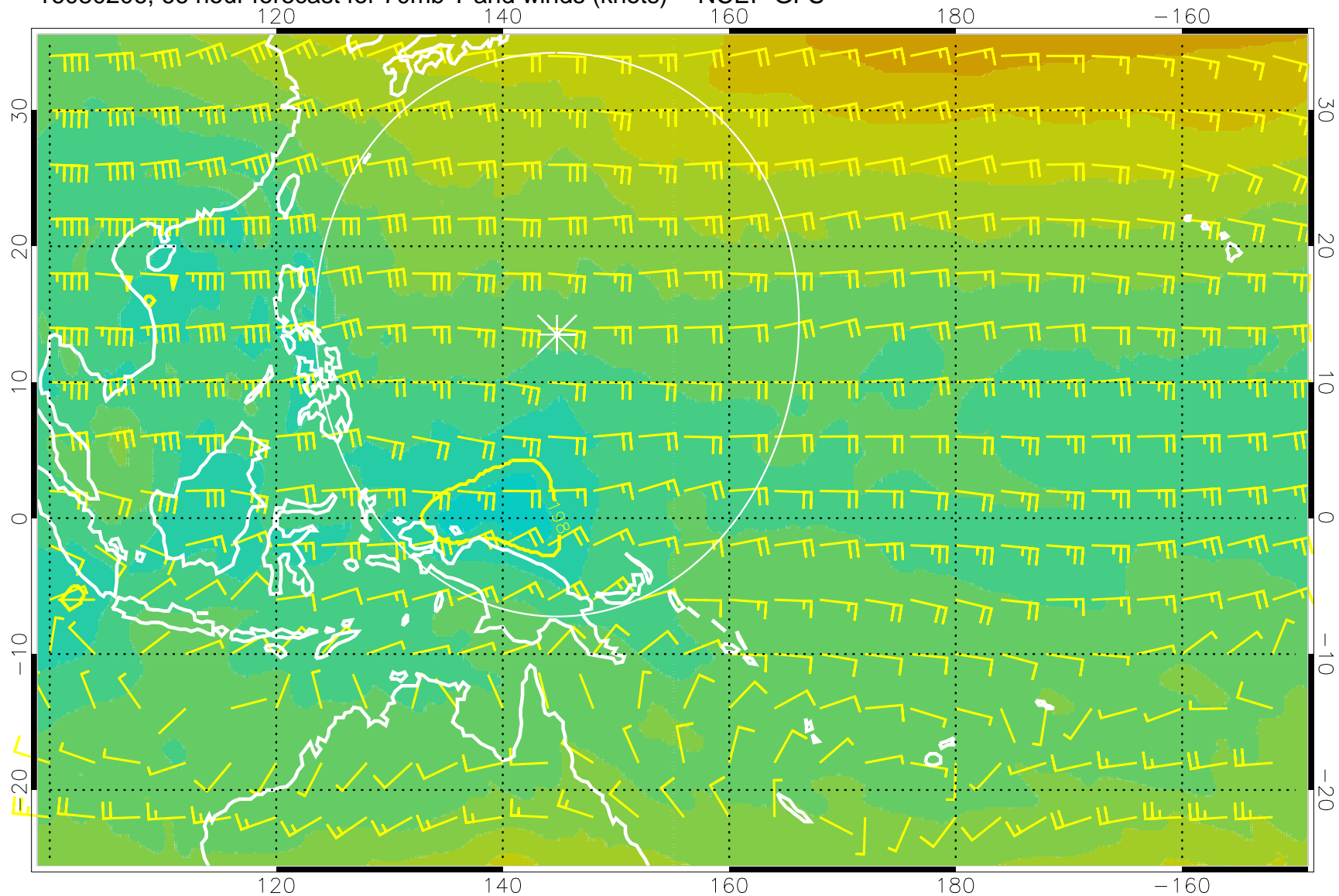
16080206, 66 hour forecast for 70mb T and winds (knots) -- NCEP GFS
