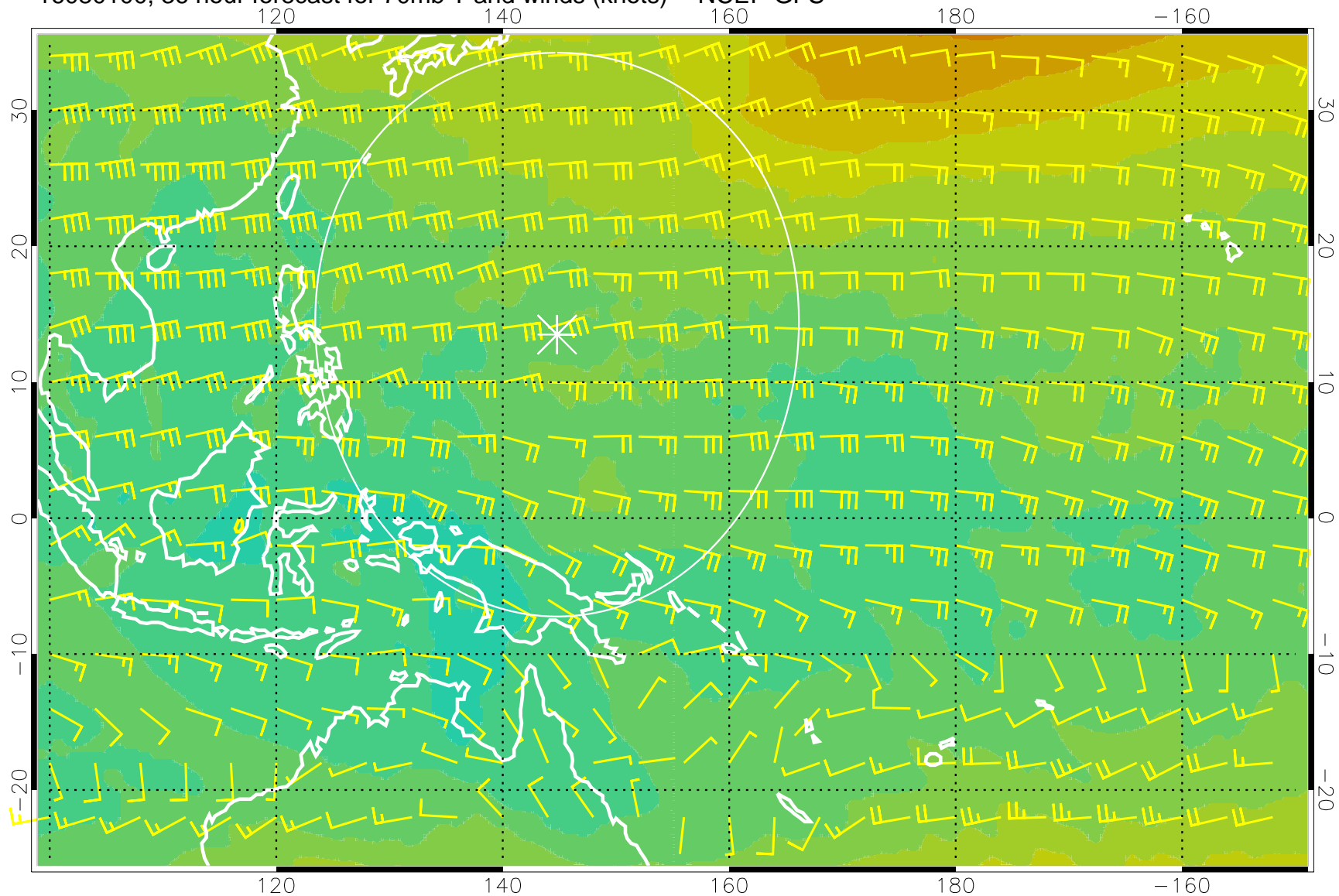
16080100, 36 hour forecast for 70mb T and winds (knots) -- NCEP GFS
