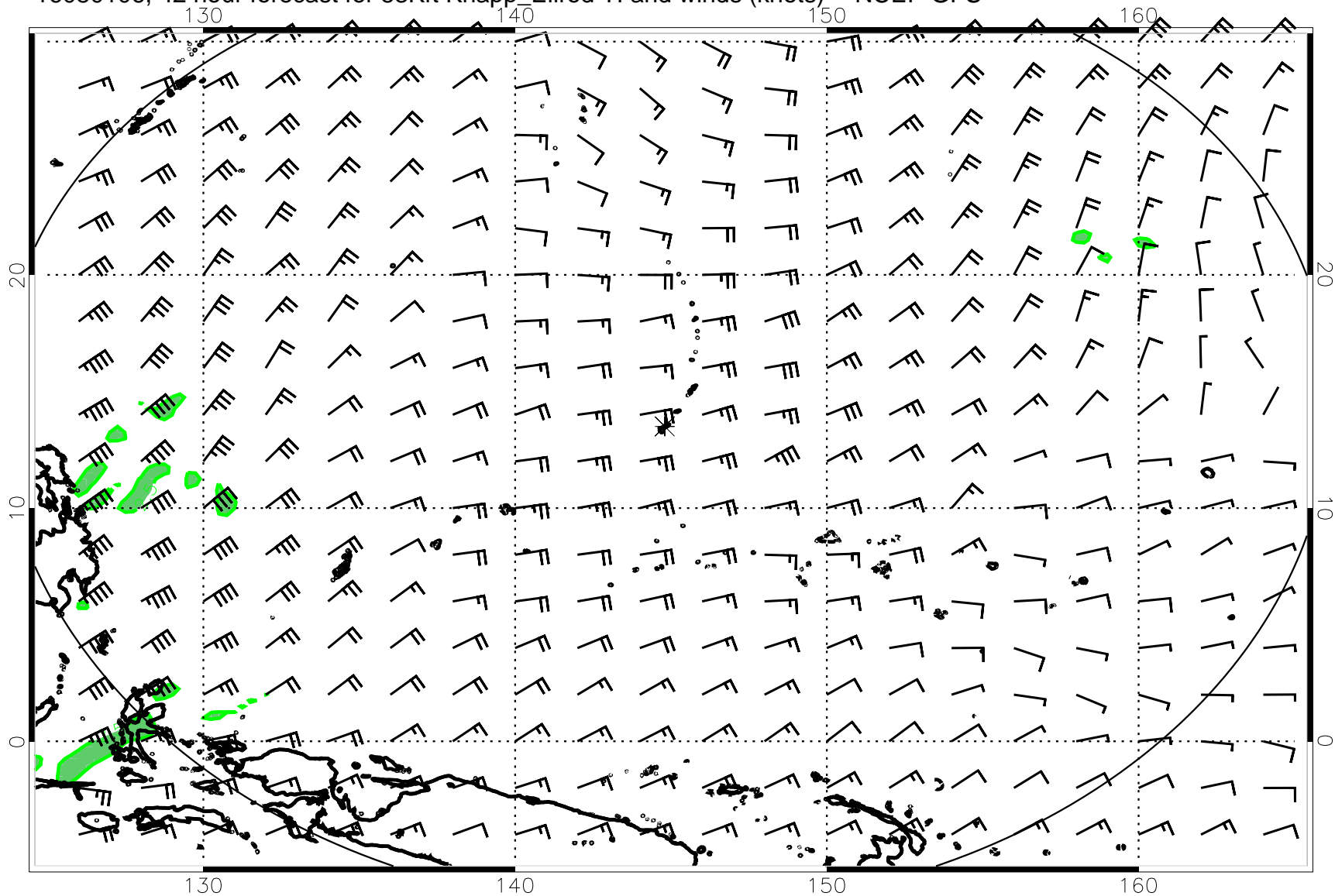
16080106, 42 hour forecast for 53Kft Knapp_Ellrod TI and winds (knots) -- NCEP GFS
