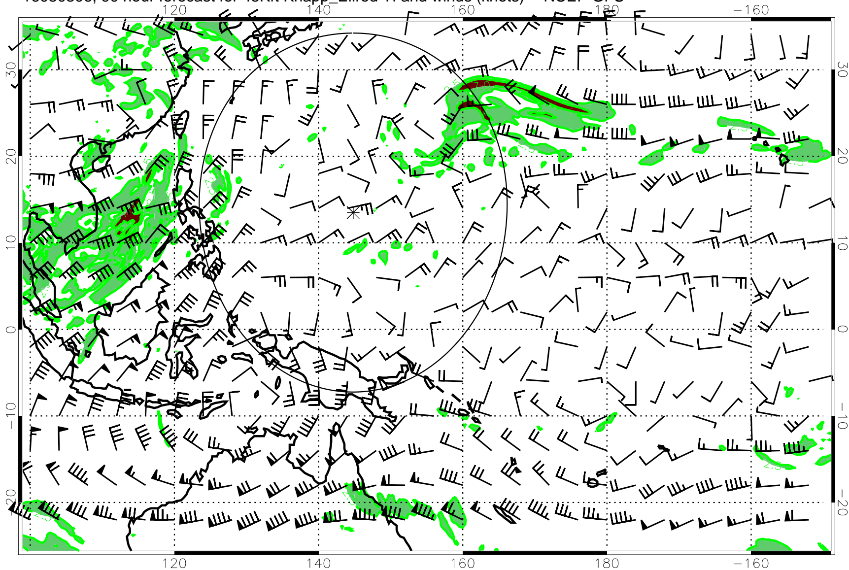
16080306, 90 hour forecast for 45Kft Knapp_Ellrod TI and winds (knots) -- NCEP GFS
