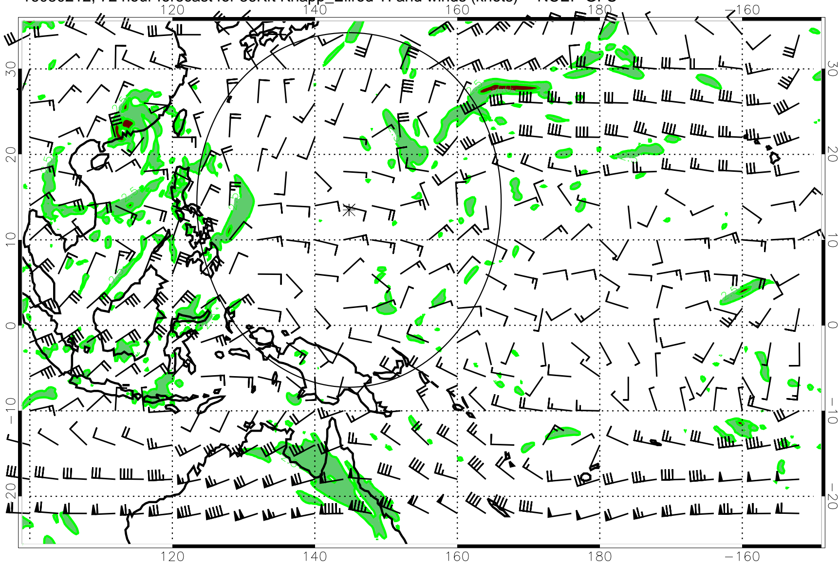
16080212, 72 hour forecast for 36Kft Knapp_Ellrod TI and winds (knots) -- NCEP GFS
