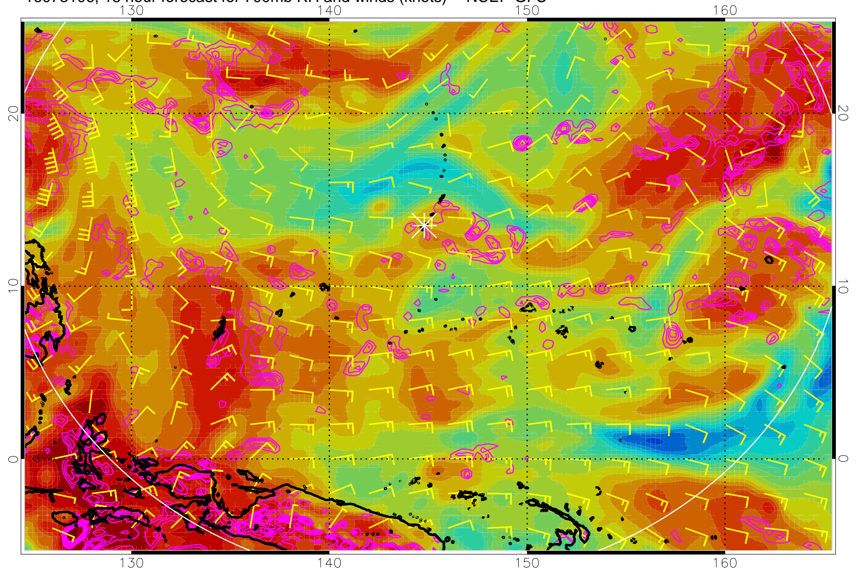
16073106, 18 hour forecast for 700mb RH and winds (knots) -- NCEP GFS
