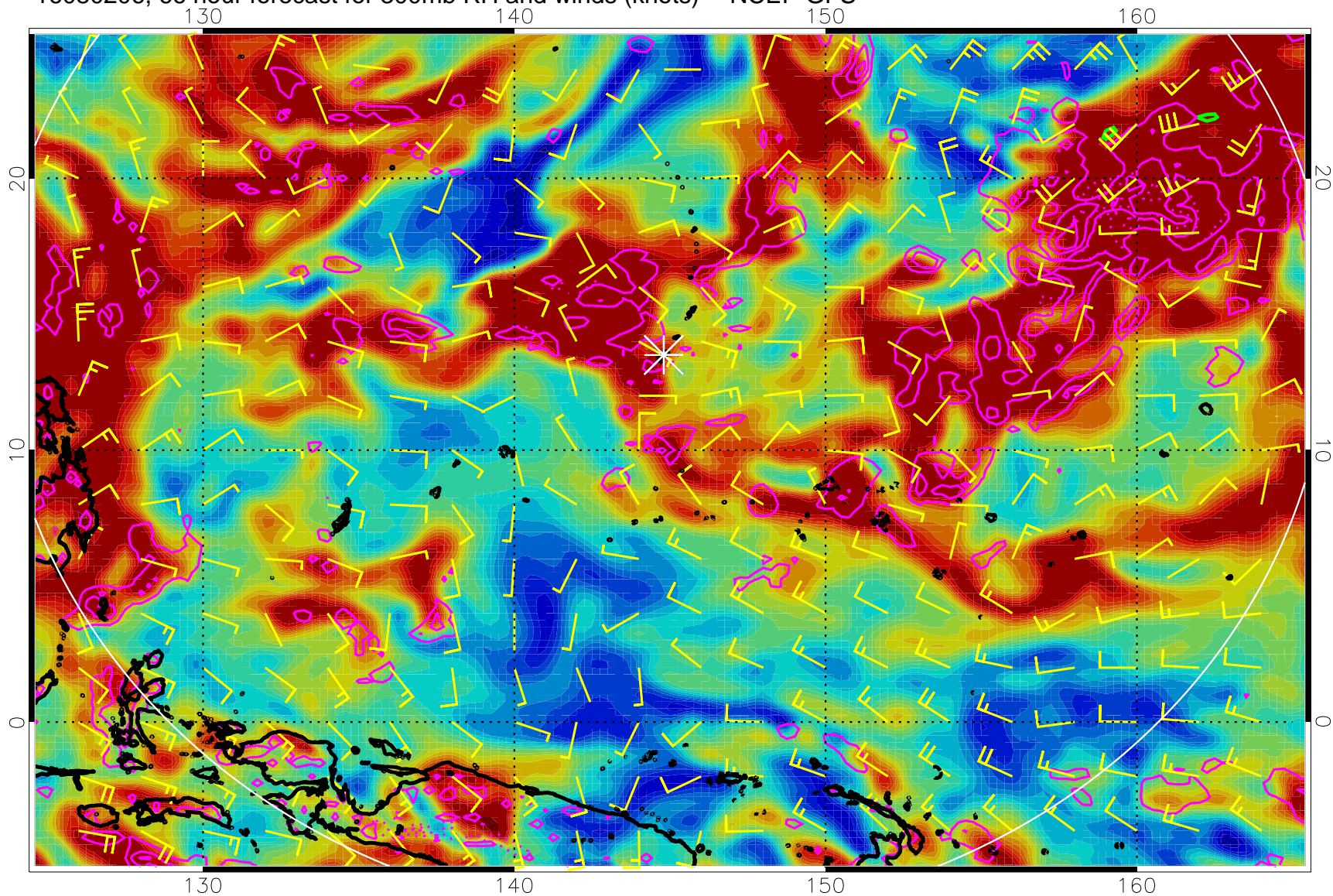
16080206, 66 hour forecast for 300mb RH and winds (knots) -- NCEP GFS
