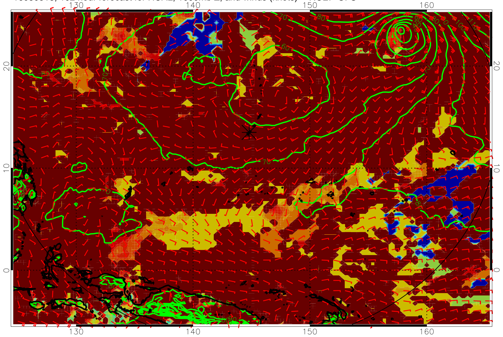
16080318, 102 hour forecast for HCAL, 1000mb Z, and winds (knots) -- NCEP GFS
