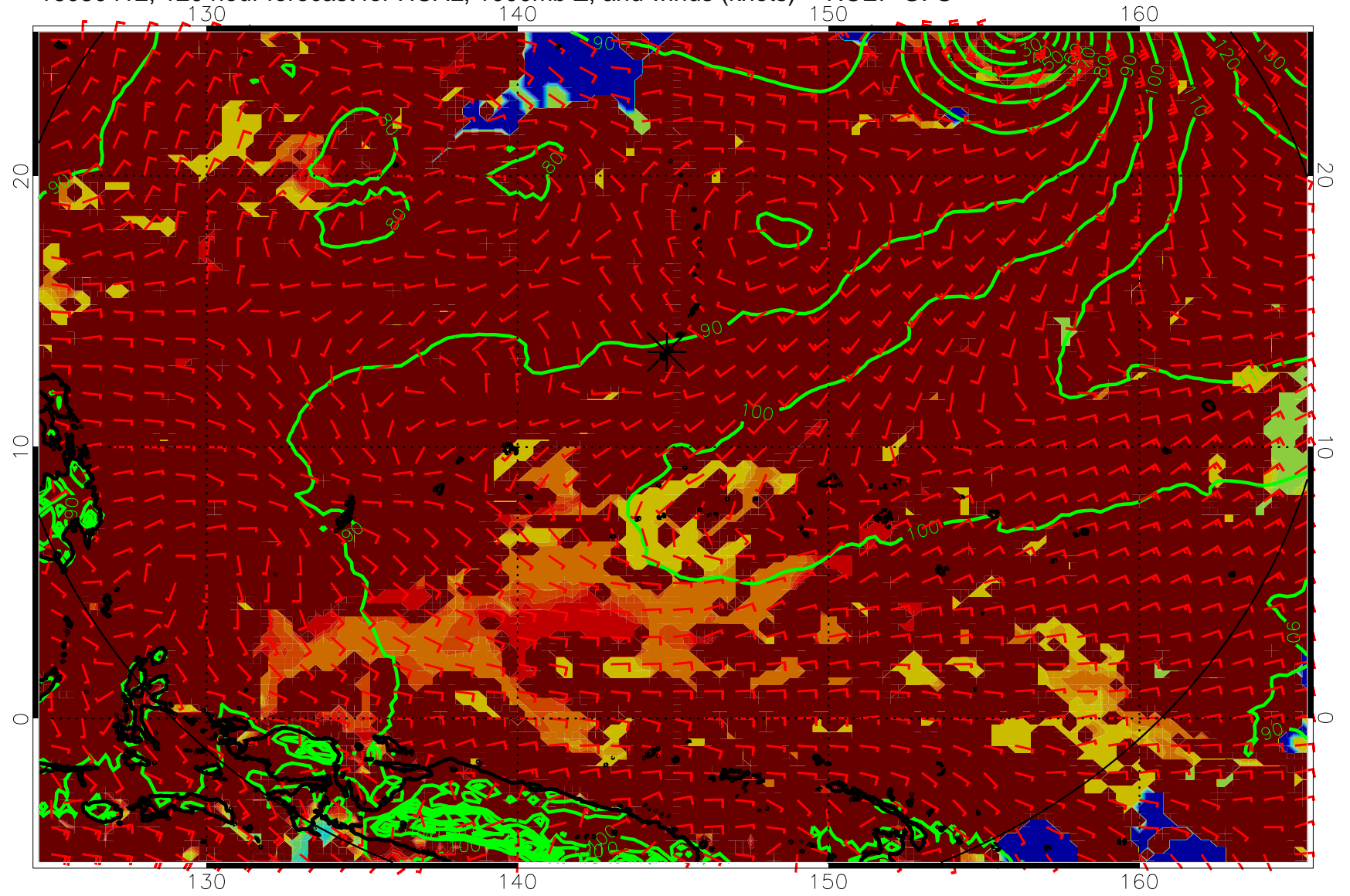
16080412, 120 hour forecast for HCAL, 1000mb Z, and winds (knots) -- NCEP GFS
