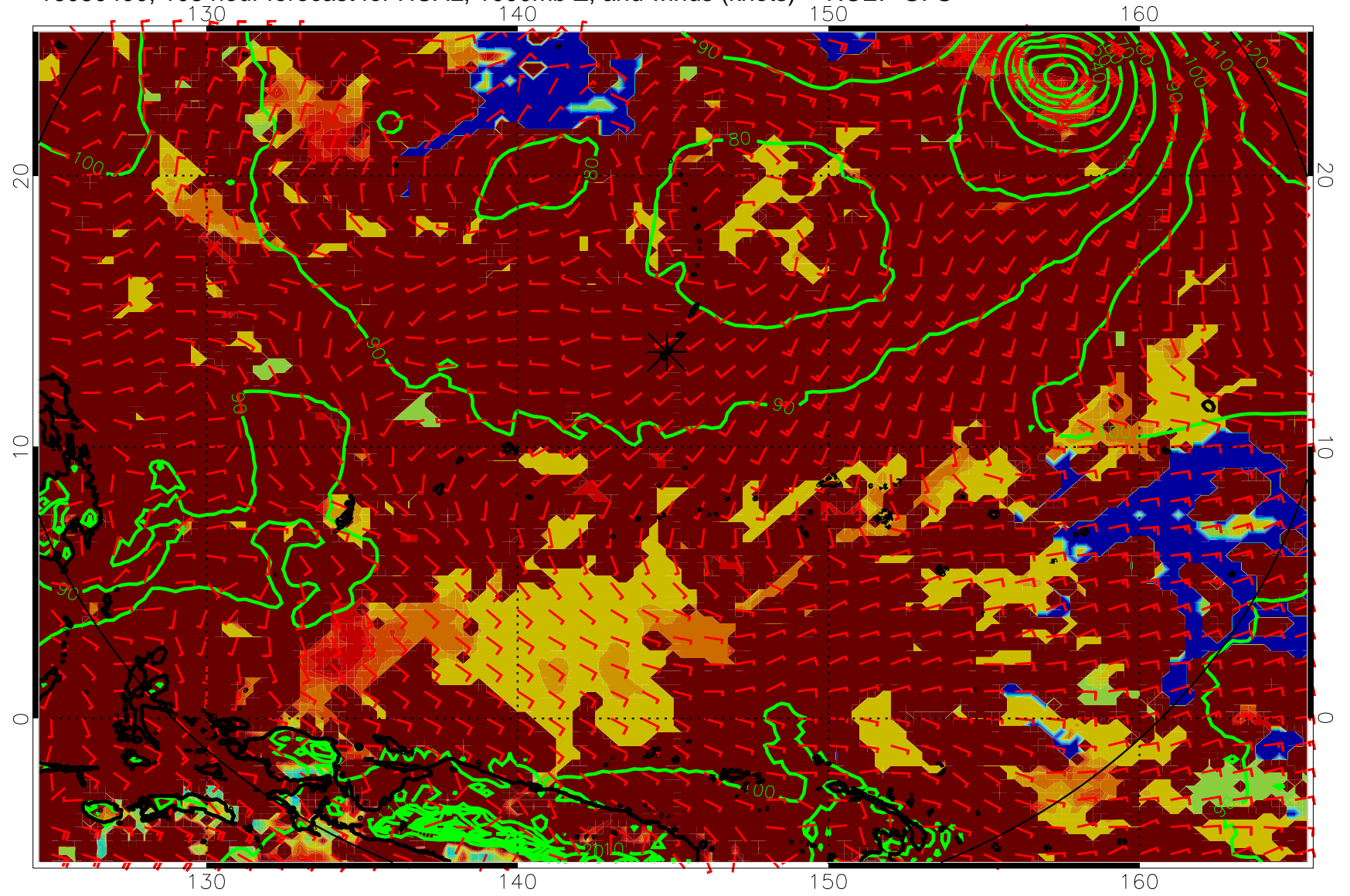
16080400, 108 hour forecast for HCAL, 1000mb Z, and winds (knots) -- NCEP GFS
