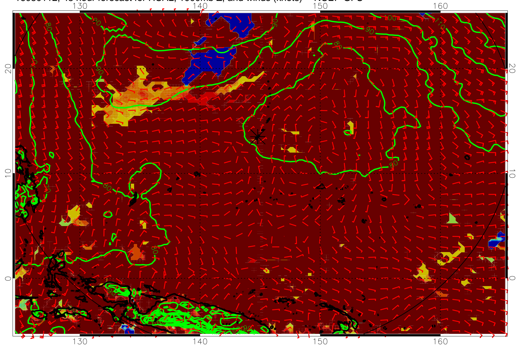
16080112, 48 hour forecast for HCAL, 1000mb Z, and winds (knots) -- NCEP GFS
