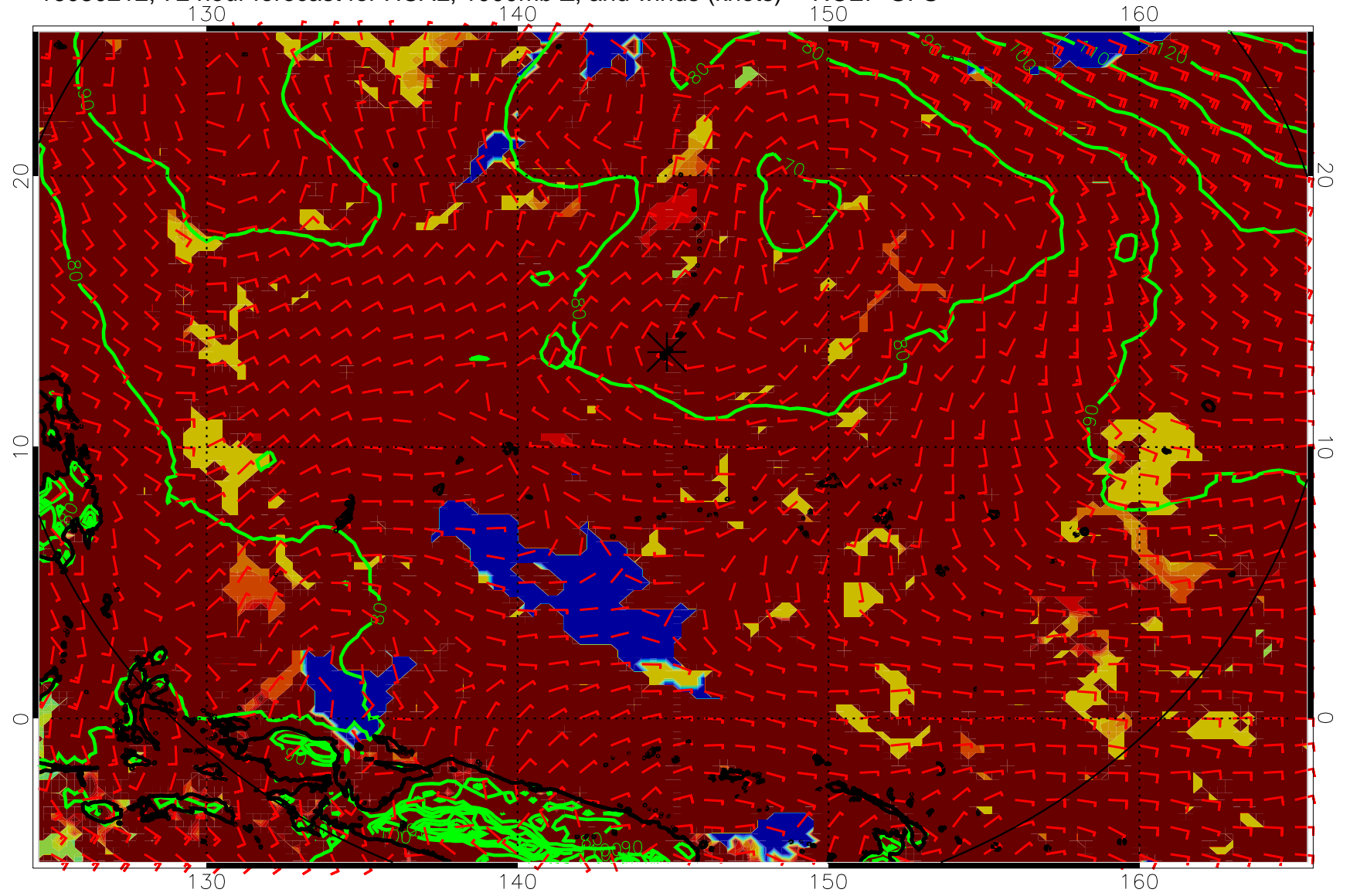
16080212, 72 hour forecast for HCAL, 1000mb Z, and winds (knots) -- NCEP GFS
