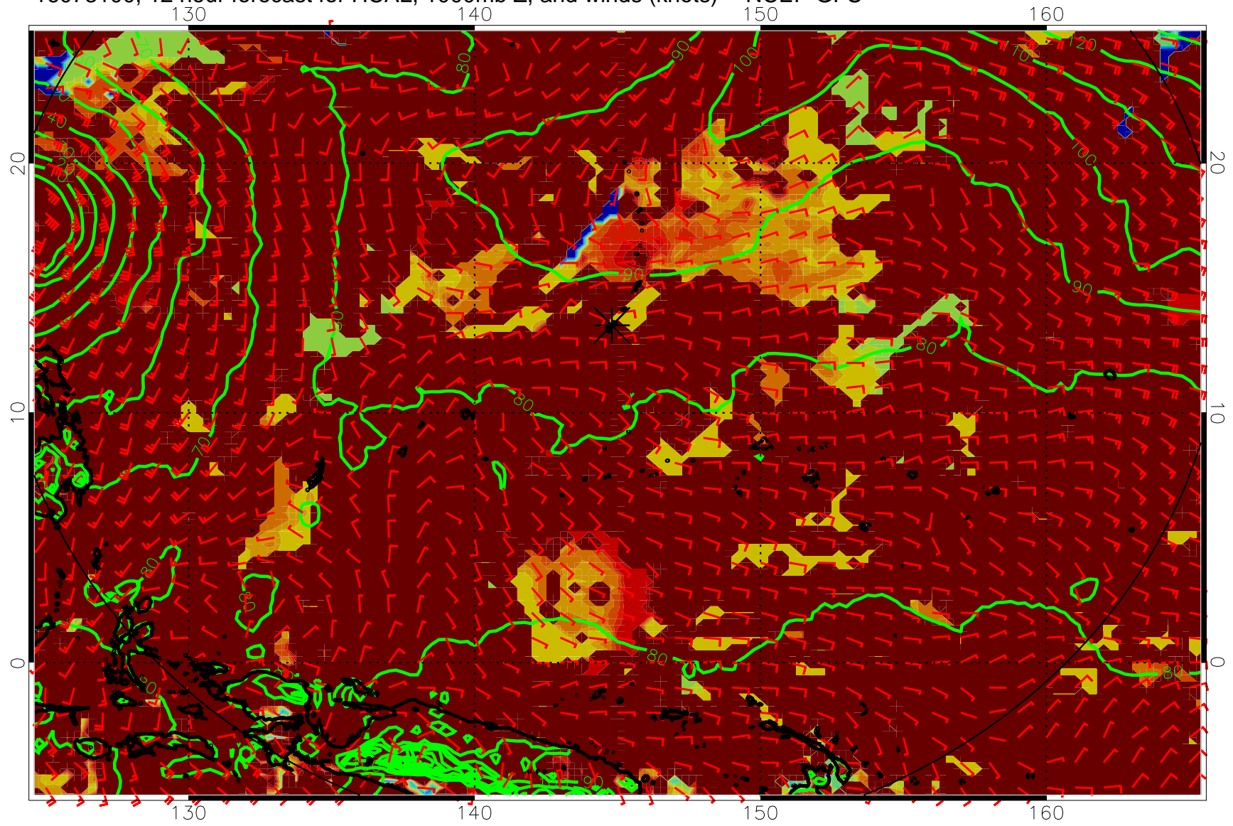
16073100, 12 hour forecast for HCAL, 1000mb Z, and winds (knots) -- NCEP GFS
