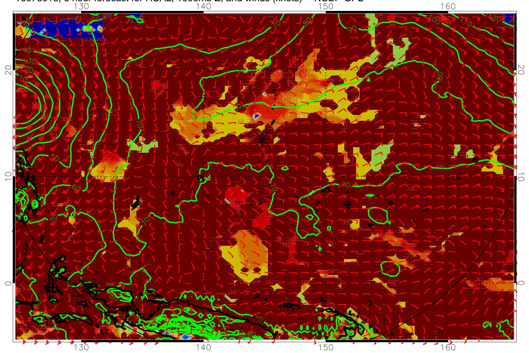
16073018, 6 hour forecast for HCAL, 1000mb Z, and winds (knots) -- NCEP GFS
