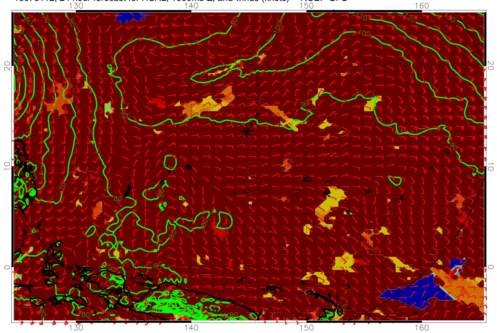
16073112, 24 hour forecast for HCAL, 1000mb Z, and winds (knots) -- NCEP GFS
