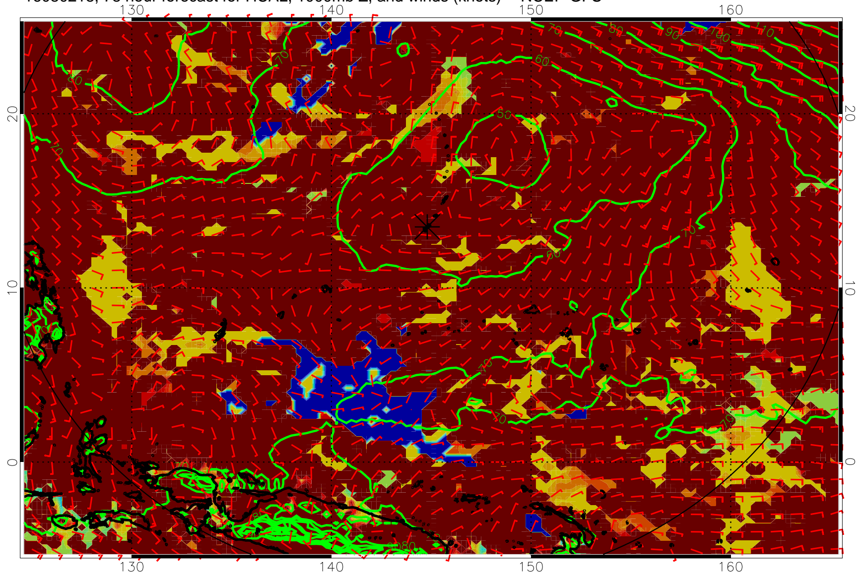
16080218, 78 hour forecast for HCAL, 1000mb Z, and winds (knots) -- NCEP GFS
