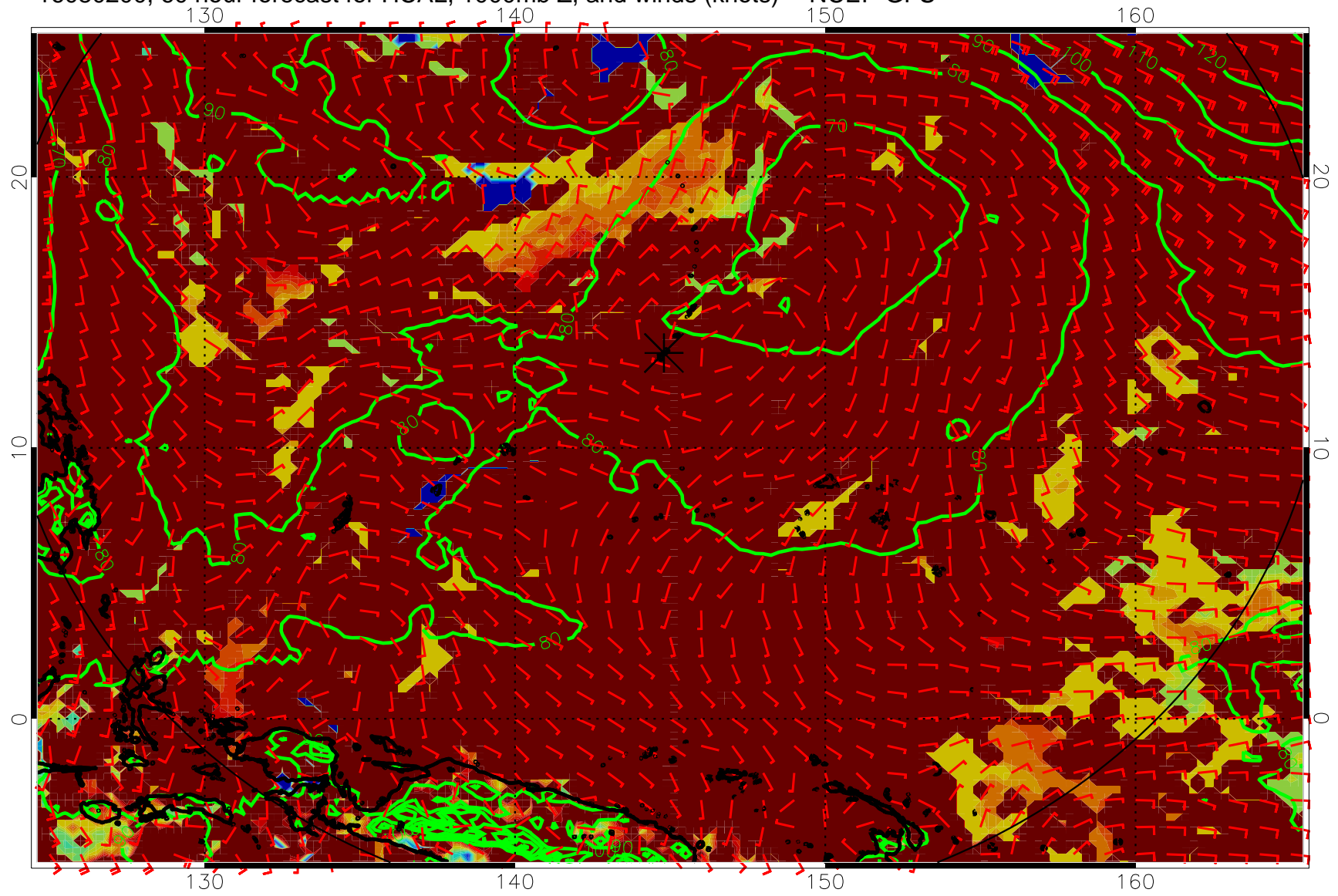
16080200, 60 hour forecast for HCAL, 1000mb Z, and winds (knots) -- NCEP GFS
