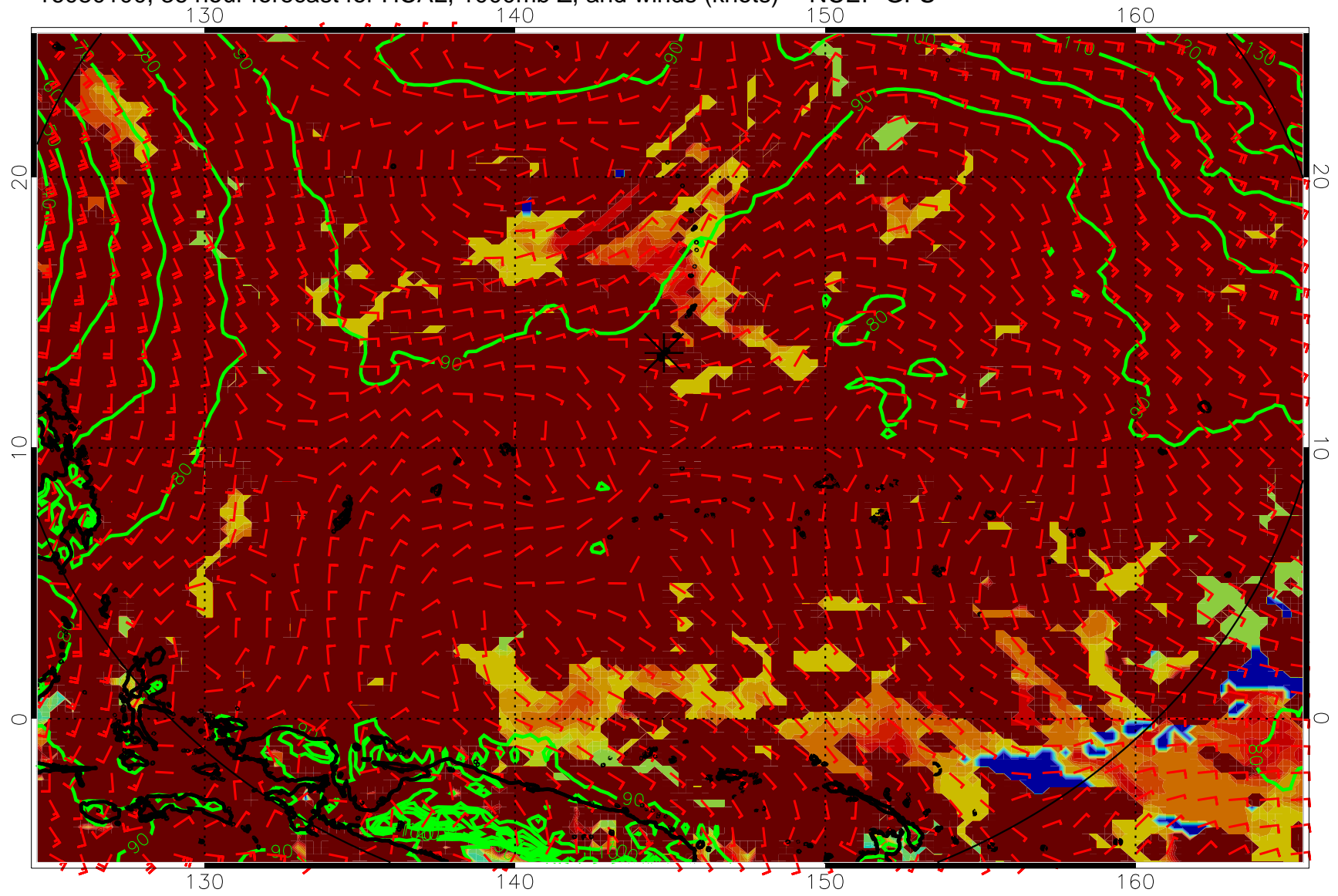
16080100, 36 hour forecast for HCAL, 1000mb Z, and winds (knots) -- NCEP GFS
