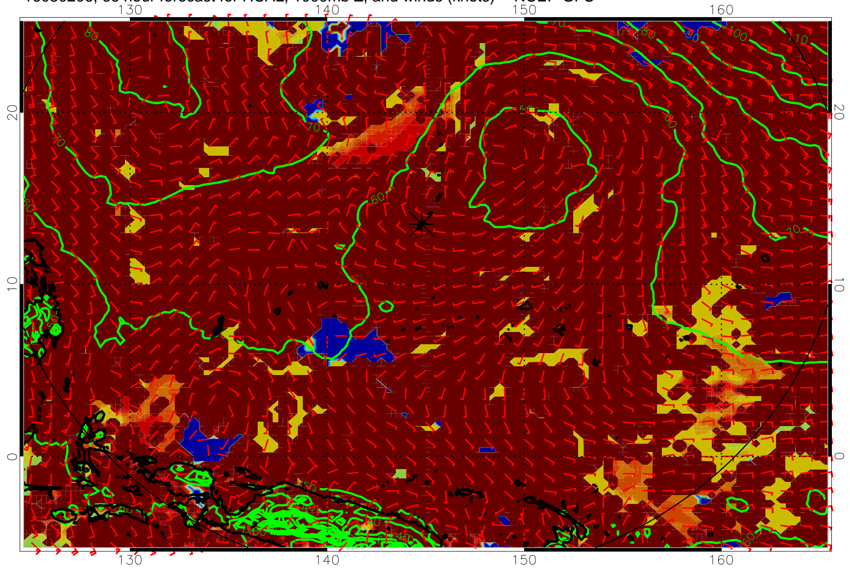
16080206, 66 hour forecast for HCAL, 1000mb Z, and winds (knots) -- NCEP GFS
