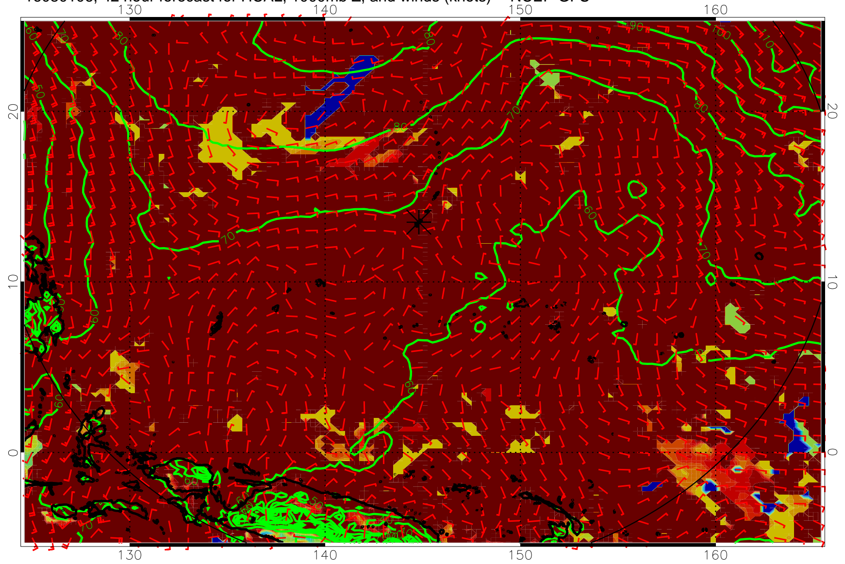
16080106, 42 hour forecast for HCAL, 1000mb Z, and winds (knots) -- NCEP GFS
