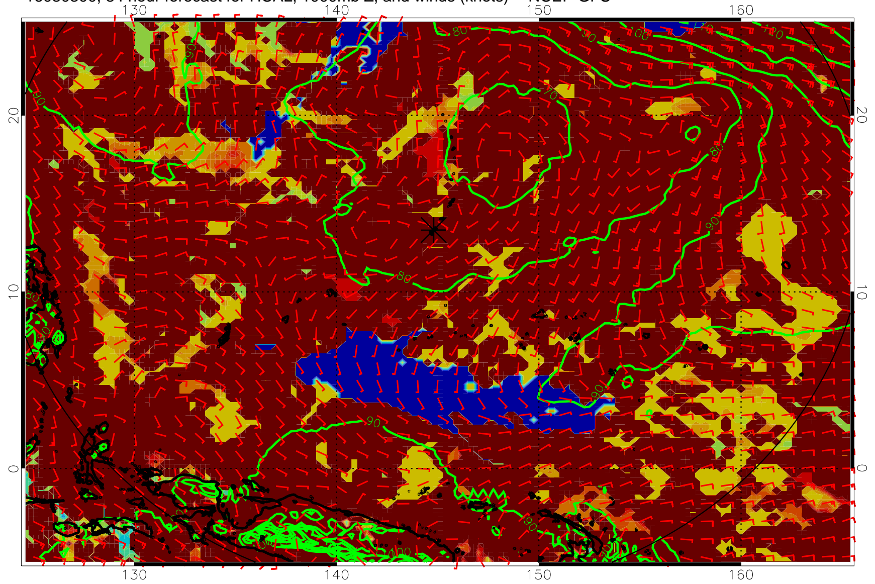
16080300, 84 hour forecast for HCAL, 1000mb Z, and winds (knots) -- NCEP GFS
