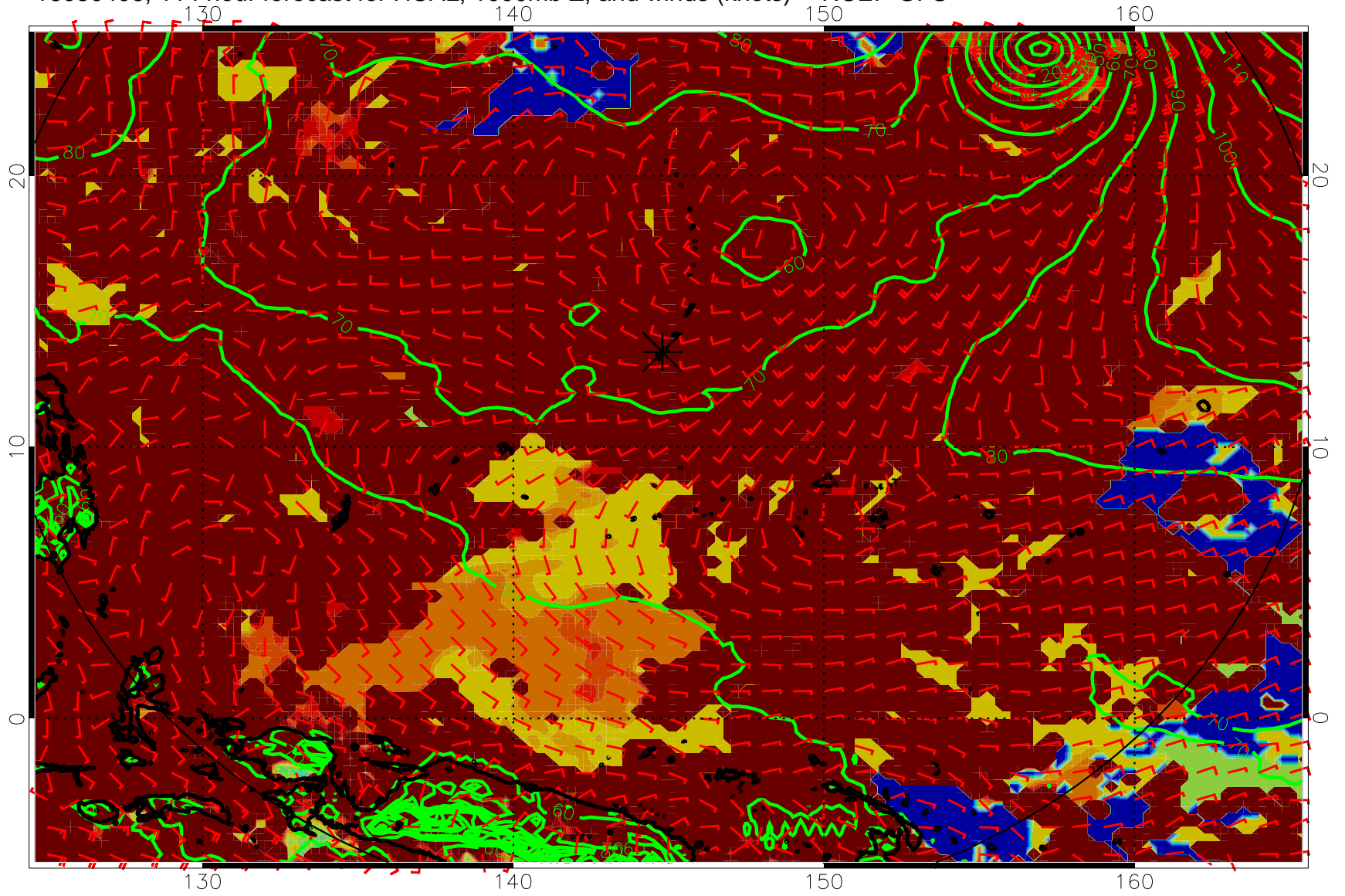
16080406, 114 hour forecast for HCAL, 1000mb Z, and winds (knots) -- NCEP GFS
