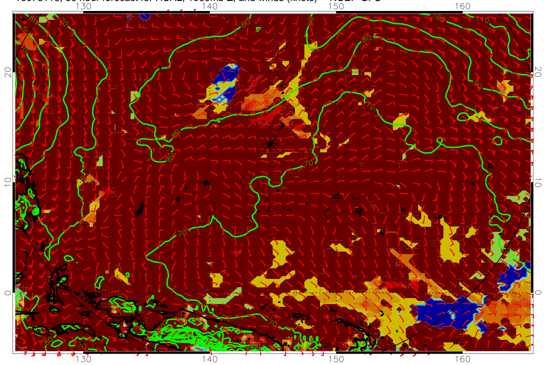
16073118, 30 hour forecast for HCAL, 1000mb Z, and winds (knots) -- NCEP GFS
