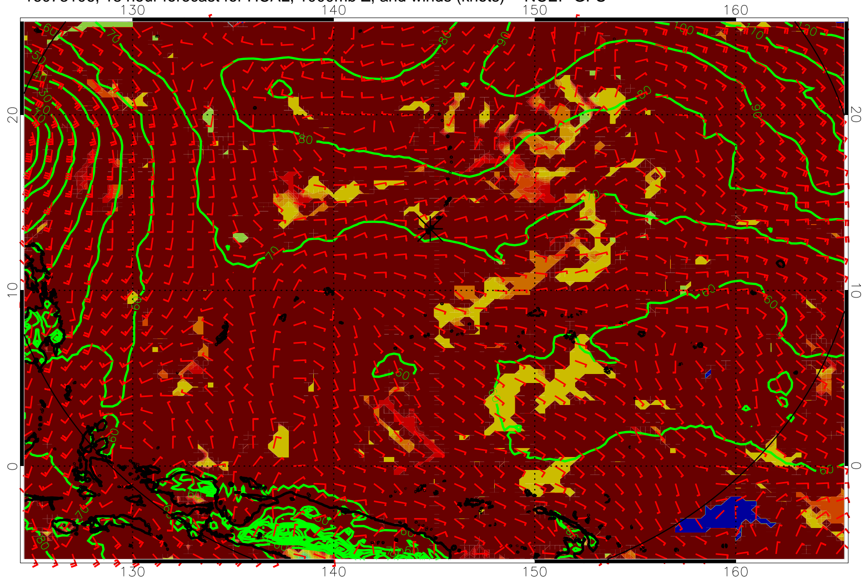
16073106, 18 hour forecast for HCAL, 1000mb Z, and winds (knots) -- NCEP GFS
