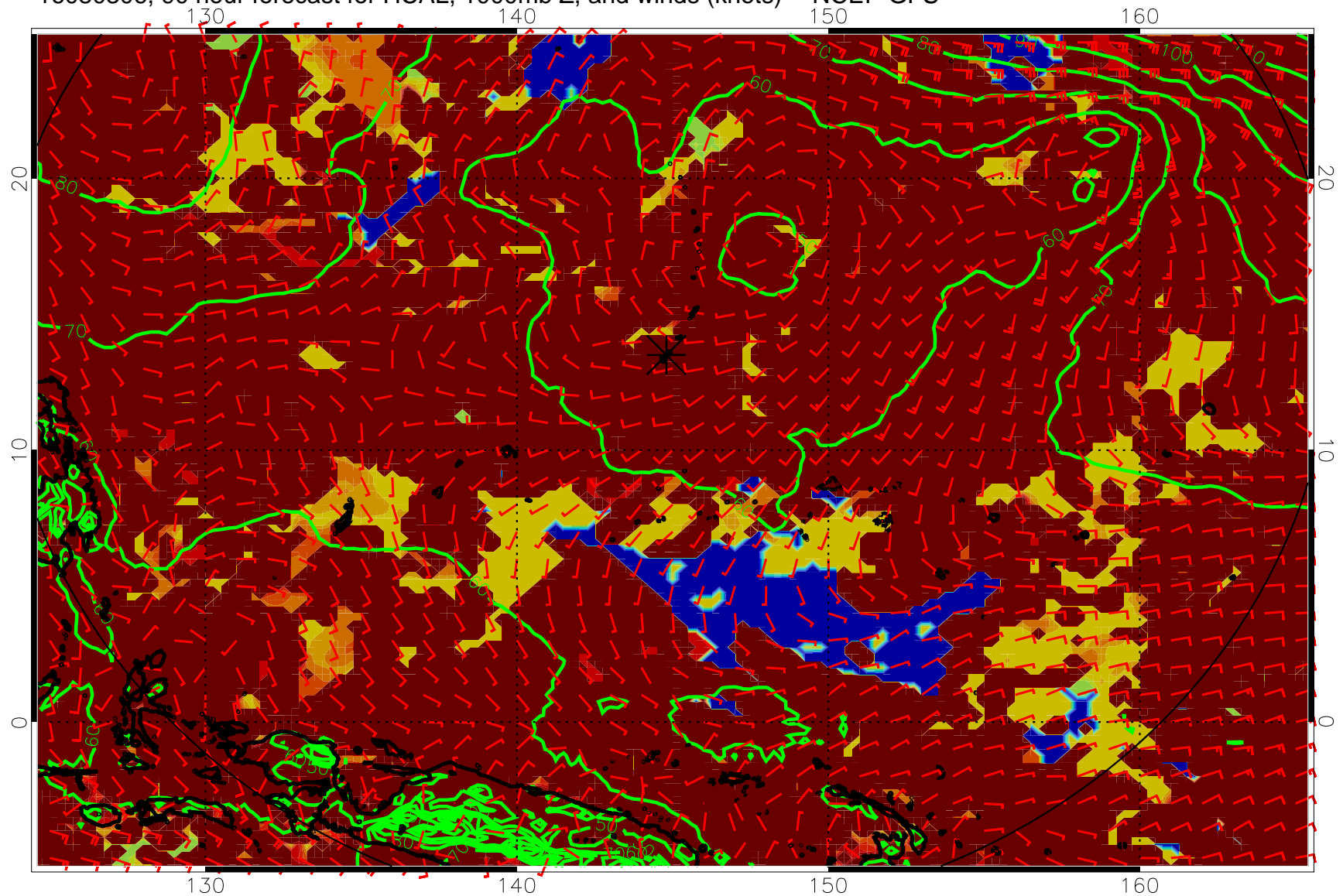
16080306, 90 hour forecast for HCAL, 1000mb Z, and winds (knots) -- NCEP GFS
