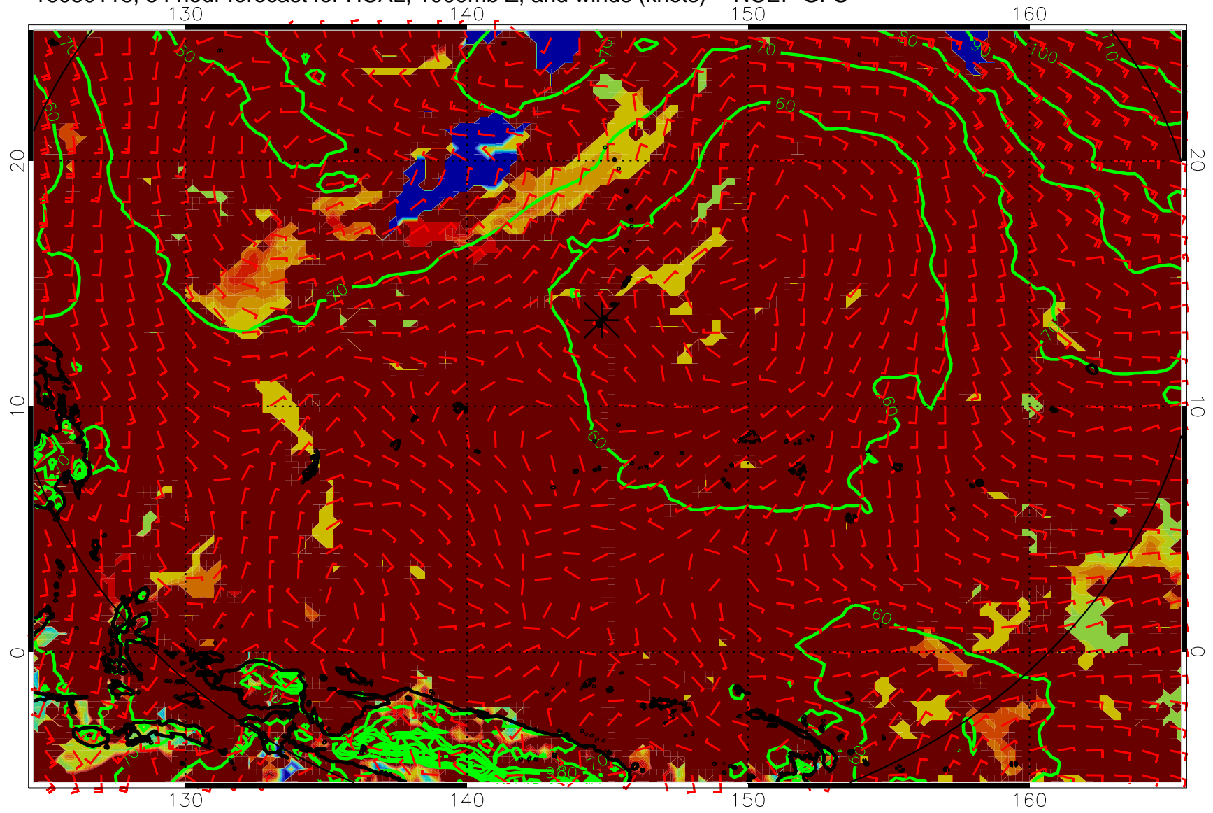
16080118, 54 hour forecast for HCAL, 1000mb Z, and winds (knots) -- NCEP GFS
