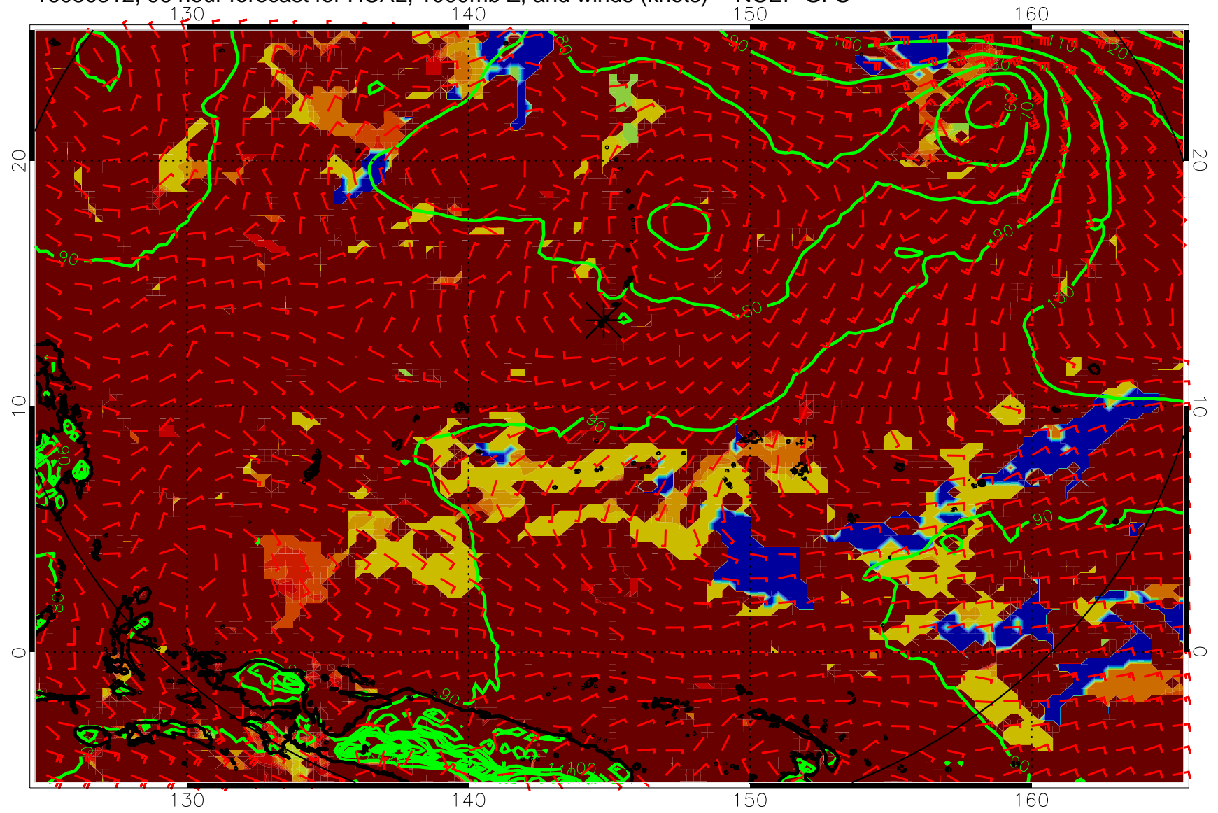
16080312, 96 hour forecast for HCAL, 1000mb Z, and winds (knots) -- NCEP GFS
