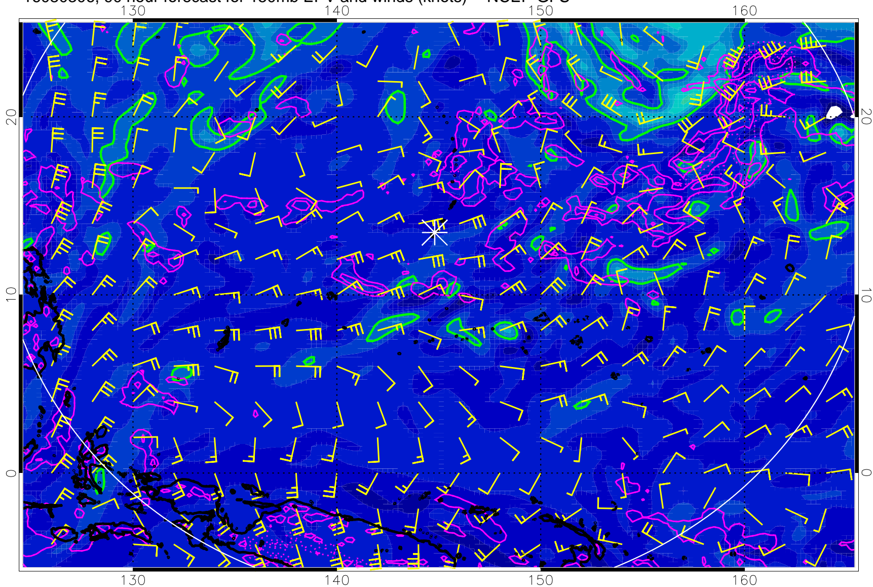
16080306, 90 hour forecast for 150mb EPV and winds (knots) -- NCEP GFS
