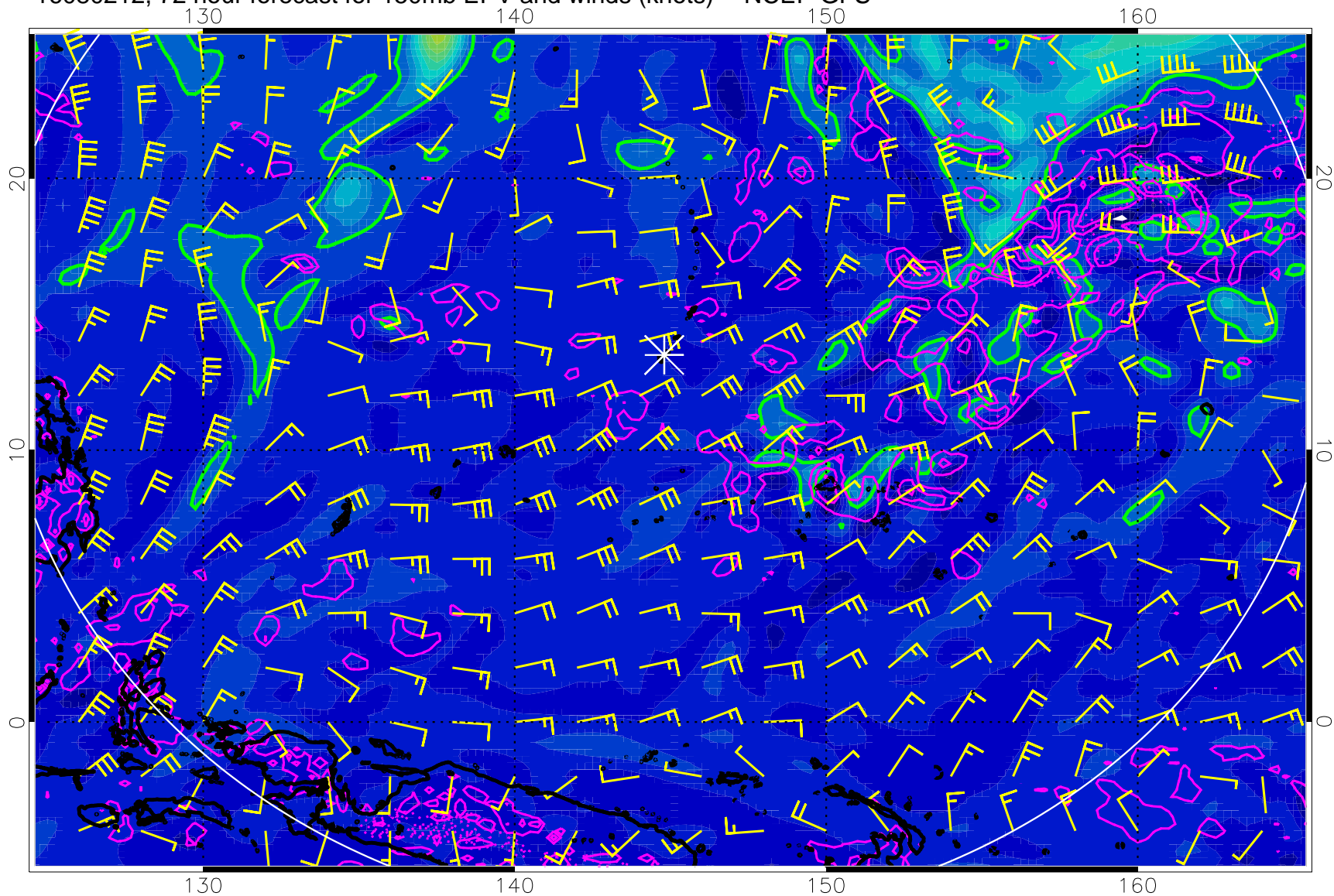
16080212, 72 hour forecast for 150mb EPV and winds (knots) -- NCEP GFS
