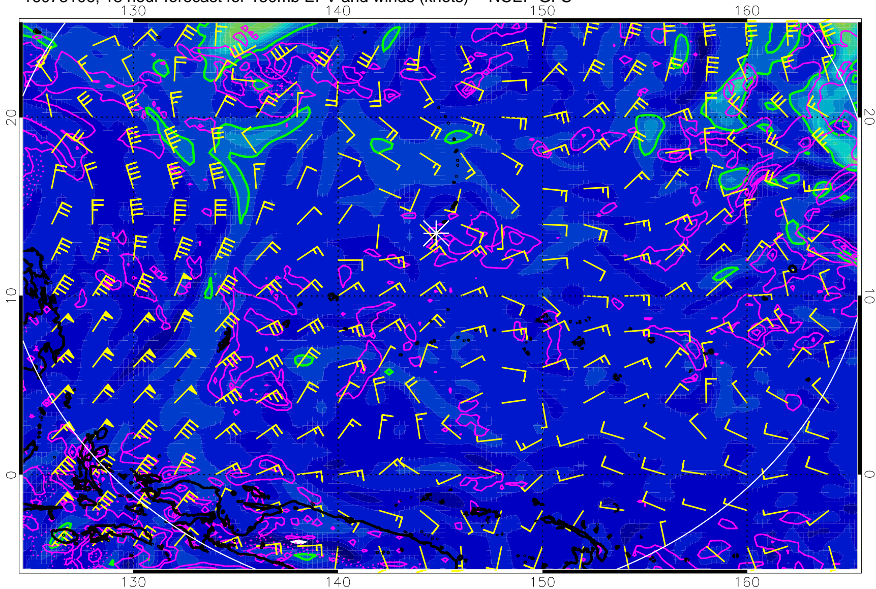
16073106, 18 hour forecast for 150mb EPV and winds (knots) -- NCEP GFS
