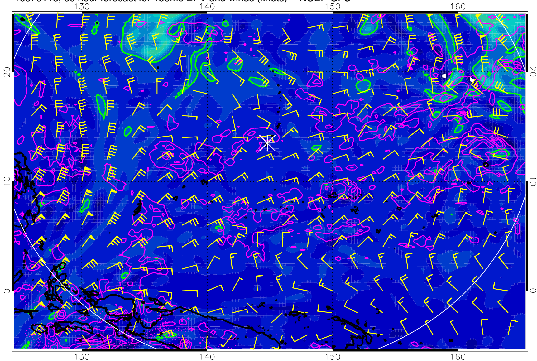
16073118, 30 hour forecast for 150mb EPV and winds (knots) -- NCEP GFS
