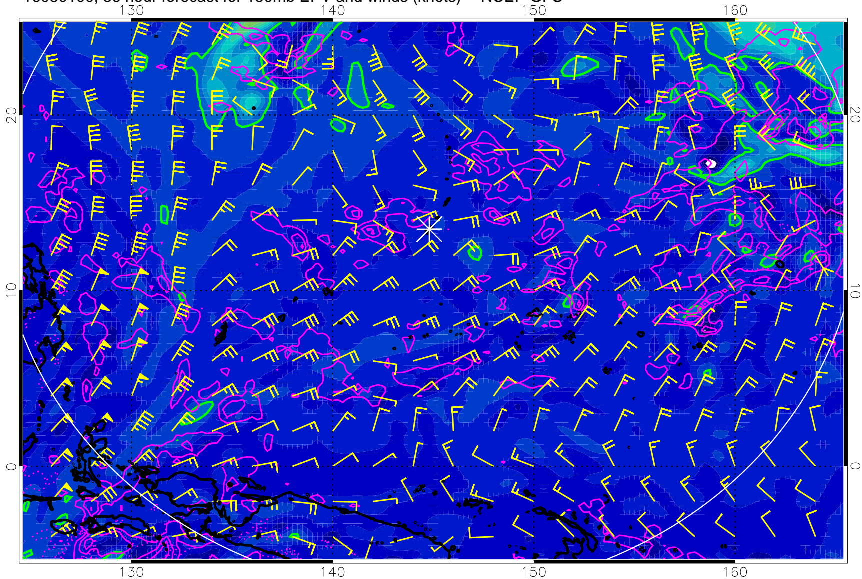
16080100, 36 hour forecast for 150mb EPV and winds (knots) -- NCEP GFS
