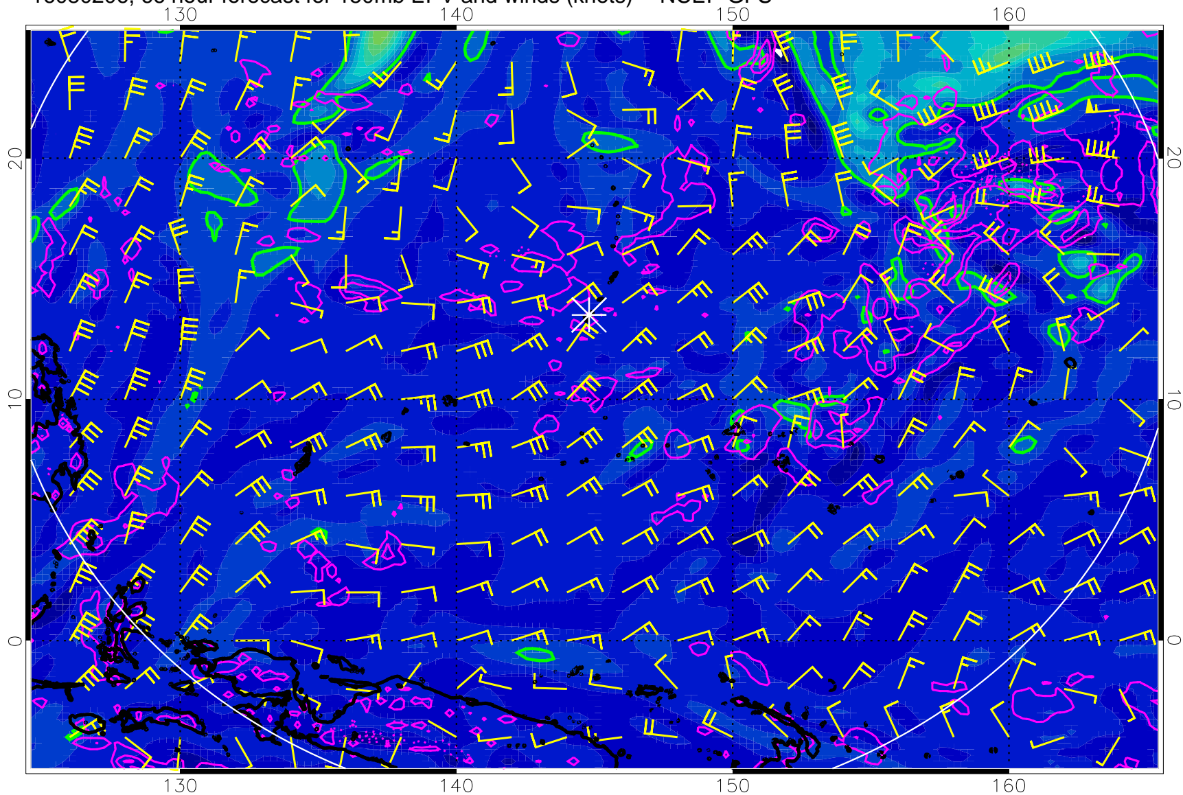
16080206, 66 hour forecast for 150mb EPV and winds (knots) -- NCEP GFS
