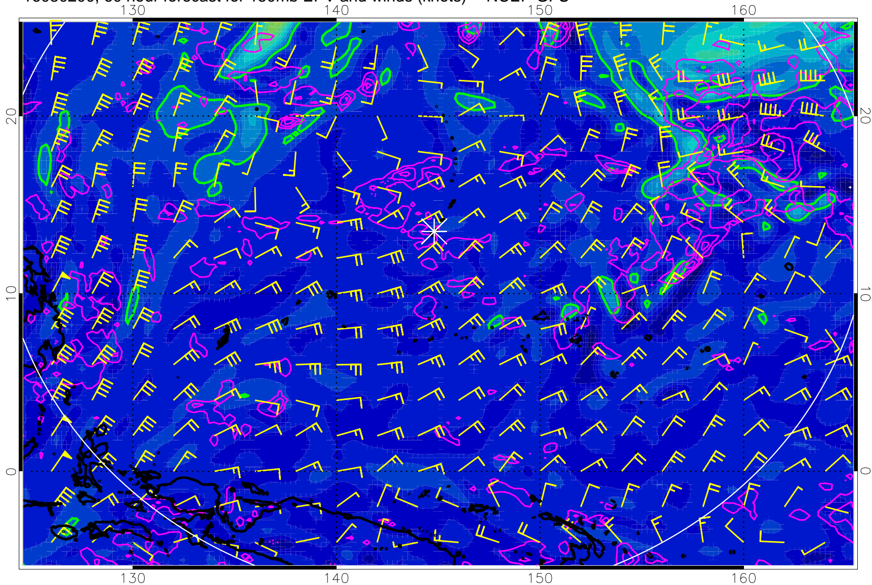
16080200, 60 hour forecast for 150mb EPV and winds (knots) -- NCEP GFS
