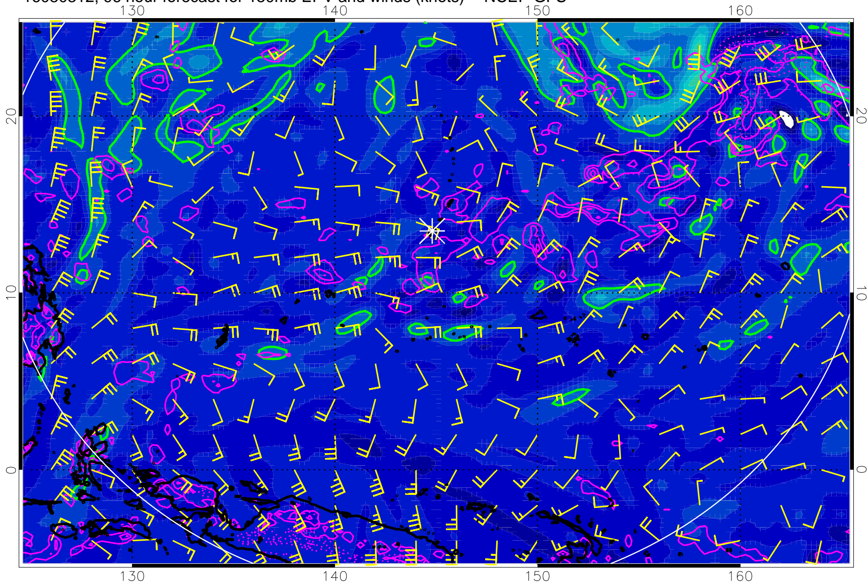
16080312, 96 hour forecast for 150mb EPV and winds (knots) -- NCEP GFS
