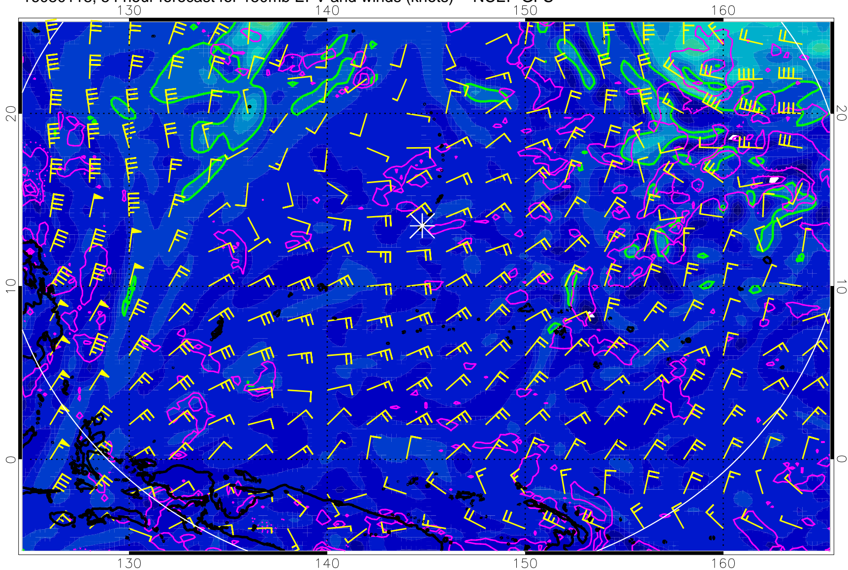
16080118, 54 hour forecast for 150mb EPV and winds (knots) -- NCEP GFS
