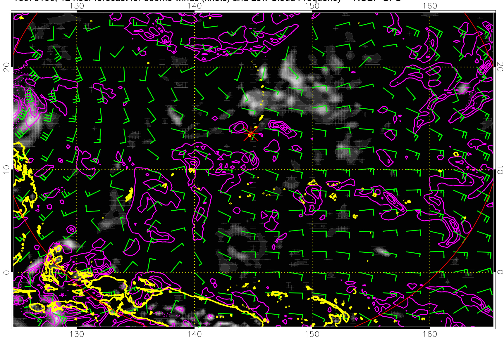
16073100, 12 hour forecast for 850mb winds (knots) and Low Cloud Frequency -- NCEP GFS
