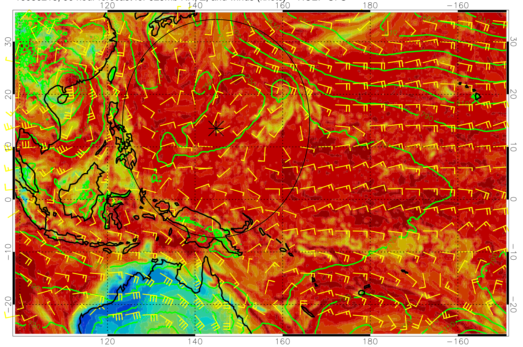
16080218, 90 hour forecast for 925mb RH, Z, and winds (knots) -- NCEP GFS
