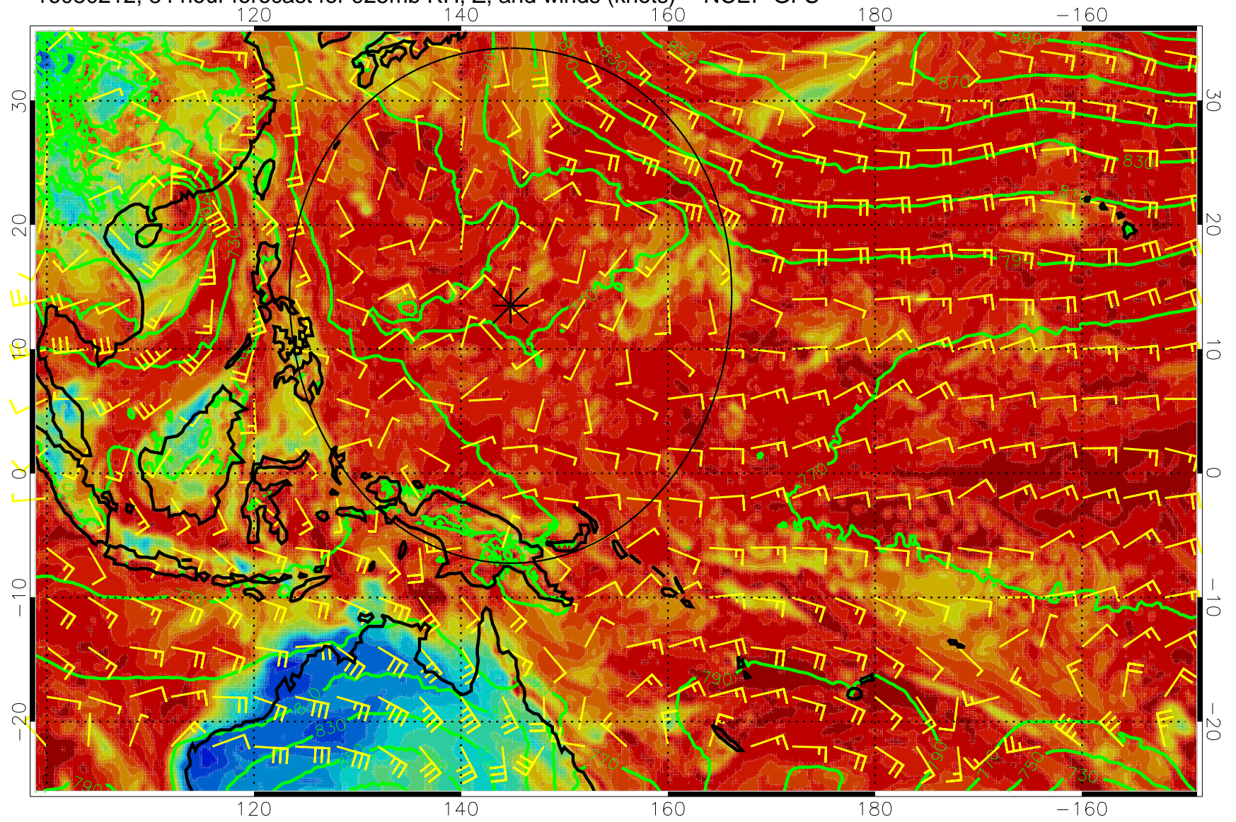
16080212, 84 hour forecast for 925mb RH, Z, and winds (knots) -- NCEP GFS
