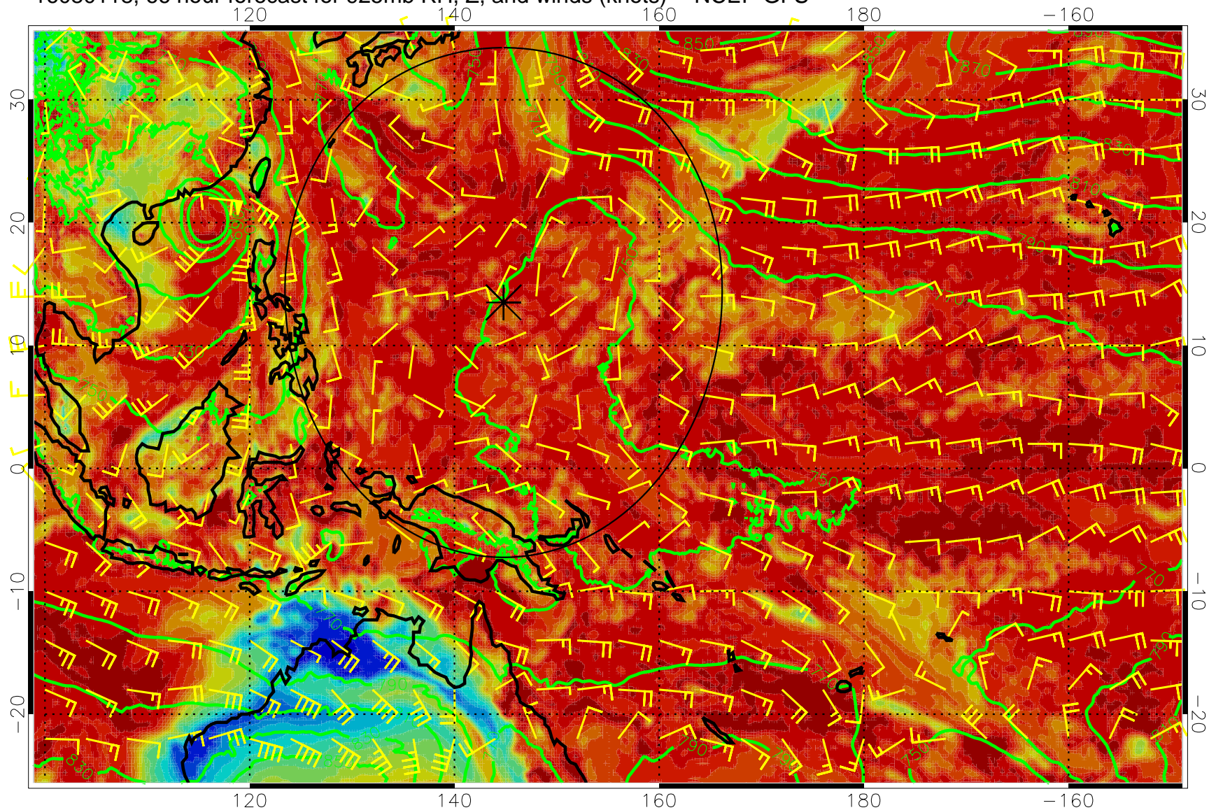
16080118, 66 hour forecast for 925mb RH, Z, and winds (knots) -- NCEP GFS
