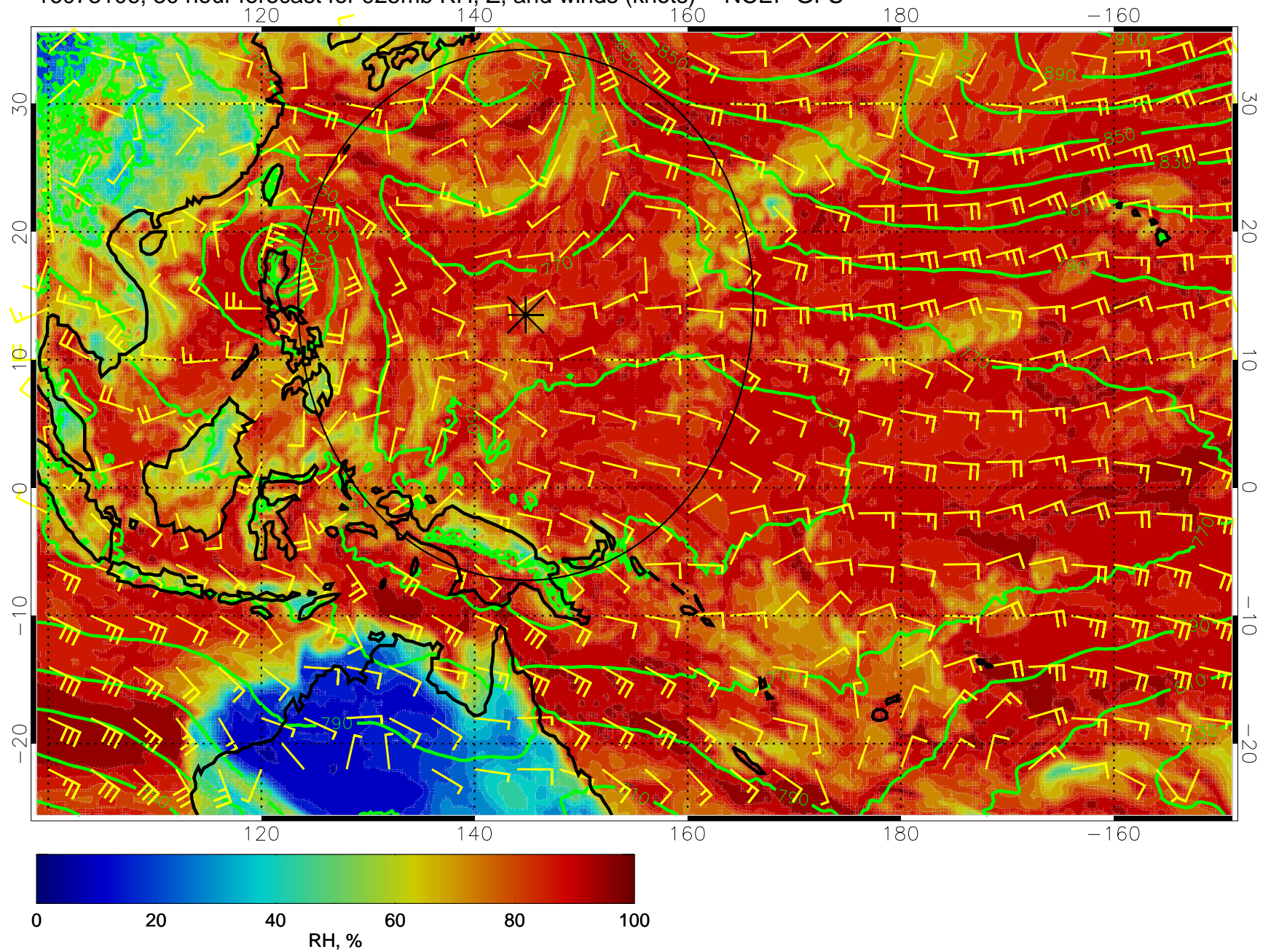
16073106, 30 hour forecast for 925mb RH, Z, and winds (knots) -- NCEP GFS
