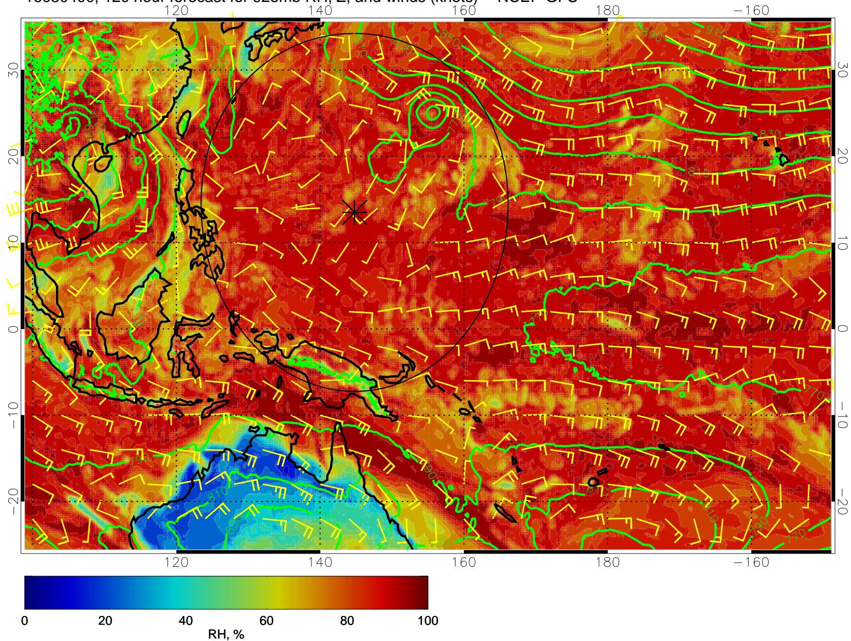
16080400, 120 hour forecast for 925mb RH, Z, and winds (knots) -- NCEP GFS
