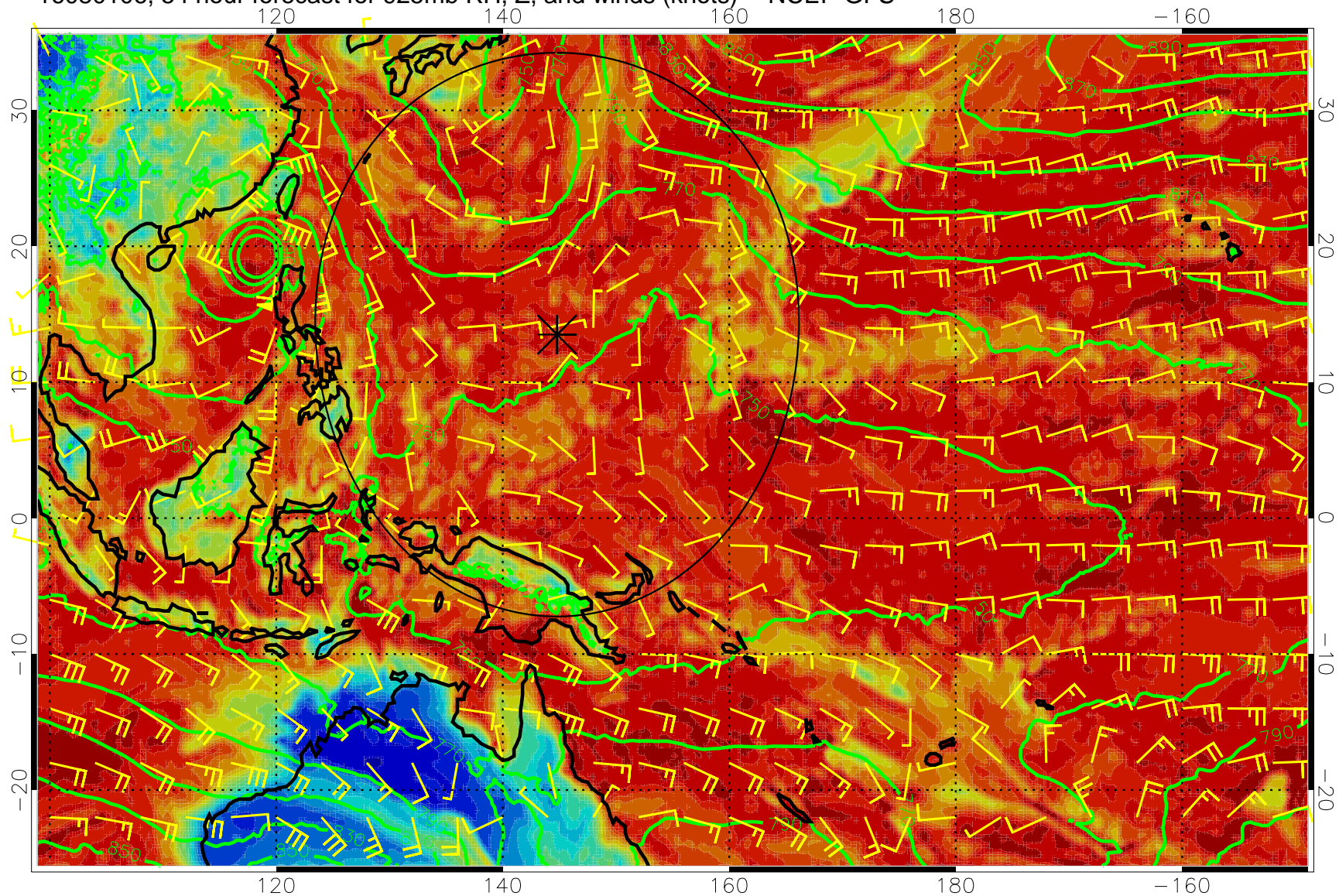
16080106, 54 hour forecast for 925mb RH, Z, and winds (knots) -- NCEP GFS
