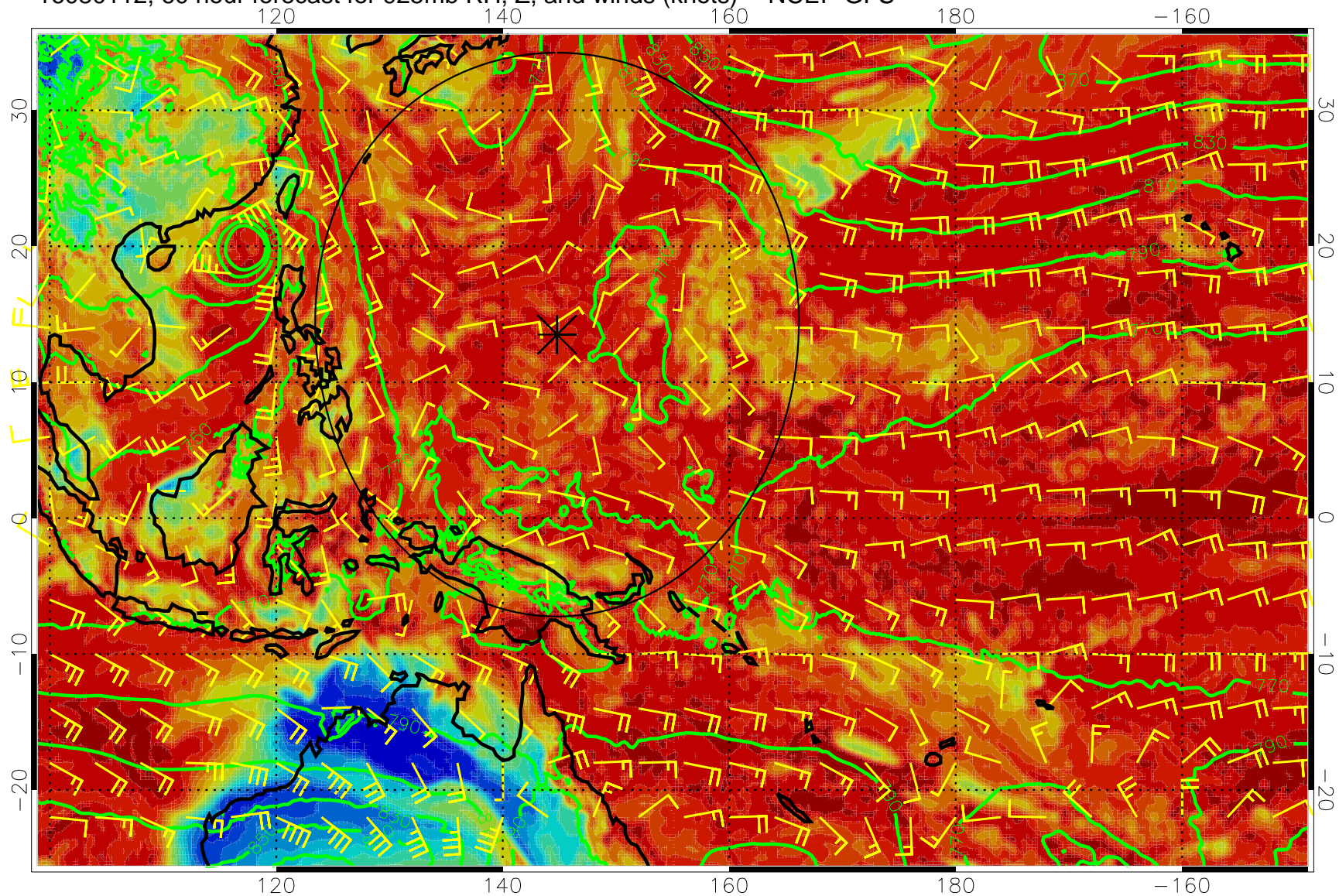
16080112, 60 hour forecast for 925mb RH, Z, and winds (knots) -- NCEP GFS
