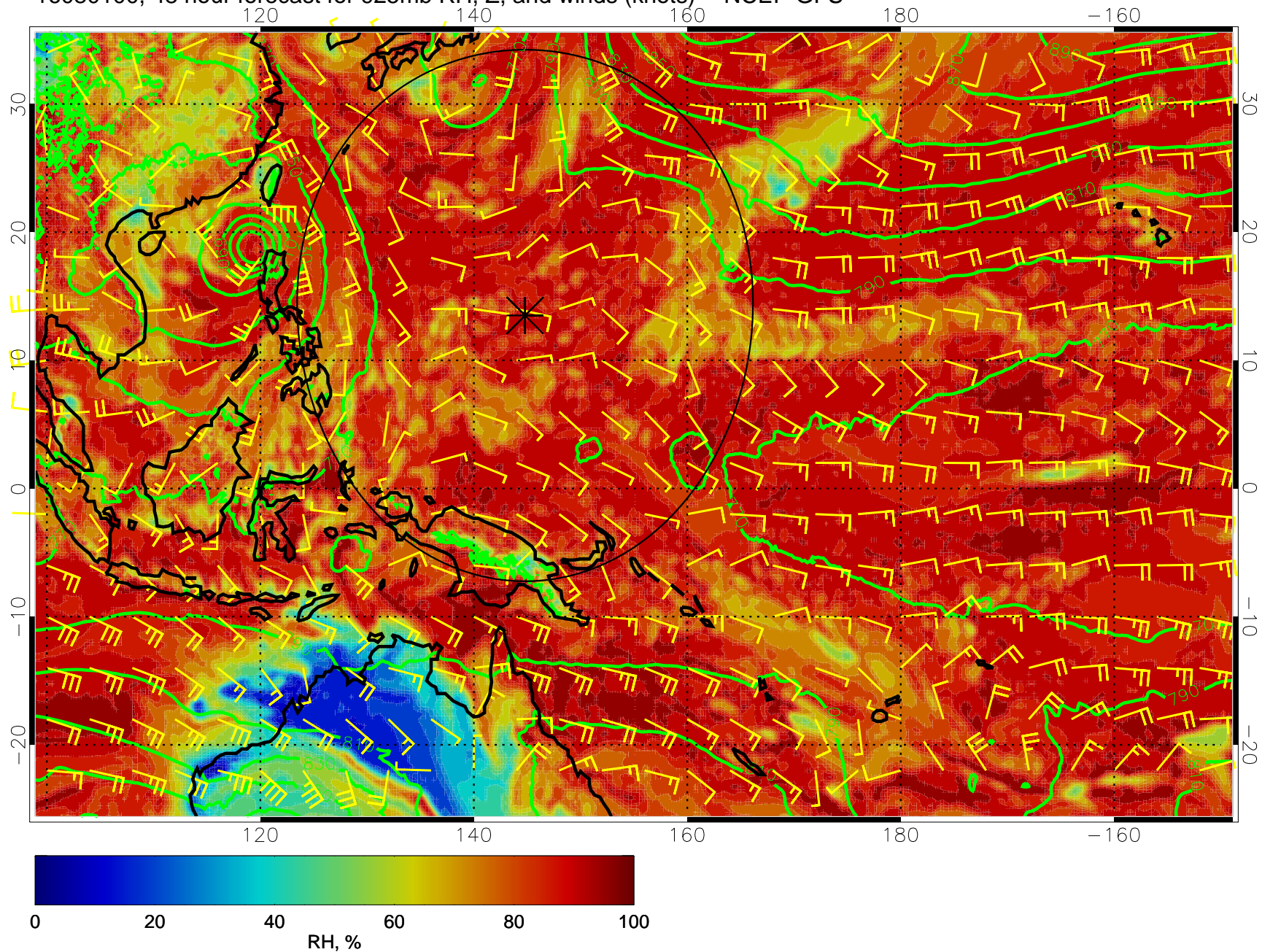
16080100, 48 hour forecast for 925mb RH, Z, and winds (knots) -- NCEP GFS
