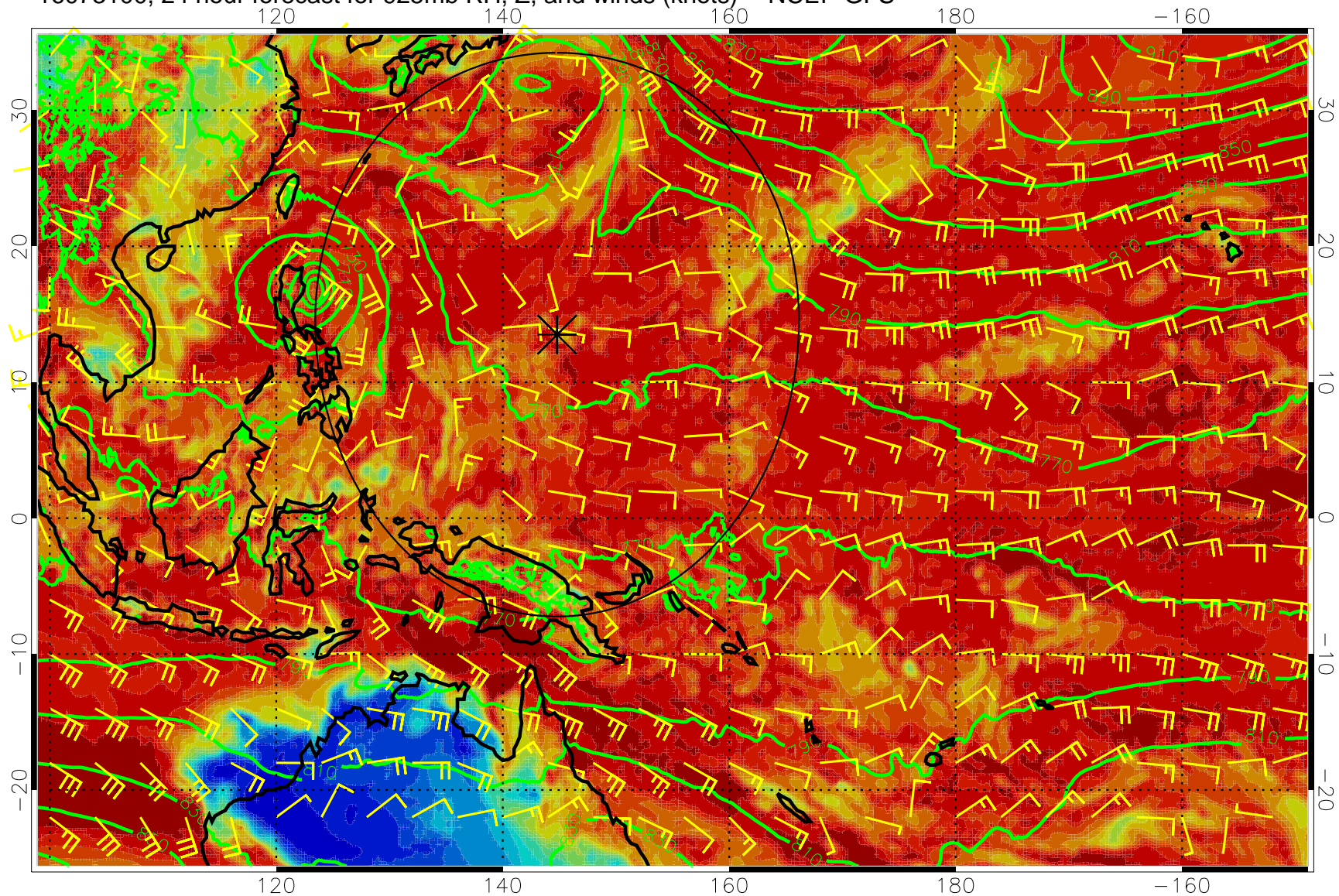
16073100, 24 hour forecast for 925mb RH, Z, and winds (knots) -- NCEP GFS
