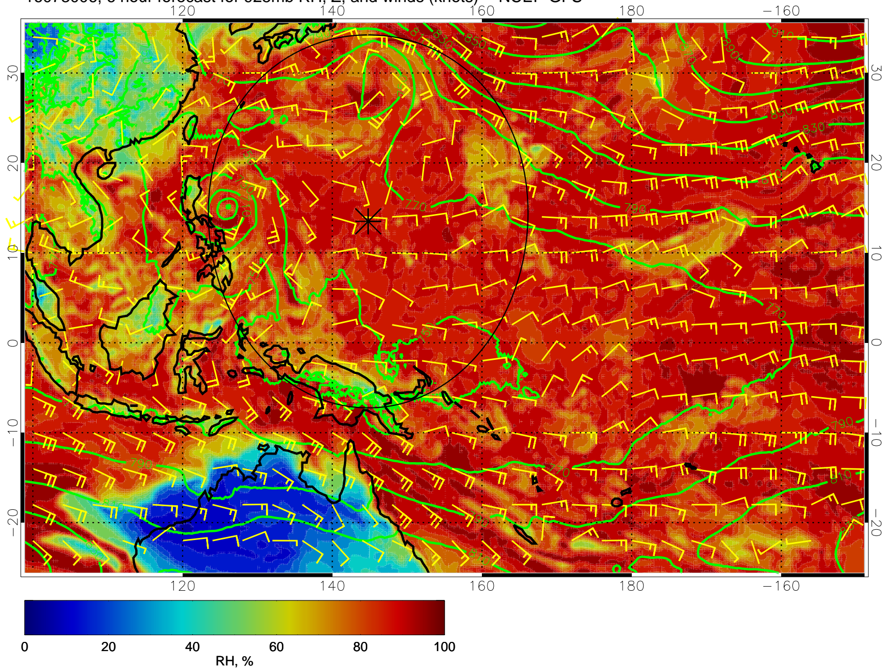
16073006, 6 hour forecast for 925mb RH, Z, and winds (knots) -- NCEP GFS
