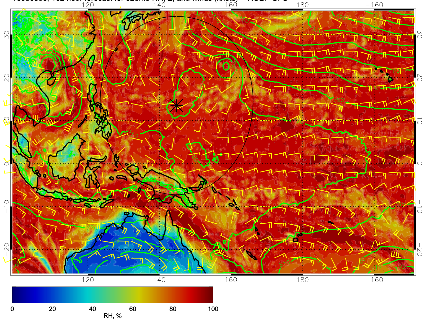
16080306, 102 hour forecast for 925mb RH, Z, and winds (knots) -- NCEP GFS
