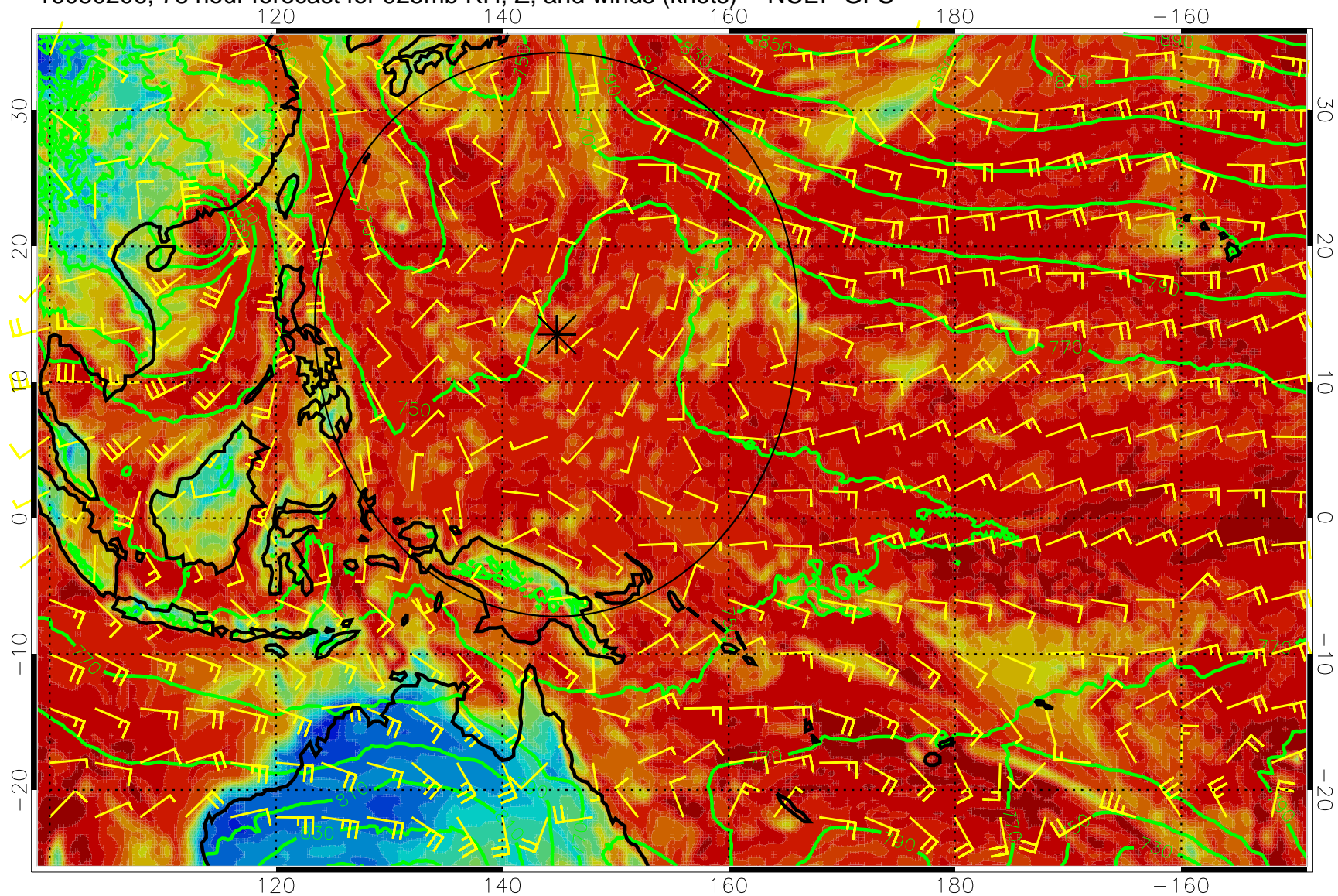
16080206, 78 hour forecast for 925mb RH, Z, and winds (knots) -- NCEP GFS
