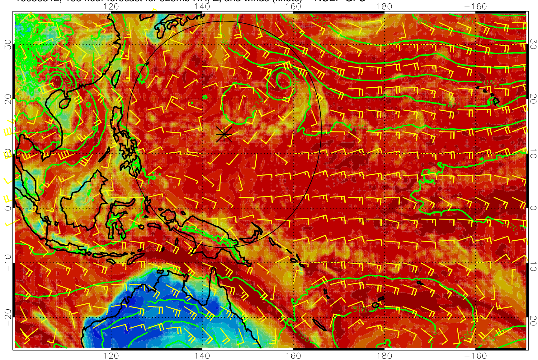
16080312, 108 hour forecast for 925mb RH, Z, and winds (knots) -- NCEP GFS
