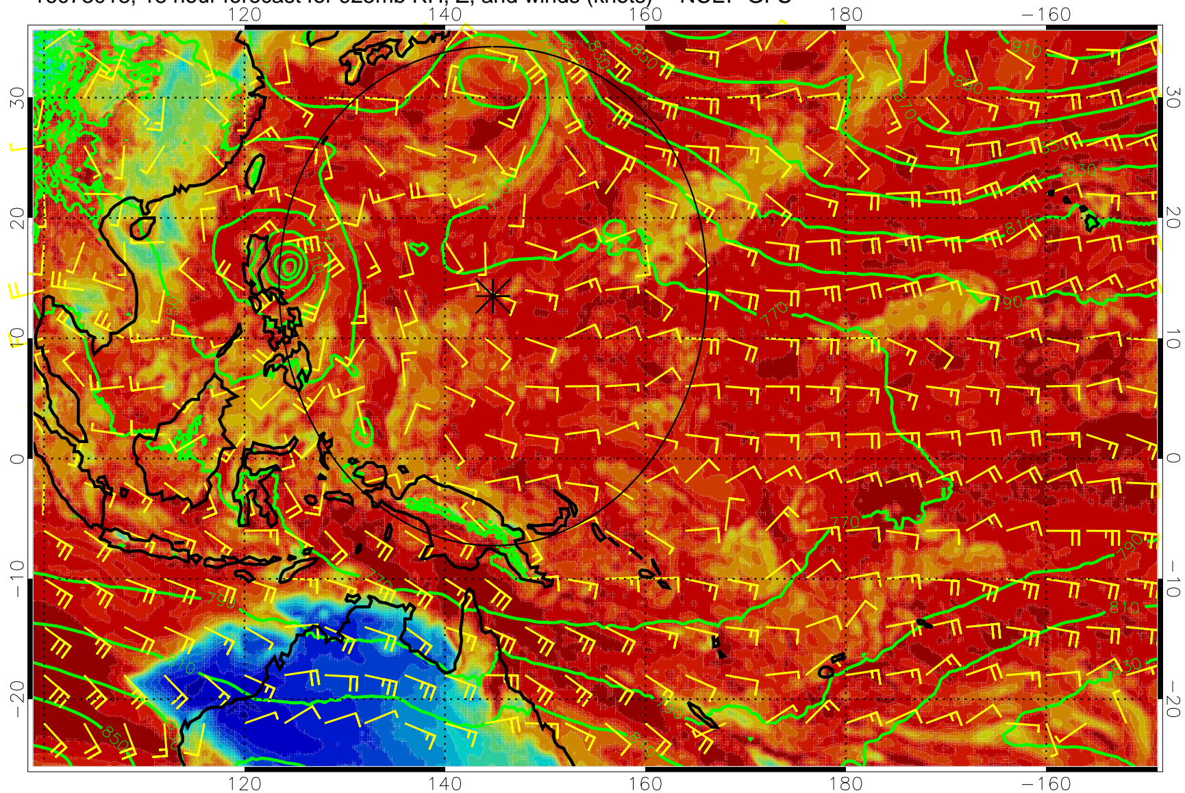
16073018, 18 hour forecast for 925mb RH, Z, and winds (knots) -- NCEP GFS
