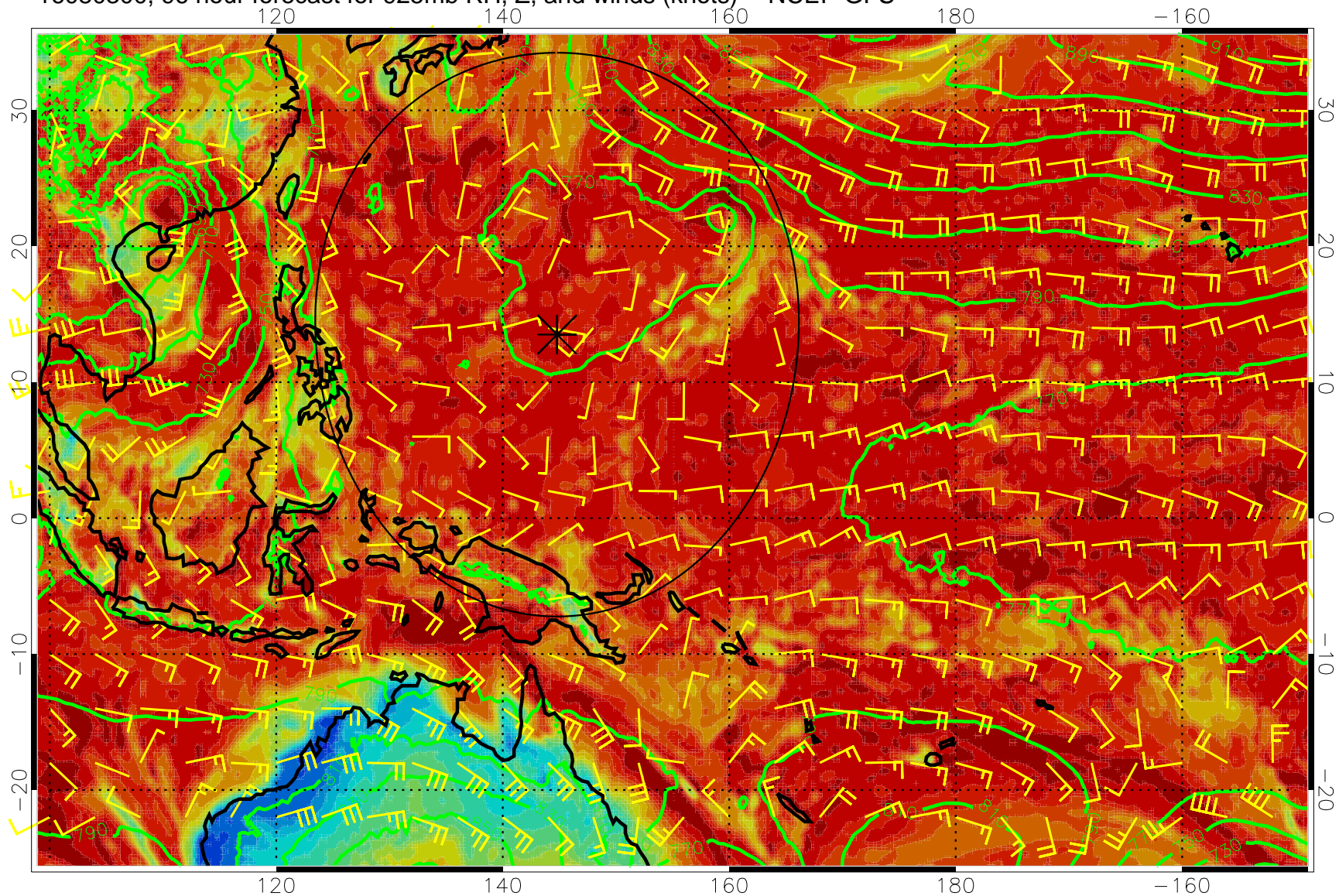
16080300, 96 hour forecast for 925mb RH, Z, and winds (knots) -- NCEP GFS
