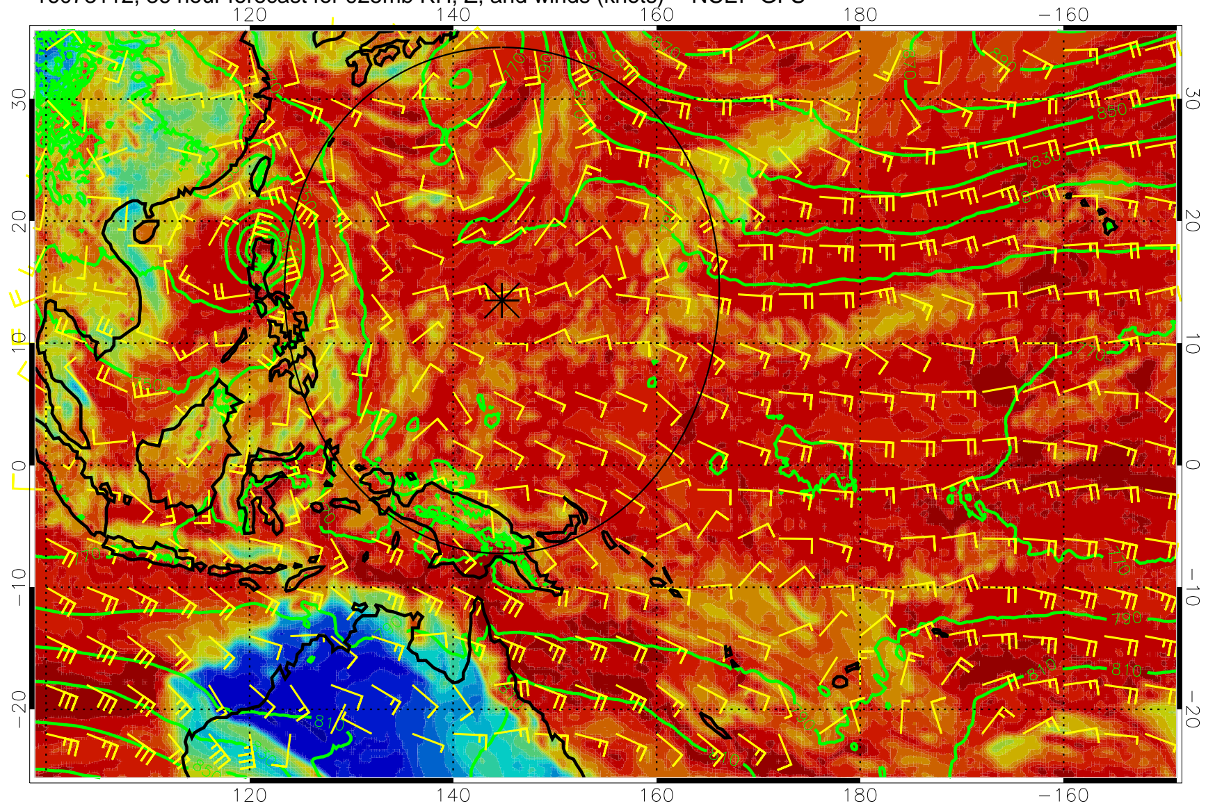
16073112, 36 hour forecast for 925mb RH, Z, and winds (knots) -- NCEP GFS
