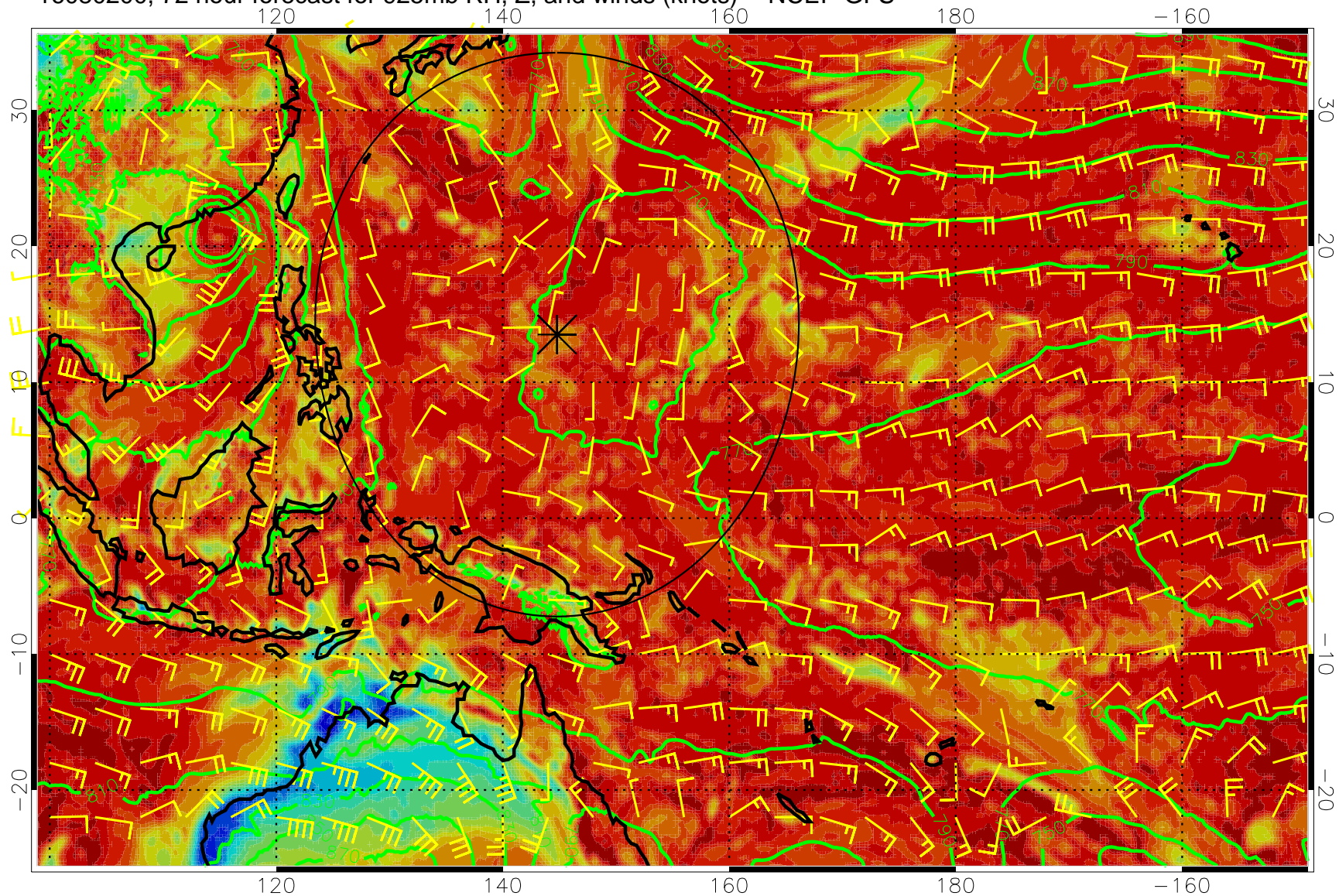
16080200, 72 hour forecast for 925mb RH, Z, and winds (knots) -- NCEP GFS
