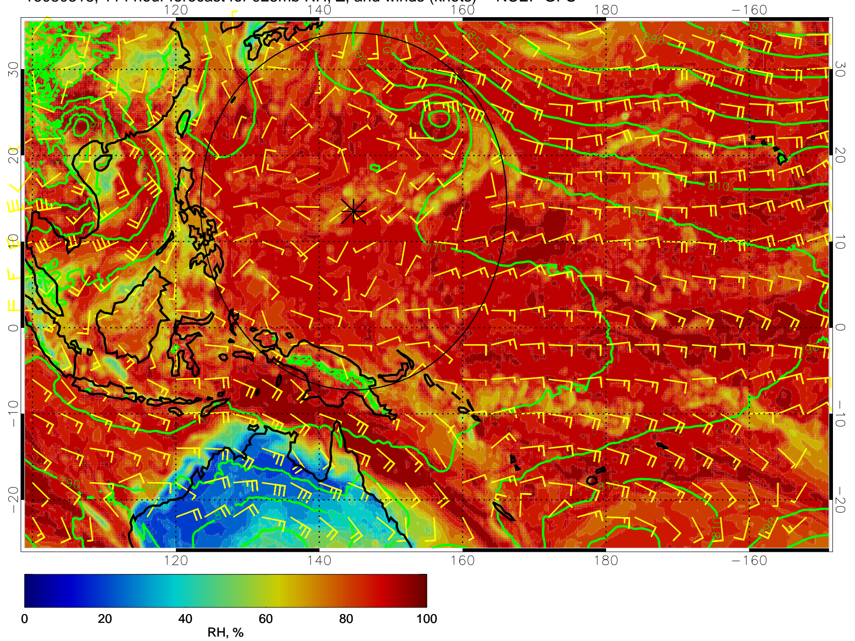
16080318, 114 hour forecast for 925mb RH, Z, and winds (knots) -- NCEP GFS
