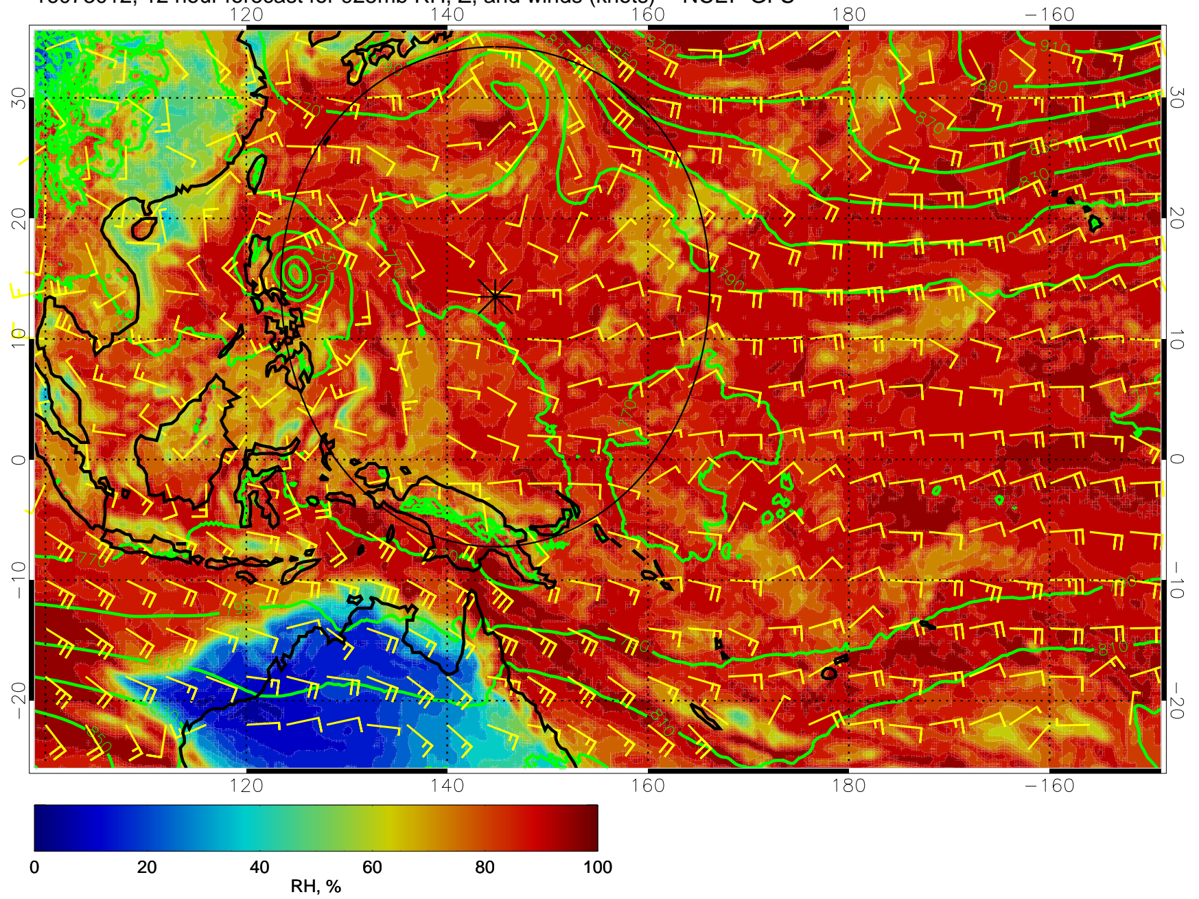
16073012, 12 hour forecast for 925mb RH, Z, and winds (knots) -- NCEP GFS
