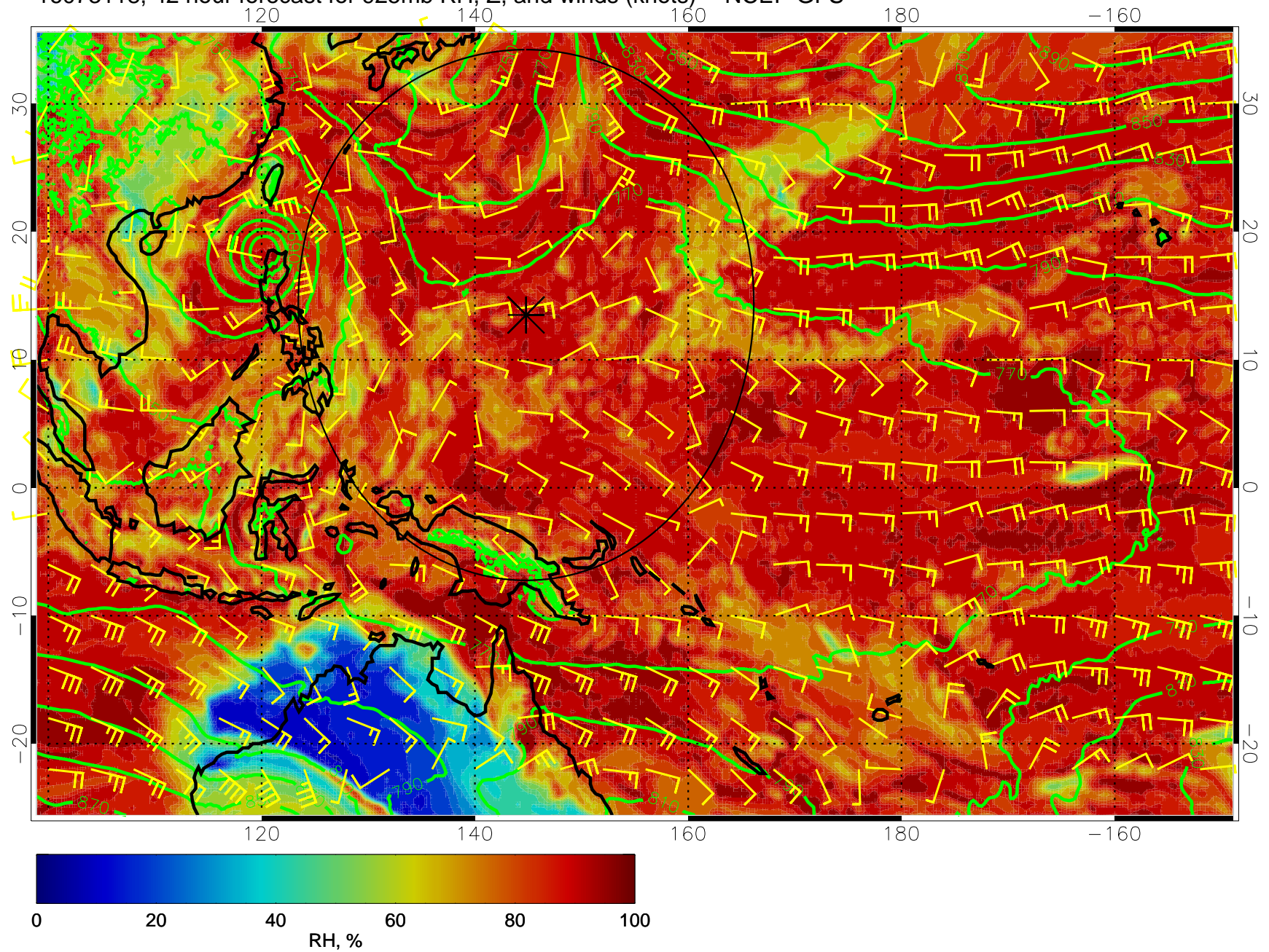
16073118, 42 hour forecast for 925mb RH, Z, and winds (knots) -- NCEP GFS
