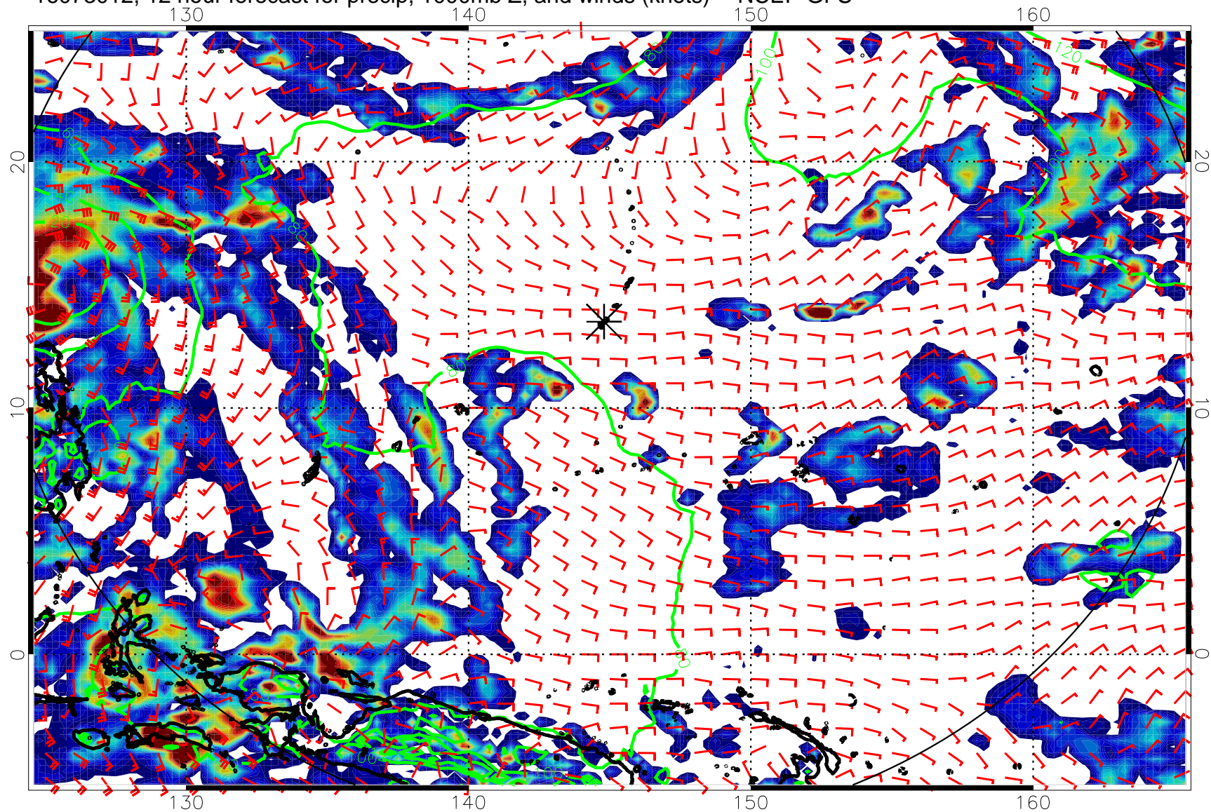
16073012, 12 hour forecast for precip, 1000mb Z, and winds (knots) -- NCEP GFS
