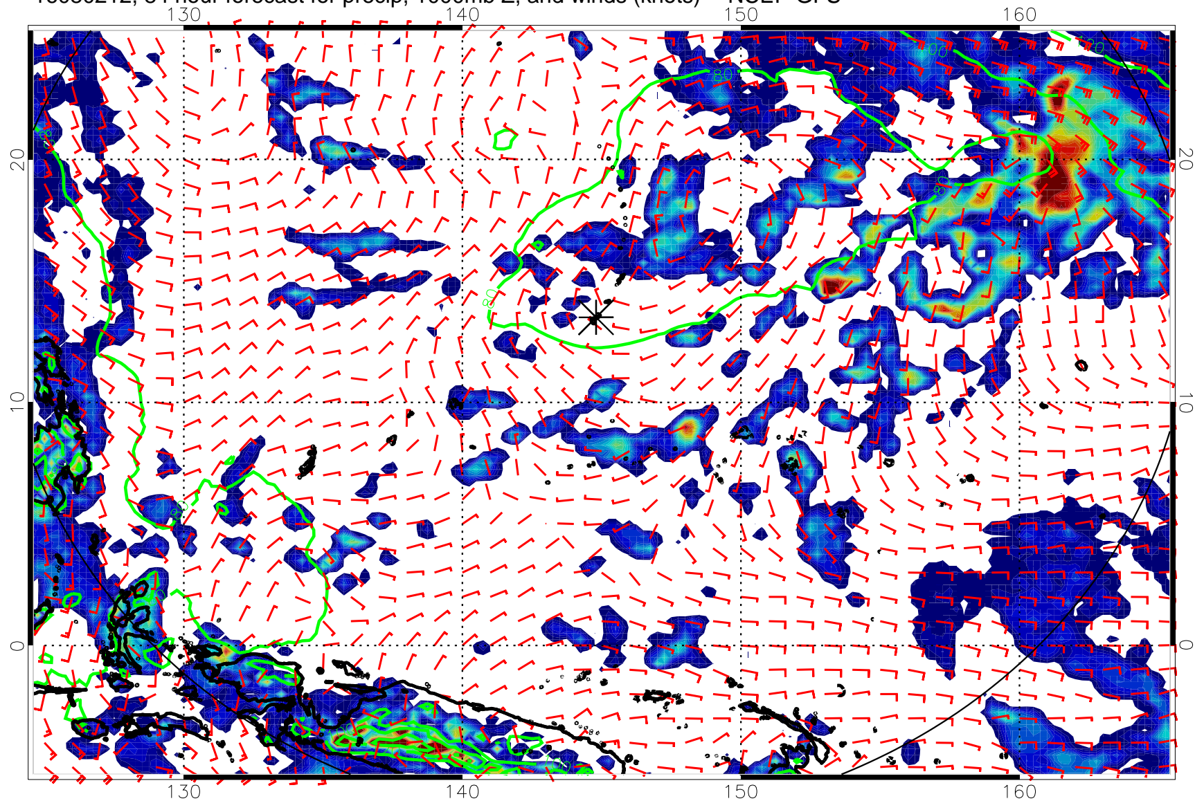
16080212, 84 hour forecast for precip, 1000mb Z, and winds (knots) -- NCEP GFS
