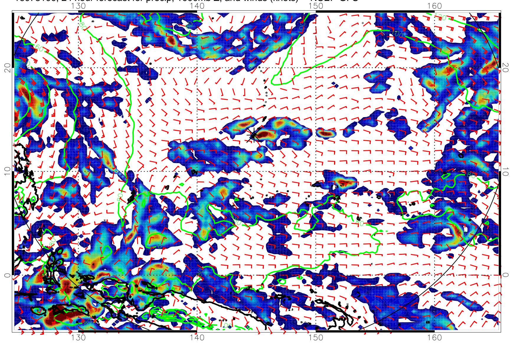
16073100, 24 hour forecast for precip, 1000mb Z, and winds (knots) -- NCEP GFS
