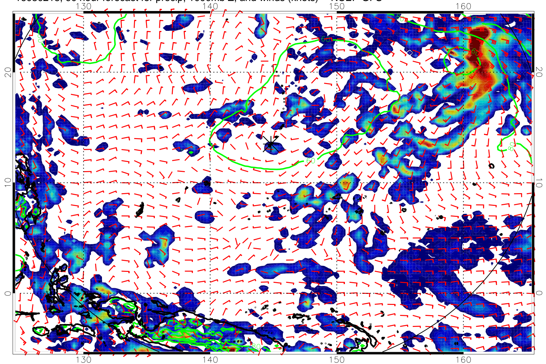
16080218, 90 hour forecast for precip, 1000mb Z, and winds (knots) -- NCEP GFS
