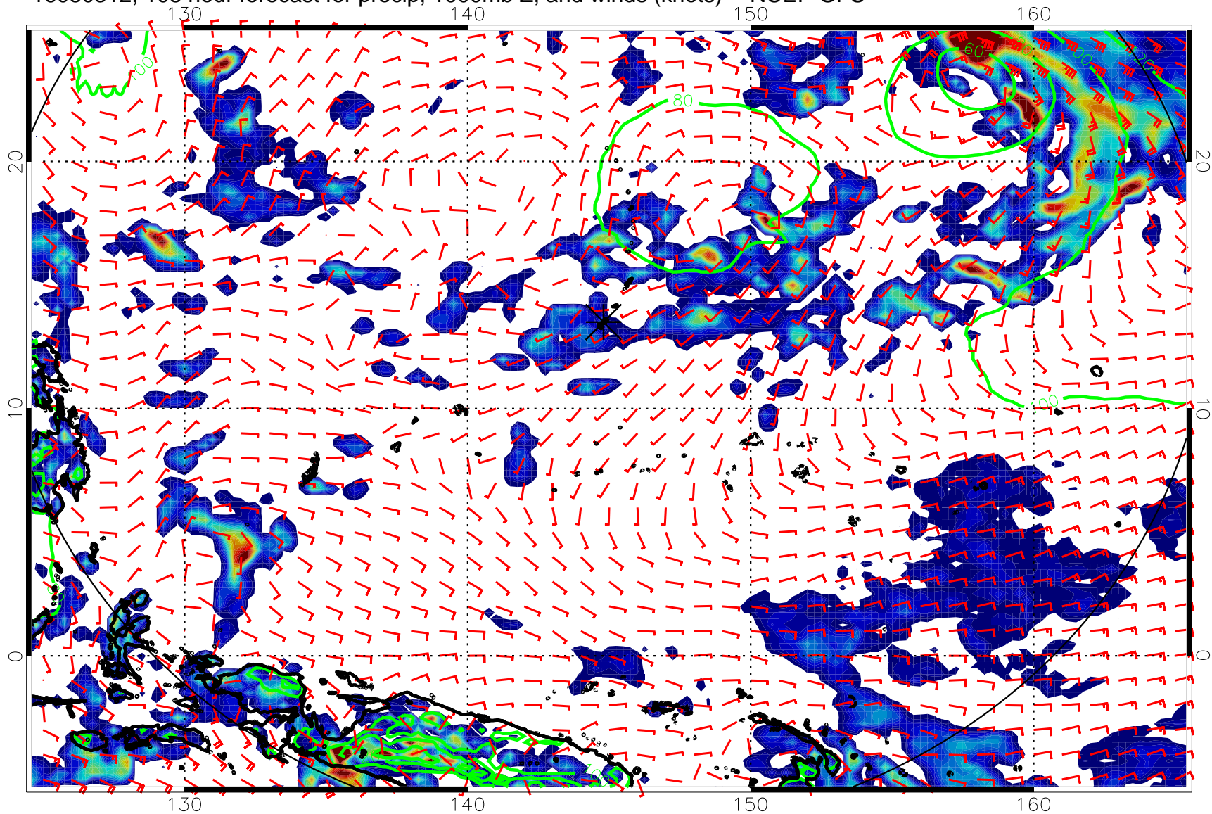
16080312, 108 hour forecast for precip, 1000mb Z, and winds (knots) -- NCEP GFS
