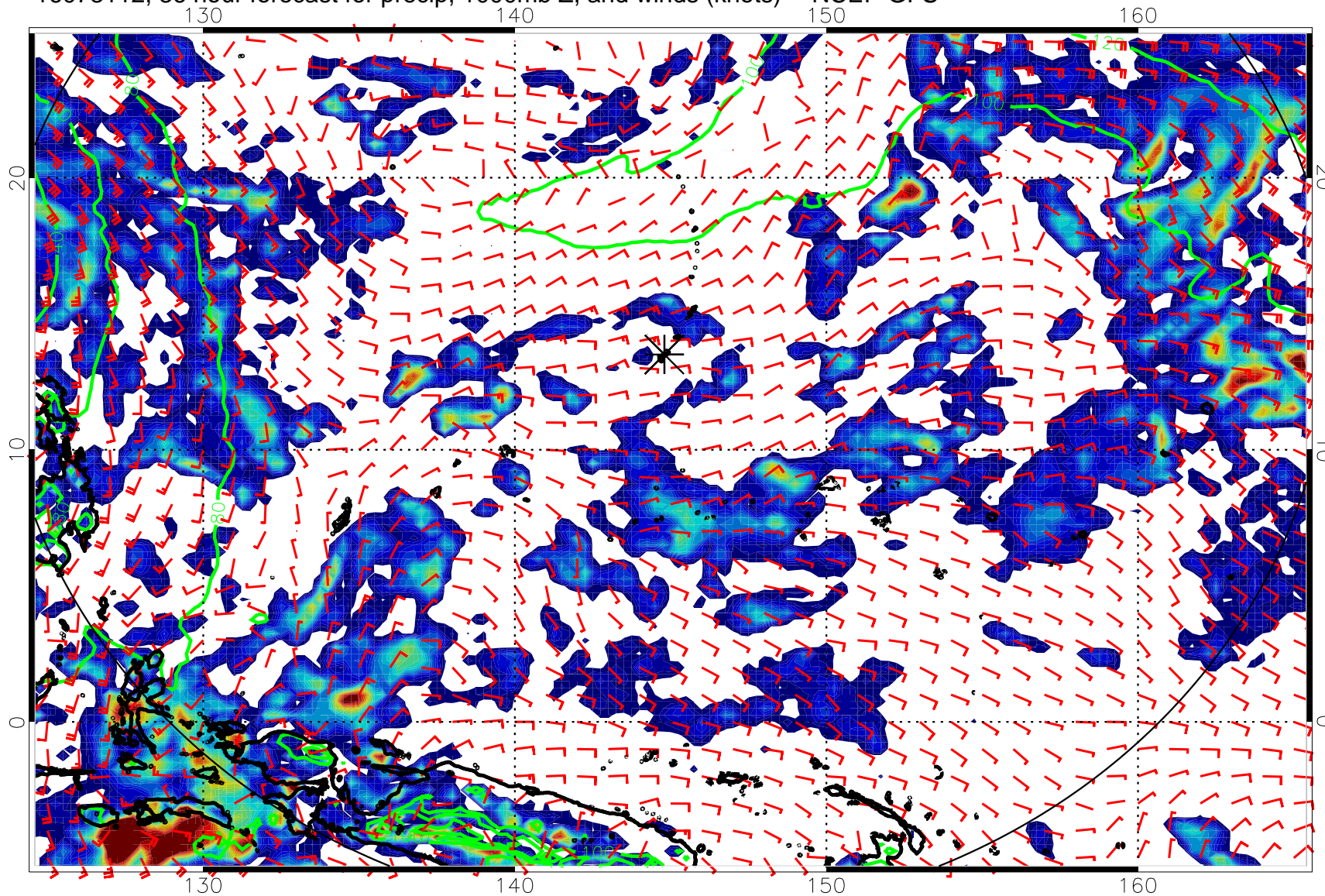
16073112, 36 hour forecast for precip, 1000mb Z, and winds (knots) -- NCEP GFS
