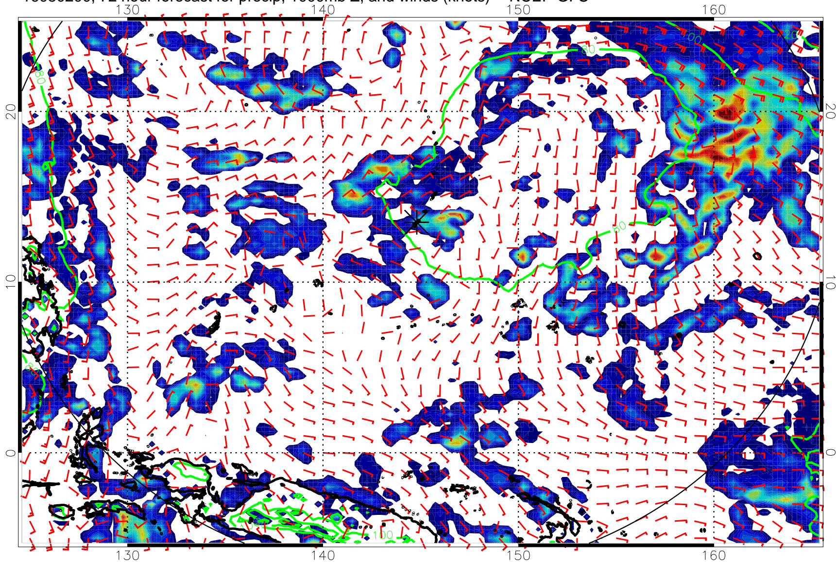
16080200, 72 hour forecast for precip, 1000mb Z, and winds (knots) -- NCEP GFS
