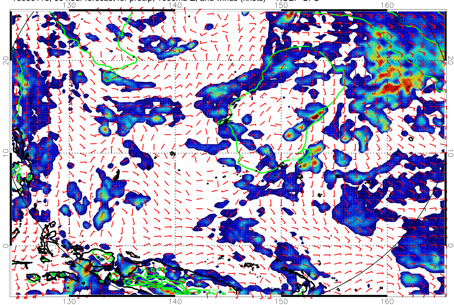
16080118, 66 hour forecast for precip, 1000mb Z, and winds (knots) -- NCEP GFS
