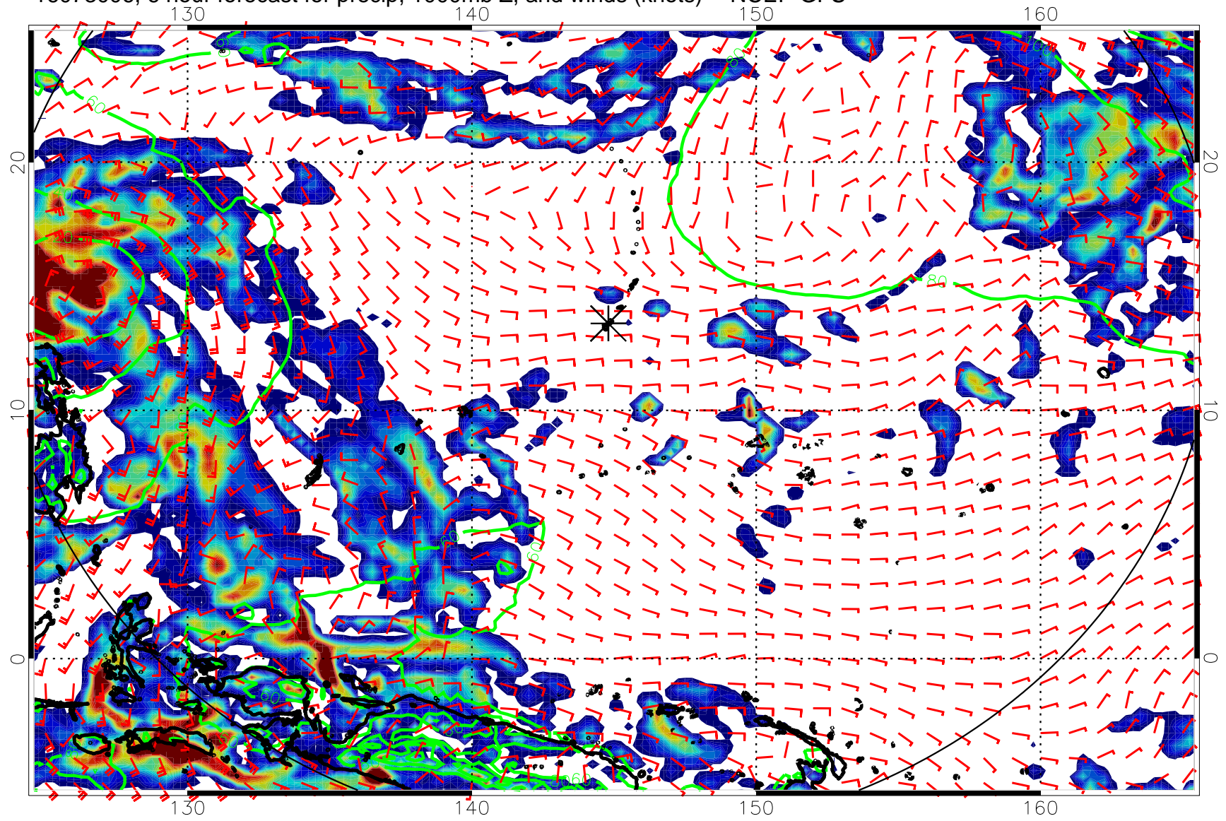
16073006, 6 hour forecast for precip, 1000mb Z, and winds (knots) -- NCEP GFS
