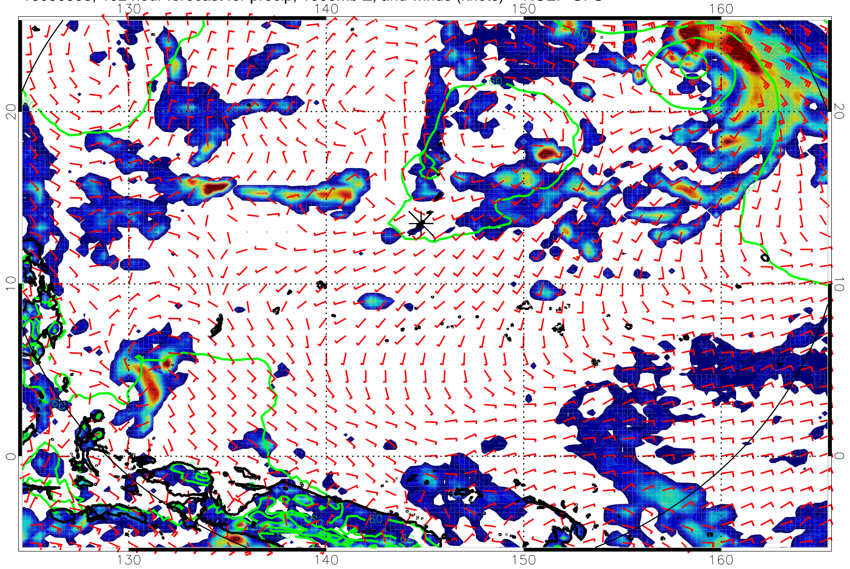
16080306, 102 hour forecast for precip, 1000mb Z, and winds (knots) -- NCEP GFS
