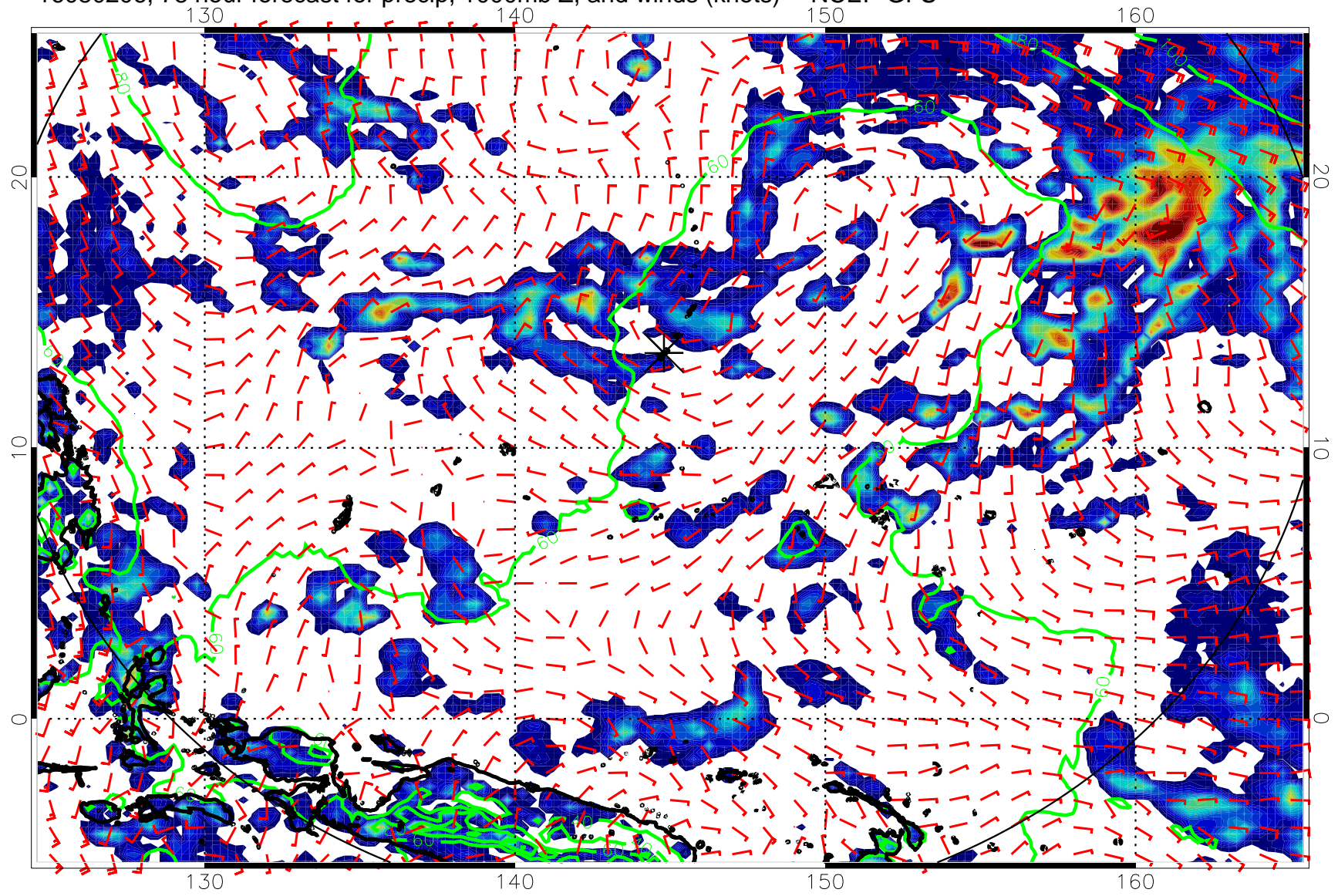
16080206, 78 hour forecast for precip, 1000mb Z, and winds (knots) -- NCEP GFS
