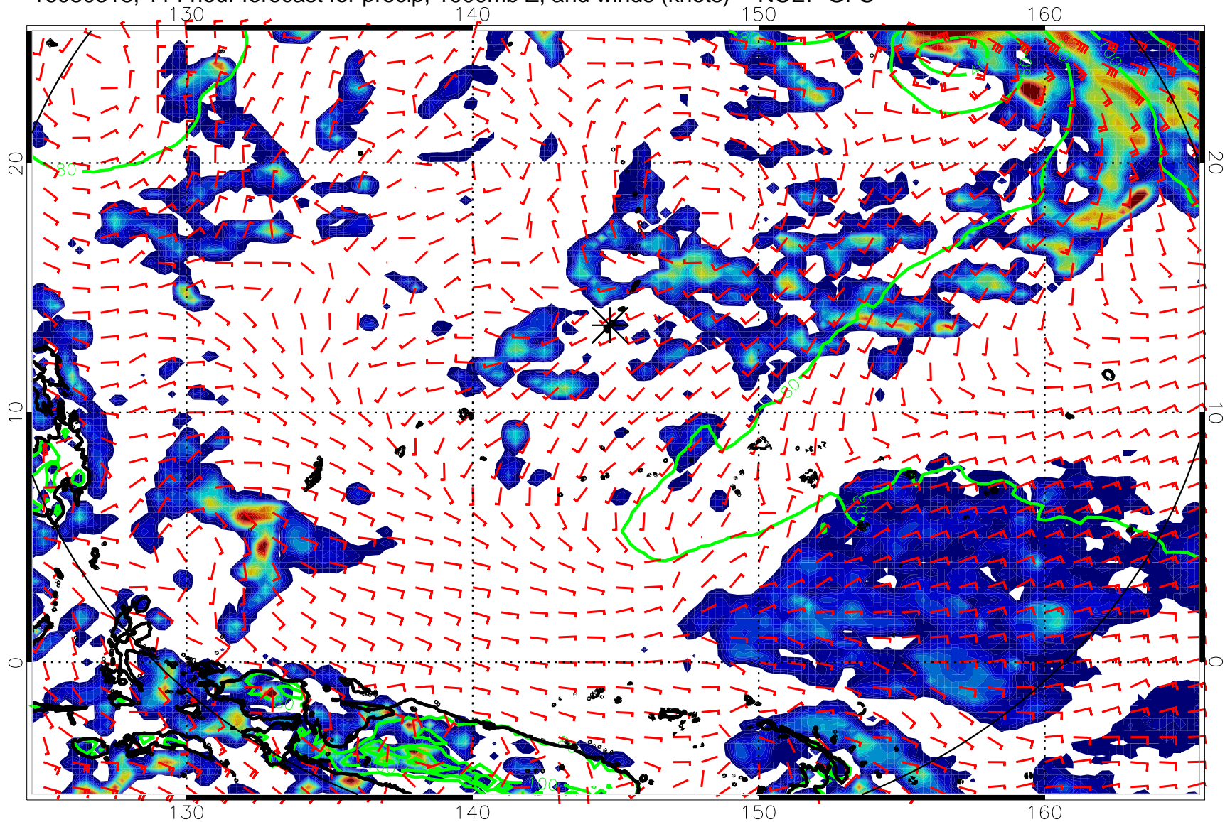
16080318, 114 hour forecast for precip, 1000mb Z, and winds (knots) -- NCEP GFS
