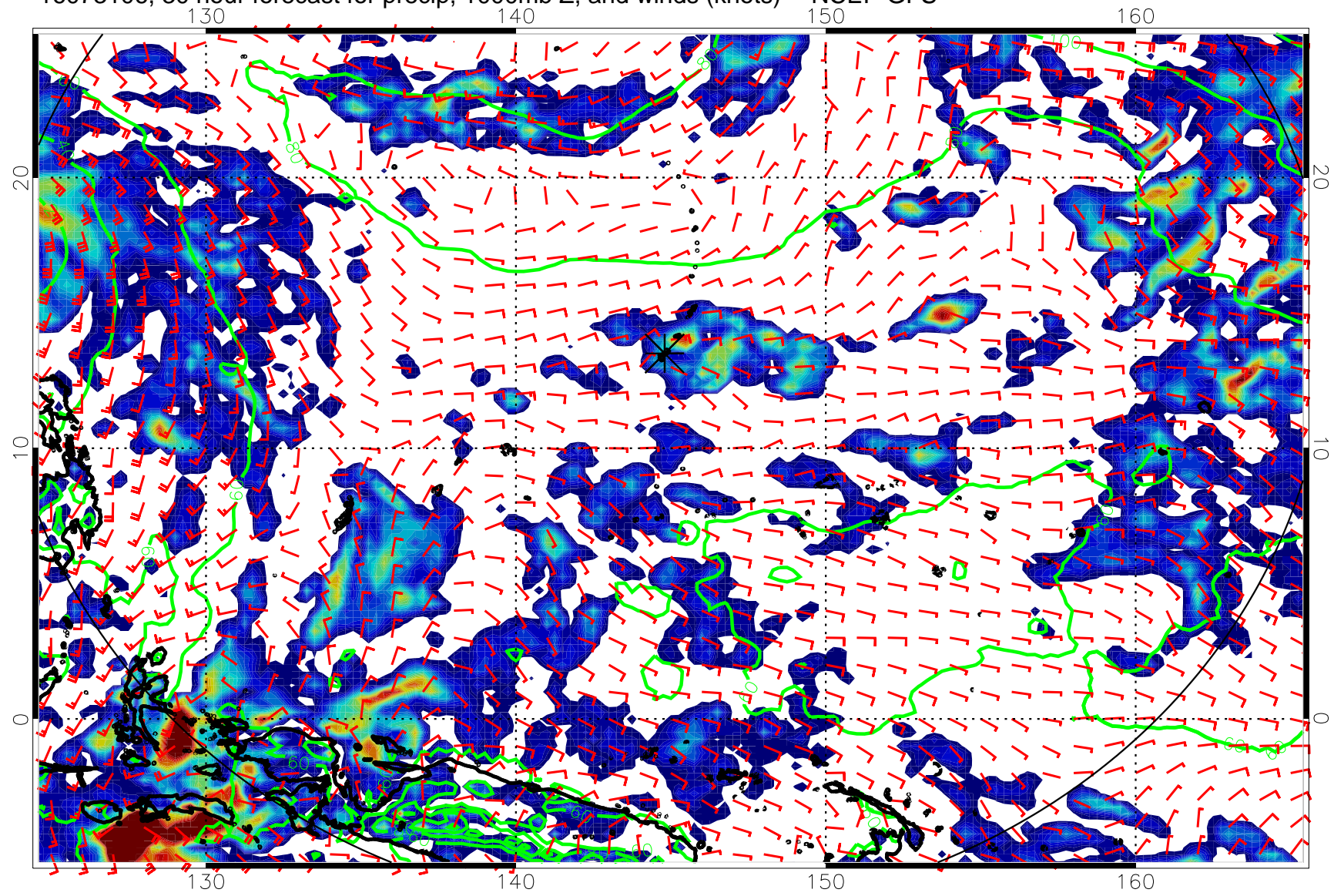
16073106, 30 hour forecast for precip, 1000mb Z, and winds (knots) -- NCEP GFS
