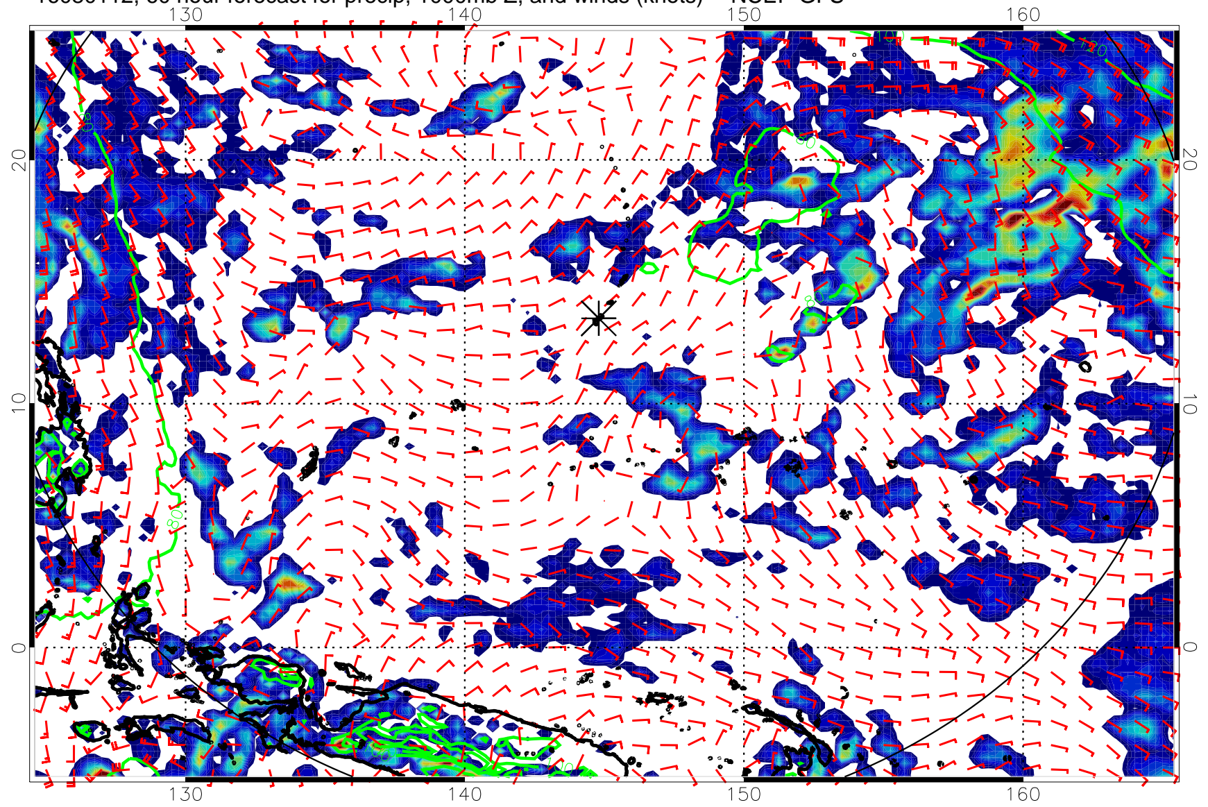
16080112, 60 hour forecast for precip, 1000mb Z, and winds (knots) -- NCEP GFS
