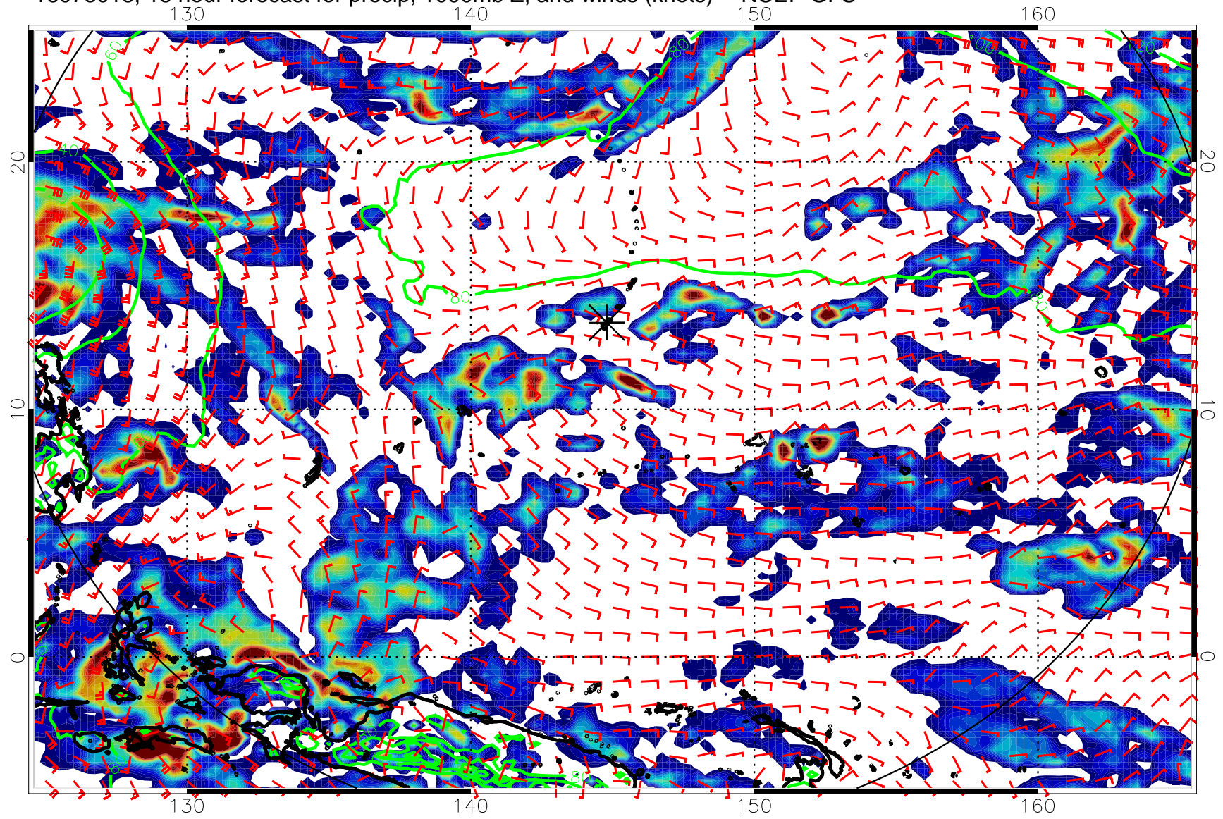
16073018, 18 hour forecast for precip, 1000mb Z, and winds (knots) -- NCEP GFS
