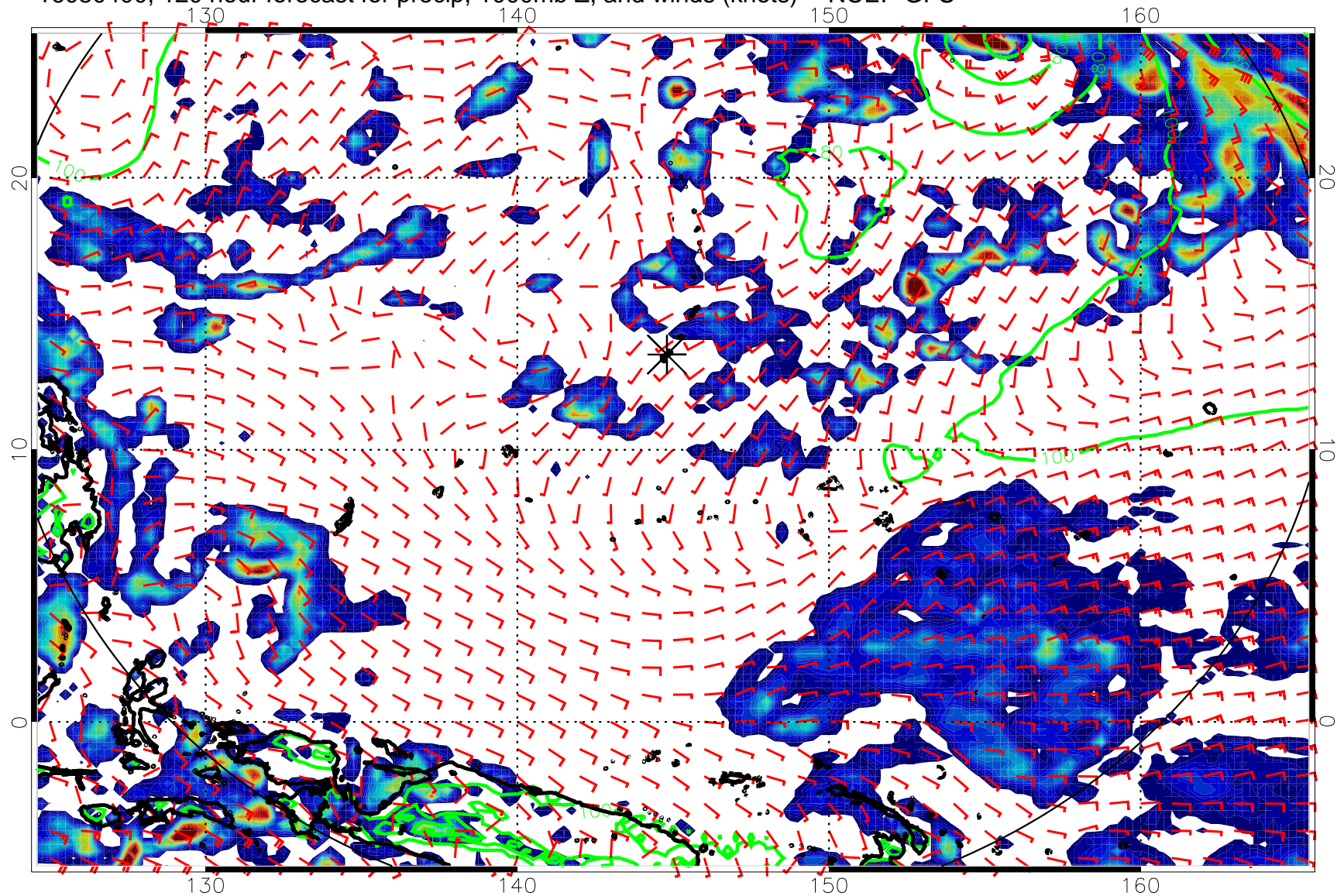
16080400, 120 hour forecast for precip, 1000mb Z, and winds (knots) -- NCEP GFS
