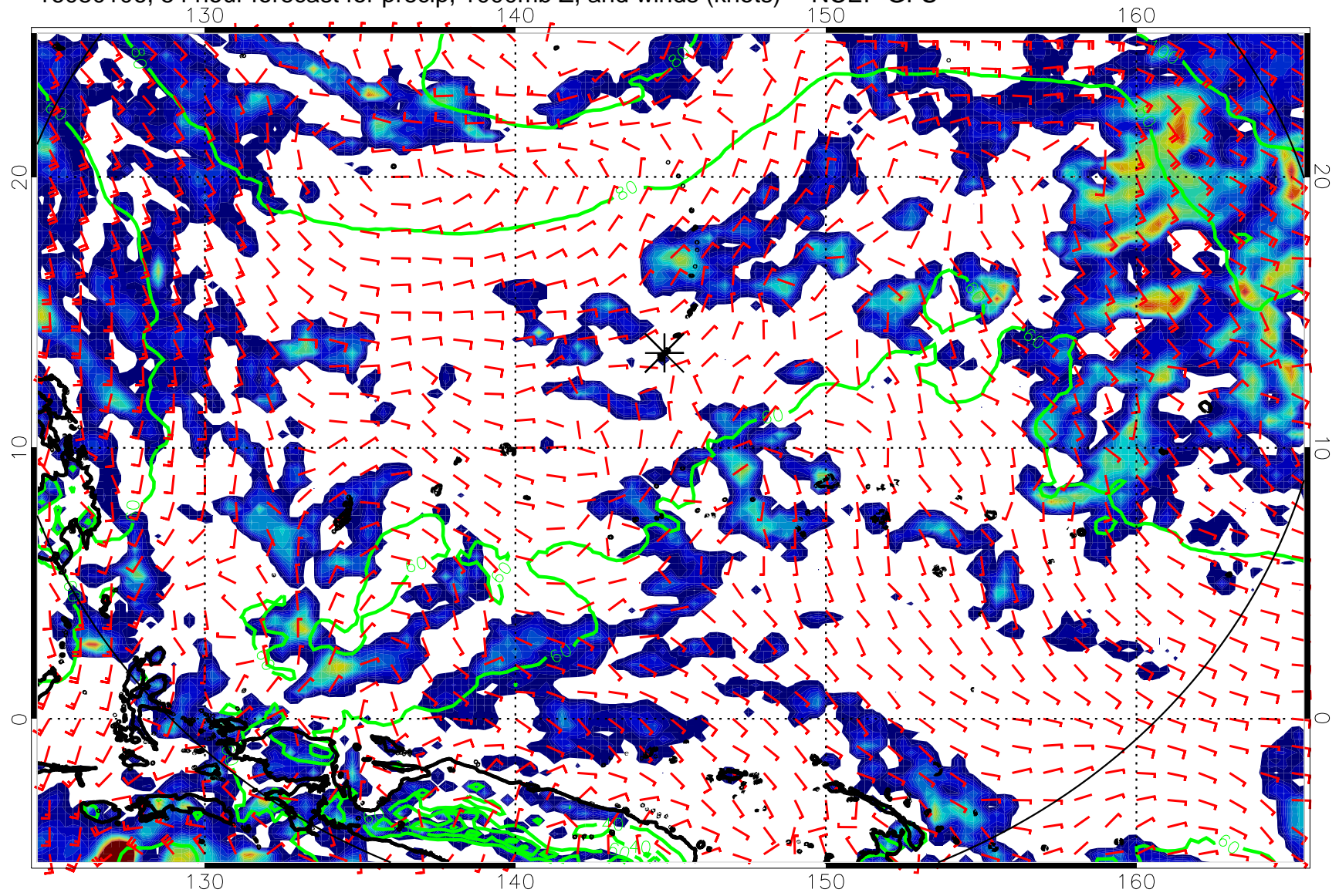
16080106, 54 hour forecast for precip, 1000mb Z, and winds (knots) -- NCEP GFS
