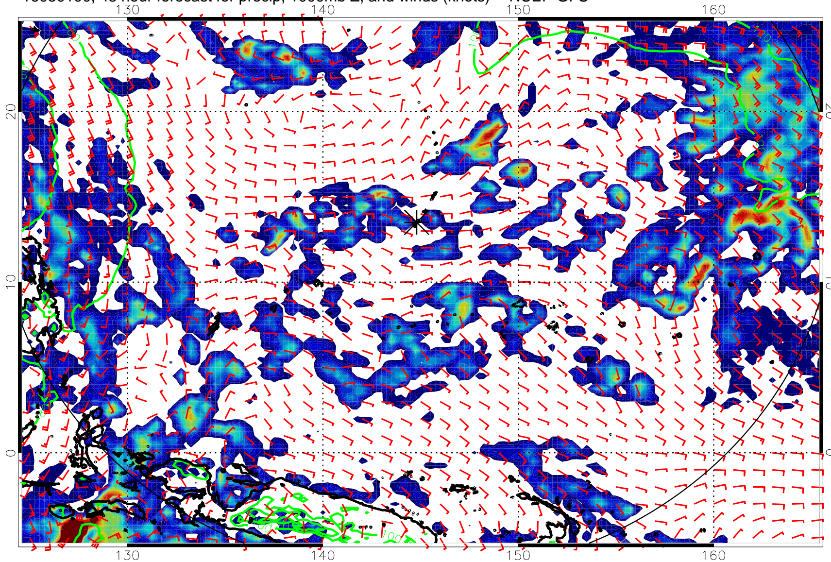
16080100, 48 hour forecast for precip, 1000mb Z, and winds (knots) -- NCEP GFS
