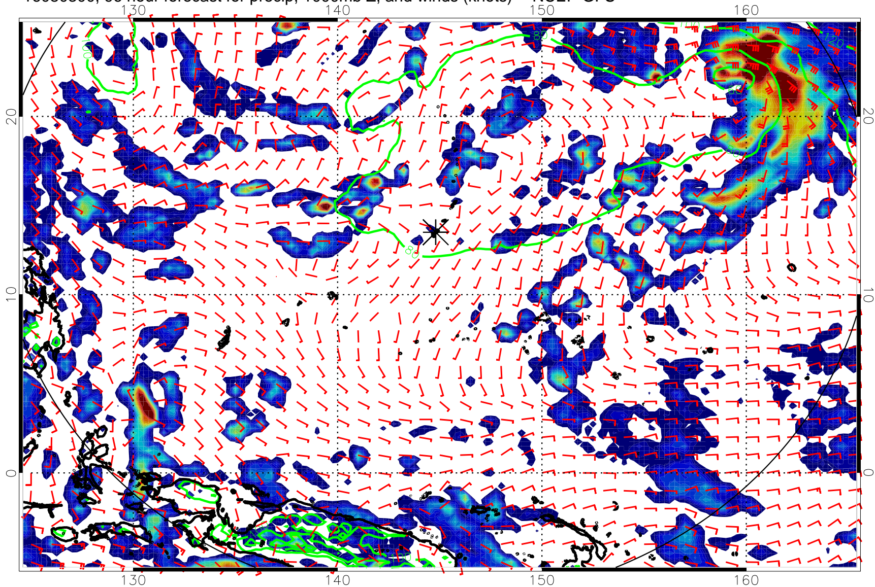
16080300, 96 hour forecast for precip, 1000mb Z, and winds (knots) -- NCEP GFS
