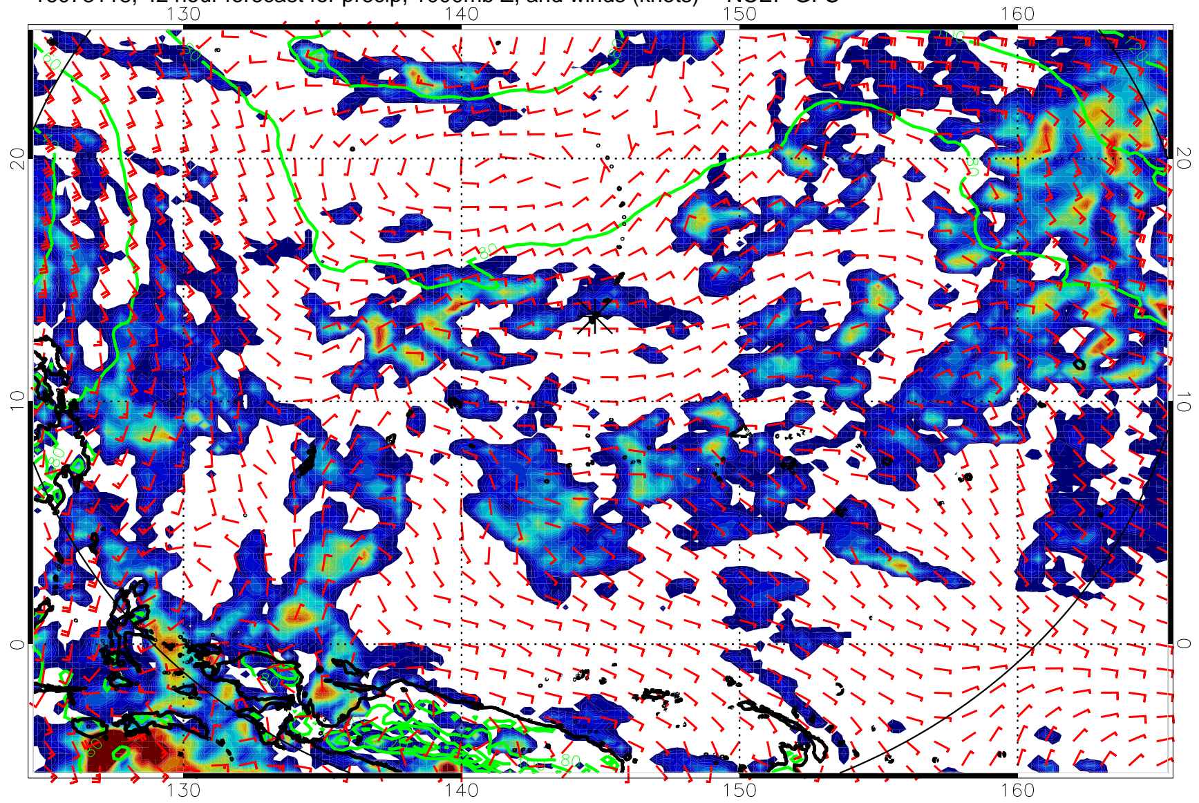
16073118, 42 hour forecast for precip, 1000mb Z, and winds (knots) -- NCEP GFS
