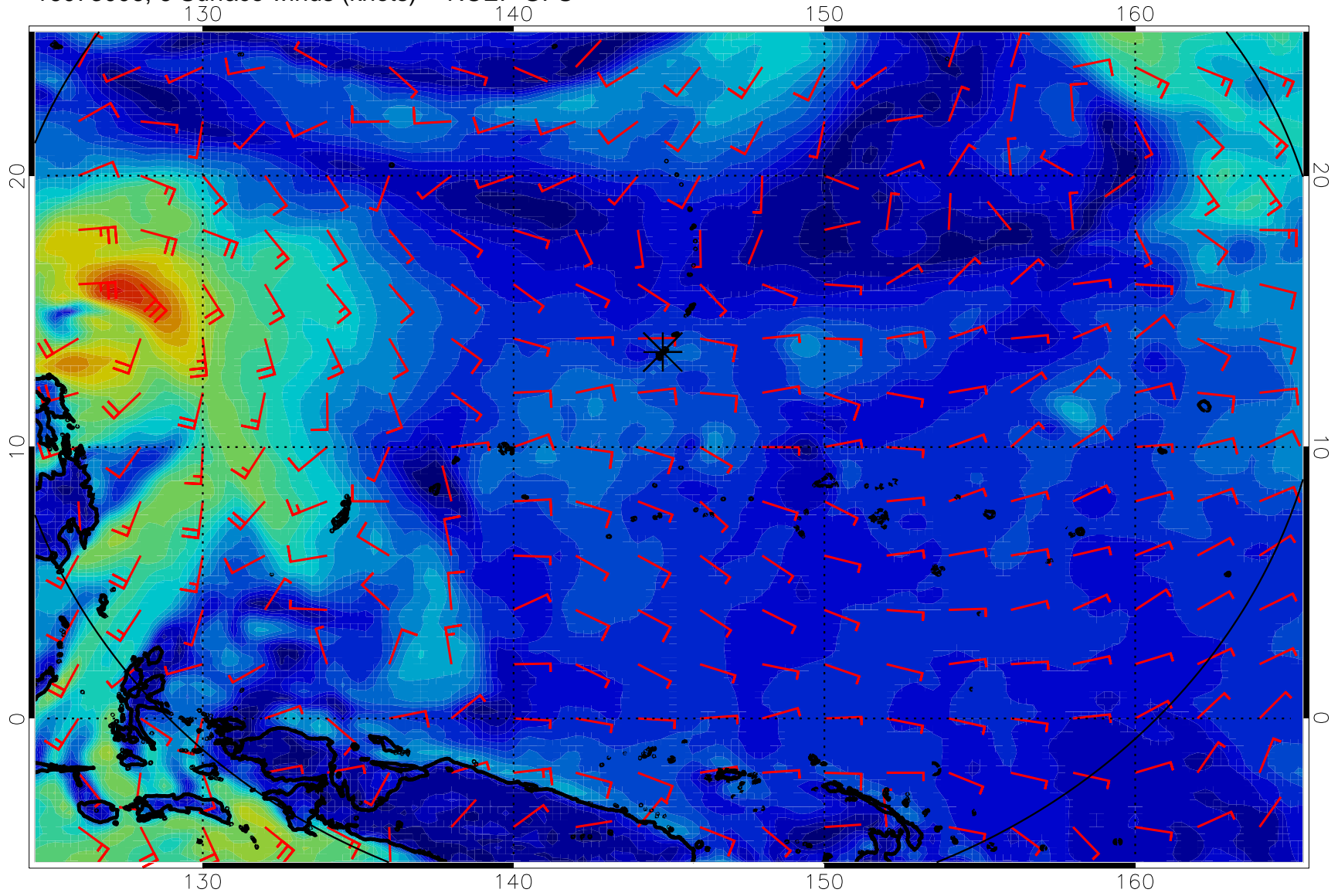
16073006, 6 Surface winds (knots) -- NCEP GFS
