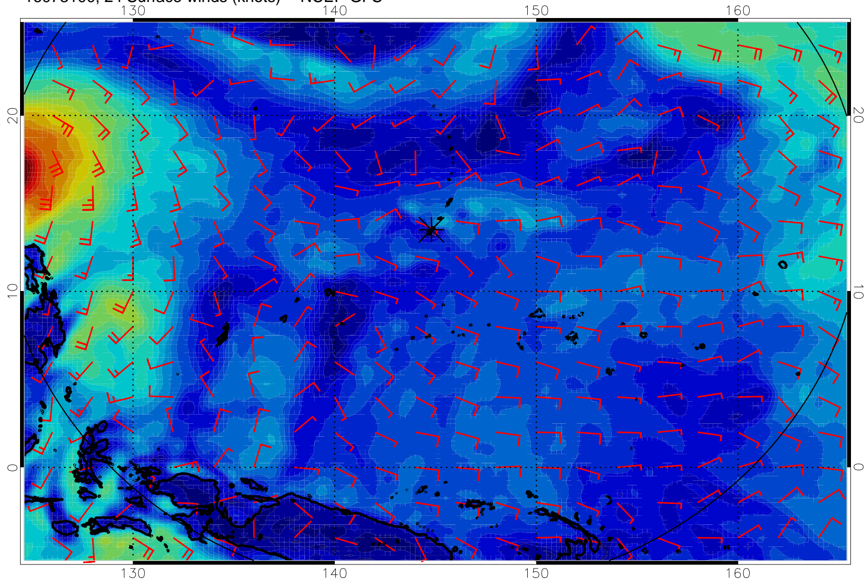
16073100, 24 Surface winds (knots) -- NCEP GFS
