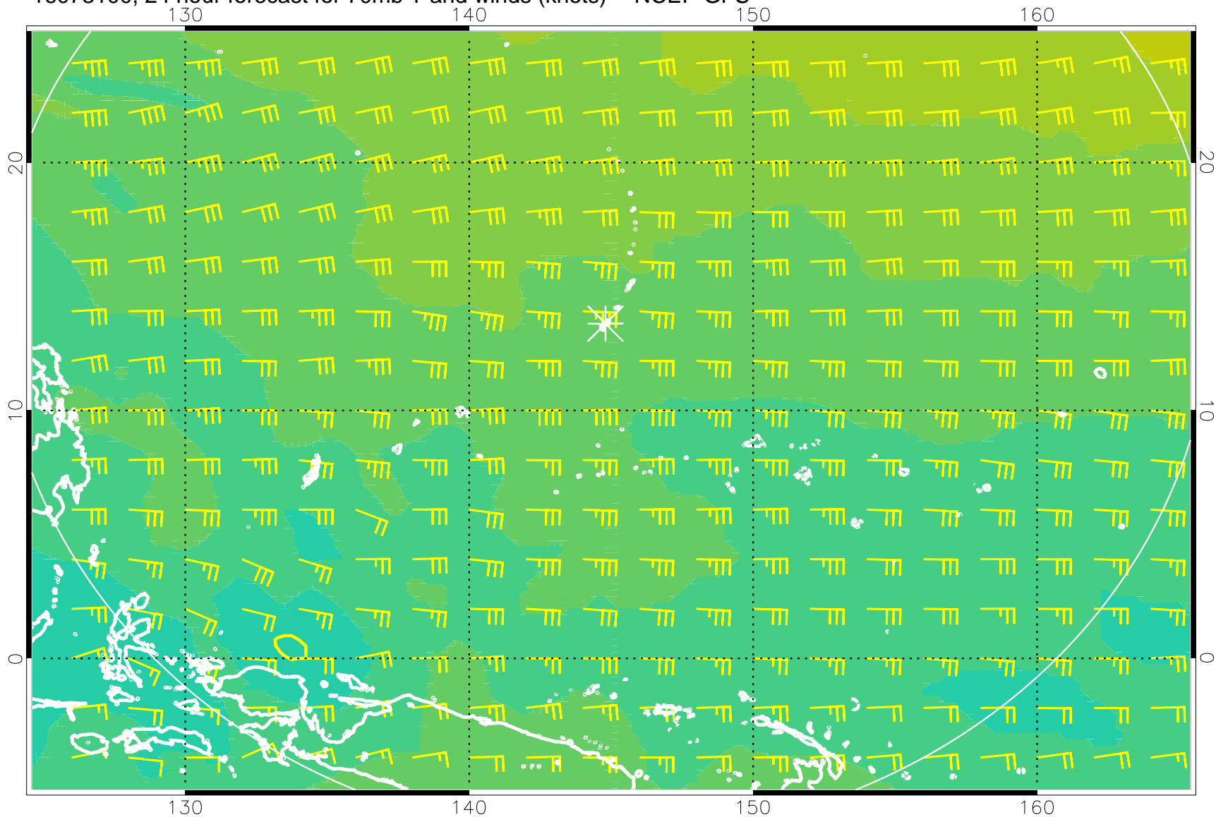
16073100, 24 hour forecast for 70mb T and winds (knots) -- NCEP GFS
