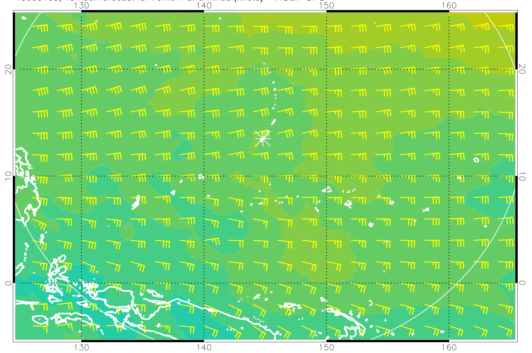
16080100, 48 hour forecast for 70mb T and winds (knots) -- NCEP GFS
