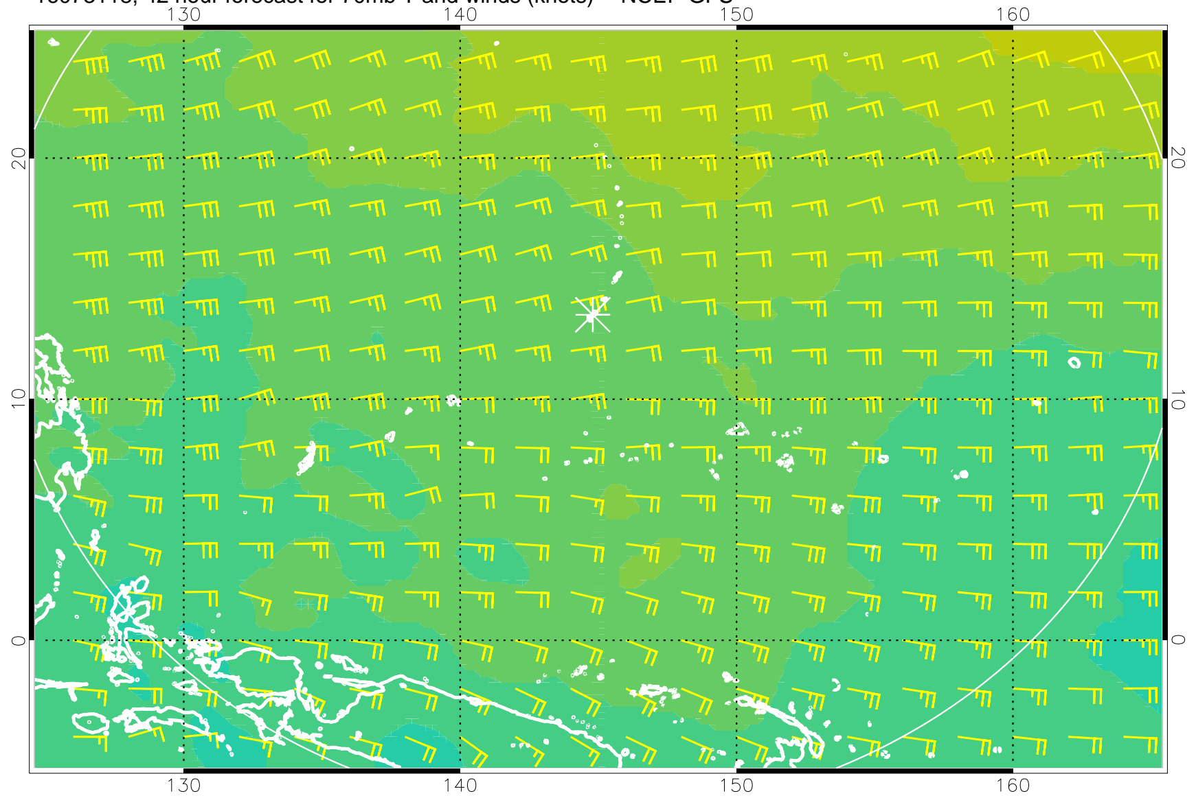
16073118, 42 hour forecast for 70mb T and winds (knots) -- NCEP GFS
