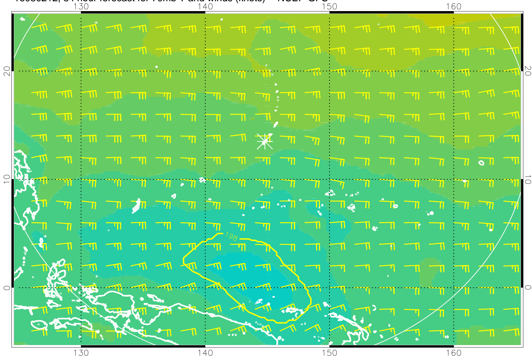
16080212, 84 hour forecast for 70mb T and winds (knots) -- NCEP GFS
