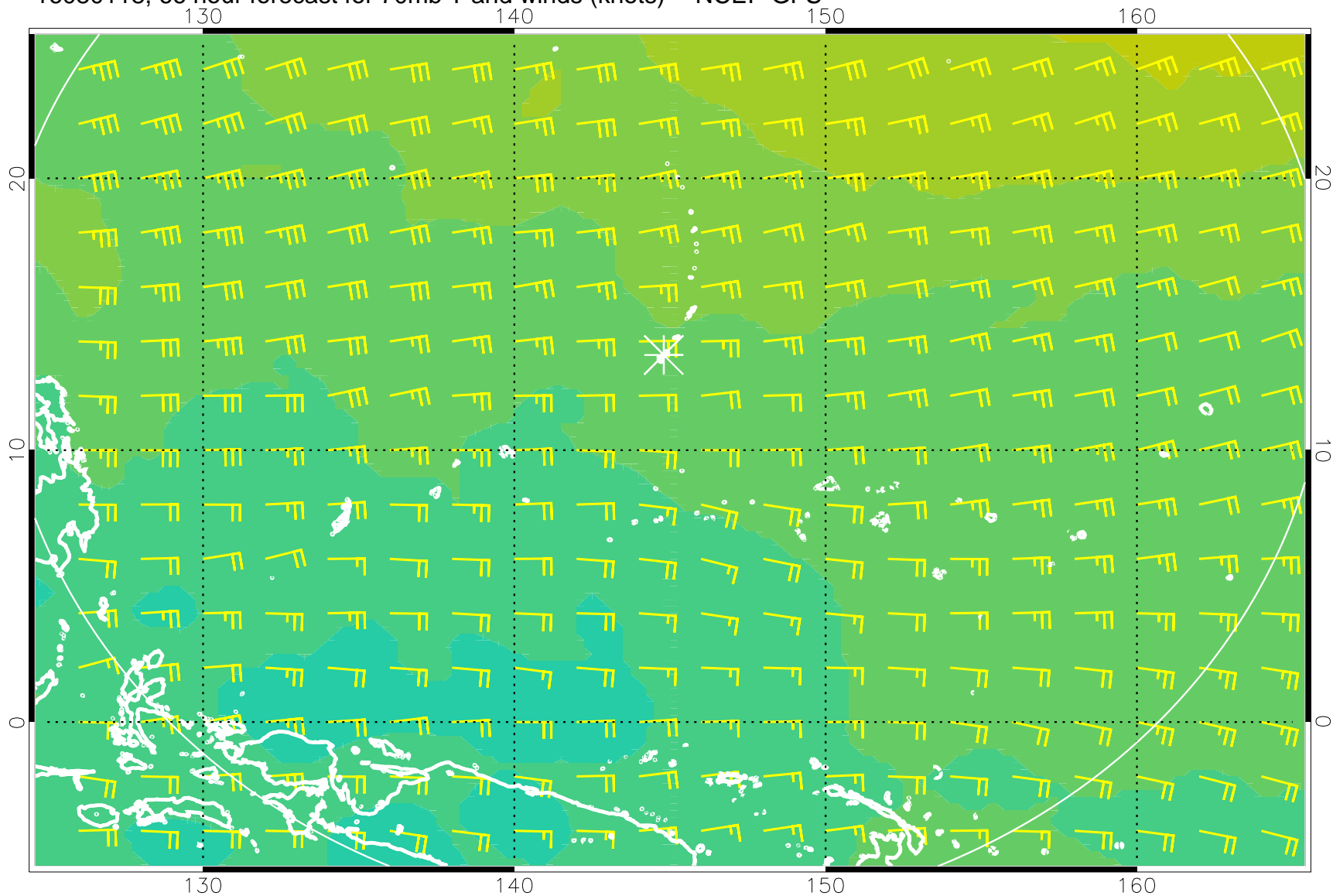
16080118, 66 hour forecast for 70mb T and winds (knots) -- NCEP GFS
