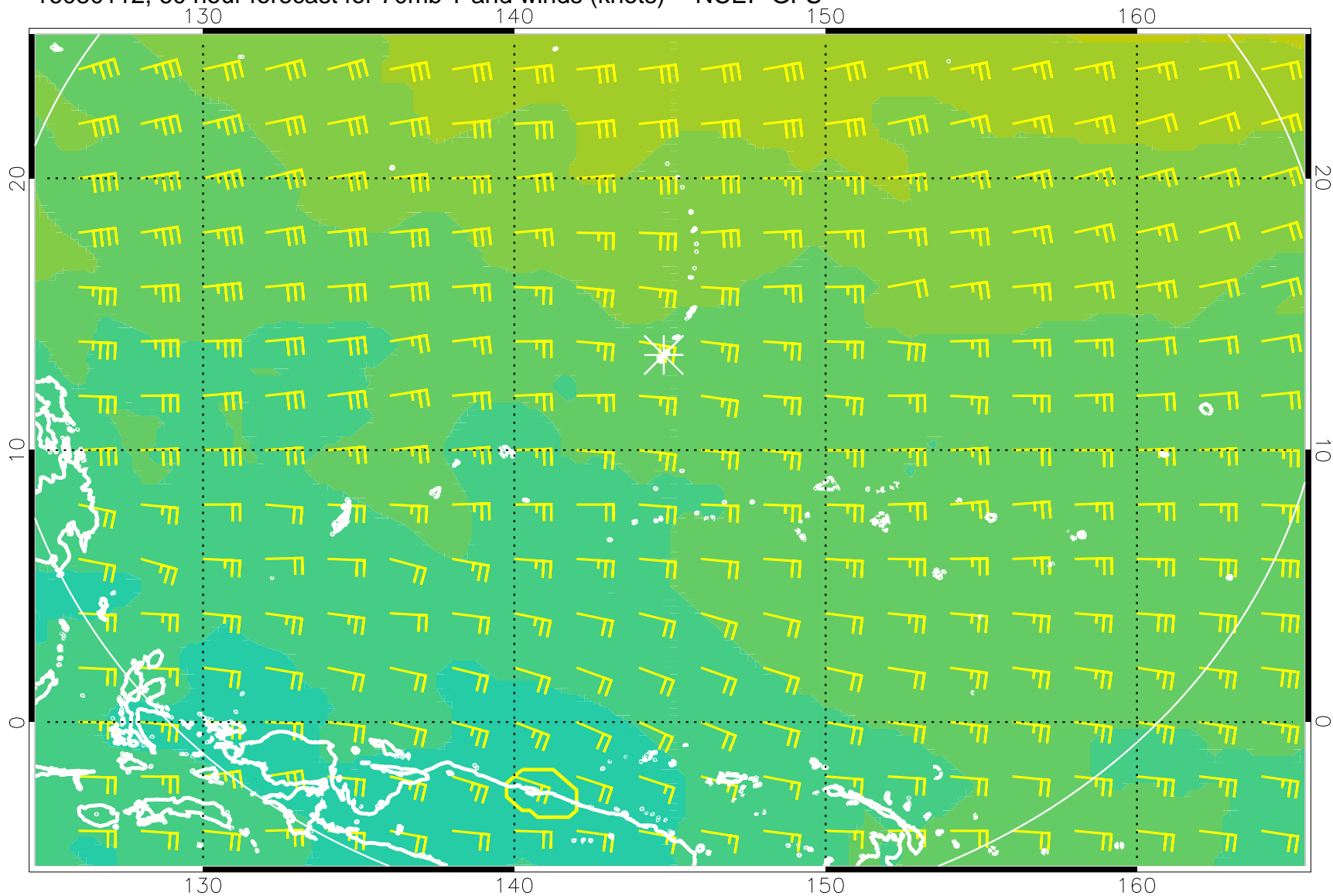
16080112, 60 hour forecast for 70mb T and winds (knots) -- NCEP GFS
