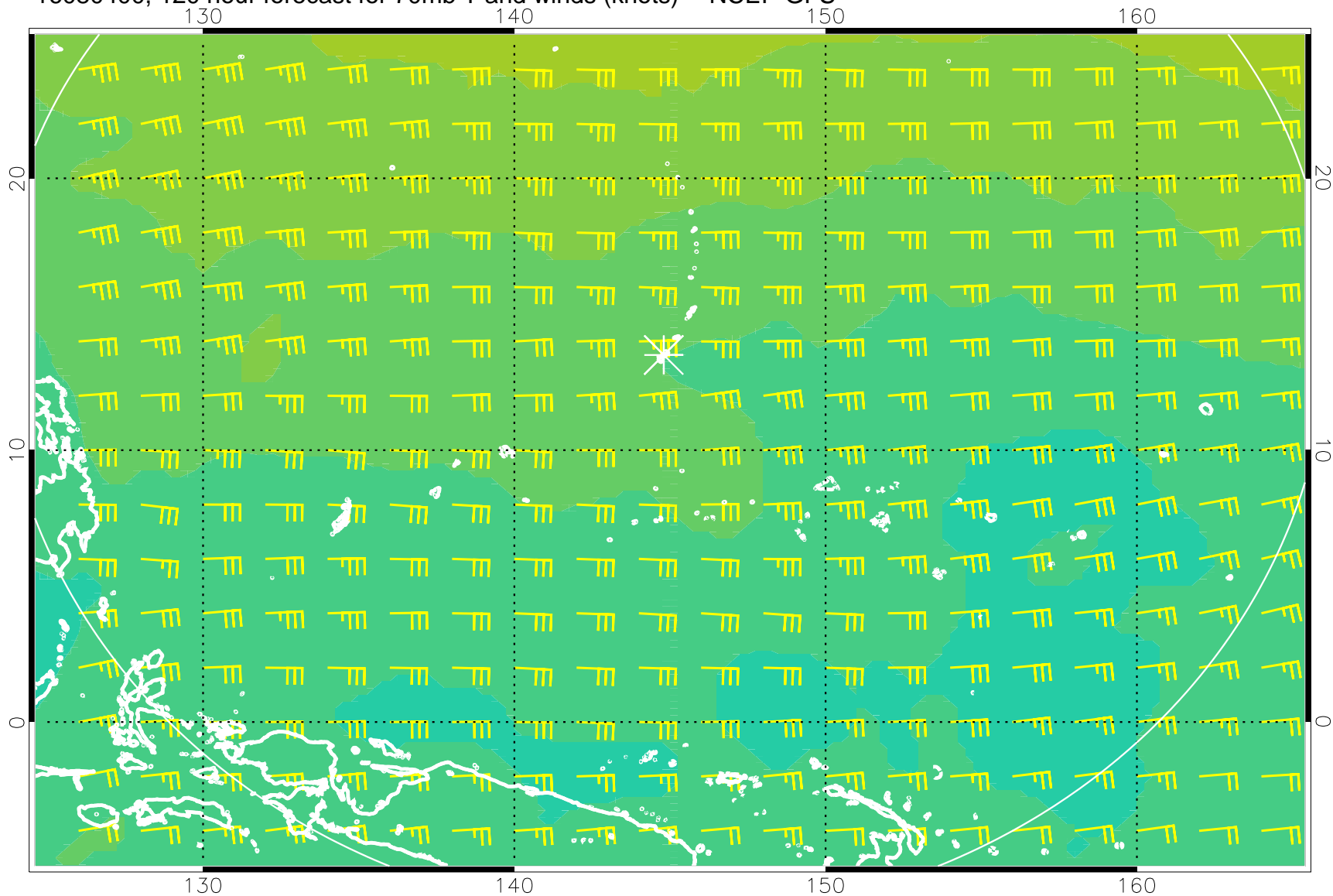
16080400, 120 hour forecast for 70mb T and winds (knots) -- NCEP GFS
