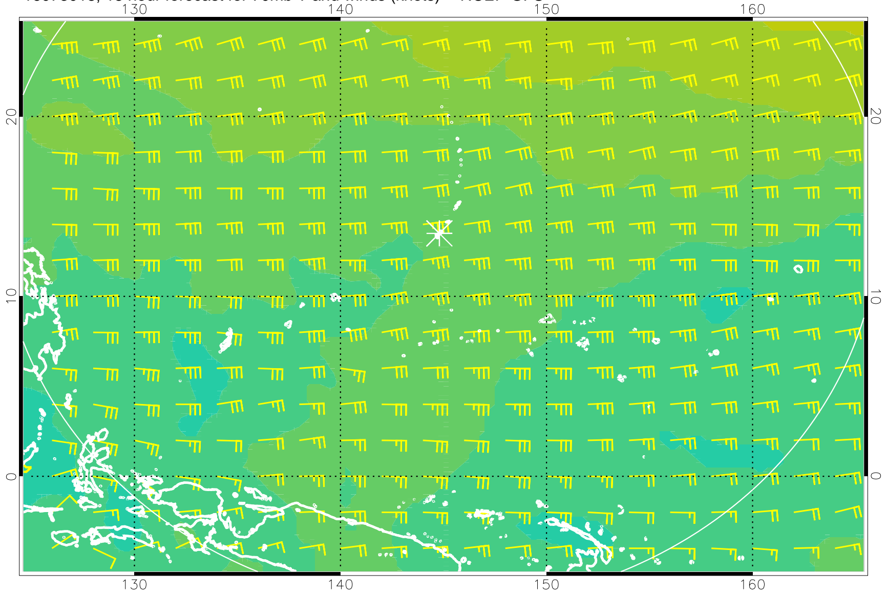
16073018, 18 hour forecast for 70mb T and winds (knots) -- NCEP GFS
