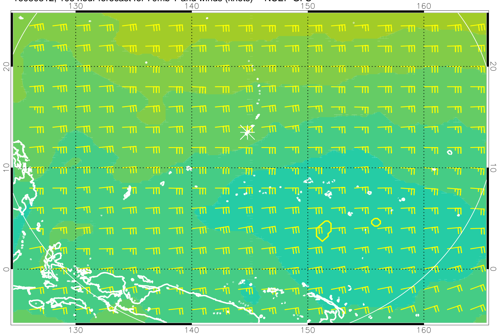
16080312, 108 hour forecast for 70mb T and winds (knots) -- NCEP GFS
