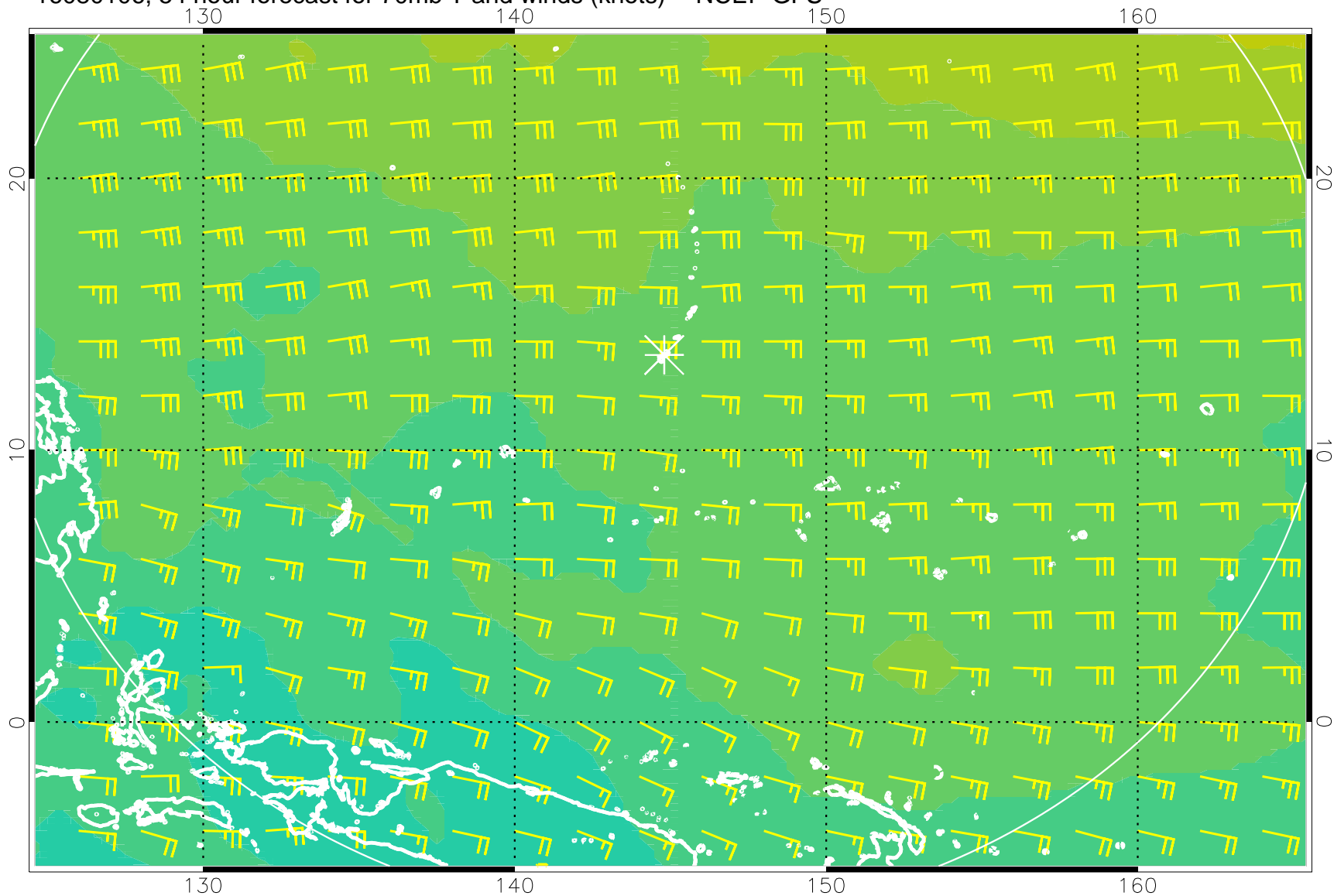
16080106, 54 hour forecast for 70mb T and winds (knots) -- NCEP GFS
