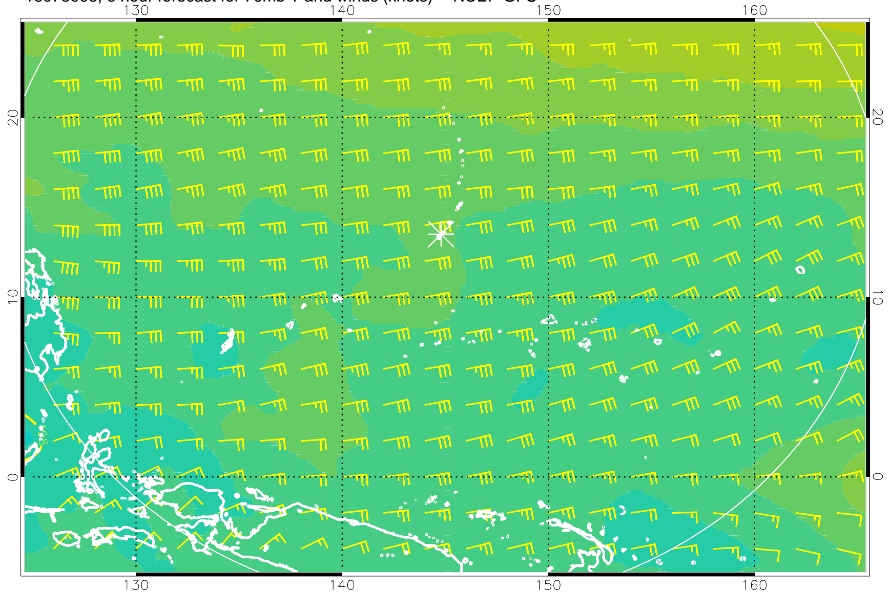
16073006, 6 hour forecast for 70mb T and winds (knots) -- NCEP GFS
