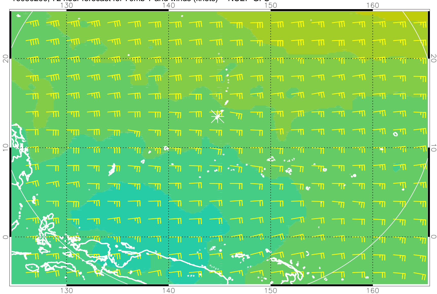
16080200, 72 hour forecast for 70mb T and winds (knots) -- NCEP GFS
