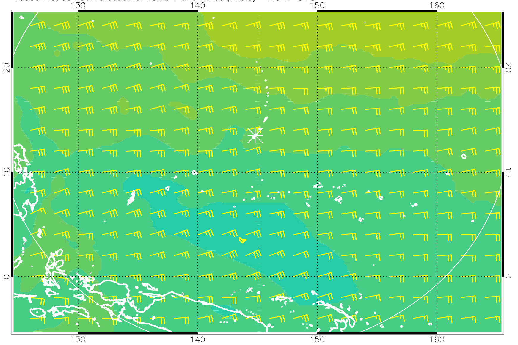
16080218, 90 hour forecast for 70mb T and winds (knots) -- NCEP GFS
