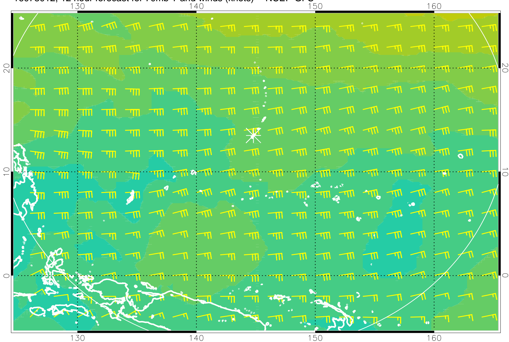
16073012, 12 hour forecast for 70mb T and winds (knots) -- NCEP GFS
