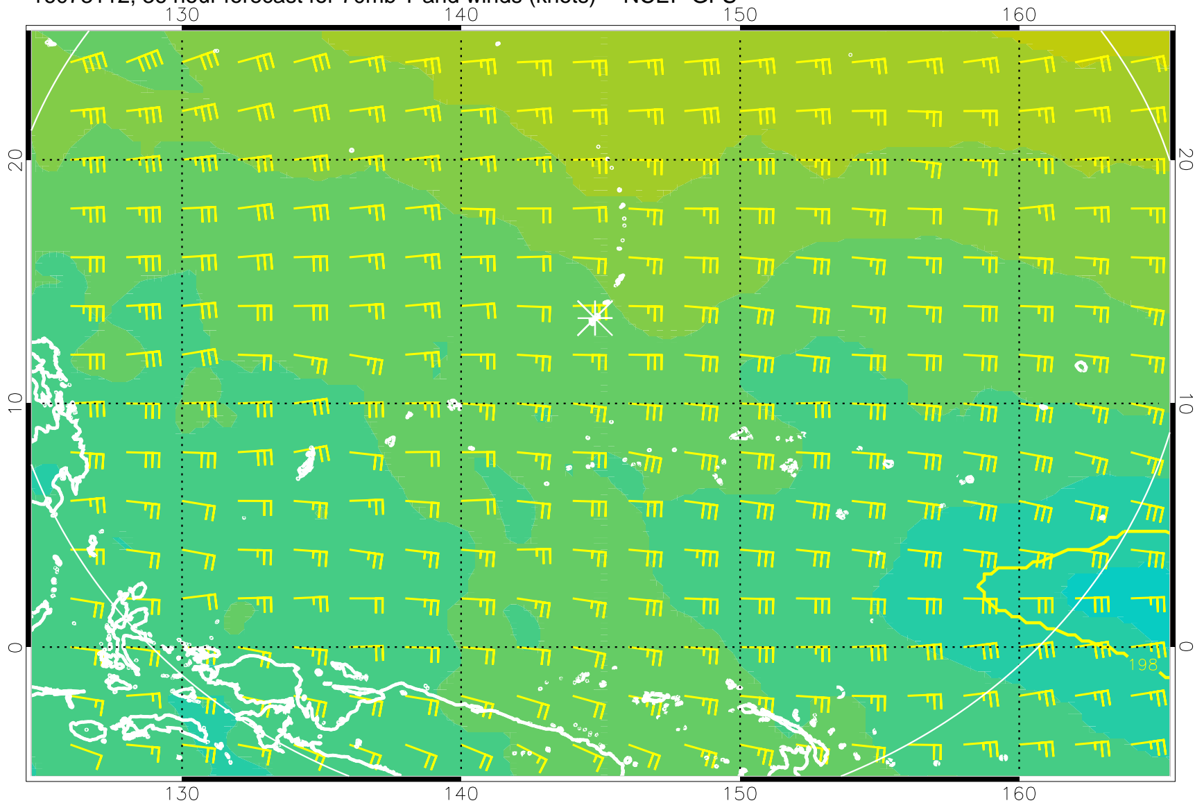
16073112, 36 hour forecast for 70mb T and winds (knots) -- NCEP GFS
