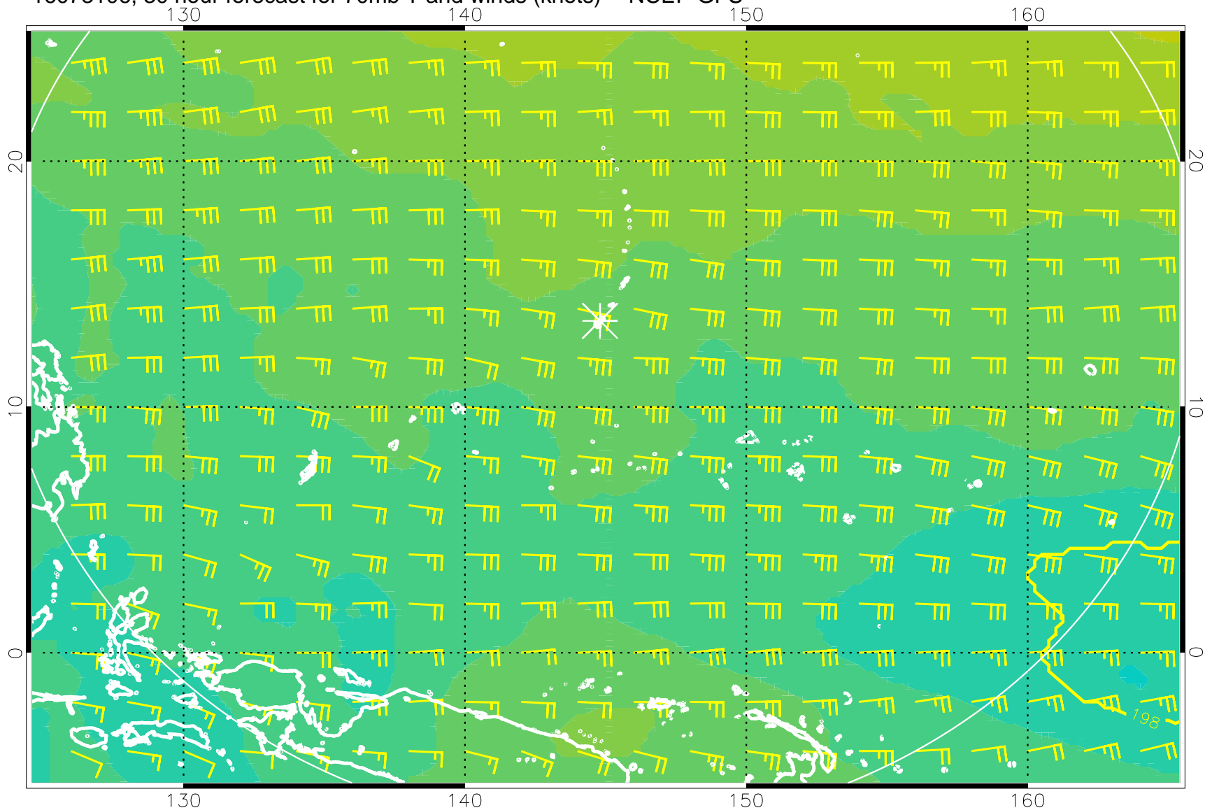
16073106, 30 hour forecast for 70mb T and winds (knots) -- NCEP GFS
