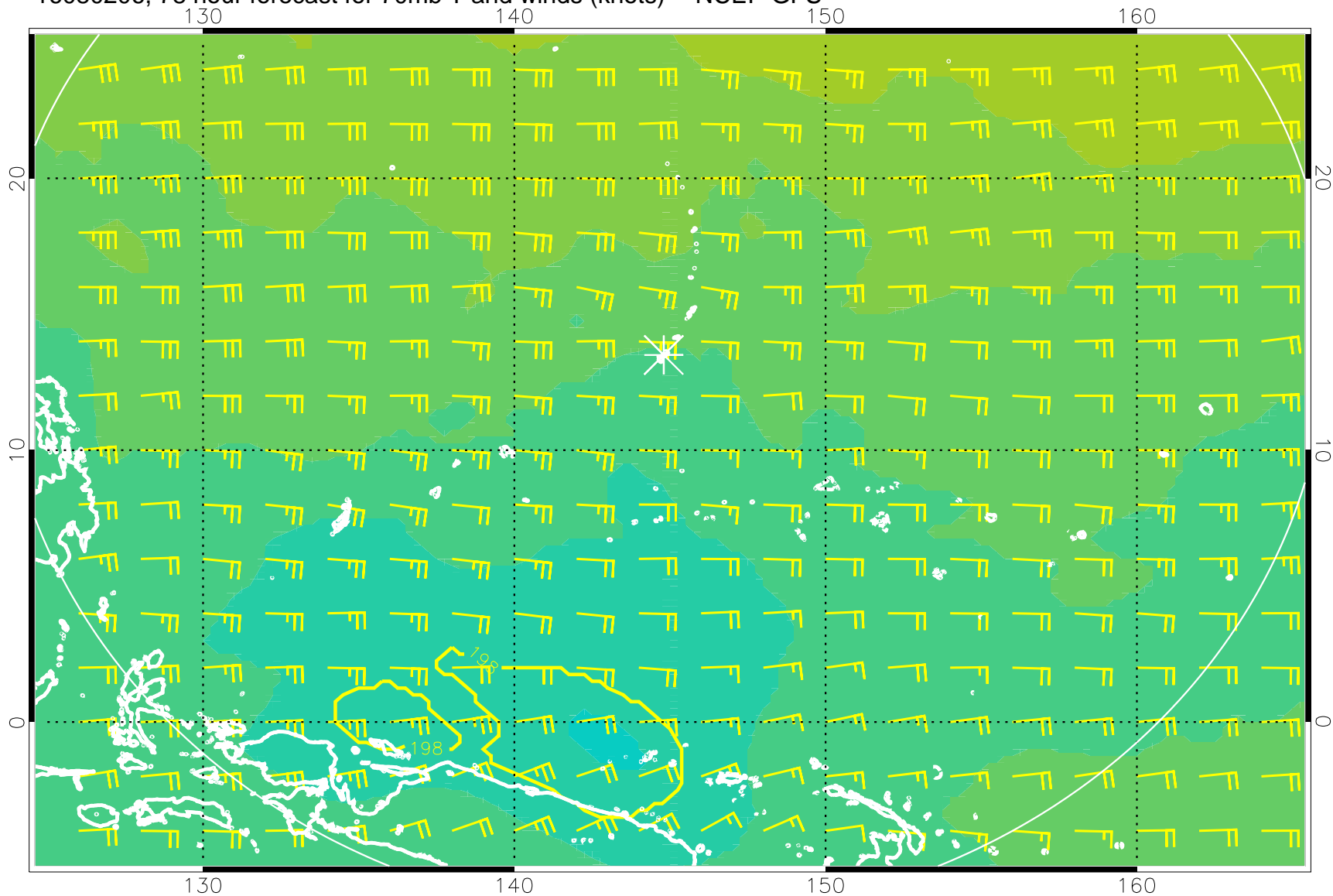
16080206, 78 hour forecast for 70mb T and winds (knots) -- NCEP GFS
