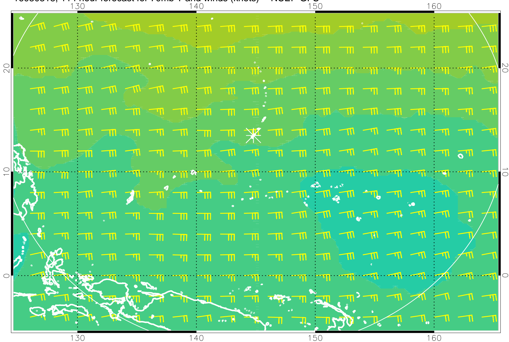
16080318, 114 hour forecast for 70mb T and winds (knots) -- NCEP GFS
