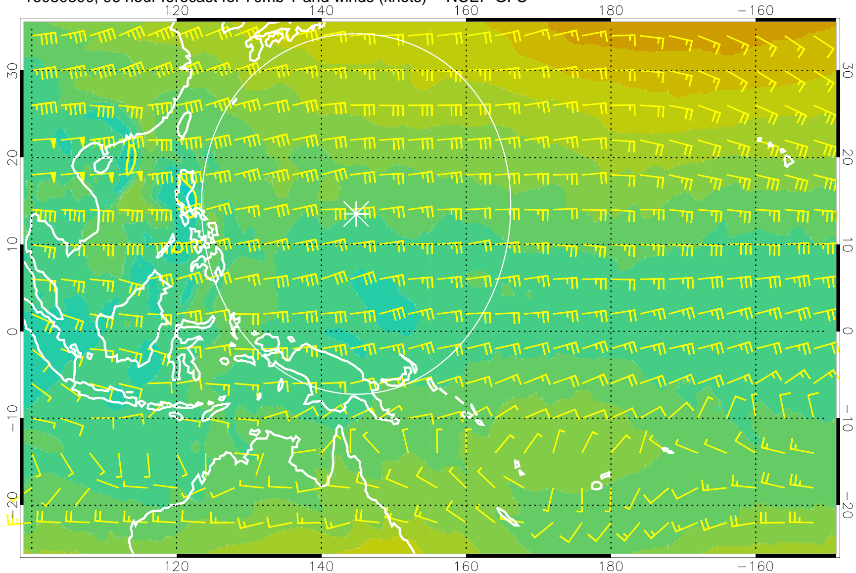
16080300, 96 hour forecast for 70mb T and winds (knots) -- NCEP GFS
