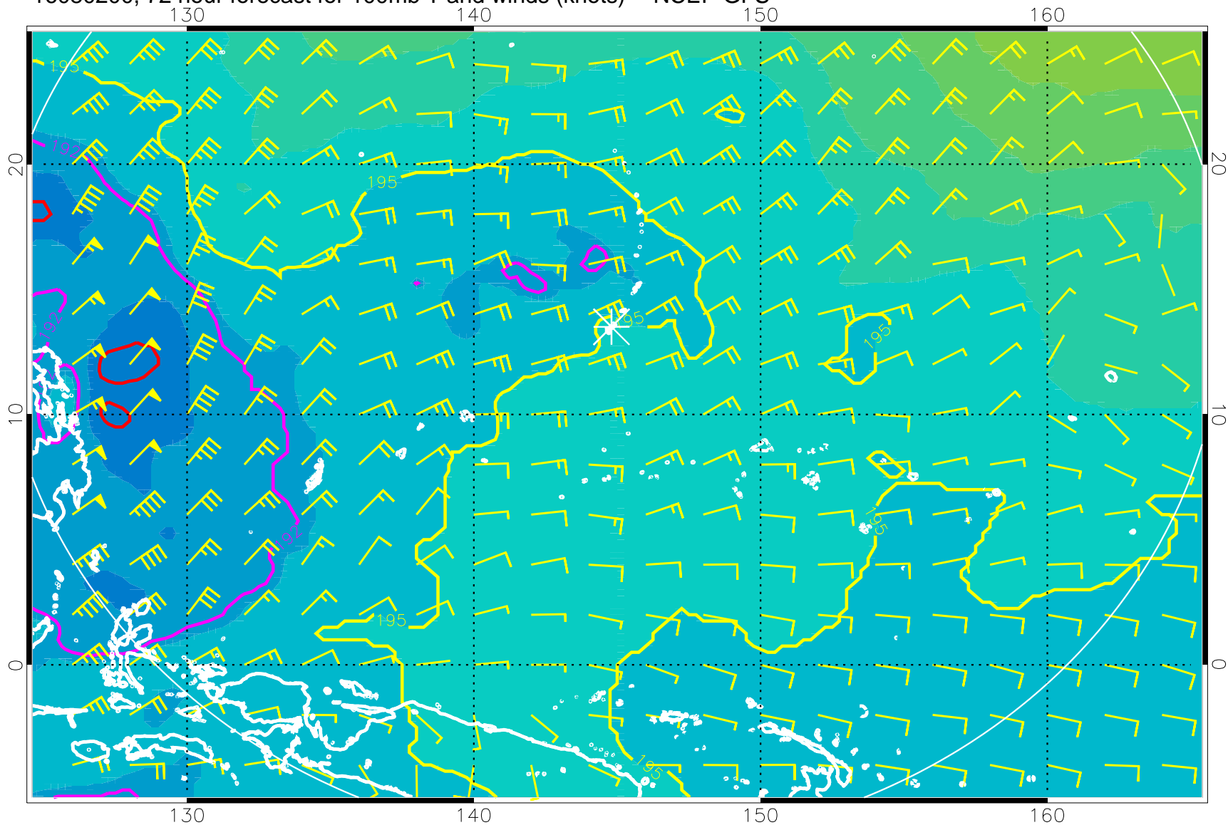
16080200, 72 hour forecast for 100mb T and winds (knots) -- NCEP GFS
