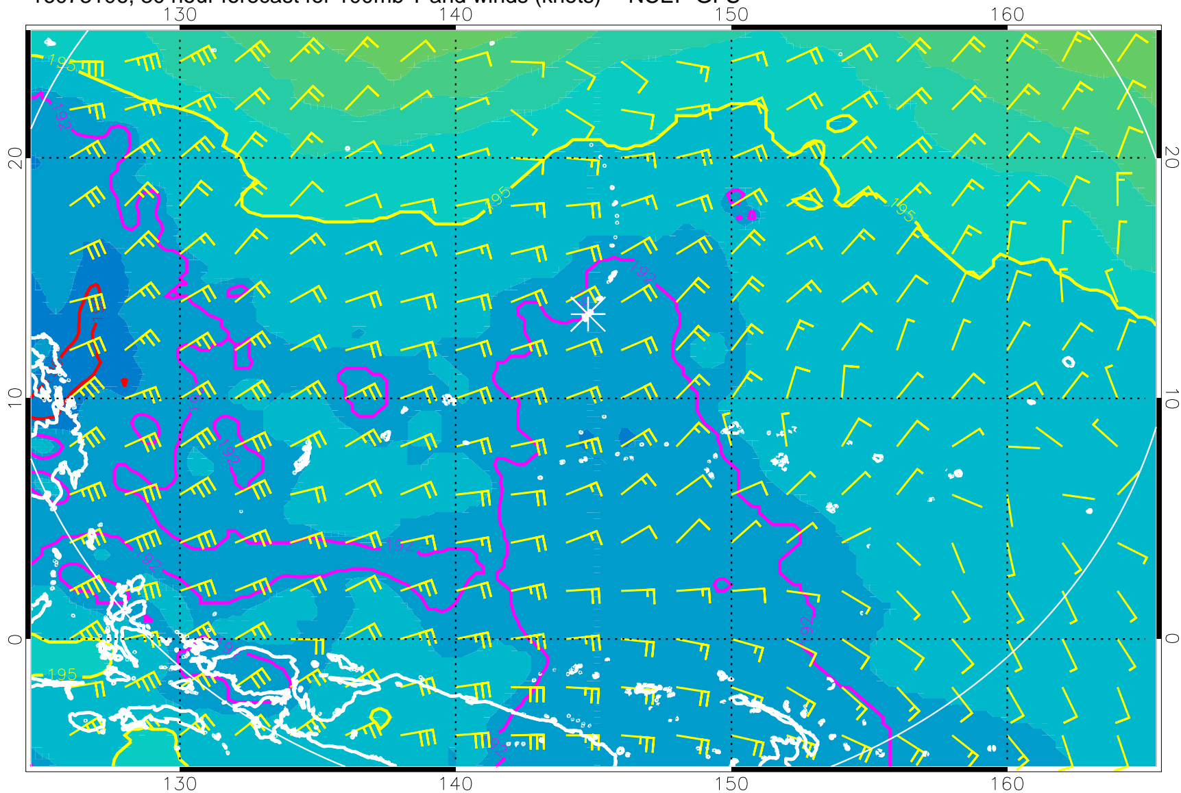
16073106, 30 hour forecast for 100mb T and winds (knots) -- NCEP GFS
