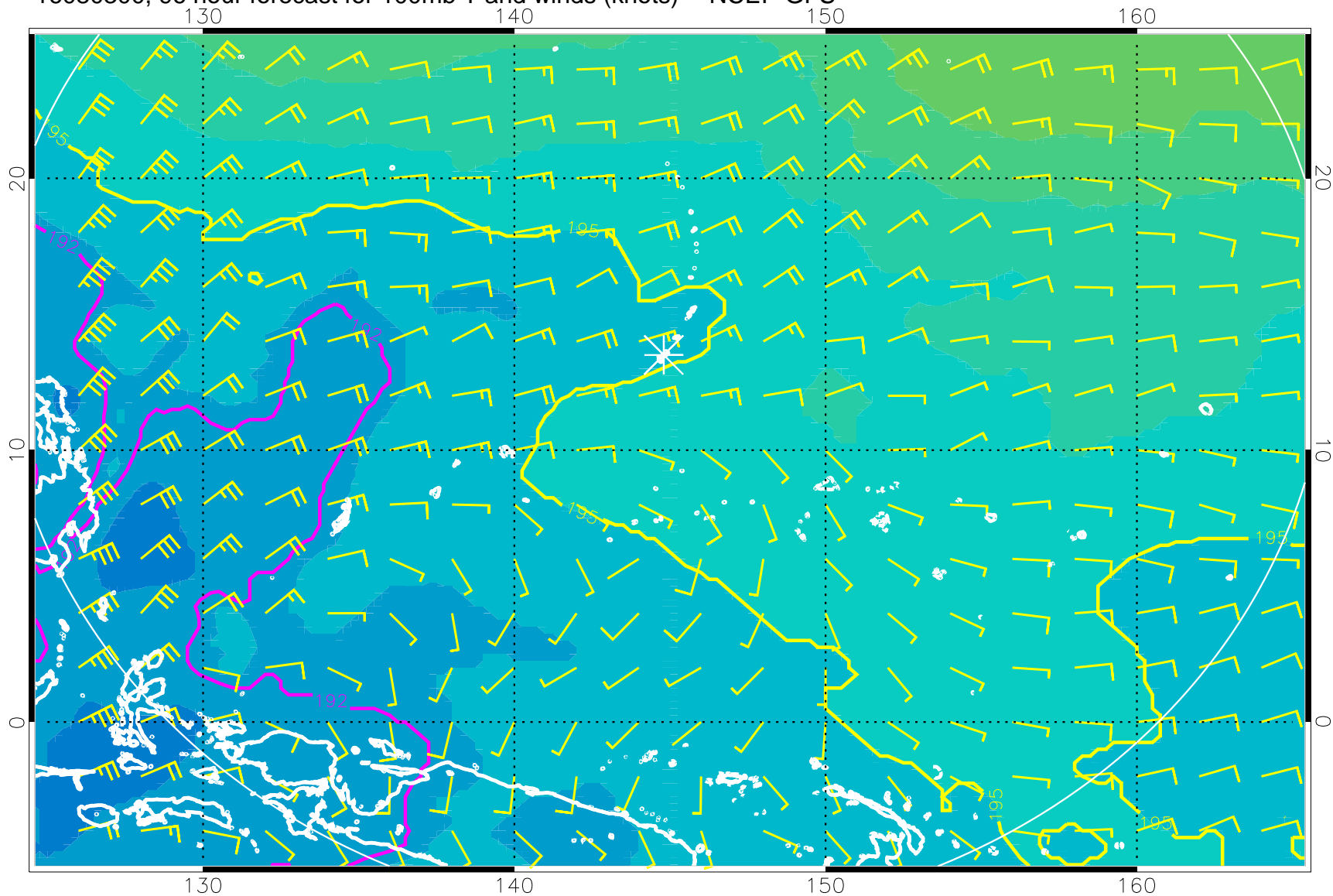
16080300, 96 hour forecast for 100mb T and winds (knots) -- NCEP GFS
