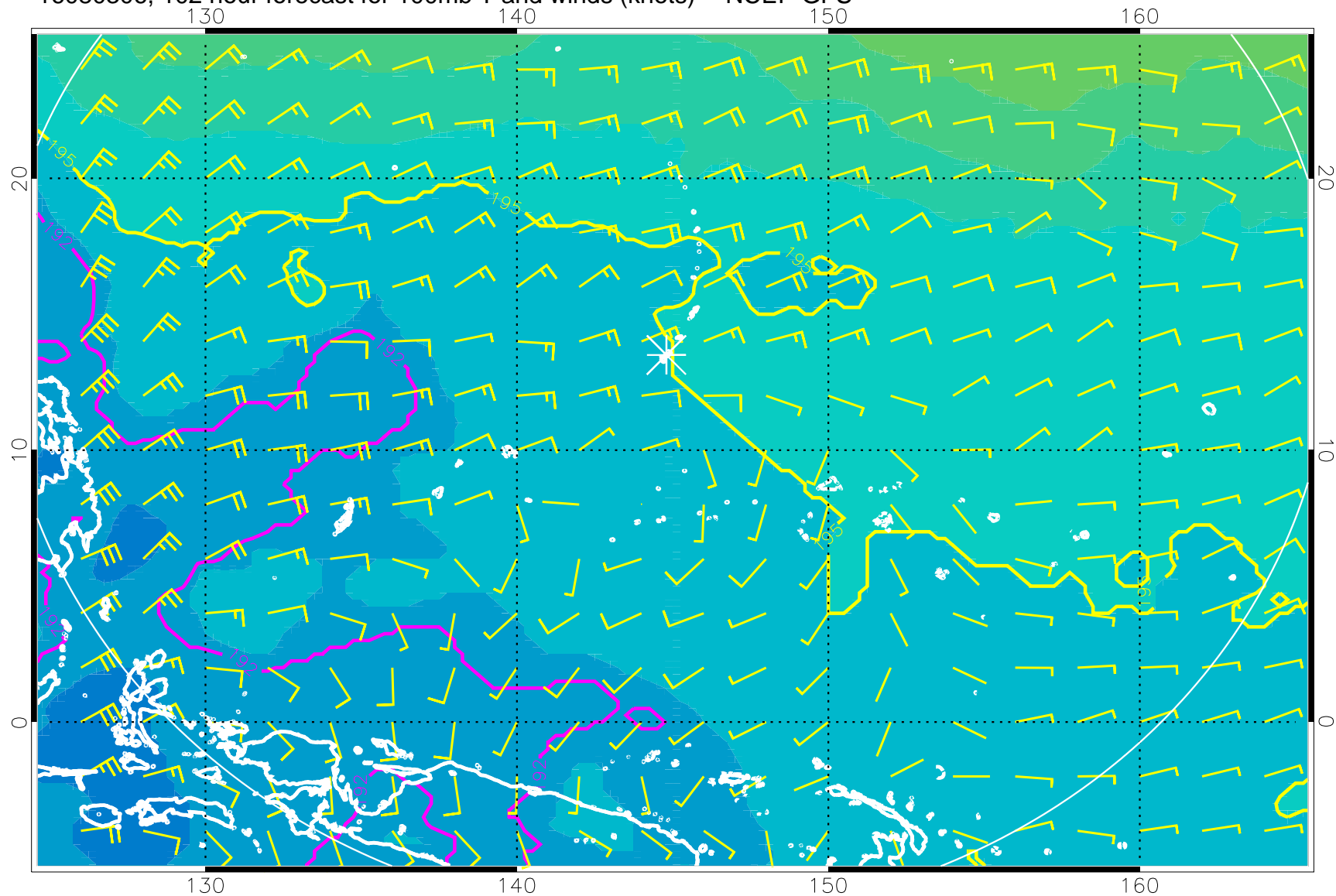
16080306, 102 hour forecast for 100mb T and winds (knots) -- NCEP GFS
