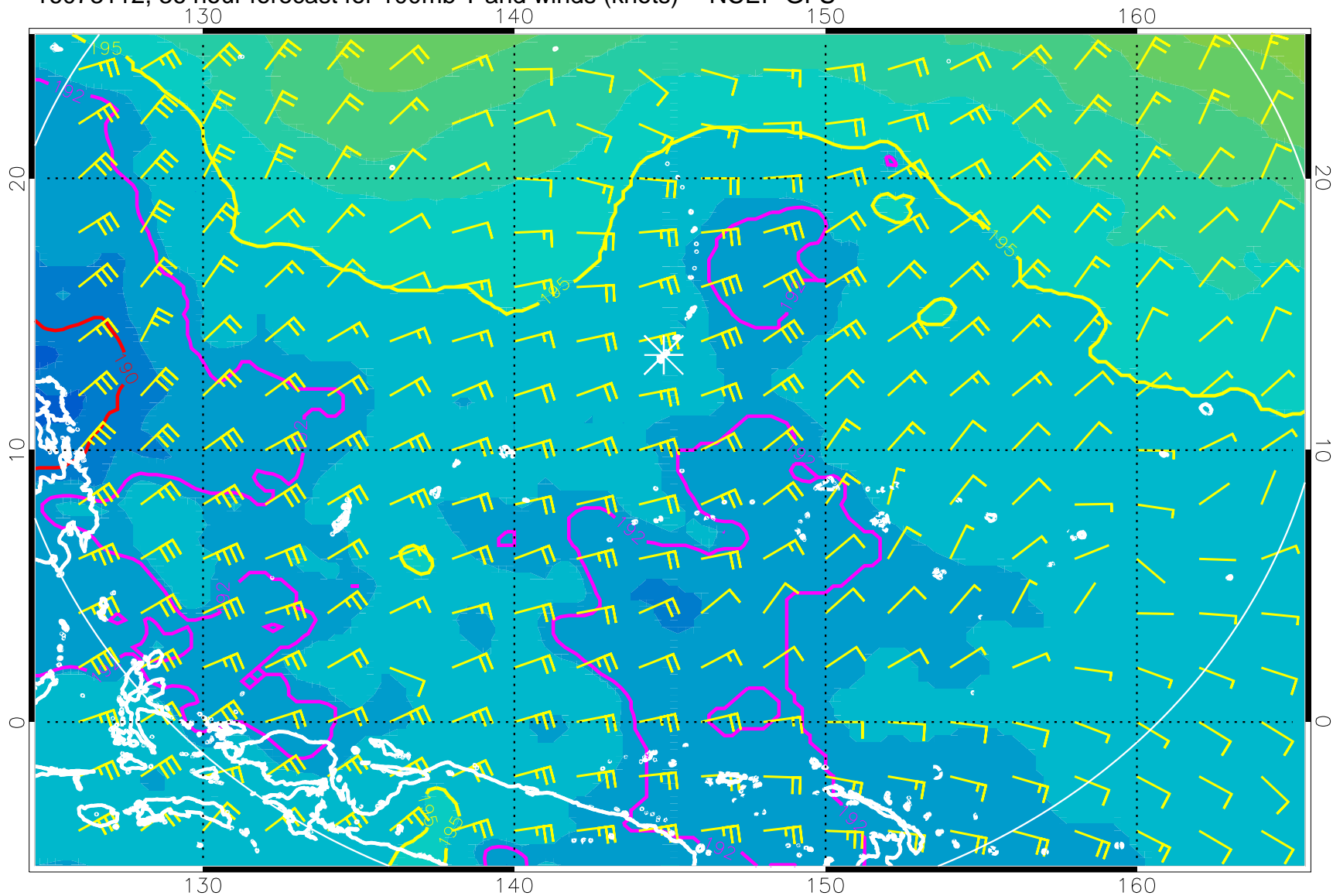
16073112, 36 hour forecast for 100mb T and winds (knots) -- NCEP GFS
