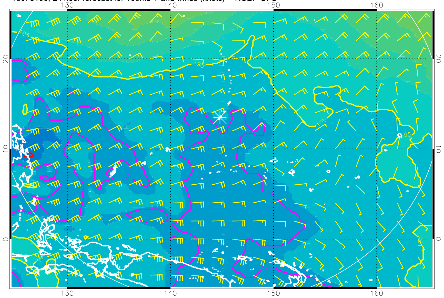
16073100, 24 hour forecast for 100mb T and winds (knots) -- NCEP GFS
