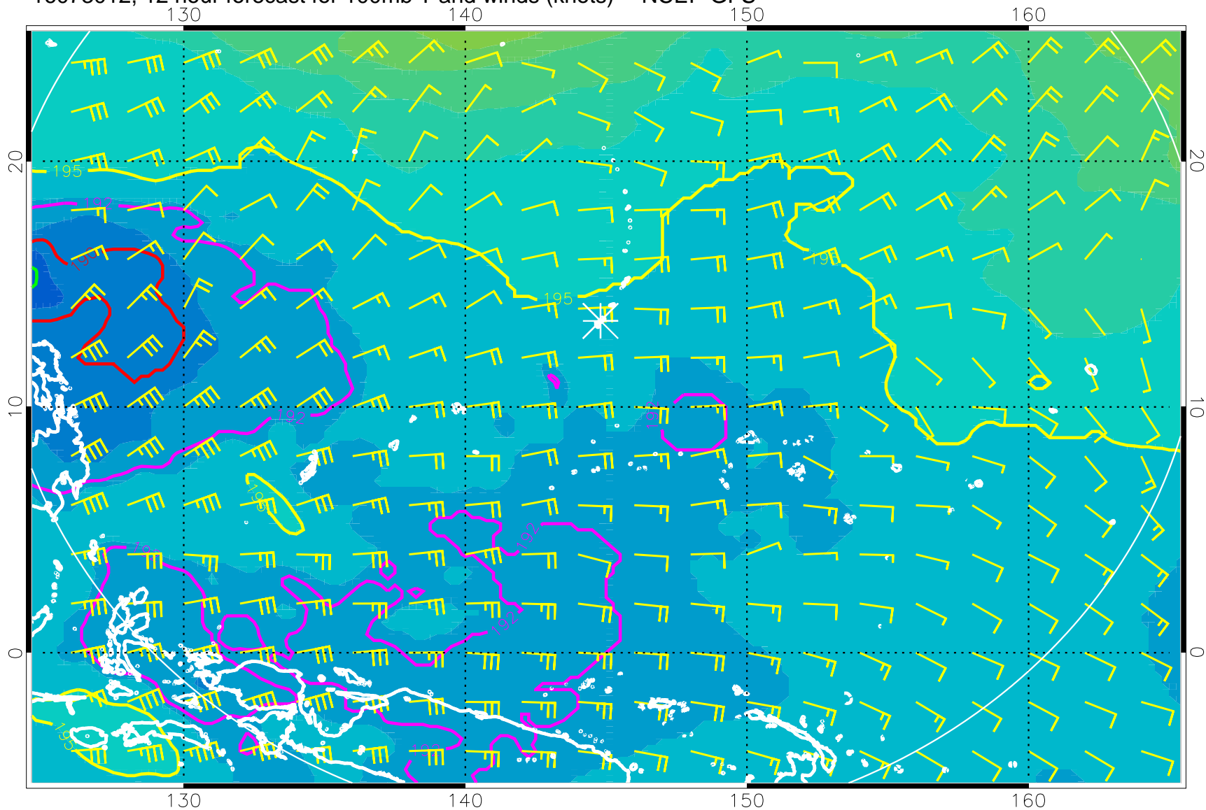
16073012, 12 hour forecast for 100mb T and winds (knots) -- NCEP GFS
