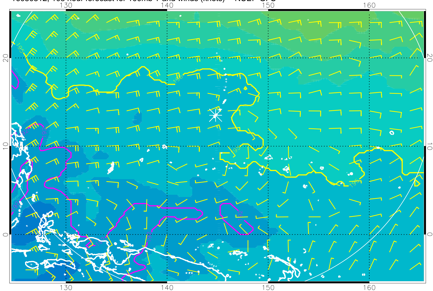
16080312, 108 hour forecast for 100mb T and winds (knots) -- NCEP GFS
