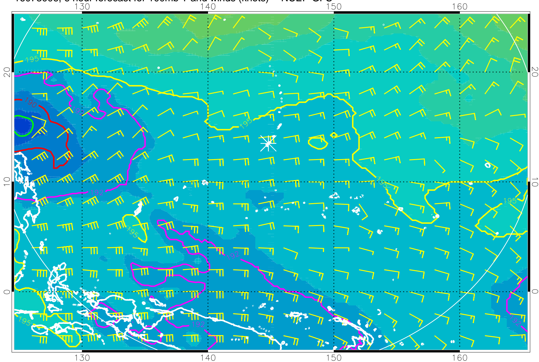
16073006, 6 hour forecast for 100mb T and winds (knots) -- NCEP GFS
