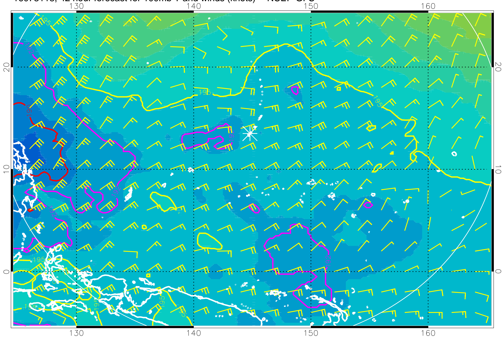
16073118, 42 hour forecast for 100mb T and winds (knots) -- NCEP GFS
