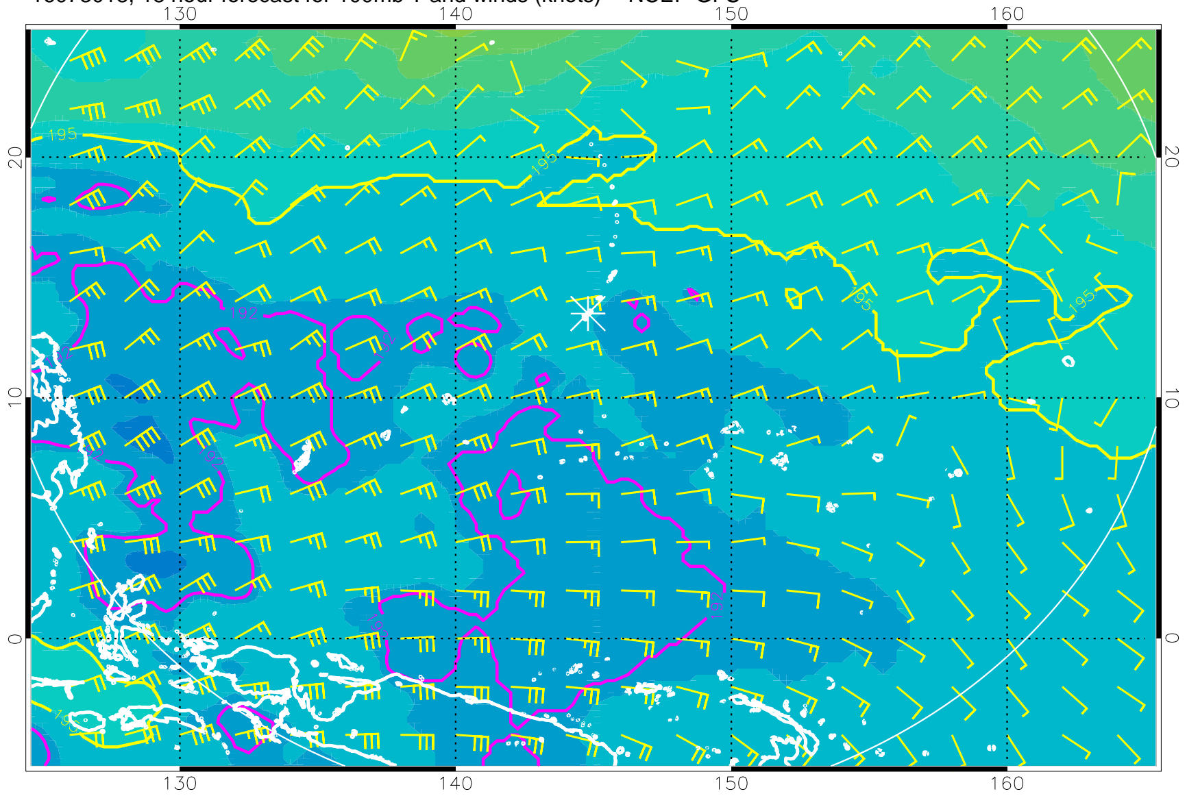
16073018, 18 hour forecast for 100mb T and winds (knots) -- NCEP GFS
