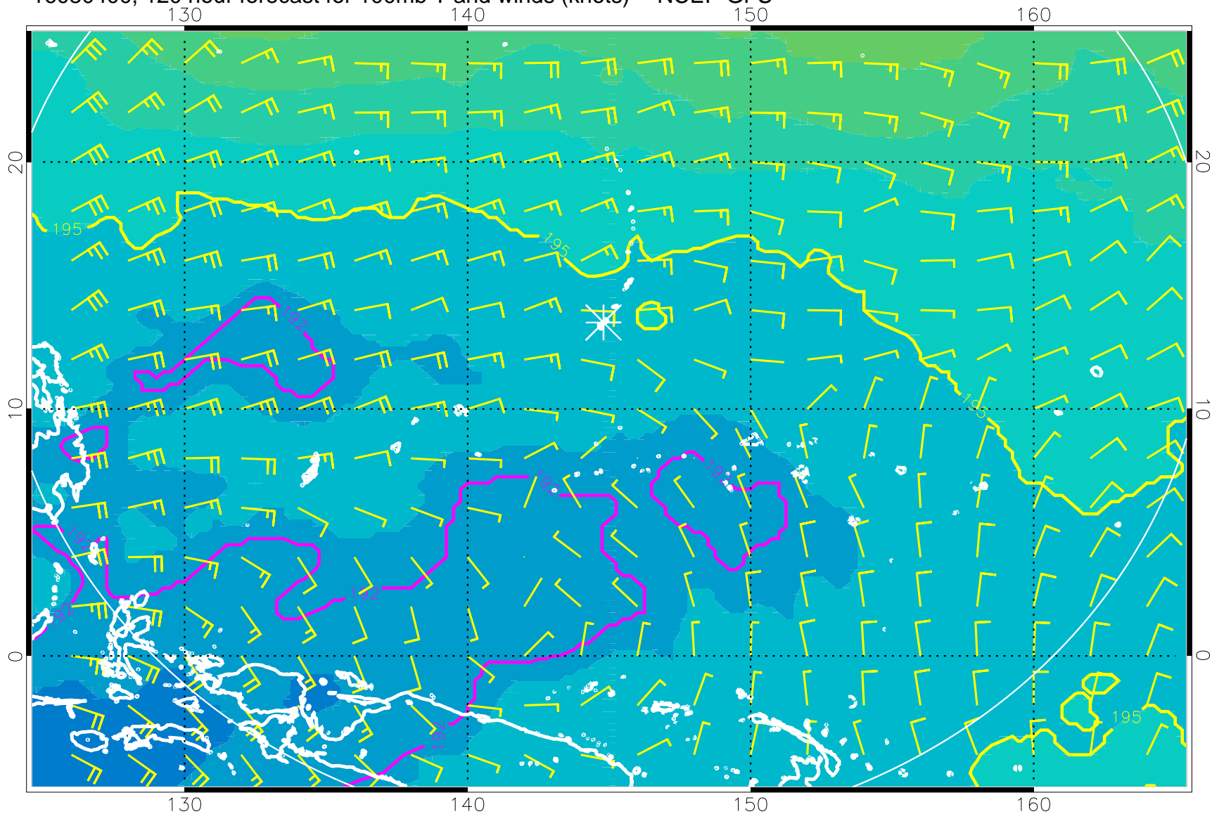
16080400, 120 hour forecast for 100mb T and winds (knots) -- NCEP GFS
