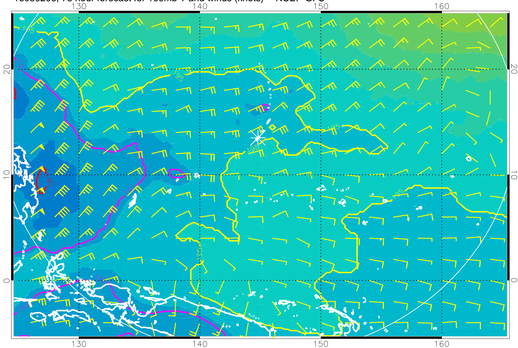
16080206, 78 hour forecast for 100mb T and winds (knots) -- NCEP GFS
