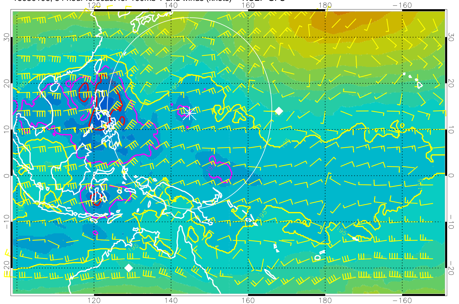
16080106, 54 hour forecast for 100mb T and winds (knots) -- NCEP GFS
