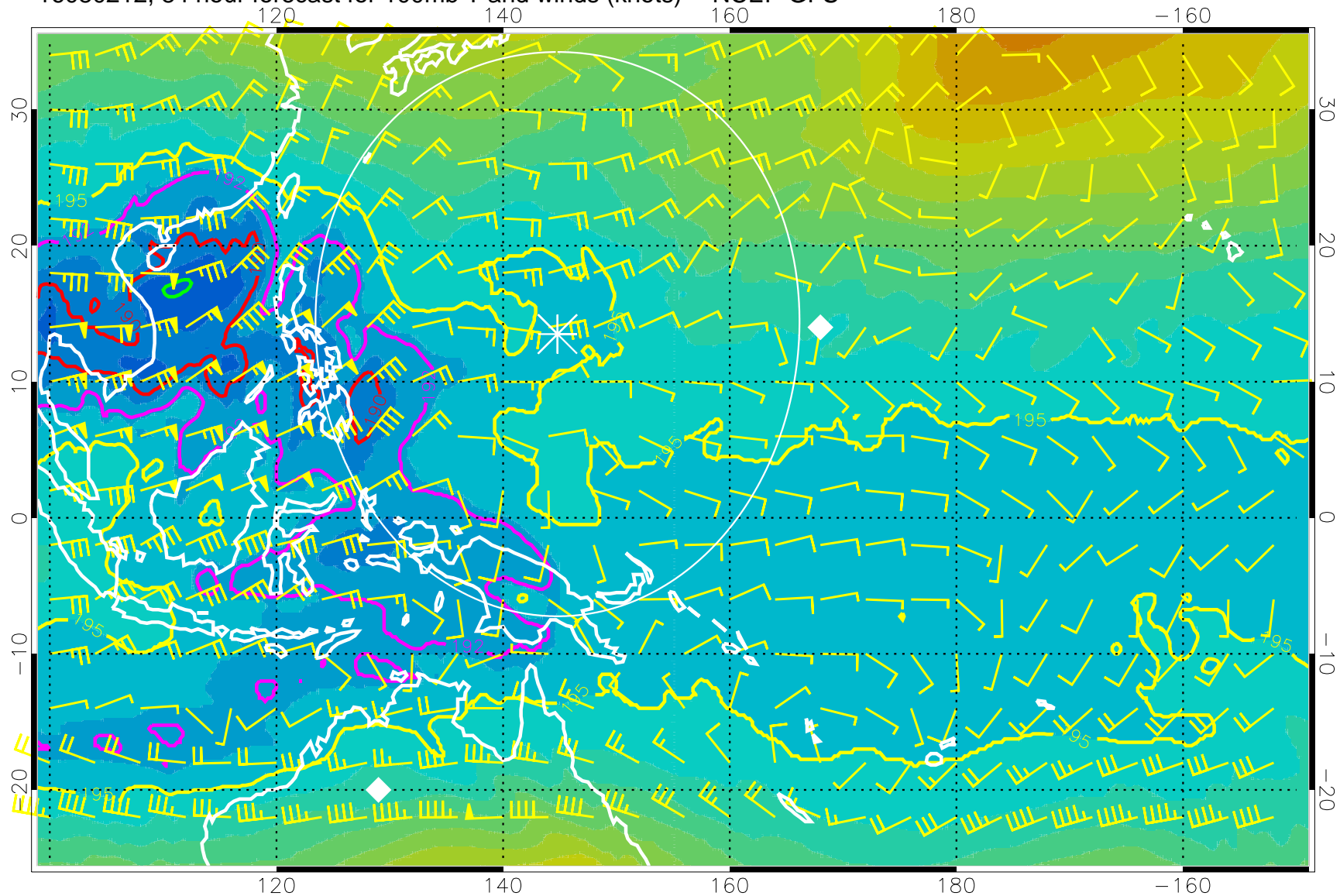
16080212, 84 hour forecast for 100mb T and winds (knots) -- NCEP GFS
