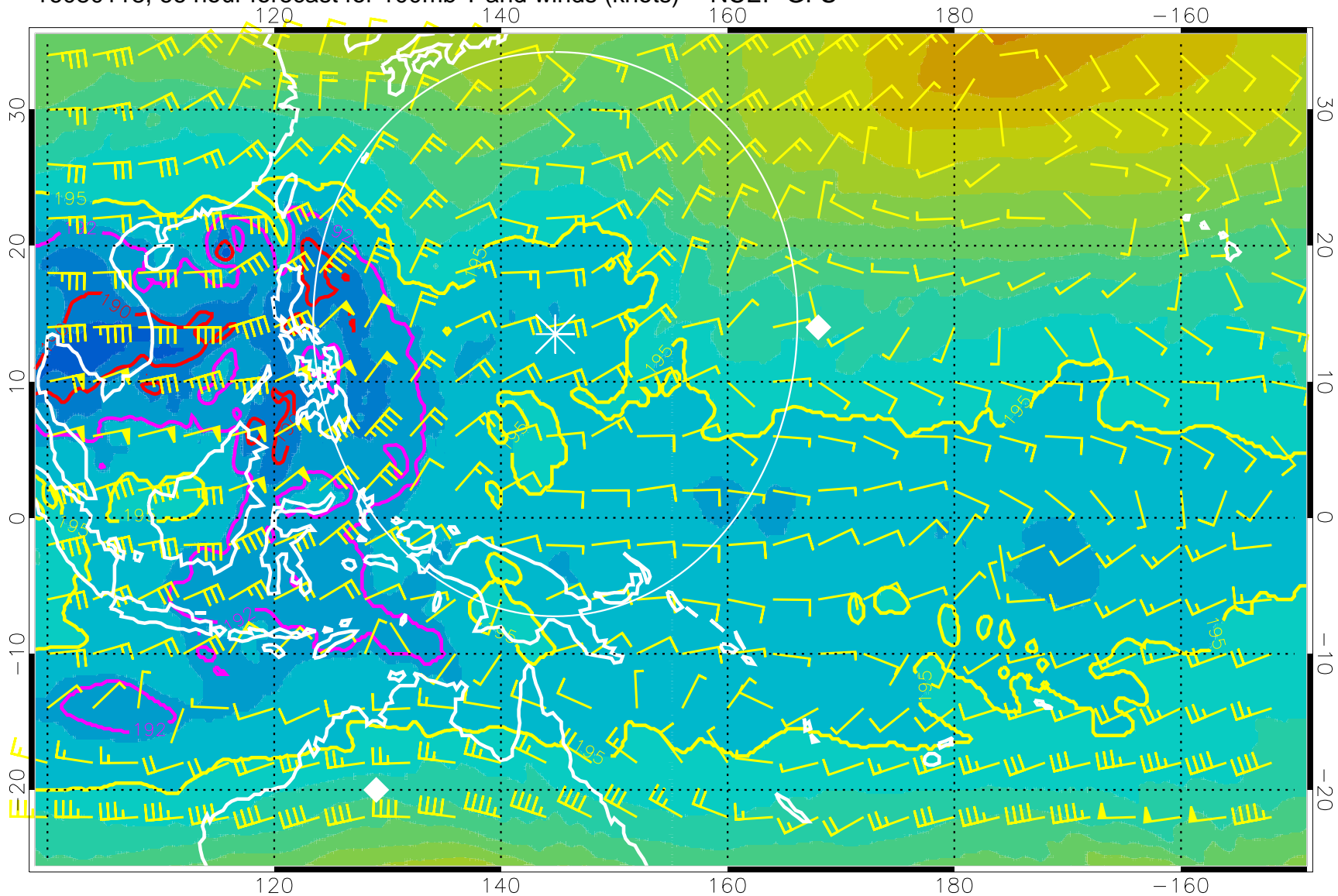
16080118, 66 hour forecast for 100mb T and winds (knots) -- NCEP GFS
