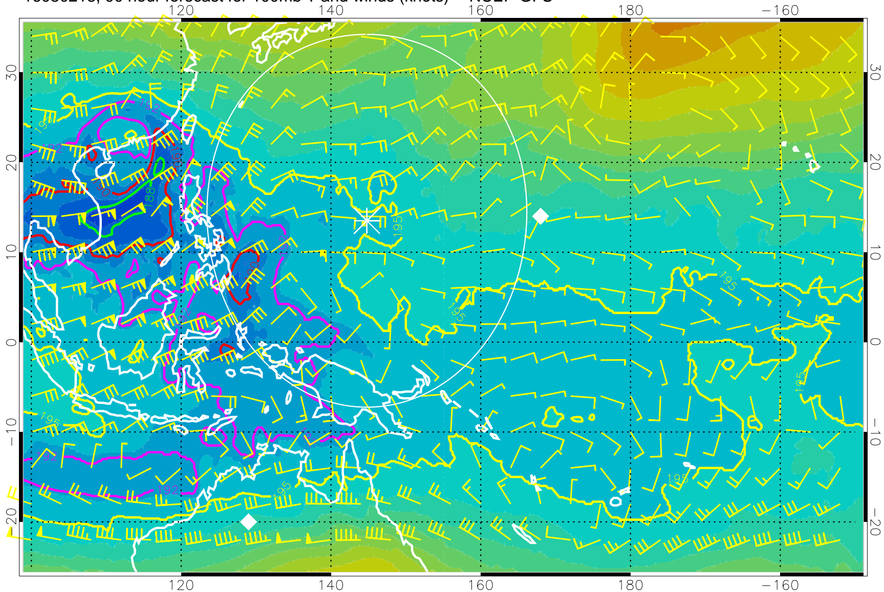
16080218, 90 hour forecast for 100mb T and winds (knots) -- NCEP GFS
