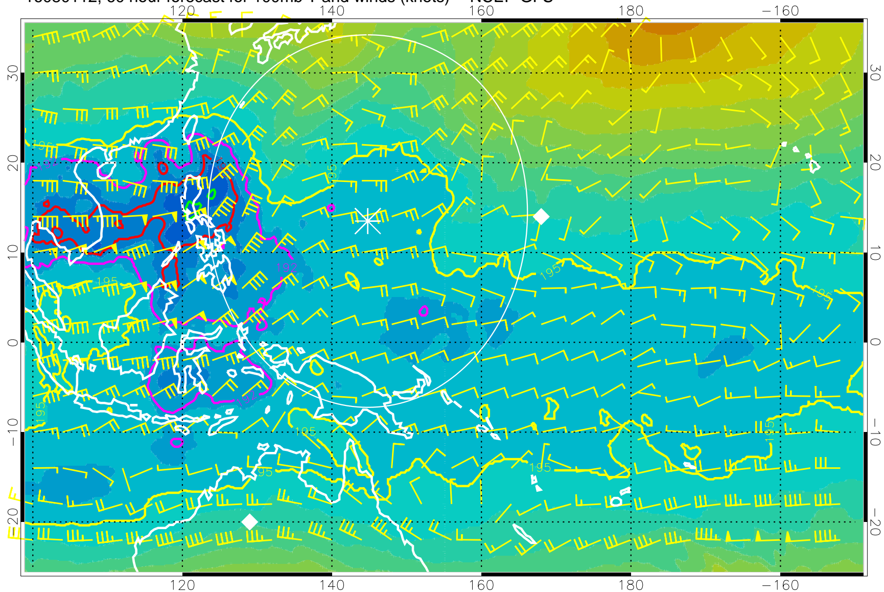
16080112, 60 hour forecast for 100mb T and winds (knots) -- NCEP GFS
