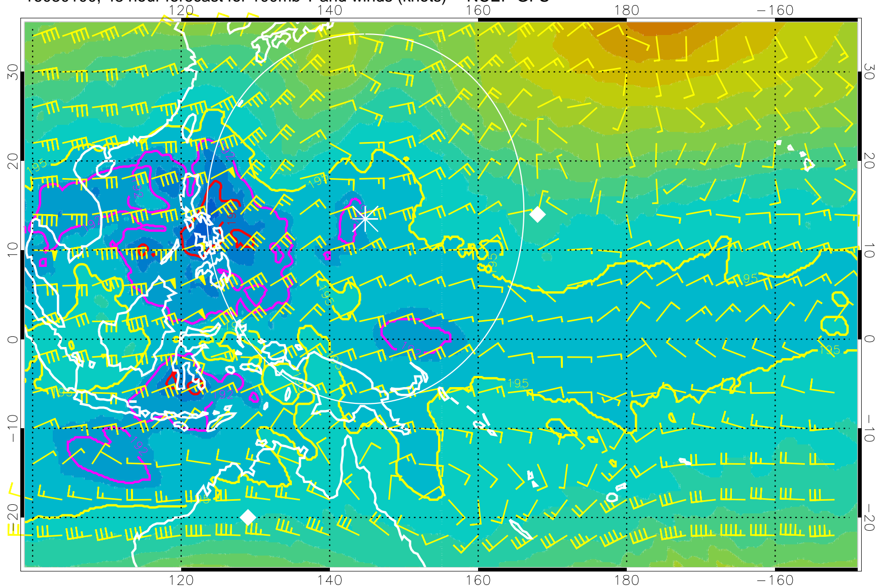
16080100, 48 hour forecast for 100mb T and winds (knots) -- NCEP GFS
