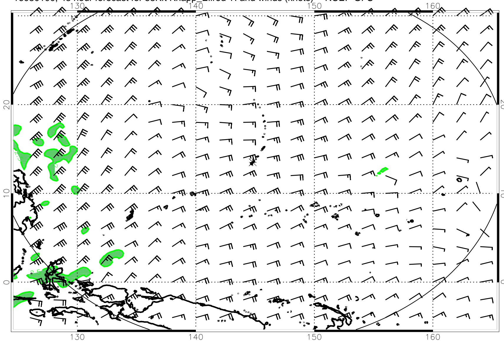
16080100, 48 hour forecast for 53Kft Knapp_Ellrod TI and winds (knots) -- NCEP GFS
