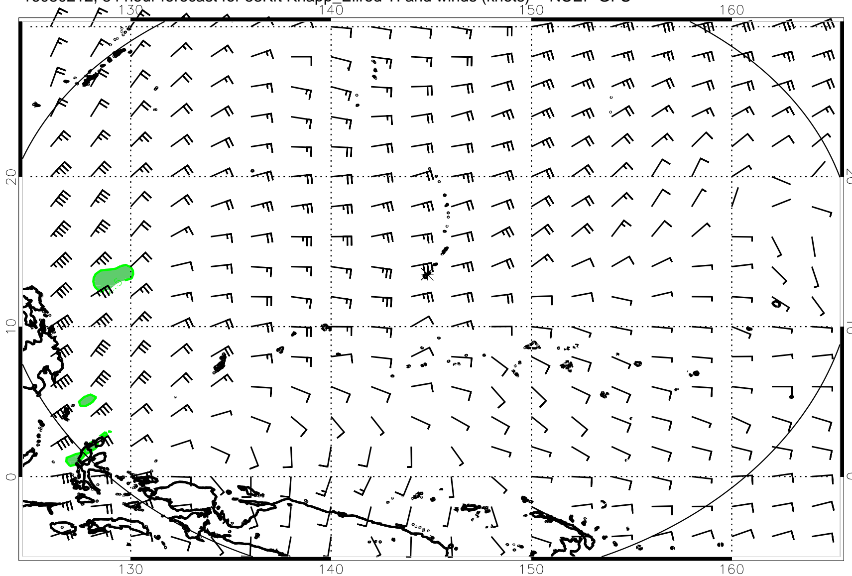
16080212, 84 hour forecast for 53Kft Knapp_Ellrod TI and winds (knots) -- NCEP GFS
