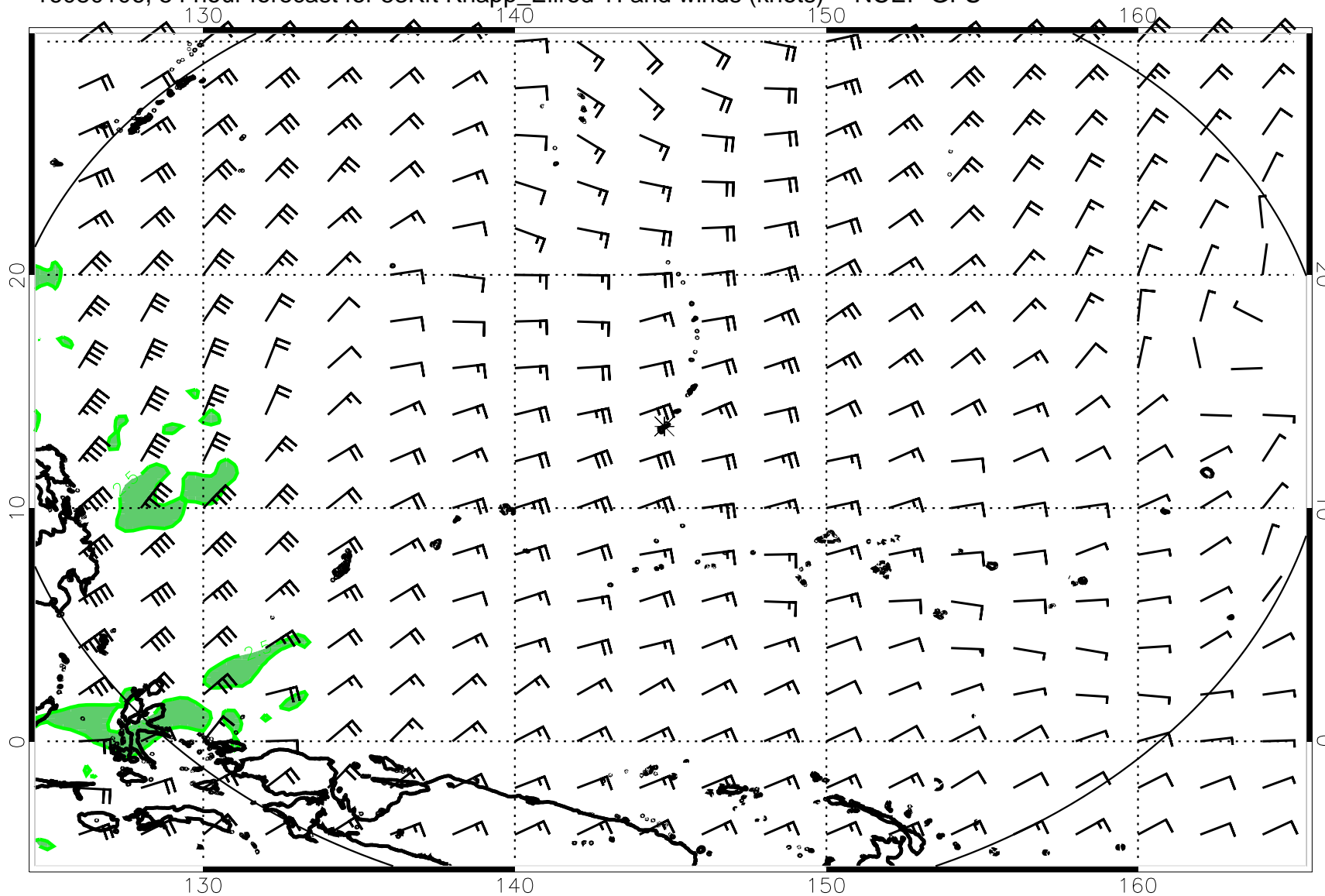
16080106, 54 hour forecast for 53Kft Knapp_Ellrod TI and winds (knots) -- NCEP GFS
