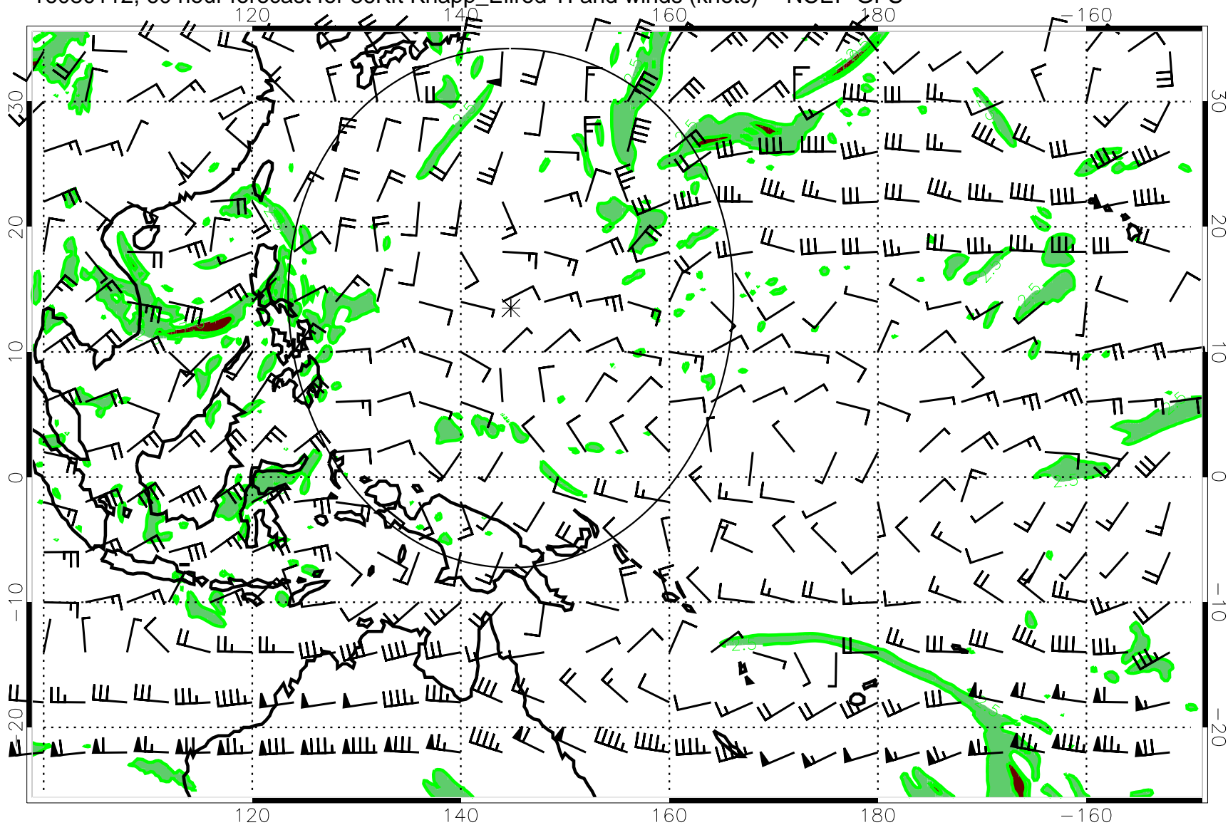
16080112, 60 hour forecast for 36Kft Knapp_Ellrod TI and winds (knots) -- NCEP GFS
