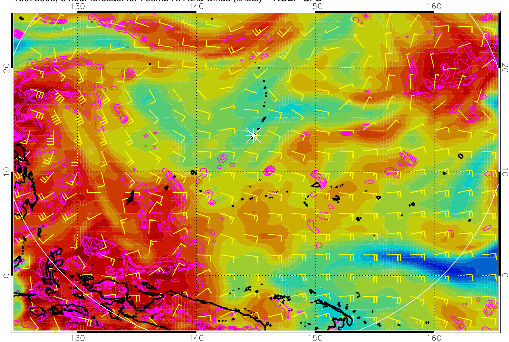
16073006, 6 hour forecast for 700mb RH and winds (knots) -- NCEP GFS
