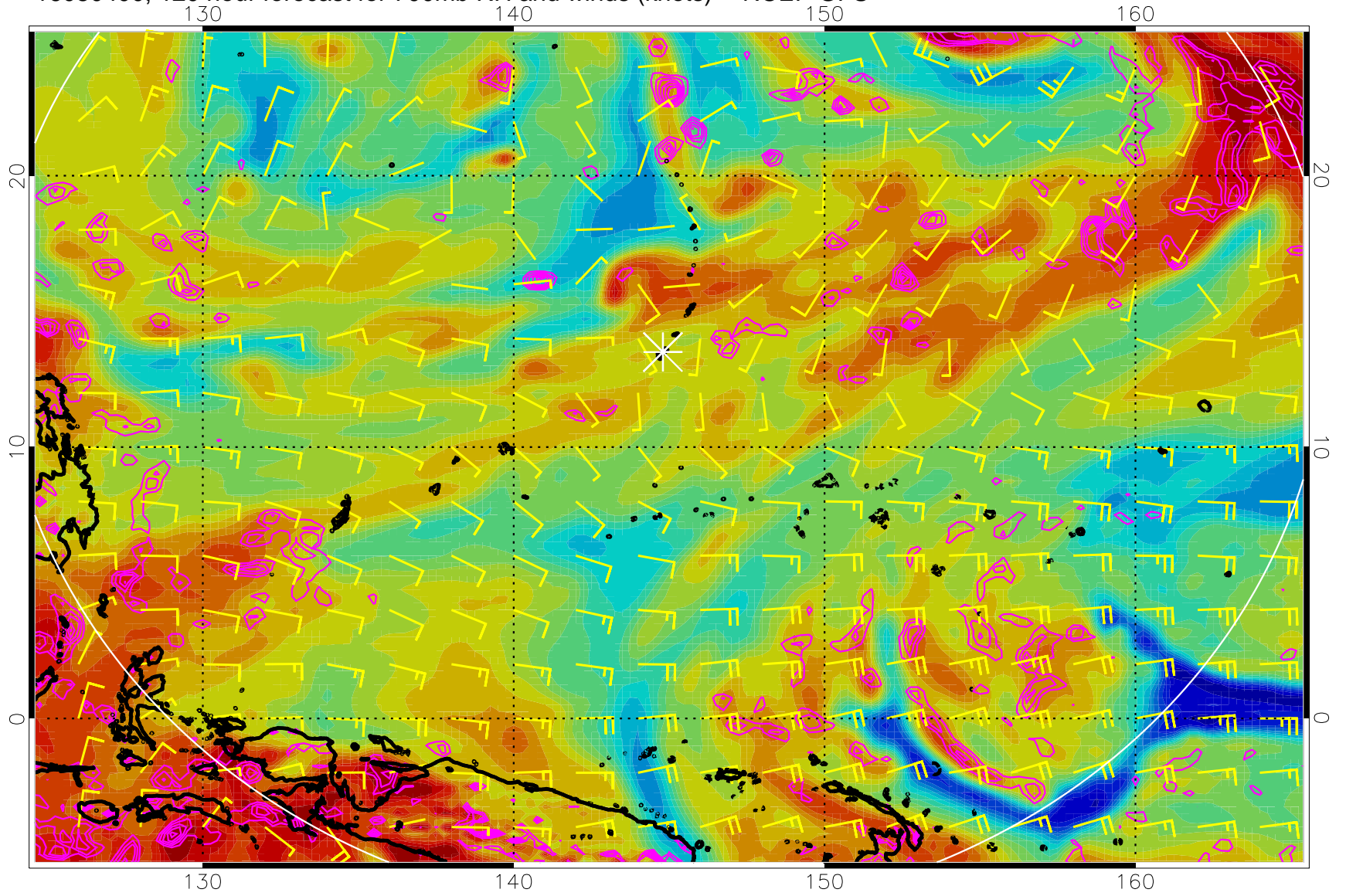
16080400, 120 hour forecast for 700mb RH and winds (knots) -- NCEP GFS
