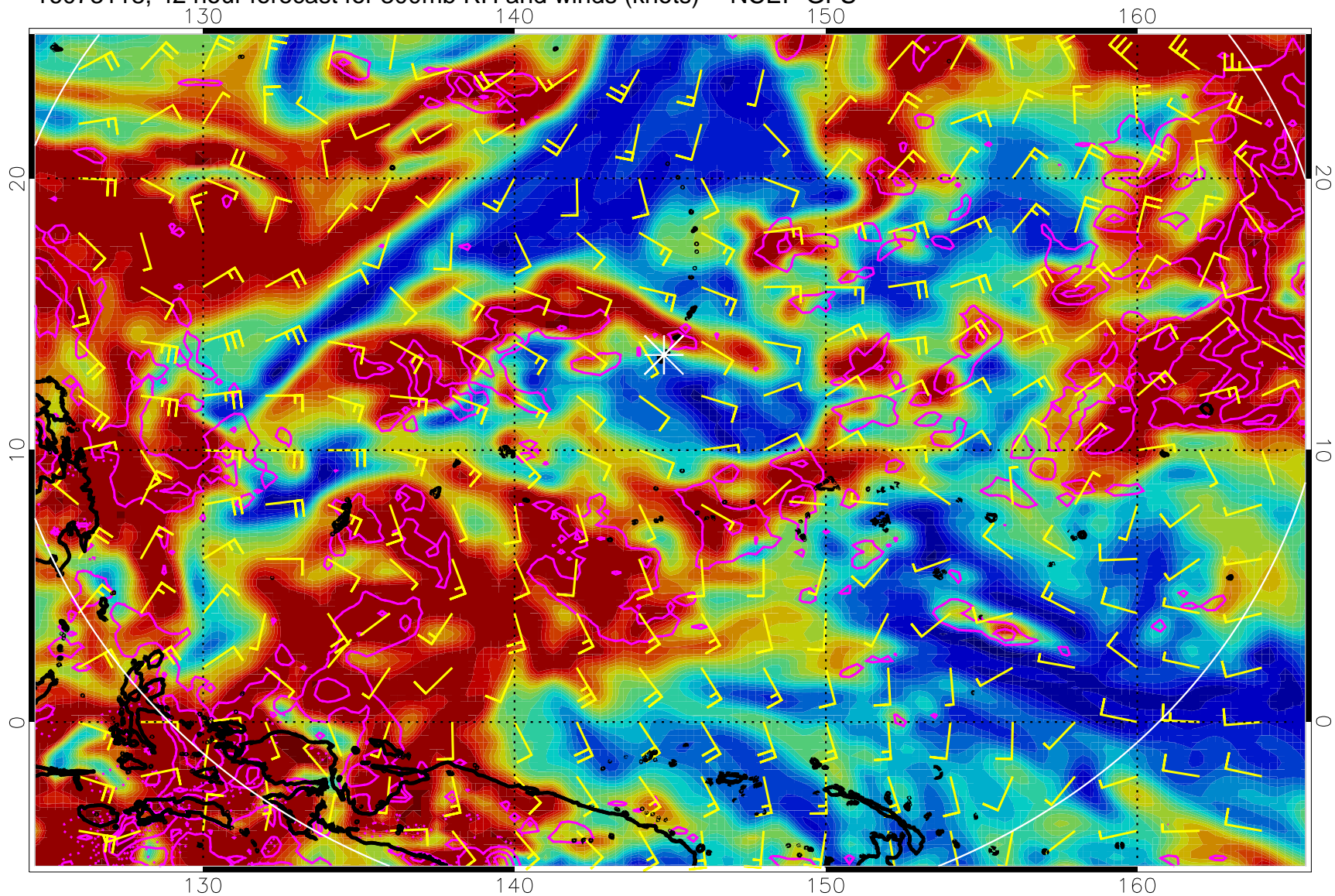
16073118, 42 hour forecast for 300mb RH and winds (knots) -- NCEP GFS
