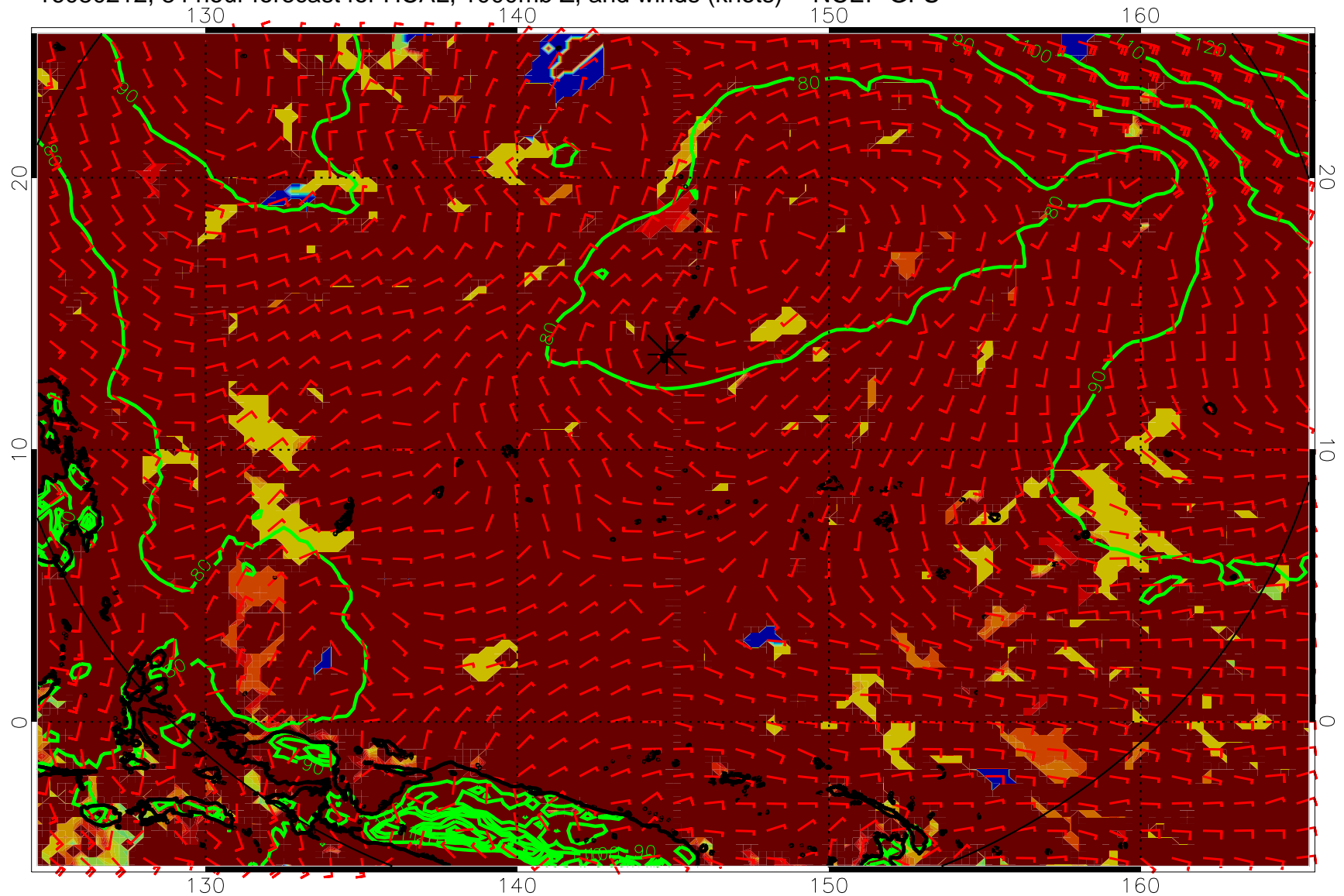
16080212, 84 hour forecast for HCAL, 1000mb Z, and winds (knots) -- NCEP GFS
