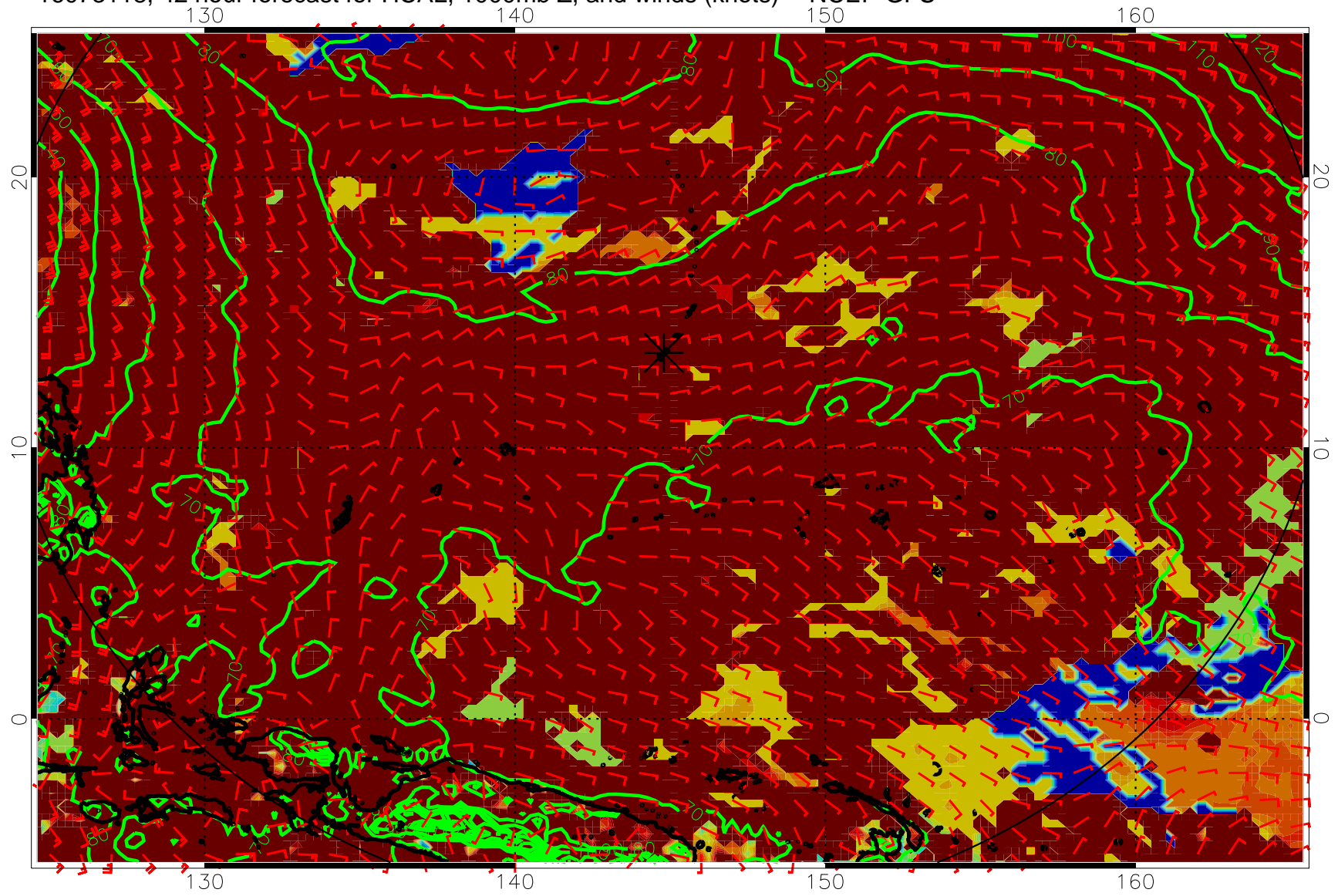
16073118, 42 hour forecast for HCAL, 1000mb Z, and winds (knots) -- NCEP GFS
