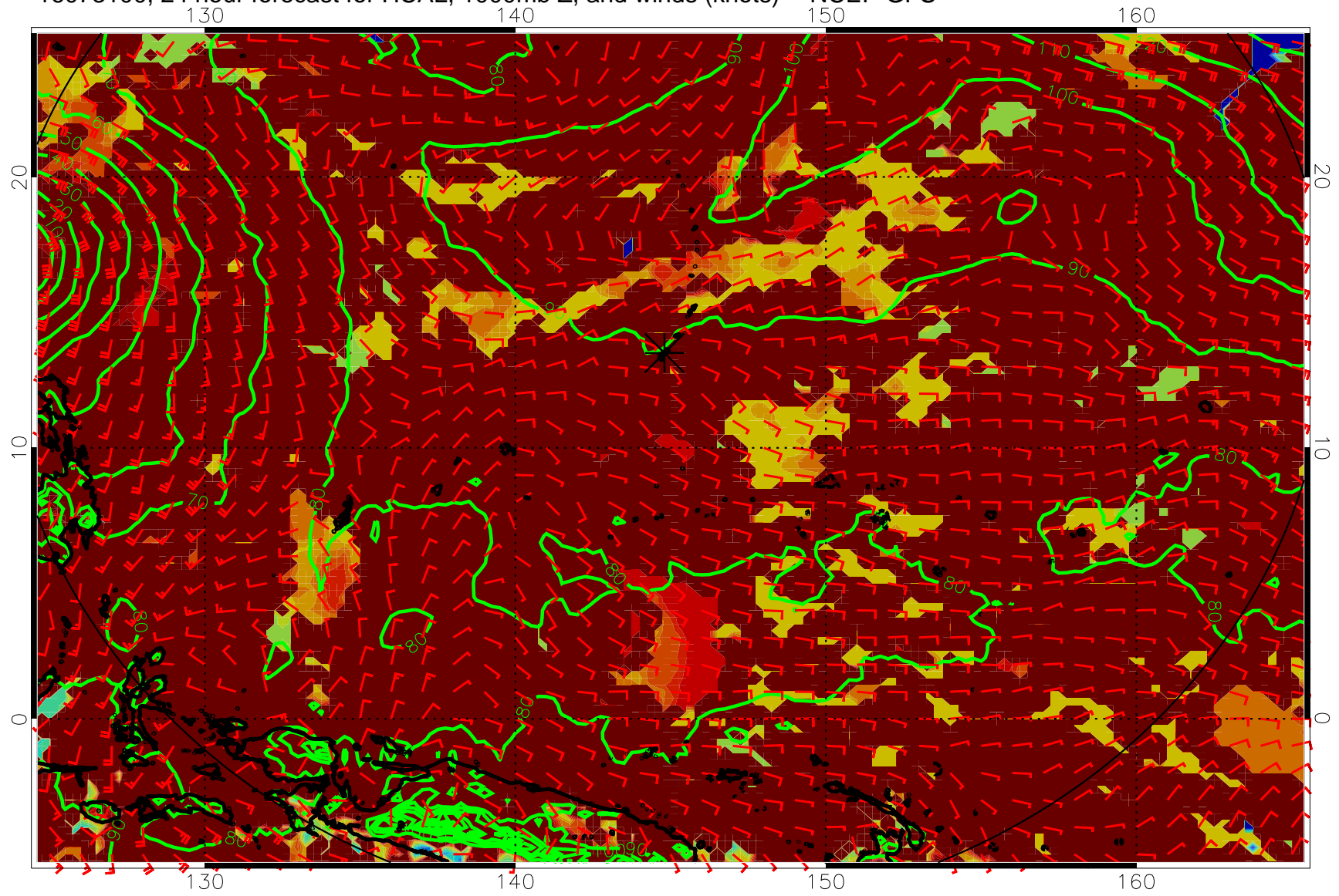
16073100, 24 hour forecast for HCAL, 1000mb Z, and winds (knots) -- NCEP GFS
