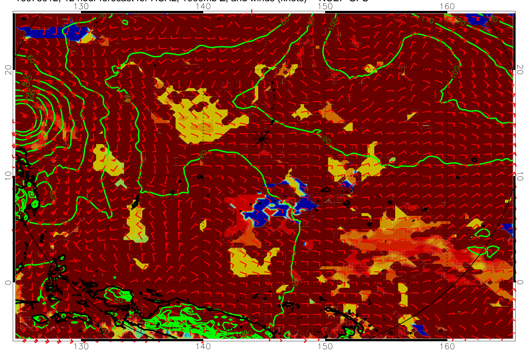
16073012, 12 hour forecast for HCAL, 1000mb Z, and winds (knots) -- NCEP GFS
