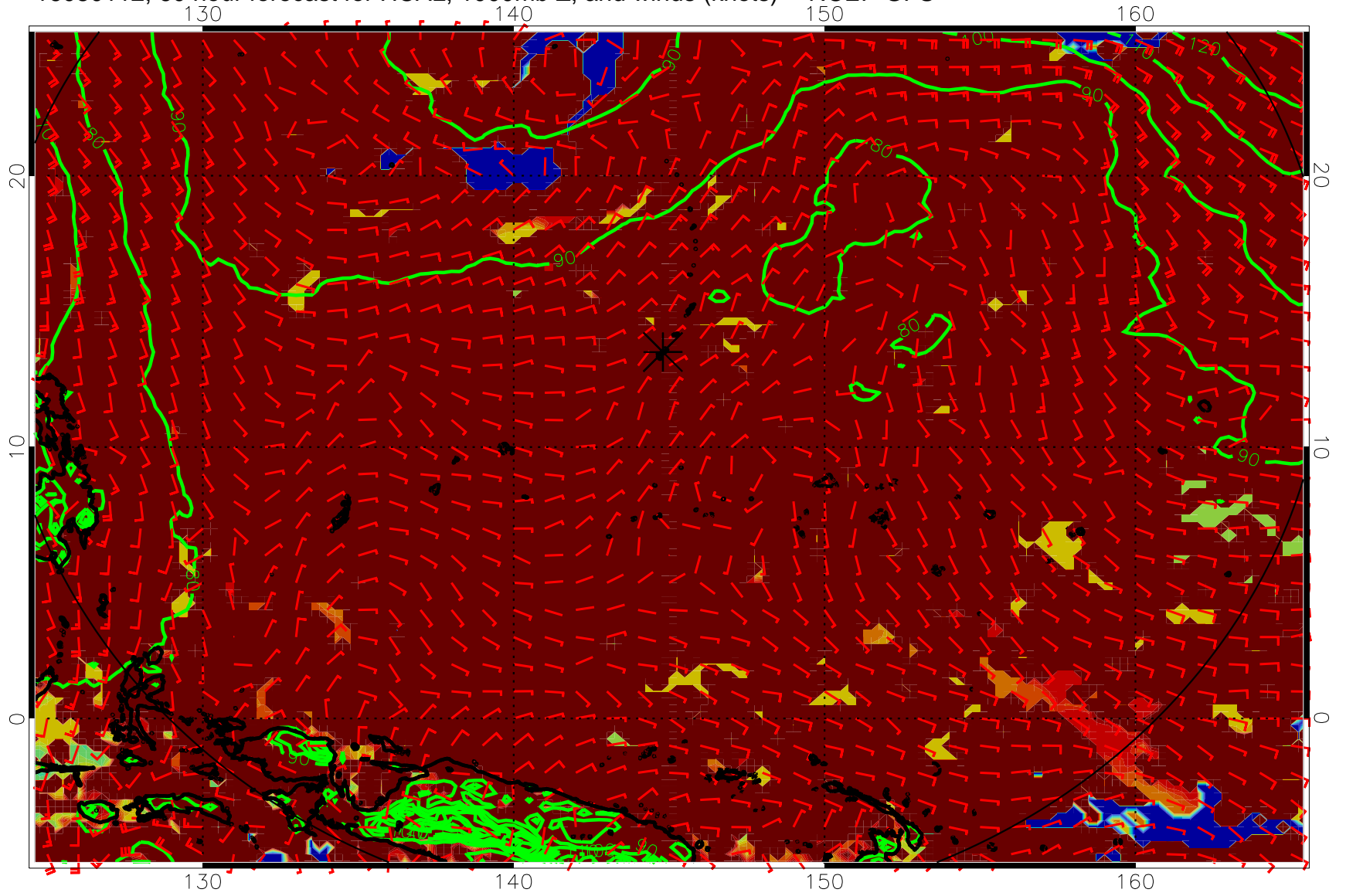
16080112, 60 hour forecast for HCAL, 1000mb Z, and winds (knots) -- NCEP GFS
