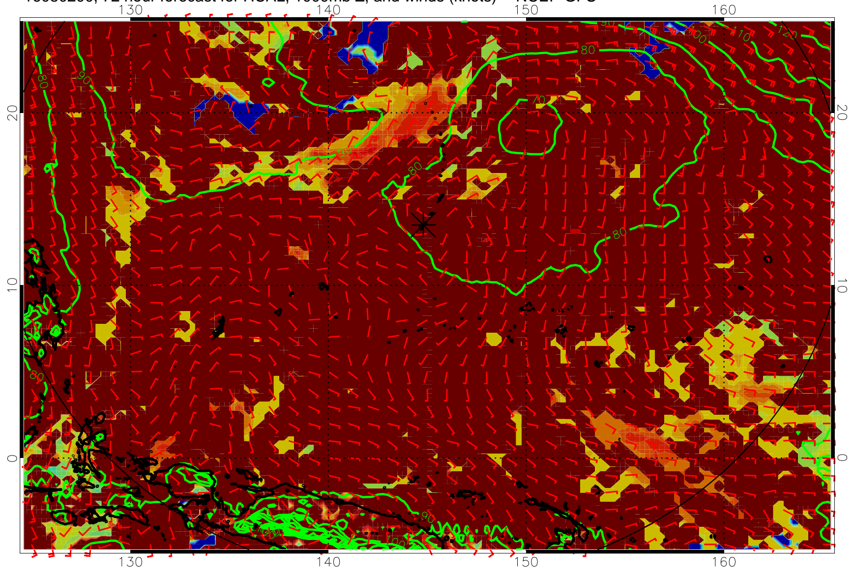
16080200, 72 hour forecast for HCAL, 1000mb Z, and winds (knots) -- NCEP GFS
