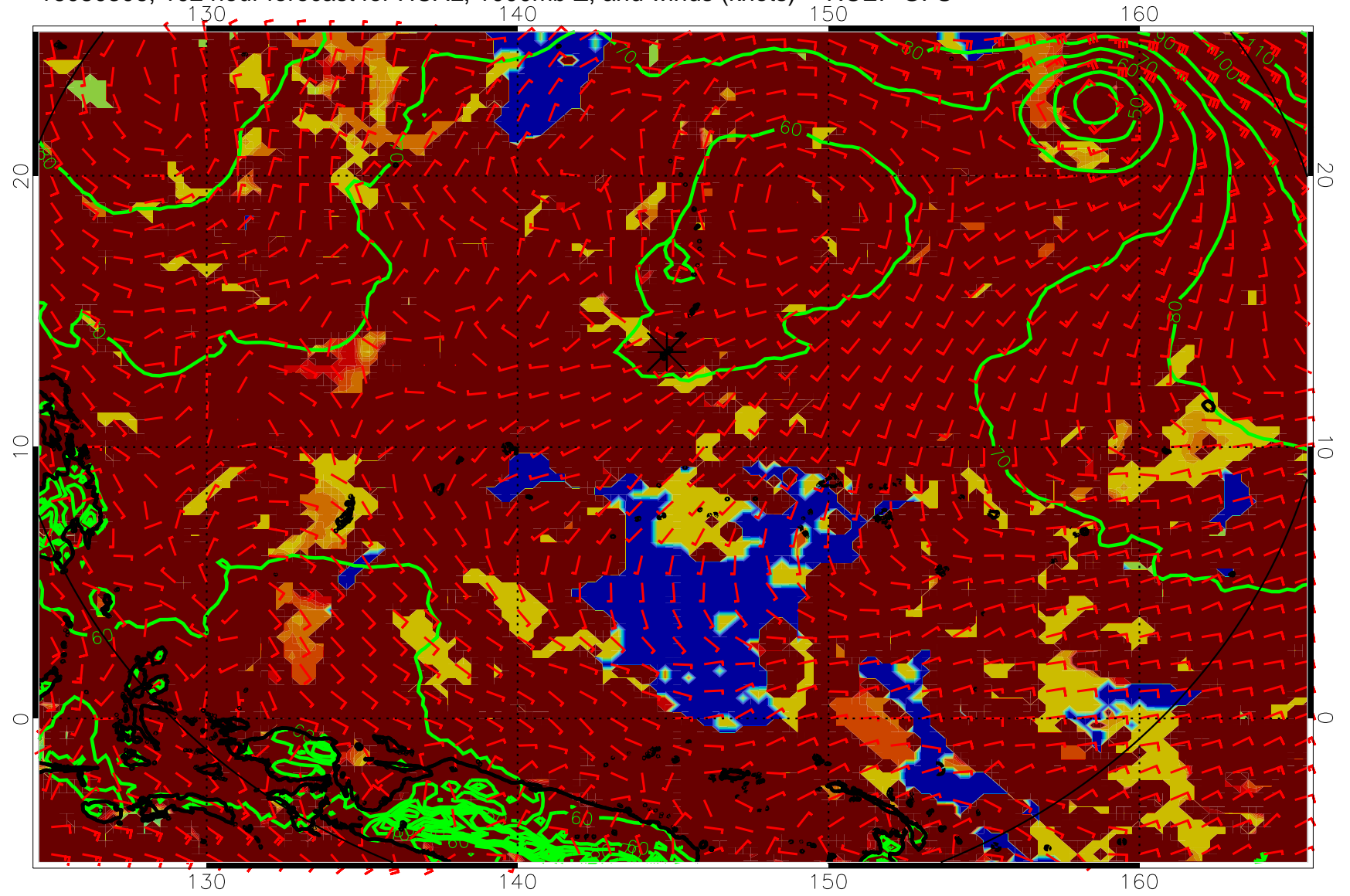
16080306, 102 hour forecast for HCAL, 1000mb Z, and winds (knots) -- NCEP GFS
