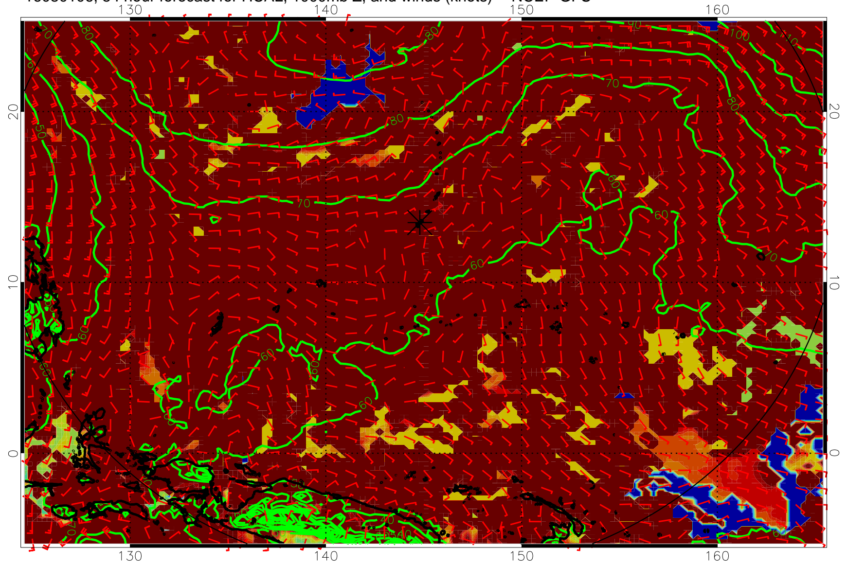
16080106, 54 hour forecast for HCAL, 1000mb Z, and winds (knots) -- NCEP GFS
