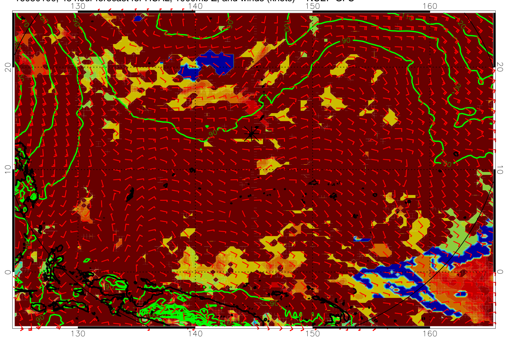
16080100, 48 hour forecast for HCAL, 1000mb Z, and winds (knots) -- NCEP GFS
