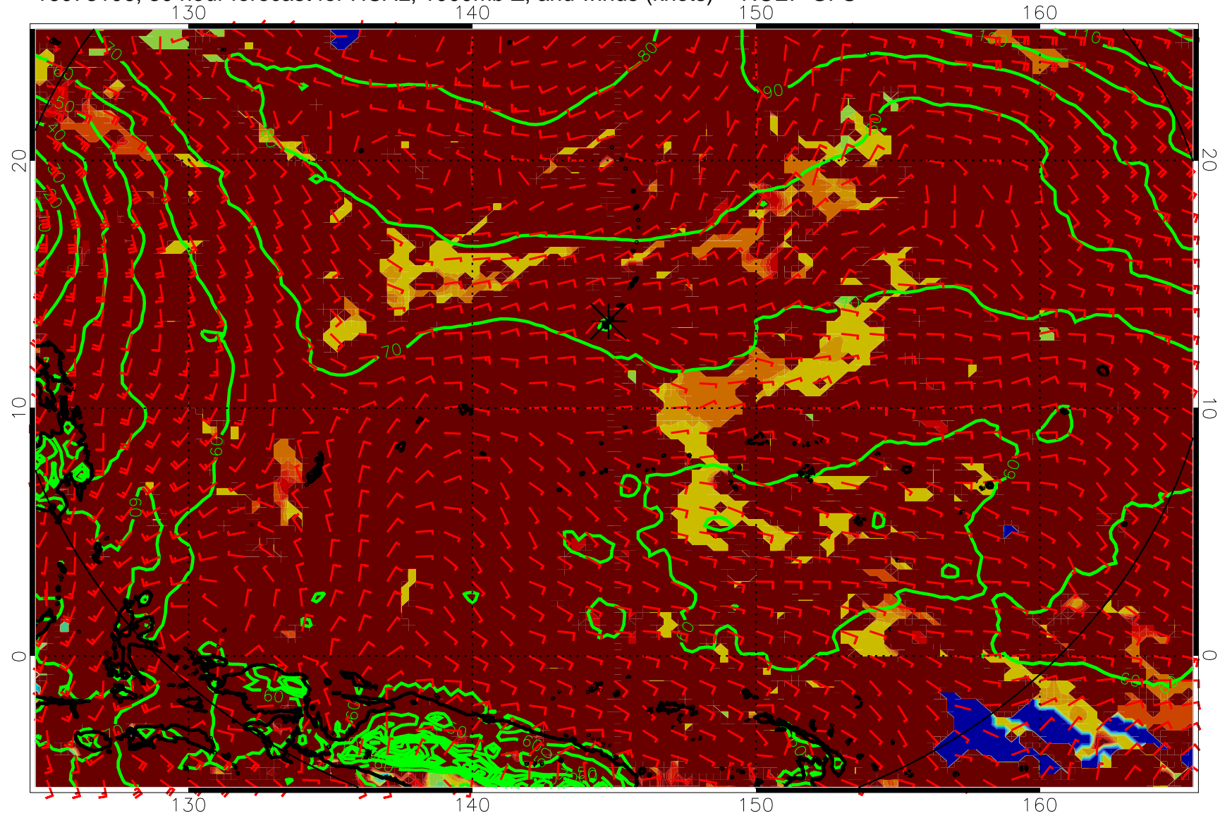
16073106, 30 hour forecast for HCAL, 1000mb Z, and winds (knots) -- NCEP GFS
