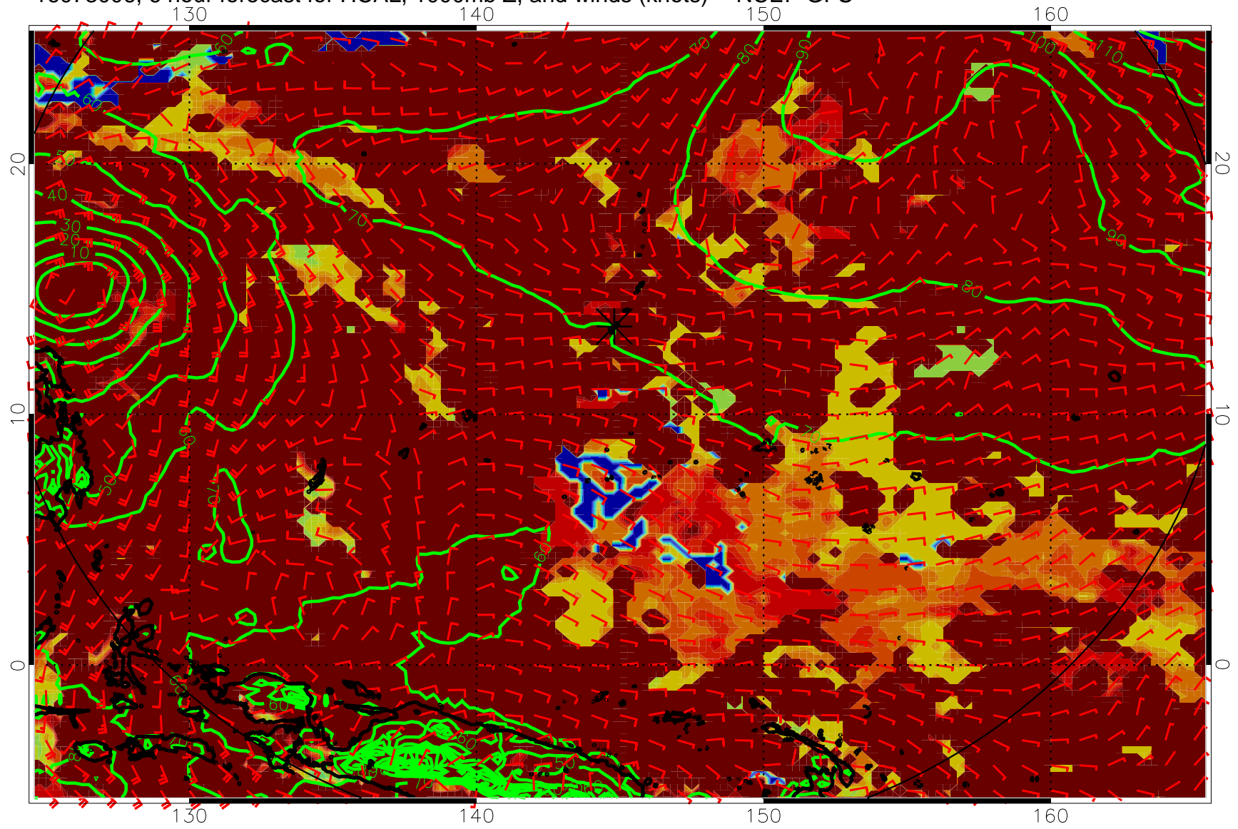
16073006, 6 hour forecast for HCAL, 1000mb Z, and winds (knots) -- NCEP GFS
