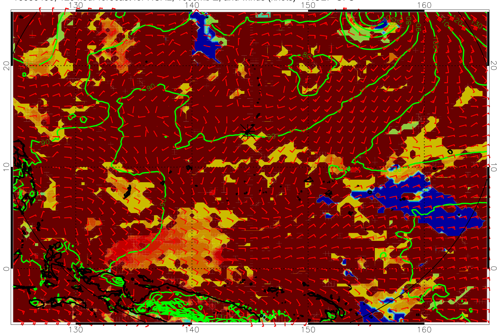
16080400, 120 hour forecast for HCAL, 1000mb Z, and winds (knots) -- NCEP GFS
