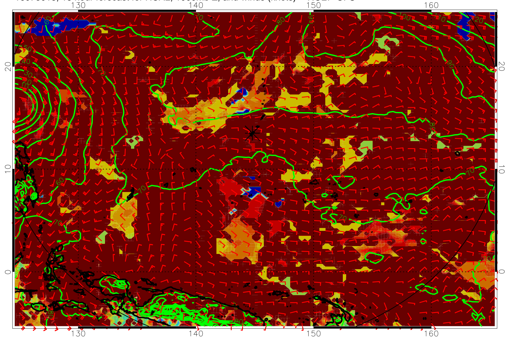
16073018, 18 hour forecast for HCAL, 1000mb Z, and winds (knots) -- NCEP GFS
