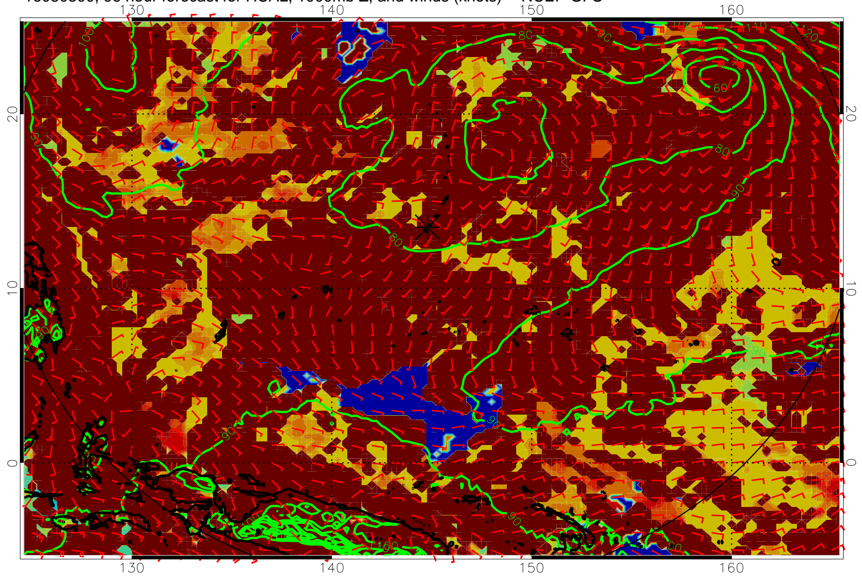
16080300, 96 hour forecast for HCAL, 1000mb Z, and winds (knots) -- NCEP GFS
