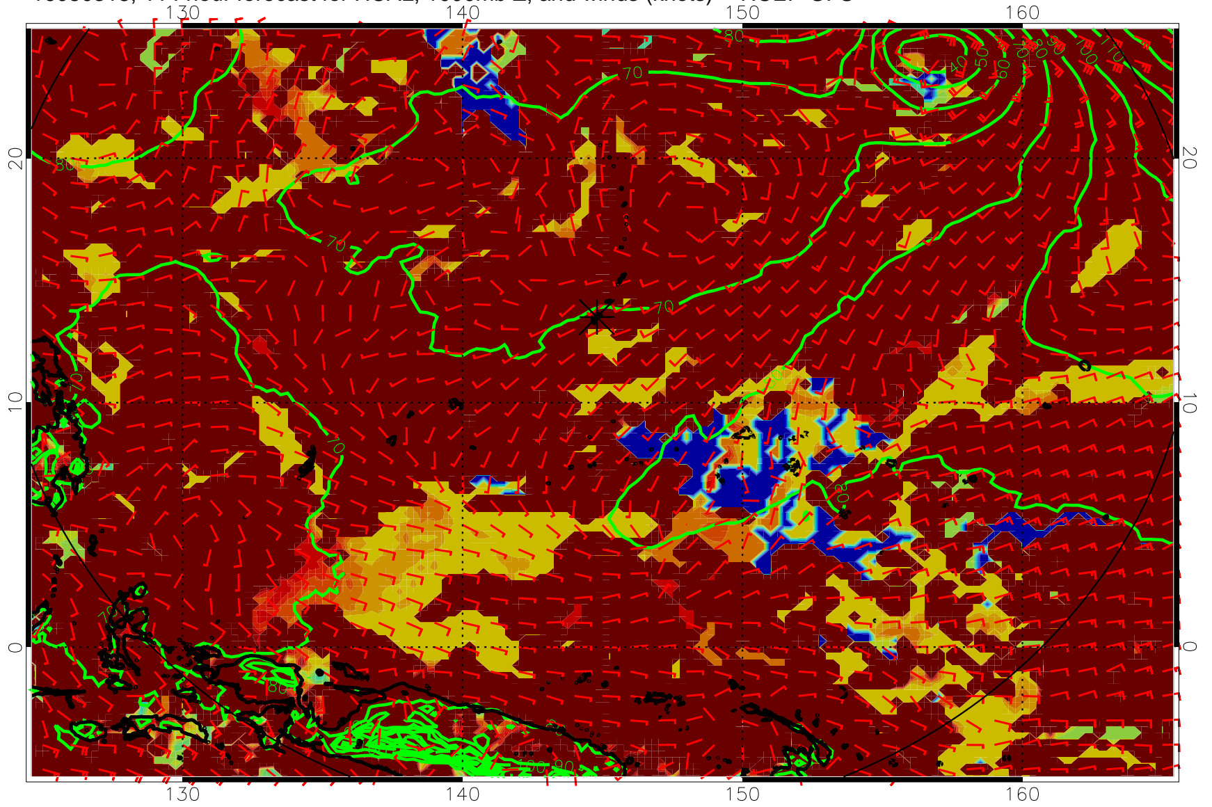
16080318, 114 hour forecast for HCAL, 1000mb Z, and winds (knots) -- NCEP GFS
