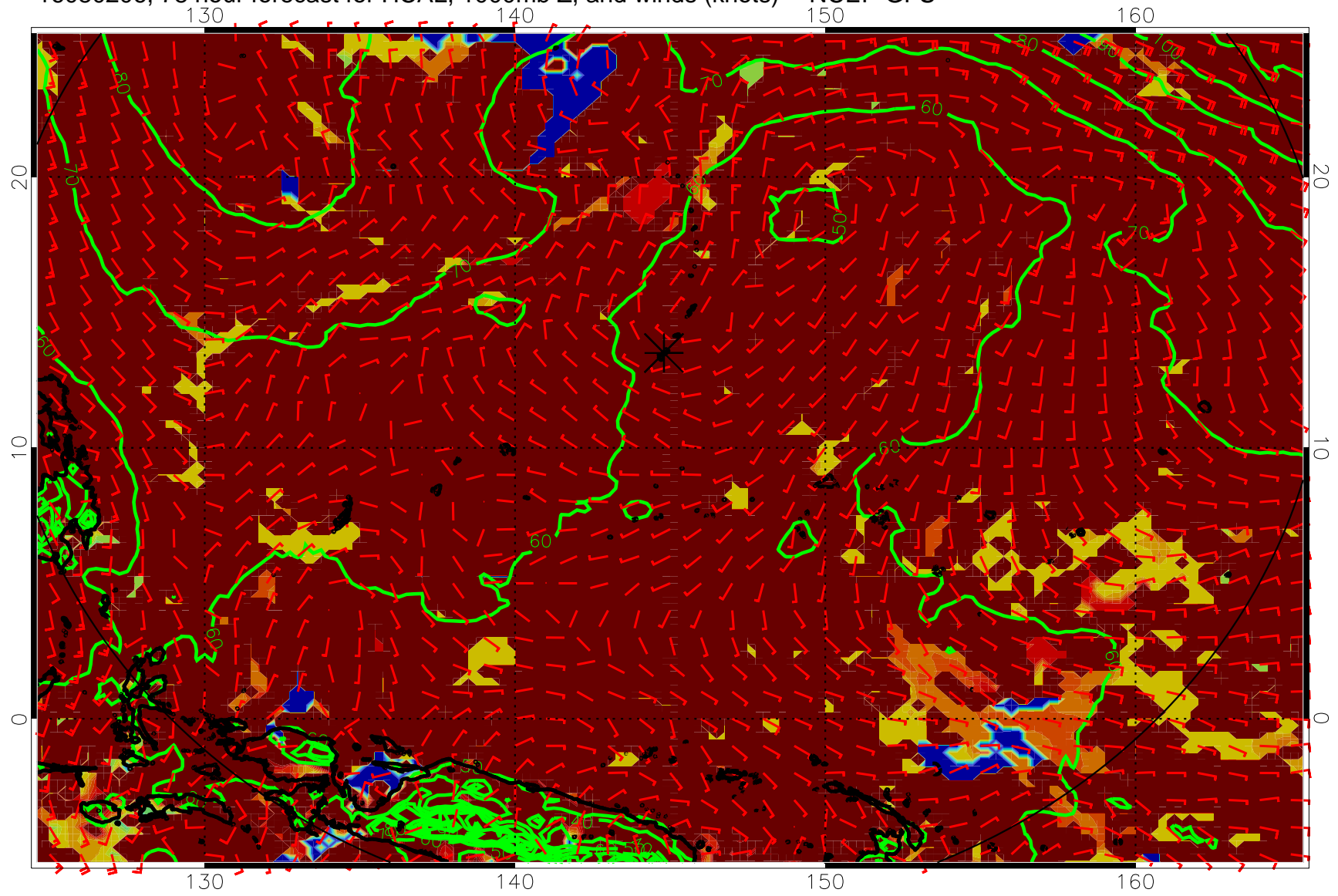
16080206, 78 hour forecast for HCAL, 1000mb Z, and winds (knots) -- NCEP GFS
