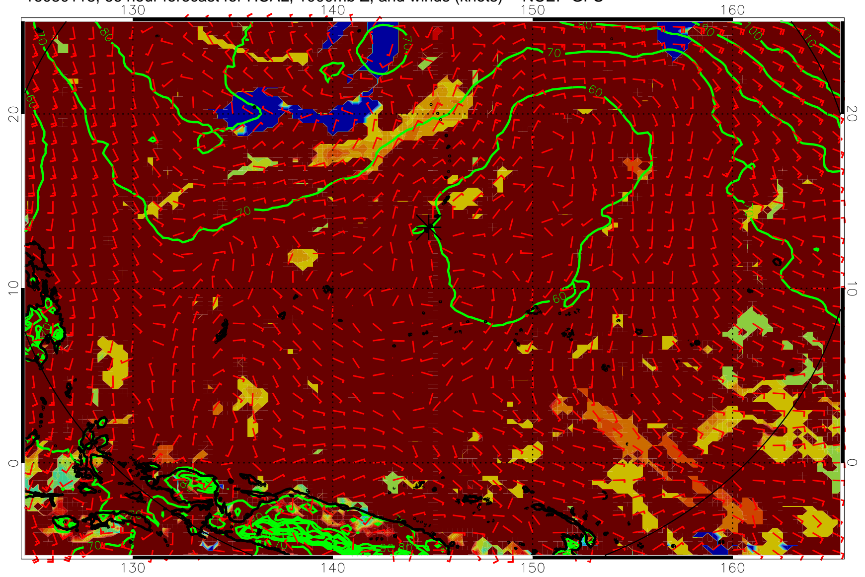
16080118, 66 hour forecast for HCAL, 1000mb Z, and winds (knots) -- NCEP GFS
