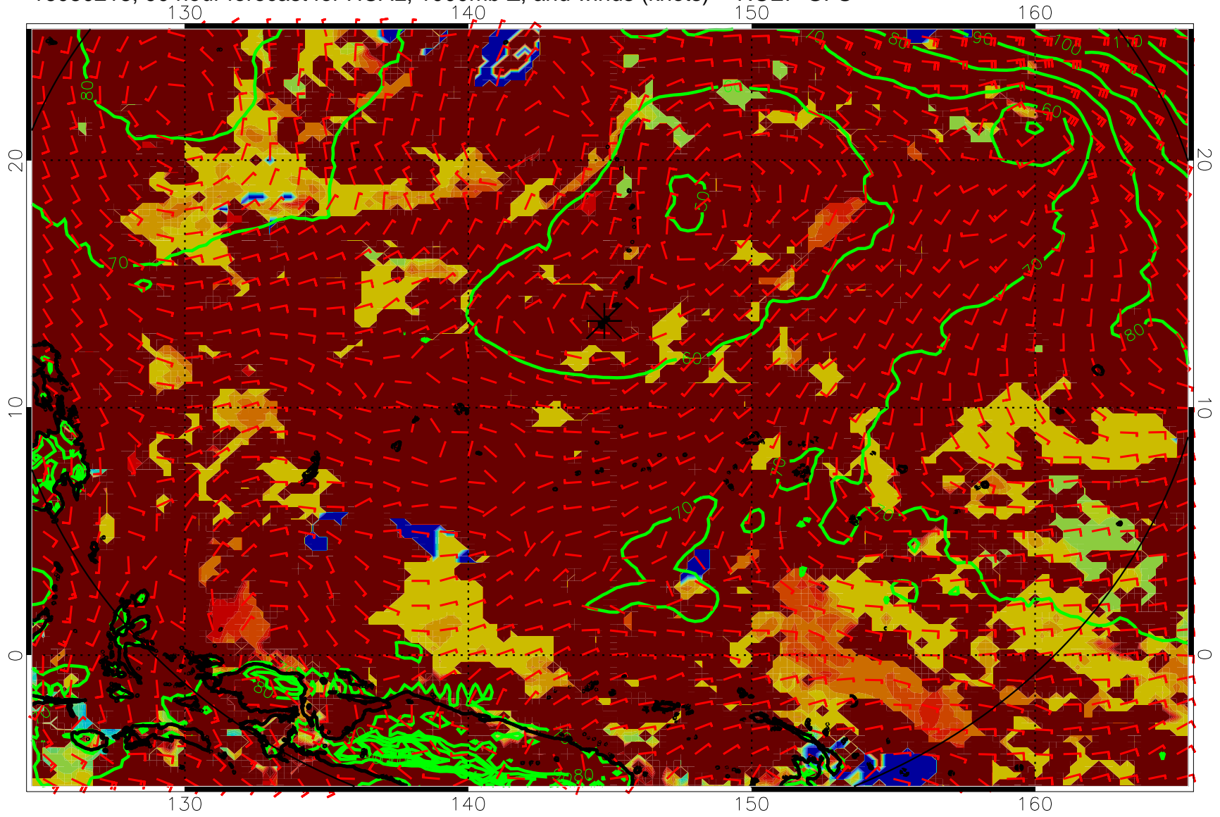
16080218, 90 hour forecast for HCAL, 1000mb Z, and winds (knots) -- NCEP GFS
