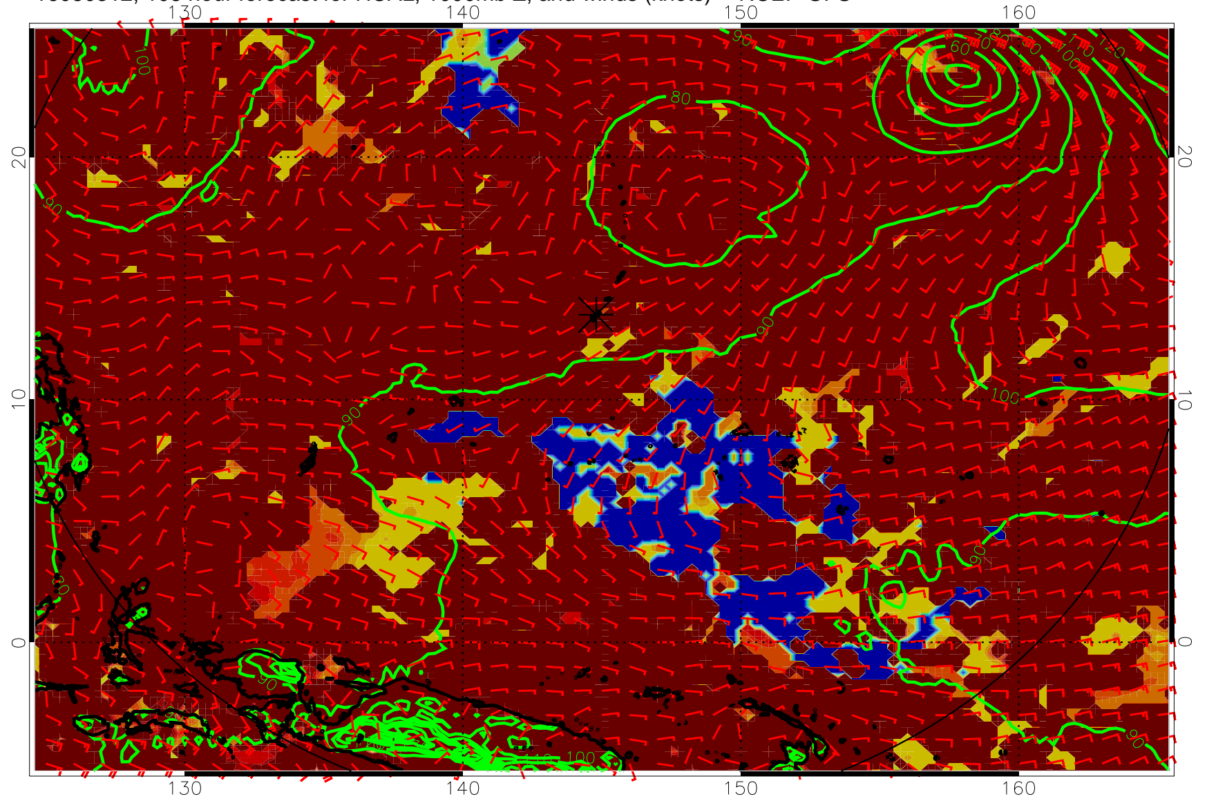
16080312, 108 hour forecast for HCAL, 1000mb Z, and winds (knots) -- NCEP GFS
