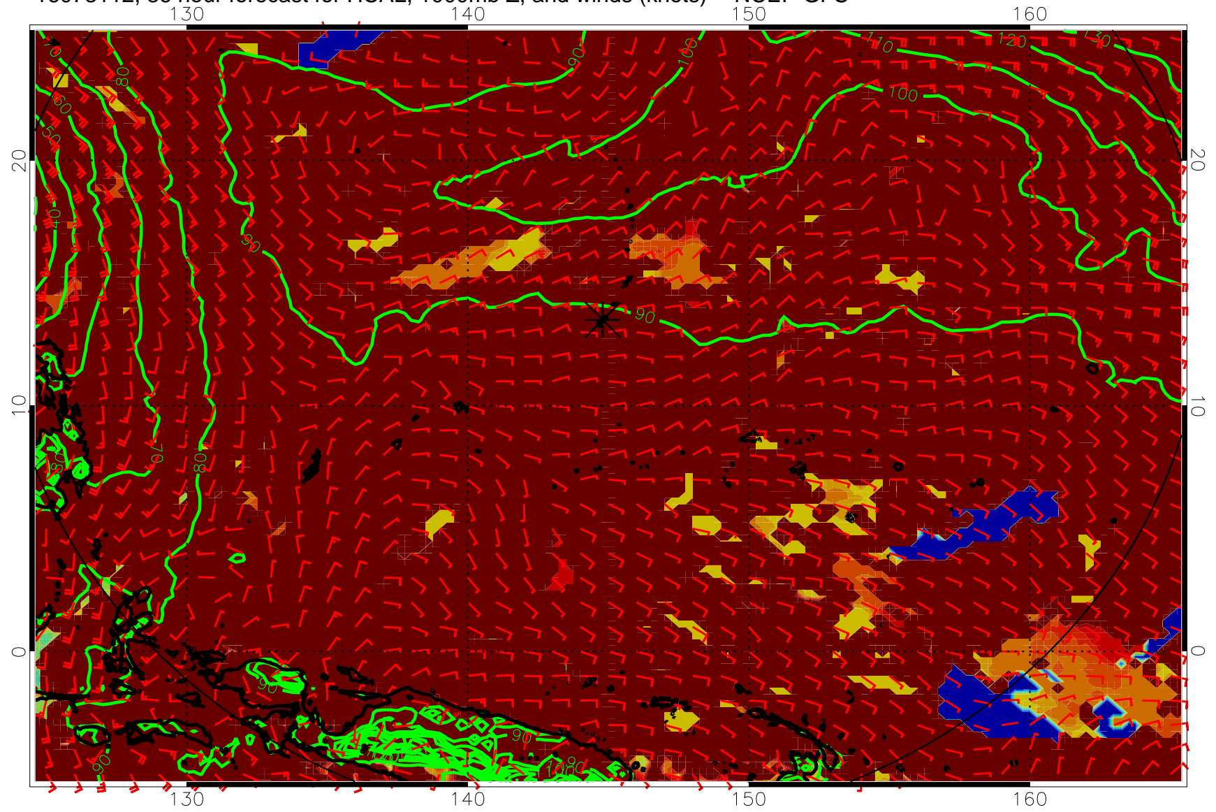
16073112, 36 hour forecast for HCAL, 1000mb Z, and winds (knots) -- NCEP GFS
