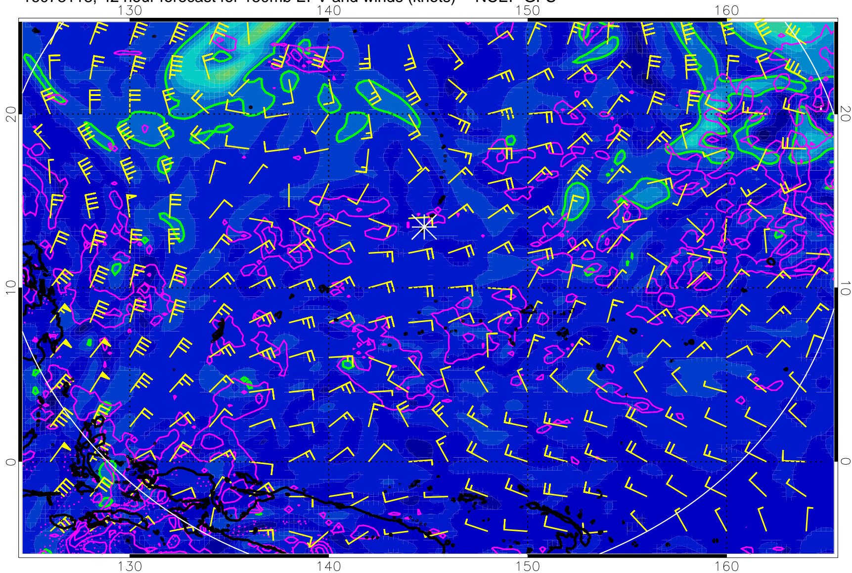
16073118, 42 hour forecast for 150mb EPV and winds (knots) -- NCEP GFS
