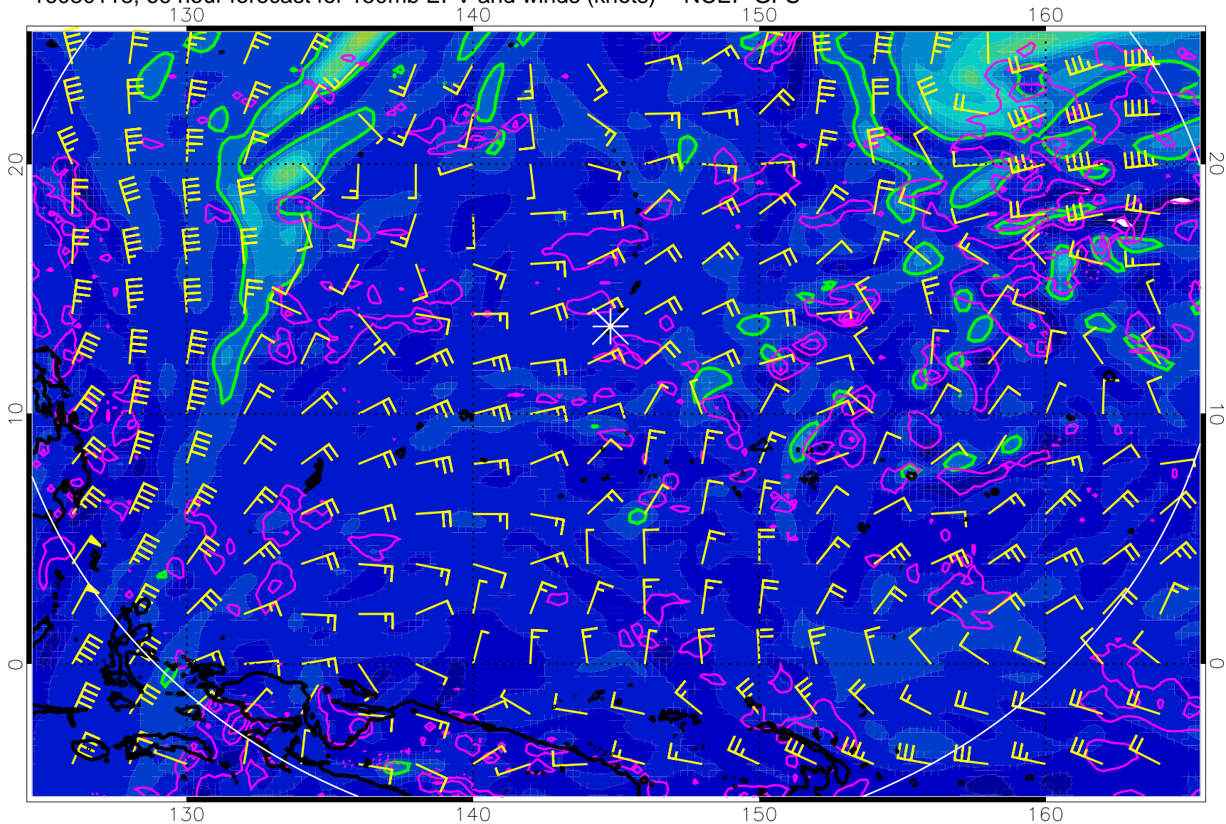
16080118, 66 hour forecast for 150mb EPV and winds (knots) -- NCEP GFS
