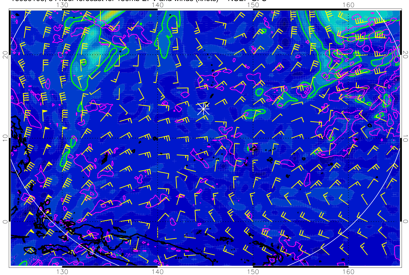
16080106, 54 hour forecast for 150mb EPV and winds (knots) -- NCEP GFS
