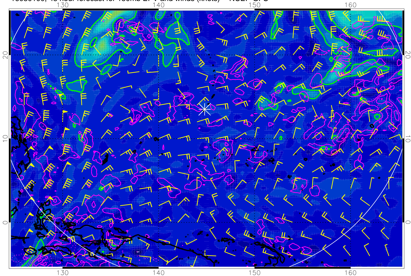
16080100, 48 hour forecast for 150mb EPV and winds (knots) -- NCEP GFS
