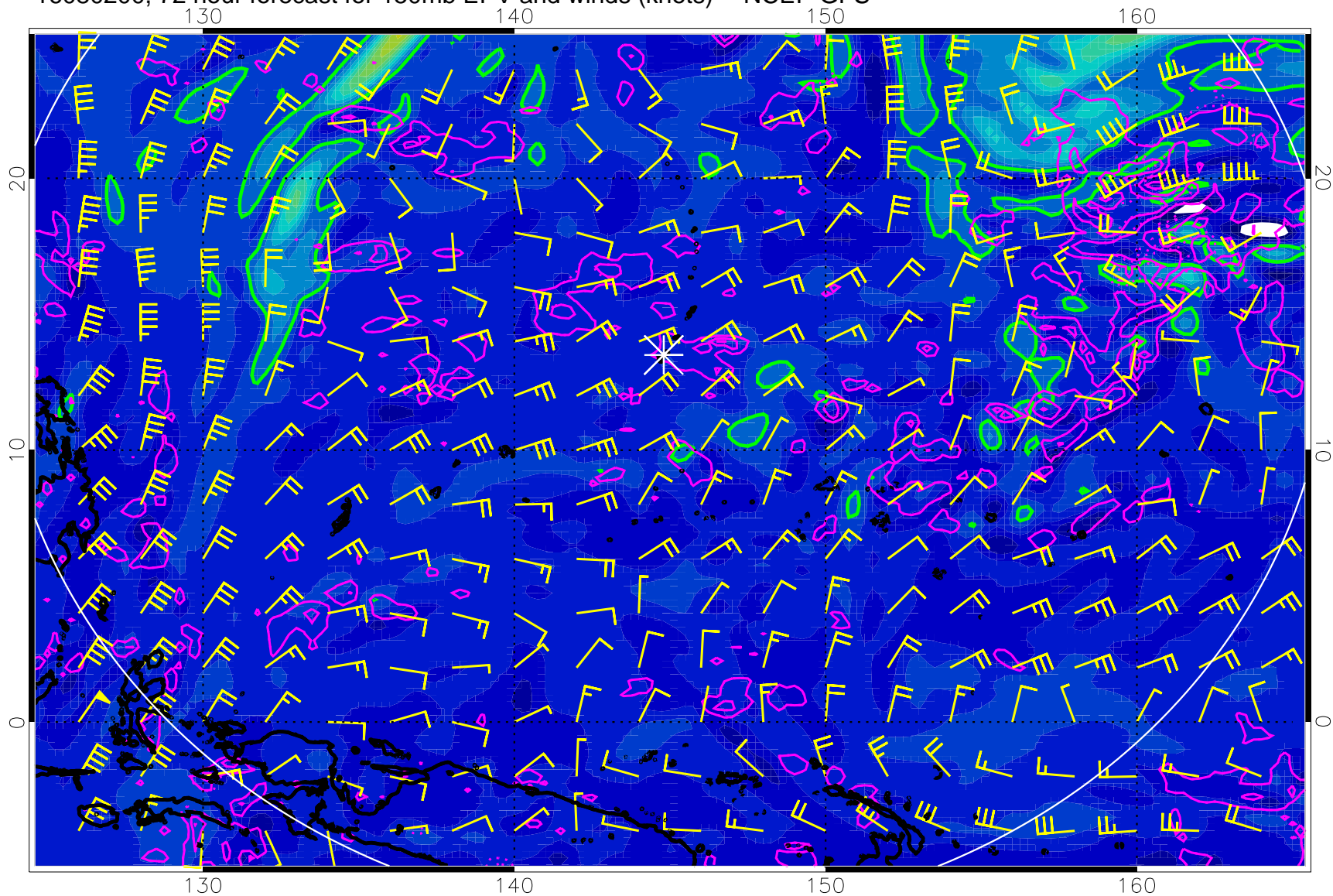
16080200, 72 hour forecast for 150mb EPV and winds (knots) -- NCEP GFS
