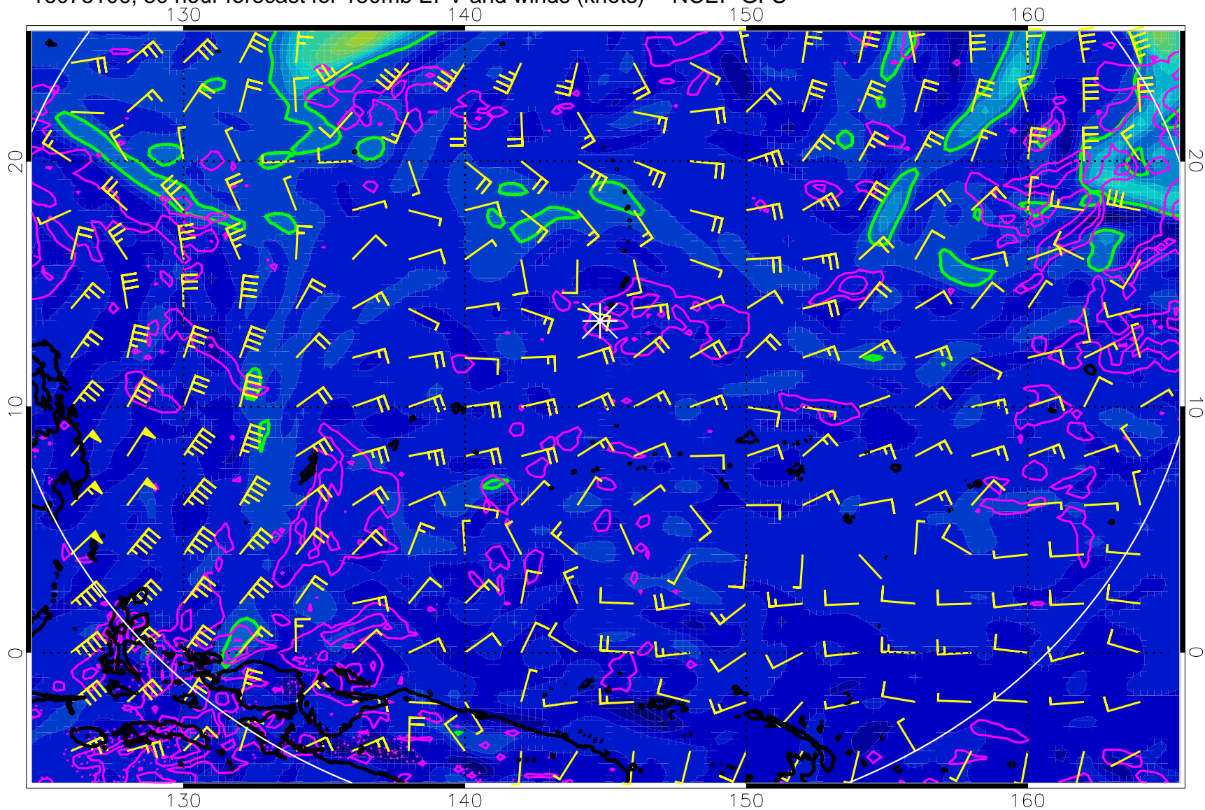
16073106, 30 hour forecast for 150mb EPV and winds (knots) -- NCEP GFS
