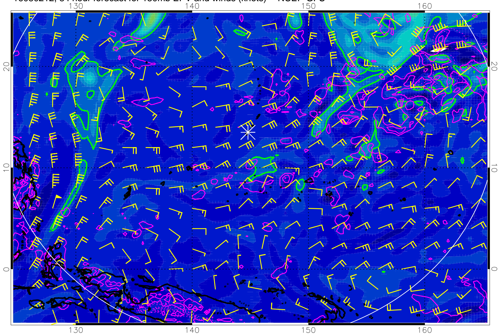
16080212, 84 hour forecast for 150mb EPV and winds (knots) -- NCEP GFS
