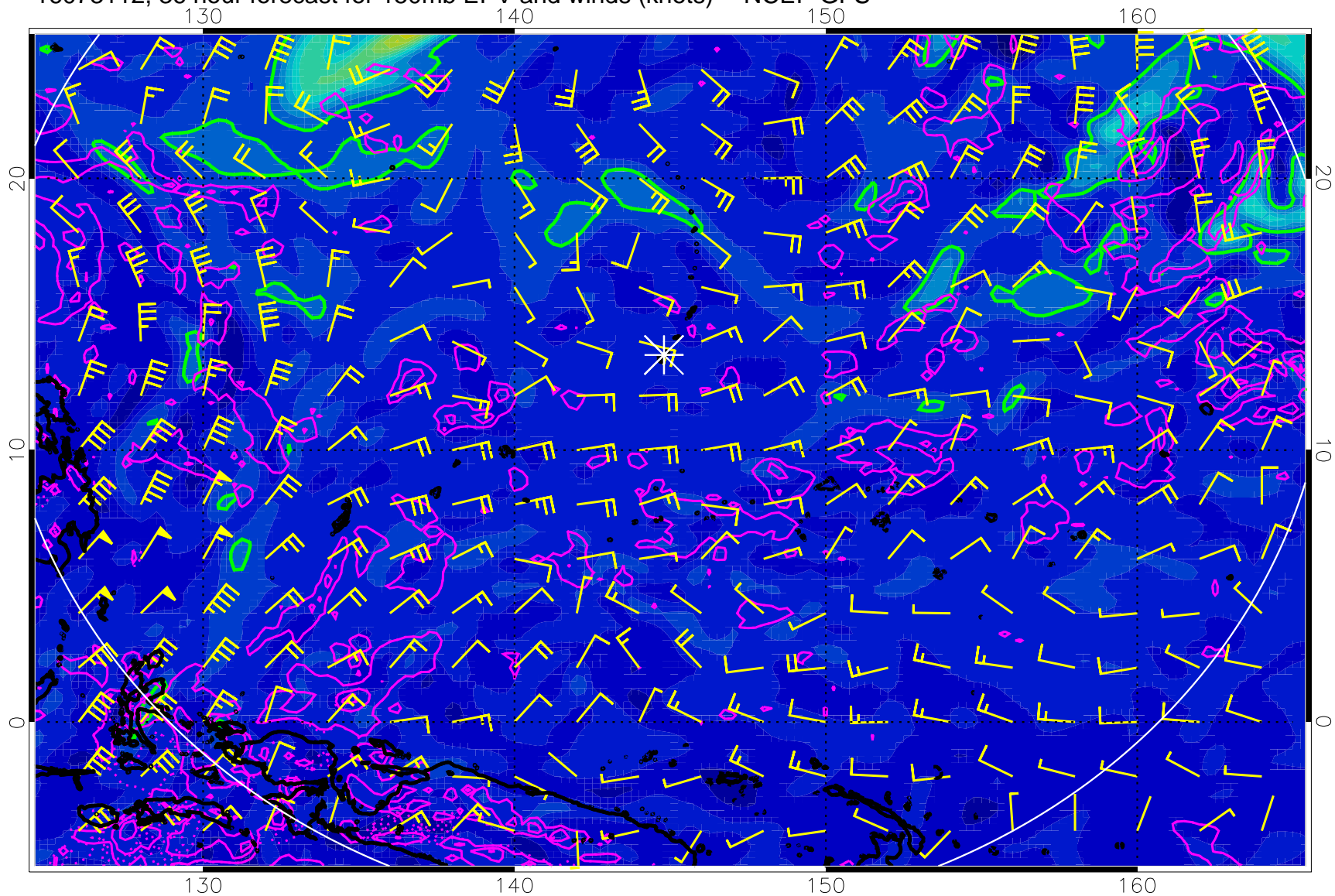
16073112, 36 hour forecast for 150mb EPV and winds (knots) -- NCEP GFS
