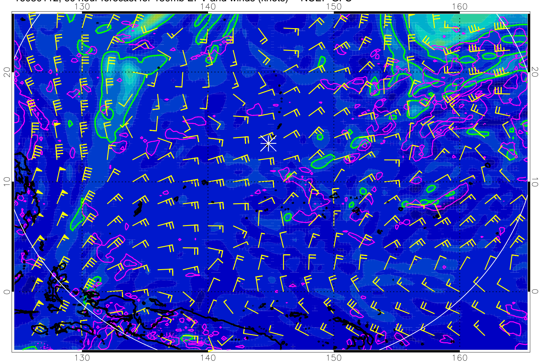
16080112, 60 hour forecast for 150mb EPV and winds (knots) -- NCEP GFS
