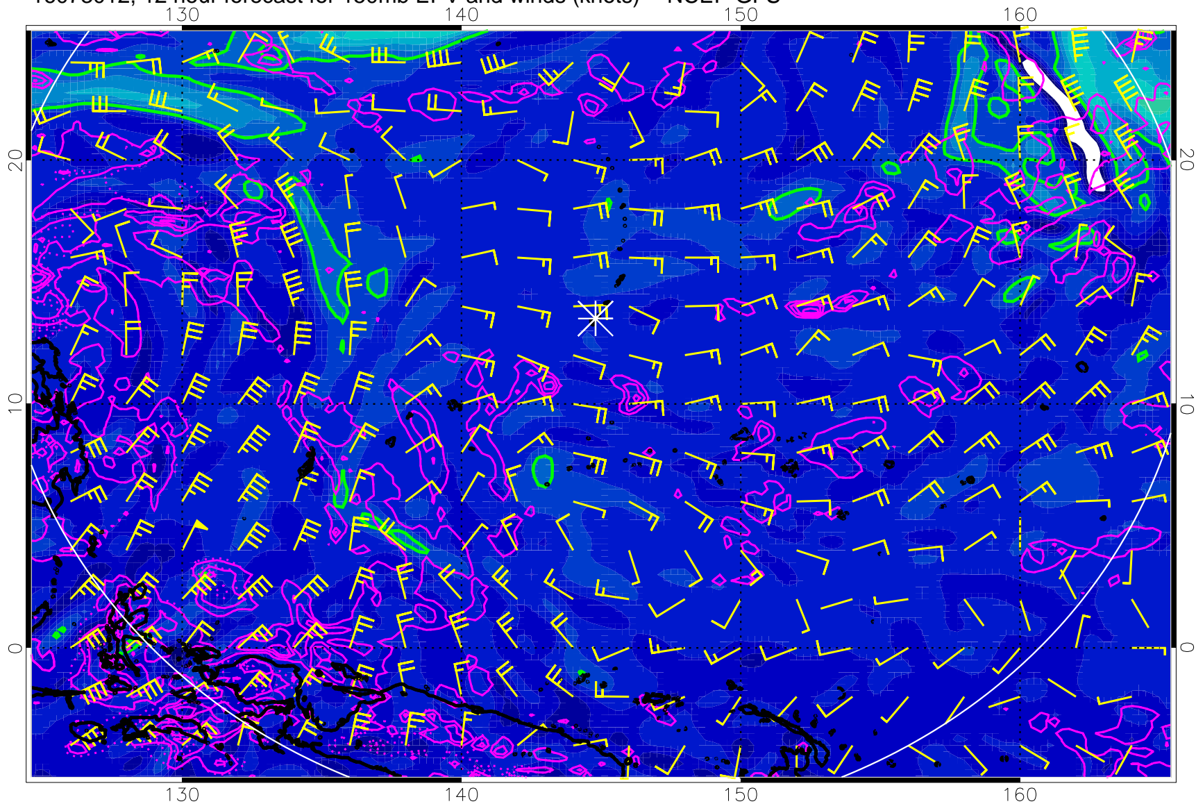
16073012, 12 hour forecast for 150mb EPV and winds (knots) -- NCEP GFS
