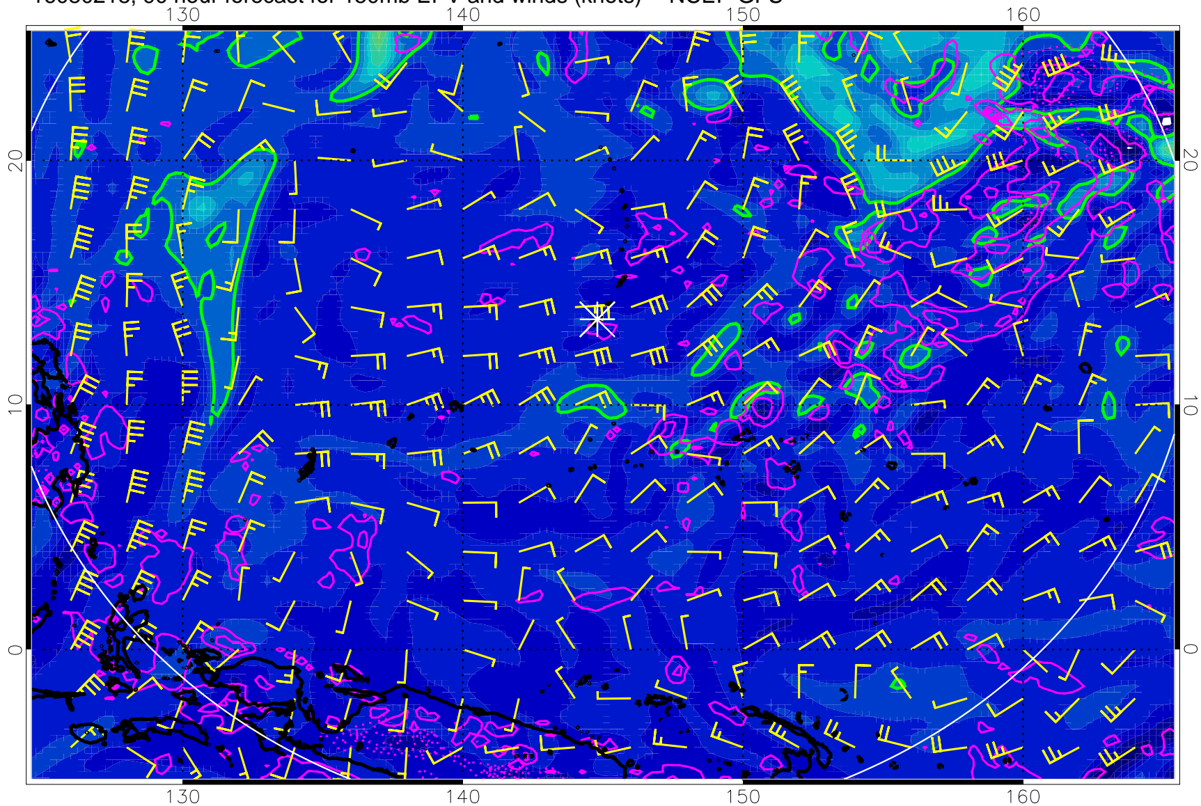
16080218, 90 hour forecast for 150mb EPV and winds (knots) -- NCEP GFS
