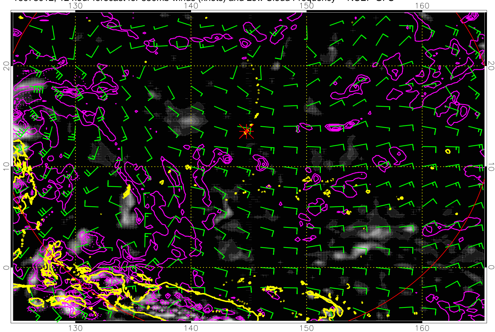
16073012, 12 hour forecast for 850mb winds (knots) and Low Cloud Frequency -- NCEP GFS
