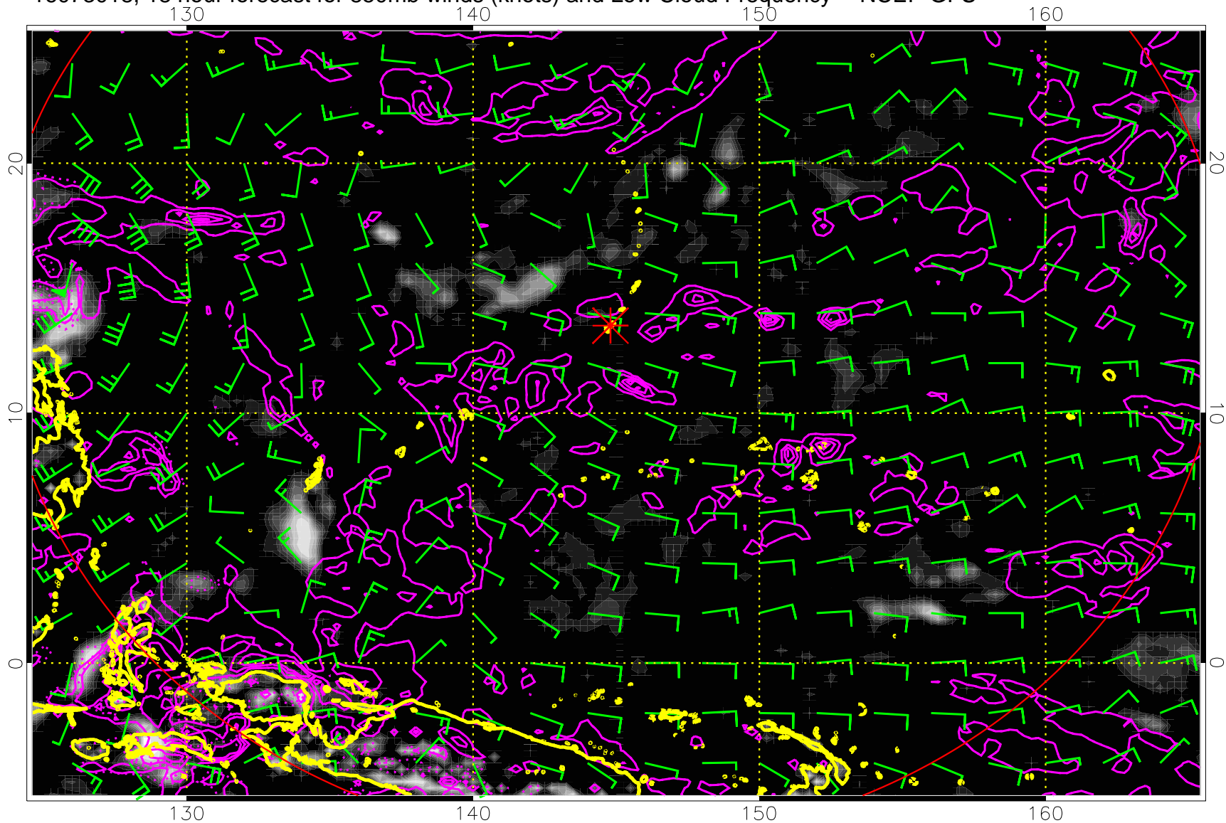
16073018, 18 hour forecast for 850mb winds (knots) and Low Cloud Frequency -- NCEP GFS
