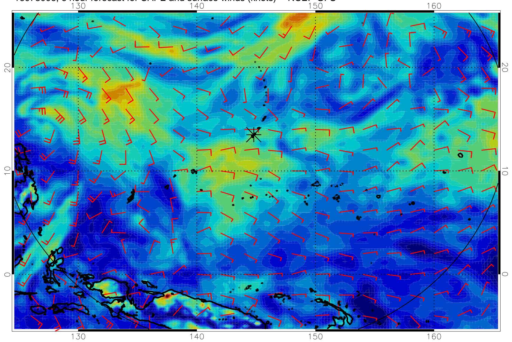
16073006, 6 hour forecast for CAPE and surface winds (knots) -- NCEP GFS
