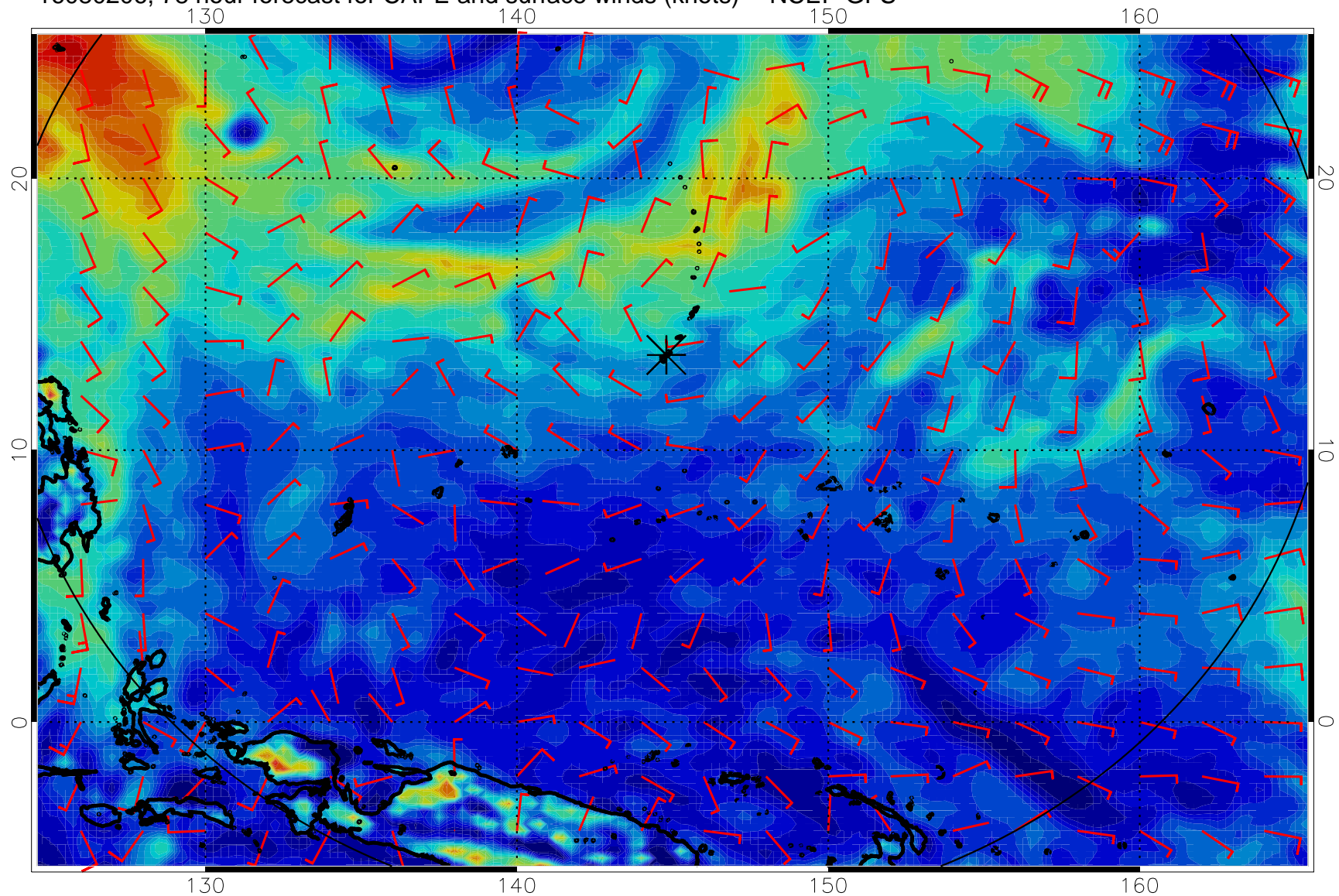
16080206, 78 hour forecast for CAPE and surface winds (knots) -- NCEP GFS
