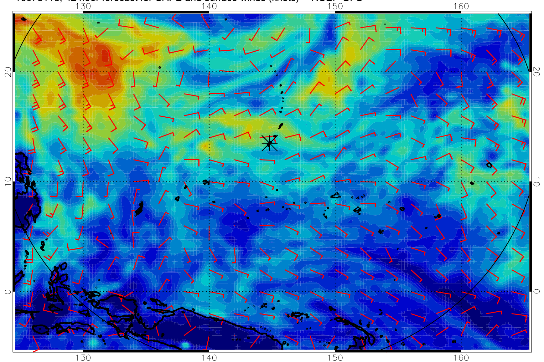
16073118, 42 hour forecast for CAPE and surface winds (knots) -- NCEP GFS
