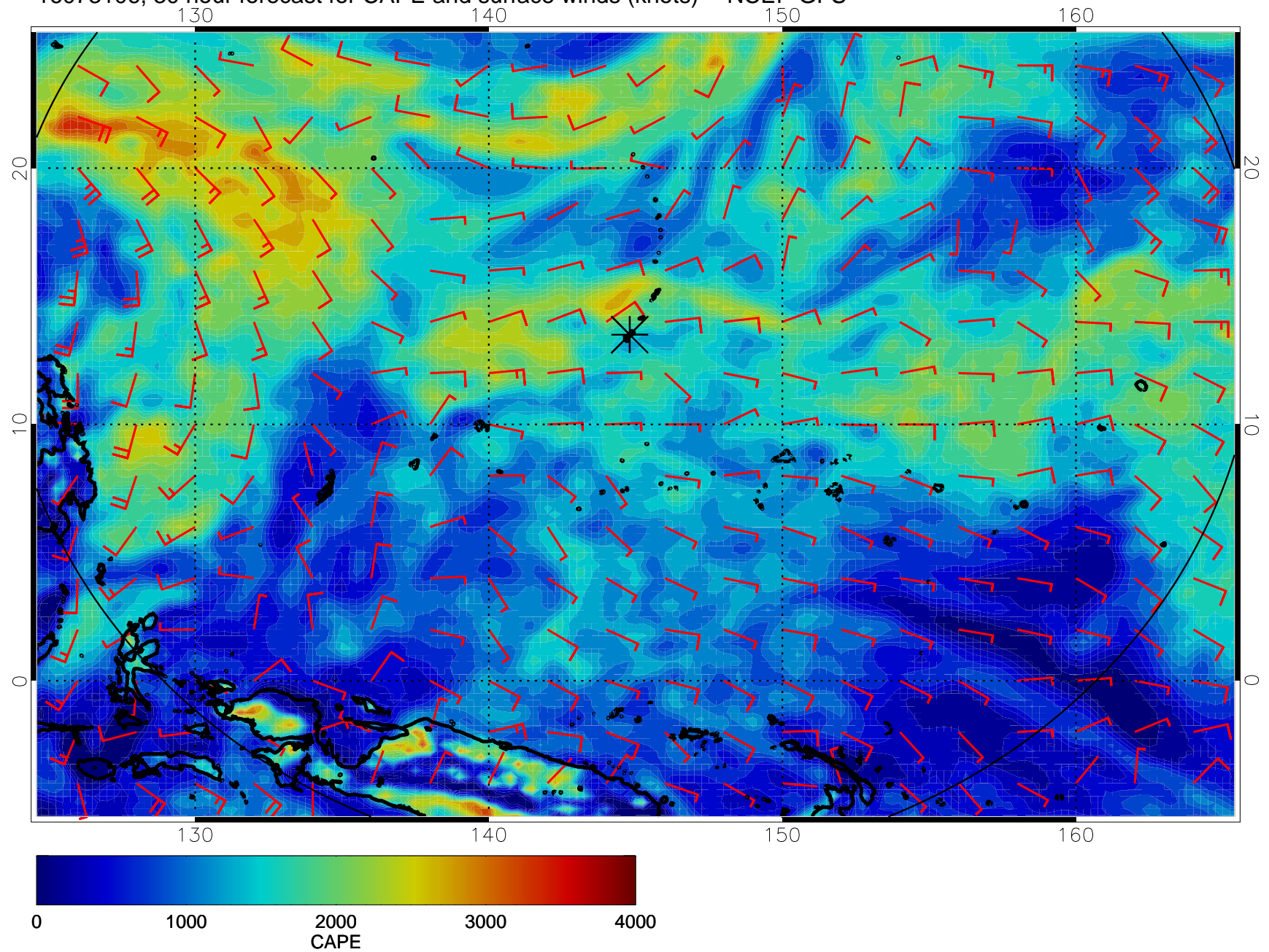
16073106, 30 hour forecast for CAPE and surface winds (knots) -- NCEP GFS
