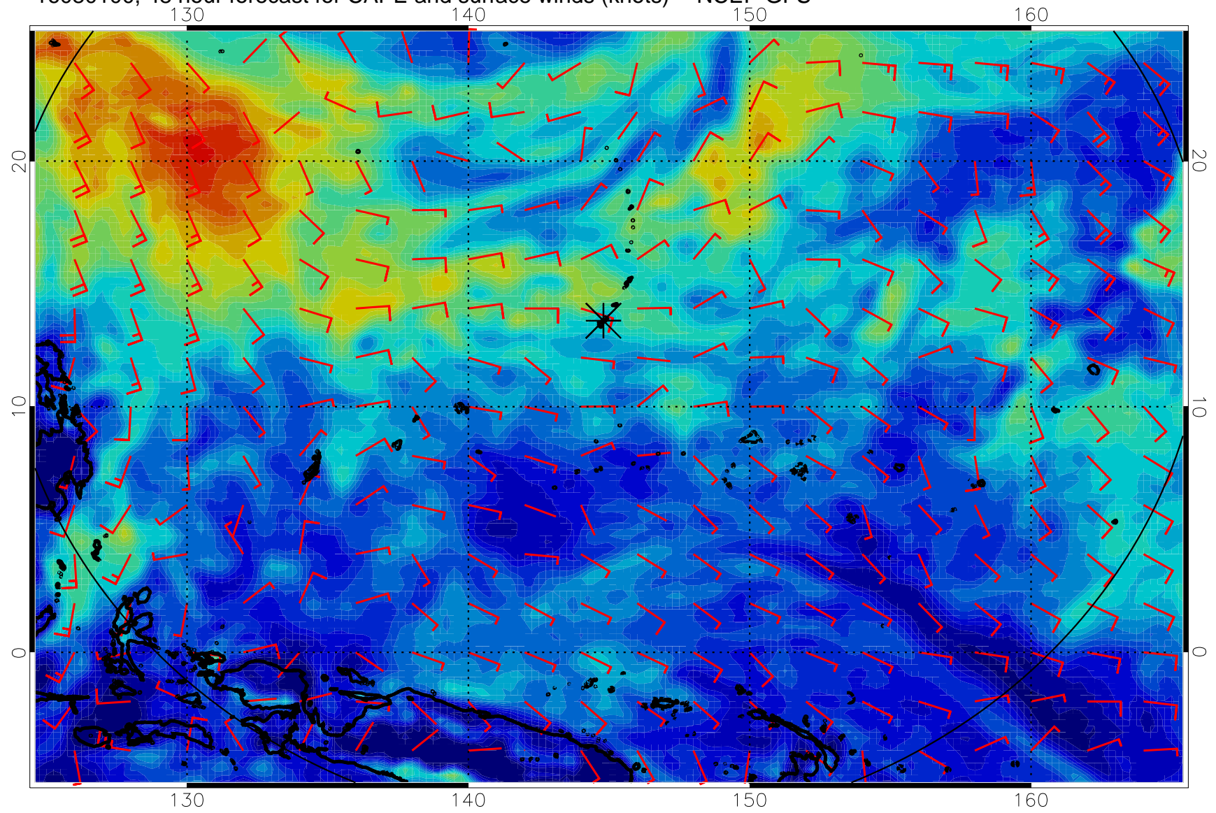
16080100, 48 hour forecast for CAPE and surface winds (knots) -- NCEP GFS
