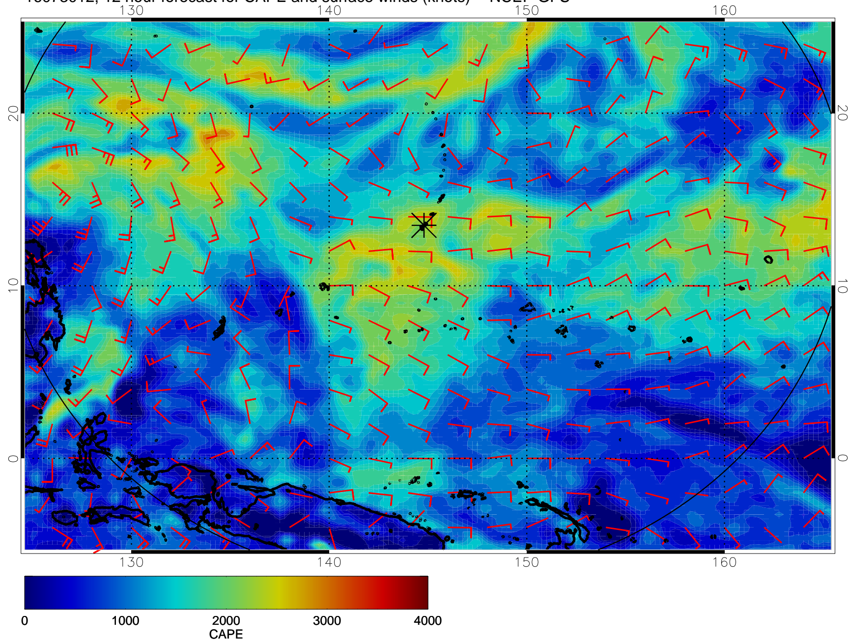
16073012, 12 hour forecast for CAPE and surface winds (knots) -- NCEP GFS
