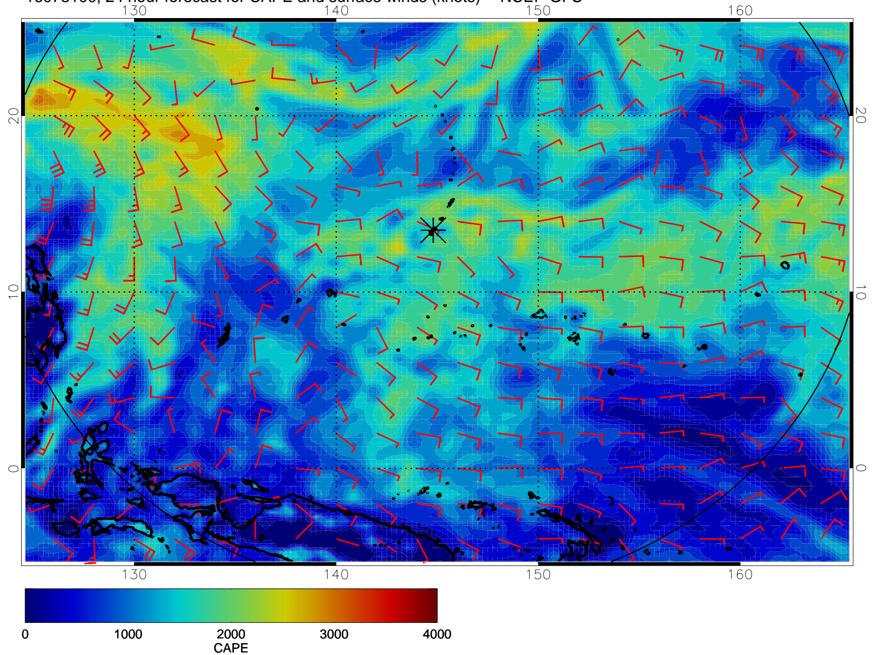
16073100, 24 hour forecast for CAPE and surface winds (knots) -- NCEP GFS
