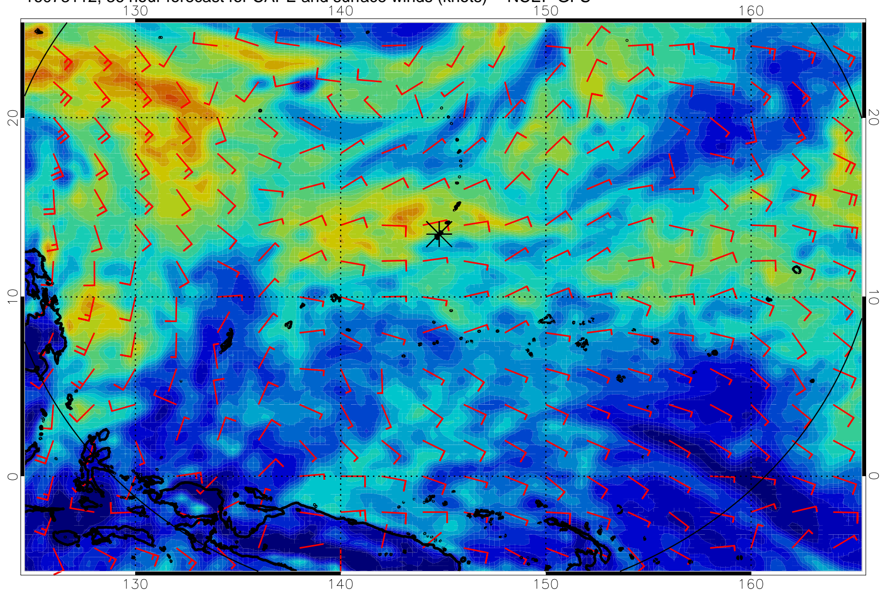
16073112, 36 hour forecast for CAPE and surface winds (knots) -- NCEP GFS
