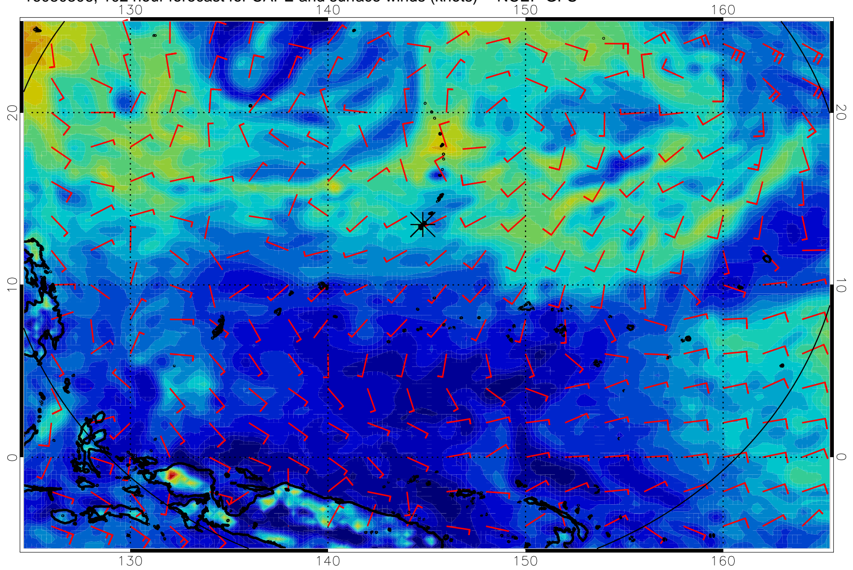
16080306, 102 hour forecast for CAPE and surface winds (knots) -- NCEP GFS
