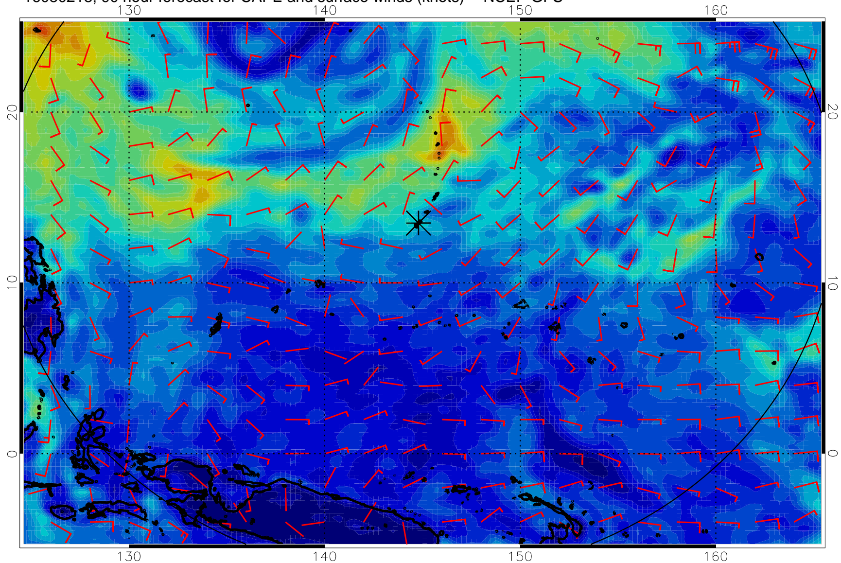
16080218, 90 hour forecast for CAPE and surface winds (knots) -- NCEP GFS
