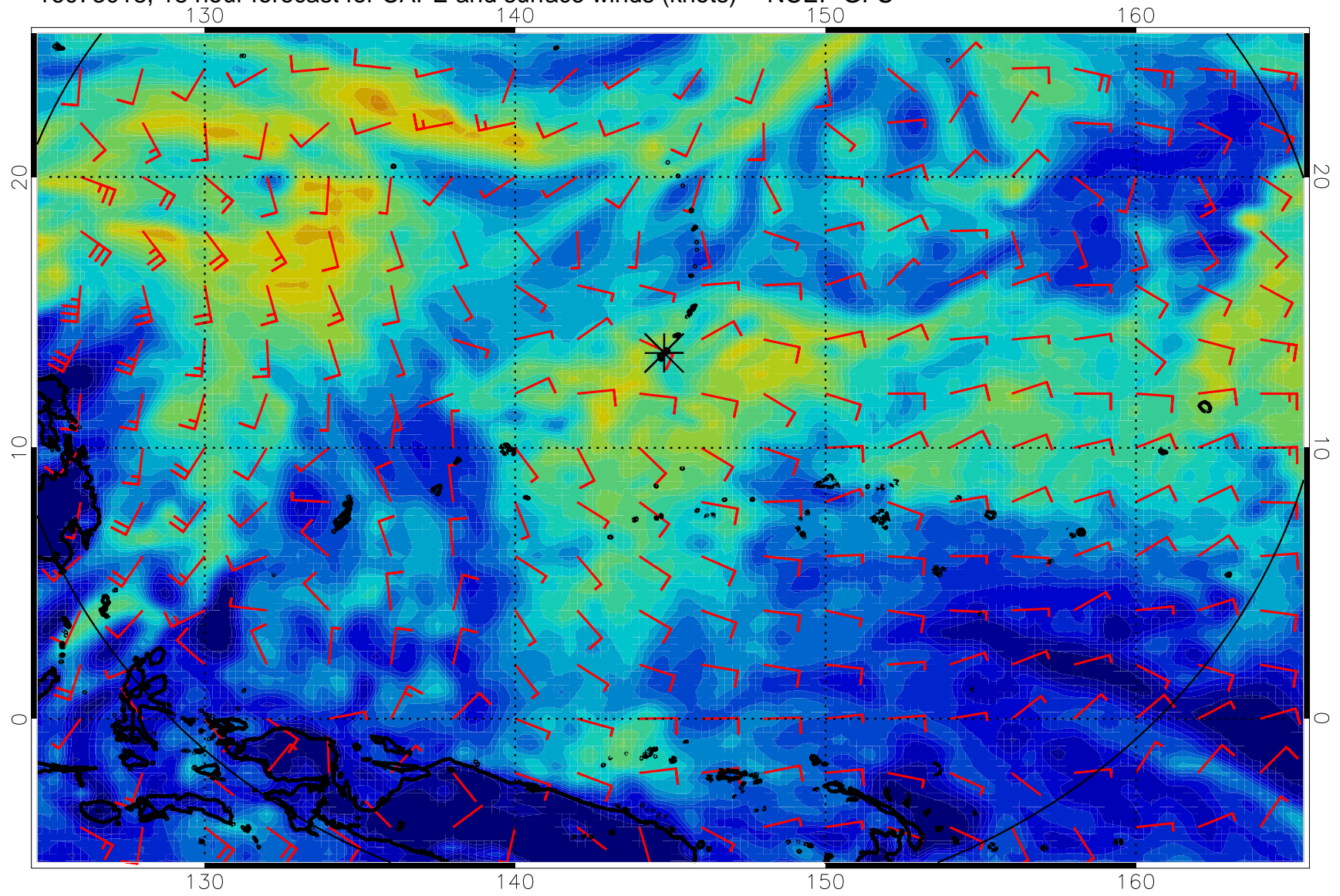
16073018, 18 hour forecast for CAPE and surface winds (knots) -- NCEP GFS
