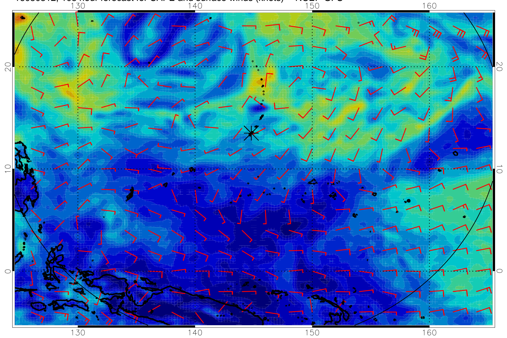
16080312, 108 hour forecast for CAPE and surface winds (knots) -- NCEP GFS
