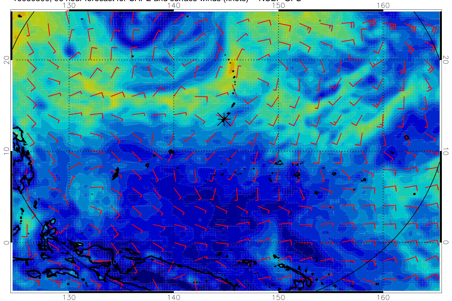
16080300, 96 hour forecast for CAPE and surface winds (knots) -- NCEP GFS
