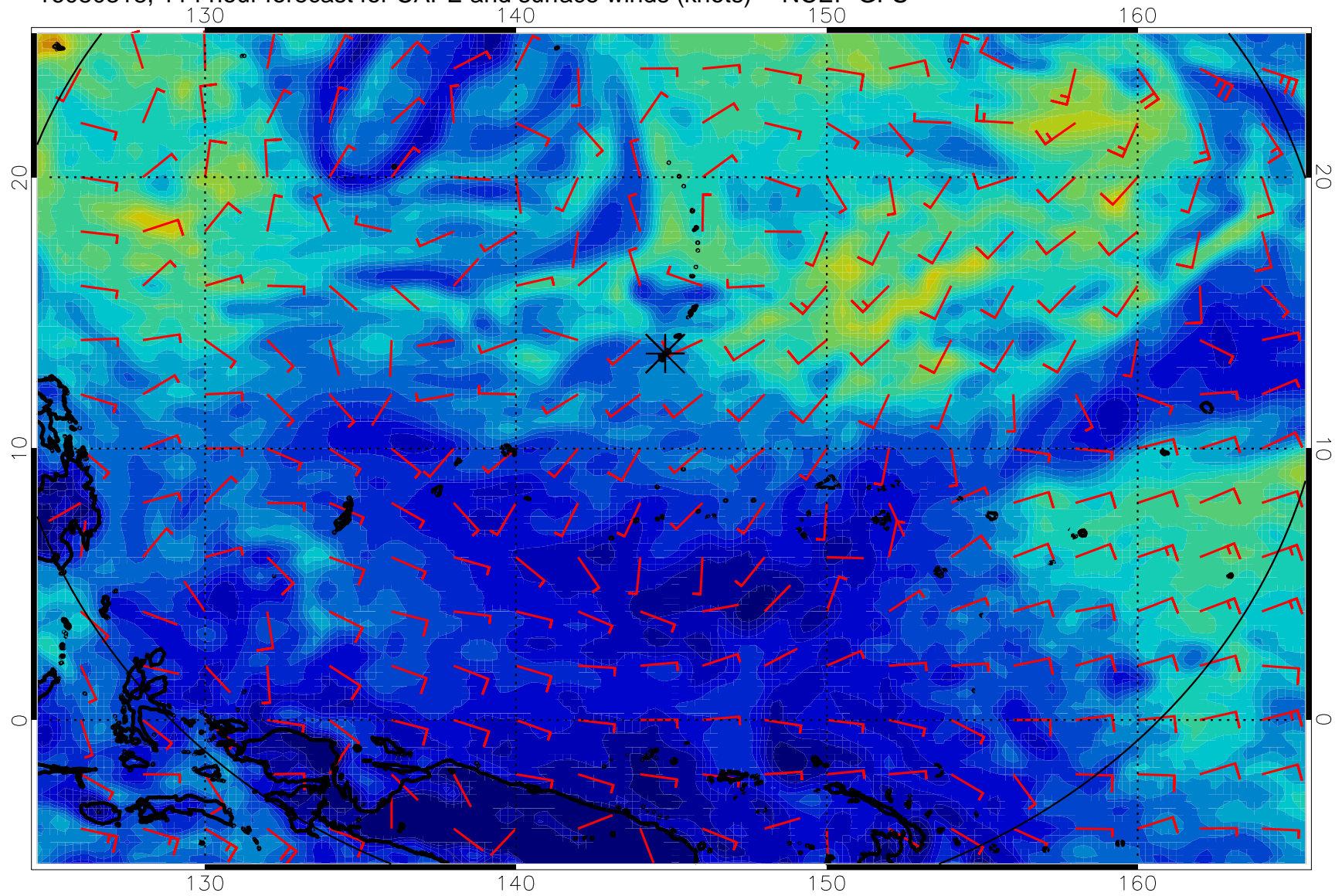
16080318, 114 hour forecast for CAPE and surface winds (knots) -- NCEP GFS
