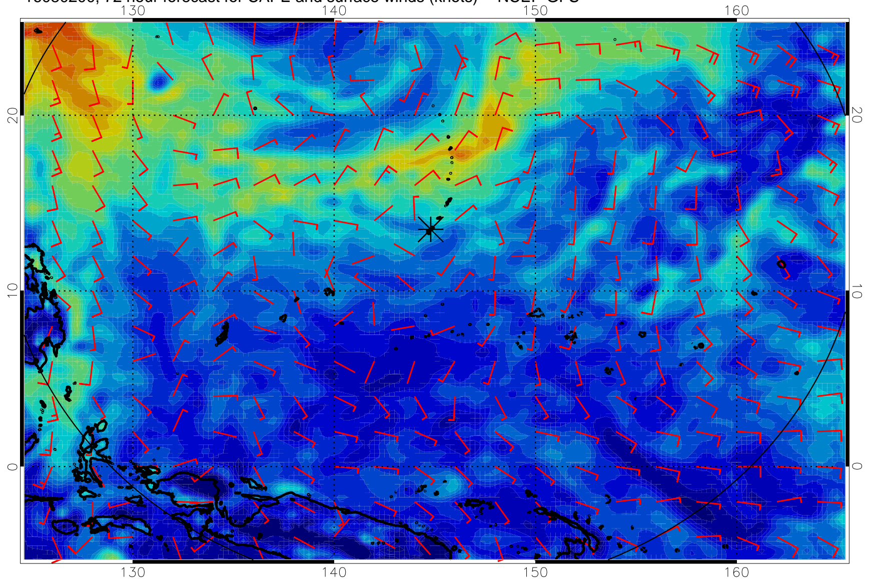
16080200, 72 hour forecast for CAPE and surface winds (knots) -- NCEP GFS
