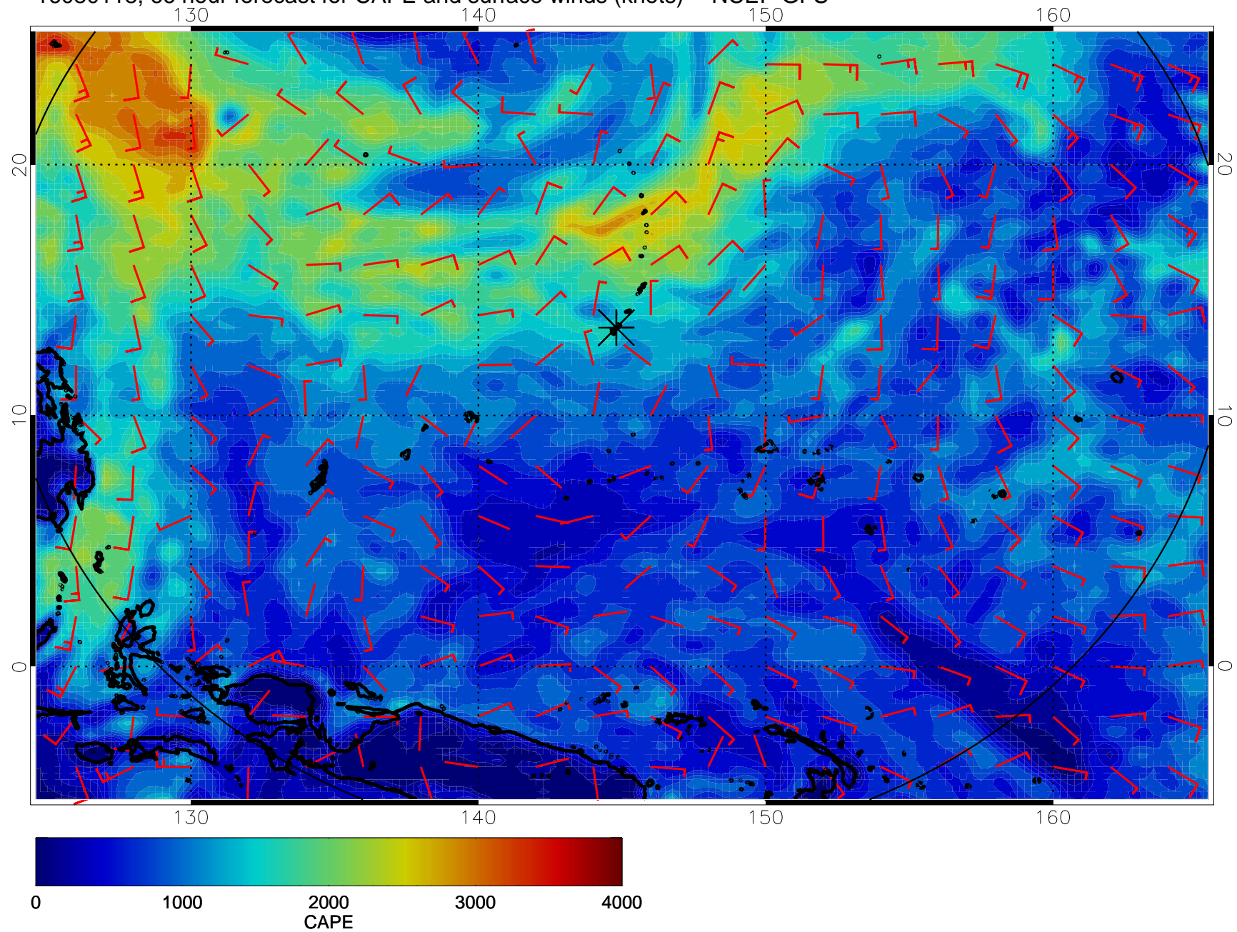
16080118, 66 hour forecast for CAPE and surface winds (knots) -- NCEP GFS
