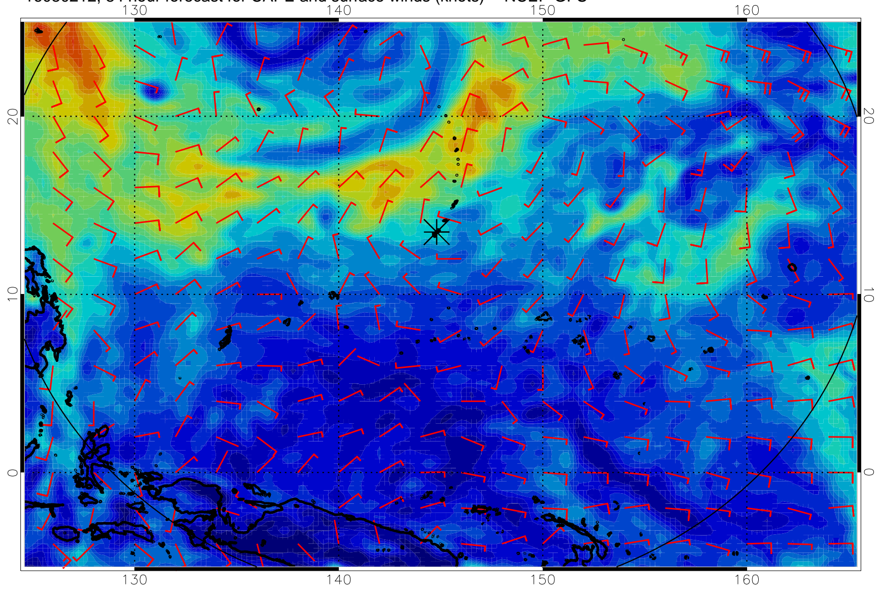
16080212, 84 hour forecast for CAPE and surface winds (knots) -- NCEP GFS
