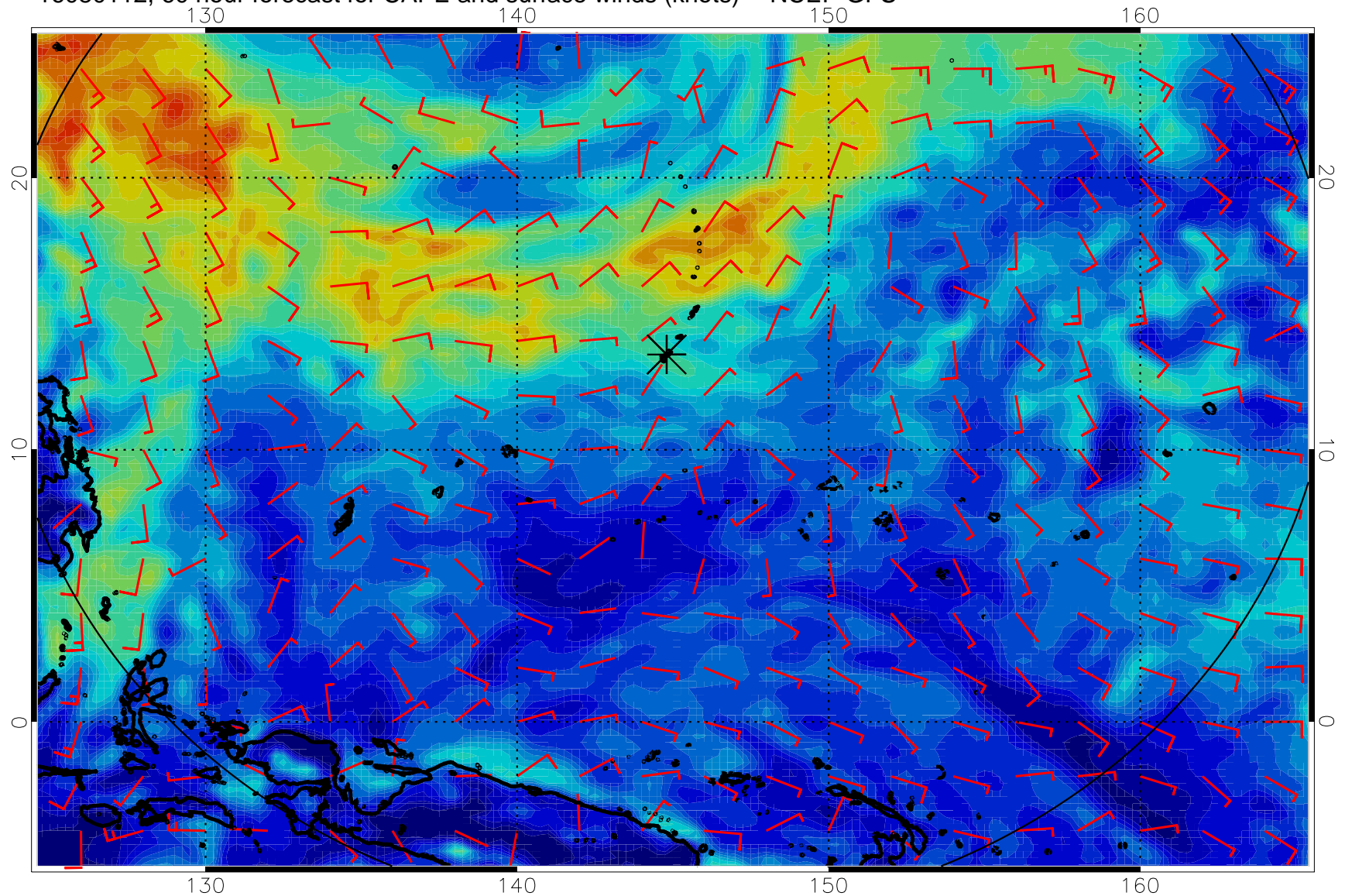
16080112, 60 hour forecast for CAPE and surface winds (knots) -- NCEP GFS
