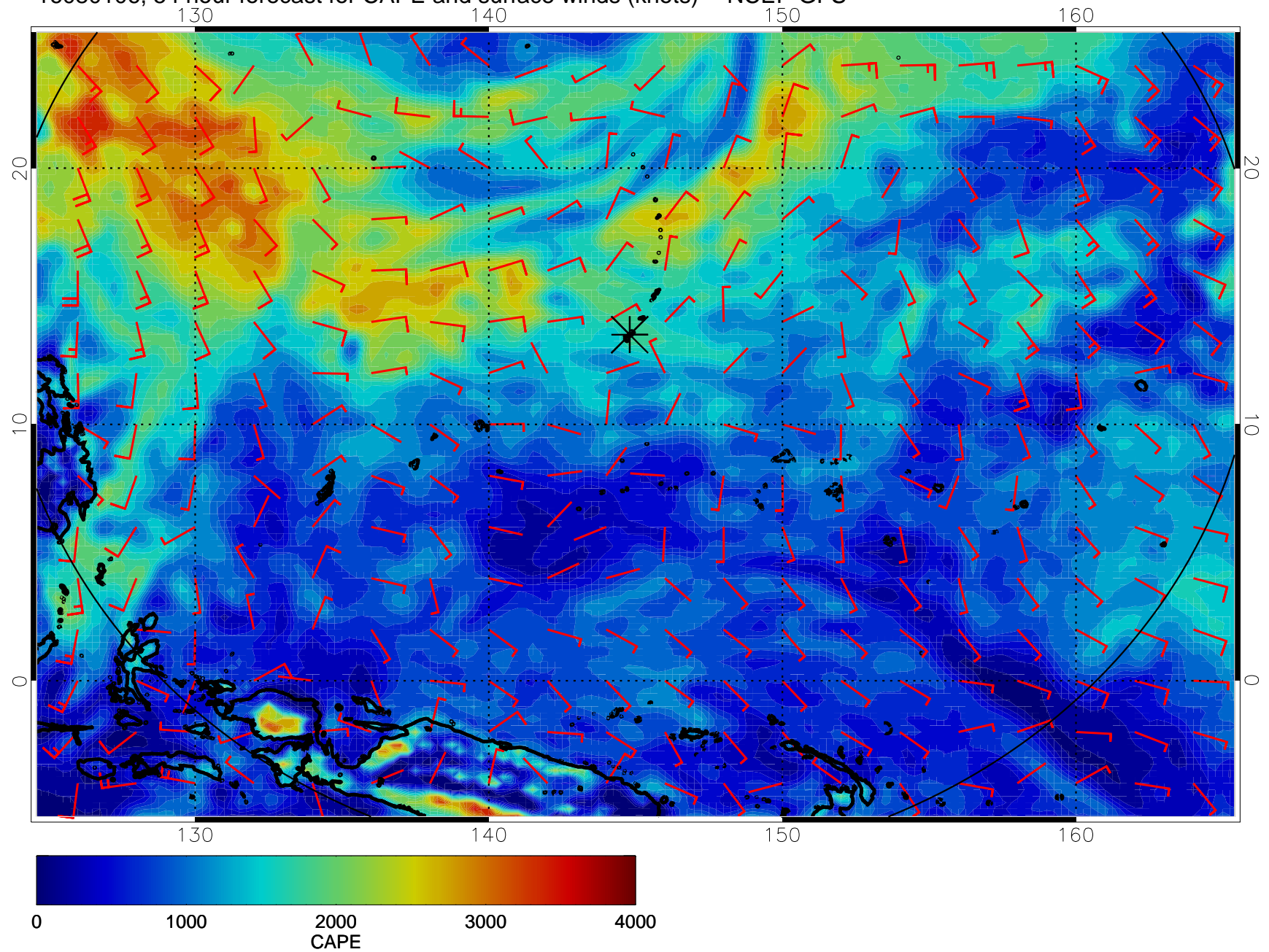
16080106, 54 hour forecast for CAPE and surface winds (knots) -- NCEP GFS
