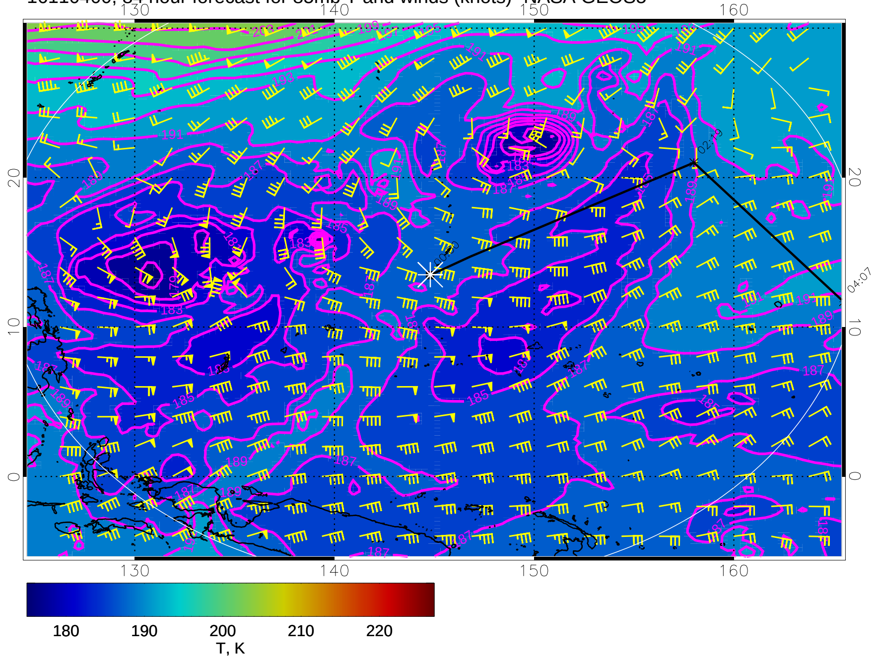
16110400, 84 hour forecast for 85mb T and winds (knots)- NASA GEOS5
