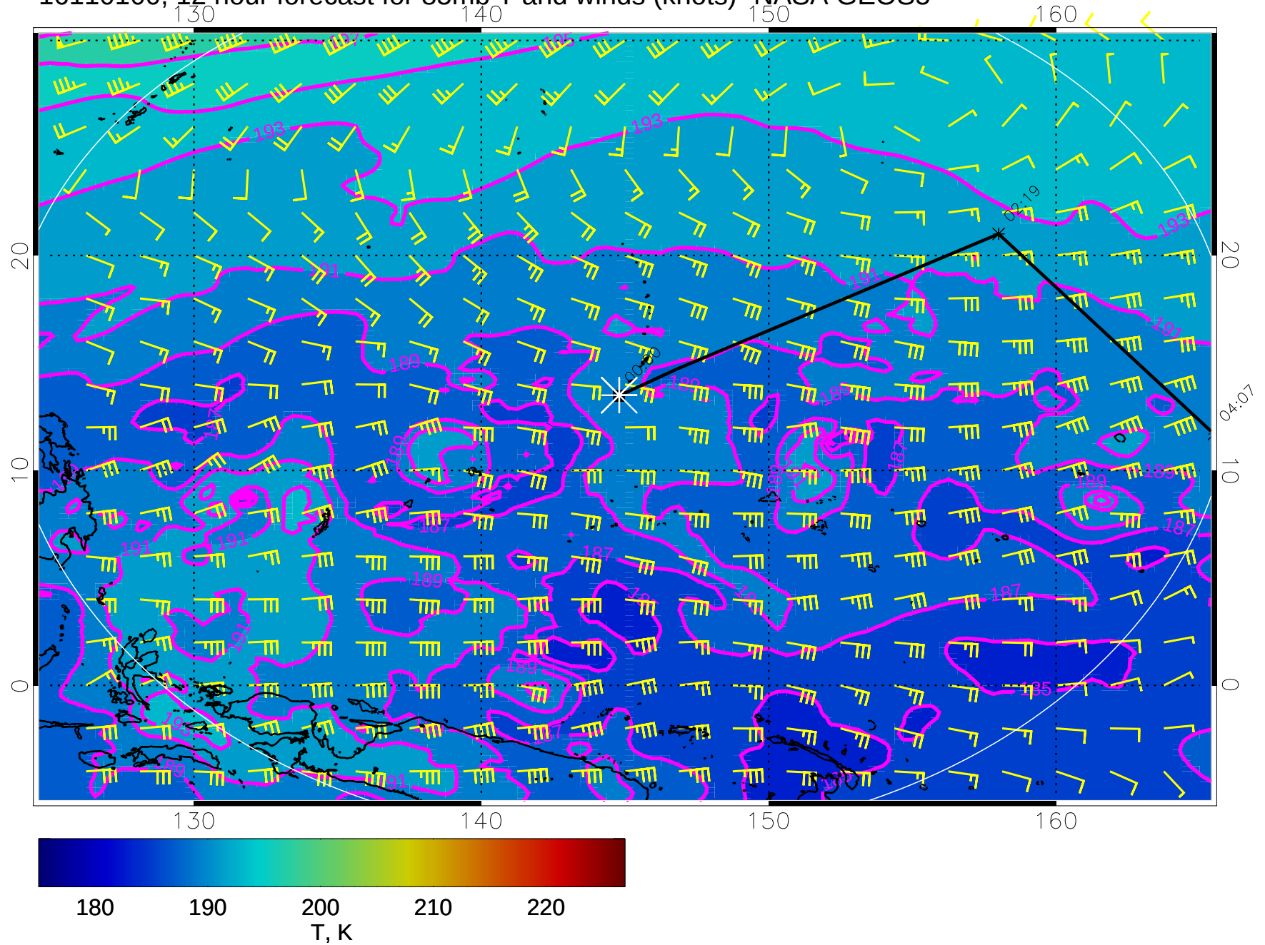
16110100, 12 hour forecast for 85mb T and winds (knots)- NASA GEOS5
