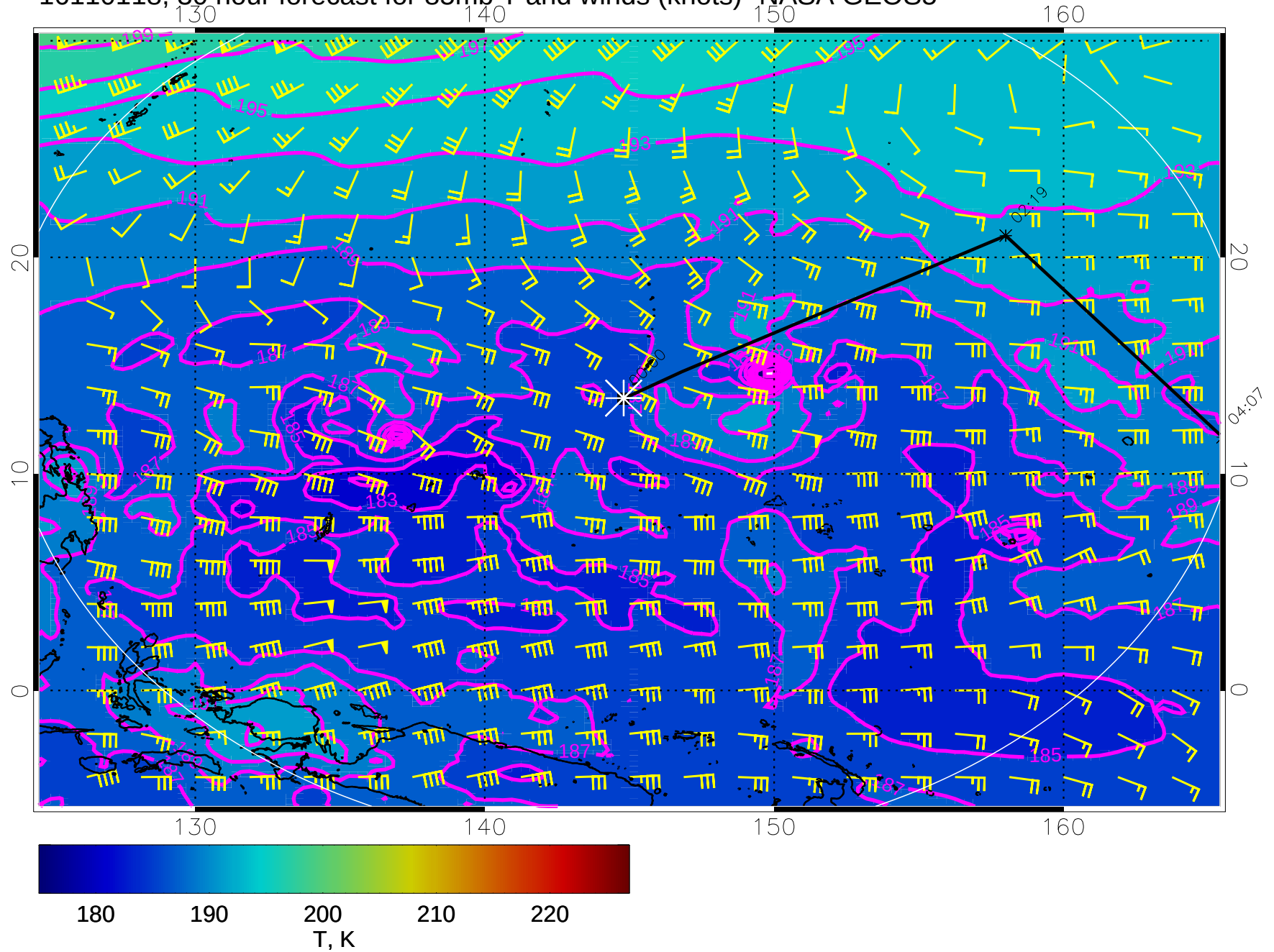
16110118, 30 hour forecast for 85mb T and winds (knots)- NASA GEOS5
