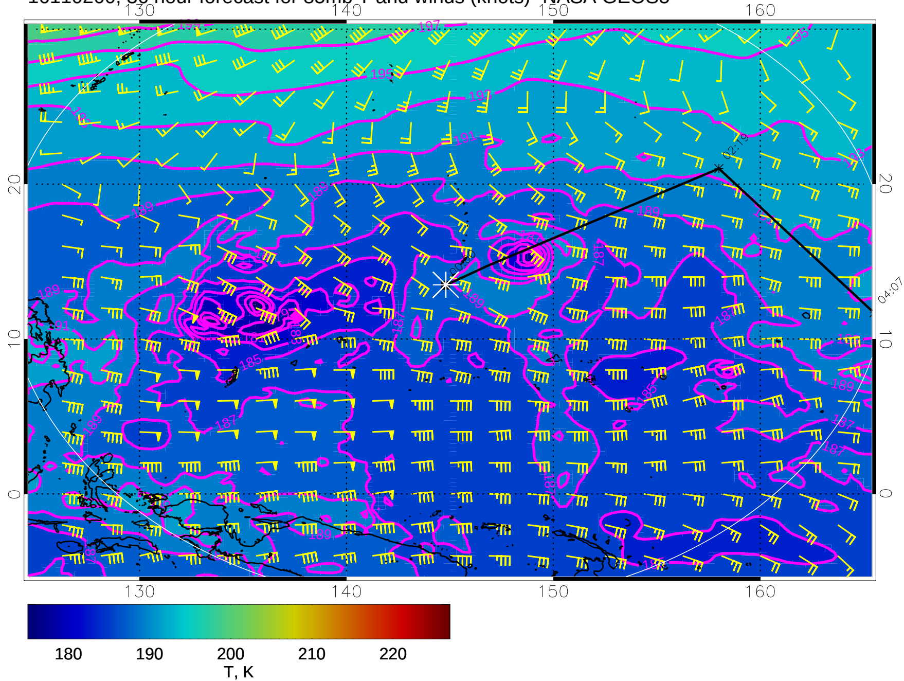
16110200, 36 hour forecast for 85mb T and winds (knots)- NASA GEOS5
