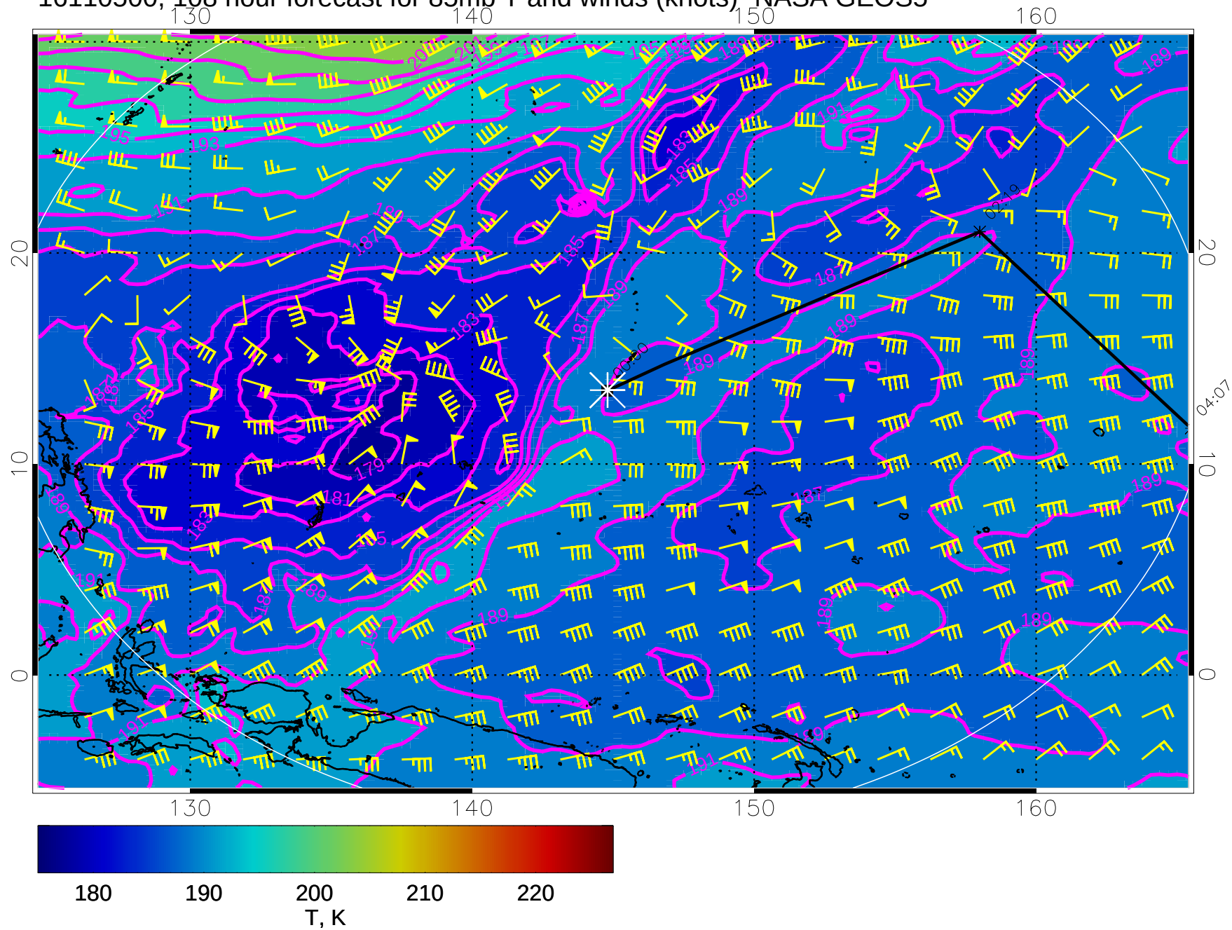
16110500, 108 hour forecast for 85mb T and winds (knots)- NASA GEOS5
