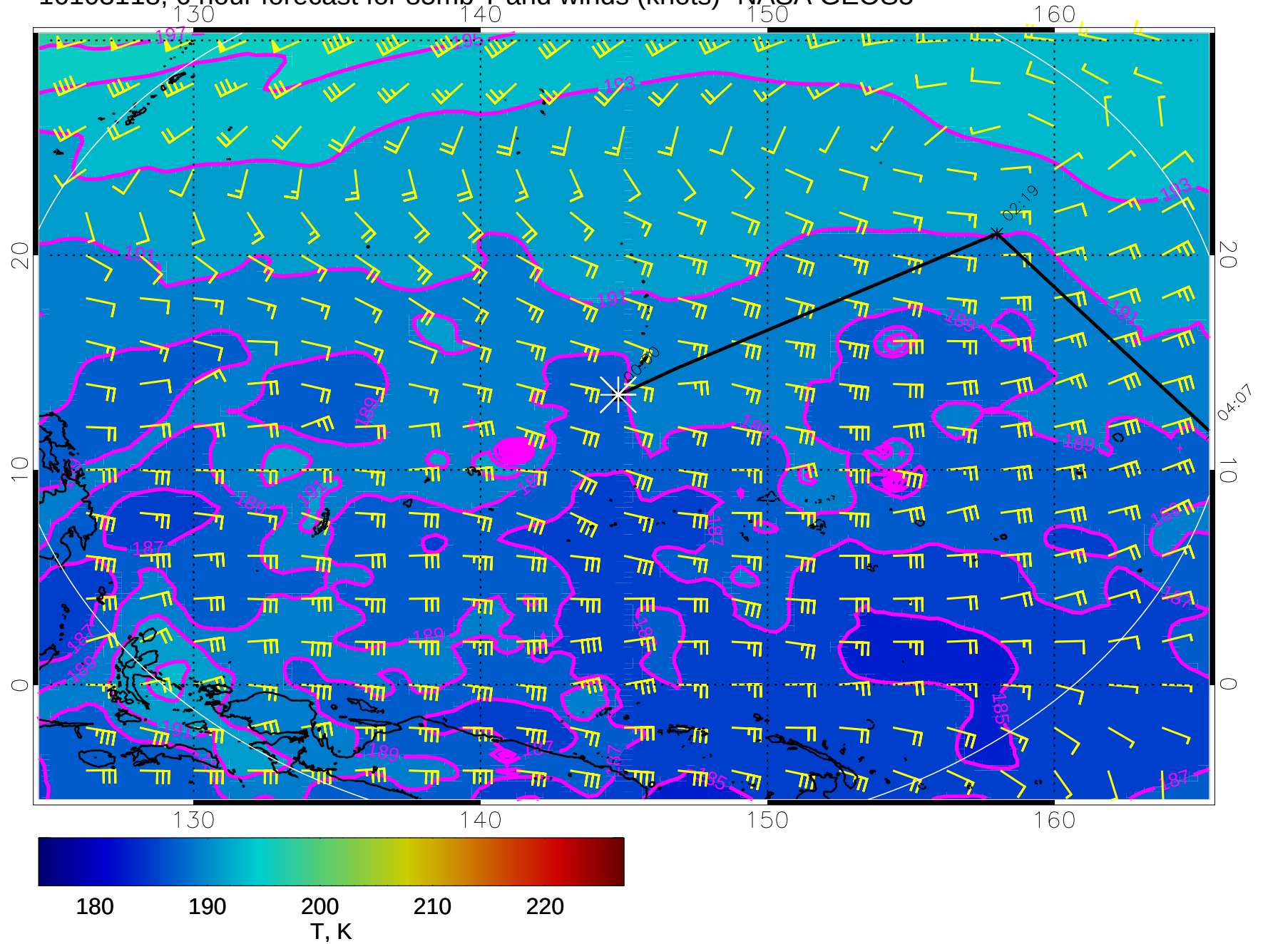
16103118, 6 hour forecast for 85mb T and winds (knots)- NASA GEOS5
