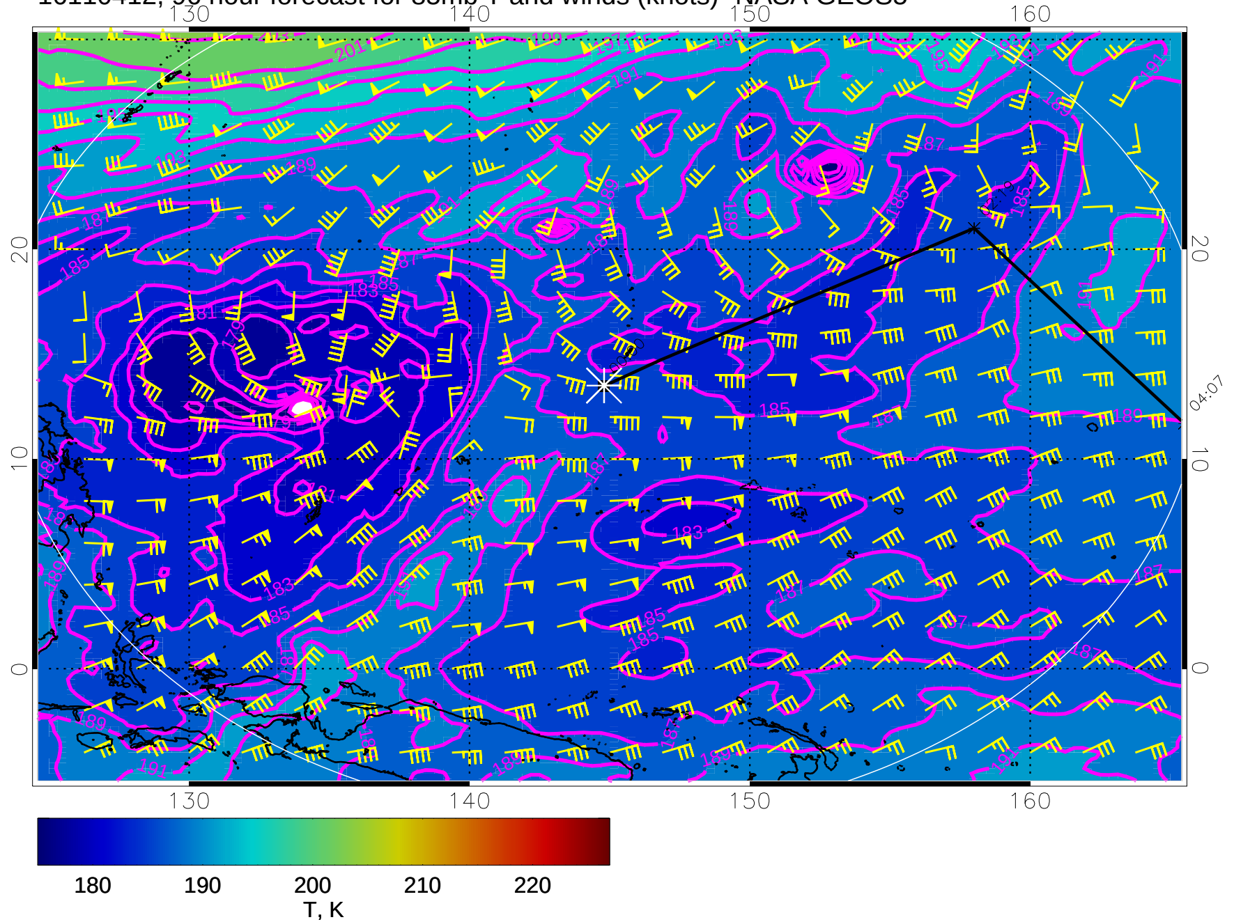
16110412, 96 hour forecast for 85mb T and winds (knots)- NASA GEOS5
