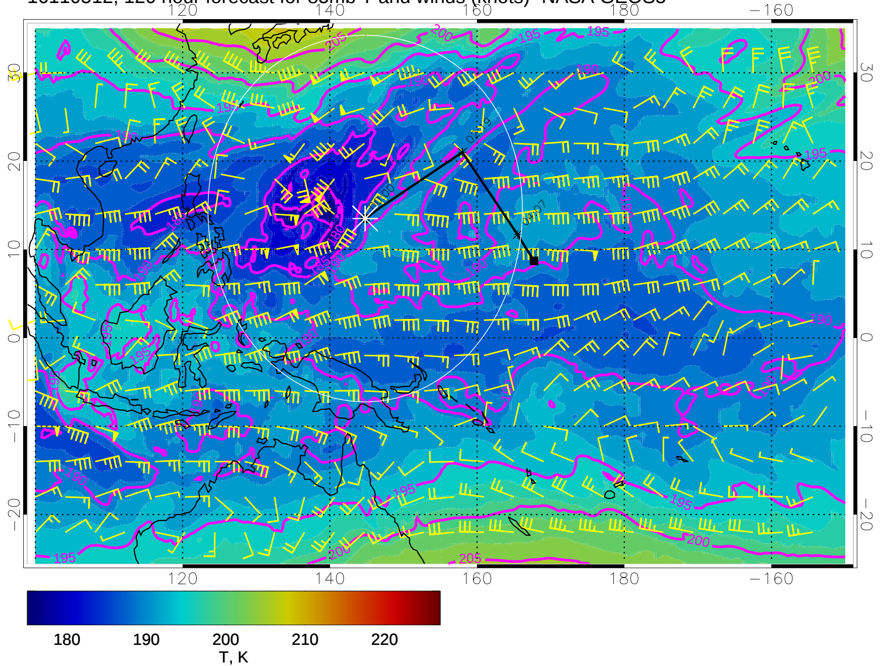
16110512, 120 hour forecast for 85mb T and winds (knots)- NASA GEOS5
