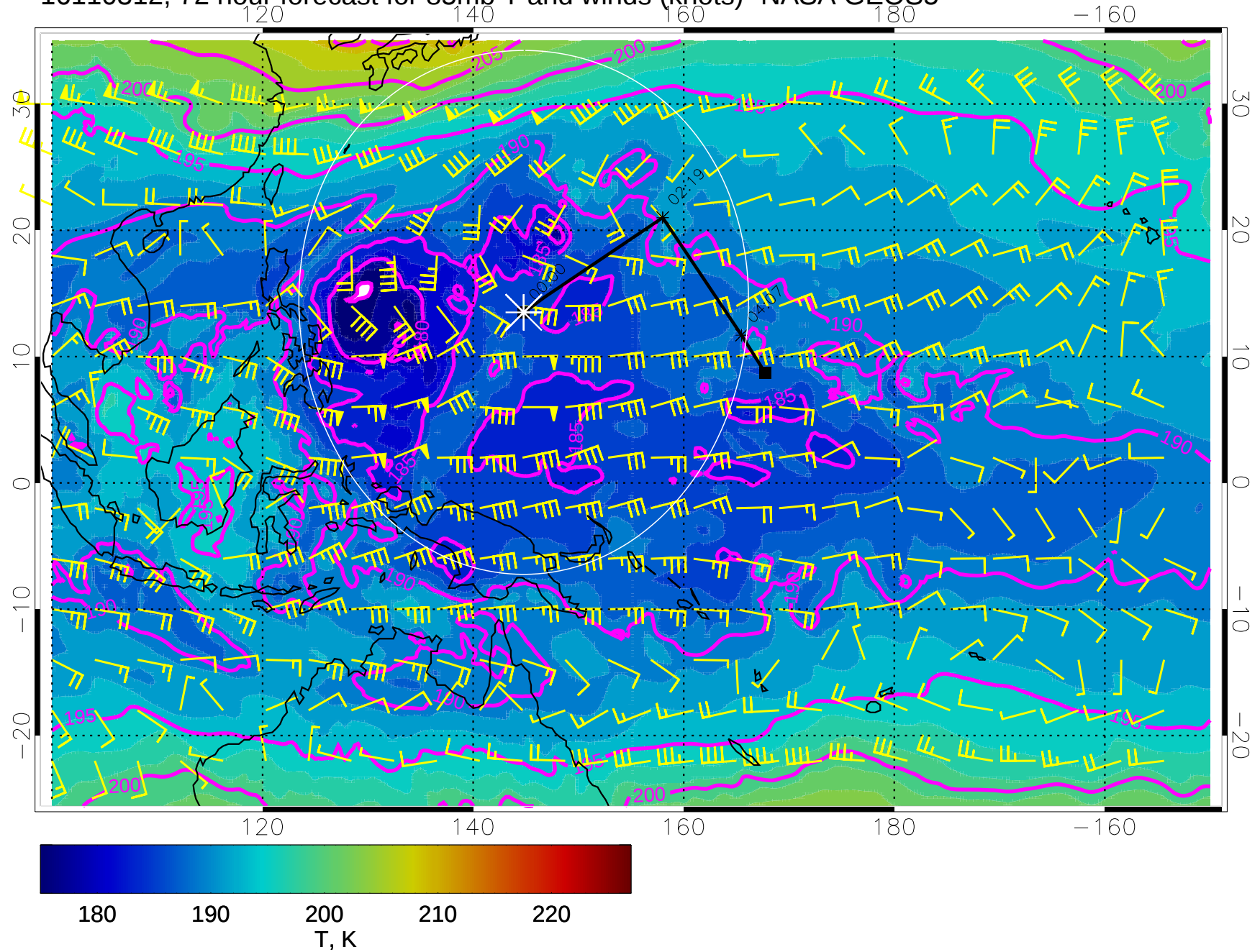
16110312, 72 hour forecast for 85mb T and winds (knots)- NASA GEOS5
