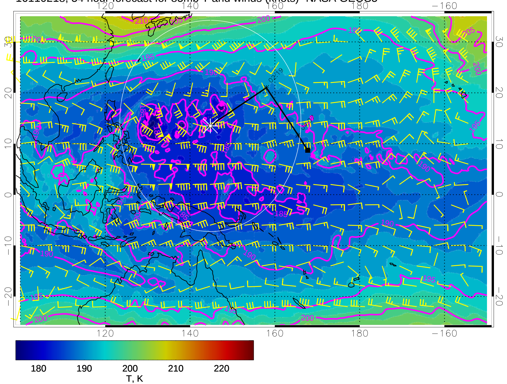
16110218, 54 hour forecast for 85mb T and winds (knots)- NASA GEOS5
