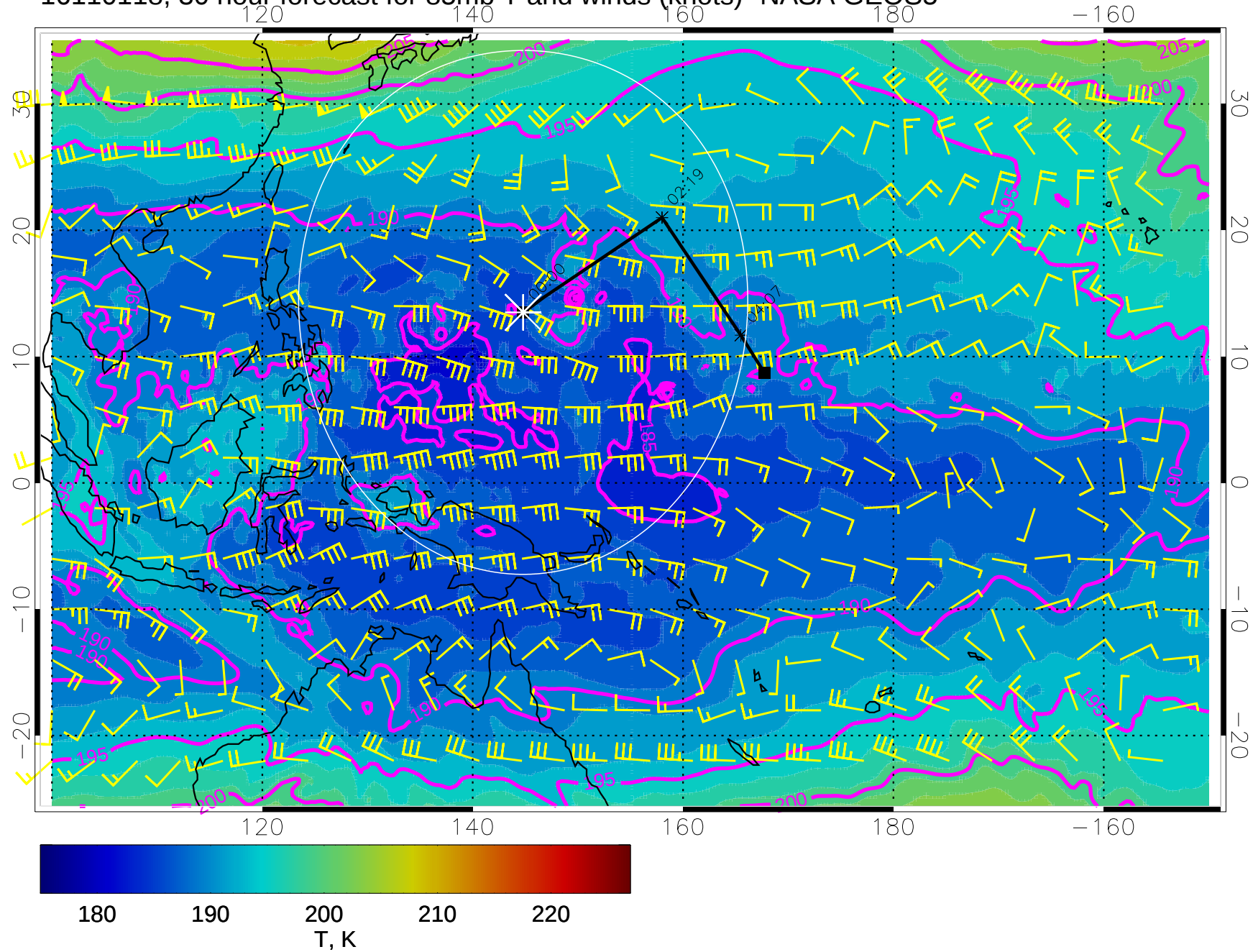
16110118, 30 hour forecast for 85mb T and winds (knots)- NASA GEOS5
