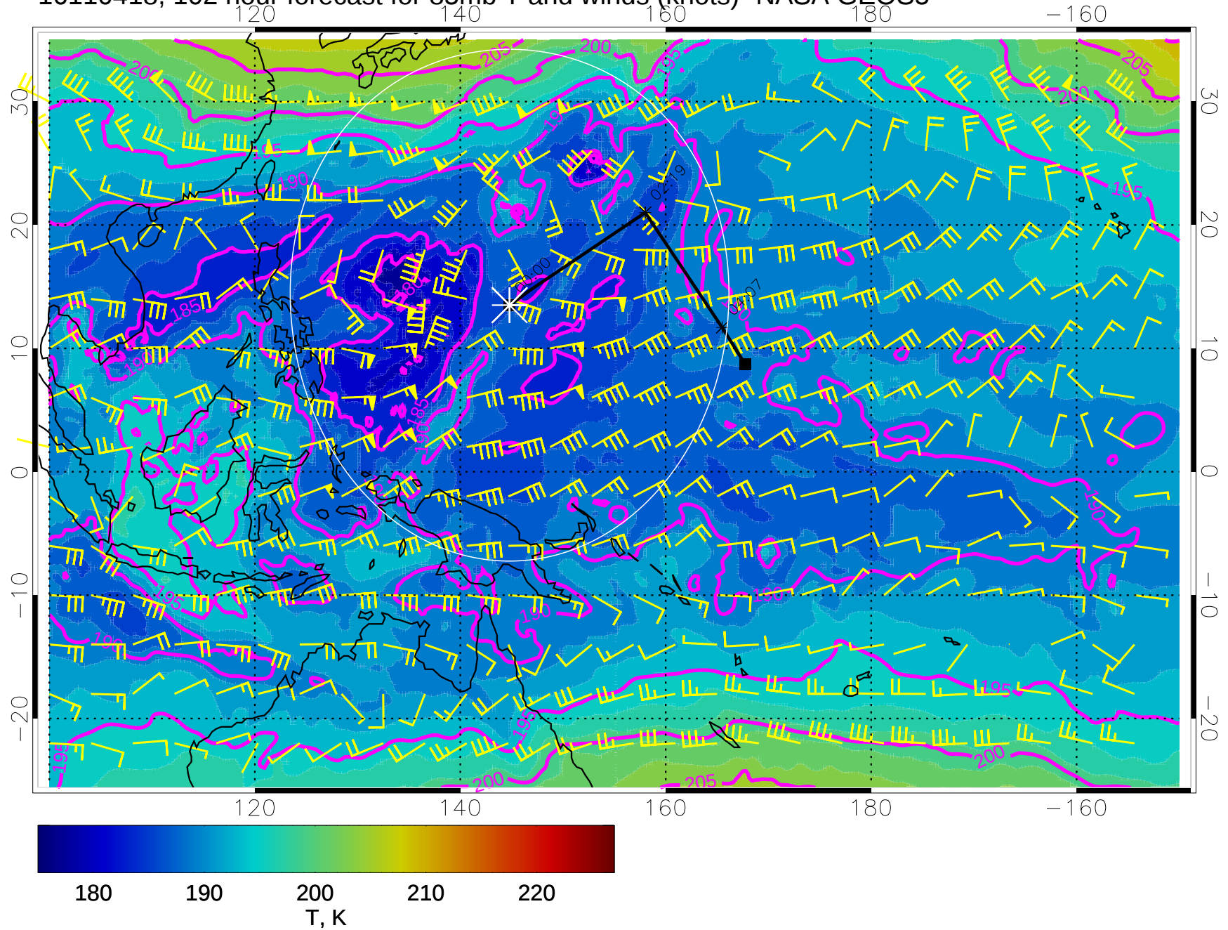
16110418, 102 hour forecast for 85mb T and winds (knots)- NASA GEOS5
