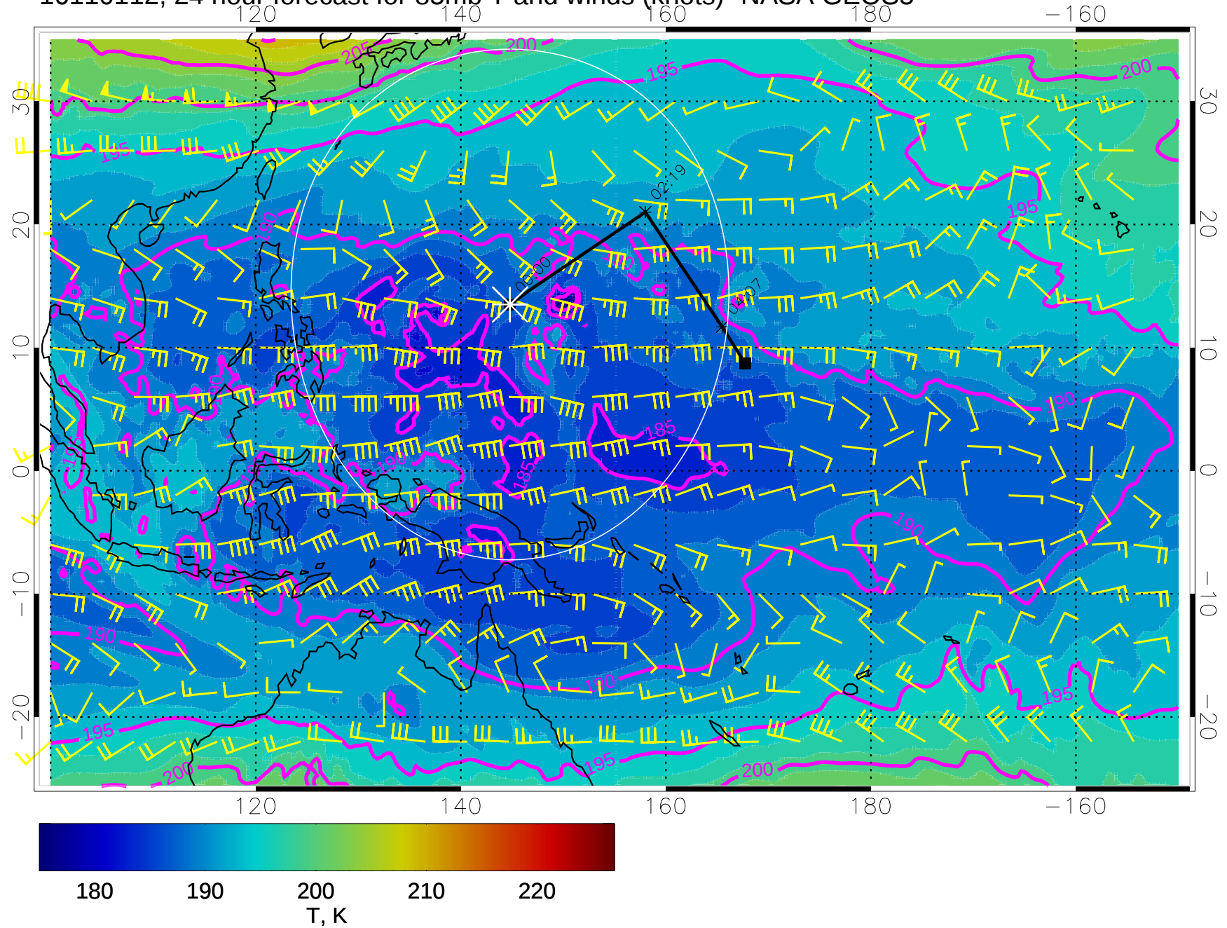
16110112, 24 hour forecast for 85mb T and winds (knots)- NASA GEOS5
