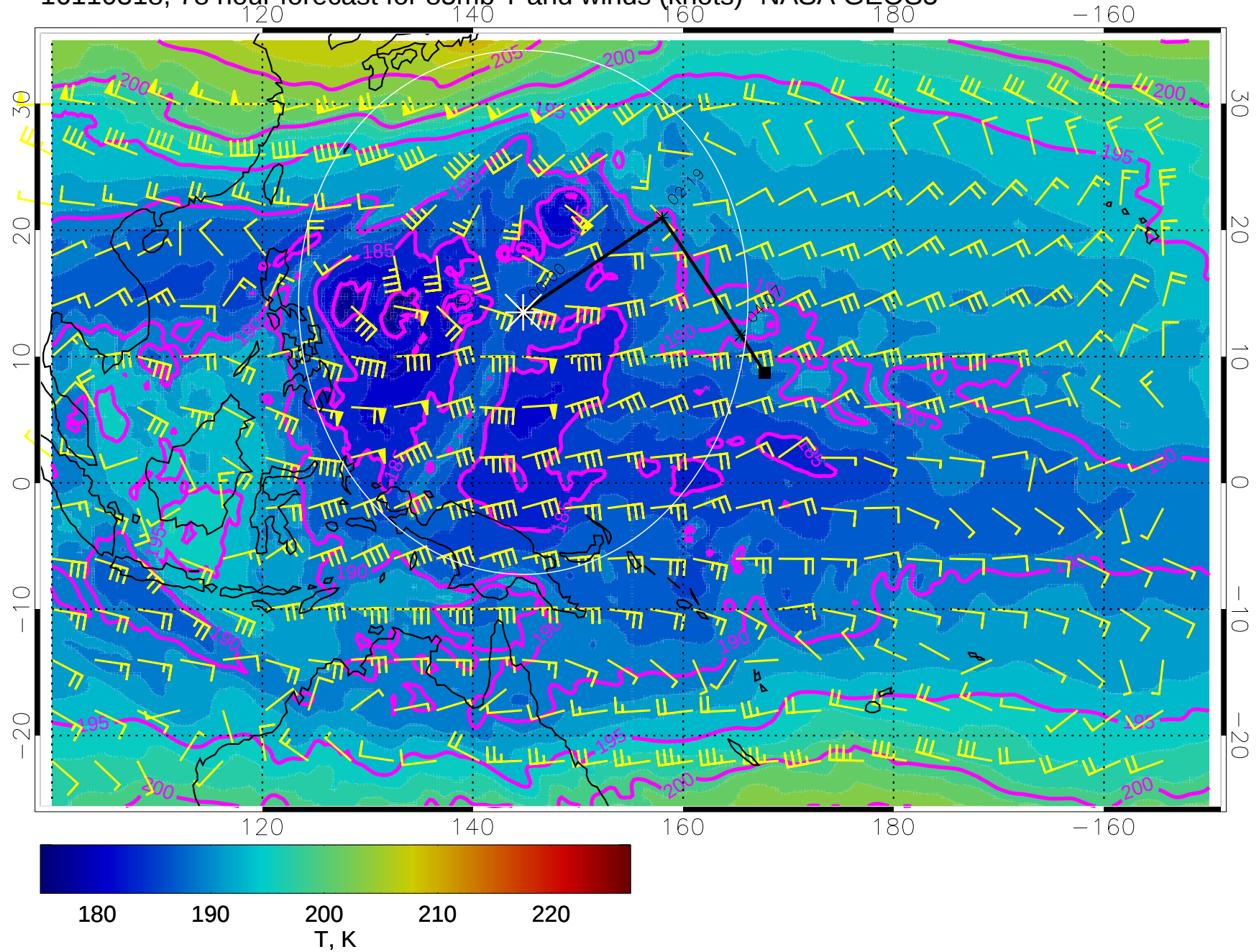
16110318, 78 hour forecast for 85mb T and winds (knots)- NASA GEOS5
