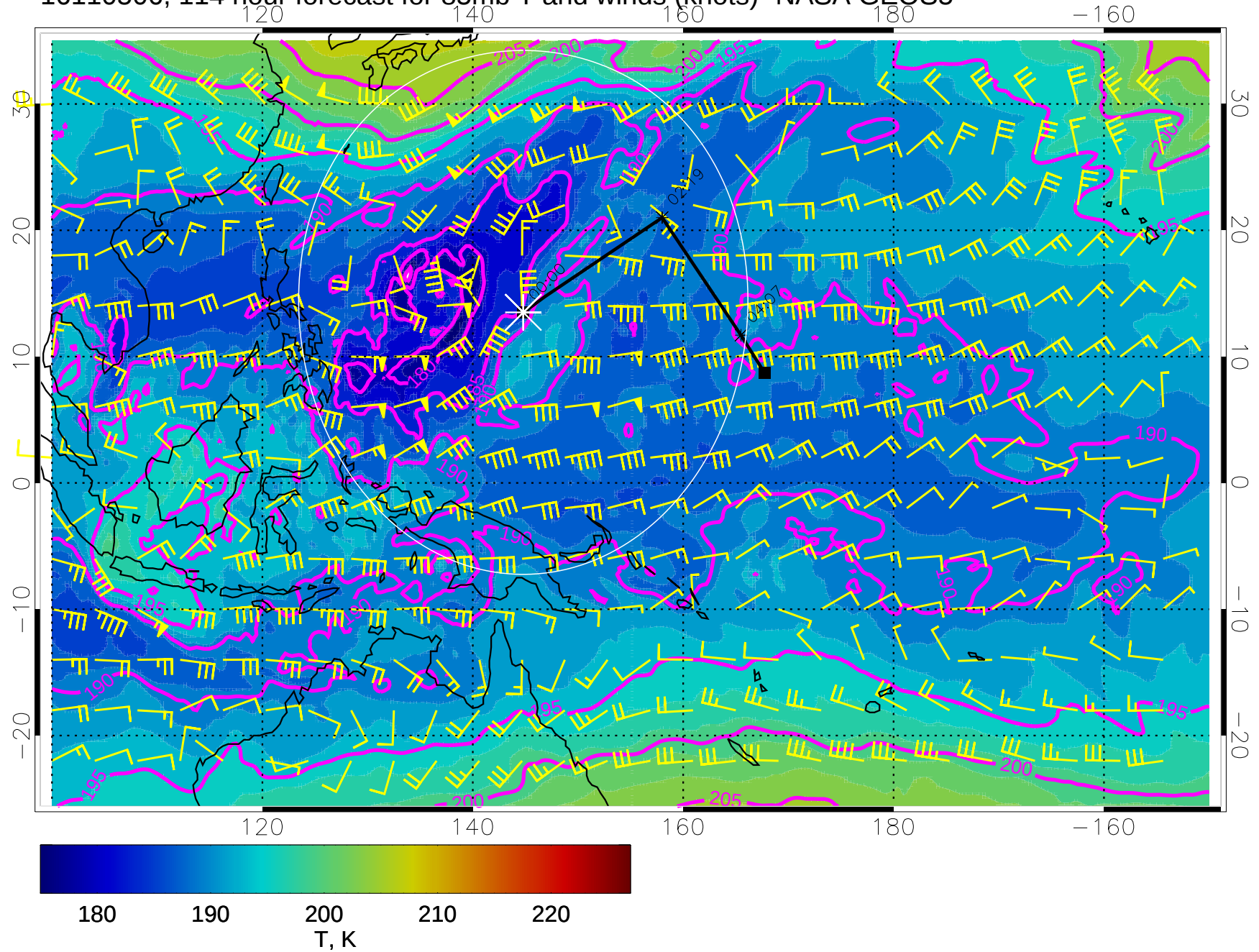
16110506, 114 hour forecast for 85mb T and winds (knots)- NASA GEOS5
