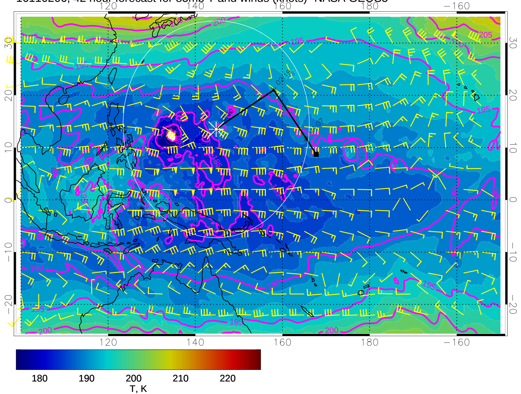
16110206, 42 hour forecast for 85mb T and winds (knots)- NASA GEOS5
