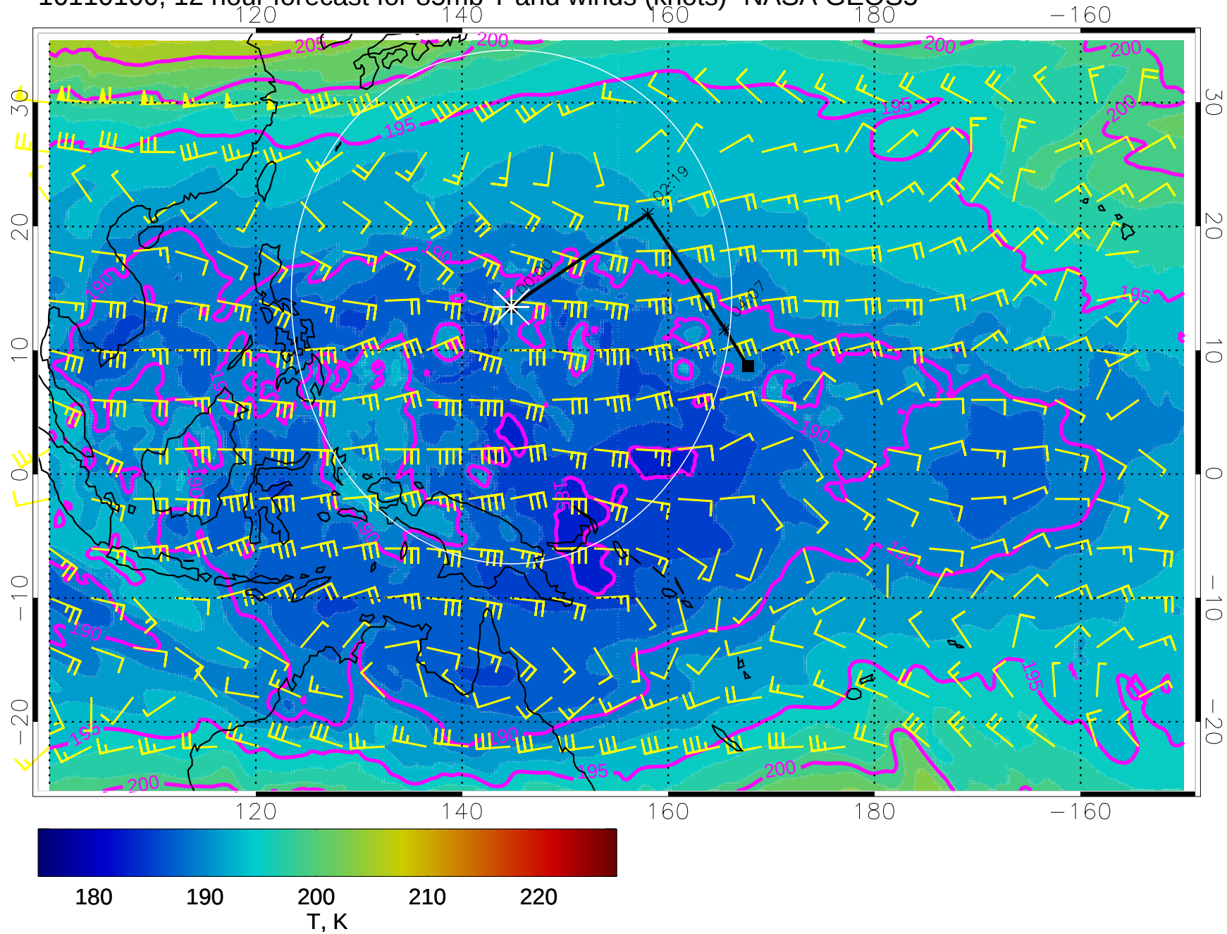
16110100, 12 hour forecast for 85mb T and winds (knots)- NASA GEOS5
