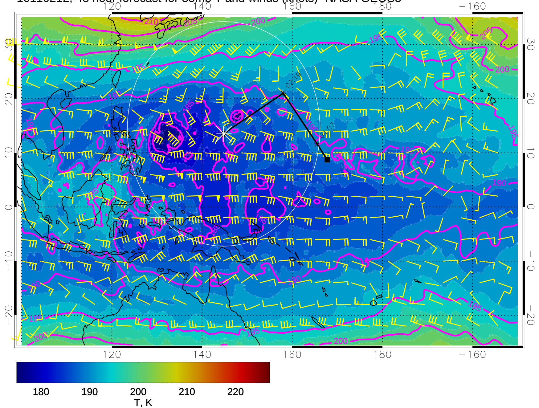
16110212, 48 hour forecast for 85mb T and winds (knots)- NASA GEOS5
