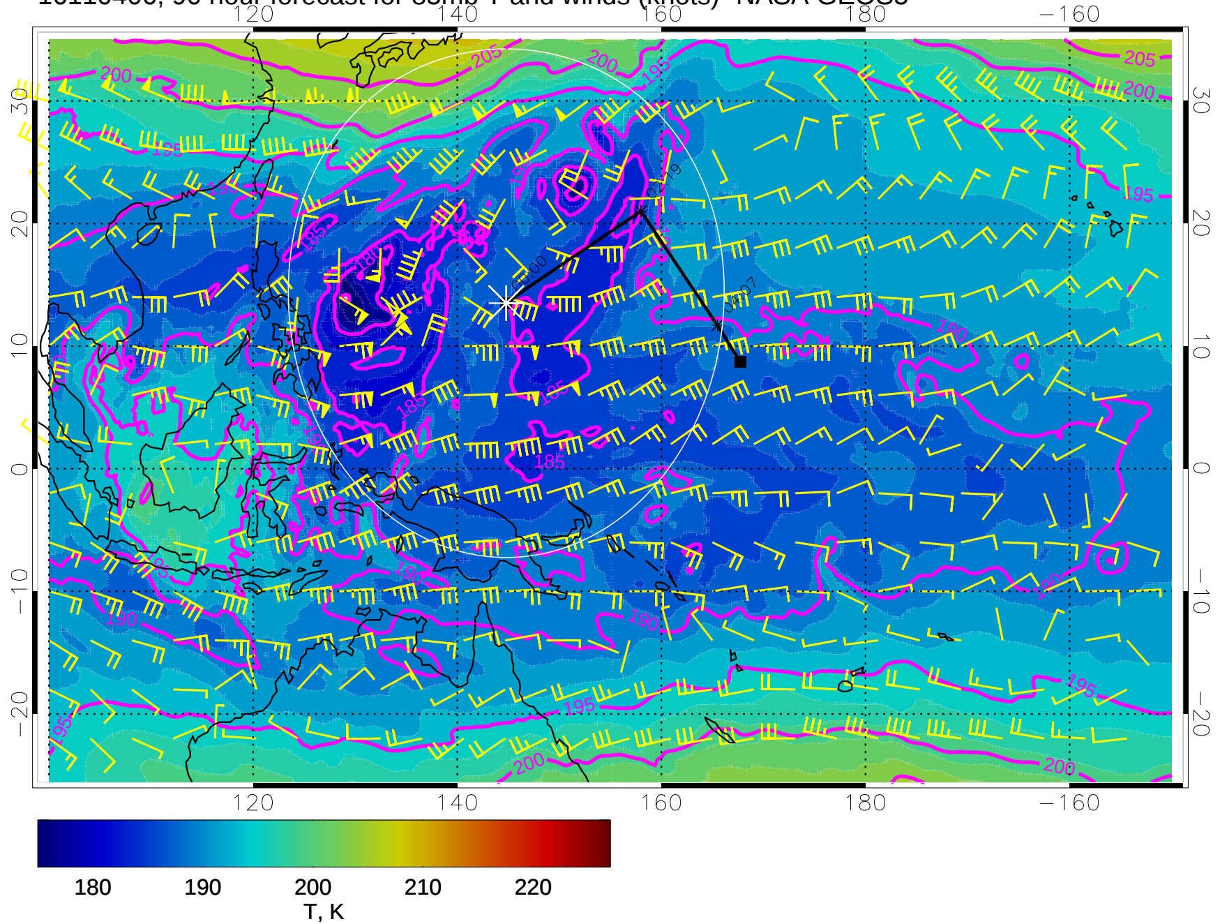
16110406, 90 hour forecast for 85mb T and winds (knots)- NASA GEOS5
