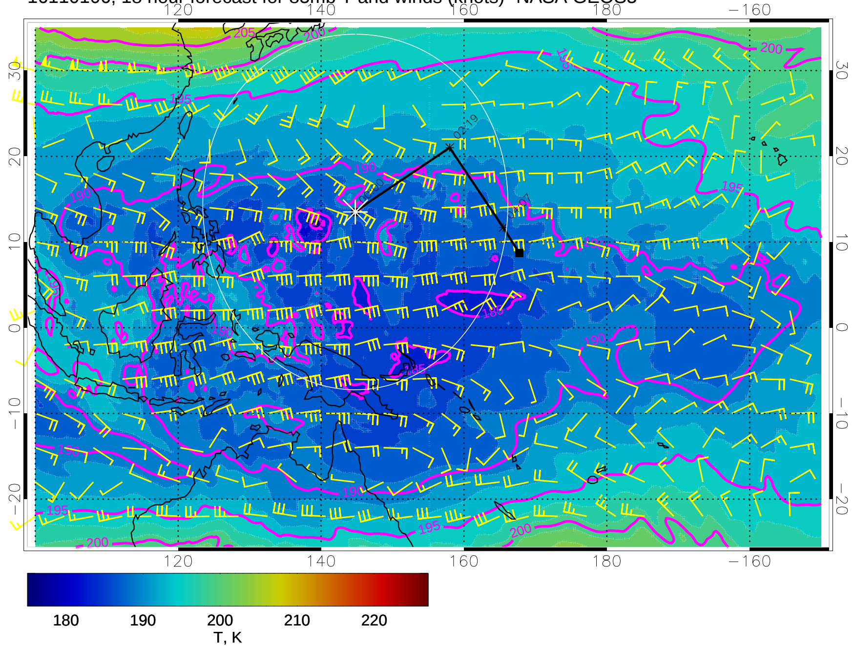
16110106, 18 hour forecast for 85mb T and winds (knots)- NASA GEOS5
