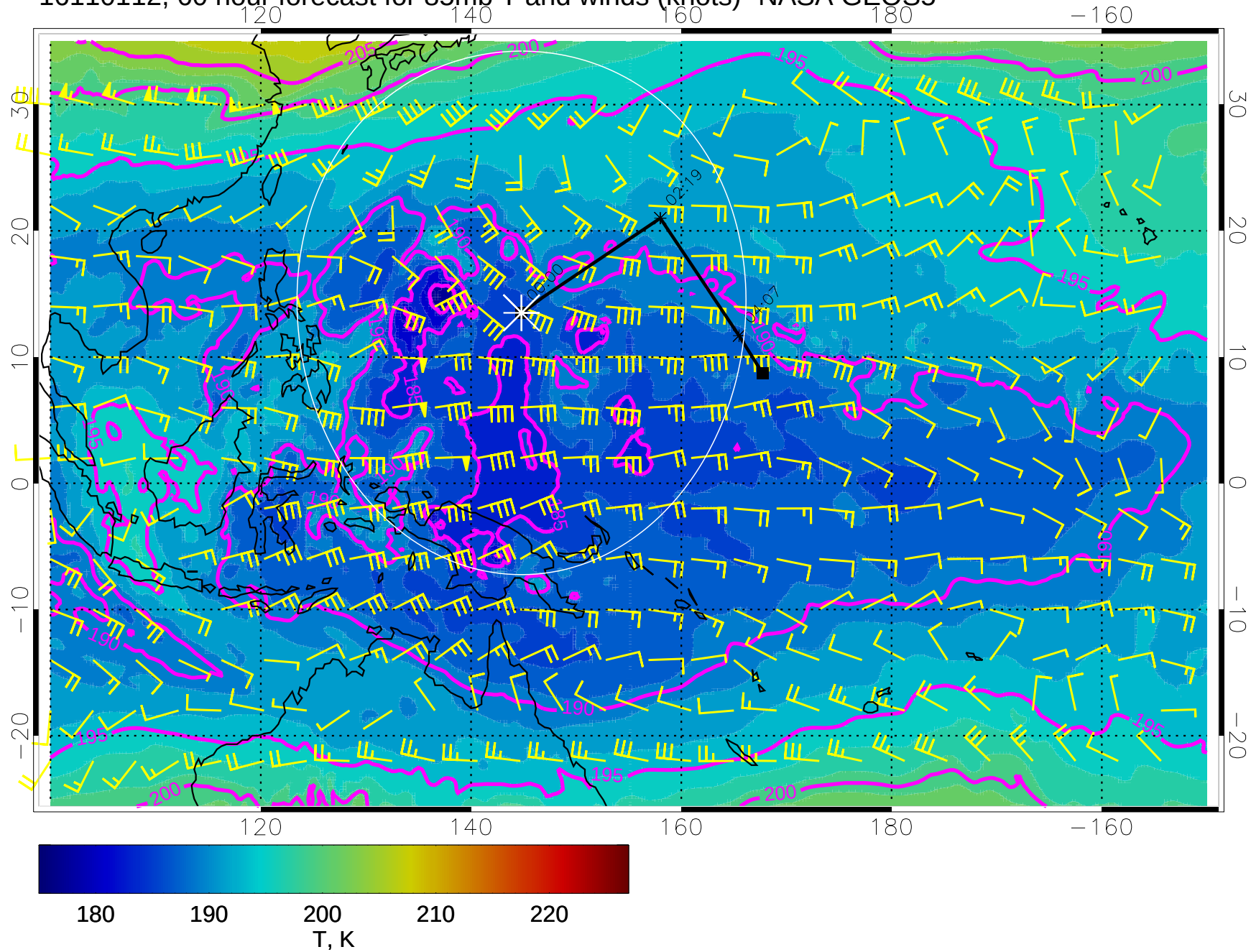
16110112, 60 hour forecast for 85mb T and winds (knots)- NASA GEOS5
