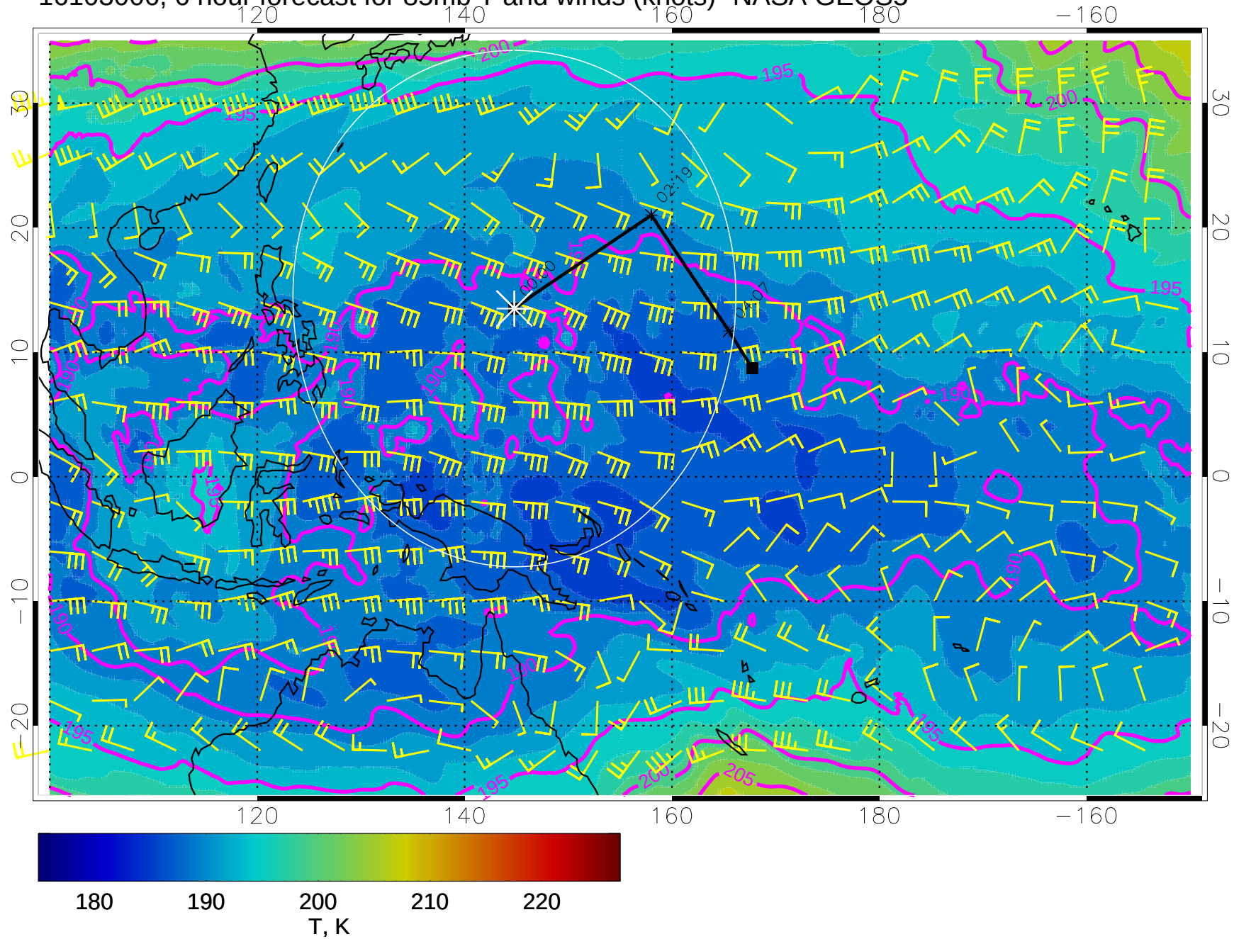
16103006, 6 hour forecast for 85mb T and winds (knots)- NASA GEOS5
