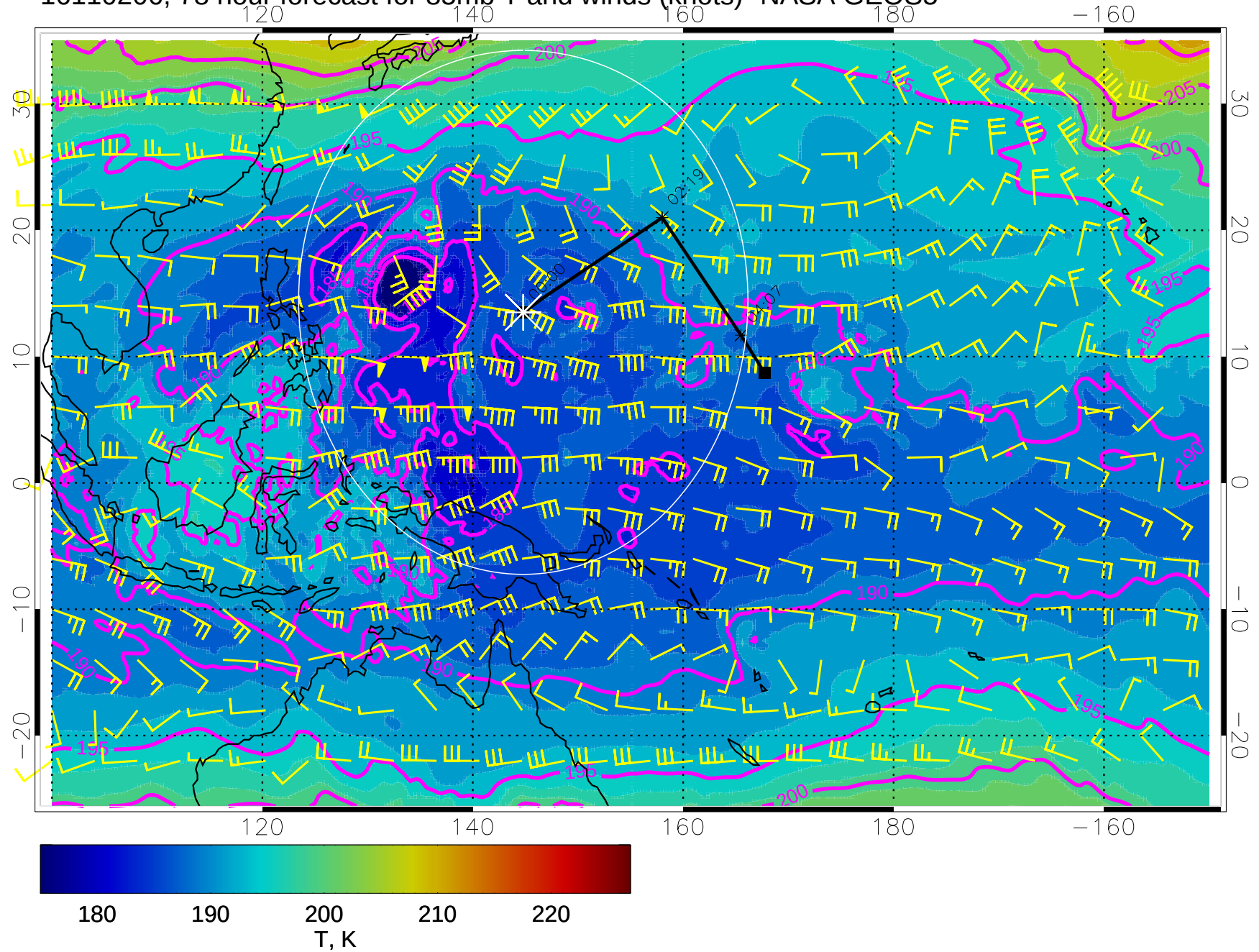
16110206, 78 hour forecast for 85mb T and winds (knots)- NASA GEOS5
