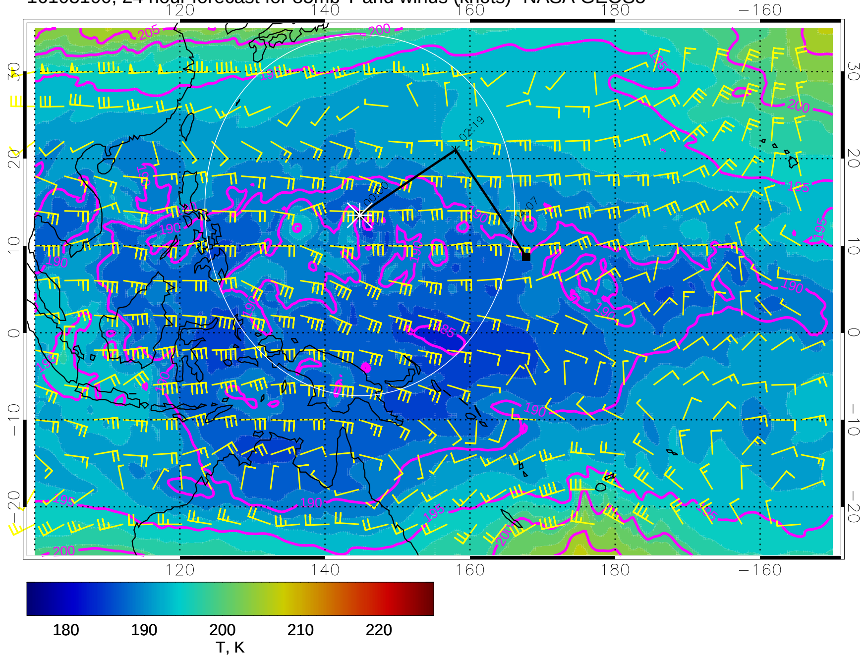
16103100, 24 hour forecast for 85mb T and winds (knots)- NASA GEOS5
