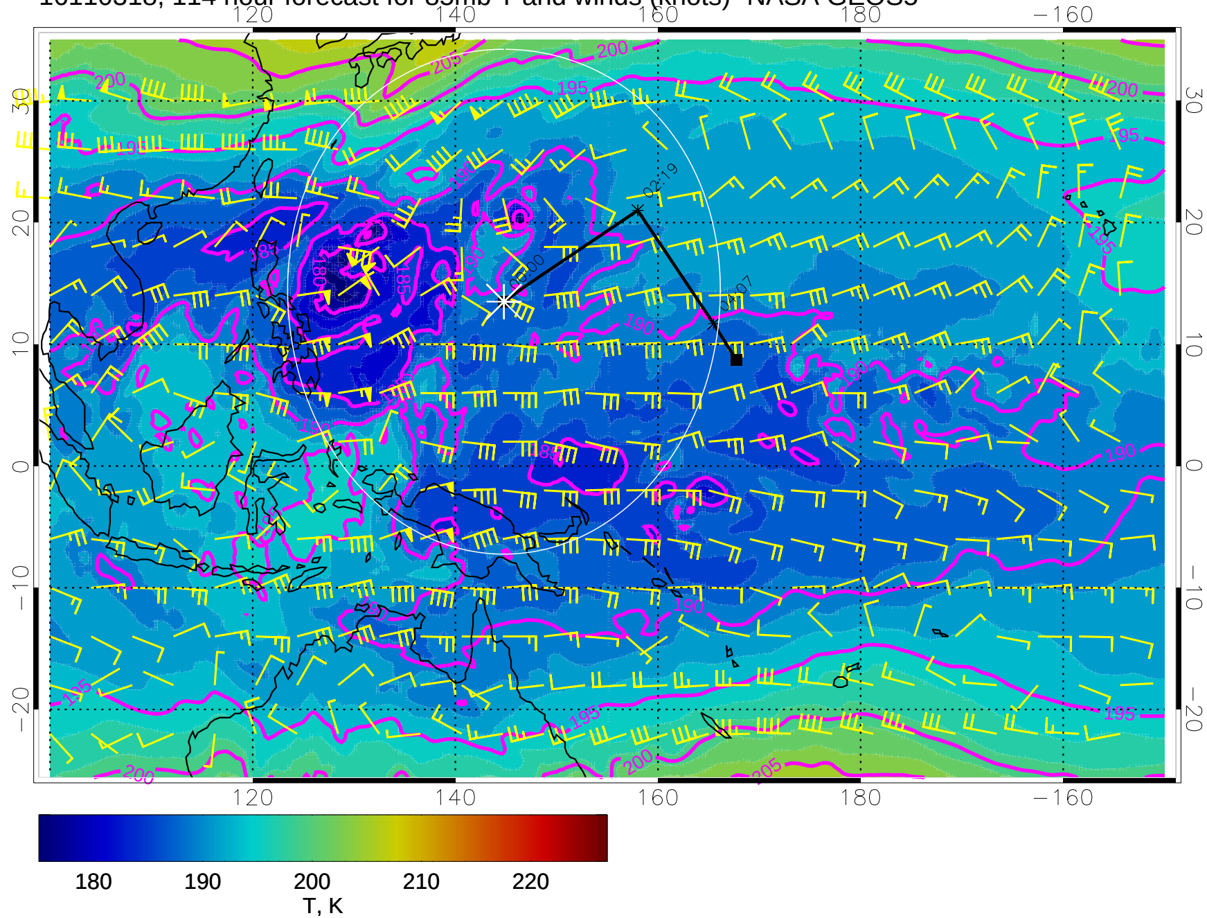
16110318, 114 hour forecast for 85mb T and winds (knots)- NASA GEOS5
